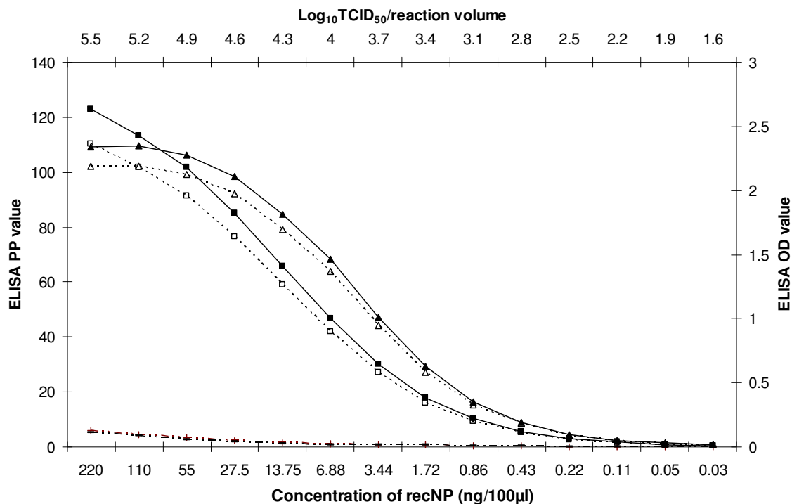
Figure 3.2. Dose response curves of recNP (PP ■, OD □), RVFV Ar20368 RSA 81 (PP ▲, OD Δ), and control antigen (PP +, OD -).
