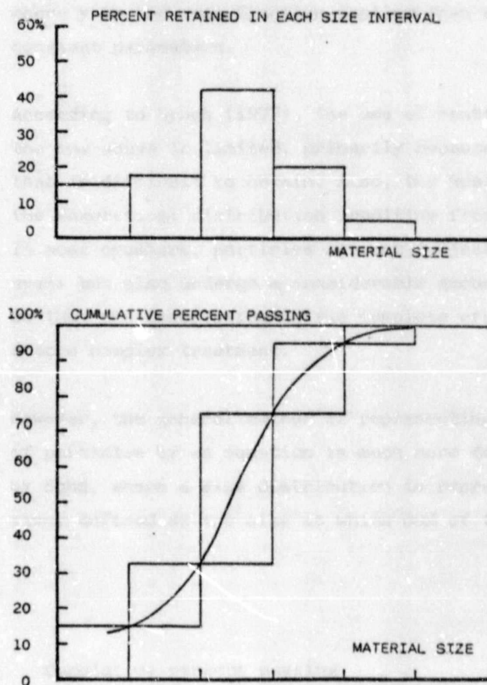
Figure 2.1 Representing the size distribution of an aggregate sample
