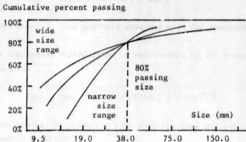
Figure 2.2 Example of a single size representing several size-distributions
