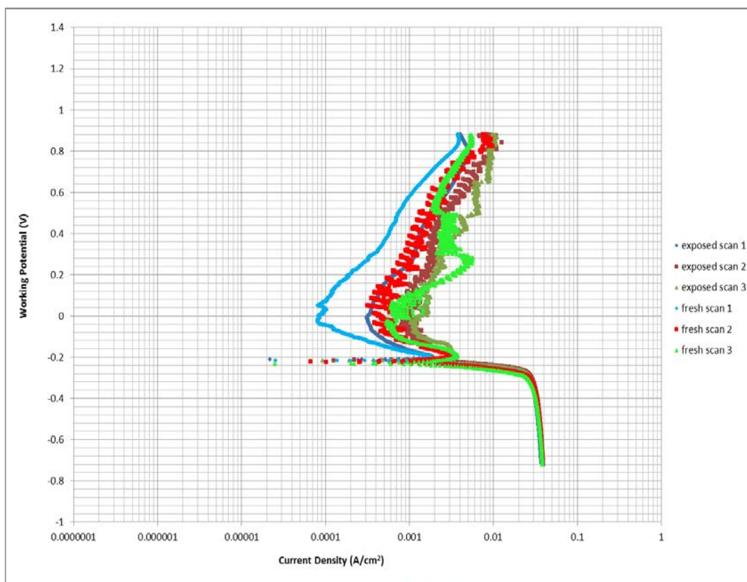
Figure 172: Log i vs E graphs for the 2.44 wt% Ru sample in 1 M \text{H}_2\text{SO}_4 + 1% NaCl at 45°C
