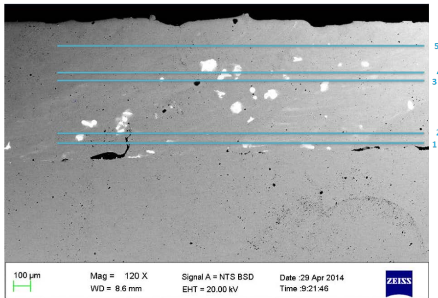
Figure 145: Cross sectional view of the 2.92 wt% Ru sample indicating different surface exposure possibilities
