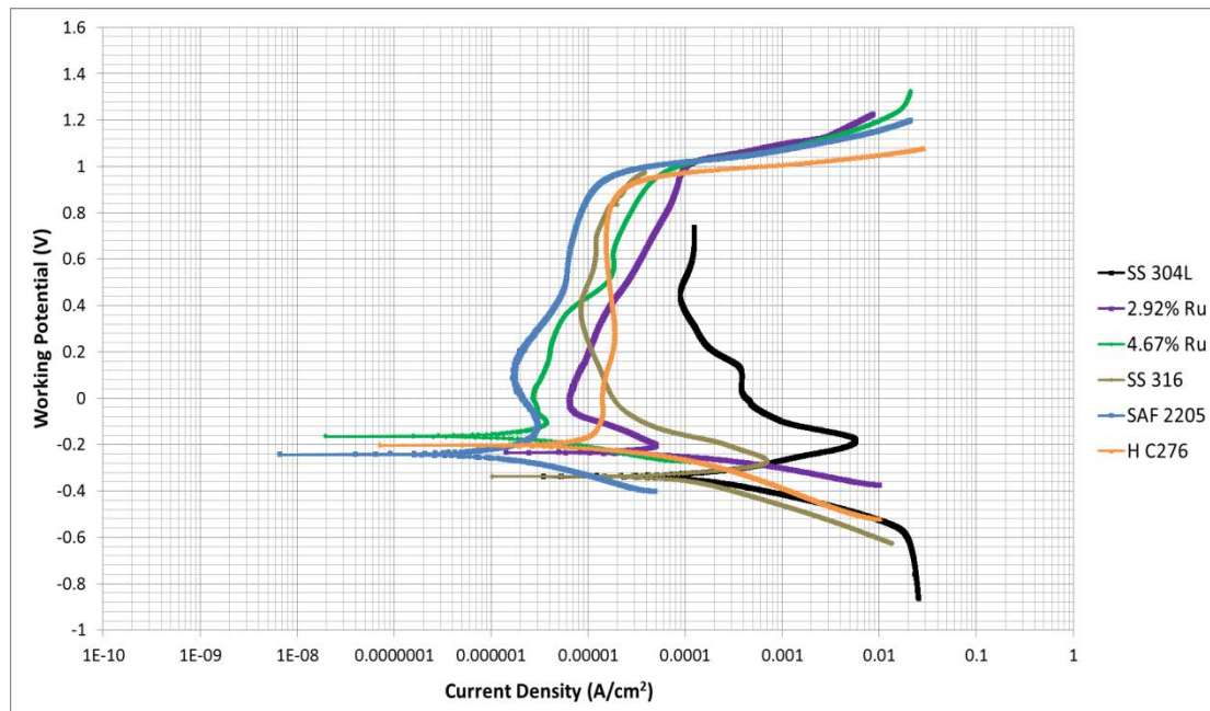
Figure 78: Log I vs E graphs from the exposed surface scan comparing ruthenium samples to other steels in 1 M \text{H}_2\text{SO}_4 + 1\% \text{NaCl} at 25^\circ\text{C}
