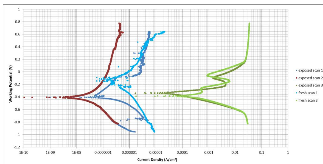
Figure 178: Log i vs E graphs for the 2.44 wt% Ru sample in 1 M HCl at 25°C
