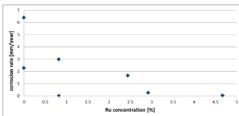
Figure 71: Corrosion rate comparison at various ruthenium compositions from the exposed surface scan in 1 M \text{H}_2\text{SO}_4 + 1% NaCl at 25°C
