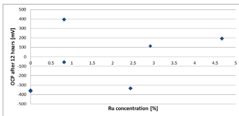
Figure 73: OCP comparison at various ruthenium compositions from the exposed surface scan in 1 M H 2 SO 4 + 1% NaCl at 25°C
