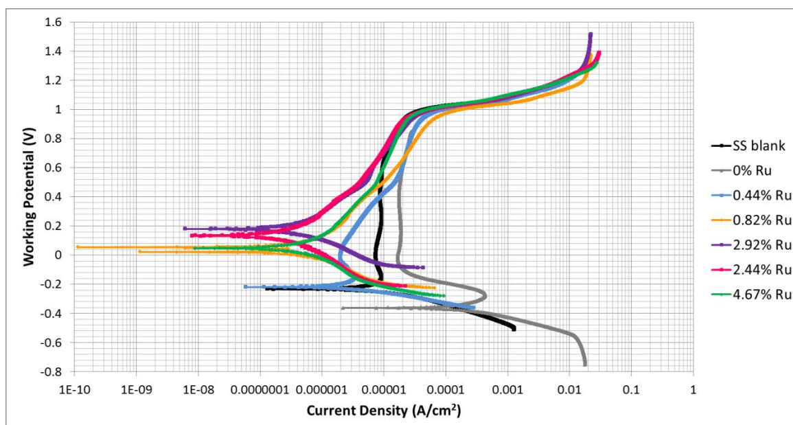
Figure 42: Log i vs E graphs from the exposed surface scan comparing all samples in 1 M H_2SO_4 at 25°C
