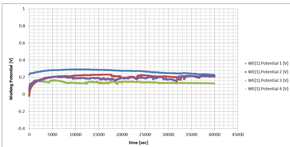
Figure 64: E vs time graphs for the 4.67 wt% Ru sample in 1 M H_2SO_4 + 1% NaCl at 25°C
