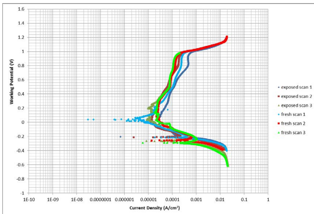
Figure 164: Log i vs E graphs for the 2.92 wt% Ru sample in 1 M H_2SO_4 at 45^\circ C
