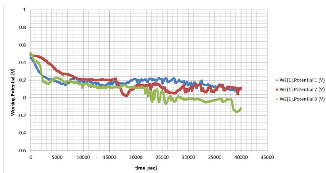
Figure 165: E vs time graphs for the 2.92 wt% Ru sample in 1 M H_2SO_4 at 45^\circ C
