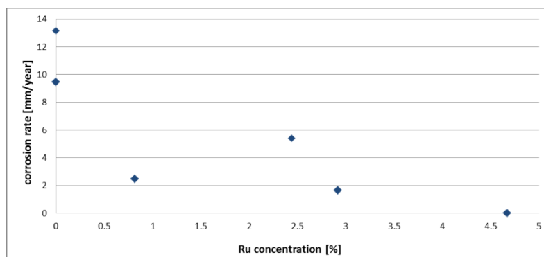
Figure 92: Corrosion rate comparison at various ruthenium compositions from the exposed surface scan in 1 M \text{H}_2\text{SO}_4 at 45^\circ\text{C}
