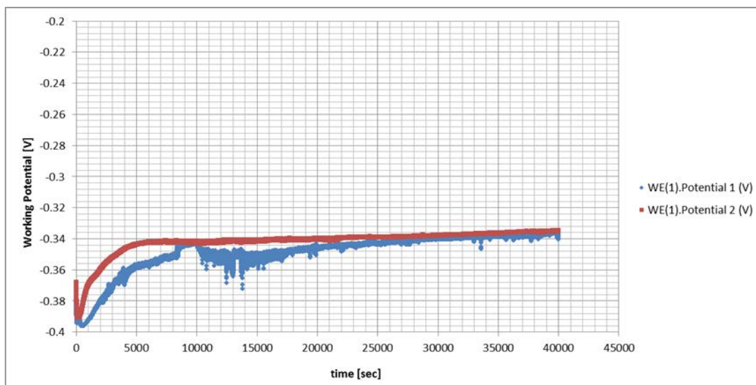
Figure 161: E vs time graphs for the 2.44 wt% Ru sample in 1 M \text{H}_2\text{SO}_4 + 1% NaCl at 25°C
