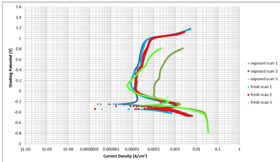
Figure 61: Log i vs E graphs for the 0.82 wt% Ru sample #2 in 1 M \text{H}_2\text{SO}_4 + 1% NaCl at 25°C
