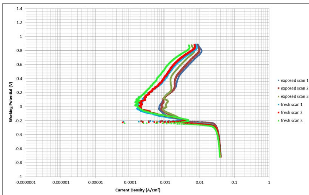
Figure 101: Log i vs E graphs for the 0.82 wt% Ru sample in 1 M \text{H}_2\text{SO}_4 + 1% NaCl at 45°C
