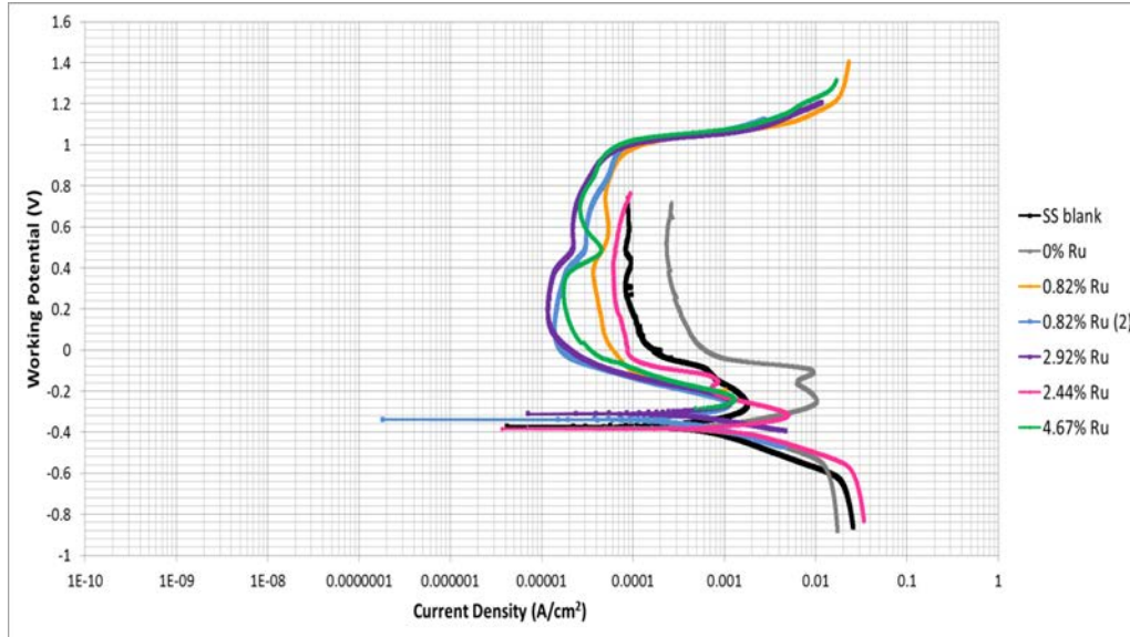
Figure 66: Log i vs E graphs from the fresh surface scan comparing all samples in 1 M \text{H}_2\text{SO}_4 + 1 % NaCl at 25°C
