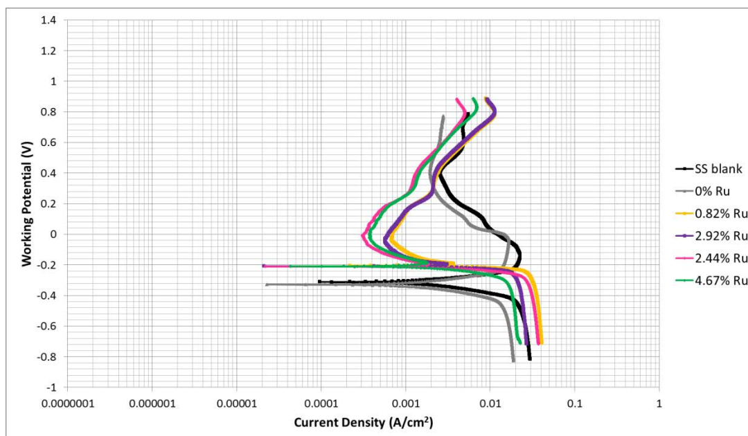
Figure 105: Log i vs E graphs from the exposed surface scan comparing all samples in 1 M \text{H}_2\text{SO}_4 + 1% NaCl at 45°C
