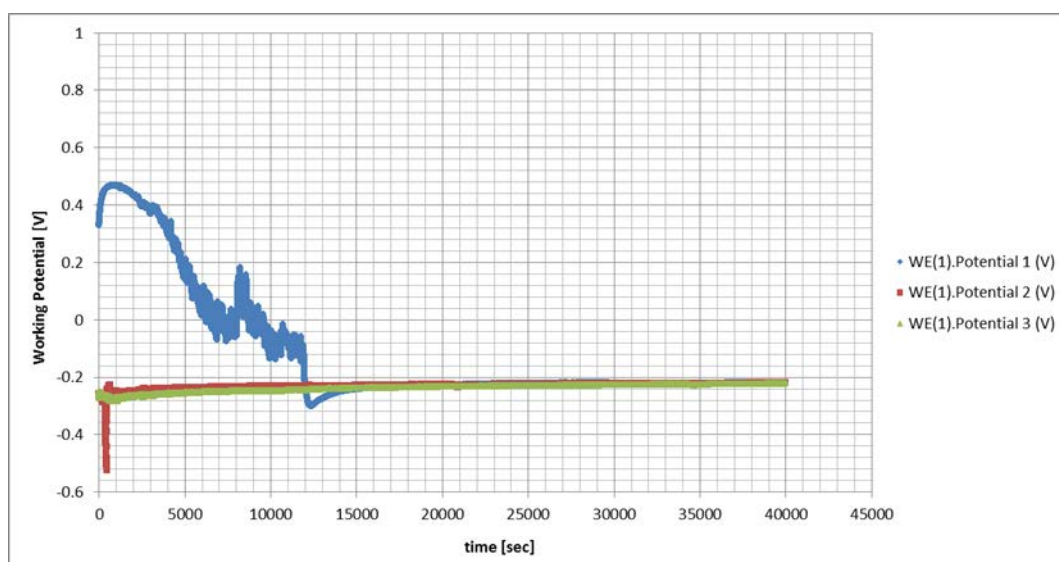
Figure 173: E vs time graphs for the 2.44 wt% Ru sample in 1 M \text{H}_2\text{SO}_4 + 1% NaCl at 45°C
