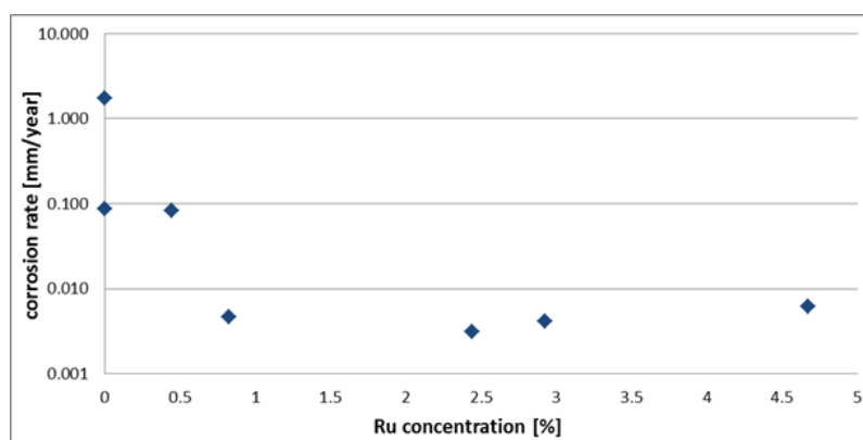
Figure 48: Corrosion rate at various ruthenium compositions for the exposed surface scan in 1 M \text{H}_2\text{SO}_4 at 25°C
