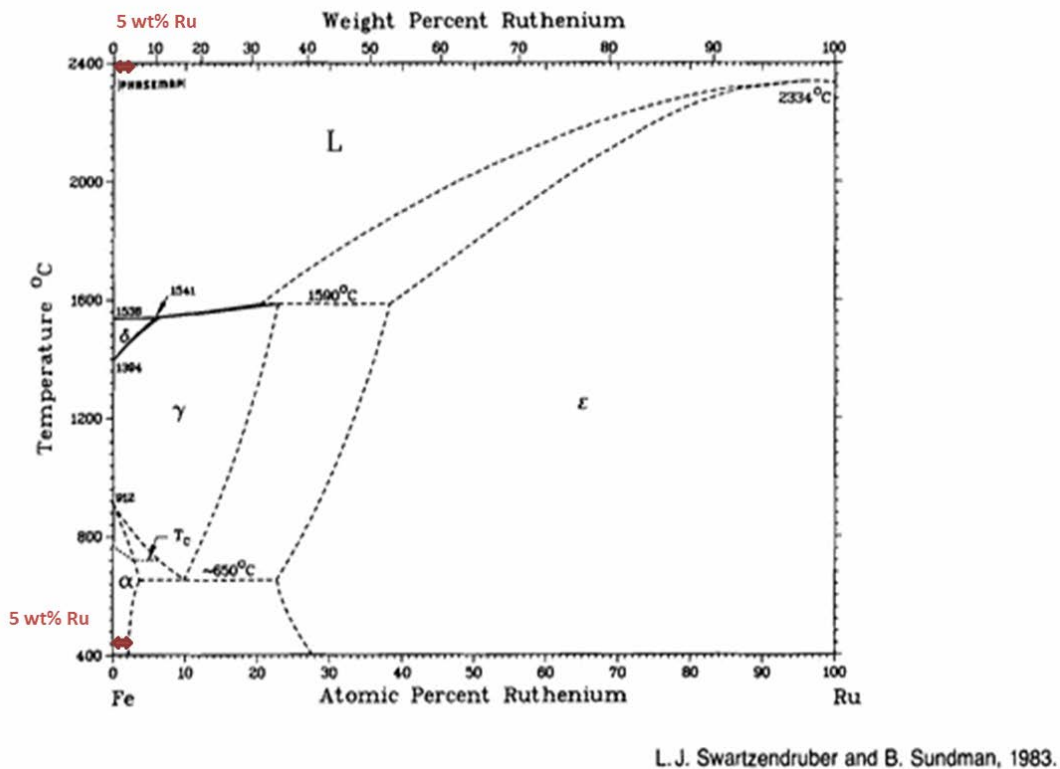
Figure 146: Equilibrium Phase Diagram of the Fe-Ru system
