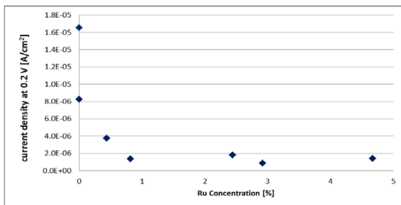
Figure 47: i at 0.2V comparison at various ruthenium compositions for the exposed surface scan in 1 M \text{H}_2\text{SO}_4 at 25°C
