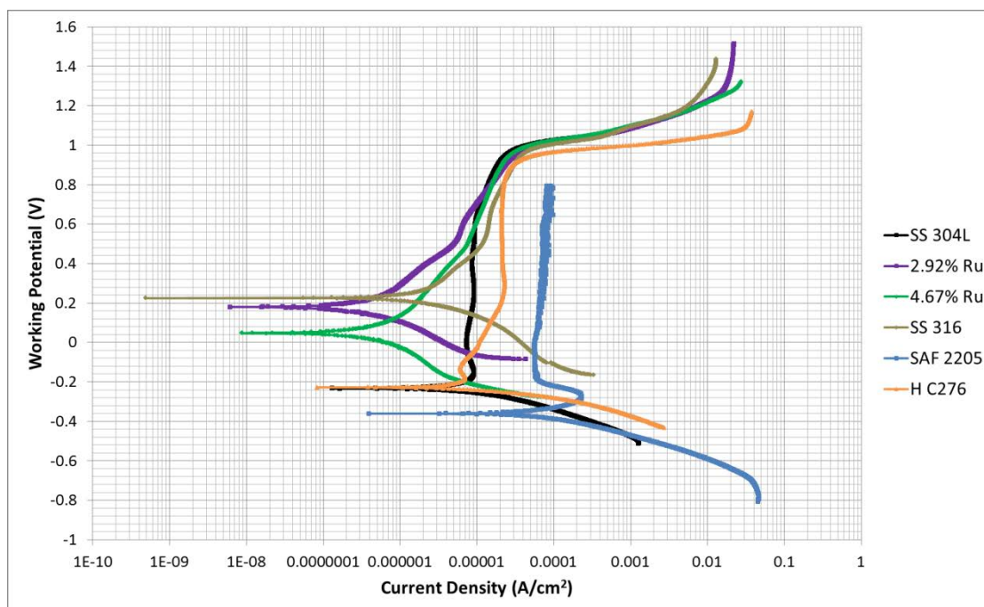
Figure 55: Log I vs E graphs from the exposed surface scan comparing ruthenium samples to other steels in 1 M \text{H}_2\text{SO}_4 at 25°C
