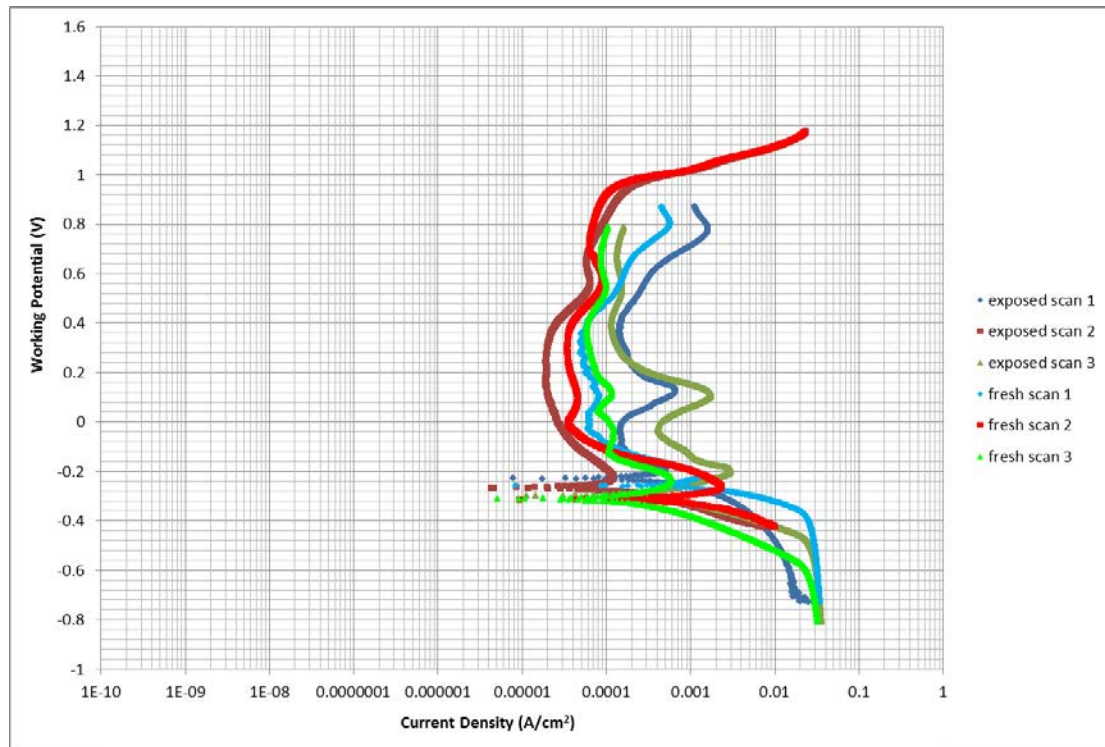
Figure 82: Log i vs E graphs for the 0.82 wt% Ru sample in 1 M \text{H}_2\text{SO}_4 at 45^\circ\text{C}
