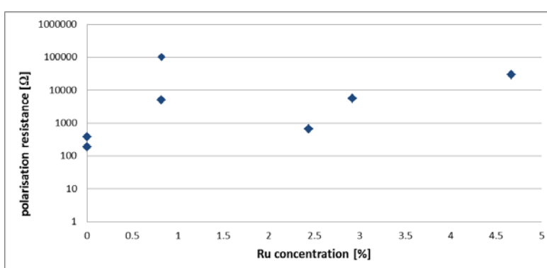
Figure 72: Polarisation resistance comparison at various ruthenium compositions from the exposed surface scan in 1 M \text{H}_2\text{SO}_4 + 1% NaCl at 25°C
