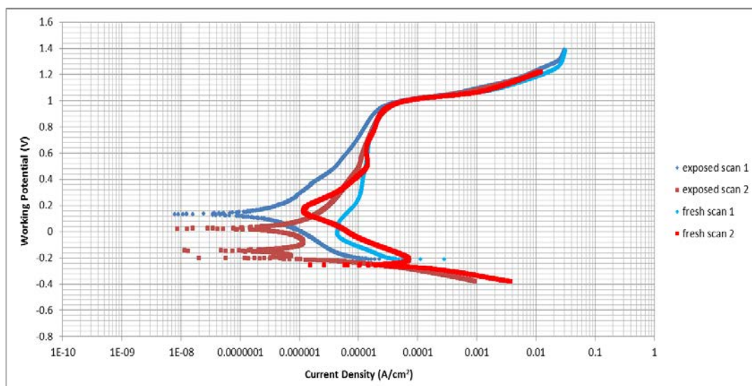
Figure 154: Log i vs E graphs for the 2.44 wt% Ru sample in 1 M \text{H}_2\text{SO}_4 at 25°C
