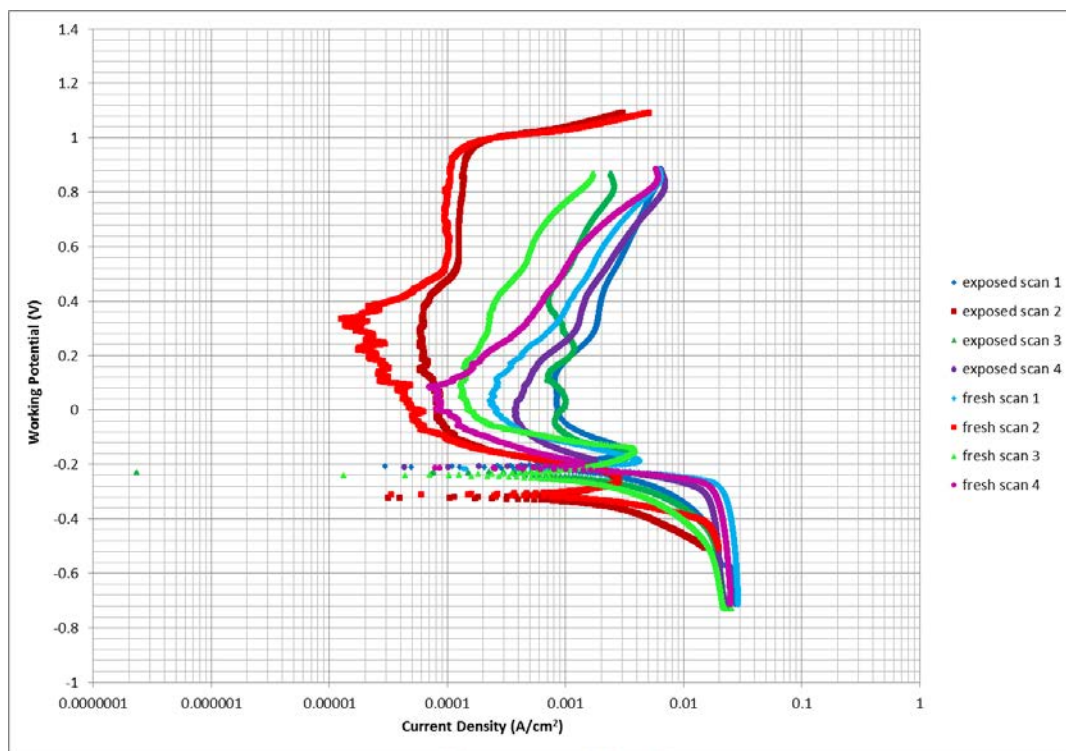
Figure 103: Log i vs E graphs for the 4.67 wt% Ru sample in 1 M \text{H}_2\text{SO}_4 + 1% NaCl at 45°C
