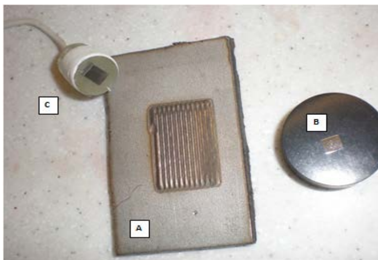
Figure 18: Samples used for the experimentation where A is the cladded coupon, B is the hot mounted sample for SEM analysis and C is the cold mounted sample for electrochemical testing
