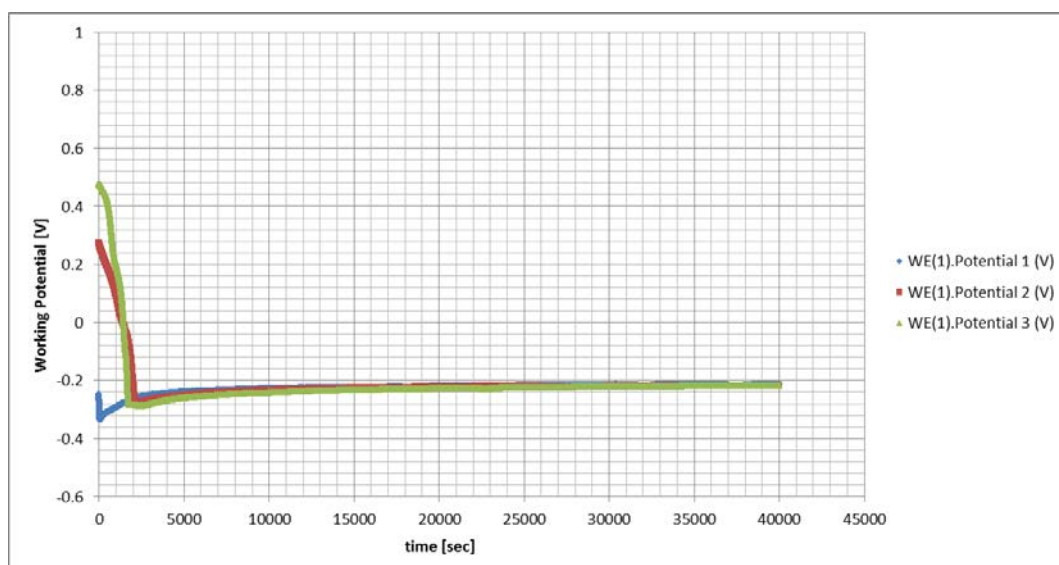
Figure 102: E vs time graphs for the 0.82 wt% Ru sample in 1 M \text{H}_2\text{SO}_4 + 1% NaCl at 45°C
