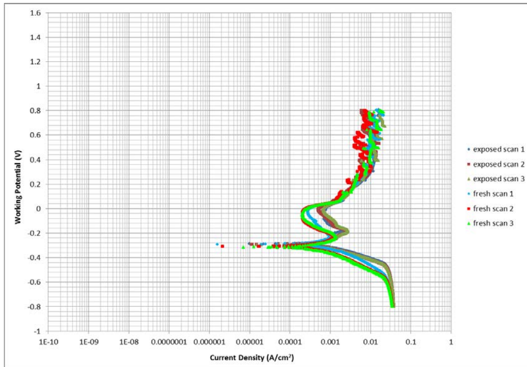
Figure 166: Log i vs E graphs for the 2.44 wt% Ru sample in 1 M \text{H}_2\text{SO}_4 at 45^\circ\text{C}
