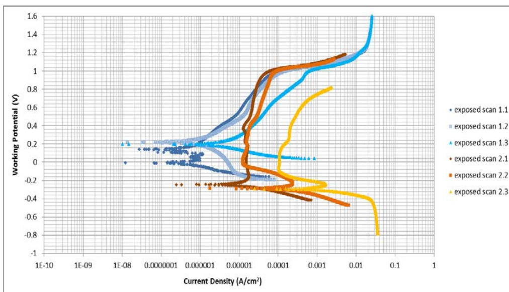
Figure 147: Log i vs E graphs for the two 0.82 wt% Ru samples in 1 M \text{H}_2\text{SO}_4 + 1% NaCl at 25°C
