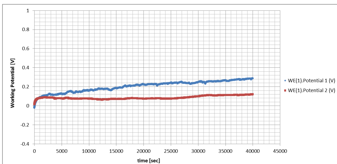
Figure 155: E vs time graphs for the 2.44 wt% Ru sample in 1 M \text{H}_2\text{SO}_4 at 25°C
