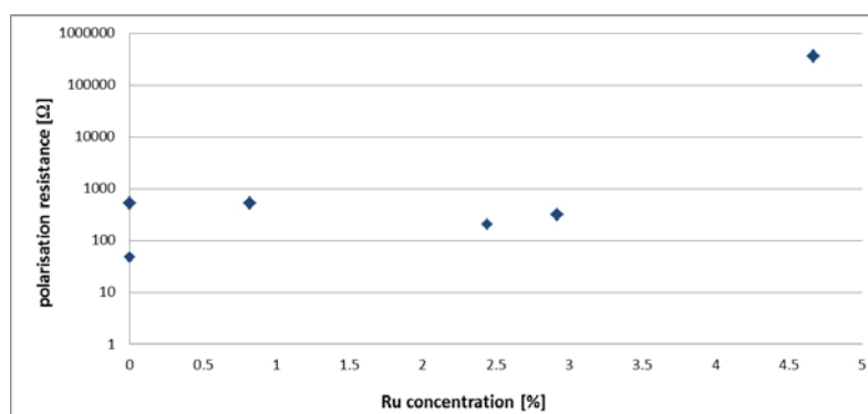
Figure 93: Polarisation resistance at various ruthenium compositions from the exposed surface scan in 1 M \text{H}_2\text{SO}_4 at 45^\circ\text{C}
