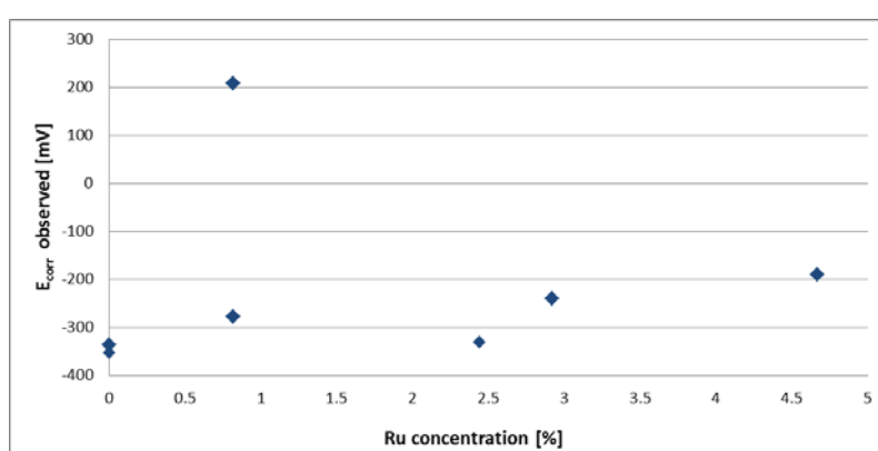
Figure 68: E_{\text{corr}} comparison at various ruthenium compositions from the exposed surface scan in 1 M \text{H}_2\text{SO}_4 + 1% NaCl at 25°C
