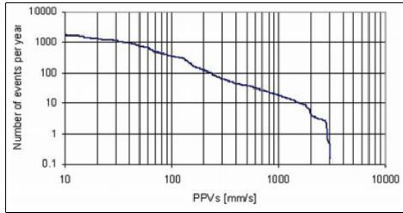
Figure 2.10 Peak particle velocities of the seismic events at Tau Tona mine, Milev and Spottiswoode (2005)
