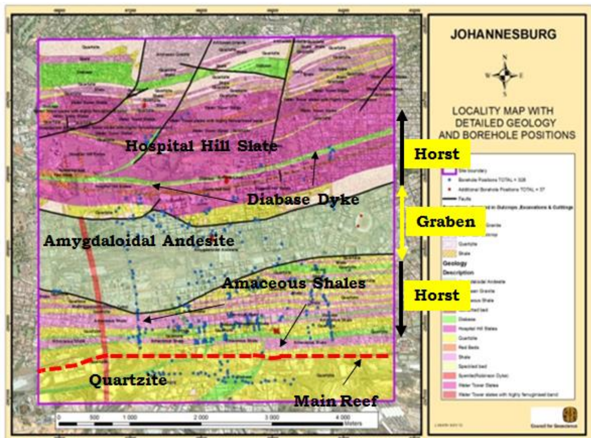
Figure 4.9 Geological map of study area, after Council for Geoscience (2013)
