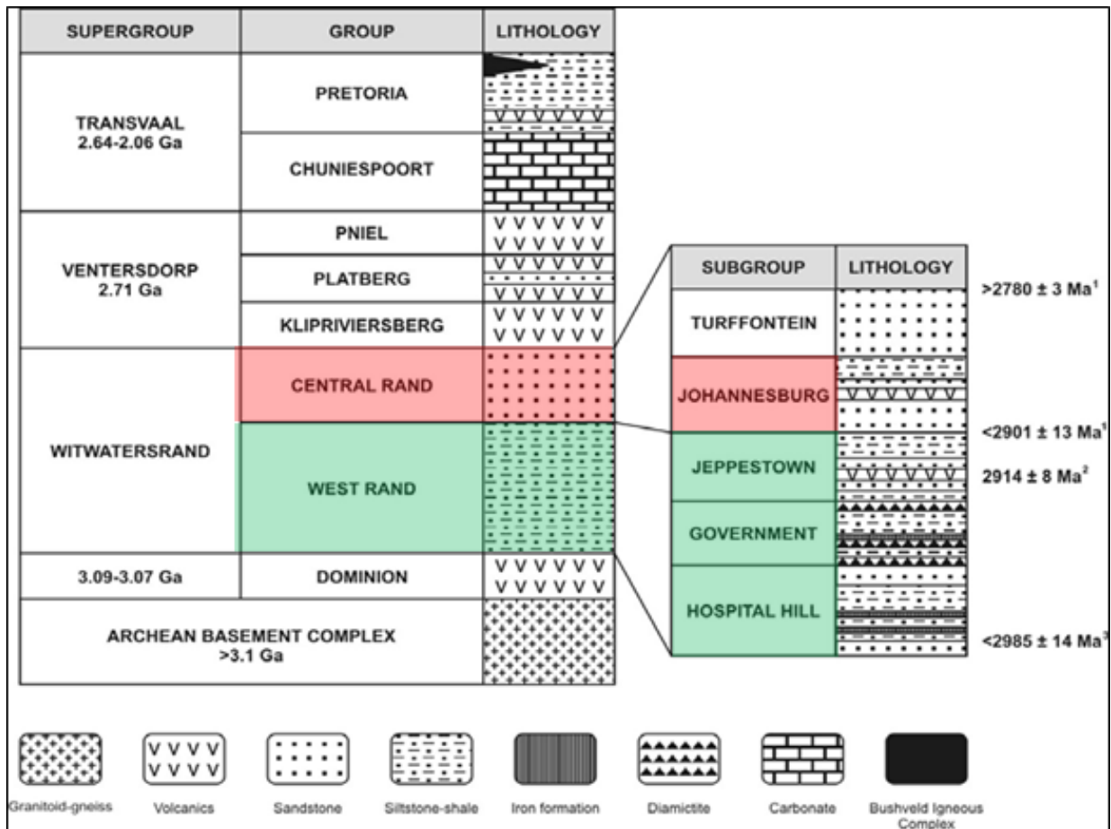
Figure 4.7 Simplified regional stratigraphy of Witwatersrand, after Dankert and Hein (2010)
