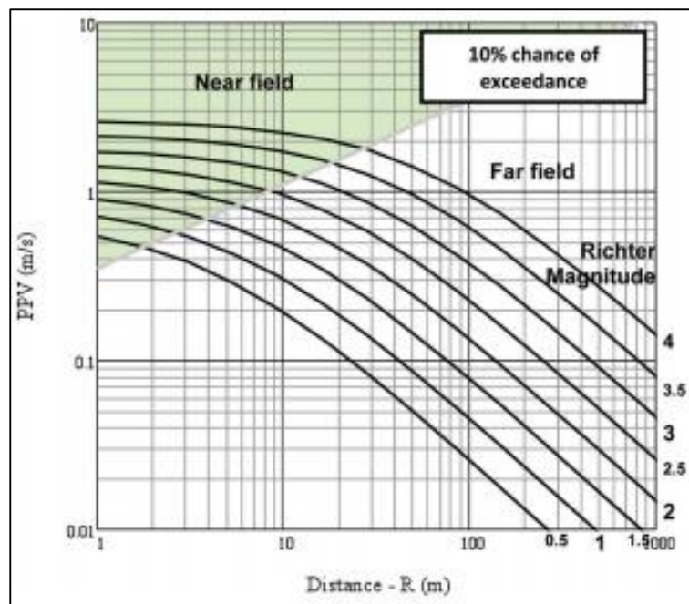
Figure 2.11 Correlation of peak velocity, magnitude and distance in South Africa mining areas, Potvin and Wesseloo (2010)
