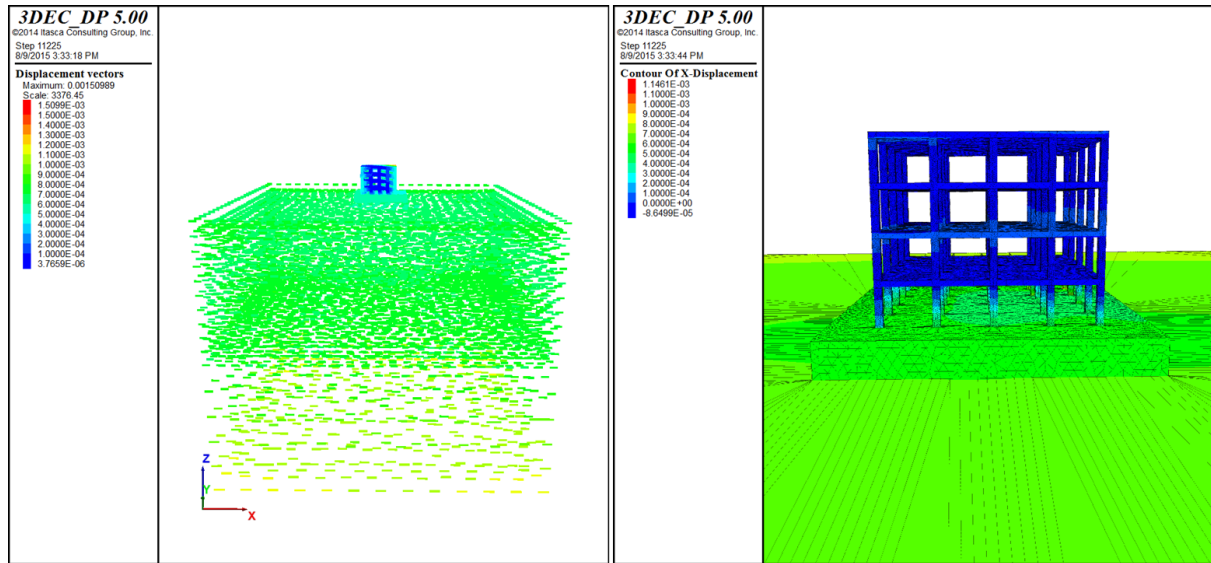
Figure 6.25 Horizontal displacement at T=1.5 sec
