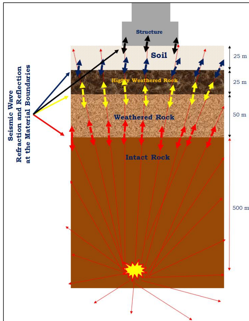
Figure 3.7 Idealized model showing depth of seismic source, geological layers and surface structure
