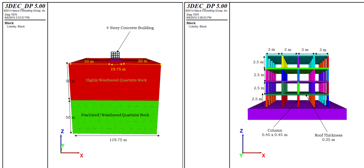
Figure 6.20 Model size and geometry of four storey concrete building
