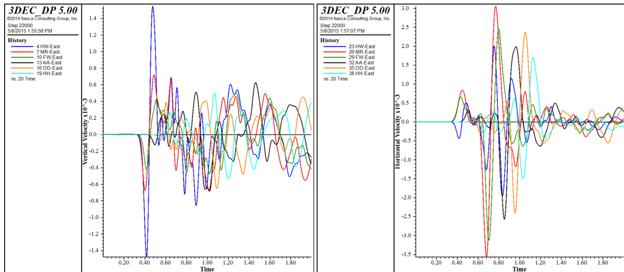
Figure 5.28 Slip along a flooded joint due to gradual rise in pore pressure, plots of velocity time histories on the east edge of the model; left – vertical velocity time histories, right –horizontal velocity time histories
