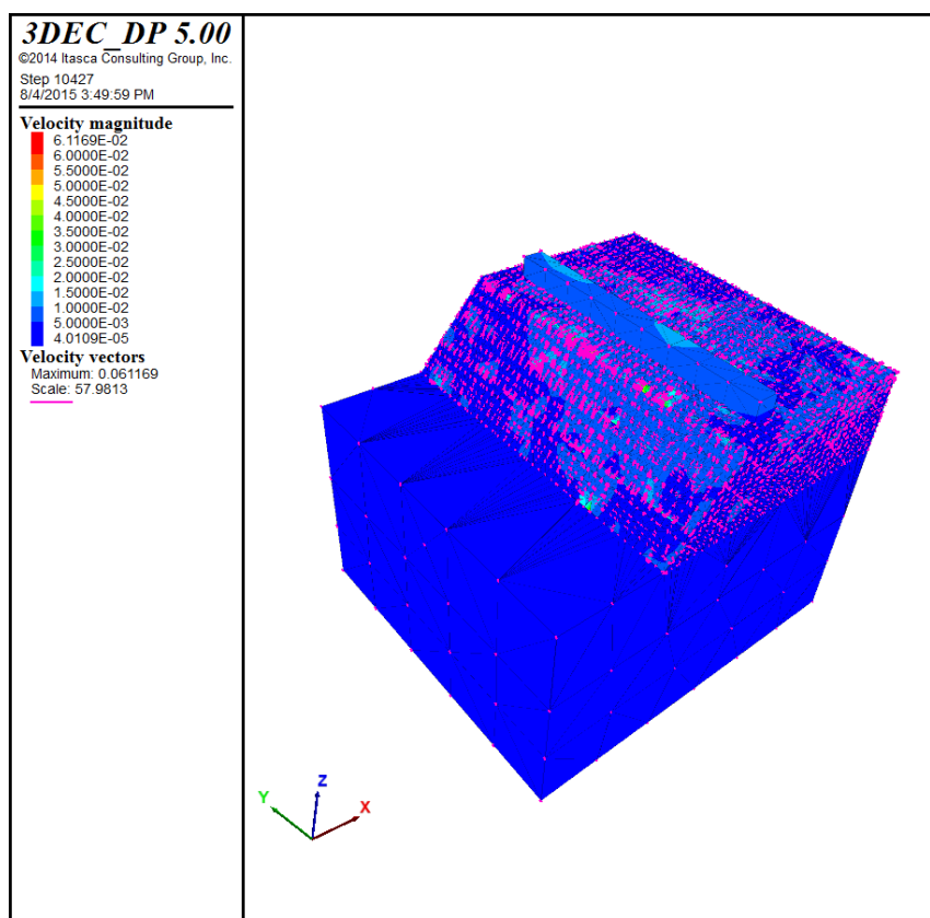
Figure 6.42 Velocity contours and vectors at 1.0 sec duration
