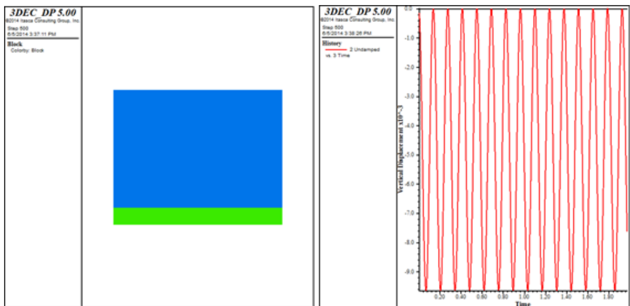
Figure 5.5 Seismic waveform with one discontinuity (frequency = 5 Hz, amplitude = 9.6 mm)
