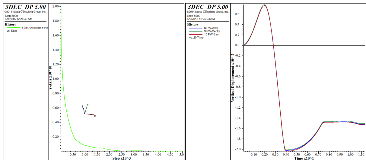
Figure 5.17 Initial static equilibrium; left – plot of unbalanced force, right – plot of vertical displacement histories in Foot Wall
