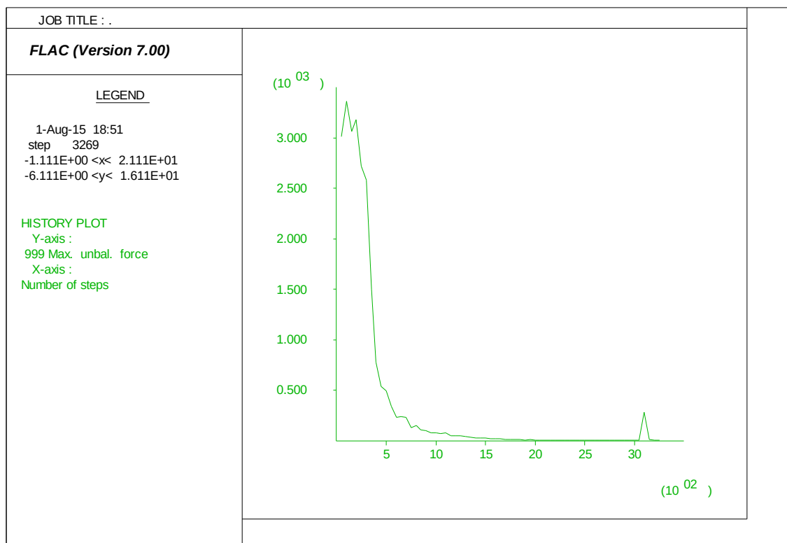
Figure 6.61 Plot of unbalanced force; initial static equilibrium
