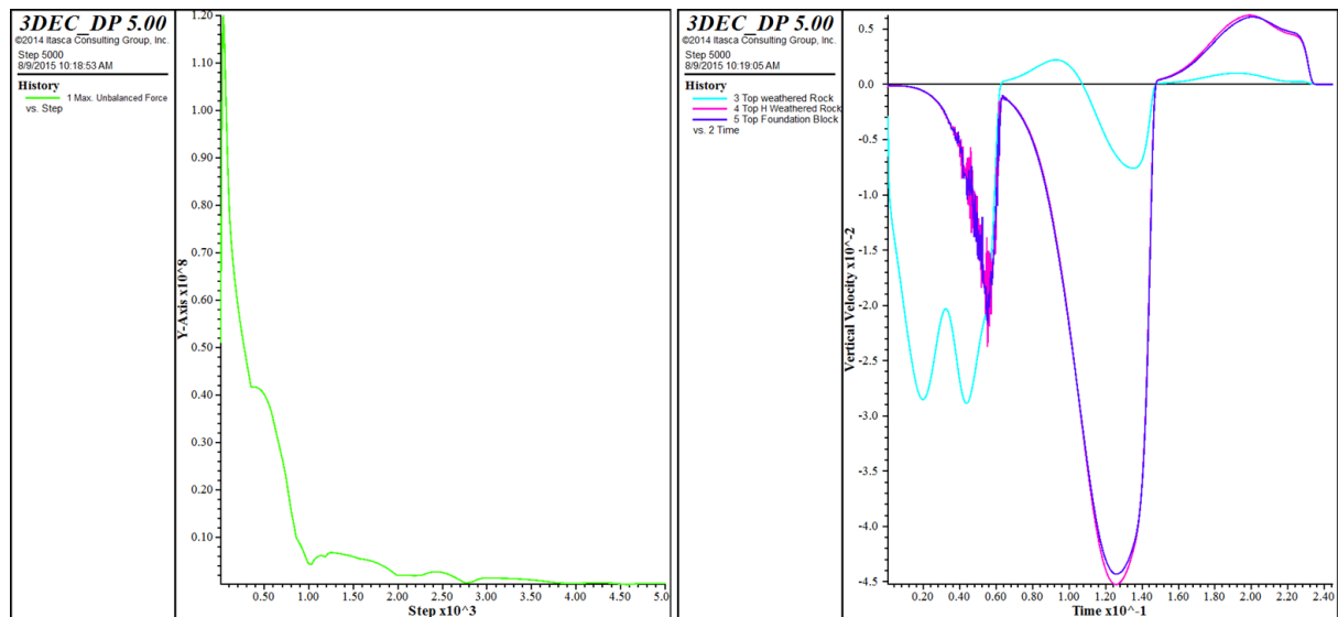
Figure 6.14 Plot of unbalanced force (left) and vertical velocity histories (right)
