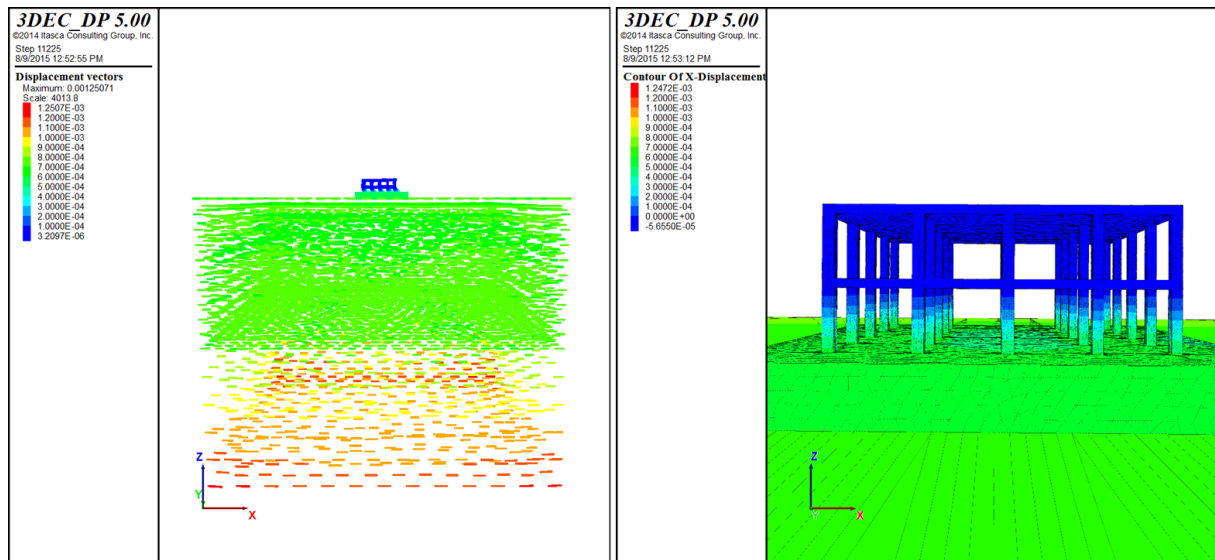
Figure 6.18 Horizontal displacement at T = 1.50 sec
