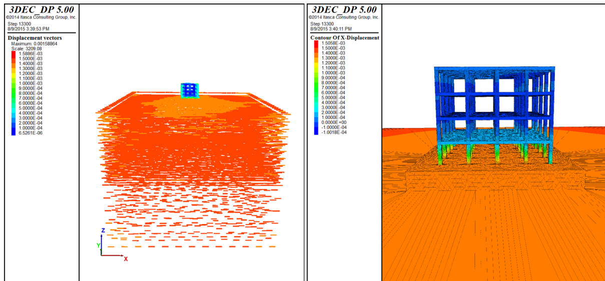
Figure 6.26 Horizontal displacement at T=2.0 sec
