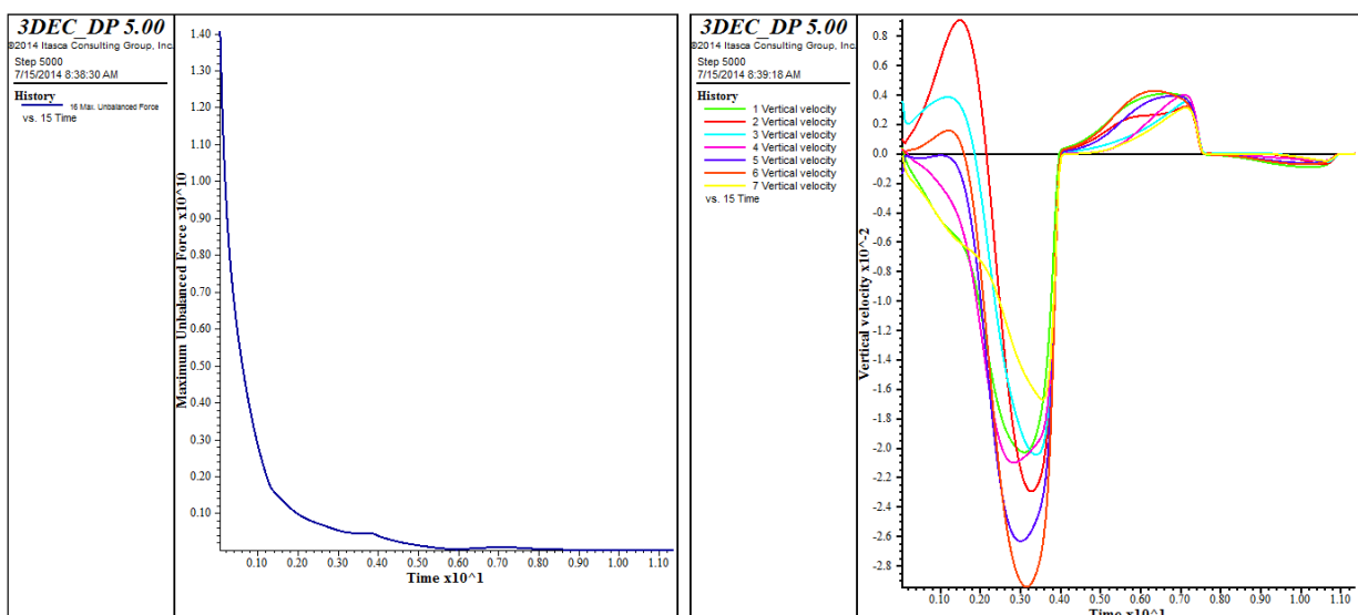
Figure 5.10 Initial Static Equilibrium; left-Unbalanced Force, Right-Vertical Velocity Histories
