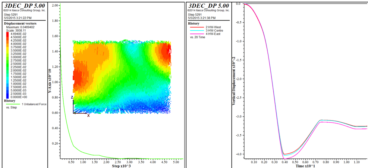
Figure 5.30 Static equilibrium; left-plot of unbalanced force, right-plot of vertical displacement histories in Hanging Wall
