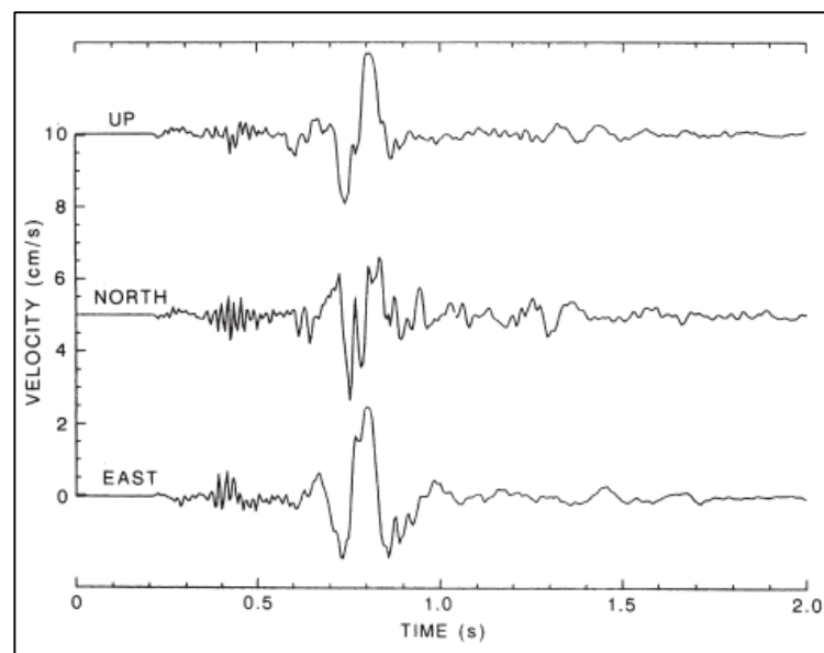
Figure 2.9 Peak velocity recorded at surface, 2.7 km above the source due to a mining induced earthquake of M4.4, McGarr (2002)
