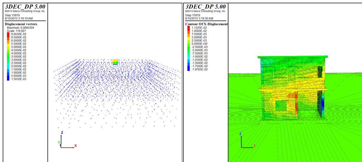
Figure 6.12 Horizontal displacement at T =2.0 sec
