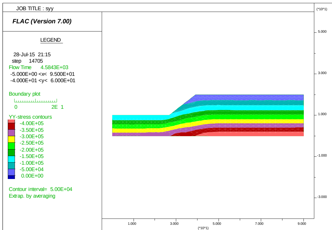
Figure 6.54 Plot of contours of vertical stress showing equilibrium (gradual distribution)
