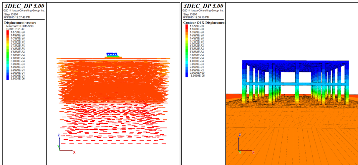
Figure 6.19 Horizontal displacement at T =2.0 sec
