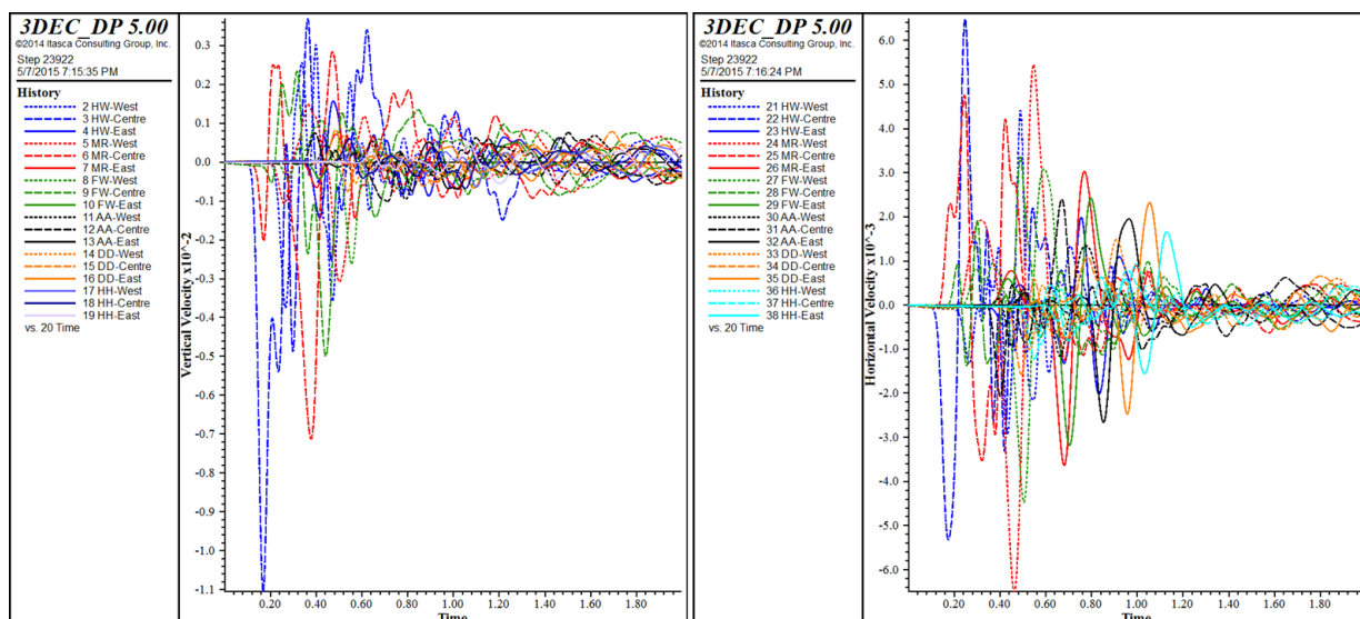
Figure 5.24 Slip along a dry joint, plots of velocity time histories on the entire model; left – vertical velocity time histories, right –horizontal velocity time histories
