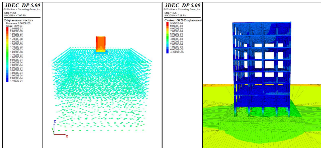
Figure 6.32 Horizontal displacement at T=1.5 sec
