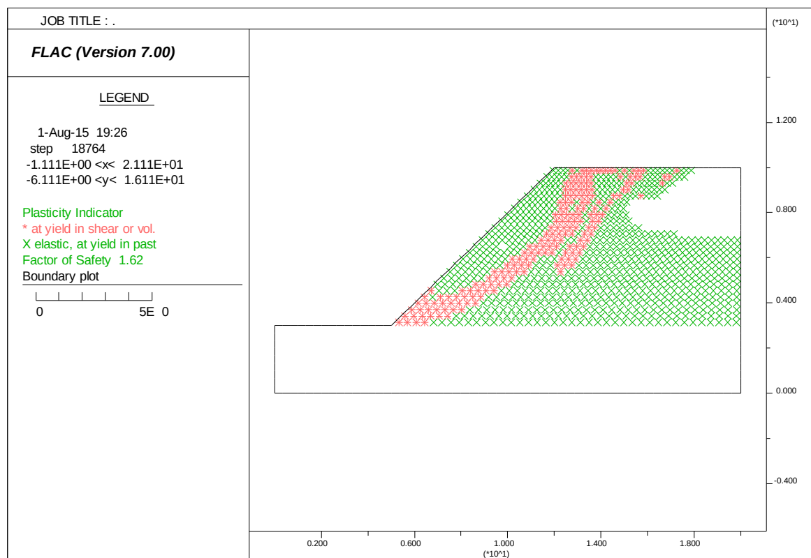
Figure 6.66 Plot of plasticity indicator and factor of safety
