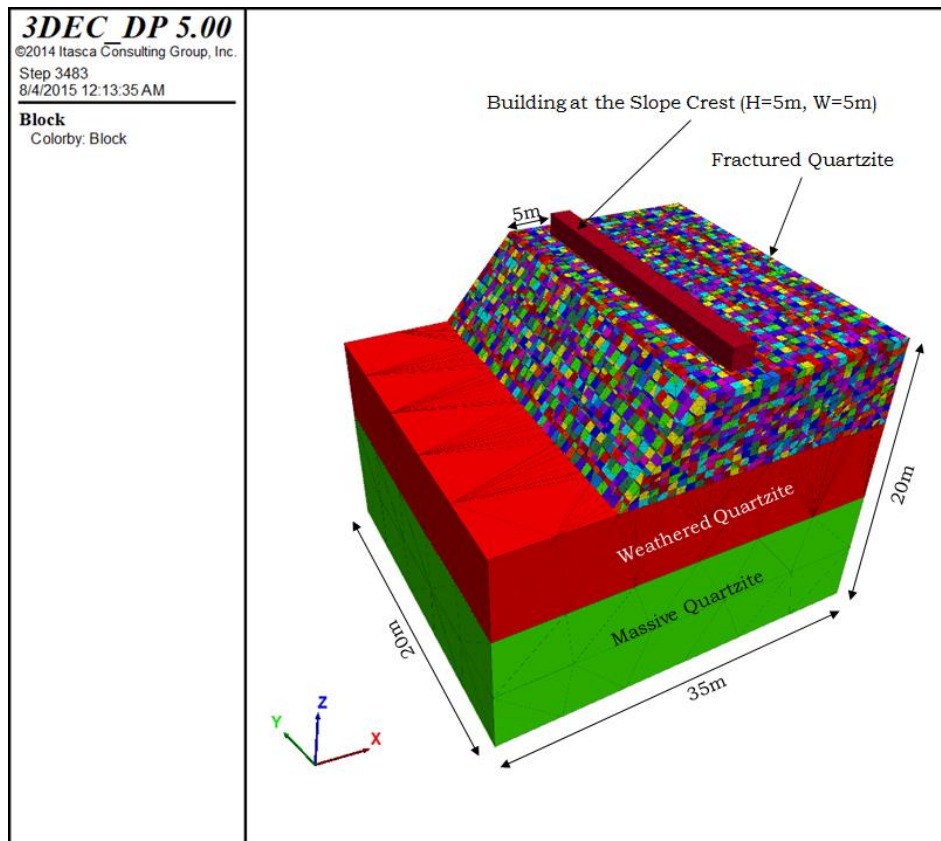
Figure 6.34 Quartzite slope geometry
