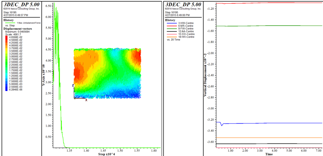
Figure 5.49 Plot of displacement vectors on left, vertical displacement histories at the centre points on the model shown on right
