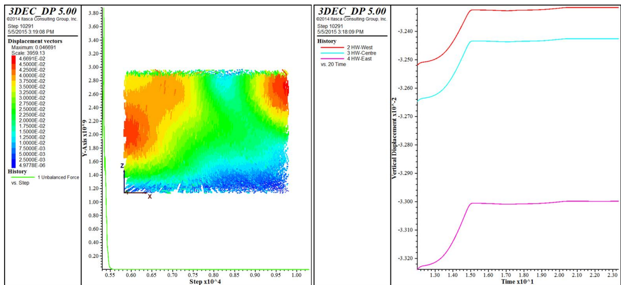
Figure 5.33 Post excavation equilibrium; left-plot of unbalanced force, right-plot of displacement histories in Hanging Wall
