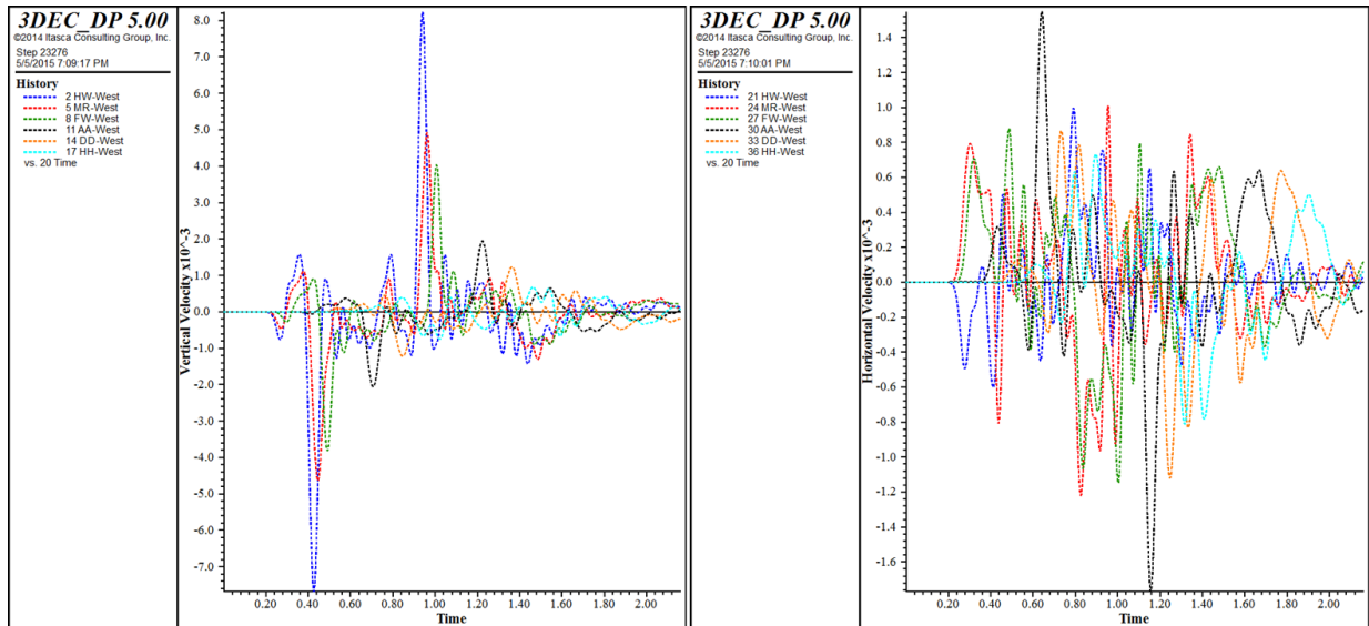
Figure 5.39 Ground motions due to fall of ground at the west edge of the model; Left-vertical velocity time histories, Right-horizontal velocity time histories
