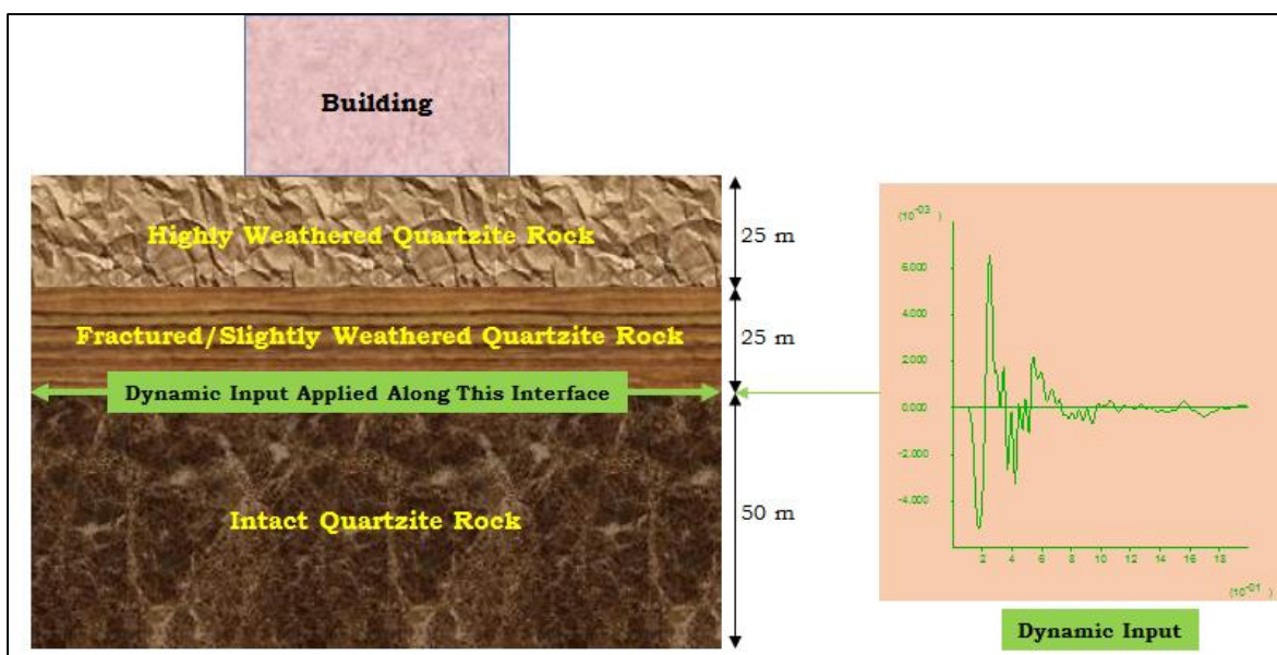
Figure 6.5 Dynamic application at the bedrock
