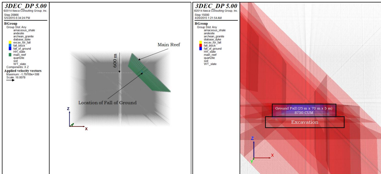
Figure 5.32 Excavation; left-location of Main Reef and Fall of Ground, Right-close-up of Excavation and Fall of Ground
