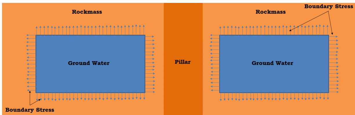
Figure 3.4 Boundary stress to represent effect of flooded voids in 3DEC
