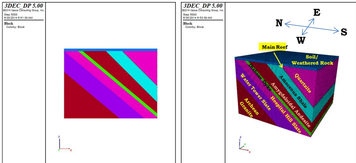
Figure 5.3 Model Geometry; left-elevation from the West, Right-material groups (labelling shown in the right figure holds good for the left figure as well)
