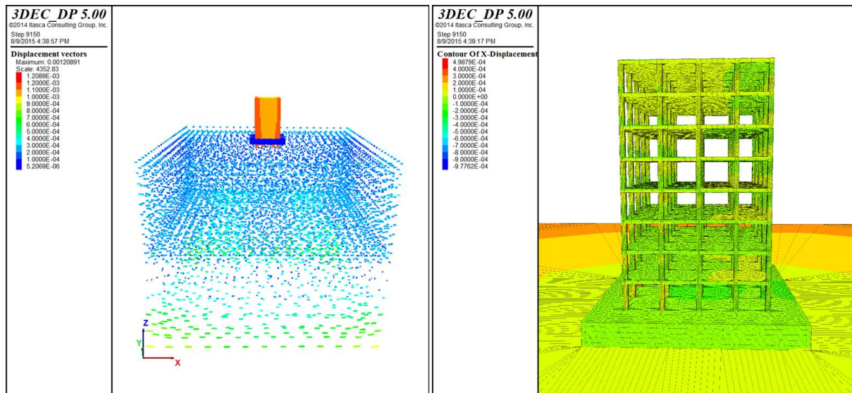
Figure 6.31 Horizontal displacement at T=1.0 sec
