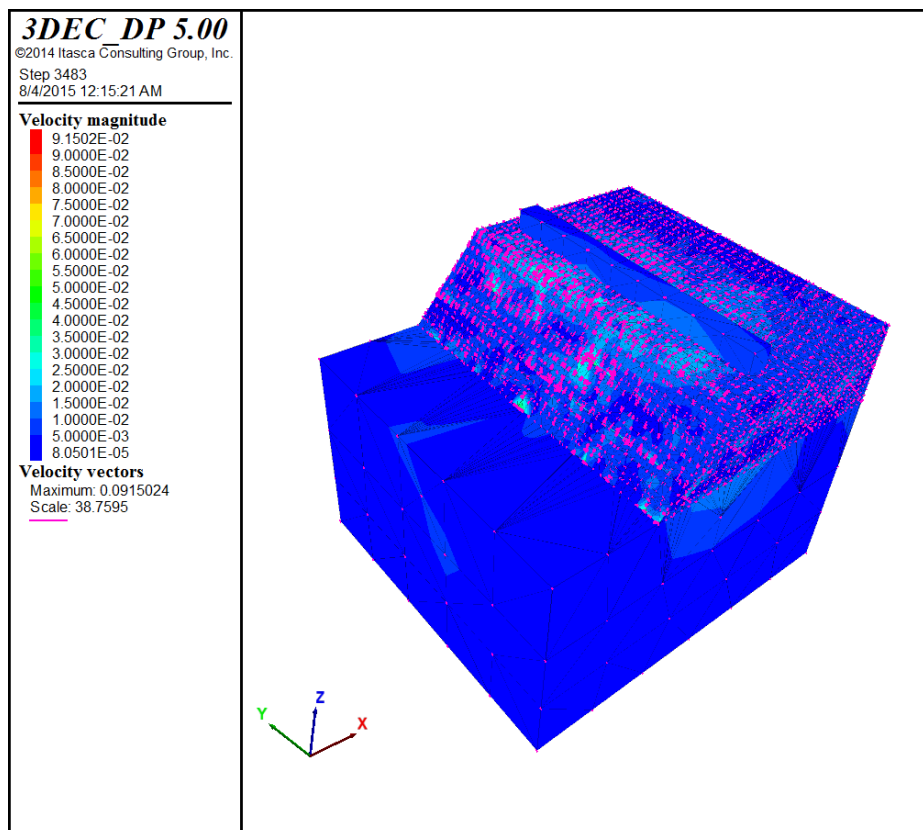
Figure 6.39 Velocity contours and vectors at 0.5 sec duration
