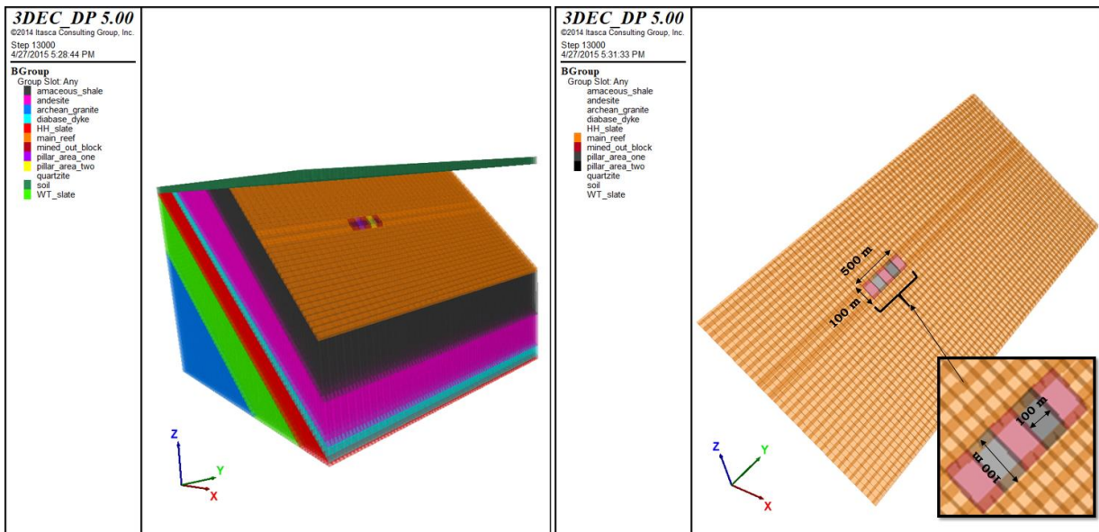
Figure 5.44 Location and layout of mining pillars (shown in grey colour) and excavations (shown in pink colours)
