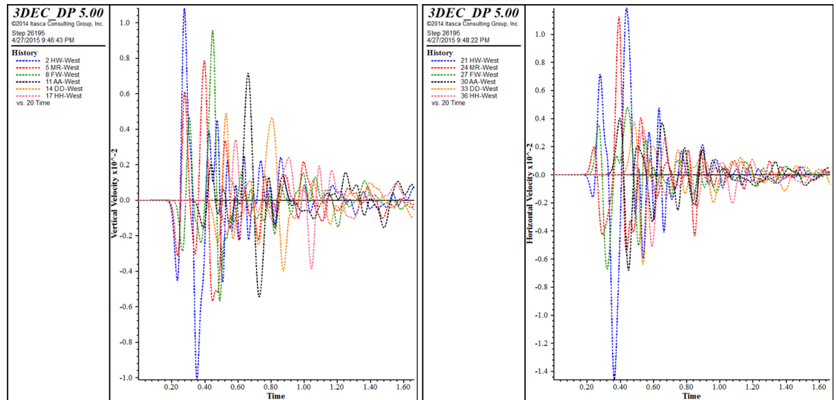
Figure 5.53 Left; vertical velocity histories, Right; horizontal velocity histories at the western edge of each geological group
