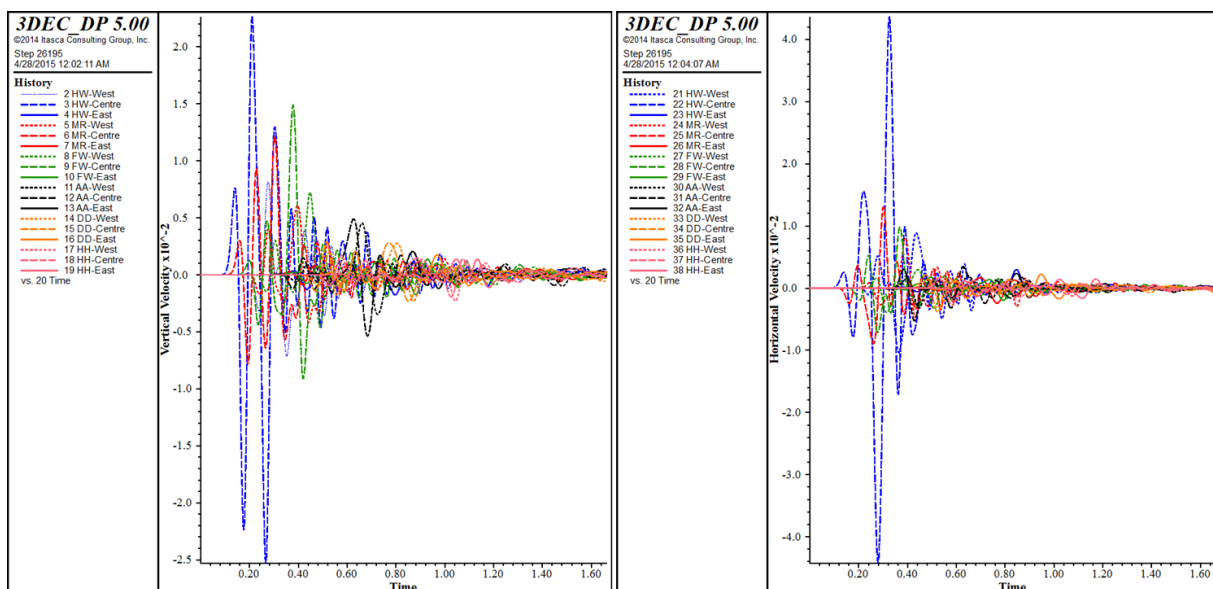
Figure 5.60 Left; all vertical velocity histories, Right; all horizontal velocity histories
