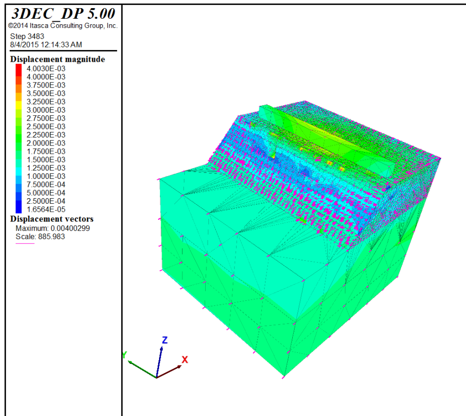
Figure 6.38 Displacement contours and vectors at 0.5 sec duration
