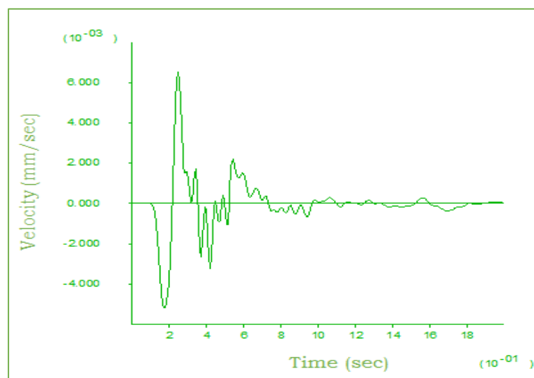
Figure 6.4 Ground motion (horizontal velocity time history) selected for dynamic structural analysis
