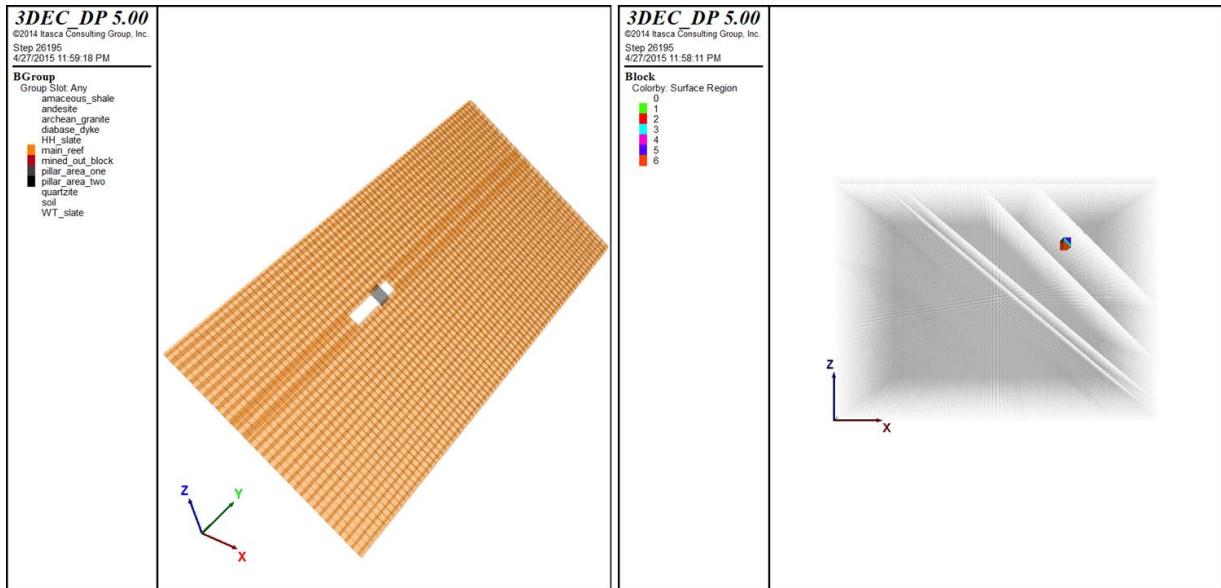
Figure 5.56 Left; one pillar excavated, Right; creation of six regions for setting boundary stress to represent effect of water filled voids
