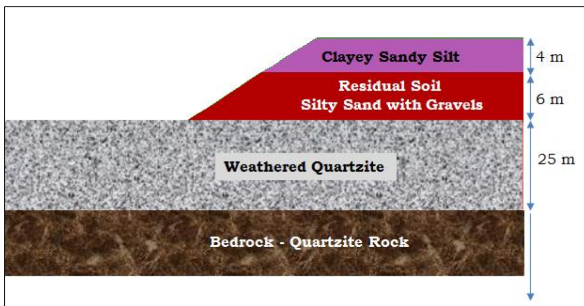
Figure 6.50 Geological profile of the tailings dam slope
