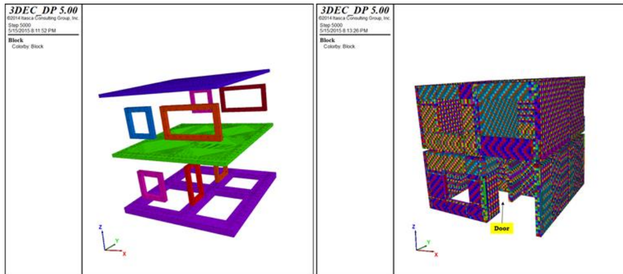
Figure 6.7 Model Geometry; left-concrete elements (foundation, windows, doors, roofs), right-geometry of brick walls of 1st and 2nd stories
