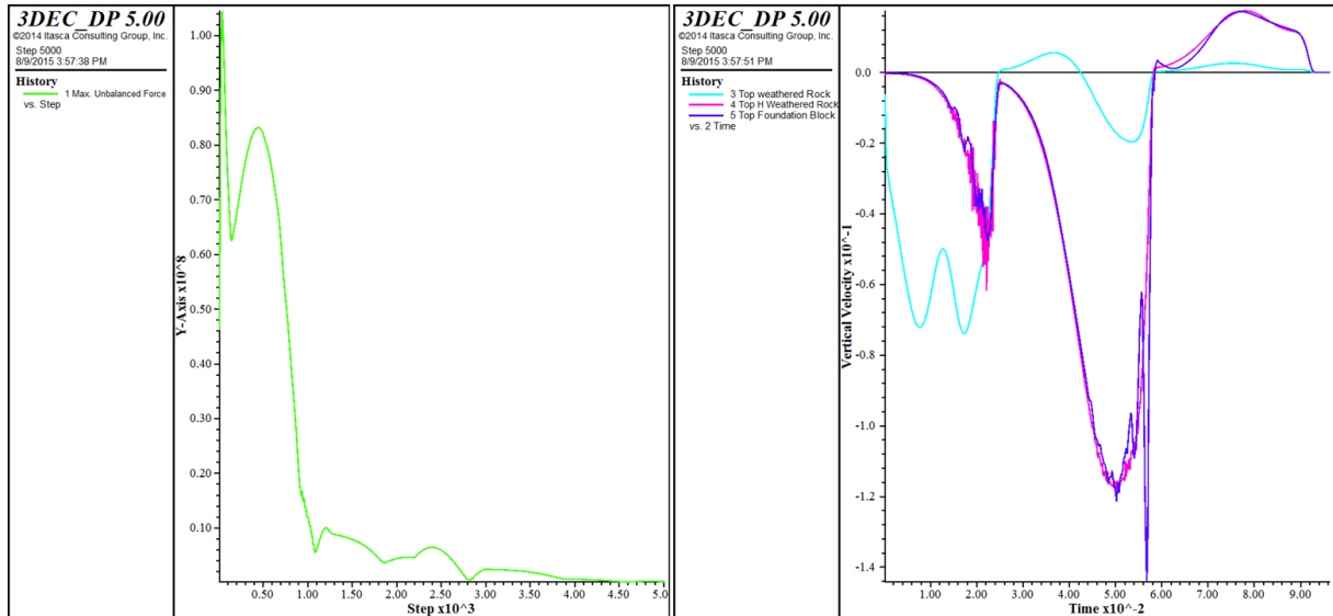
Figure 6.28 Plot of unbalanced force (left) and vertical velocity histories (right)
