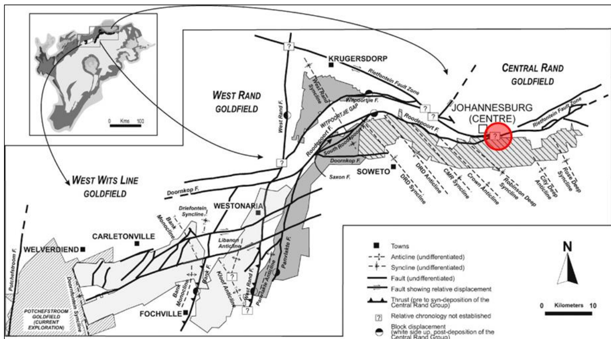
Figure 4.8 Geological structures in the Central Rand, Dankert and Hein (2010)
