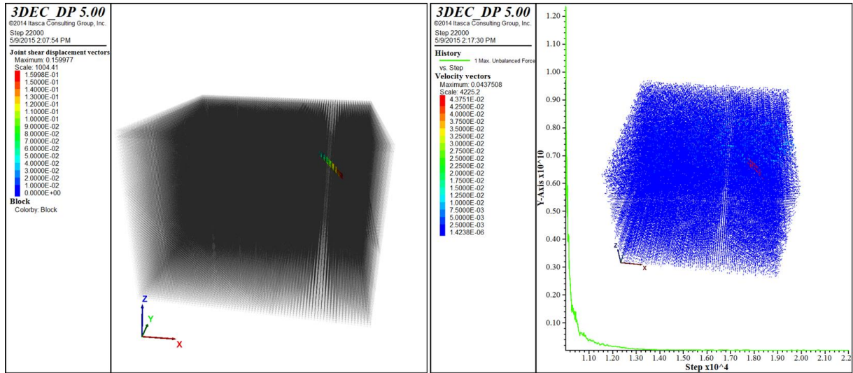
Figure 5.25 Slip along a flooded joint due to gradual rise in pore pressure; left – plot of joint shear displacement, right – plot of unbalanced force and velocity histories
