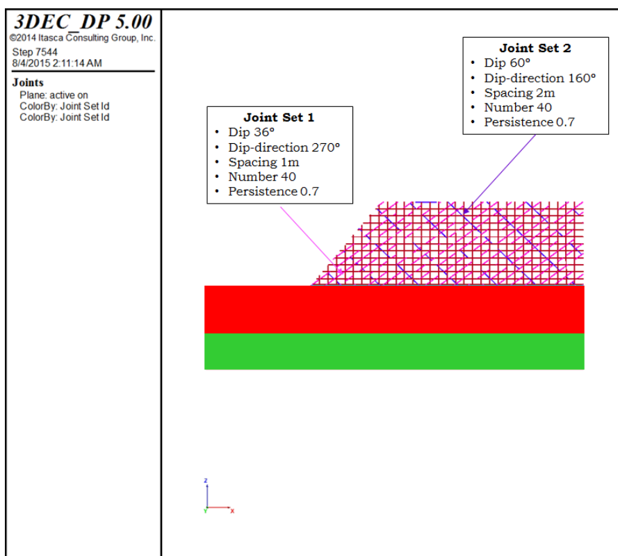
Figure 6.35 Joint sets in the slope
