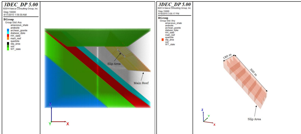
Figure 5.16 Model geometry; left – location of the slip area, right - size of the slip area
