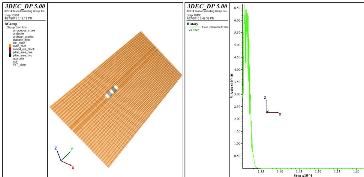
Figure 5.48 Excavations shown in white colour in the left figure, plot of unbalanced force on right
