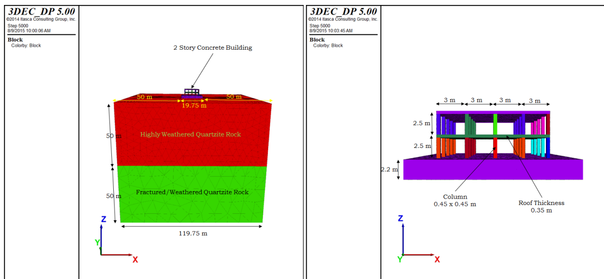
Figure 6.13 Model size and geometry of two storey concrete building
