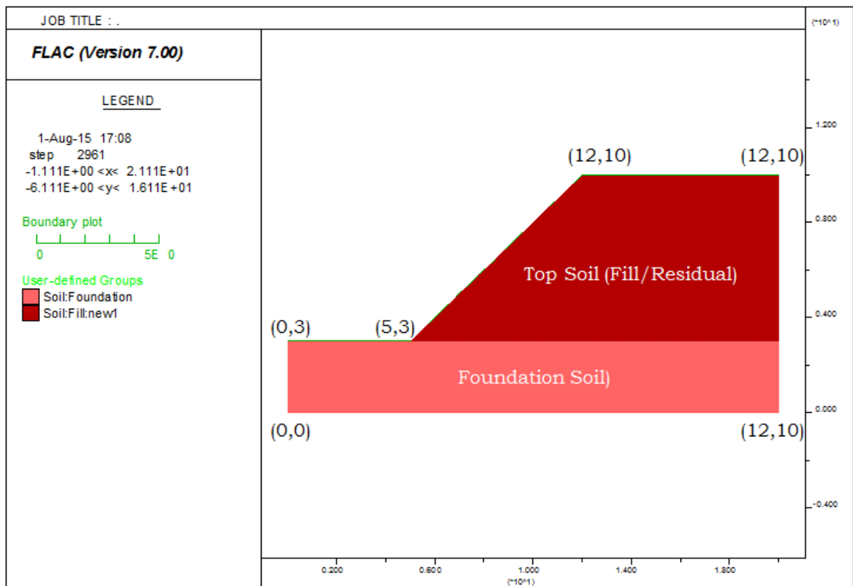
Figure 6.60 Slope geometry
