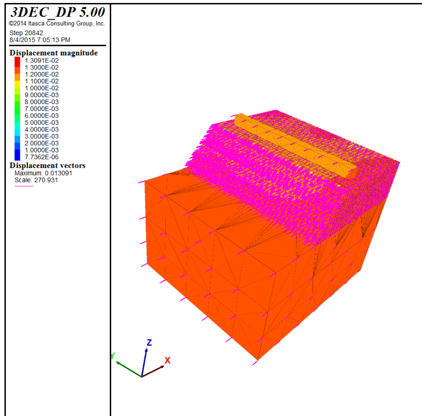
Figure 6.44 Displacement contours and vectors at 1.5 sec duration
