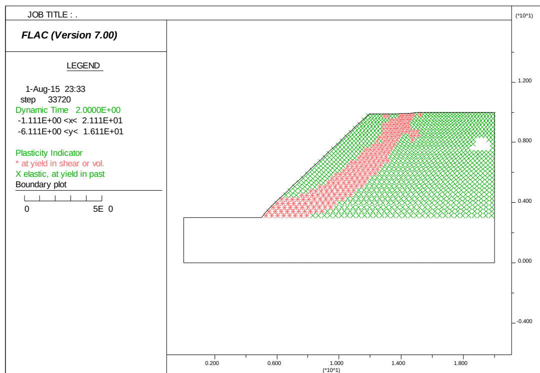
Figure 6.69 Plot of plasticity indicators
