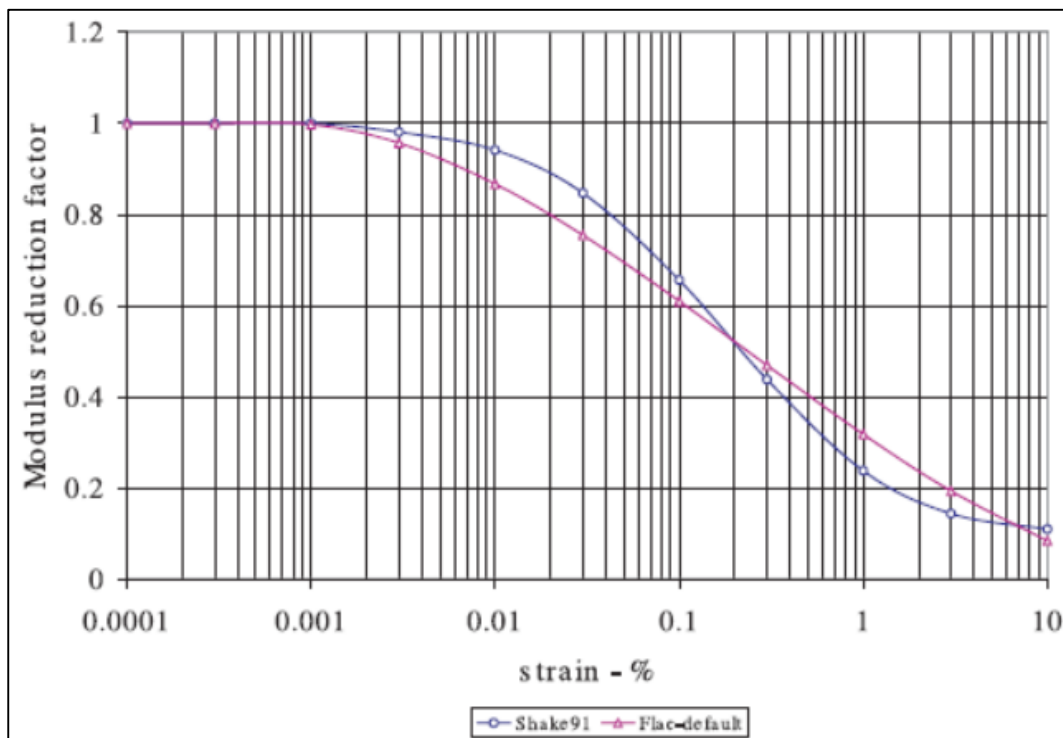
Figure 3.9 Modulus reduction curve for clayey soil (FLAC default hysteric damping with L1 = -3.156 , L2 = 1.904 ), Itasca (2014)
