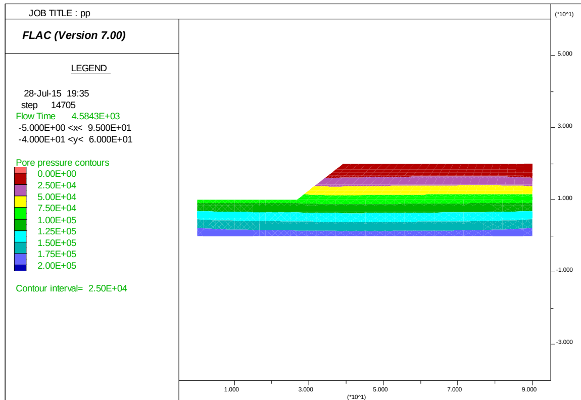
Figure 6.53 Plot of pore-pressure contours showing equilibrium (steady state condition)
