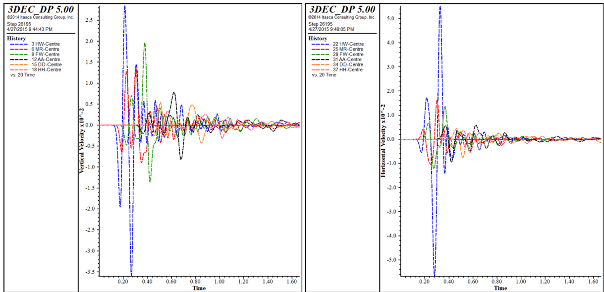
Figure 5.52 Left; vertical velocity histories, Right; horizontal velocity histories at the centre of each geological group
