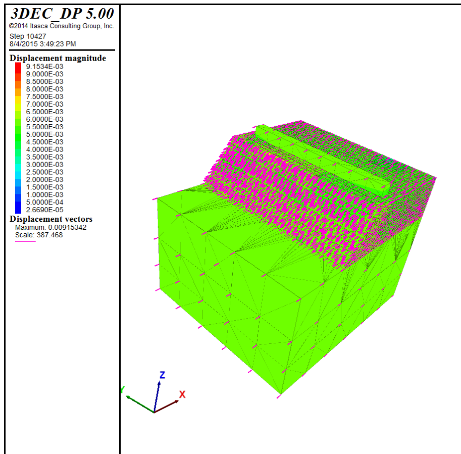
Figure 6.41 Displacement contours and vectors at 1.0 sec duration
