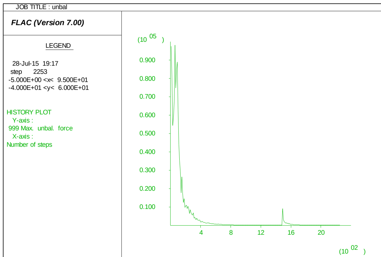
Figure 6.52 Plot of unbalanced force showing the model reached equilibrium
