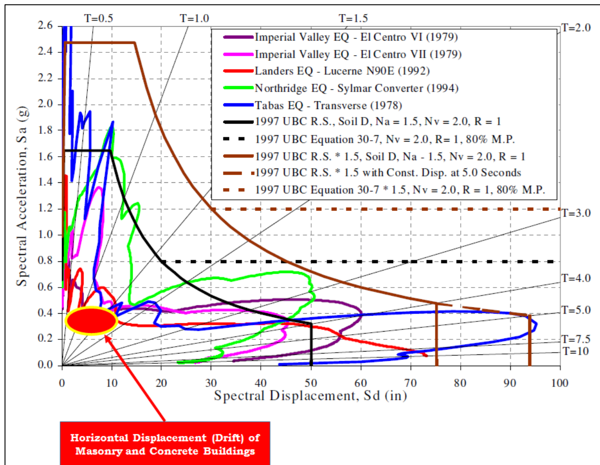
Figure 6.74 Horizontal displacements compared to “ Spectral Acceleration-Spectral Displacement , Searer et al. (2004)”
