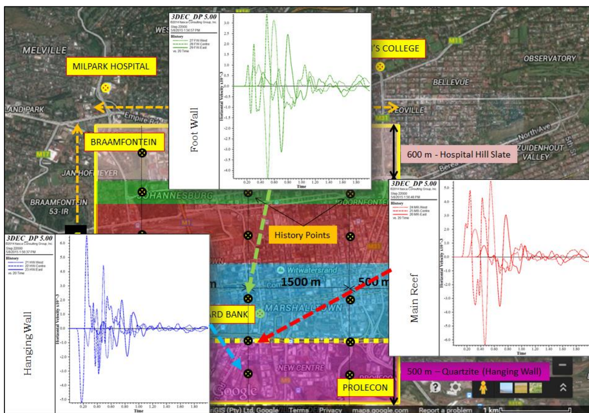
Figure 5.62 Ground motion recommendations for seismic structure analysis
