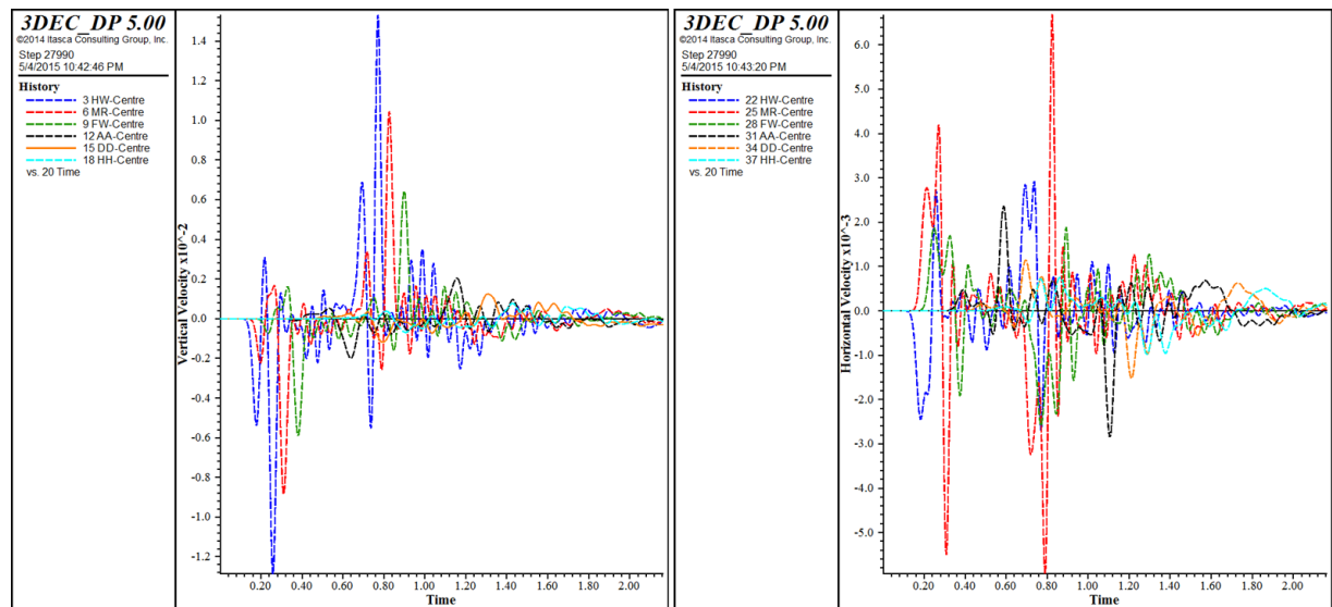
Figure 5.36 Ground motions due to fall of ground at the centre of the model; Left-vertical velocity time histories, Right-horizontal velocity time histories
