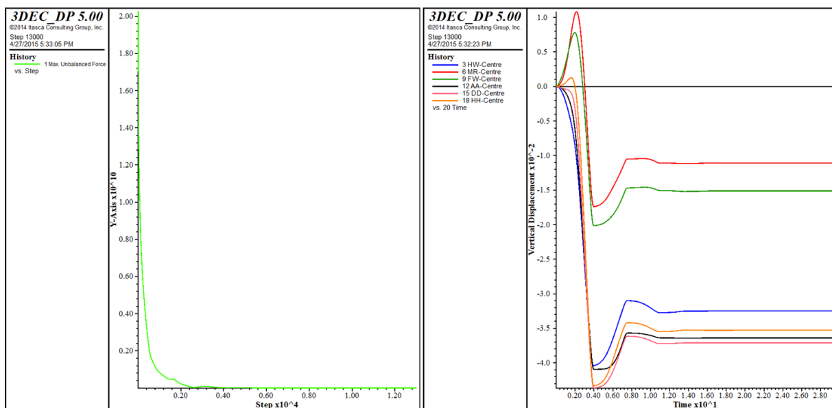
Figure 5.45 Initial static equilibrium condition of the model; plot of unbalanced force on left and vertical displacement histories at the centre points on the right
