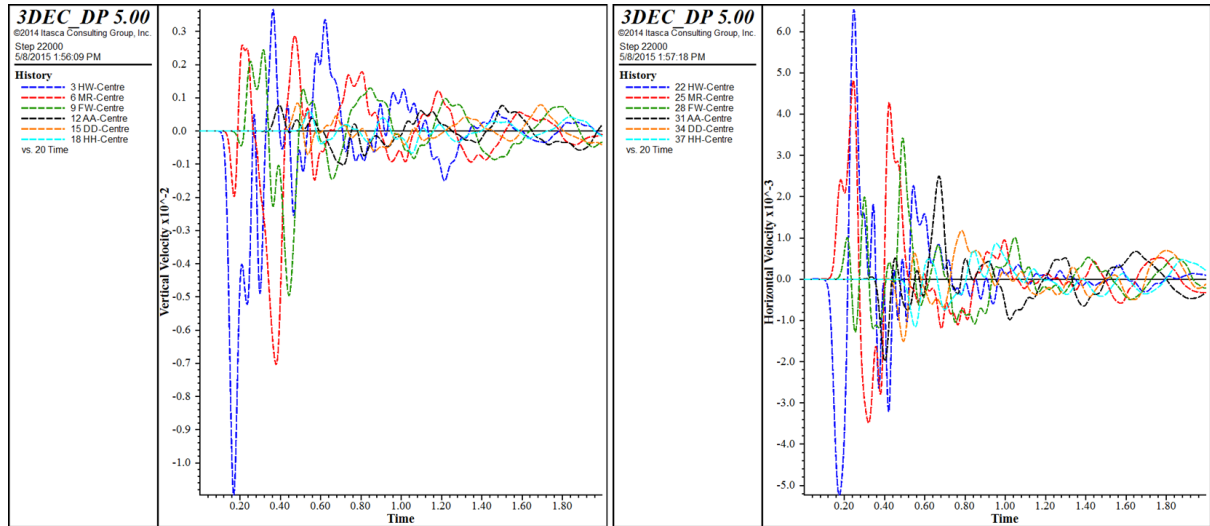
Figure 5.27 Slip along a flooded joint due to gradual rise in pore pressure, plots of velocity time histories on the centre of the model; left – vertical velocity time histories, right –horizontal velocity time histories
