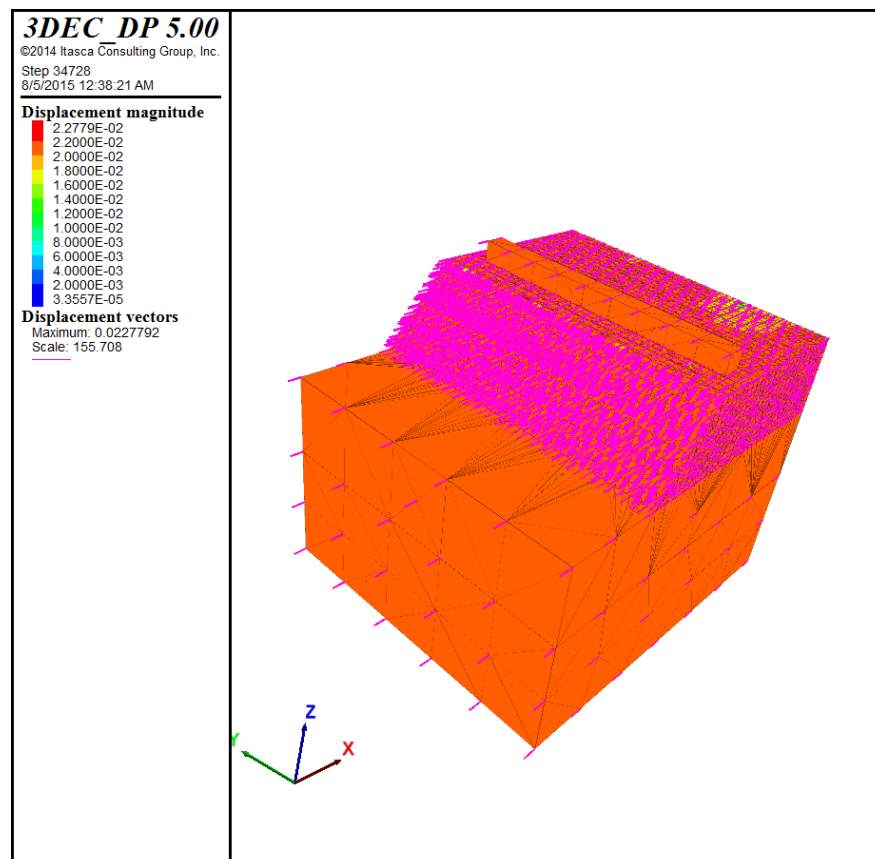
Figure 6.47 Displacement contours and vectors at 2.0 sec duration
