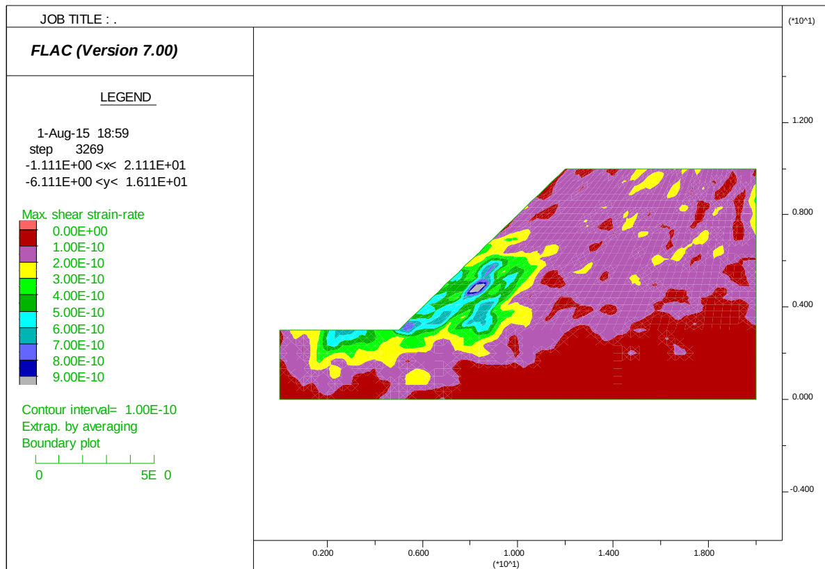
Figure 6.62 Plot of shear strain contours showing elastic strain range
