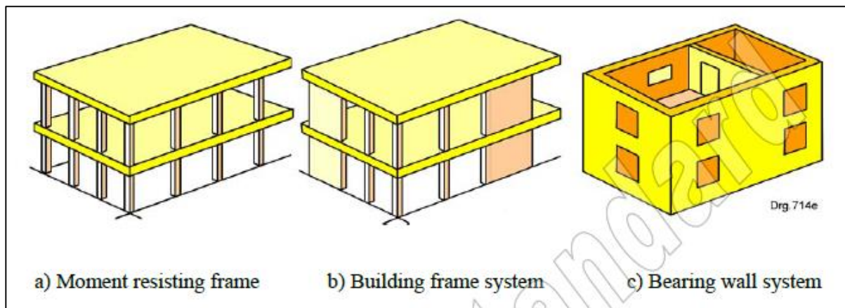
Figure 2.27 Guideline for the structural systems for dynamic analysis, SANS 10160-4:2009
