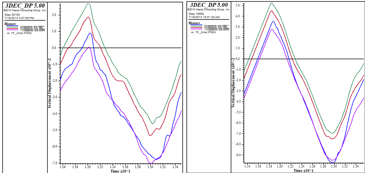
Figure 5.8 Partial density scaling / un-damped; left-vertical velocity histories, right-vertical displacement histories
