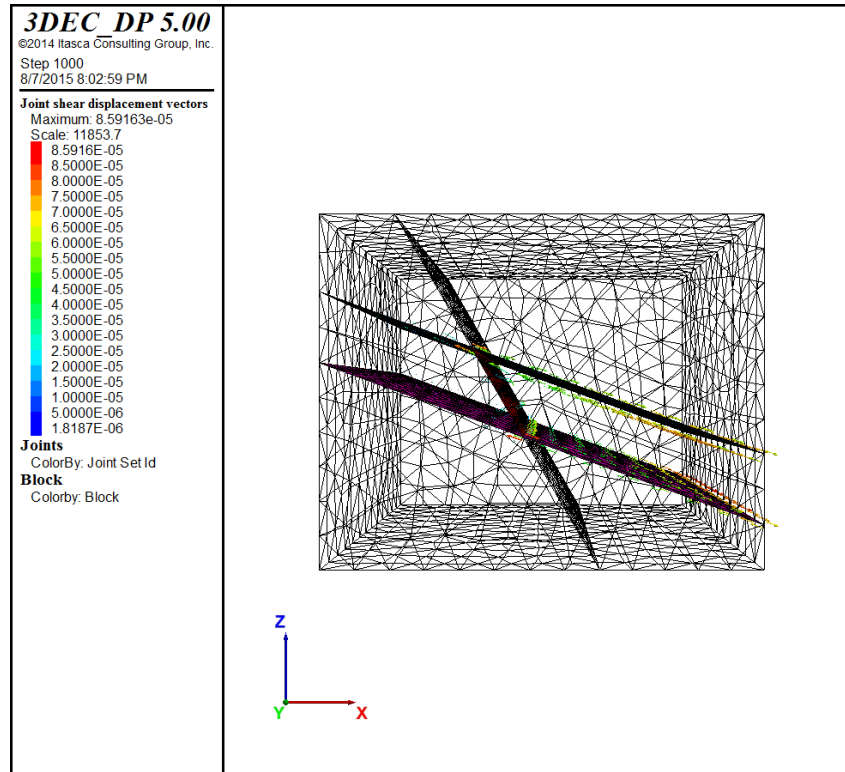
Figure 6.72 Joint shear displacement at the end of static simulation
