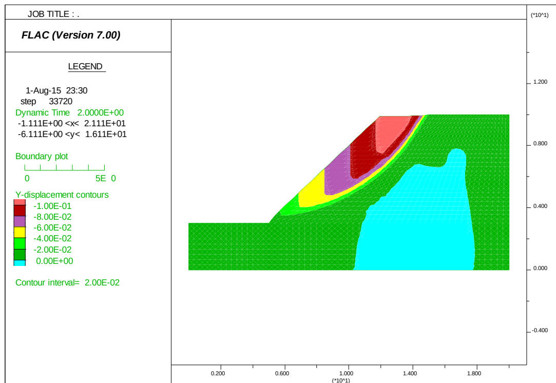
Figure 6.68 Plot of y-displacement contours
