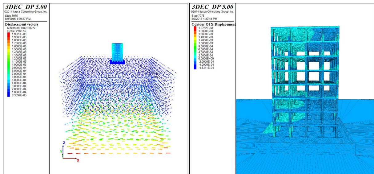
Figure 6.30 Horizontal displacement at T=0.5 sec
