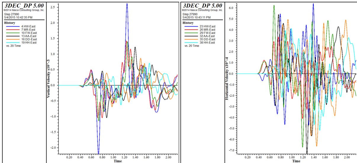
Figure 5.37 Ground motions due to fall of ground at the east of the model; Left-vertical velocity time histories, Right-horizontal velocity time histories
