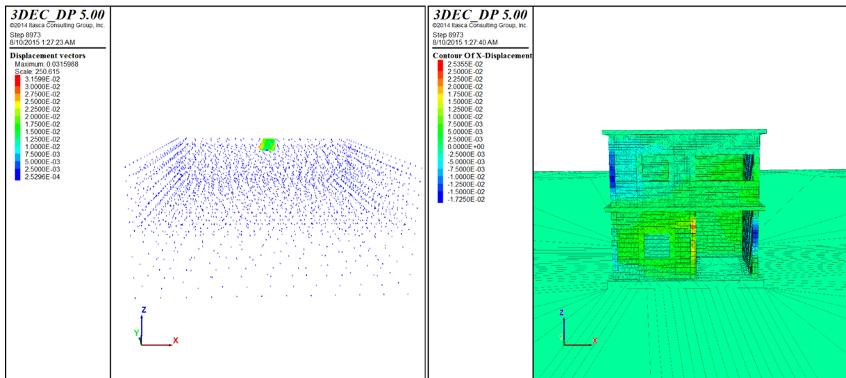
Figure 6.10 Horizontal displacement at T = 1.0 sec
