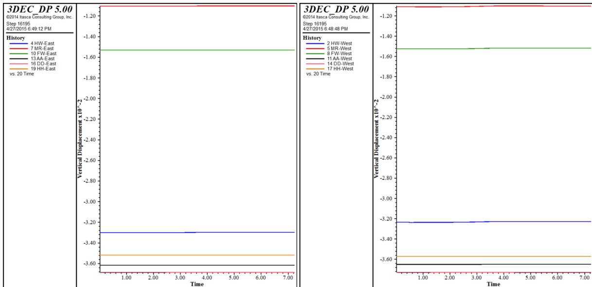
Figure 5.50 Plot of vertical displacement histories of point located on the eastern points is shown in the figure on left and western points on the right
