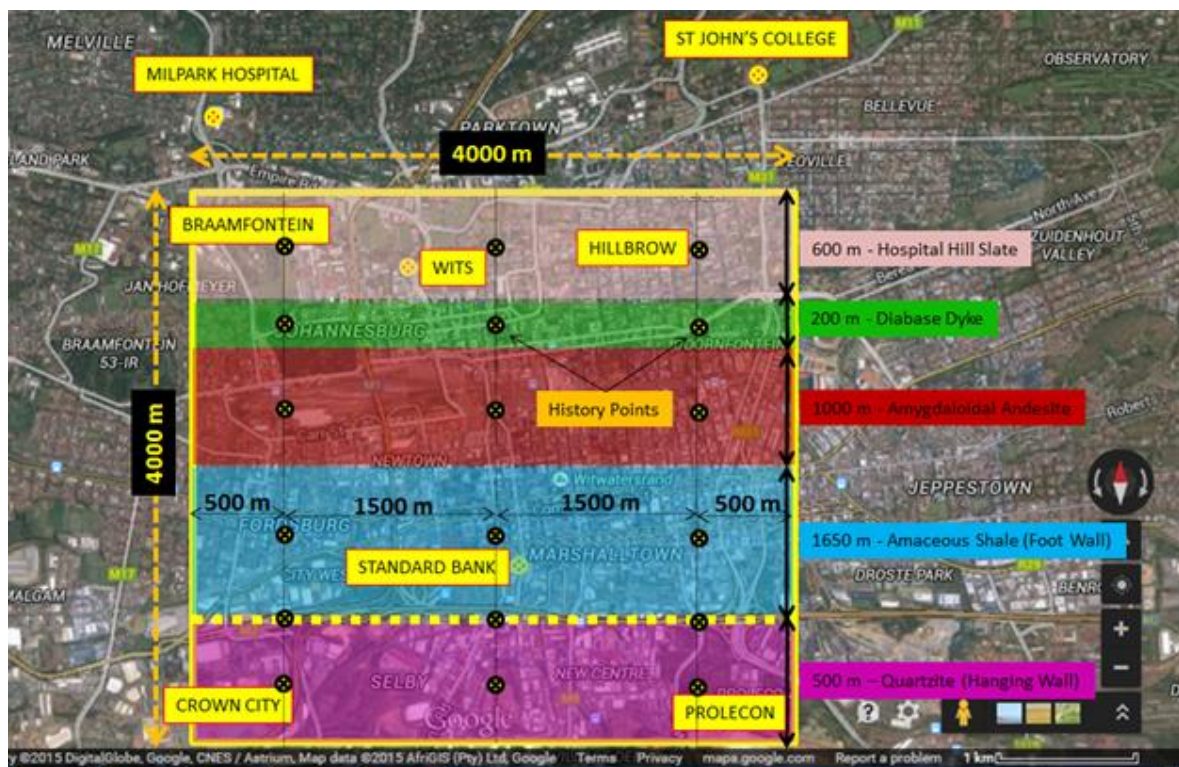
Figure 5.15 History points (black circles) at the bedrock (100 m below ground surface)
