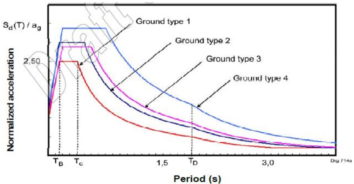
Figure 2.26 Normalized design response spectra according to SANS 10160-4:2009 (for ground type, refer o Table 2.3)
