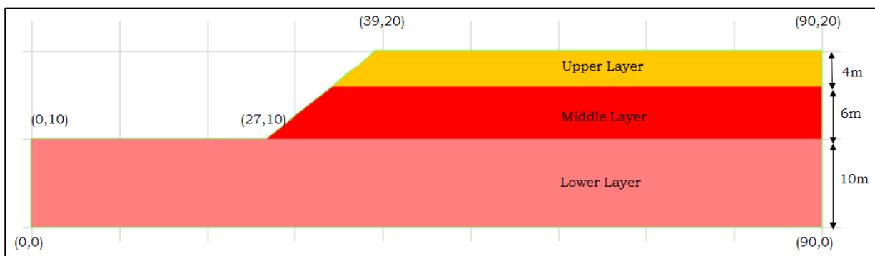
Figure 6.51 Geometry of the model
