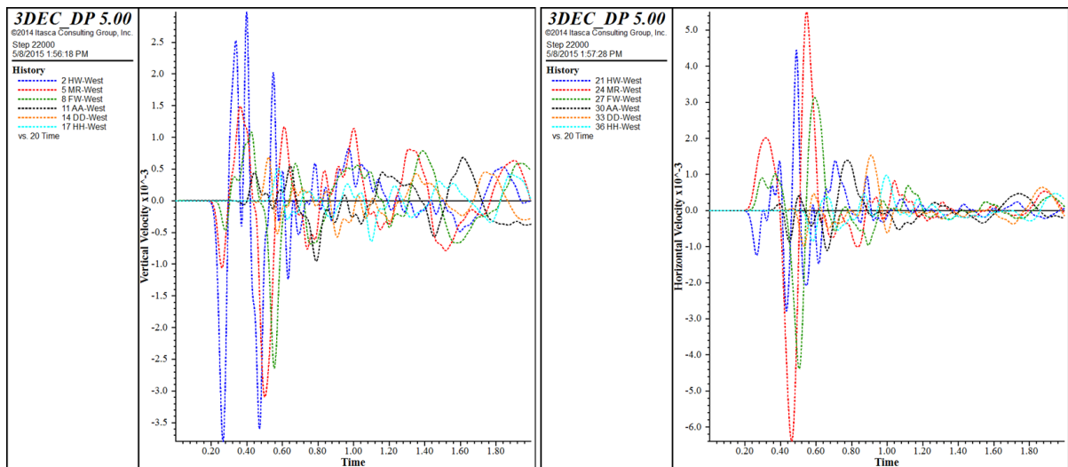
Figure 5.26 Slip along a flooded joint due to gradual rise in pore pressure, plots of velocity time histories on the west edge of model; left – vertical velocity time histories, right – horizontal velocity time histories
