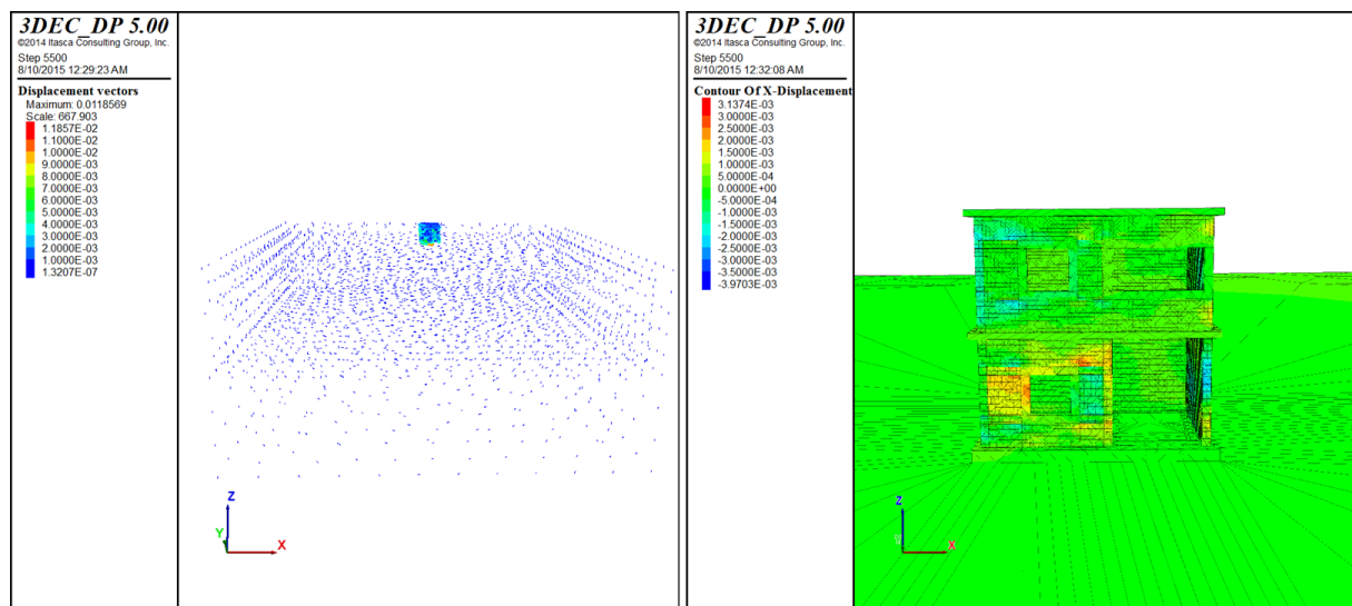
Figure 6.9 Horizontal displacement at T =0.5 sec
