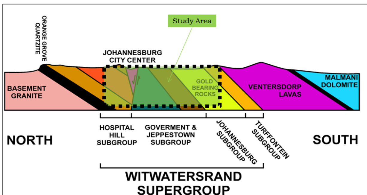
Figure 4.6 North-south cross-section through the Witwatersrand Basin beneath Johannesburg city (not to scale), after Norman and Whitfield (2006)
