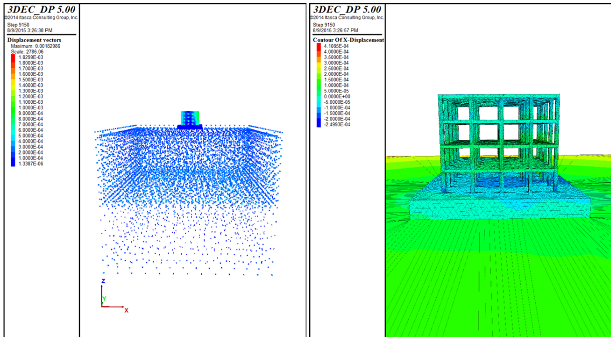
Figure 6.24 Horizontal displacement at T=1.0 sec
