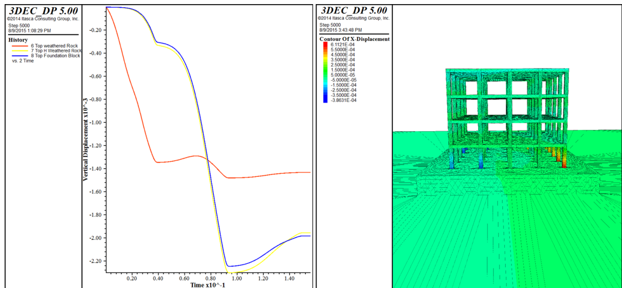
Figure 6.22 Plot of vertical displacement histories (left) and contour of horizontal displacement (right)
