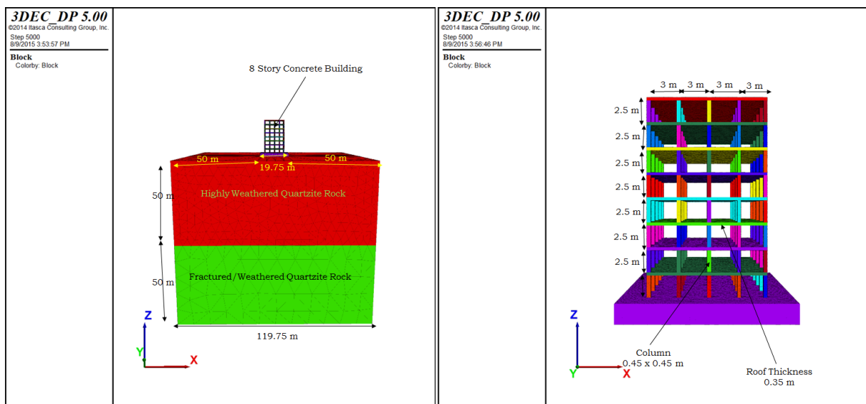
Figure 6.27 Model size and geometry of eight storey concrete building
