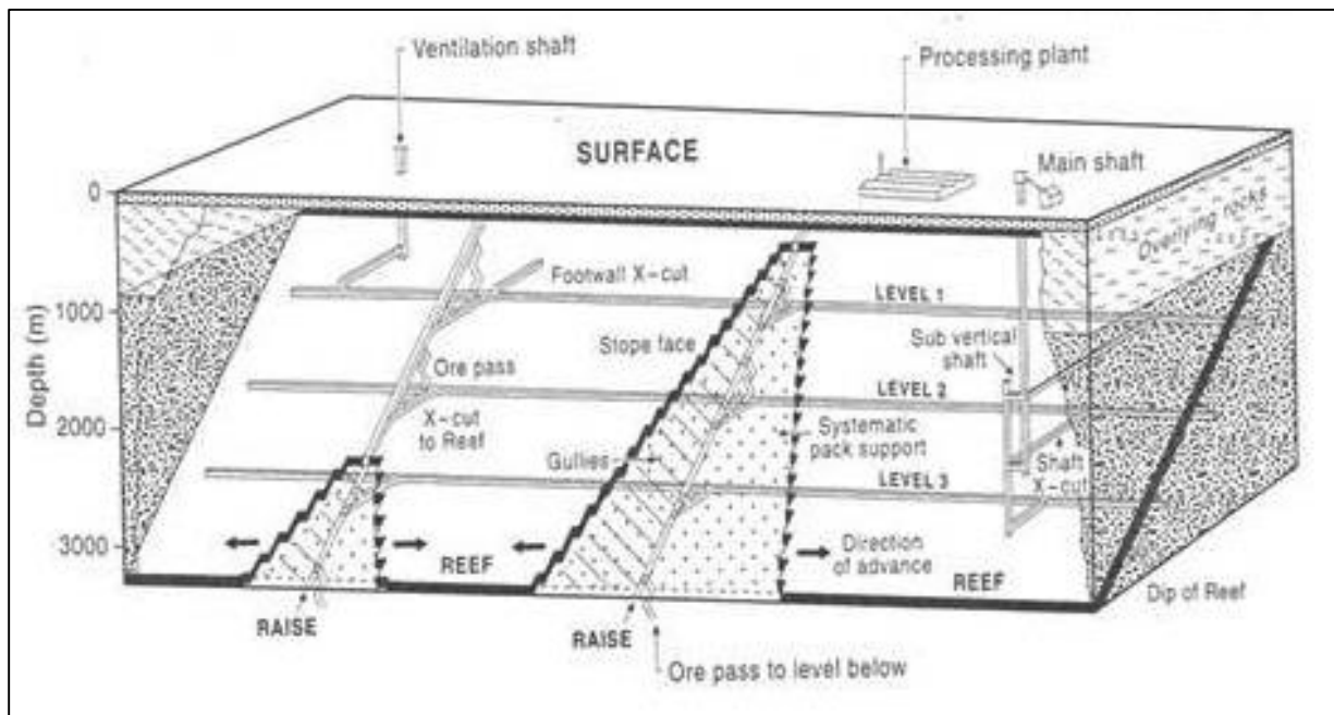
Figure 4.2 Underground mining method (breast stoping) for mining of narrow conglomerate reefs, Viljoen (2009)
