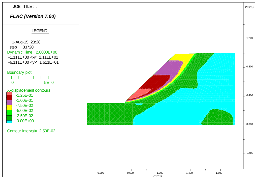
Figure 6.67 Plot of x-displacement contours
