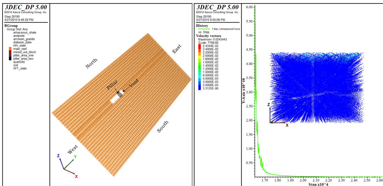
Figure 5.51 Plot on left shows excavated pillar, plot on right shows the model is critically damped
