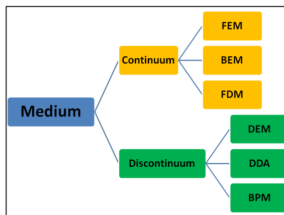
Figure 2.23 Numerical modelling techniques vis-à-vis type of medium
