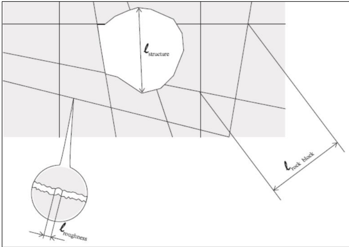
Figure 3.3 Length scales in rock mass and joint, Itasca (2014)
