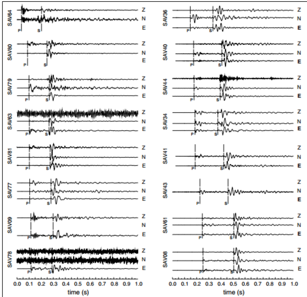
Figure 2.8 Velocity time history of a mining induced earthquake at Savuka Mine, South Africa, Julia et al. (2009)
