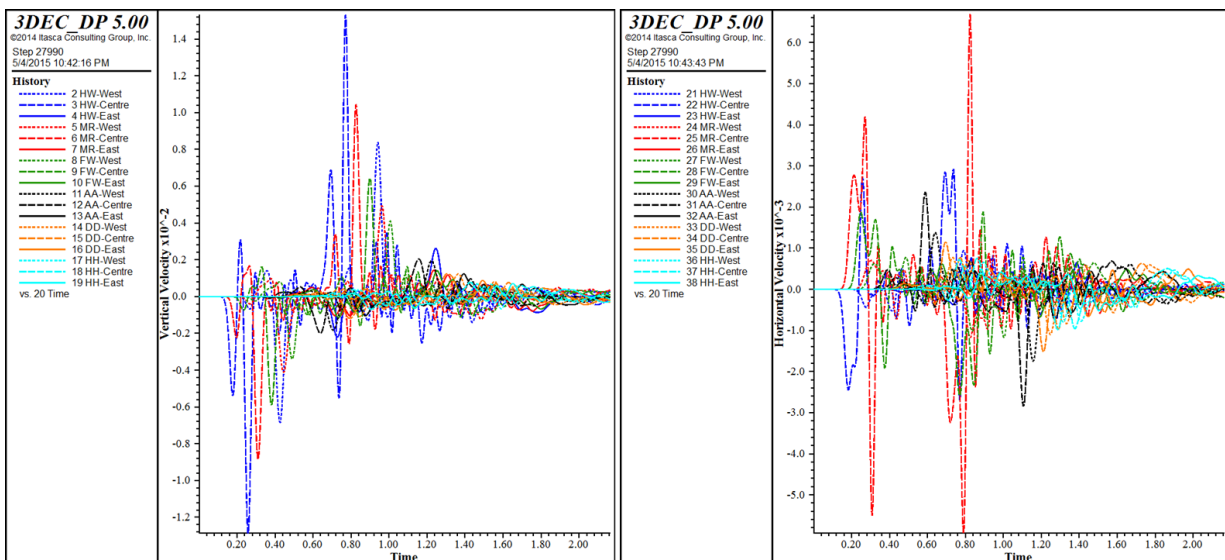
Figure 5.38 Ground motions due to fall of ground at the entire model; Left-vertical velocity time histories, Right-horizontal velocity time histories
