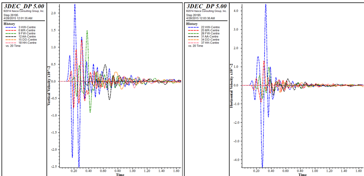
Figure 5.57 Left; vertical velocity histories, Right; horizontal velocity histories at the centre of each geological group
