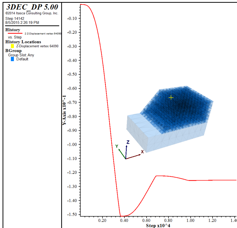
Figure 6.37 Plot of vertical displacement history of a point (shown in yellow cross) at the crest
