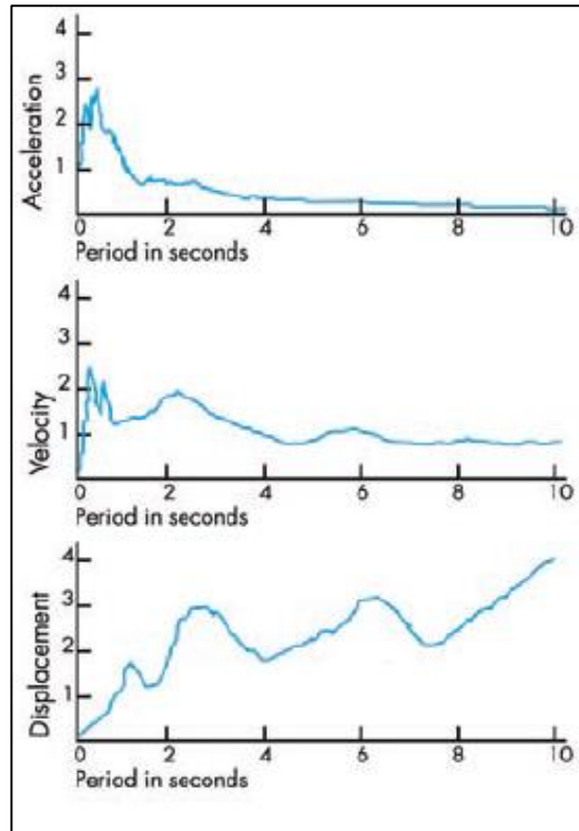
Figure 2.21 Typical response spectra, Christopher (2013)
