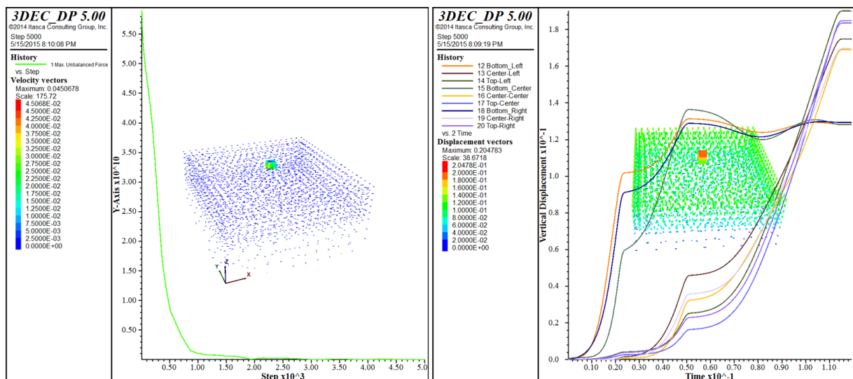
Figure 6.8 Initial equilibrium; left-plot of vertical velocity, right-plots vertical displacements
