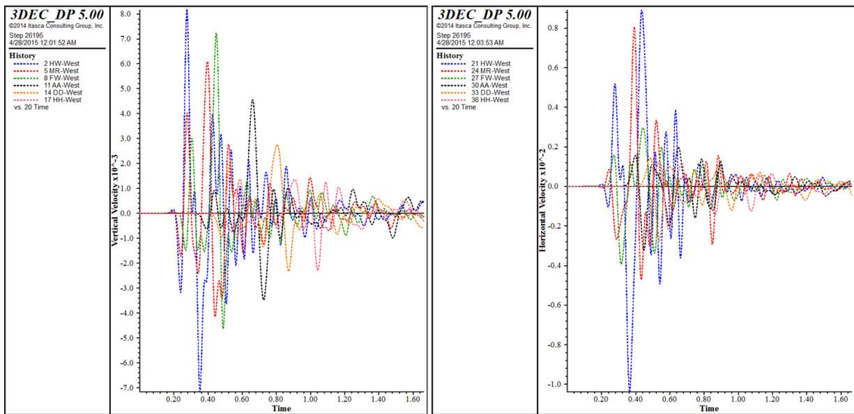
Figure 5.58 Left; vertical velocity histories, Right; horizontal velocity histories at the western edge of each geological group
