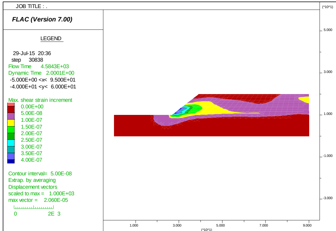
Figure 6.57 Maximum shear strain contours; damped Mohr Coulomb simulation
