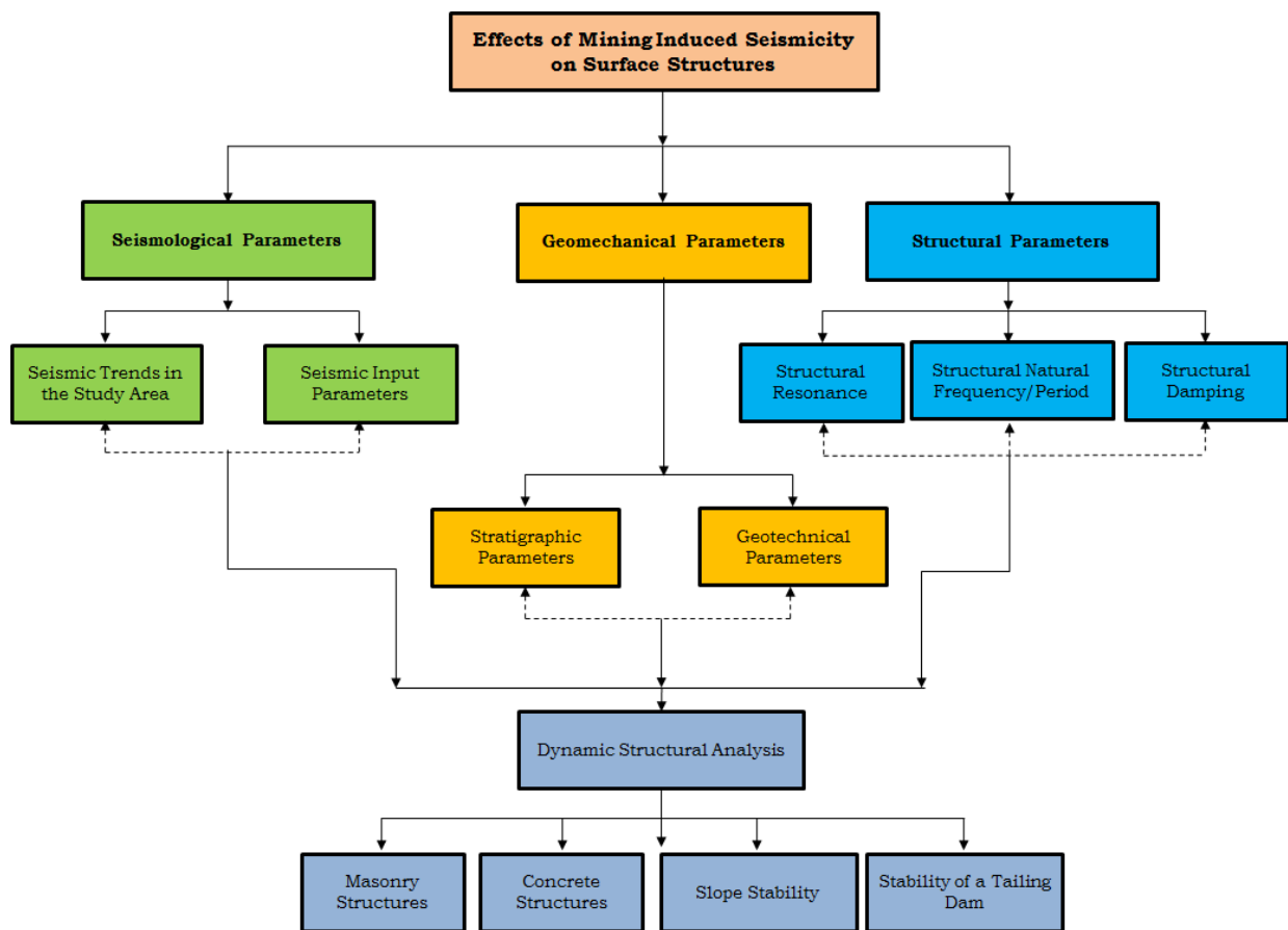
Figure 6.1 Considerations for evaluation of the effects of the mining induced seismicity on surface structures in CBD Area
