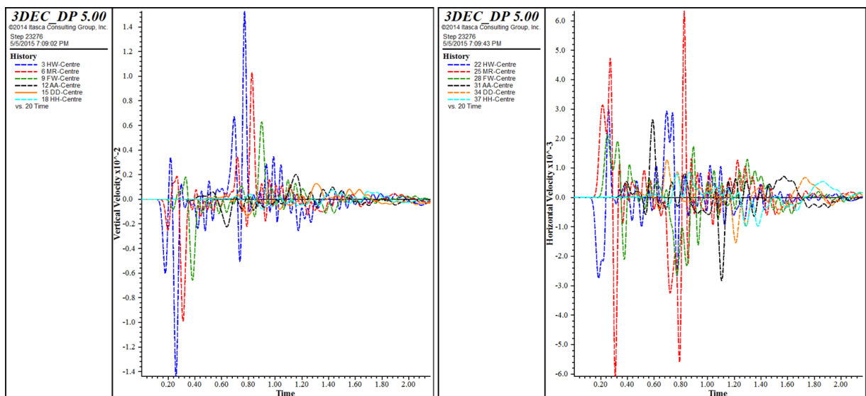
Figure 5.40 Ground motions due to fall of ground at the centre of the model; Left-vertical velocity time histories, Right-horizontal velocity time histories
