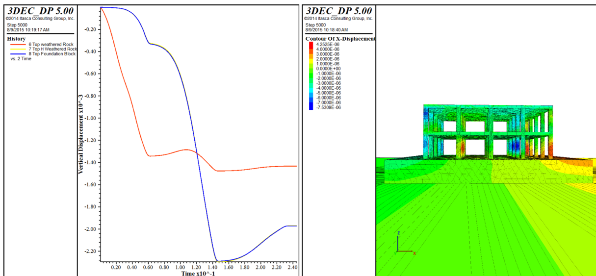
Figure 6.15 Plot of vertical displacement histories (left) and contour of horizontal displacement (right)
