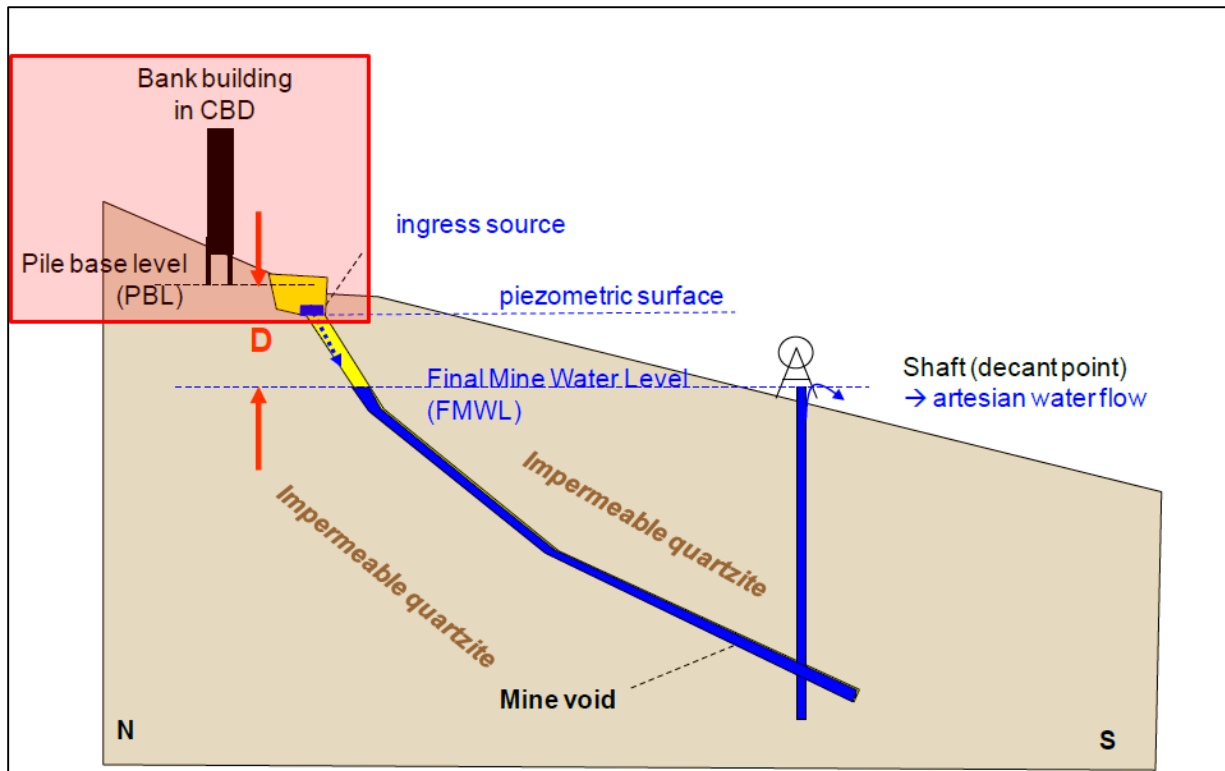
Figure 4.11 A north-south oriented idealized model (not to scale) to visualize flooding levels in abandoned mines, after Winde (2011)
