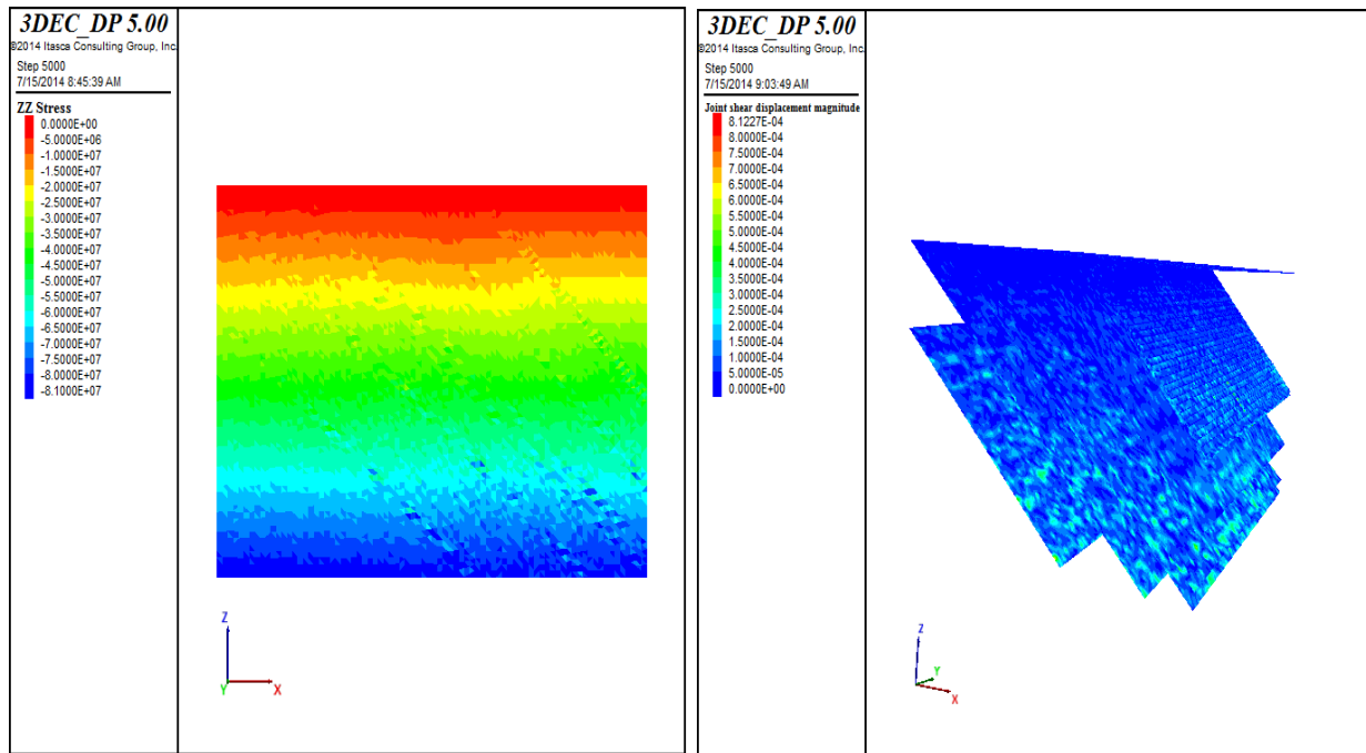
Figure 5.13 Initial Static Equilibrium; left-stress in zz-plane, Right-Joint Shear Displacement
