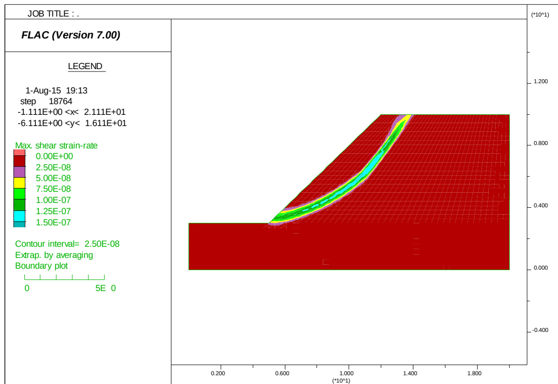
Figure 6.65 Plot of shear strain contours
