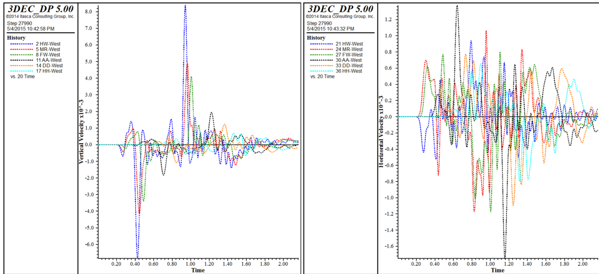
Figure 5.35 Ground motions due to fall of ground on the west edge of the model; Left-vertical velocity time histories, Right-horizontal velocity time histories
