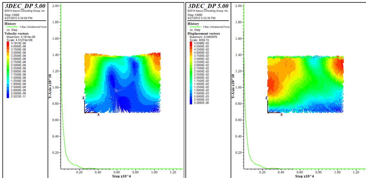
Figure 5.47 Initial static equilibrium condition of the model; left; plot of velocity vectors, right; displacement vectors
