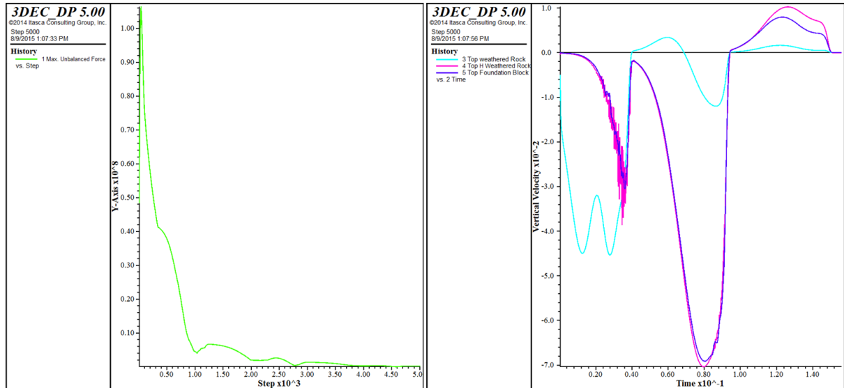
Figure 6.21 Plot of unbalanced force (left) and vertical velocity histories (right)
