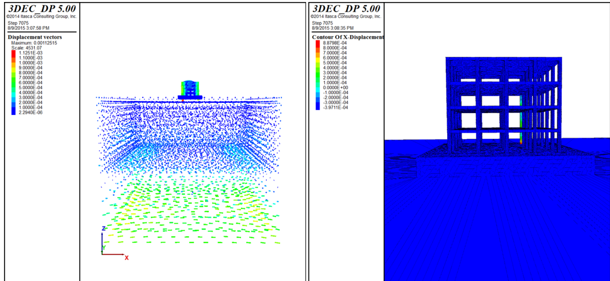
Figure 6.23 Horizontal displacement at T=0.5 sec
