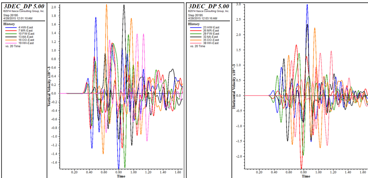
Figure 5.59 Left; vertical velocity histories, Right; horizontal velocity histories at the eastern edge of each geological group
