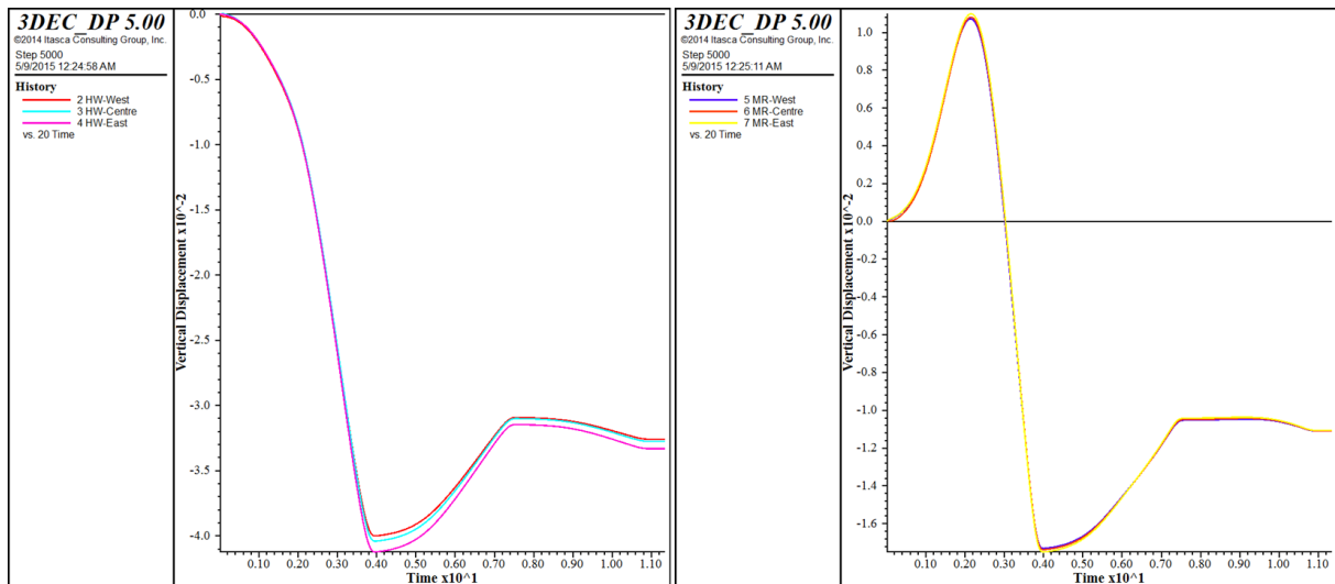
Figure 5.18 Initial static equilibrium; left – plot of vertical displacement histories in Hanging Wall, right – plot of vertical displacement histories in Main Reef
