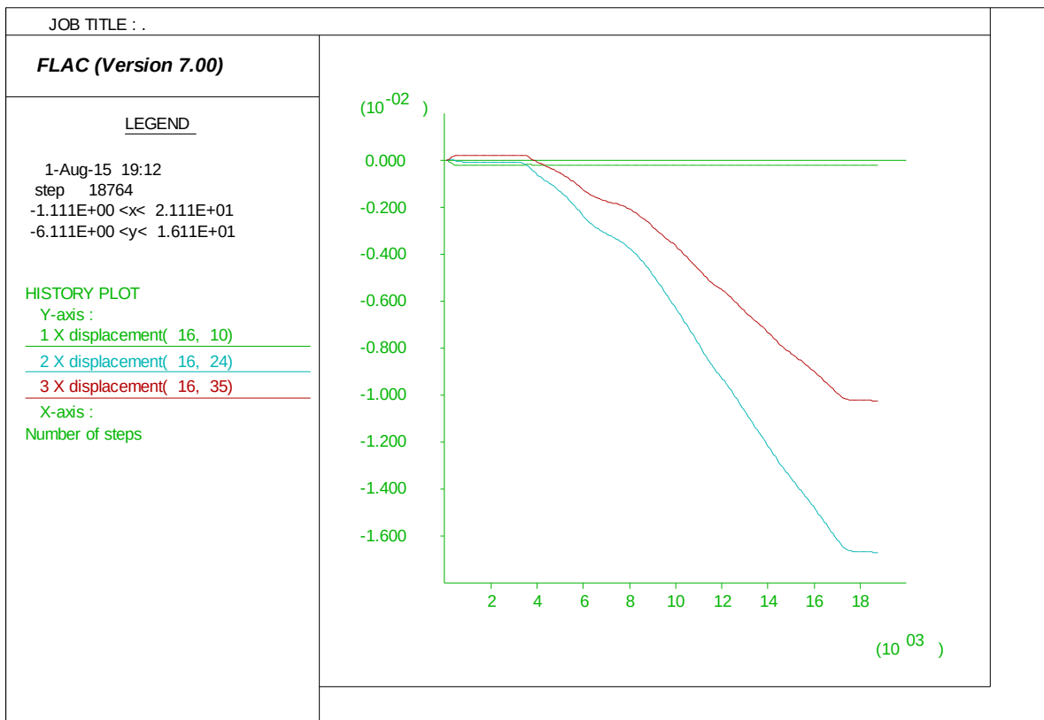
Figure 6.64 Plot of x-displacement histories
