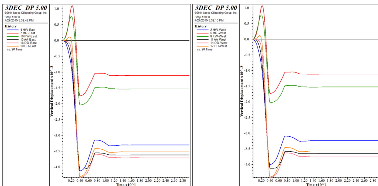
Figure 5.46 Initial static equilibrium condition of the model; left; plot of vertical displacement histories on eastern points, right; vertical displacement histories at the western points on the model
