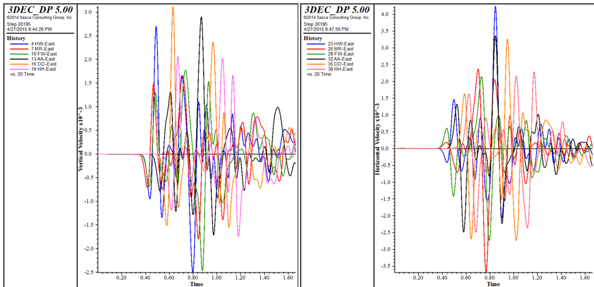
Figure 5.54 Left; vertical velocity histories, Right; horizontal velocity histories at the eastern edge of each geological group
