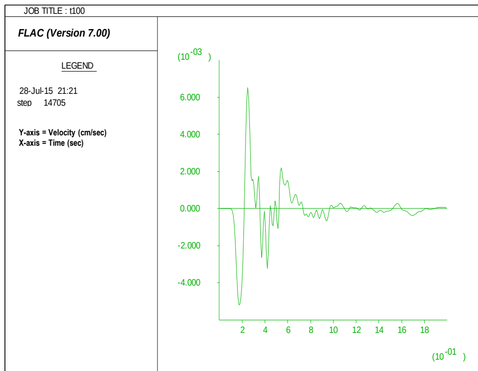
Figure 6.55 Input ground motion (velocity time history)
