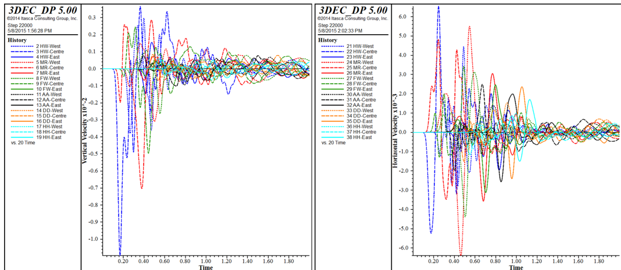
Figure 5.29 Slip along a flooded joint due to gradual rise in pore pressure, plots of velocity time histories on the entire model; left – vertical velocity time histories, right –horizontal velocity time histories
