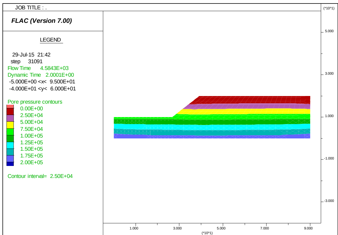
Figure 6.59 Pore-pressure contours; gradual gradients show no signs of plastic deformation/liquefaction
