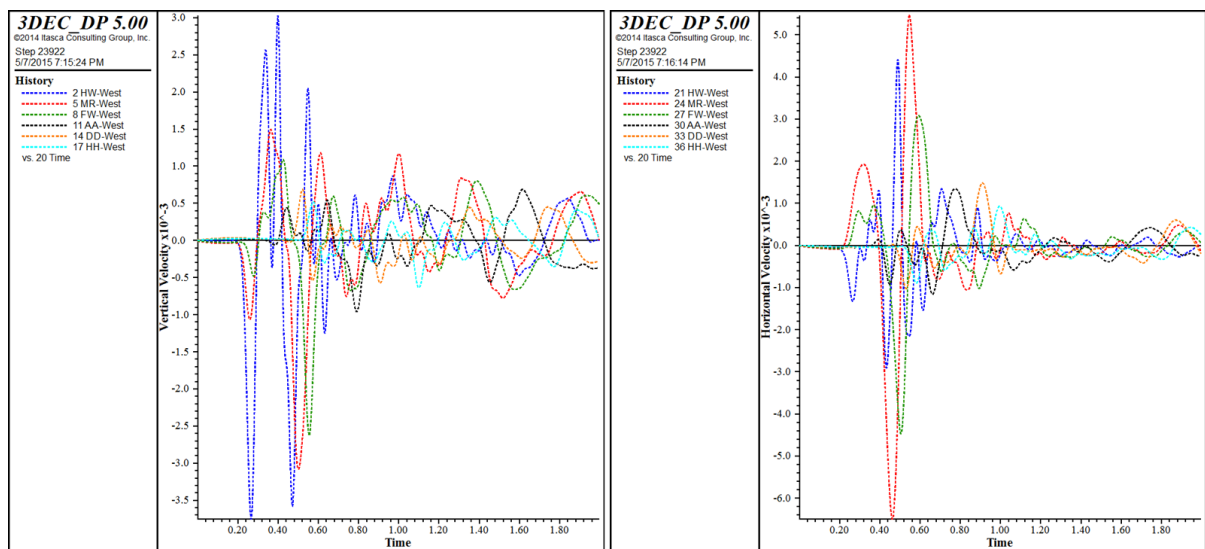
Figure 5.21 Slip along a dry joint, plots of velocity time histories on the west edge of model; left – vertical velocity time histories, right –horizontal velocity time histories
