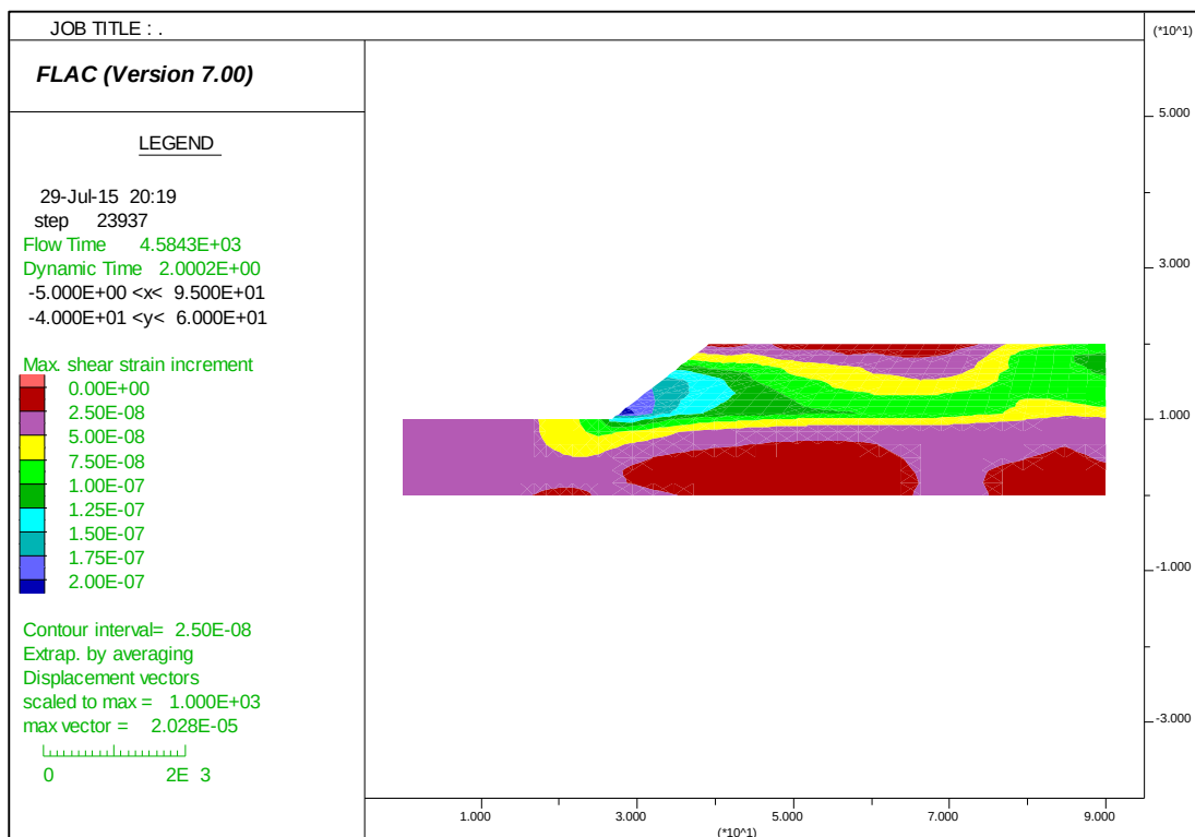
Figure 6.56 Maximum shear strain contours during un-damped and elastic material
