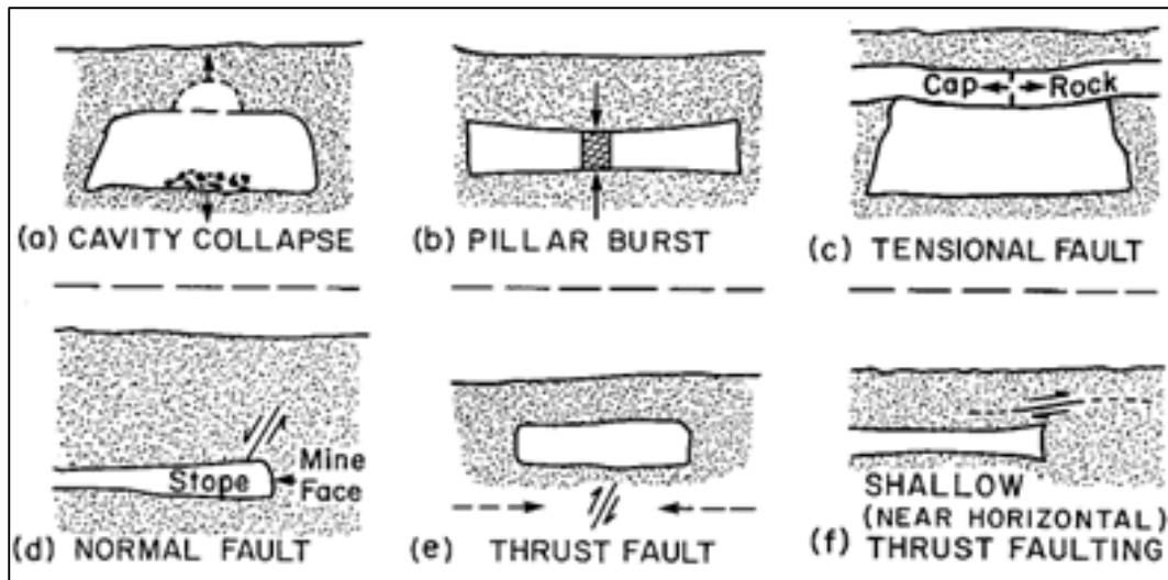
Figure 2.7 Mechanism for mining seismicity, Hasegawa et al., (1989)
