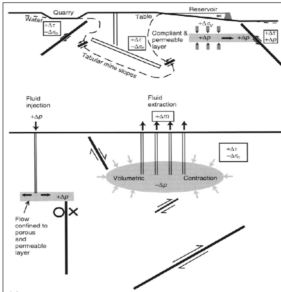
Figure 2.6 Sources of induced seismicity; changes in shear stress ( \Delta\tau ), pore pressure ( \Delta p ), volume change ( \Delta v ) and applied forces ( \Delta n ), McGarr et al. (2002)
