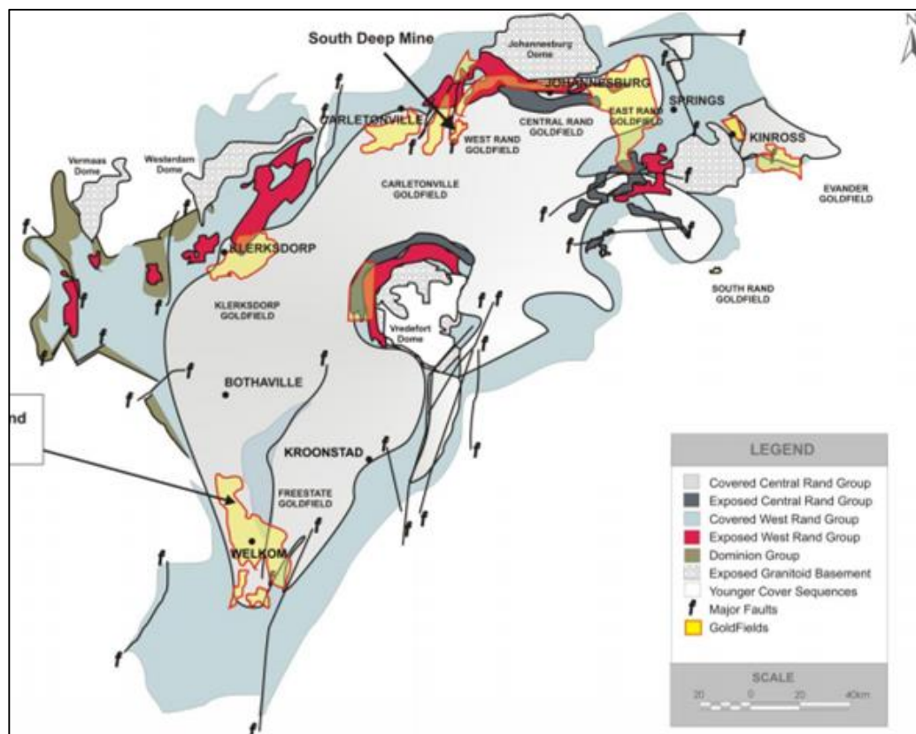
Figure 2.2 Witwatersrand Basin, Randgold (2010)
