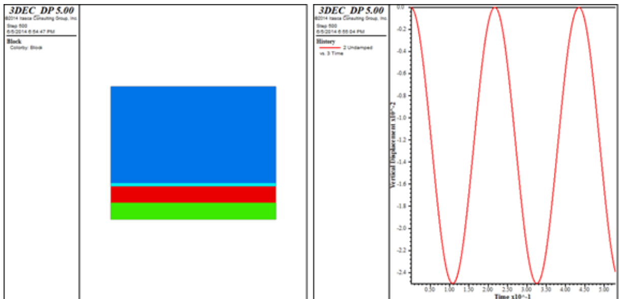
Figure 5.7 Seismic waveform with three discontinuities (frequency = 0.30 Hz, amplitude = 2.5 cm)
