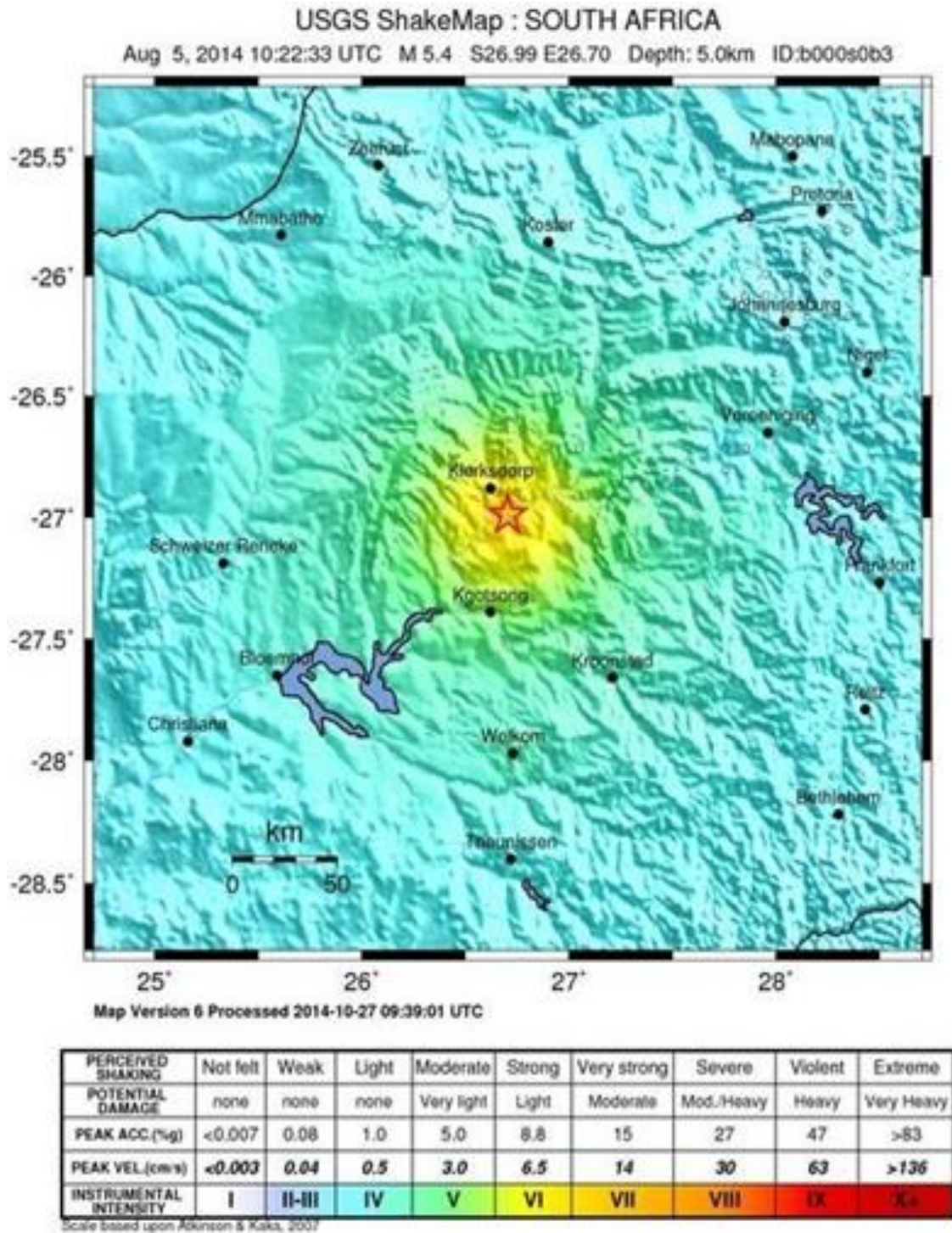
Figure 2.17 Shake map of 5 August 2014, Orkney seismic event, USGS (2014)
