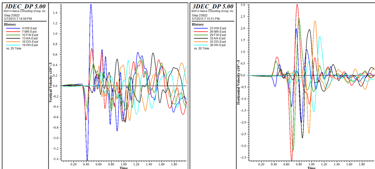
Figure 5.23 Slip along a dry joint, plots of velocity time histories on east edge of the model; left – vertical velocity time histories, right –horizontal velocity time histories
