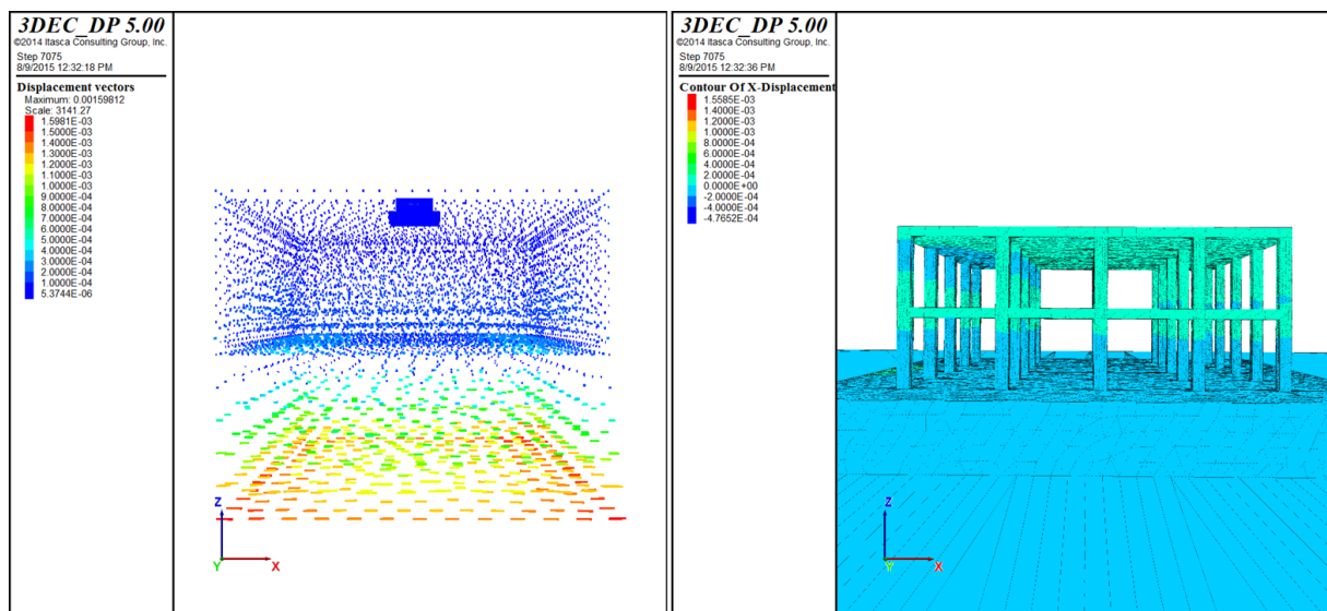
Figure 6.16 Horizontal displacement at T = 0.5 sec
