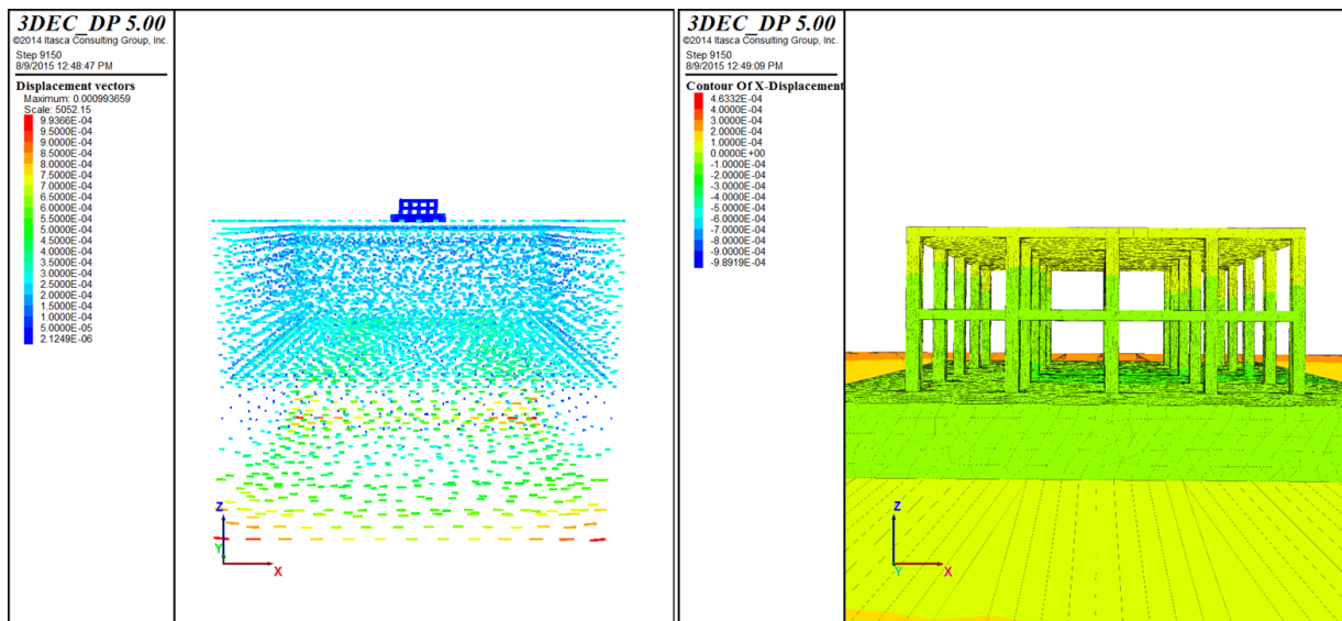
Figure 6.17 Horizontal displacement at T = 1.0 sec
