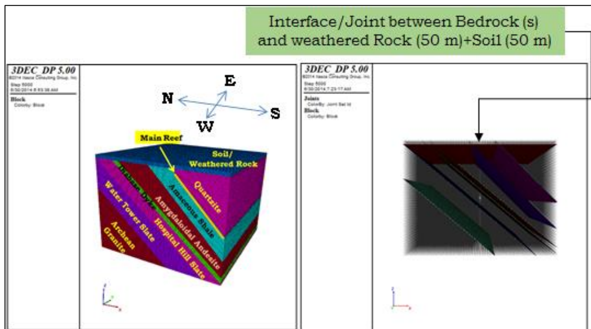
Figure 4.14 Left; stratigraphy (layering) of material, Right; orientation of joints
