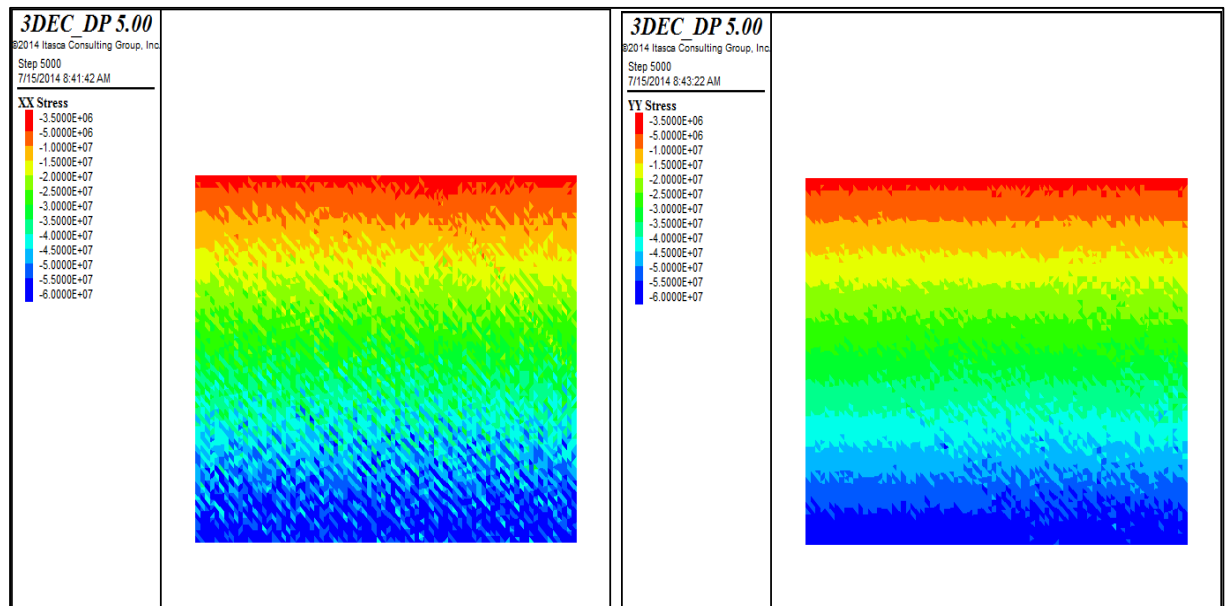
Figure 5.12 Initial Static Equilibrium; left-stress in xx-plane, Right-Stress in yy-plane
