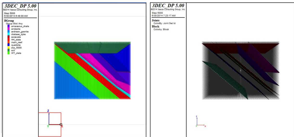
Figure 5.4 Material Groups (left) and Geological Discontinuities (right) (labelling shown in Figure 5.3 (right) holds good for the left figure as well)
