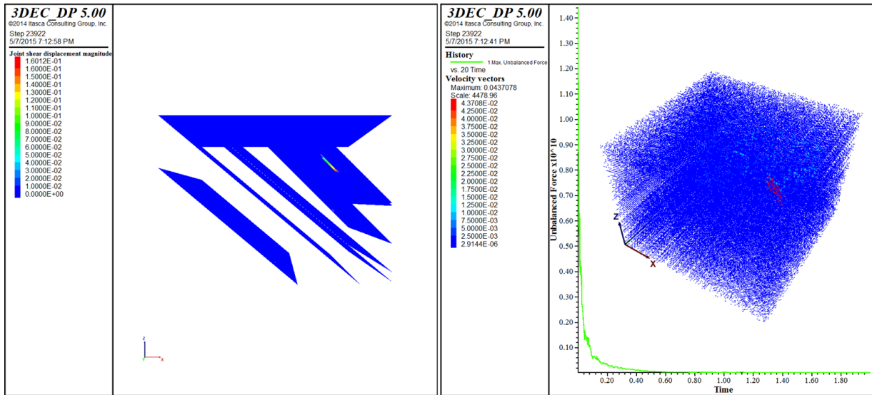
Figure 5.20 Slip along a dry joint; left – plot of joint shear displacement, right – plot of unbalanced force and velocity vectors
