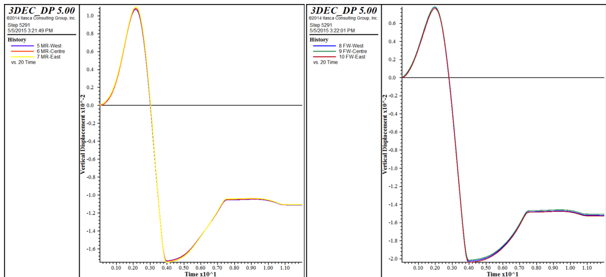
Figure 5.31 Static equilibrium; left-plot of vertical displacement histories in Main Reef, right-plot of vertical displacement histories in Foot Wall
