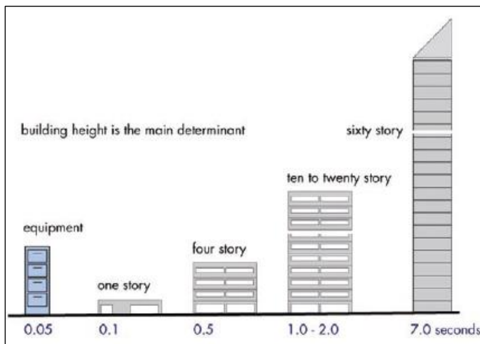
Figure 2.19 Natural period of various structures, Christopher (2013)
