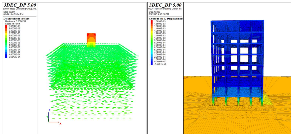
Figure 6.33 Horizontal displacement at T =2.0 sec
