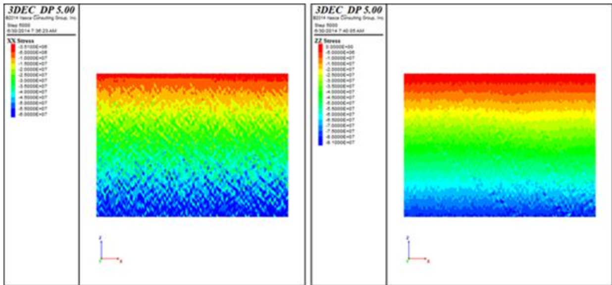
Figure 5.9 Insitu stresses initialized in the 3DEC model
