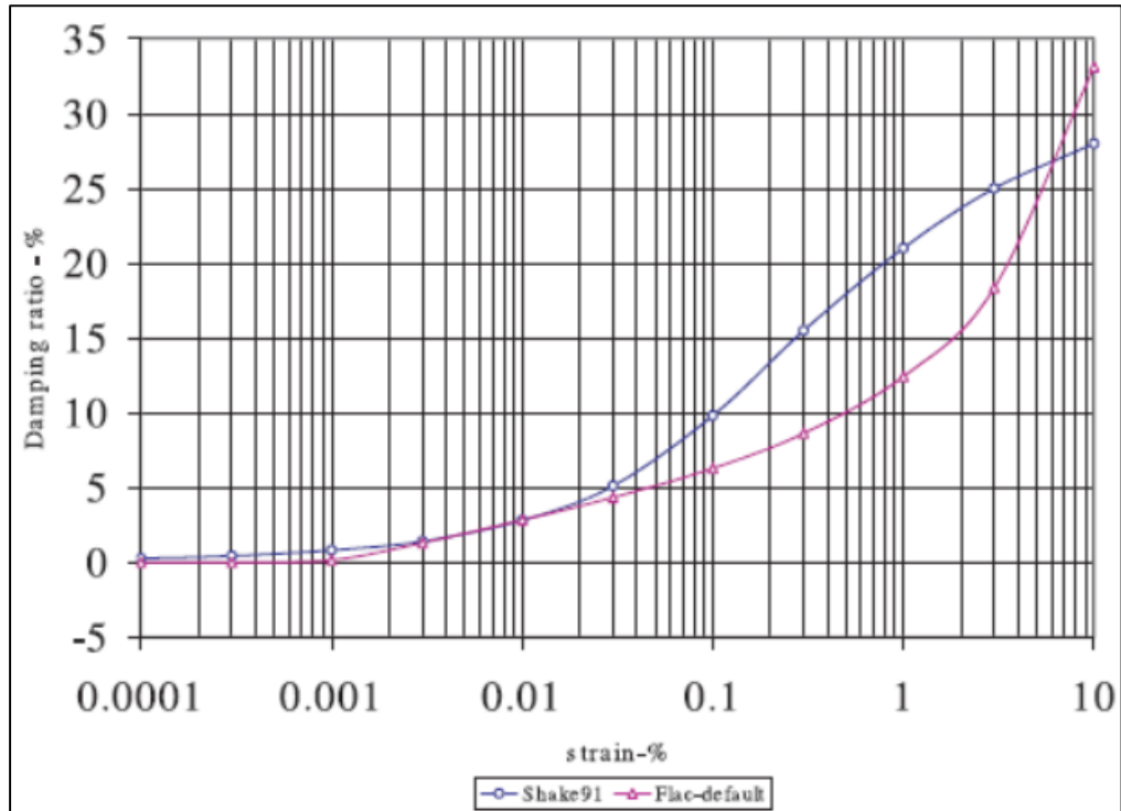
Figure 3.10 Damping ratio curve for clayey soil (FLAC default hysteric damping with L_1 = -3.156 , L_2 = 1.904 ), Itasca (2014)
