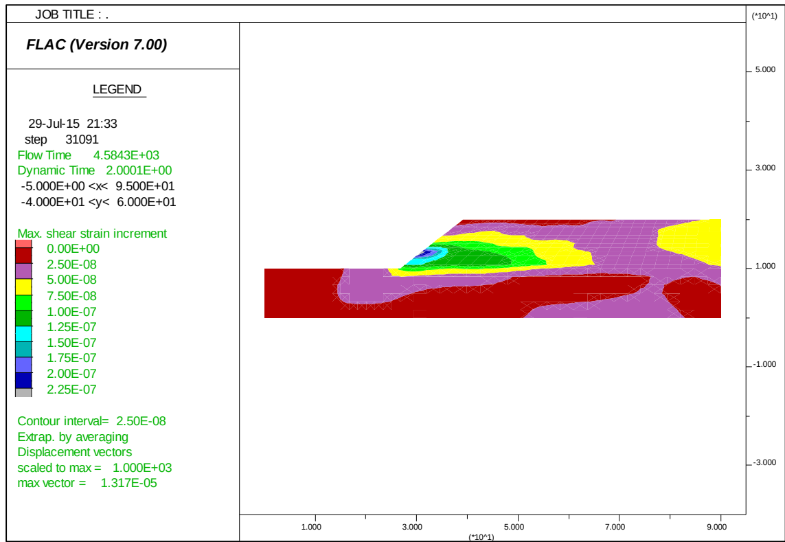
Figure 6.58 Maximum shear strain contours; damped Finn-Byrne model
