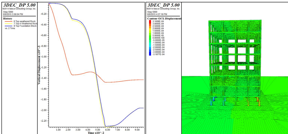
Figure 6.29 Plot of vertical displacement histories (left) and contour of horizontal displacement (right)
