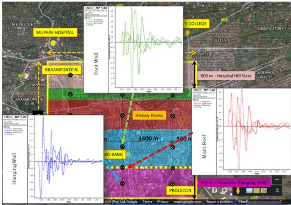
Figure 6.3 Ground motions estimated at Hanging Wall, Main Reef and Foot Wall
