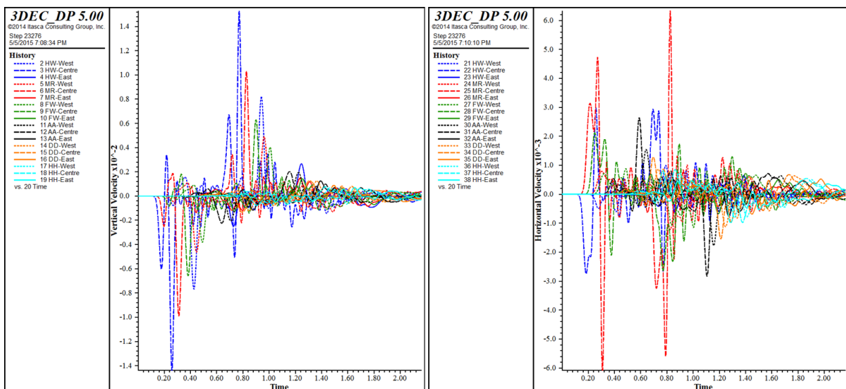
Figure 5.42 Ground motions due to fall of ground at the entire model; Left- vertical velocity time histories, Right-horizontal velocity time histories
