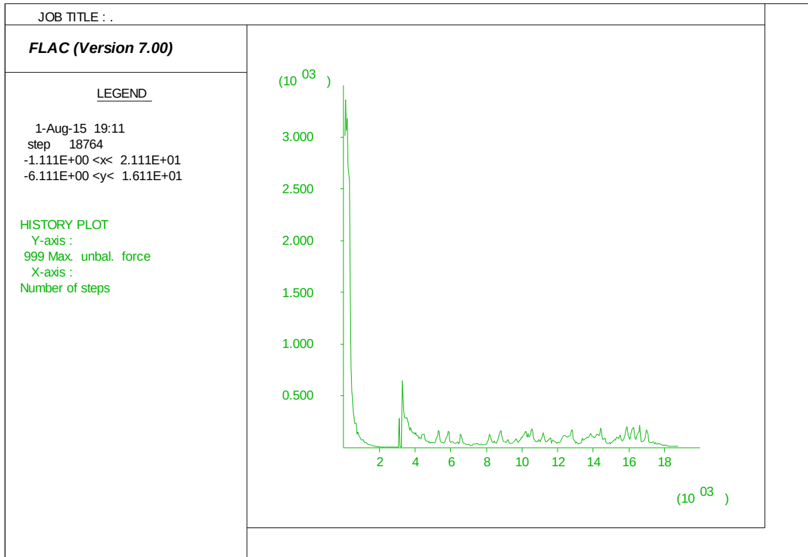
Figure 6.63 Plot of unbalanced force
