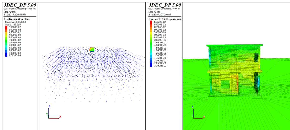
Figure 6.11 Horizontal displacement at T = 1.5 sec
