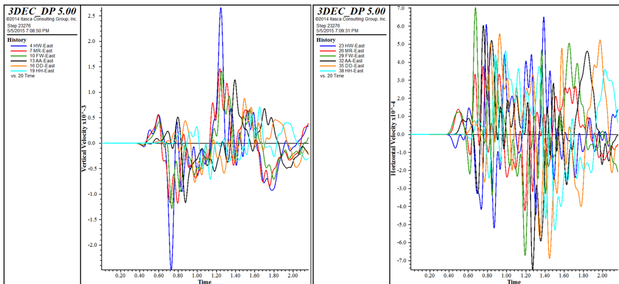
Figure 5.41 Ground motions due to fall of ground at the east of the model; Left-vertical velocity time histories, Right-horizontal velocity time histories
