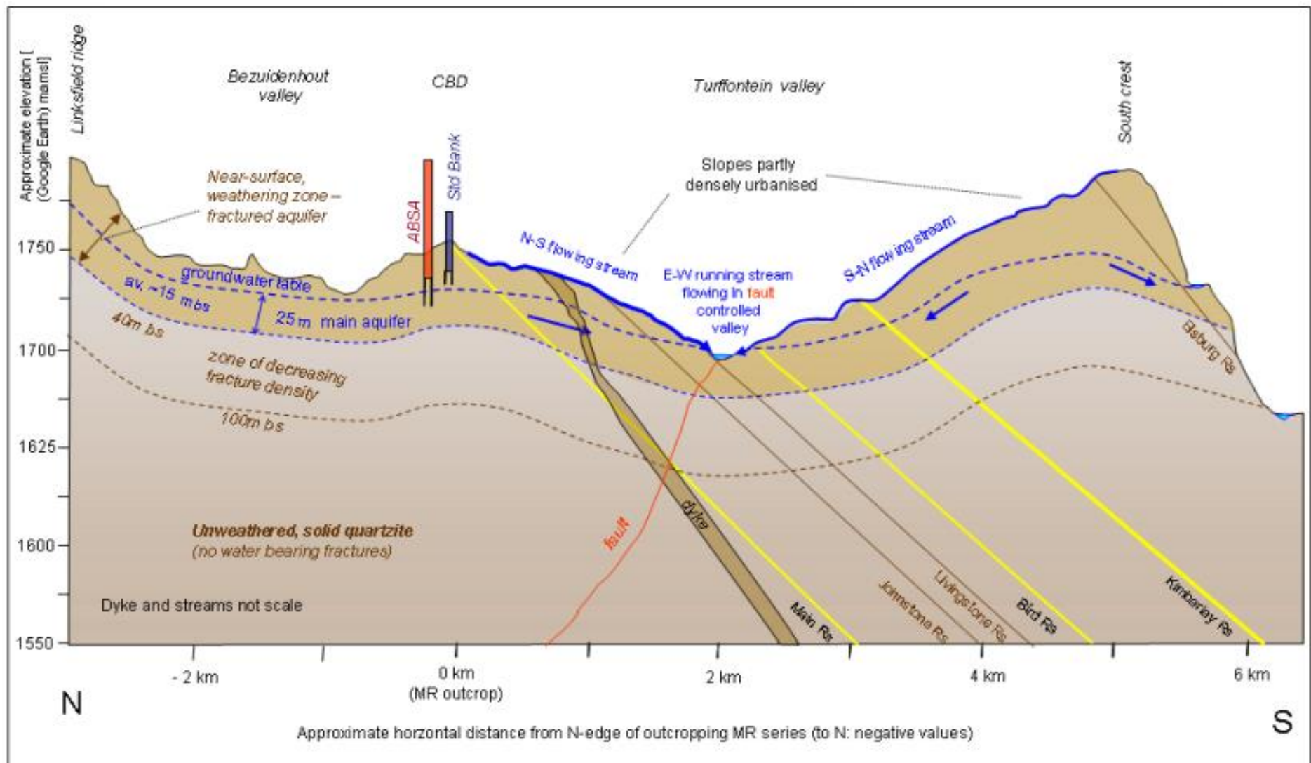
Figure 4.13 Post mining geological and geohydrological conditions in the central part of the Central Rand, Winde (2011)
