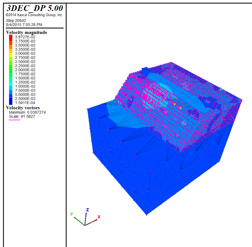
Figure 6.45 Displacement contours and vectors at 1.5 sec duration
