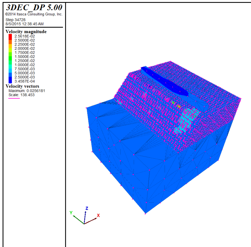
Figure 6.48 Velocity contours and vectors at 2.0 sec duration
