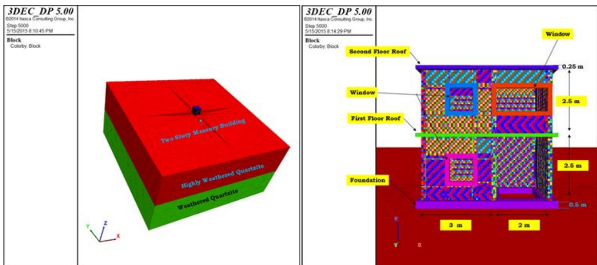
Figure 6.6 Model Geometry; left-foundation ground (quartzite rock), right-geometry and layout of two storey masonry building
