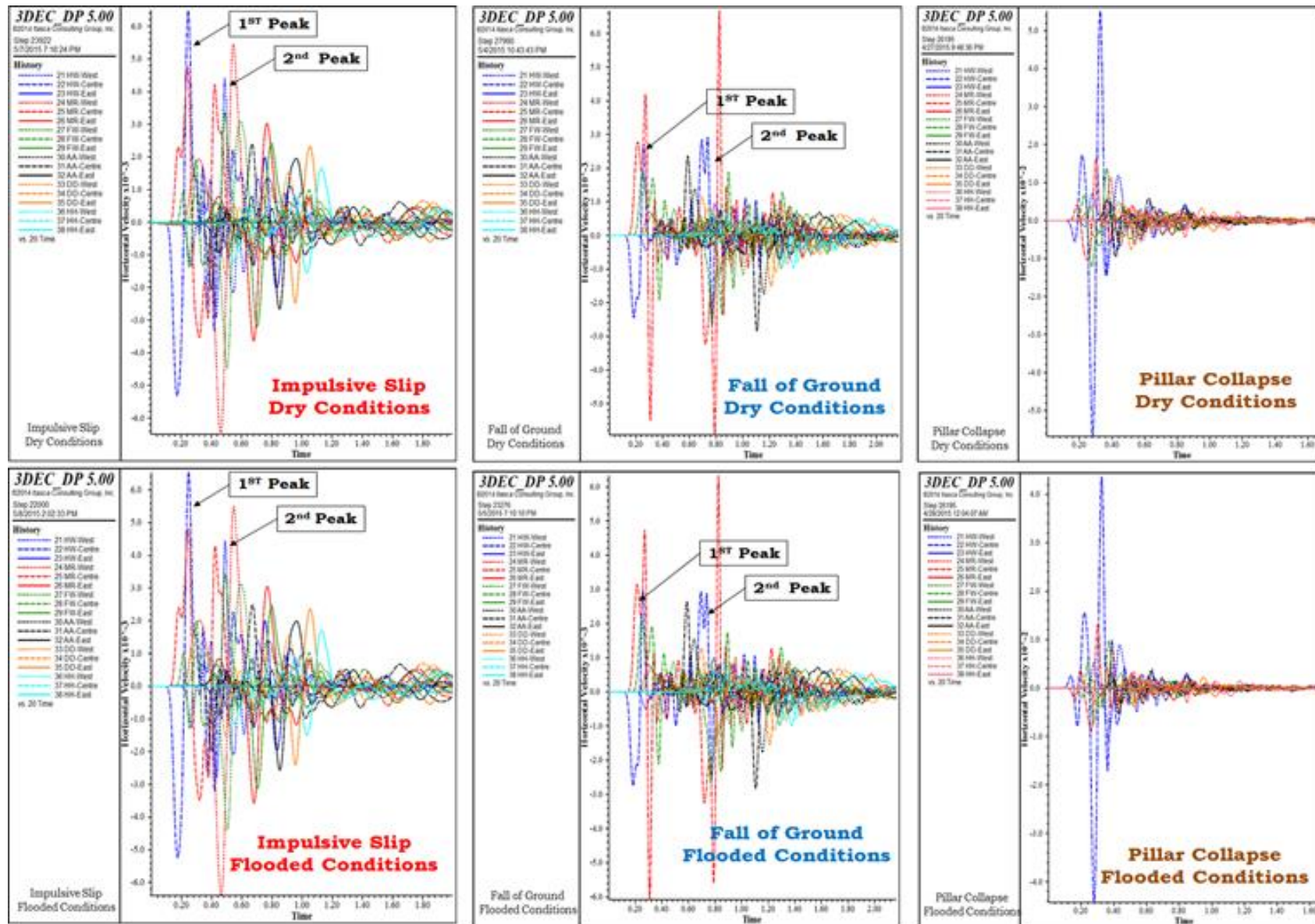
Figure 6.2 Ground motions in terms of horizontal velocity time histories in dry and flooded condition
