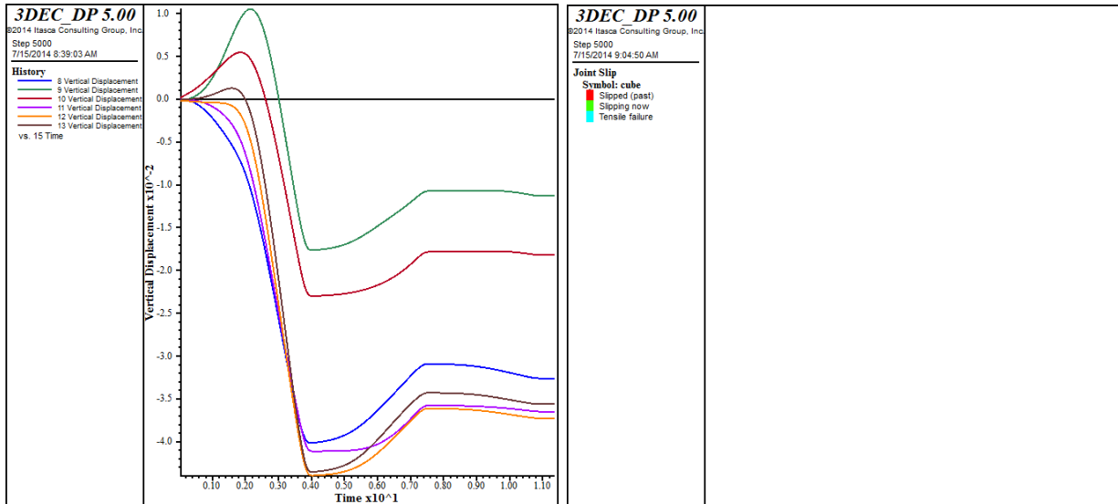
Figure 5.11 Initial Static Equilibrium; left-Vertical Displacement Histories, Right-Joint Slip (no joint slip observed)
