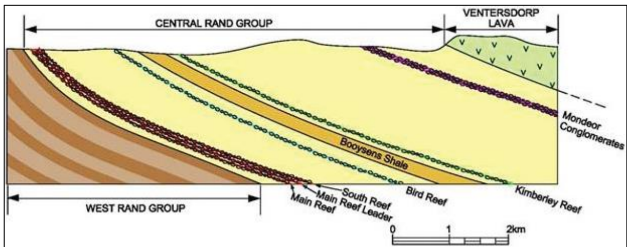
Figure 4.1 Gold bearing conglomerate reefs of the Central Rand Group, Superior Mining (2013)
