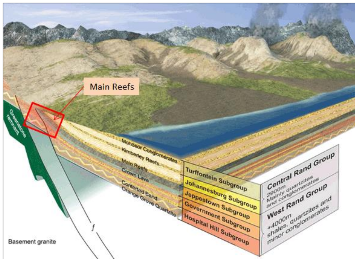
Figure 4.5 Generalized geological model of the study area (not to scale), after Gold Fields (2013)
