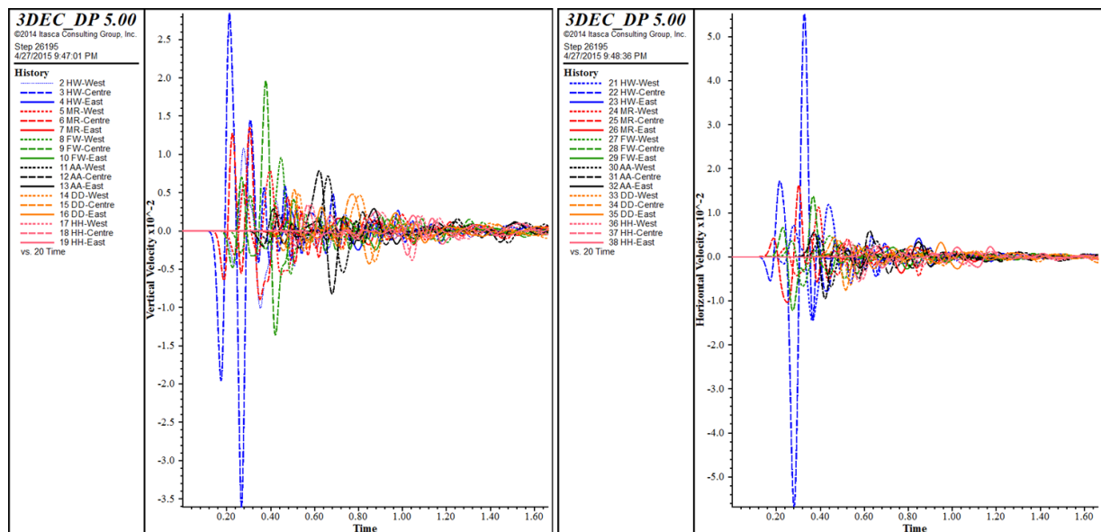
Figure 5.55 Left; all vertical velocity histories, Right; all horizontal velocity histories
