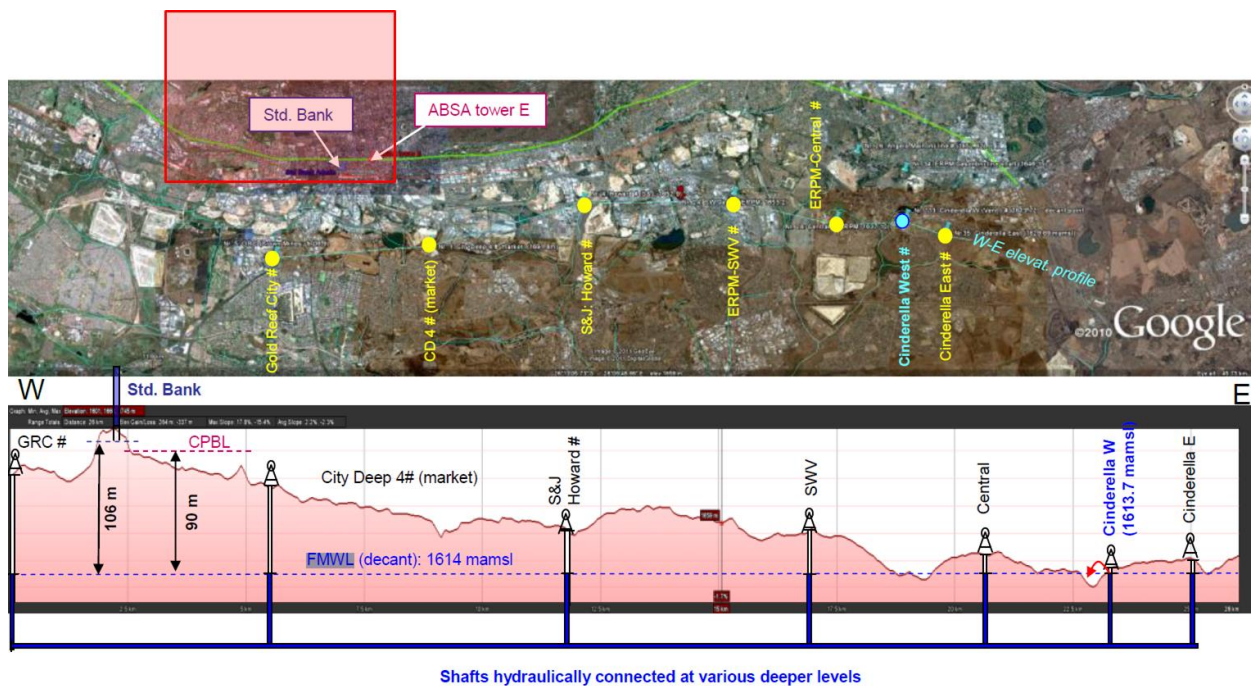
Figure 4.12 An east-west oriented profile (not to scale) showing Final Mine Water Level indicating a safety margin of 106 m below the Standard Bank building, after Winde (2011)
