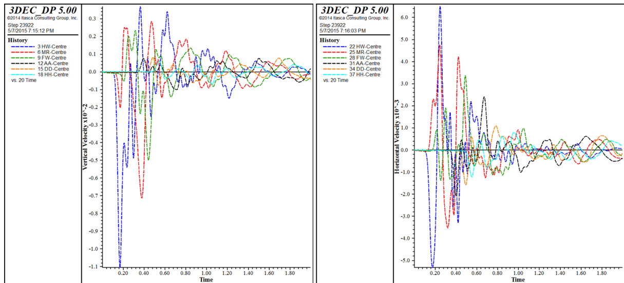
Figure 5.22 Slip along a dry joint, plots of velocity time histories on centre of the model; left – vertical velocity time histories, right –horizontal velocity time histories
