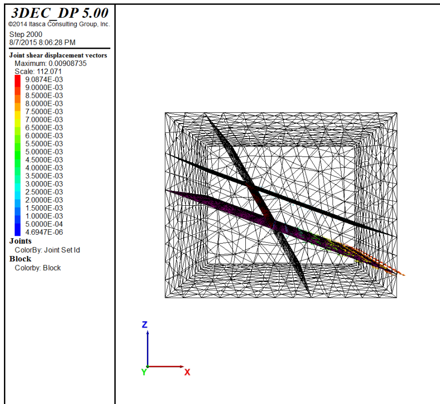
Figure 6.73 Joint shear displacement at the end of the dynamic simulation
