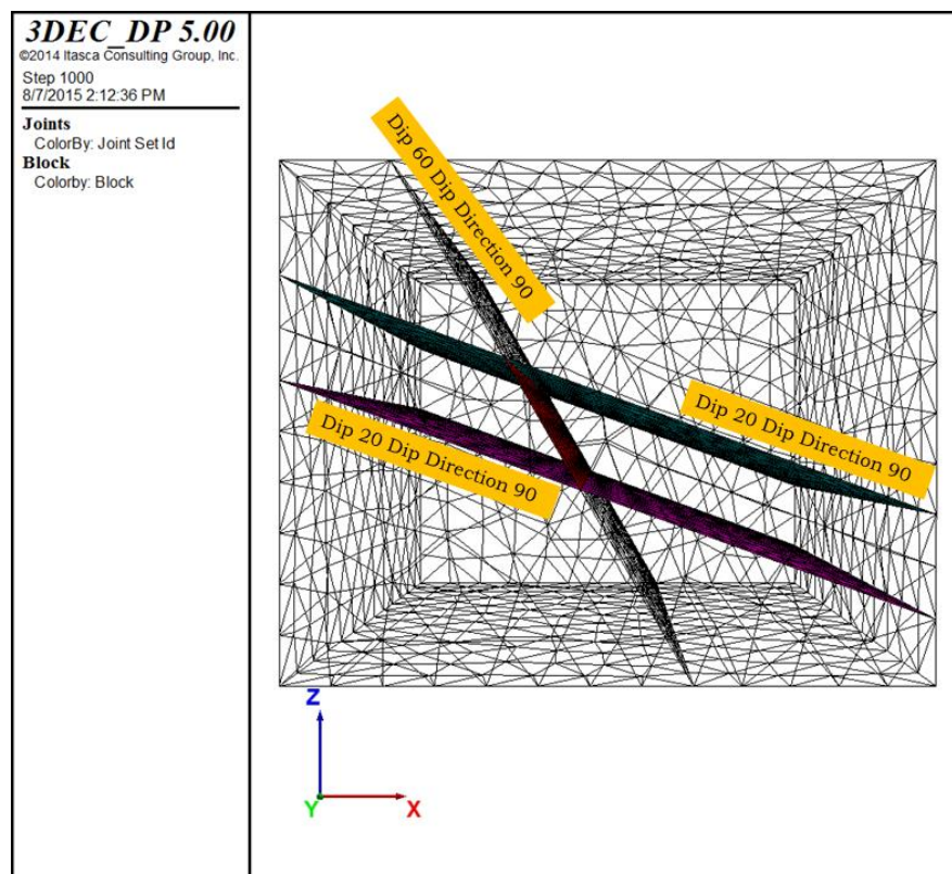
Figure 6.71 Location and orientation of the joints
