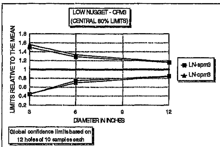
Figure 5.9: Low nugget effect model showing the central 80% confidence limits in SPM3 and CPM3 for a three, size and twelve inch diameter sample. All samples are 12m in length.
