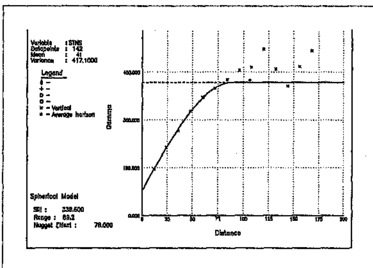
Figure 4.2: Semi-variogram of Deposit one.
