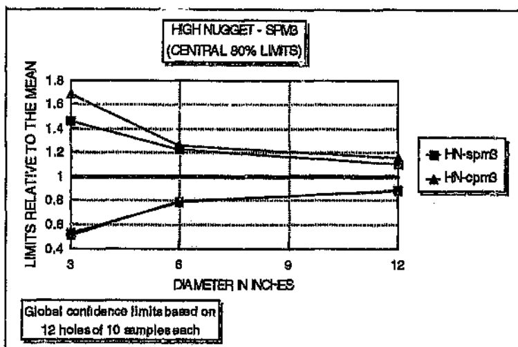
Figure 5.8: High nugget effect model showing the central 80% confidence limits in SPM3 and CPM3 for a three, size and twelve inch diameter sample. All samples are 12m in length.
