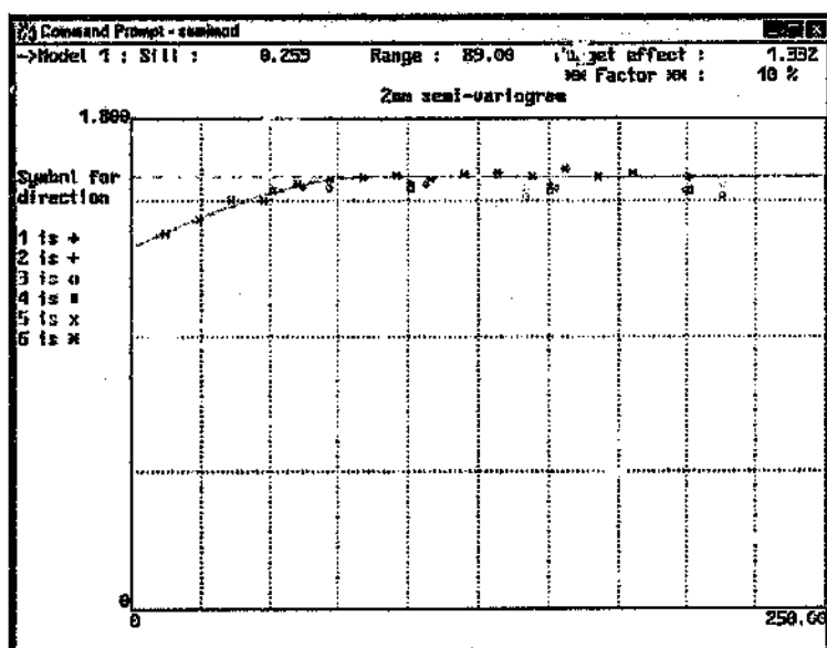
Figure 7.7: Semi-variogram of the 2mm sample data
