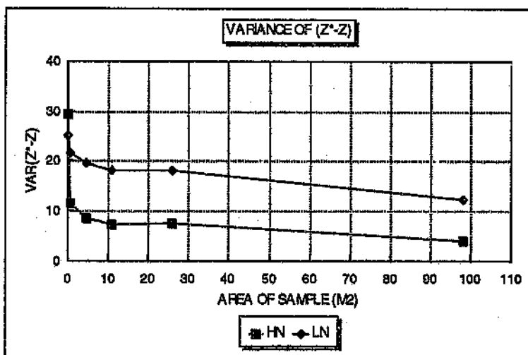
Figure 6.4: Variance of (Z^*-Z) for the high and low nugget models against the area of the sample ( 0m^2 to 110m^2 )
