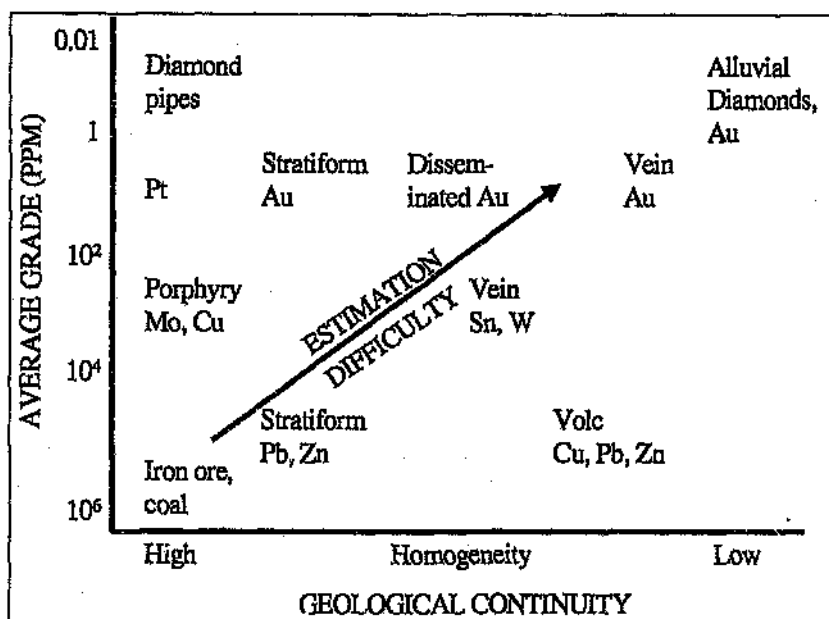
Figure 1.1: Proportion of ore mineral versus homogeneity (after King 1982)
