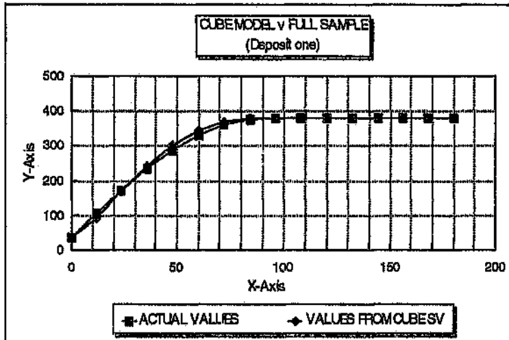
Figure 4.4: The 12m theoretical semi-variogram, estimated from the cube semi-variogram ("values from cube SV") compared to the real 12m semi-variogram ("actual values").
