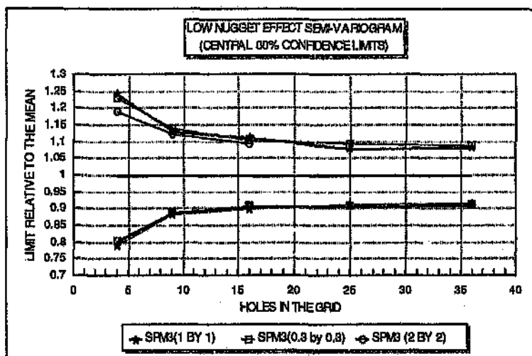
Figure 5.5: Low nugget semi-variogram model showing the central 80% confidence limits for different grids and different sample sizes
