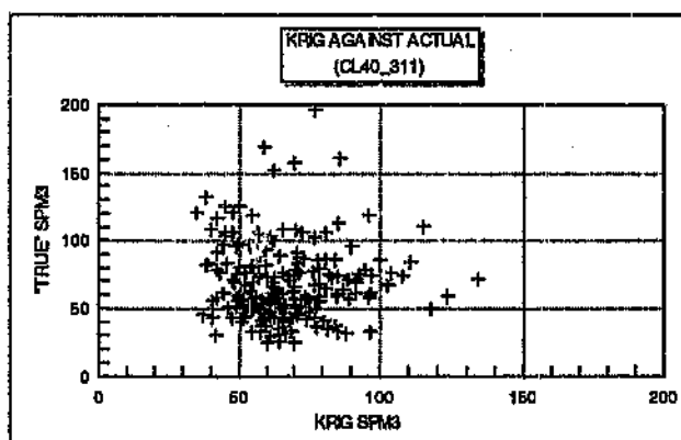
Figure 3.10: "True" block values against kriged values for the clustered data
