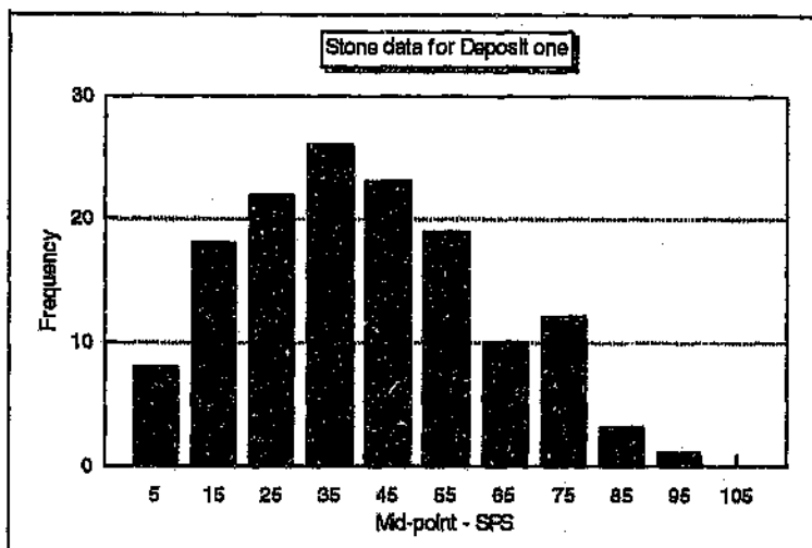
Figure 4.1: Histogram of stones per sample for Deposit one
