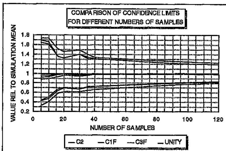
Figure 8.1: Comparison of the central 80% confidence limits for different numbers of samples. C2 is the 2mm grade, C1F is the 1mm grade factored to 2mm and C3F is the 1.5mm to 2.4mm grade factored to 2mm.
