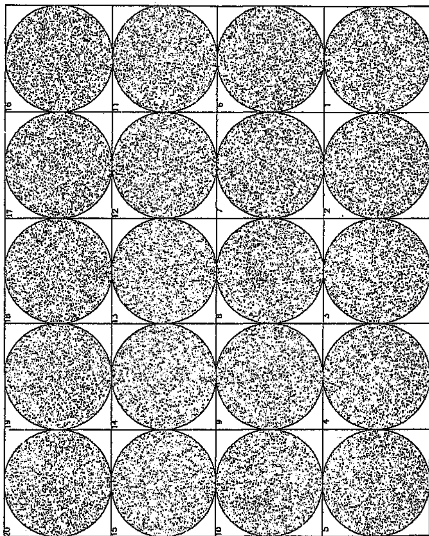
Figure 3.1 Uniform, random texture. Each circle represents a horizontal slice at 6m intervals through the simulation
