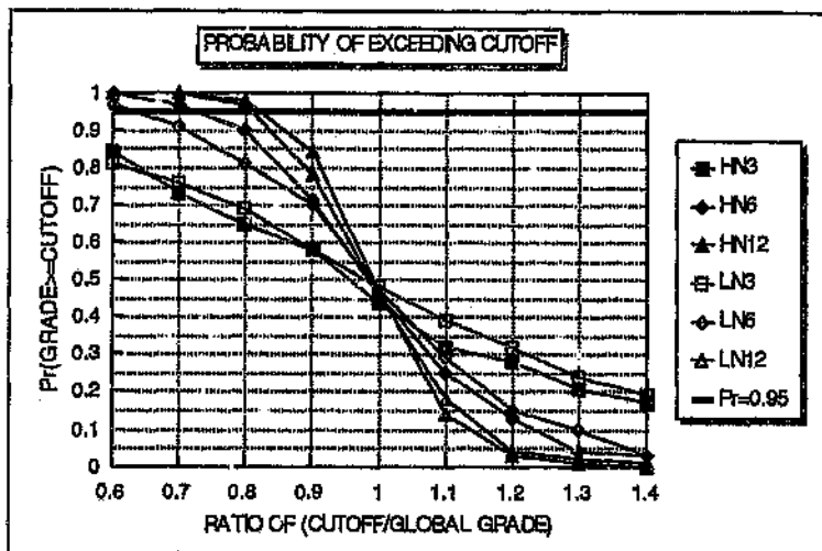
Figure 5.10: The probability of exceeding a cutoff for samples of three, six and twelve inches for the high and low nugget effect models. The cutoff is expressed as the ratio of the cutoff to the mean grade.
