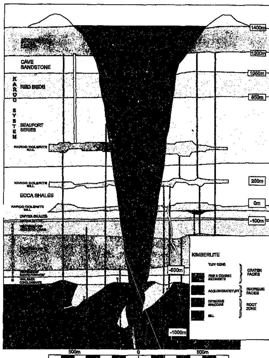
Figure 2.1: Model of kimberlite pipe (modified after Hawthorne 1975) showing the crater facies, the diatreme facies and the root zone. The sampling data used in this thesis has been taken from the diatreme facies of the pipe.
