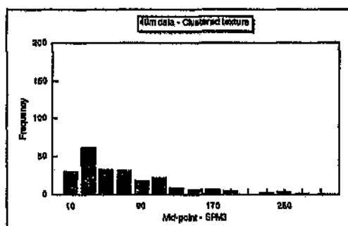
Figure 3.6: Clustered texture for 40m sample data
