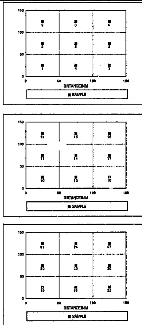
Figure 6.3: Sample numbering for the three levels of the kriging neighbourhood. The lowest level (6m) is top most, the intermediate level (18m) is next and the top level (30m) is at the bottom.
