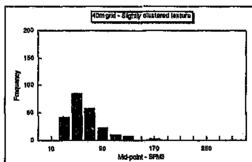
Figure 3.5: Slightly clustered texture for 40m sample data
