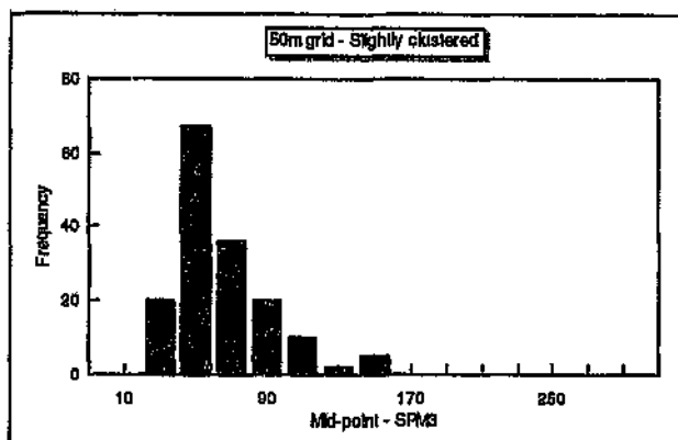
Figure 3.7: Slightly clustered texture for the 50m grid samples
