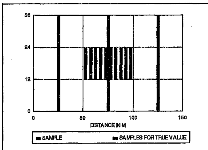
Figure 6.2: Section view of the kriging neighbourhood showing the samples surrounding the block to be kriged and the samples used to estimate the "true" value of the kriged block.
