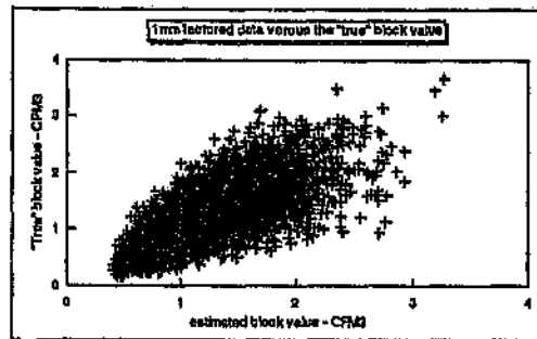
Figure 7.9 "True" estimates versus the 1mm adjusted block estimates
