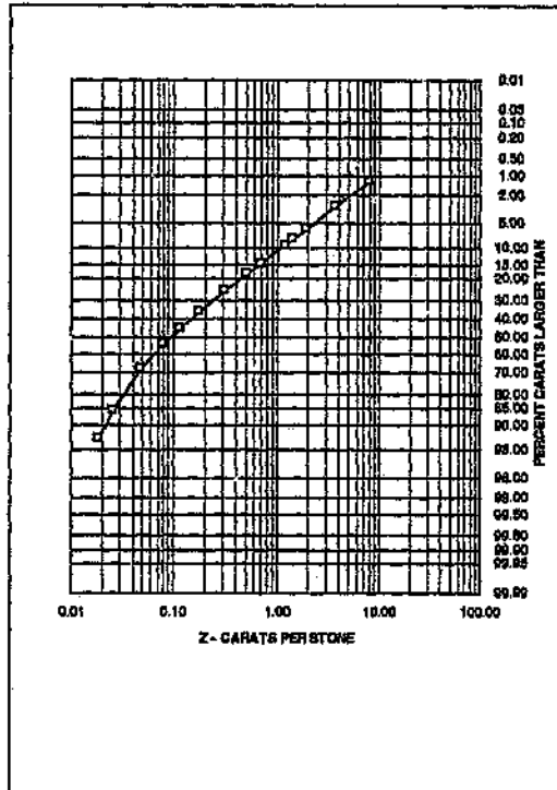
Figure 2.2: The diamond size distribution of deposit one on logarithmic probability paper. The reversed probability scale is by convention.
