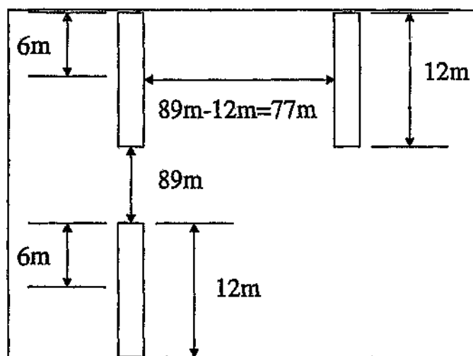
Figure 4.3: Explanation of anisotropy due to sample shape
