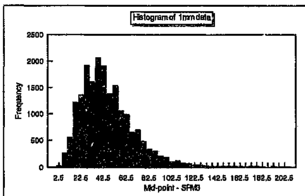
Figure 7.3 Simulated sample data at 1mm in SPM3
