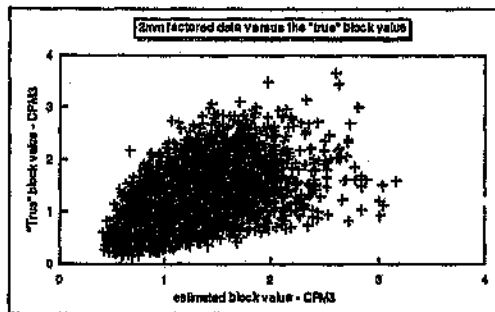
Figure 7.10 "True" block estimates versus the 2mm block estimates
