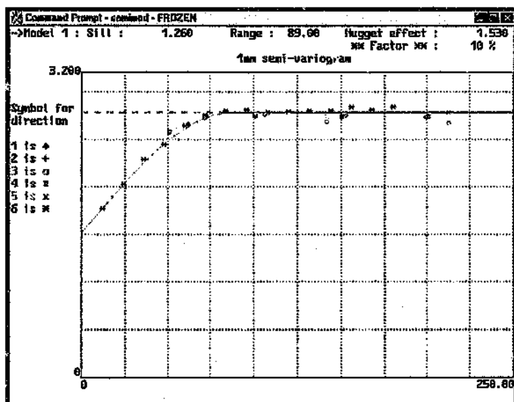
Figure 7.6: Semi-variogram of the 1mm data used for the kriging
