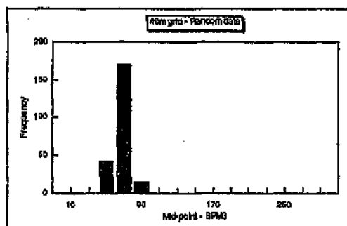
Figure 3.4: Random texture for 40m sample data
