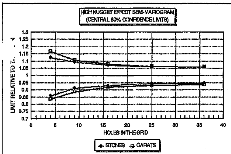
Figure 5.4: High nugget semi-varlogram model showing the central 80% confidence limits for different grids
