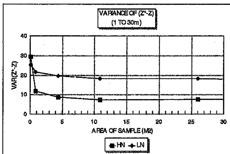
Figure 6.5: As for Figure 6.4 except the X axis has been limited to 0m^2 to 30m^2 to allow more detail.
