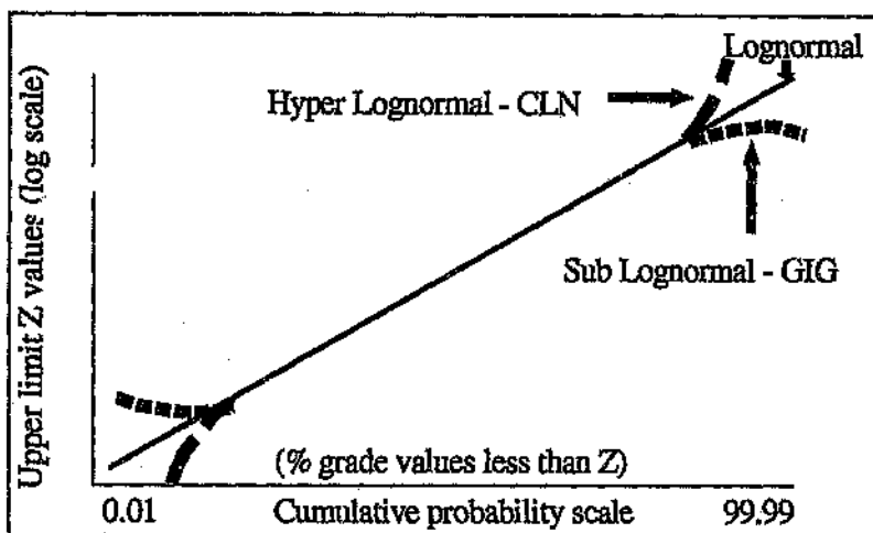
Figure 2.3: Relationship between the Compound lognormal model and the lognormal model (after Dohm 1995).
