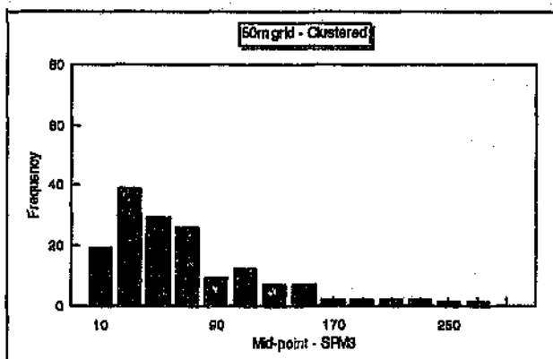
Figure 3.8: Clustered data for the 50m grid sampling
