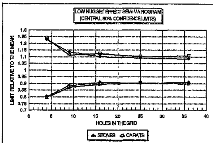
Figure 5.3: Low nugget semi-varlogram model showing the central 80% confidence limits for different grids for SPM3 (stones) and CPM3 (carats).
