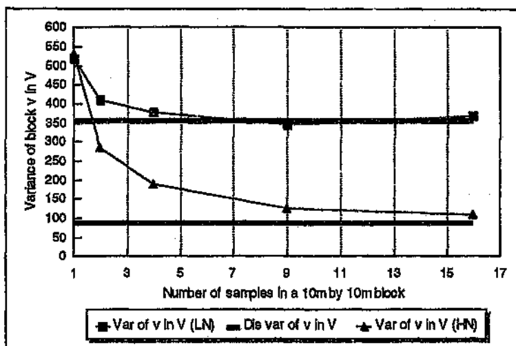
Figure 6.6: Variance of blocks based on 2, 4, 9 and 16 samples compared to the theoretical estimation variance of a 10m block for the high and low nugget semi-variogram models.
