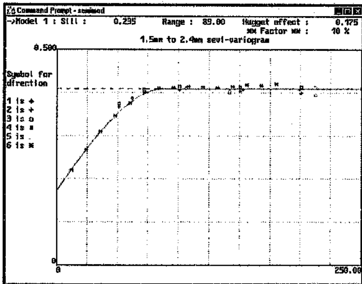
Figure 7.8: Semi-varlogram of the 1.5mm to 2.4mm sample data
