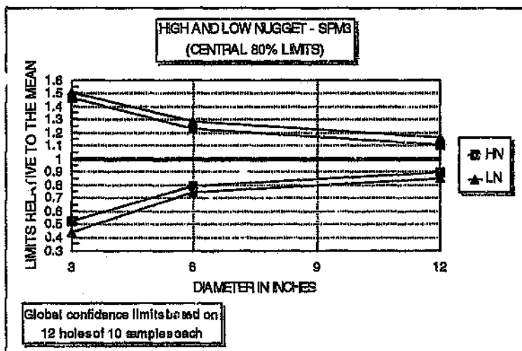
Figure 5.7: High and low nugget effect models showing the central 80% confidence limits for a three, six and twelve inch diameter sample. All samples are 12m in length.
