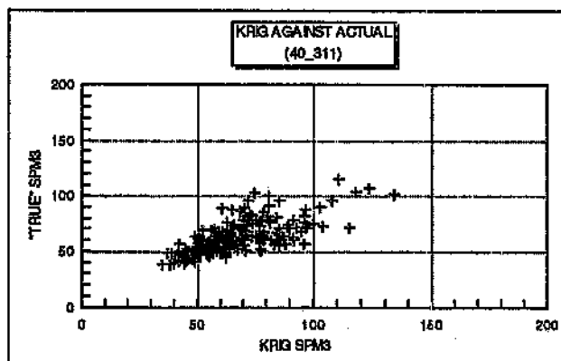
Figure 3.9: "True" values against kriged values for the 40m, slightly clustered data
