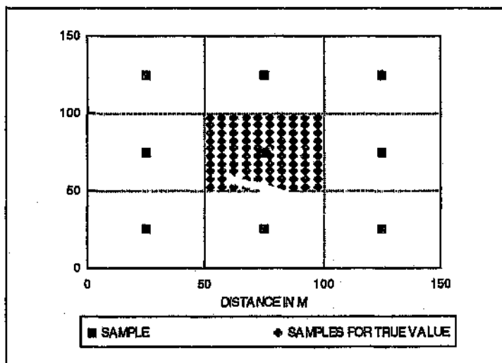
Figure 6.1: Plan view of the kriging neighbourhood showing the sample points surrounding the block to be kriged and the samples used to estimate the "true" value of the block to be kriged.
