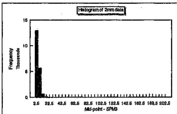
Figure 7.4 Simulated data at 2mm in SPM3
