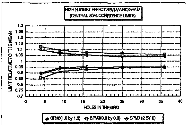
Figure 5.6: High nugget semi-variogram model showing the central 80% confidence limits for different grid and different sample sizes
