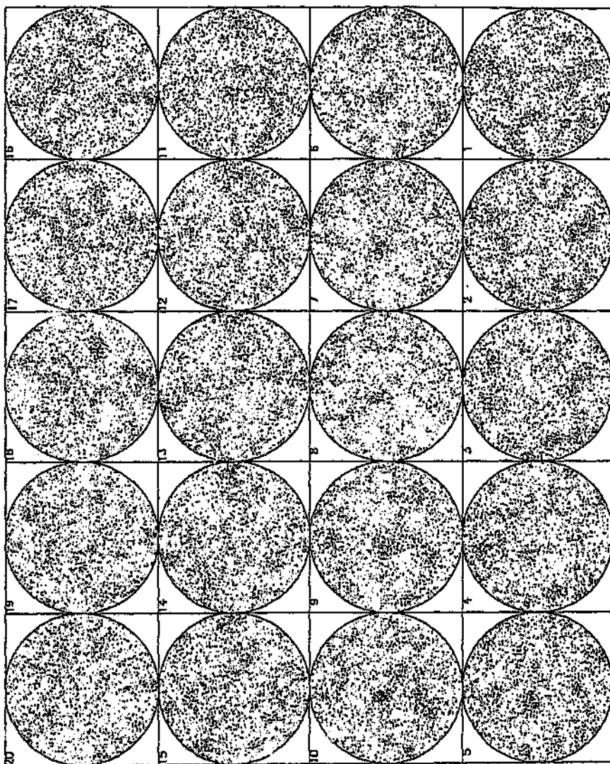
Figure 3.2 Slightly clustered texture. Each circle represents a horizontal slice at 6m intervals through the simulation.
