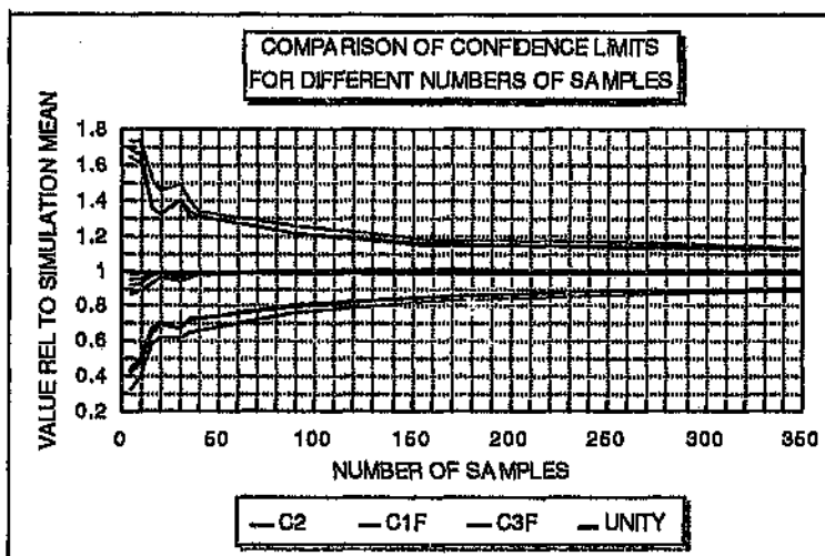
Figure 8.2: The same graph as Figure 8.1 except the X axis has been extended to 350 samples. C2 is the 2mm grade, C1F is the 1mm grade factored to 2mm and C3F is the 1.5mm to 2.4mm grade factored to 2mm.
