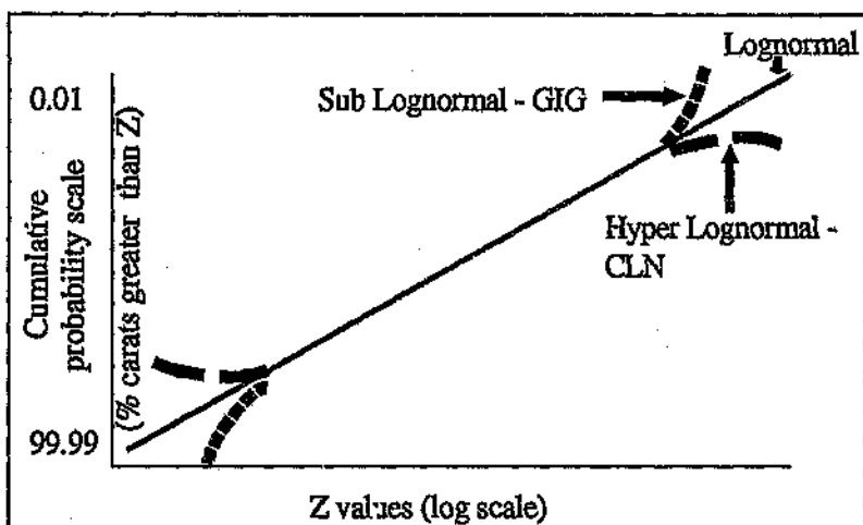
Figure 2.4: Figure 2.4 shows the axes of Figure 2.3 arranged in the same way as the diamond size distribution plot shown in Figure 2.2.
