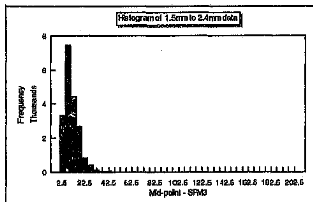
Figure 7.5 Simulated data at 1.5mm to 2.4mm in SPM3
