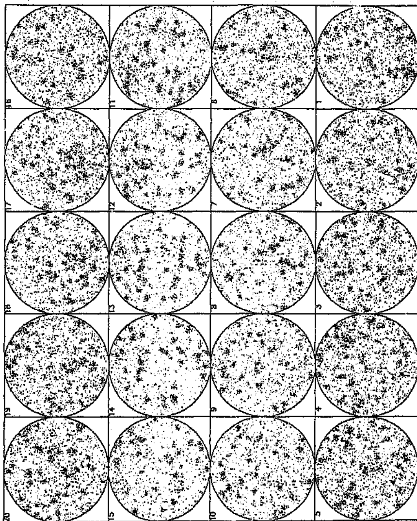
Figure 3.3 Clustered texture. Each circle represents a horizontal slice at 6m intervals through the simulation.
