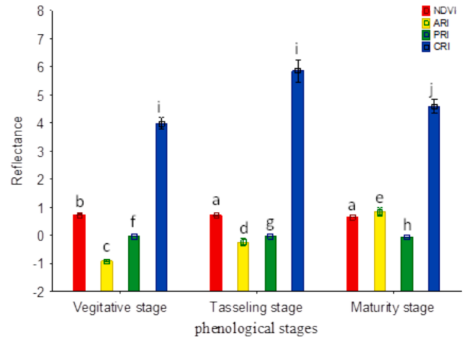
Fig. 5. The vegetation indices extracted from the spectral signatures of maize: NDVI (a-b), ARI (c-e), PRI (f-h) and CRI (i-j) during the vegetative, tasselling and maturity stages of maize. Means were related by one-way ANOVA and those followed by the same letter(s) are not significantly different ( p > 0.05 ; Fisher LSD test).
