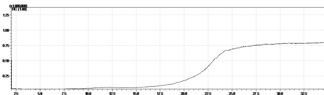
Figure B1. Chromatogram (Abundance vs Retention time) of A. obliquus under Condition 1
