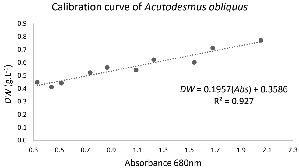
Figure A1. Calibration curve of absorbance ( \lambda = 680 \text{ nm} ) and AD dry weight
