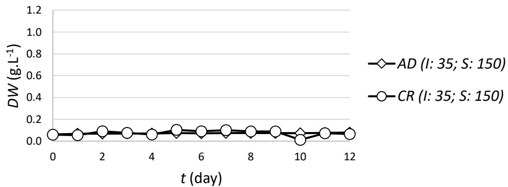
Figure 5. Dry weight of A. obliquus and Chlamydomonas under Condition 0 ( I : 35; S : 150). Error bars represent SD .
