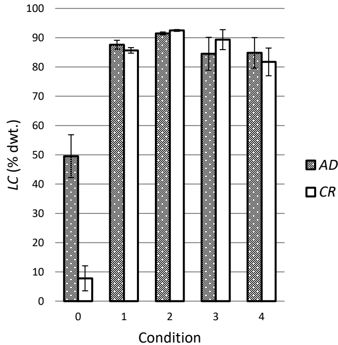
Figure 12. Percentage lipid extracts of A. obliquus and Chlamydomonas under different conditions (0, 1, 2, 3 & 4). Error bars represent SD.
