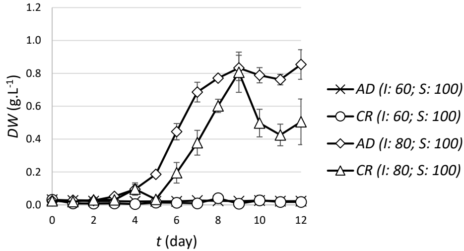
Figure 8. Dry weight of A. obliquus and Chlamydomonas under two different light intensities and agitation of S = 100 rpm (Condition 2 & 4). Error bars represent SD.
