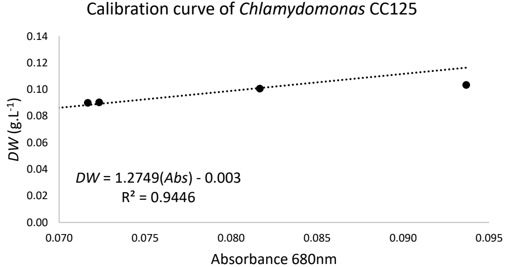
Figure A2. Calibration curve of absorbance ( \lambda = 680 \text{ nm} ) and CR dry weight
