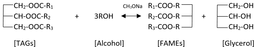
Figure 3. Transesterification reaction (Mutanda, et al. , 2011)
