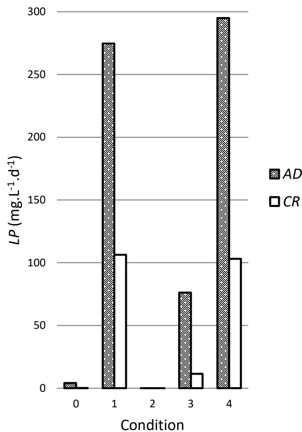
Figure 13. Maximum lipid productivities of A. obliquus and Chlamydomonas under different conditions (0, 1, 2, 3 & 4)
