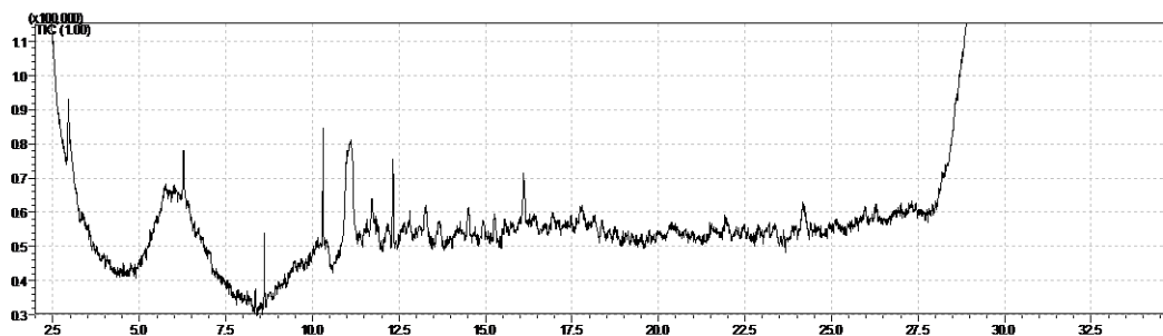
Figure B4. Chromatogram (Abundance vs Retention time) of Chlamydomonas under Condition 2
