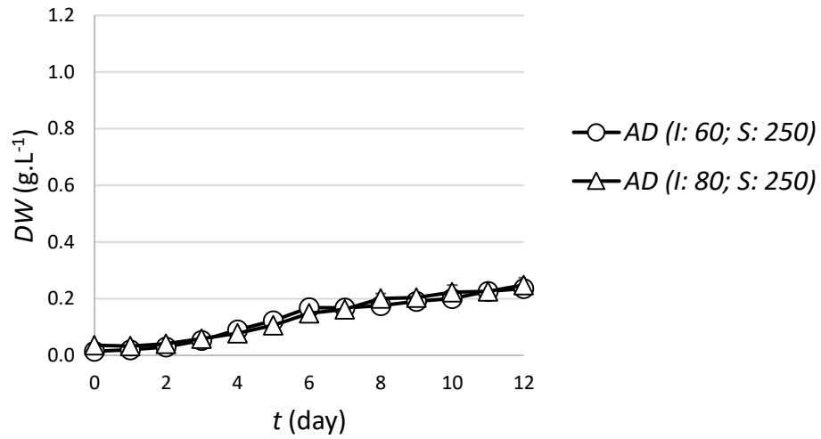
Figure 6. Dry weight of A. obliquus under two different light intensities and agitation of S = 250 rpm (Condition 1 & 3). Error bars represent SD .
