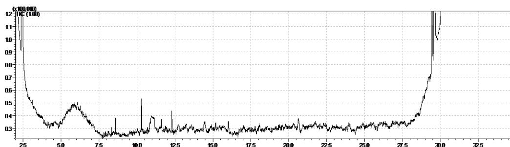
Figure B8. Chromatogram (Abundance vs Retention time) of Chlamydomonas under Condition 4
