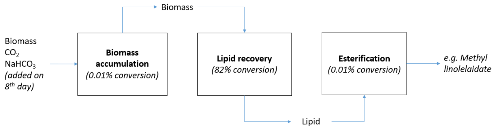
Figure 15. Summary of the carbon flow through the processes involved in studying A. obliquus FAMES under Condition 4 ( I = 80 ; S = 100 )
