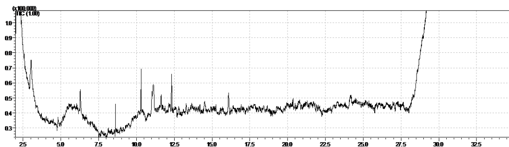
Figure B3. Chromatogram (Abundance vs Retention time) of A. obliquus under Condition 2
