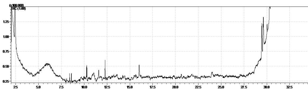
Figure B7. Chromatogram (Abundance vs Retention time) of A. obliquus under Condition 4
