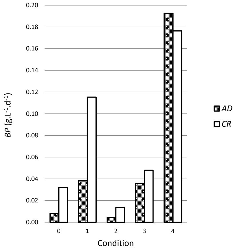
Figure 10. Maximum biomass productivity of A. obliquus and Chlamydomonas under different conditions (0, 1, 2, 3 & 4)
