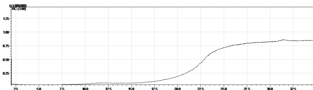
Figure B2. Chromatogram (Abundance vs Retention time) of Chlamydomonas under Condition 1
