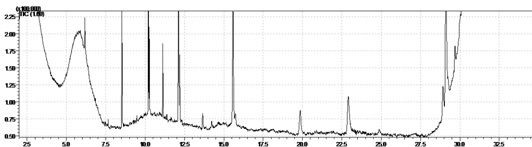
Figure B6. Chromatogram (Abundance vs Retention time) of Chlamydomonas under Condition 3
