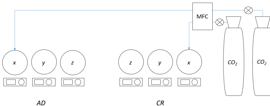
Figure 4. Batch cultivation set-up (Replicate 1 = x , Replicate 2 = y & Replicate 3 = z )
