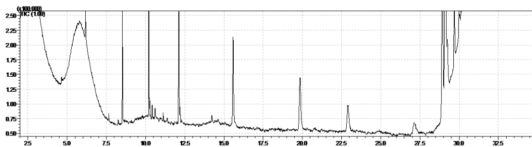
Figure B5. Chromatogram (Abundance vs Retention time) of A. obliquus under Condition 3
