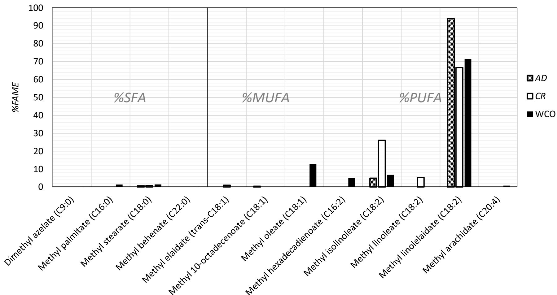
Figure 14. %FAME composition of microalgae and waste cooking oil under Condition 4 ( I = 80 ; S = 100 ). The most common area value amongst a triplicate set ( n = 3 ) was used to determine %FAME (Section 3.9.1.)
