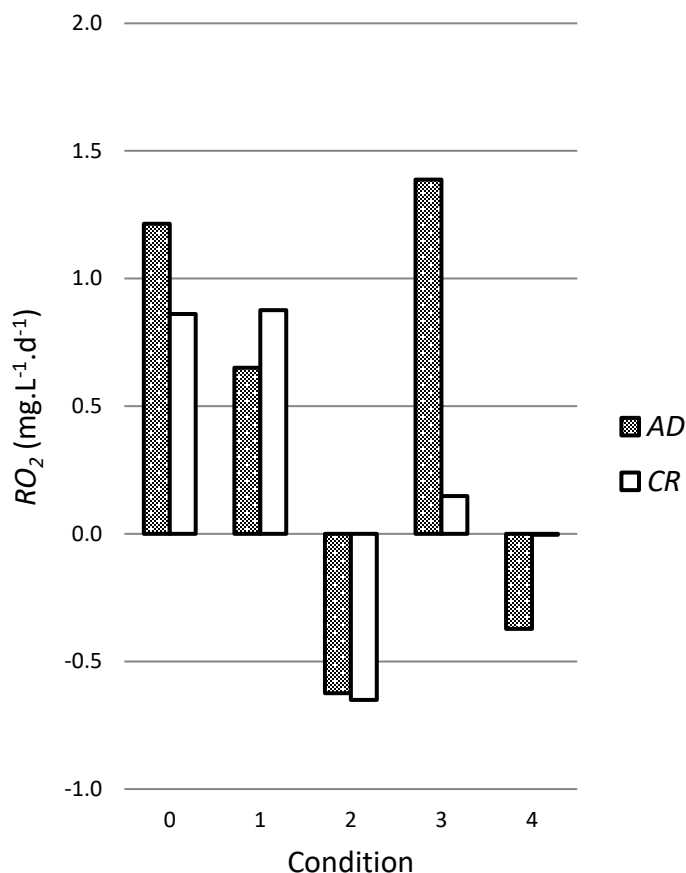
Figure 11. Maximum rate of O_2 production of A. obliquus and Chlamydomonas under different conditions (0, 1, 2, 3 & 4) ( RO_2 = 0 is ideal)
