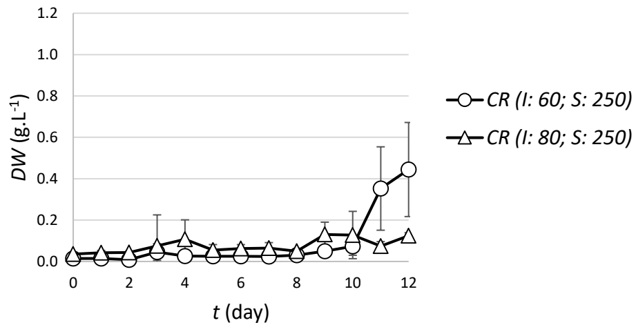
Figure 7. Dry weight of Chlamydomonas under two different light intensities and agitation of S = 250 rpm (Condition 1 & 3). Error bars represent SD .
