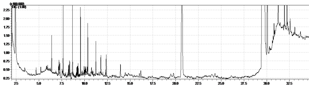
Figure B9. Chromatogram (Abundance vs Retention time) of waste cooking oil – which underwent the same transesterification procedure as algae oil (Section 3.6.3.)
