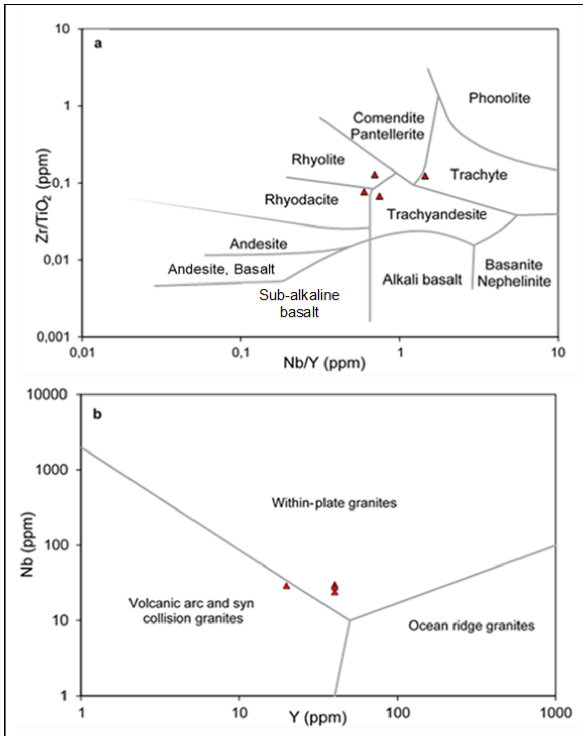
Figure 17: Bivariate trace element plots for the Blaauwboschpoort bentonite deposit. (a) Rhyolitic character versus alkalinity graph (Winchester and Floyd, 1977). (b) Discrimination diagram of Nb vs. Y (Pearce et al. , 1984)
