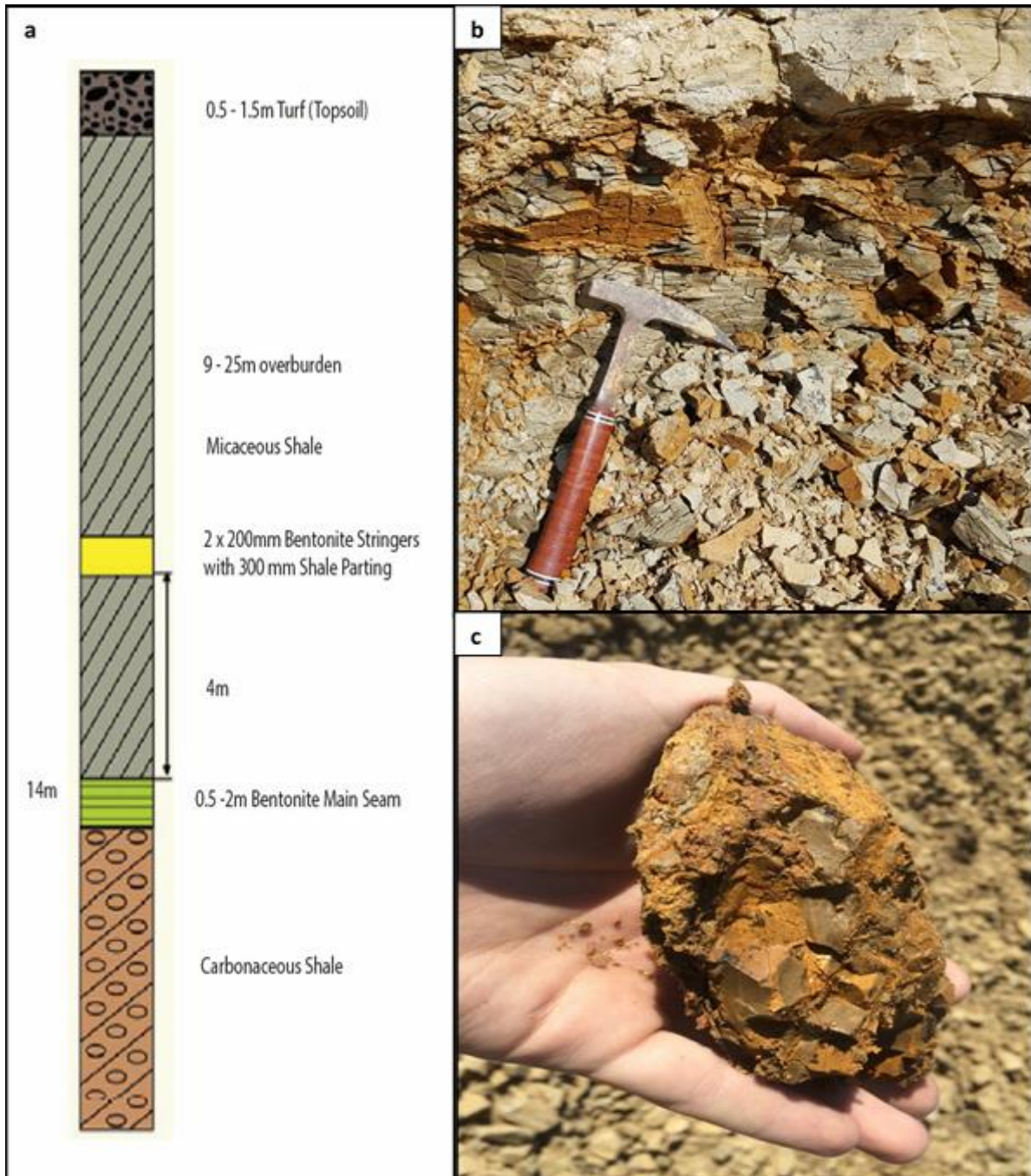
Figure 8: Stratigraphy and field evidence of the Koppies bentonite deposits. (a) Stratigraphic column, (b) In-situ khaki brown to grey bentonite seam identified as sample 2, the darker colour is due to characteristic water retention in comparison to overlying micaceous shales, (c) Structureless, and waxy orange bentonite near Sample 6 illustrating the colloidal nature. Notable manganese growths are evident.
