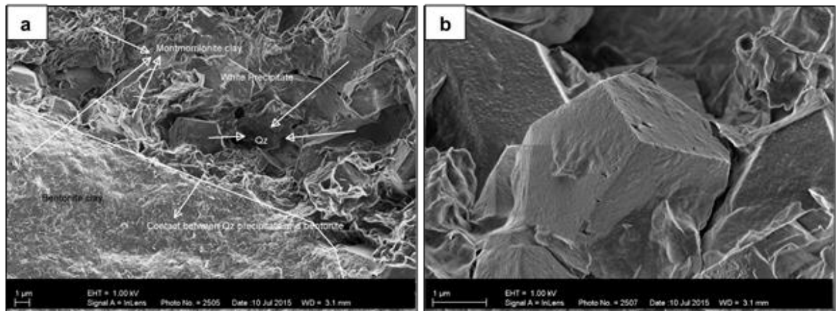
Figure 12: Scanning electron photomicrographs of the boxwork quartz and bentonite contact within a pre-existing crack within the Blaauwboschpoort bentonite deposit (a) Sharp contact between the quartz precipitate and bentonite (annotated in white), (b) Zoomed-in angular quartz crystals with smectite surface coatings.
