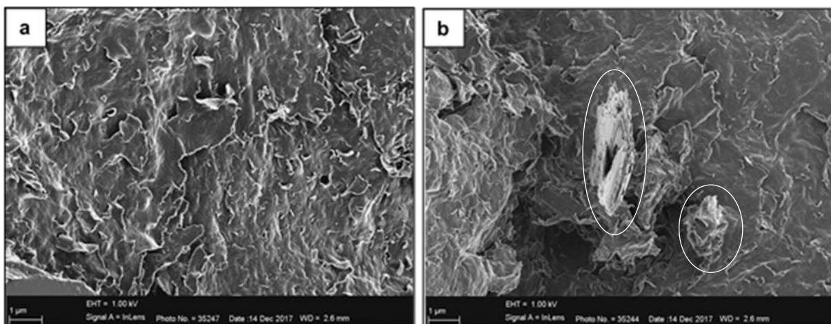
Figure 10: Scanning electron photomicrographs of smectite textures observed in the Blaauwboschpoort bentonite. (a) Smectite dominated matrix illustrating crenulated edges of the flakes. (b) Booklet, face to face associations of smectite flakes (circled in white).
