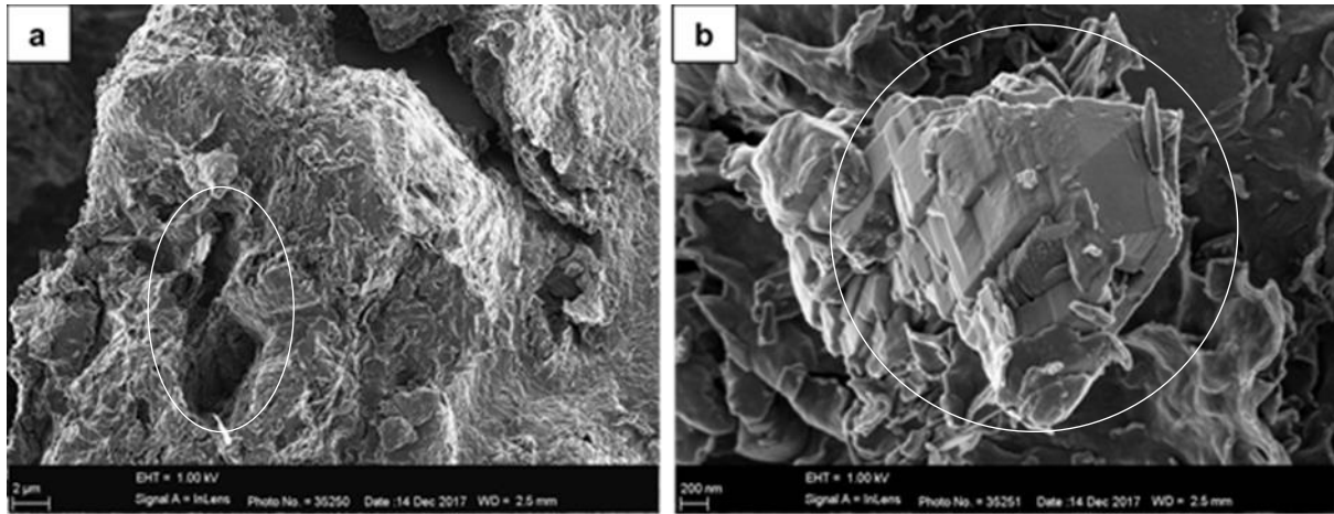
Figure 11: Scanning electron photomicrographs of inclusion minerals within the smectite matrix observed in the Blaauwboschpoort bentonite. (a) Void in the smectite matrix illustrating a remnant rounded quartz crystal (circled in white), (b) Individual zeolite grain amongst smectite mass (circled in white)
