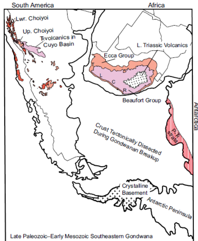
Figure 18: Simplified palaeo geological map illustrating the approximate distance between the Choiyoi Group and Volksrust Formation which is contained in the NW section of the Ecca Group (From: McKay et al. , 2016).
