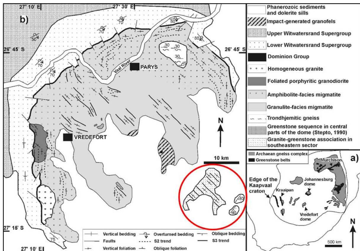
Figure 4: Geological map illustrating various upturned sequences in the Vredefort Dome and Greenlands Formation (circled in red) (From: Lana et al. , 2003).
