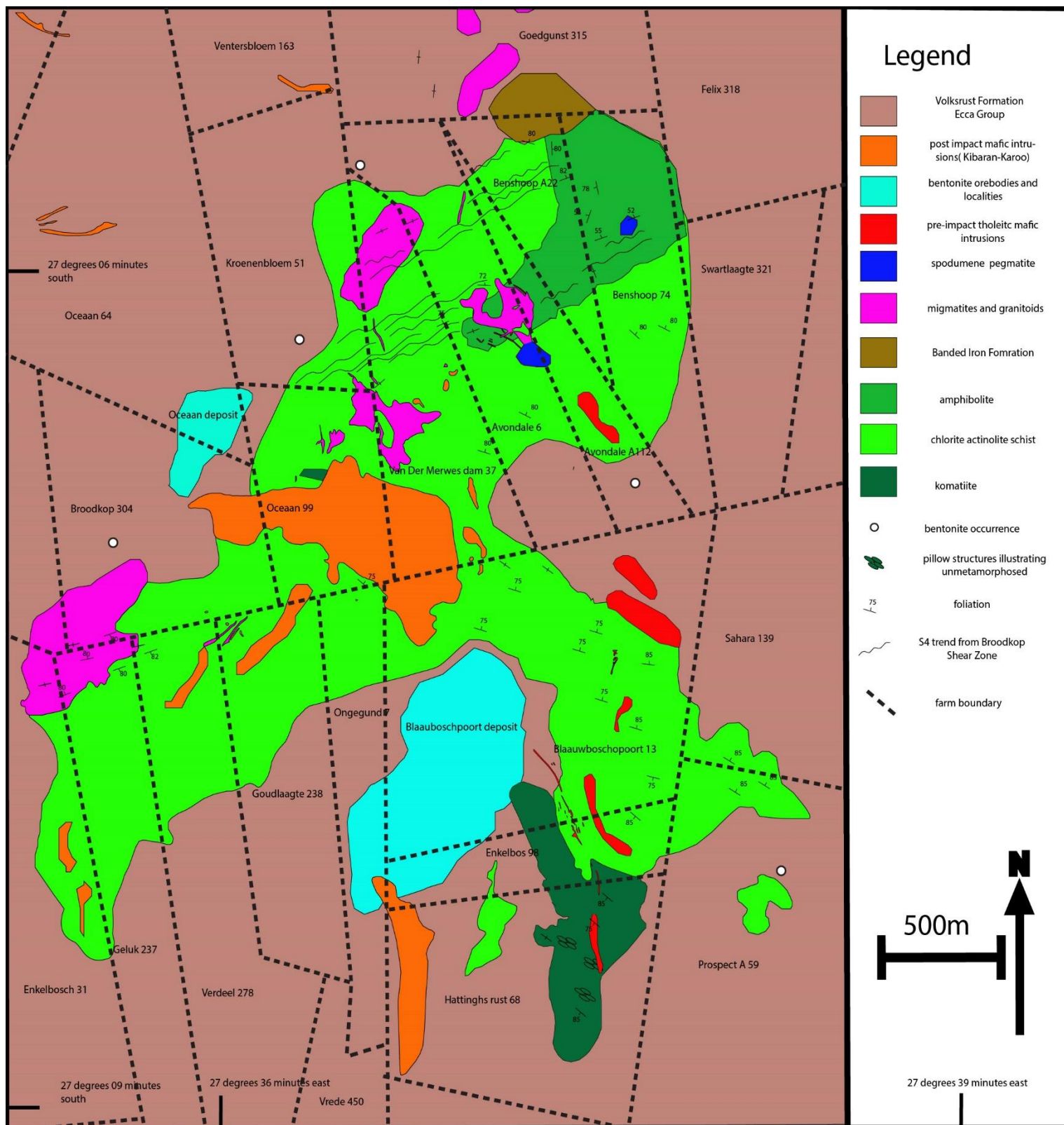
Figure 7: Composite geological map of the Greenlands Formation with the location of various bentonite deposits and occurrences.
