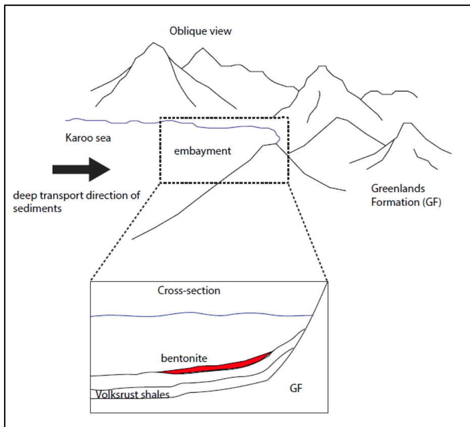
Figure 19: Idealised sketch of the depositional setting and the structural relationship between the Koppies bentonite and Greenlands Formation.
