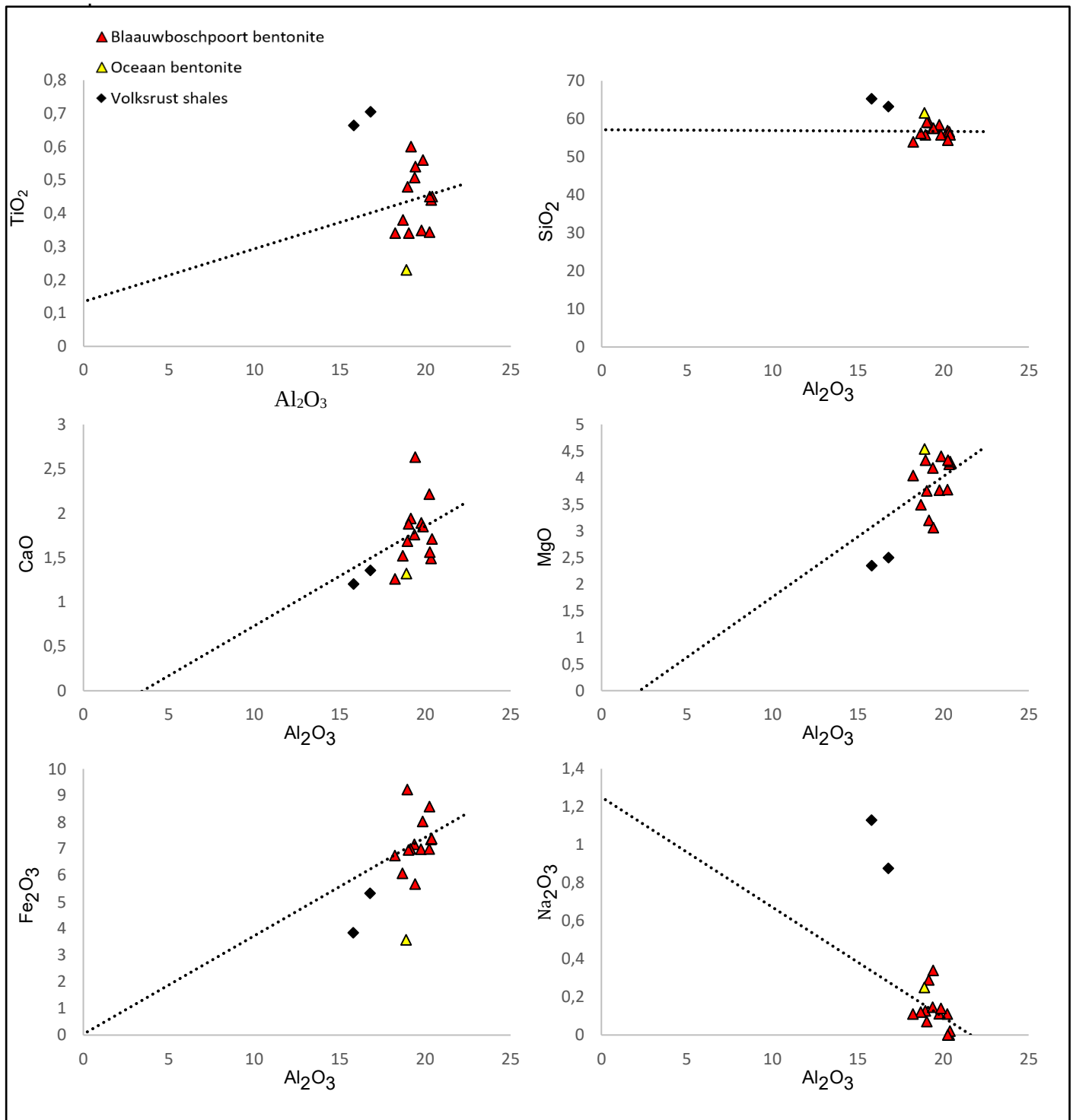
Figure 14: Immobile element Al versus mobile/immobile elements for the Koppies bentonite deposits and overlying Volksrust shales. Trend lines illustrate enrichment as a negative intercept and depletion as a positive intercept for a given element (Christidis, 1998).
