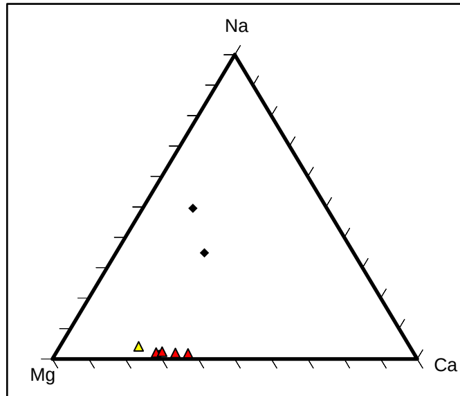
Figure 15: Ternary plot of dominant cations present in the Koppies bentonite in relation to the overlying shales (atypical chemistry of shales). The Koppies bentonite samples reflect a Na depleted array, similar to the Wyoming bentonite deposits (Altaner et al. , 1984, Knechtel and Patterson, 1962).
