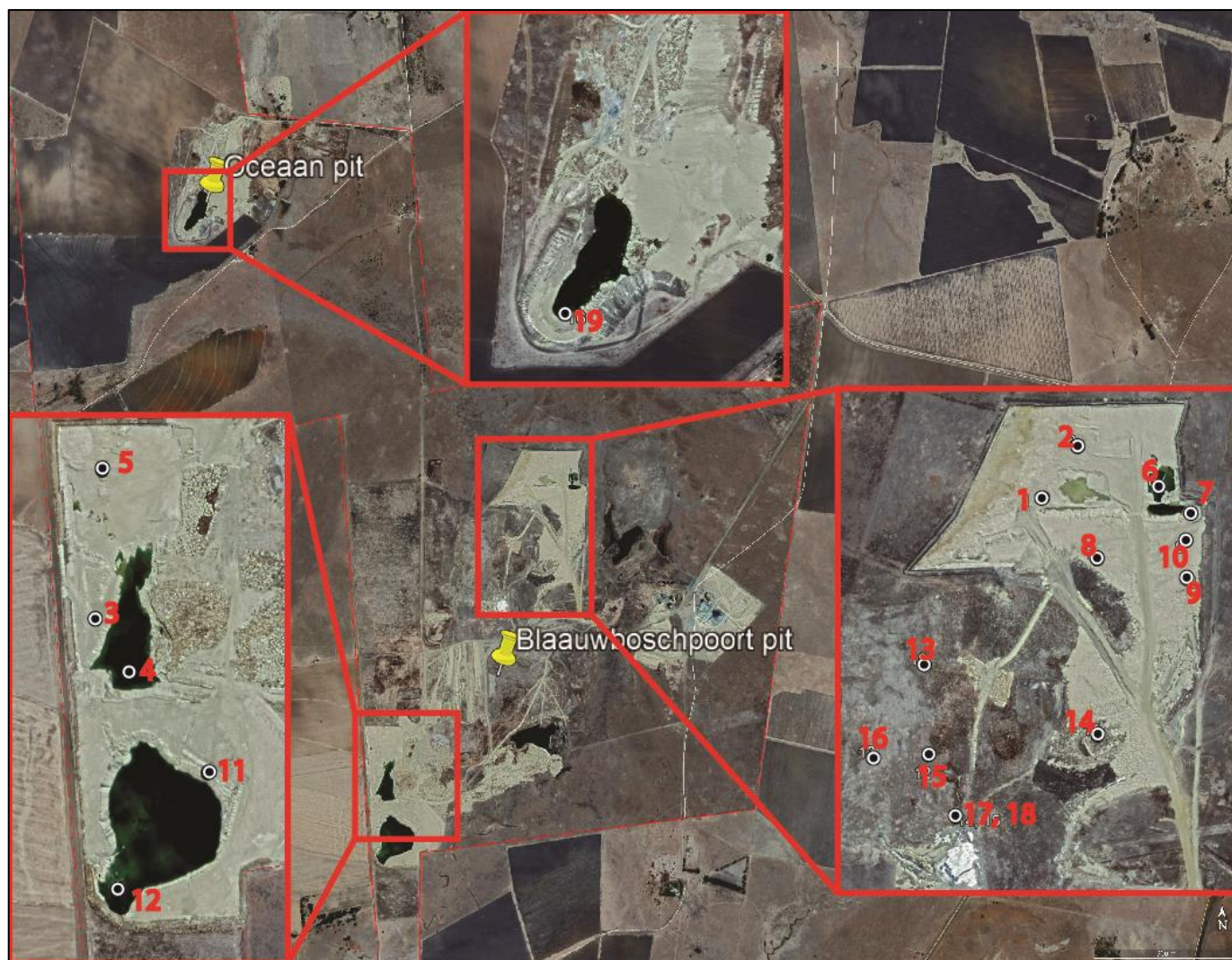
Figure 6: Sample locality map for the samples 1-19 taken from the Blaauwboschpoort and Oceaan deposits and surrounding sub-pits (Google Earth base map image).
