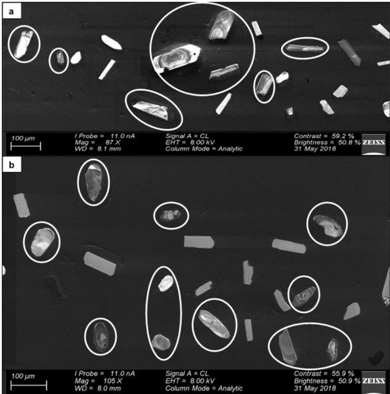
Figure 13: Recovered grains of fragmented, elongated, stumpy, large, small and zoned heavy minerals from the Blaauwboschpoort bentonite. White circles illustrate the zircons while the remainder of crystals represent apatite grains (87x magnification). (a) Zoned euhedral zircon crystals. (b) Fragmented, rounded zircon crystals.
