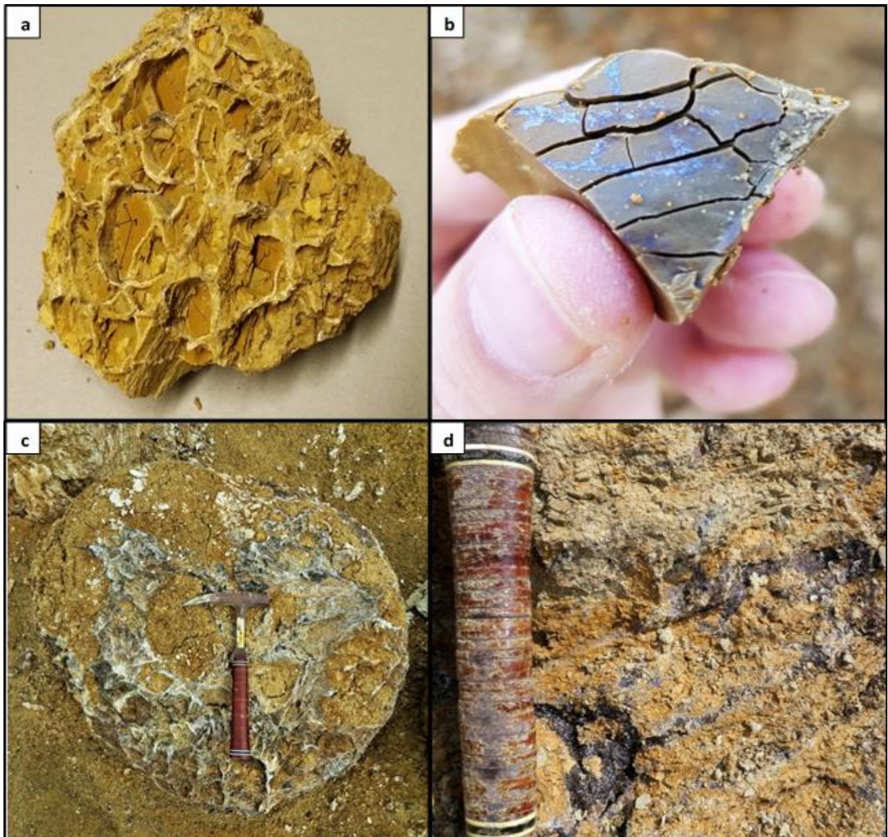
Figure 9: Field evidence and various inclusions within the Koppies bentonite deposit. a) Sample 7 showing boxwork quartz precipitate found within shallow extent of bentonite orebody. b) Dendritic manganese oxide growth in cracks within khaki brown bentonite at Sample 5 locality. c) Irregularly shaped, large barium-rich siderite concretion formed within the bentonite at Sample 4 locality. d) Bentonite present on outer surface of siderite concretion.
