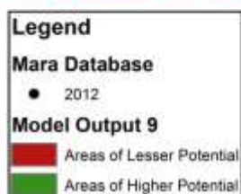
Figure 9.13: Model Output 9
