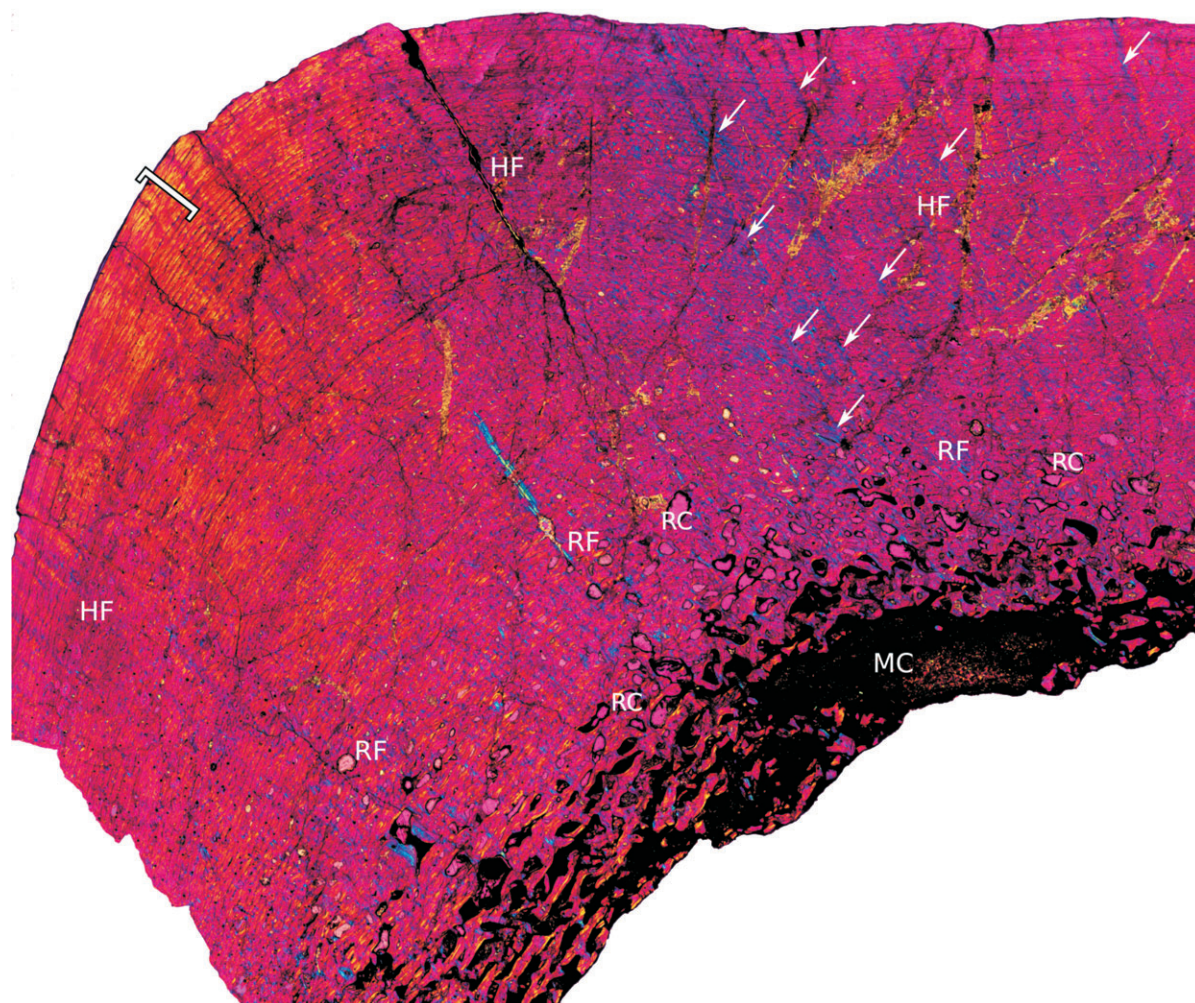
Figure 27. Femoral osteohistology of Massospondylus carinatus (BP/1/4934) in cross-polarized light. Resorption cavities demarcate the Resorption Front. The Haversian Front is located in the outer part of the middle cortex. Bracket indicates parallel-fibred bone in the outer cortex. Arrows indicate extensive Sharpey's fibres. Scale bar = 500 \mu m.
