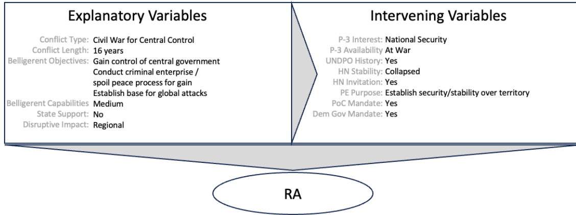
Figure 4-2: Explanatory Variable Assessment for Somalia 2007 - 2022
