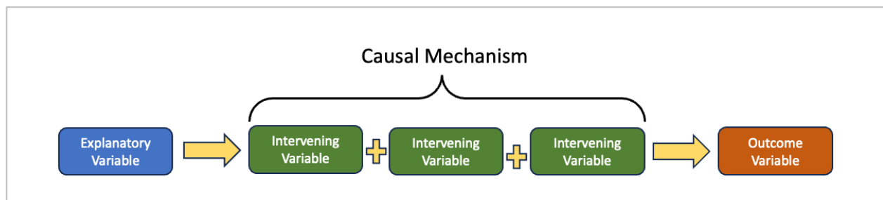
Figure 3-3: Causal Mechanisms
