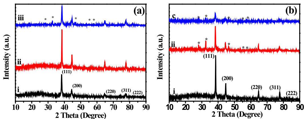
Fig. 2 PXRD patterns of (A) Ag-PDA and (B) Ag@PDA nanocomposites prepared with different concentrations of \text{AgNO}_3 [(i) 1 mM, (ii) 5 mM and (iii) 10 mM].
