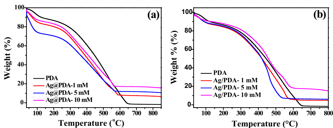
Fig. 4 TGA of (a) Ag-PDA and (b) Ag@PDA nanocomposites at different \text{AgNO}_3 concentrations.
