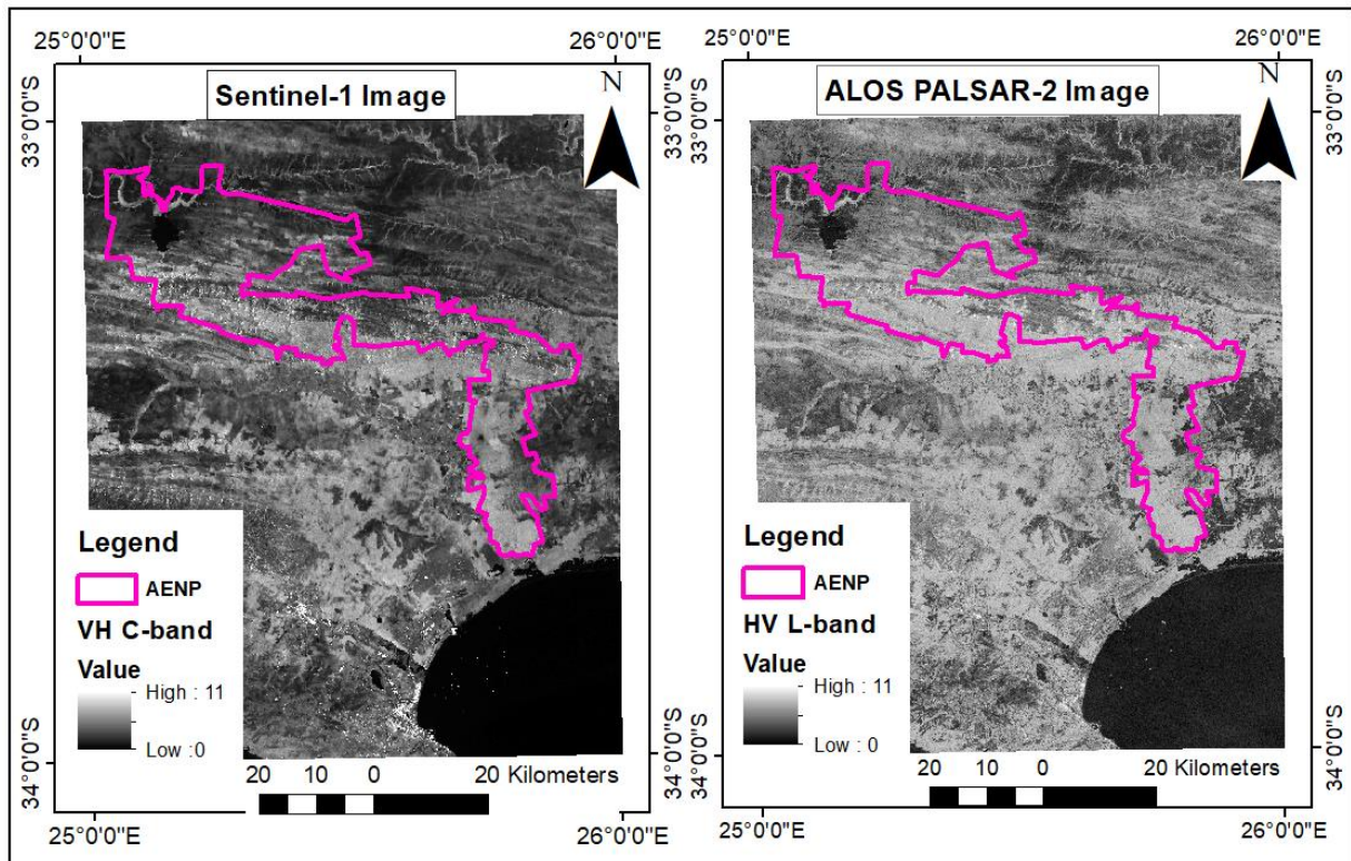
Figure 3.3: Sentinel-1 & ALOS PALSAR-2 mosaics over AENP, displaying VH and HV polarizations, respectively.
