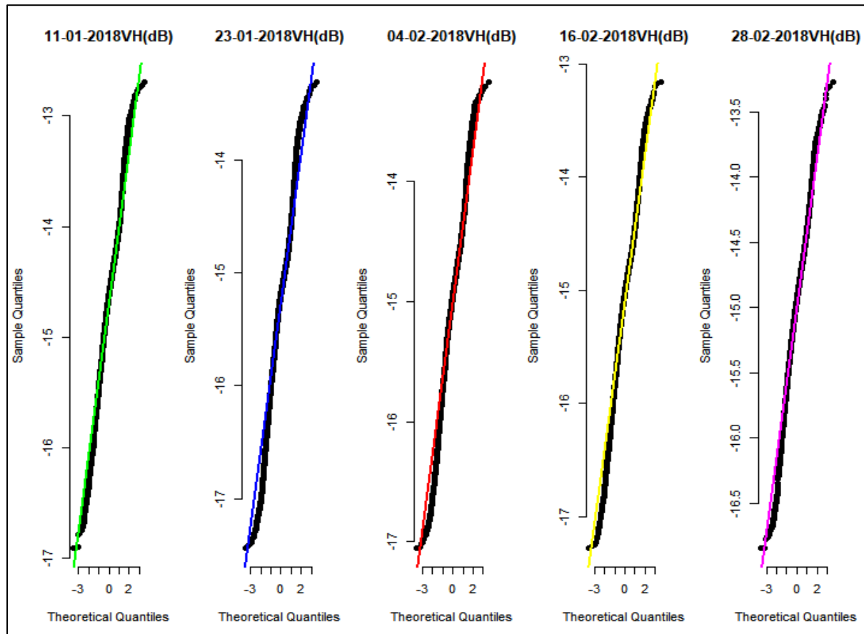
Figure 3. 7: QQ plots of Sentinel-1 VH time series
