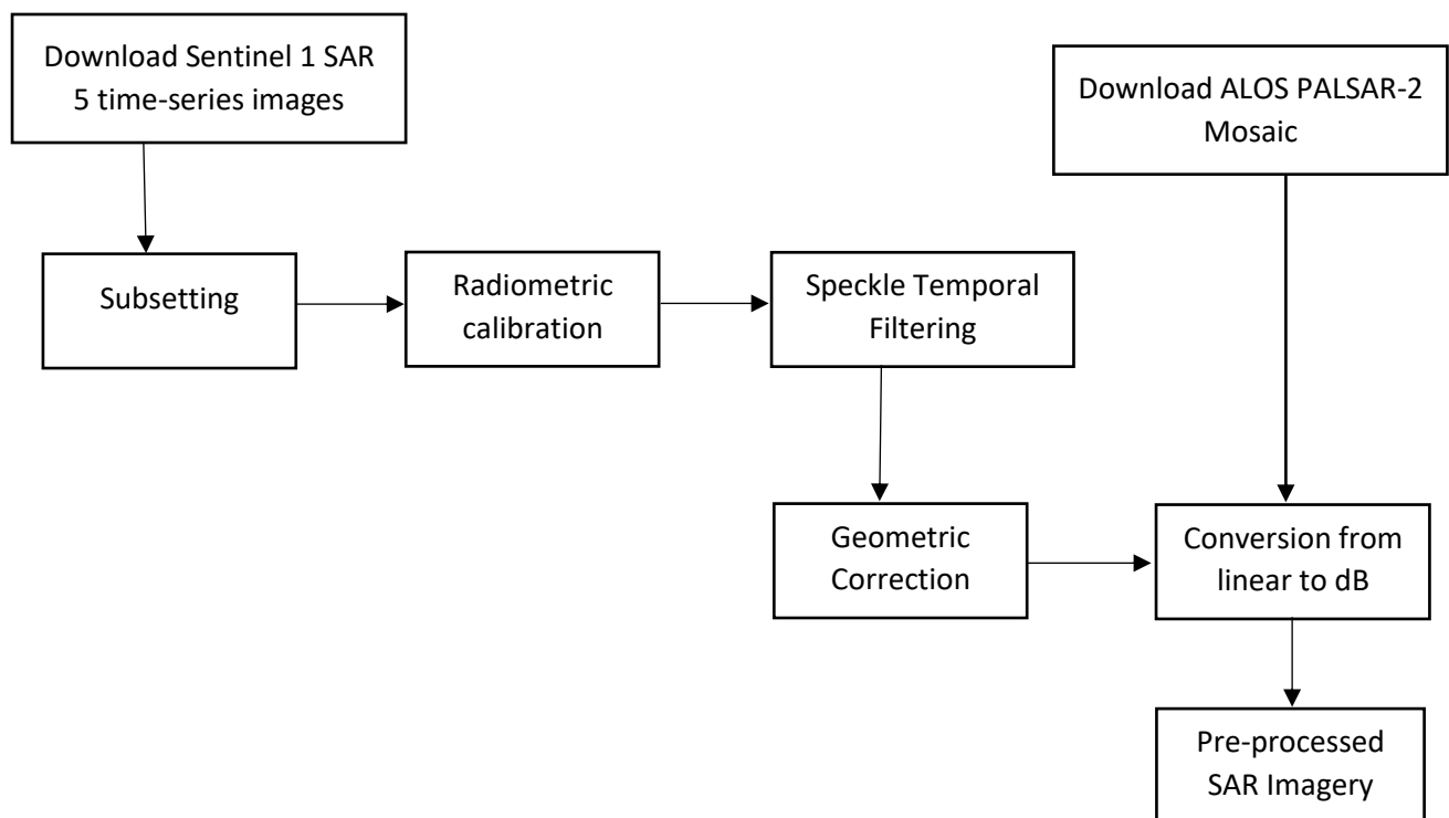
Figure 3. 2: Workflow for working with Satellite SAR data
