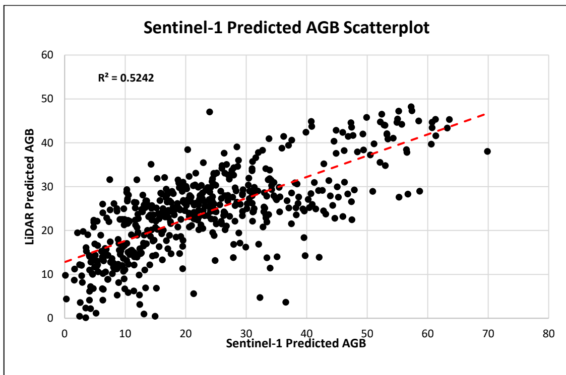
Figure 4. 4: Observed versus Predicted scatter plot Sentinel-1 using SLR
