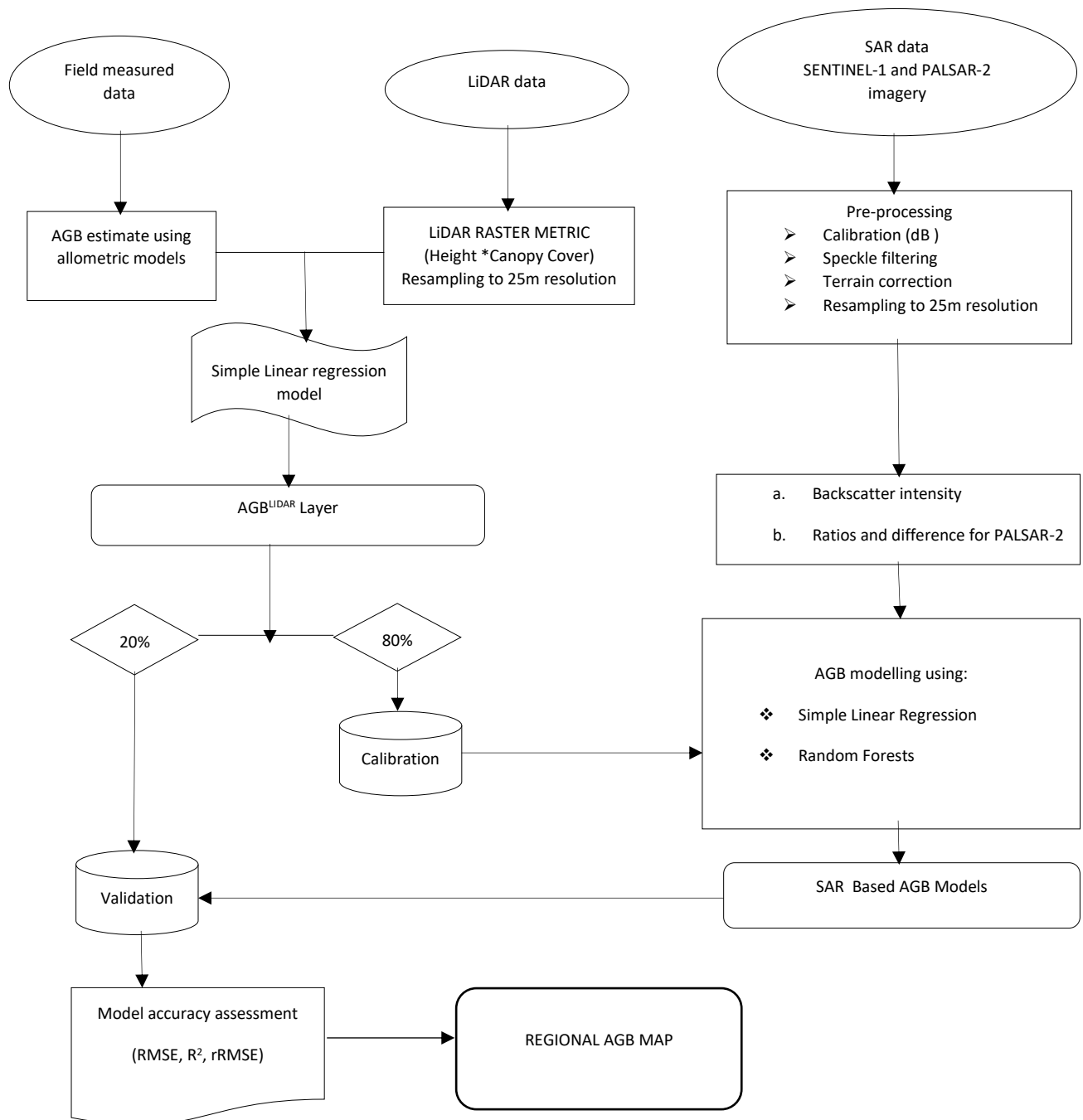
Figure 3. 4: Flow chart of steps used for forest above-ground biomass using SAR imagery
