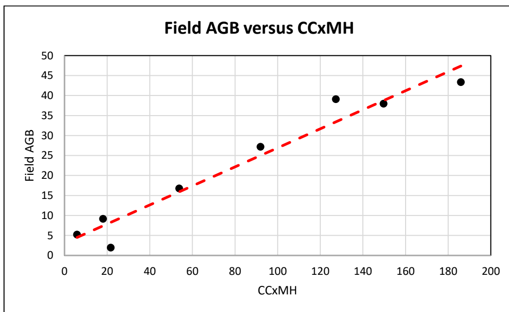
Figure 4. 1: Field AGB versus CC*MH scatterplot
