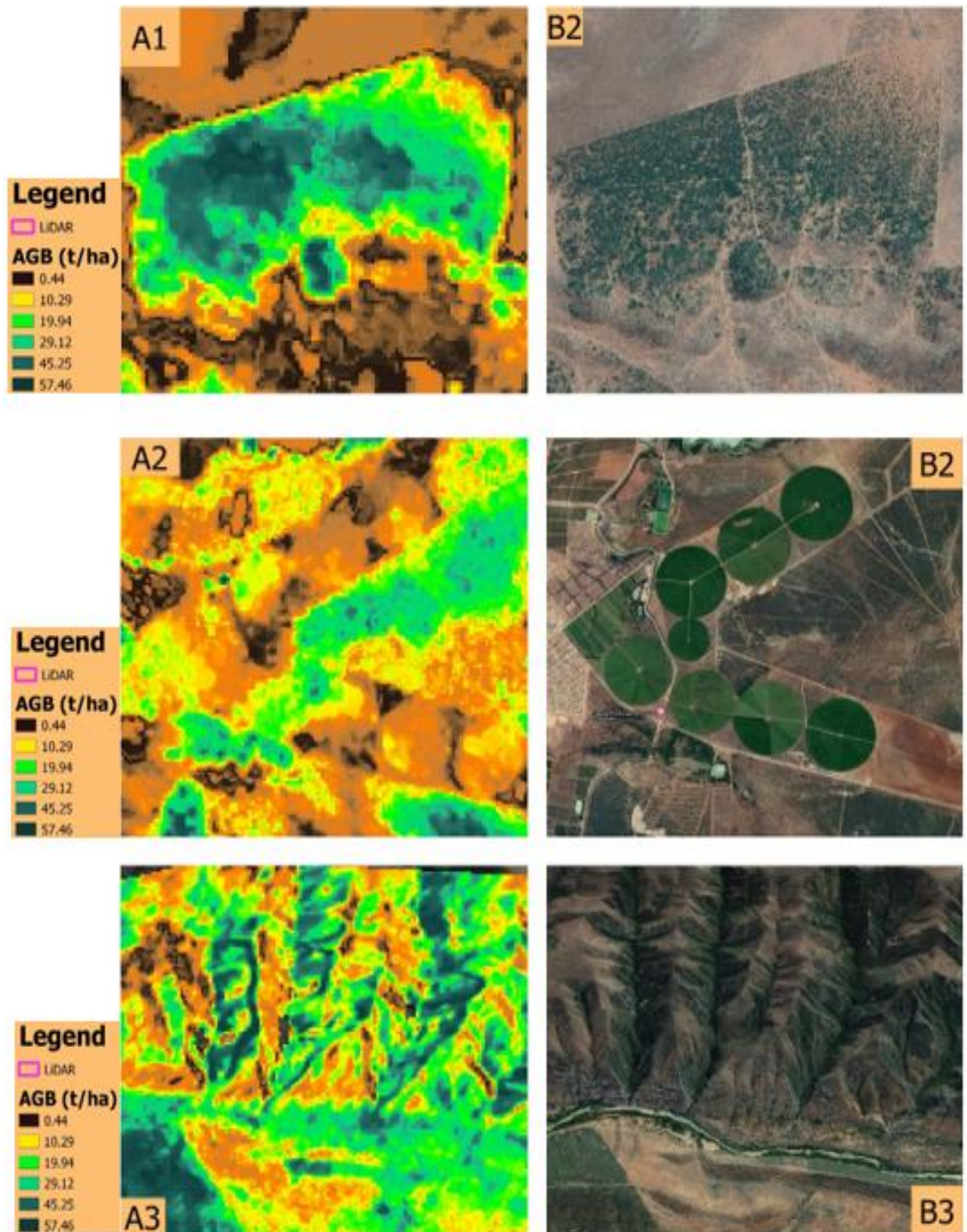
Figure 4. 10: Comparison of AGB map results to google earth image
