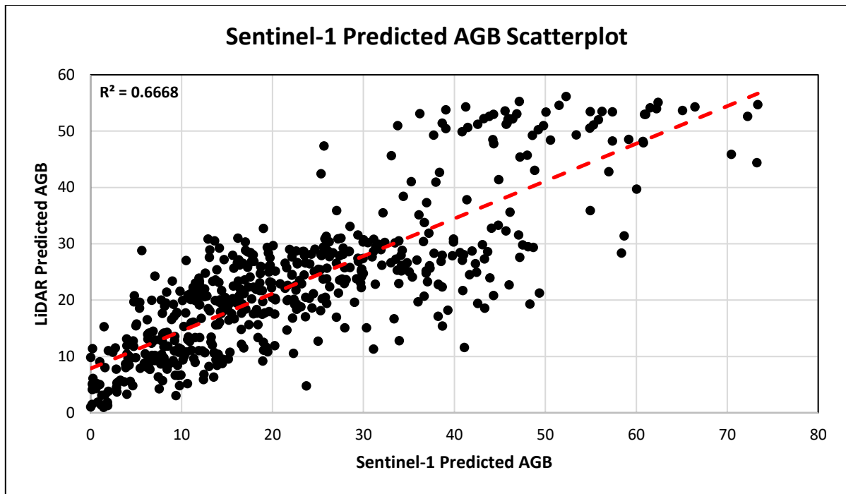
Figure 4. 6: Observed versus Predicted scatter plot Sentinel-1 using RF
