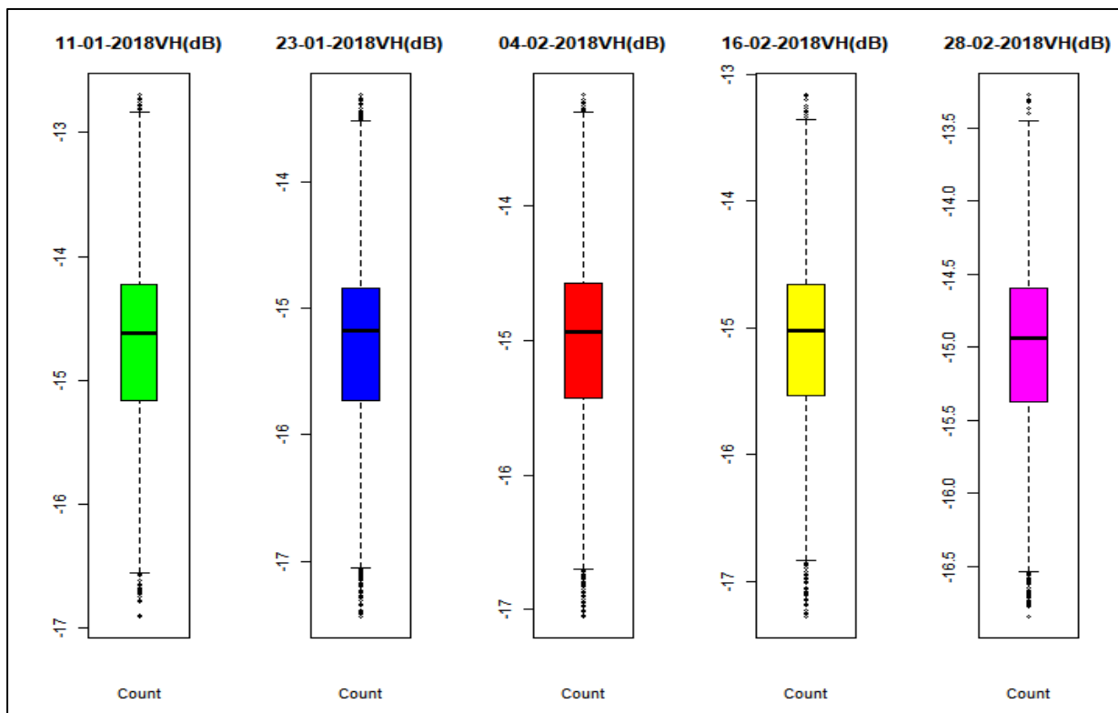
Figure 3. 6: Boxplots of Sentinel-1 VH time series
