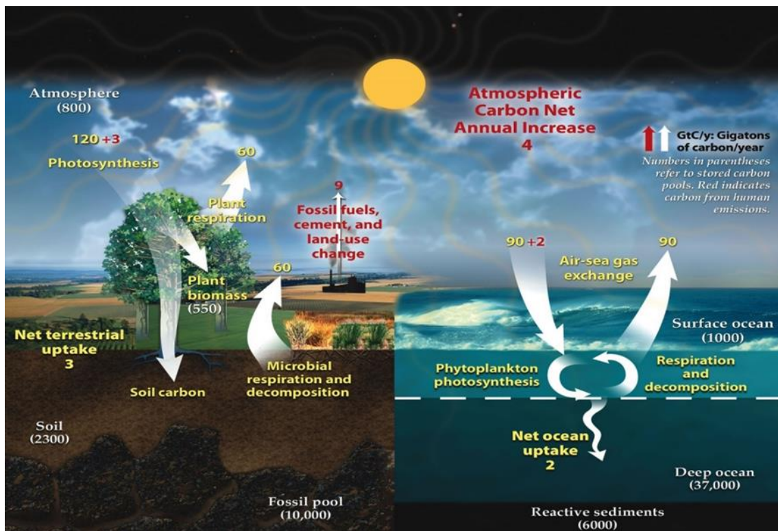
Figure 2. 1: The Fast carbon cycle (NASA, 2020)
