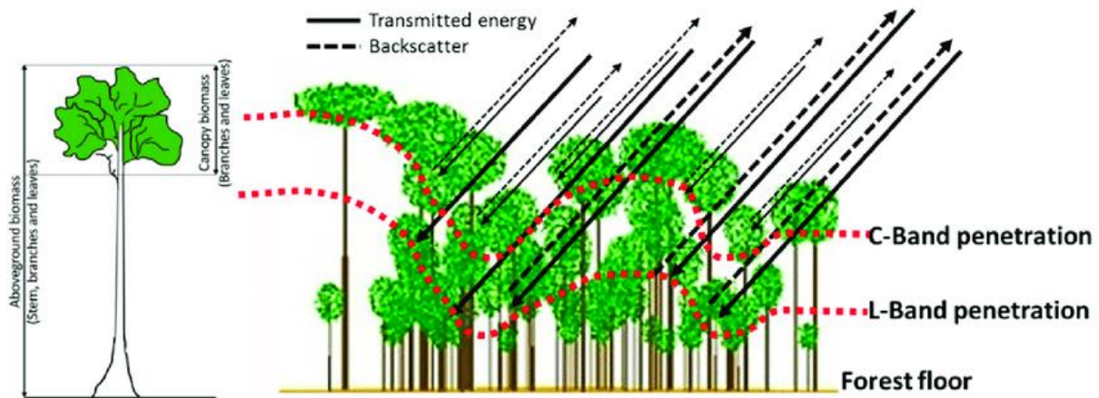
Figure 2. 2: Illustration of C and L band with vegetation interactions (Kumar et al., 2019)
