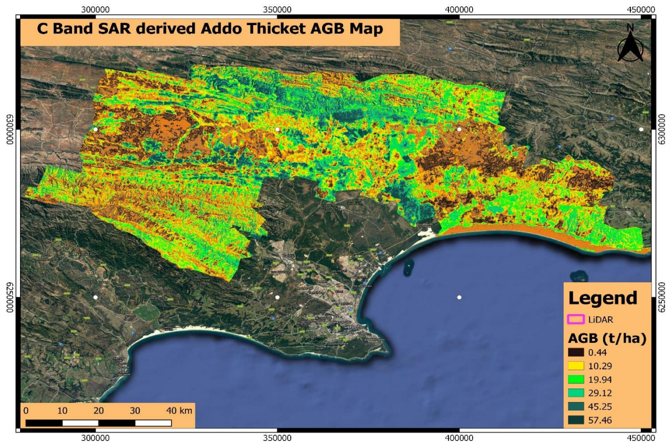
Figure 4. 9: Above Ground Biomass Map Over the Sunday River district
