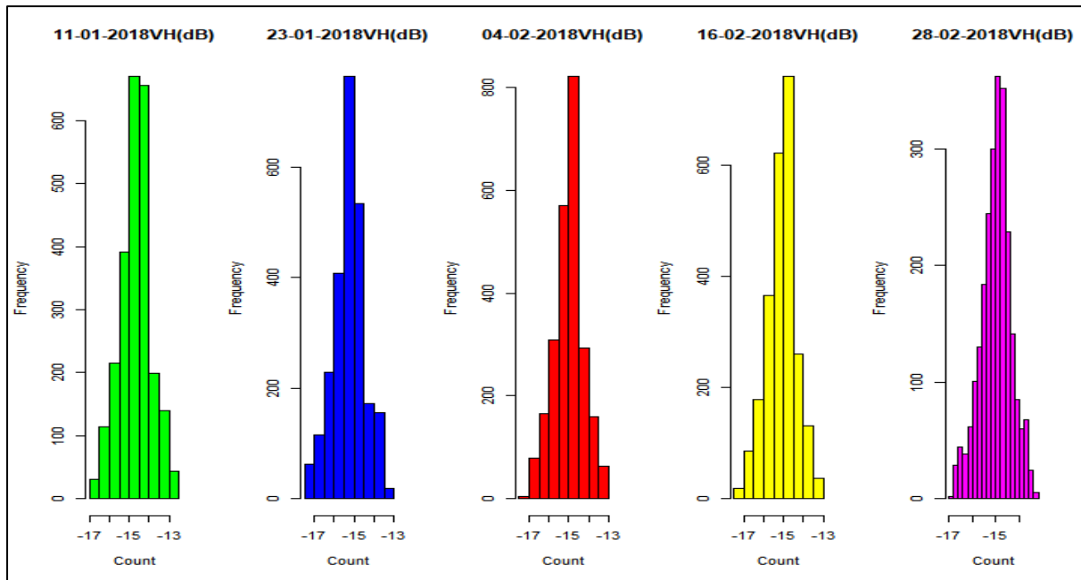
Figure 3. 5: Histograms of Sentinel-1 VH time series
