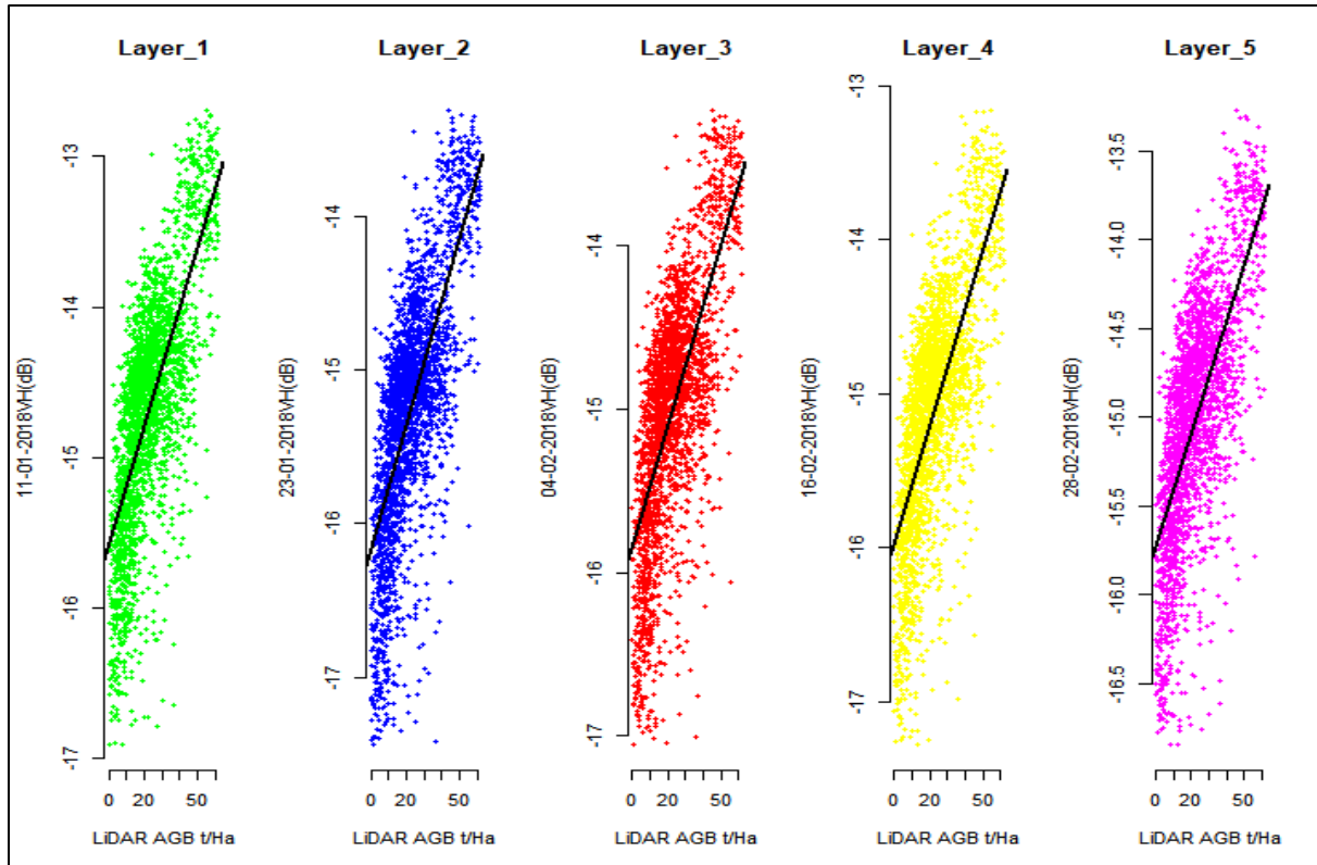
Figure 4. 8: The scatter plots of sampled AGB and SAR backscatter from Sentinel 1
