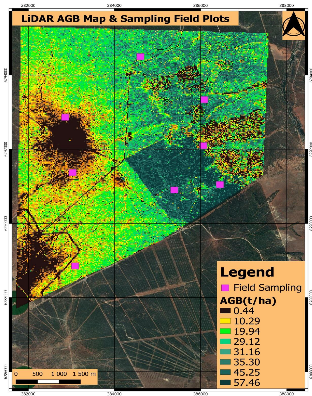
Figure 4. 3: LiDAR AGB map
