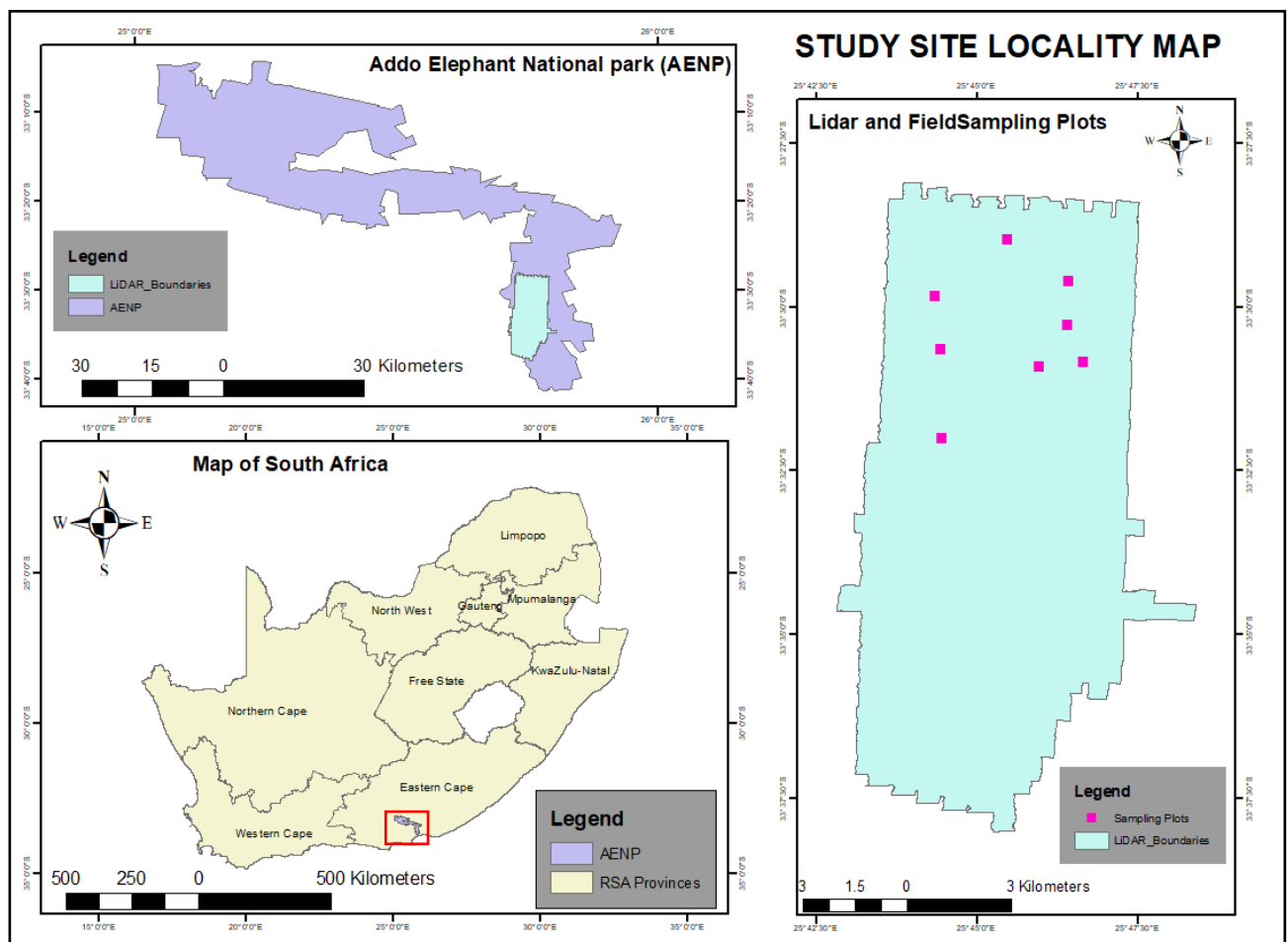
Figure 3. 1: Study locality map showing AENP located in the province of Eastern Cape, the LiDAR footprints and the field sample plots.
