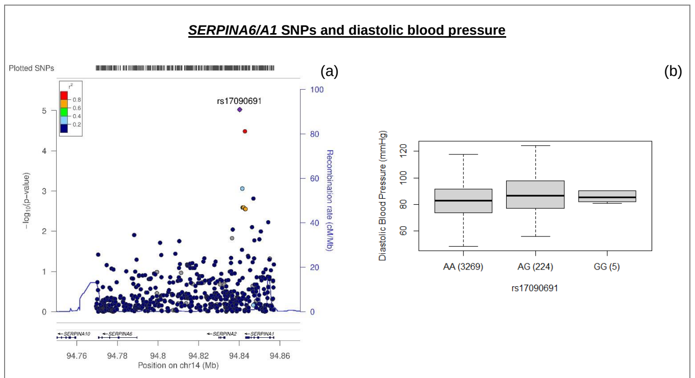
Figure 4.4: LocusZoom (a) and box and whisker (b) plots for the associations of rs17090691 at SERPINA6/A1 with diastolic blood pressure in men and women of African ancestry.
