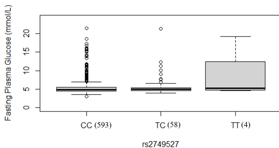
Figure S3.1: Fasting plasma glucose concentrations across the rs2749527 genotypes.
