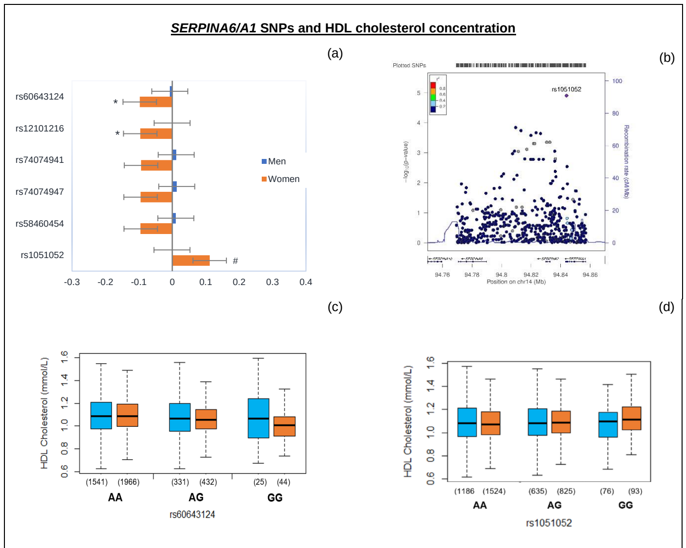
Figure 4.5: Sex-specific associations of SERPINA6/A1 SNPs with HDL cholesterol concentrations and in women of African ancestry.
