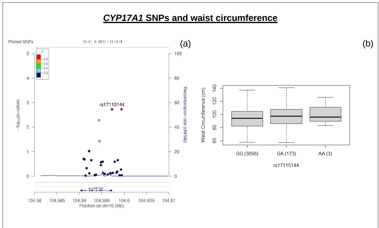
Figure 4.2: LocusZoom (a) and box and whisker (b) plots for the associations of rs17115144 at CYP17A1 with waist circumference in men and women of African ancestry.
