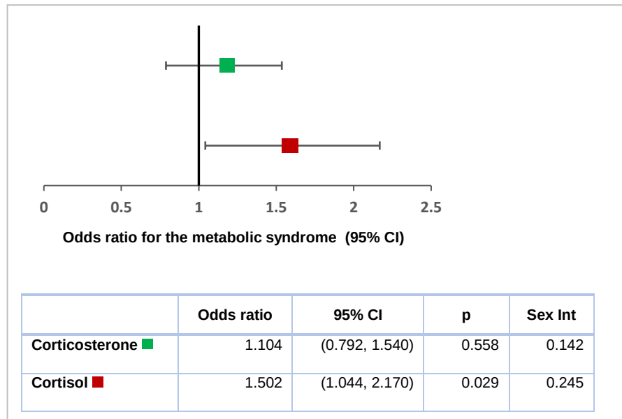
Figure 2.2: Associations between fasting serum glucocorticoid concentrations and odds of developing the metabolic syndrome.
