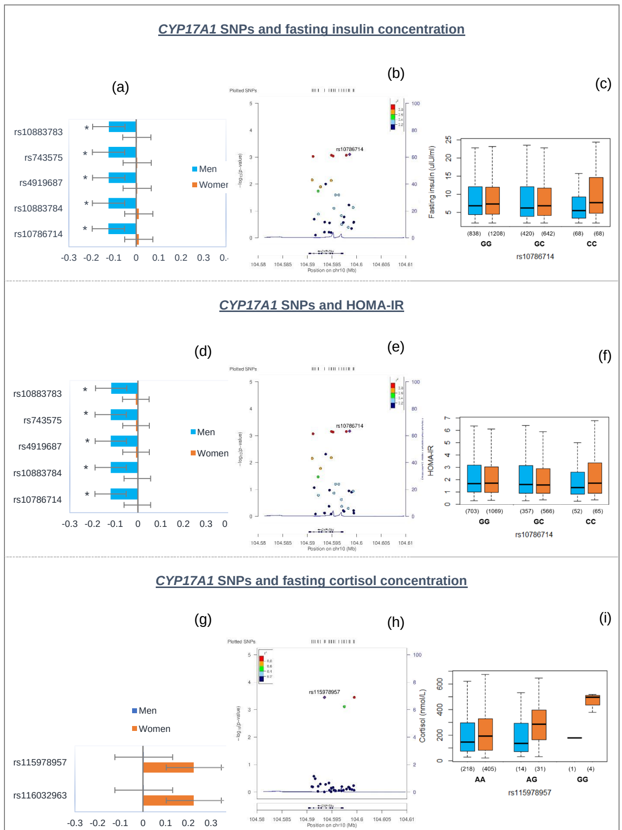
Figure 4.3: Sex-specific associations of CYP17A1 SNPs with fasting insulin concentrations and HOMA-IR (a-f), and fasting cortisol concentrations in men and women of African ancestry (g-i). Plots (a), (d) and (g) show
