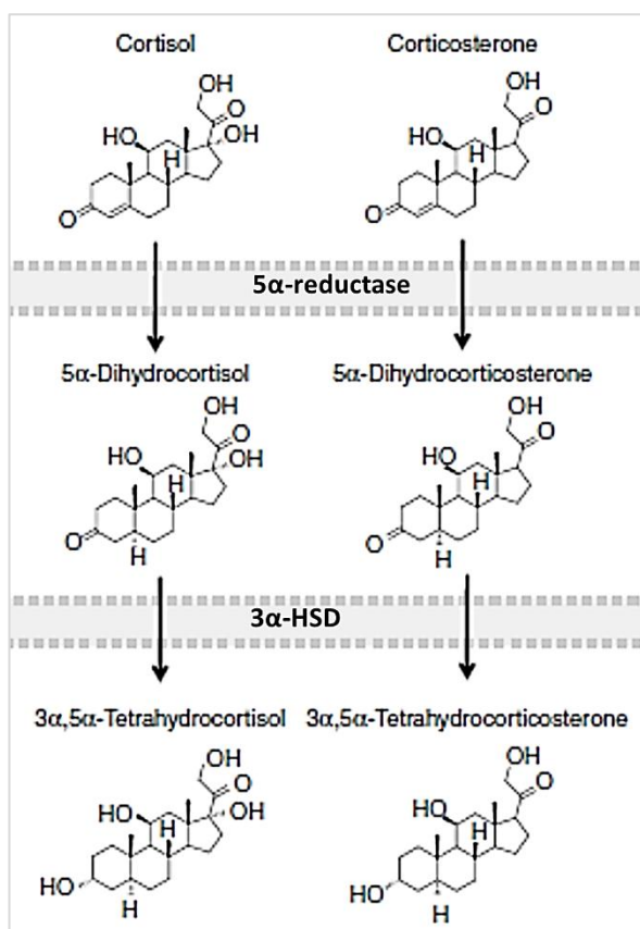
Figure 1.9: Metabolic clearance of glucocorticoids by 5α-reductase and 3α-HSD, to generate tetrahydro-glucocorticoids. Figure used with permission (166).
