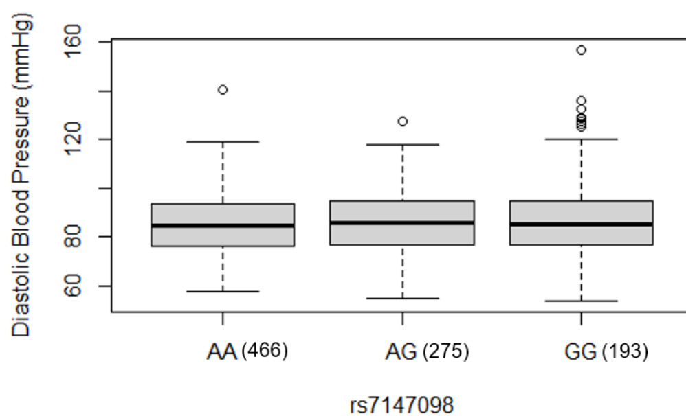
Figure S3.2: Diastolic blood pressure across the rs7147098 genotype.
