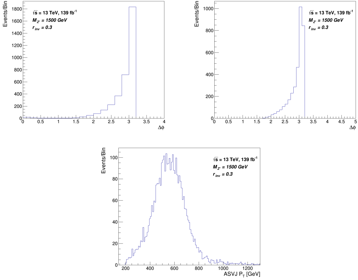
Figure 3.5: The distribution of the \Delta\phi between the farthest jet and MET (left) which selects the asvj, \Delta\phi between leading jet and MET (right) and the p_T of the asvj (bottom).
