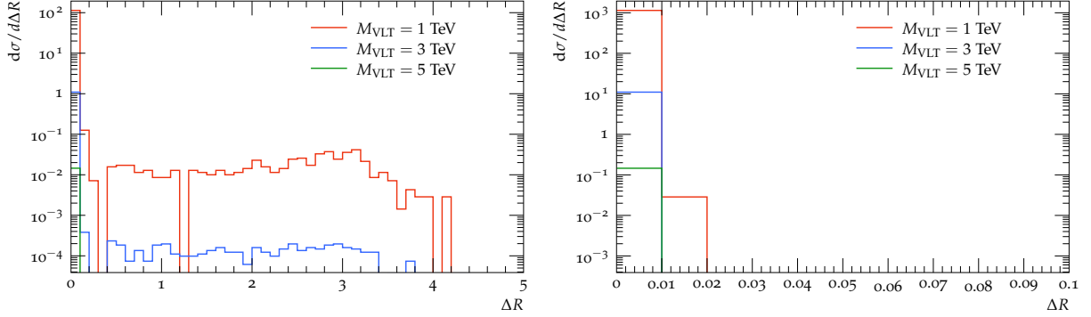
Figure 2.19: Distributions for \Delta R between the leading electron and the closest J_4 (left) and \Delta R between the two electrons originating from the dark photon (right) for the three masses considered, corresponding to VLT masses of 1, 3 and 5 TeV.
