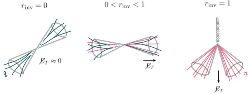
Figure 3.1: Diagram showing the jet topology and MET direction for different r_{inv} values, where the green lines are visible particles and the red are invisible.
