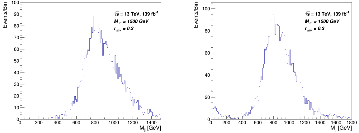
Figure 3.6: Invariant mass of leading and sub-leading jets (left) and svj and anti-svj (right)
