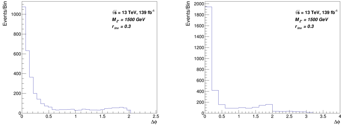
Figure 3.4: The distribution of the \Delta\phi between the closest jet and MET (left) which selects the svj and \Delta\phi between the subleading jet and MET (right).
