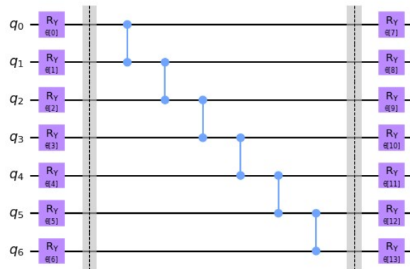
Figure 4.9: Circuit representation of R_Y and CZ gate for 7 qubit TwoLocal ansatz.
