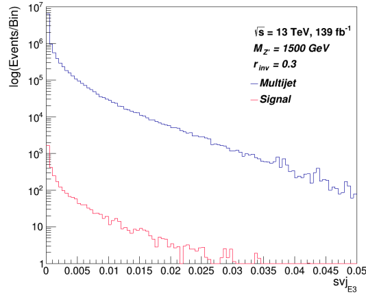
Figure 3.13: E3 substructure distribution for svj against multijet background.
