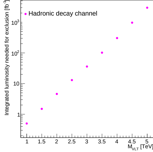
Figure 2.24: The minimum integrated luminosity needed in order to exclude VLT mass points, if no events are observed, be we can expect at least three signal events.
