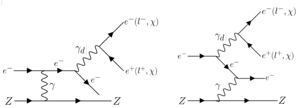
Figure 2.2: Feynman diagrams showing dark photon \gamma_d emitted from an electron in the final state (left) and initial state radiation (ISR) (right).
