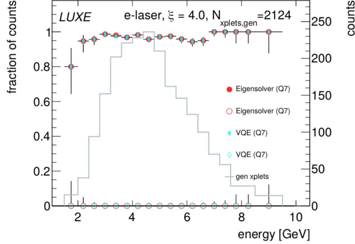
Figure 4.11: Efficiency rate of a track selected being a real track to a fake track against the particles true energy.
