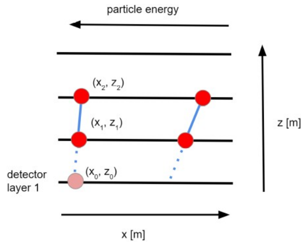
Figure 4.7: Formation of doublets and selection requirements.
