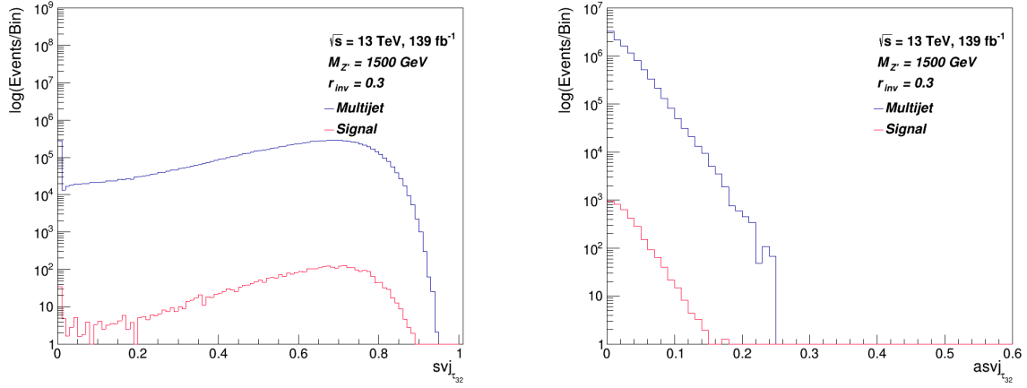
Figure 3.12: \tau_{32} distribution for svj and anti- svj (left and right respectively) against multijet background.
