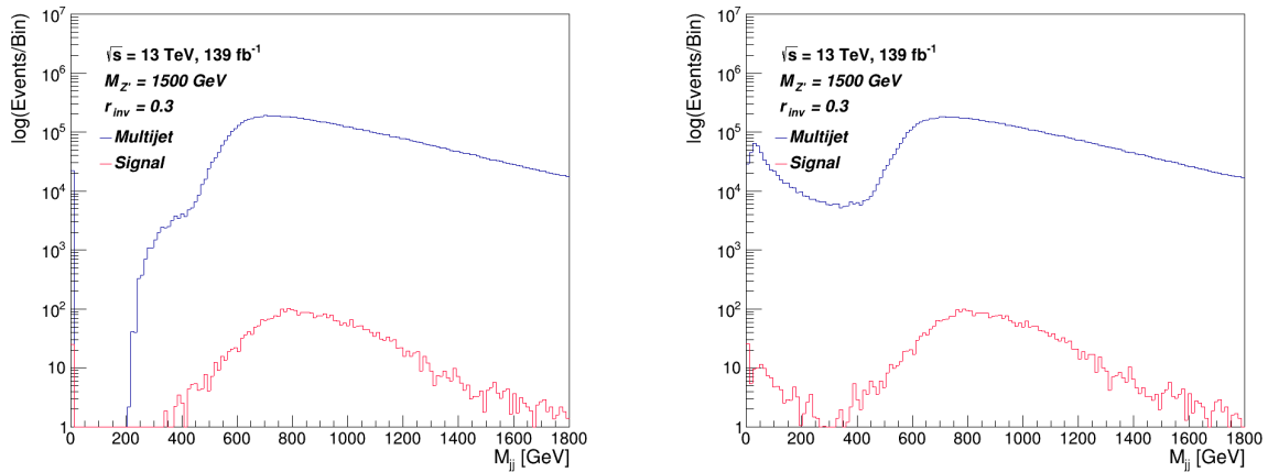
Figure 3.16: Invariant mass for signal against multijet for leading and sub-leading jet (left) and the svj and anti-svj (right).
