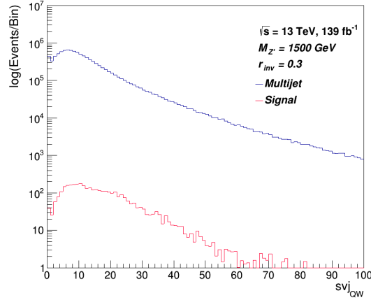
Figure 3.15: Q_W distribution for svj against multijet background.
