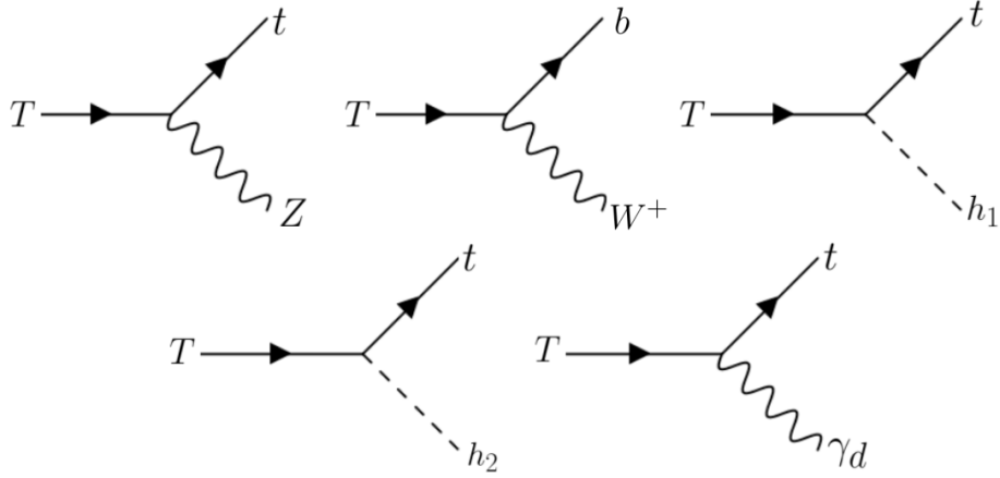
Figure 2.10: Representative Feynman diagrams for VLT decays to Zt , Wb , h_1t (top) and since T is charged under both the SM and U(1) , it can decay to h_1 and h_2 . Where h_1 is the observed Higgs boson and h_2 is a new scalar boson.
