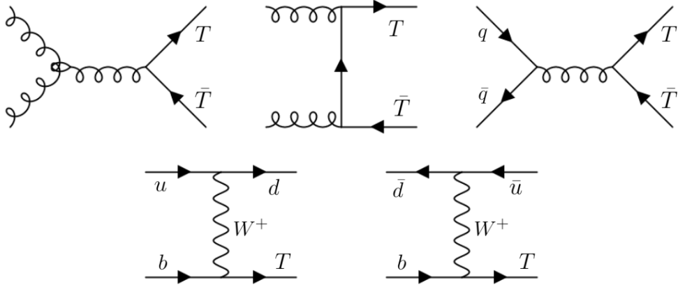
Figure 2.9: Standard VLT production modes for pair production (top) and single production with a jet (bottom) [1].
