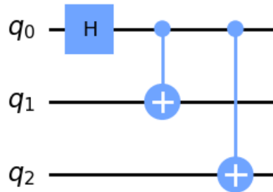
Figure 4.6: Quantum circuit for three qubits under Hadamard and CNOT gate operations
