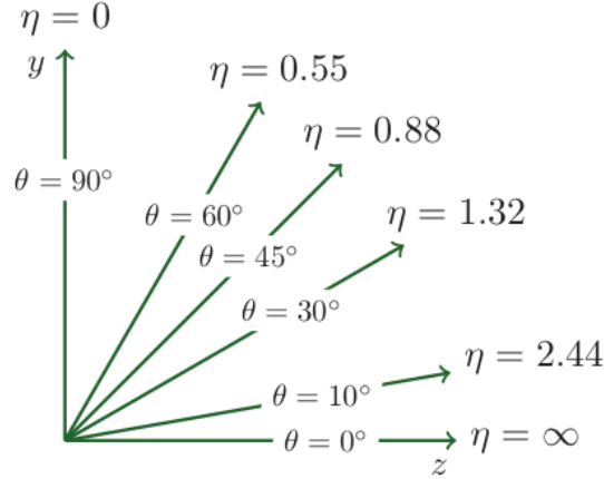
Figure 1.7: Pseudorapidity, \eta , defined to exploit cylindrical symmetry, the value of \eta increases as we move away from the center of the detector [24].
