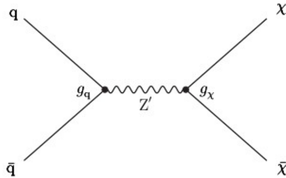
Figure 3.3: Feynman diagram of the leading-order resonant production of dark quarks through a Z' mediator, with relevant couplings to SM quarks ( g_q ) and dark quarks ( g_\chi ) indicated at the vertices.
