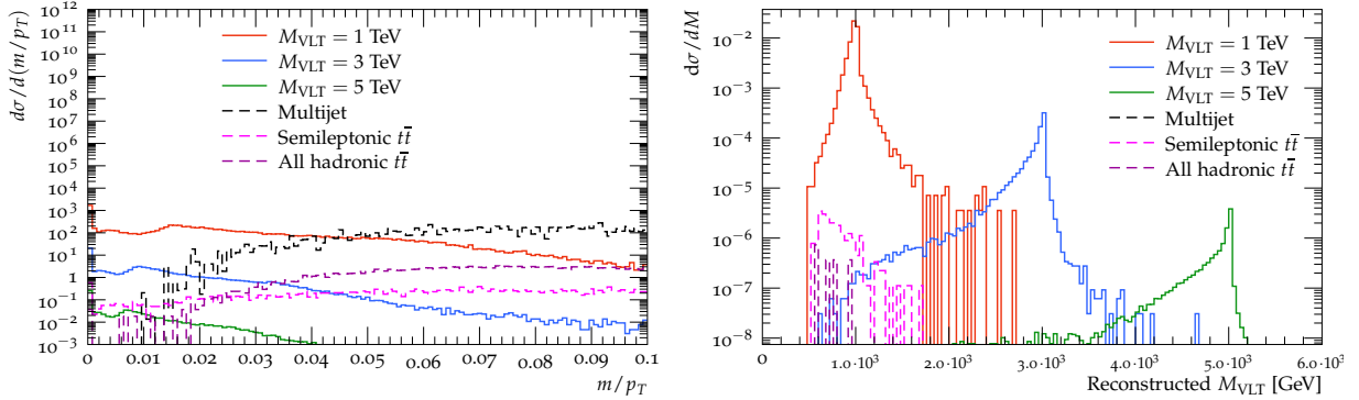
Figure 2.23: Distributions of the lepton jet candidate m/p_T ratio before applying m/p_T > 0.01 requirement (left) and VLT reconstructed mass after applying this requirement (right) for the three masses considered, corresponding to VLT masses of 1, 3 and 5 TeV, with the dominant background processes shown.
