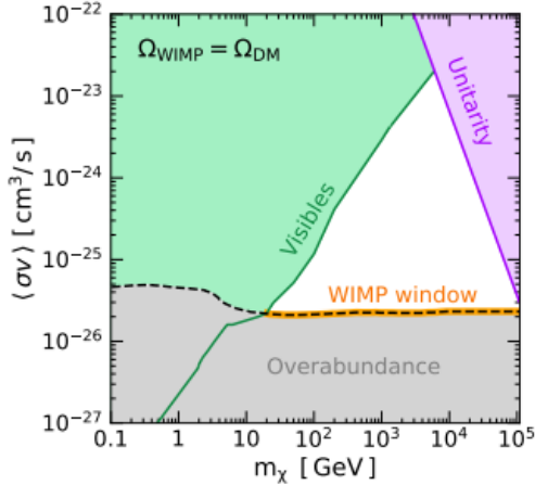
(a) Bounds on generic thermal WIMP window assuming WIMP DM is 100% of all DM.
