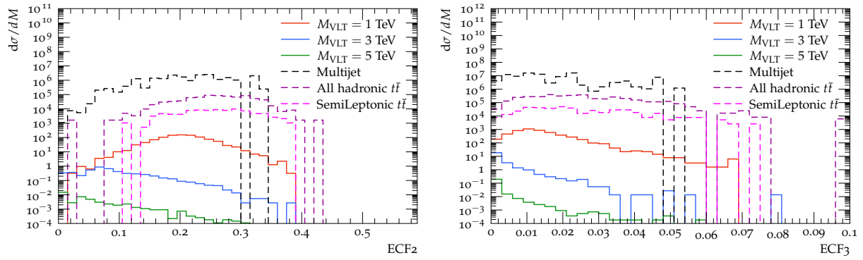
Figure 2.15: Plot showing ECF2 (left) and ECF3 (right) distributions for signal for the three masses considered, corresponding to VLT masses of 1, 3 and 5 TeV, with the dominant background processes shown.
