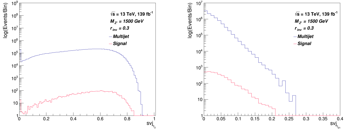
Figure 3.11: \tau_3 and \tau_{21} (left and right respectively) distribution for svj against multijet background.
