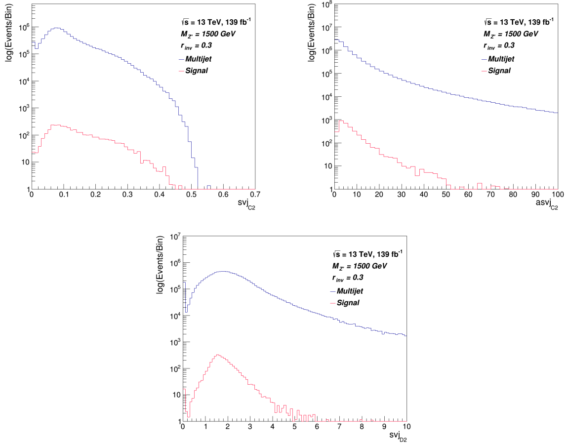
Figure 3.9: C2 distribution for svj and anti-svj (left and right respectively) and D2 distribution for svj against multijet background.
