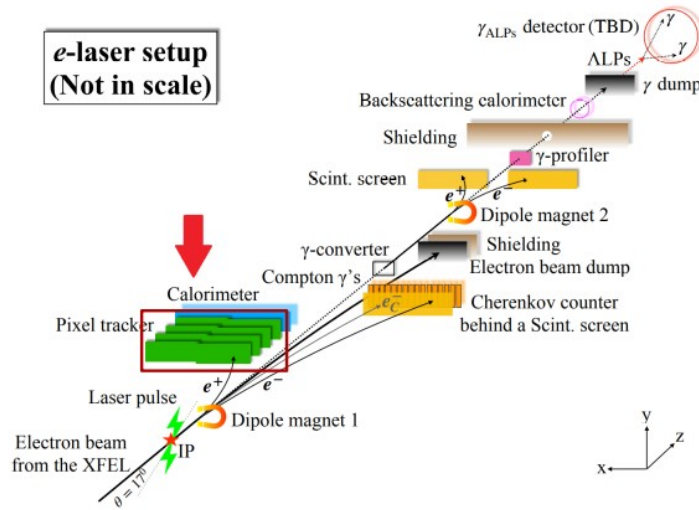
Figure 4.2: Schematic layout of LUXE for e -laser setup [105]
