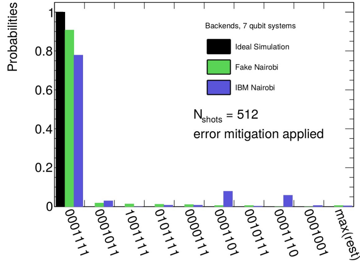
Figure 4.10: Comparison between ideal simulation, fake quantum device accounting for noise and the real quantum device.
