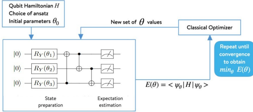
Figure 4.8: Diagram of VQE algorithm recreated from ref-[108]
