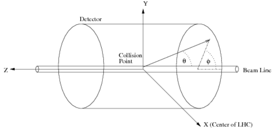
Figure 1.6: Illustration of general detector co-ordinate system [23].
