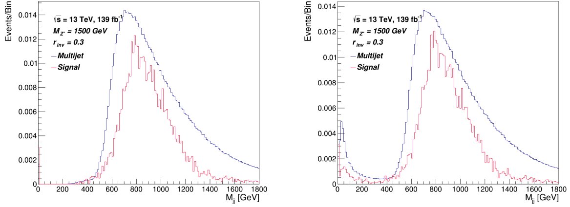
Figure 3.19: Invariant mass for signal against multijet for leading and sub-leading jet (left) and the svj and anti-svj (right) area normalised.
