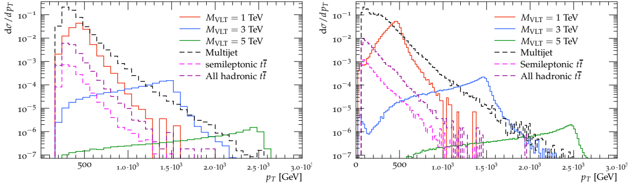
Figure 2.21: Distributions of the p_T for the top jet candidate (left) and the lepton jet (right) for the three masses considered, corresponding to VLT masses of 1, 3 and 5 TeV, with the dominant background processes shown.
