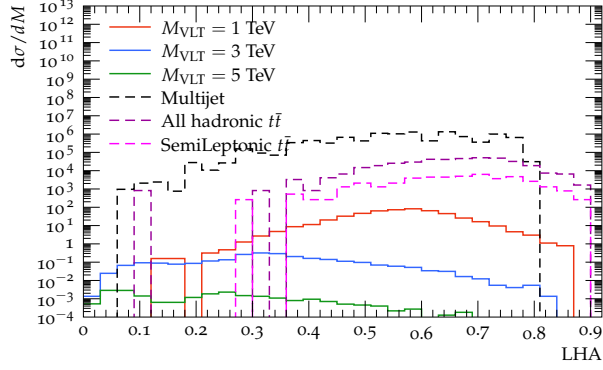
Figure 2.17: LHA distribution for signal for the three masses considered, corresponding to VLT masses of 1, 3 and 5 TeV, with the dominant background processes shown.
