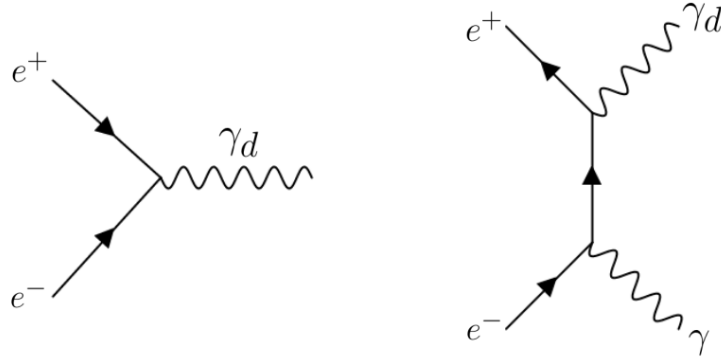
Figure 2.5: Feynman diagrams for the dark photon \gamma_d production via the resonant e^+e^- \rightarrow \gamma_d (left) and non resonant e^+e^- \rightarrow \gamma_d\gamma (right) electron-positron annihilation.
