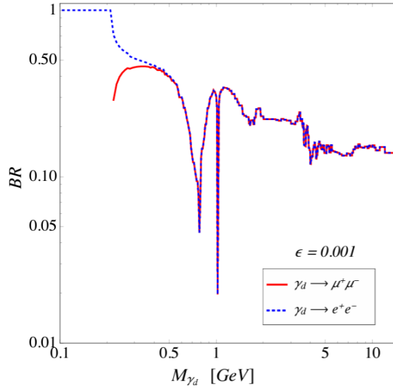
Figure 2.11: Branching ratios of \gamma_d as a function of its mass M_{\gamma_d} , into an electron-positron pair ( e^-e^+ ) given by dotted blue line and muon-antimuon pair ( \mu^-\mu^+ ) given by solid red line, where \varepsilon = 0.001 [1].
