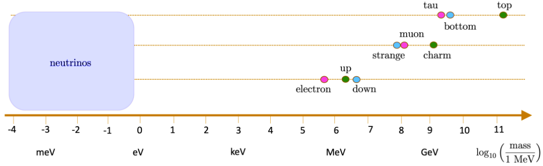
Figure 1.2: Figure showing the mass differences between generations for quarks and leptons.
