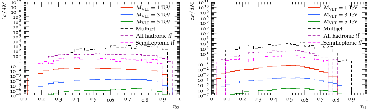
Figure 2.14: Plot showing \tau_{32} (left) and \tau_{21} (right) distributions for signal for the three masses considered, corresponding to VLT masses of 1, 3 and 5 TeV, with the dominant background processes shown.
