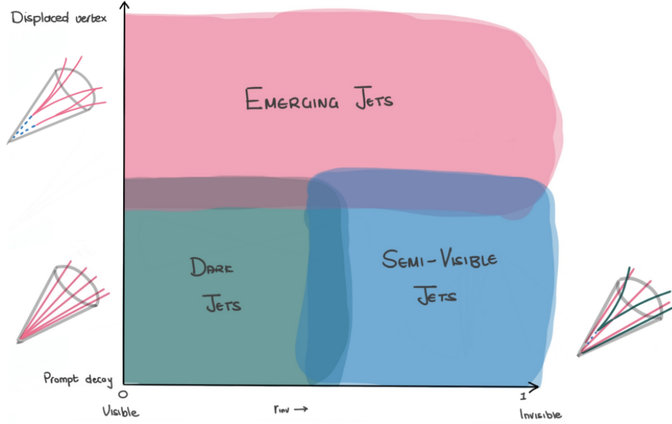
Figure 3.2: Diagram showing a basic classification of jets with respect to decay distance from vertex and different r_{inv} values.
