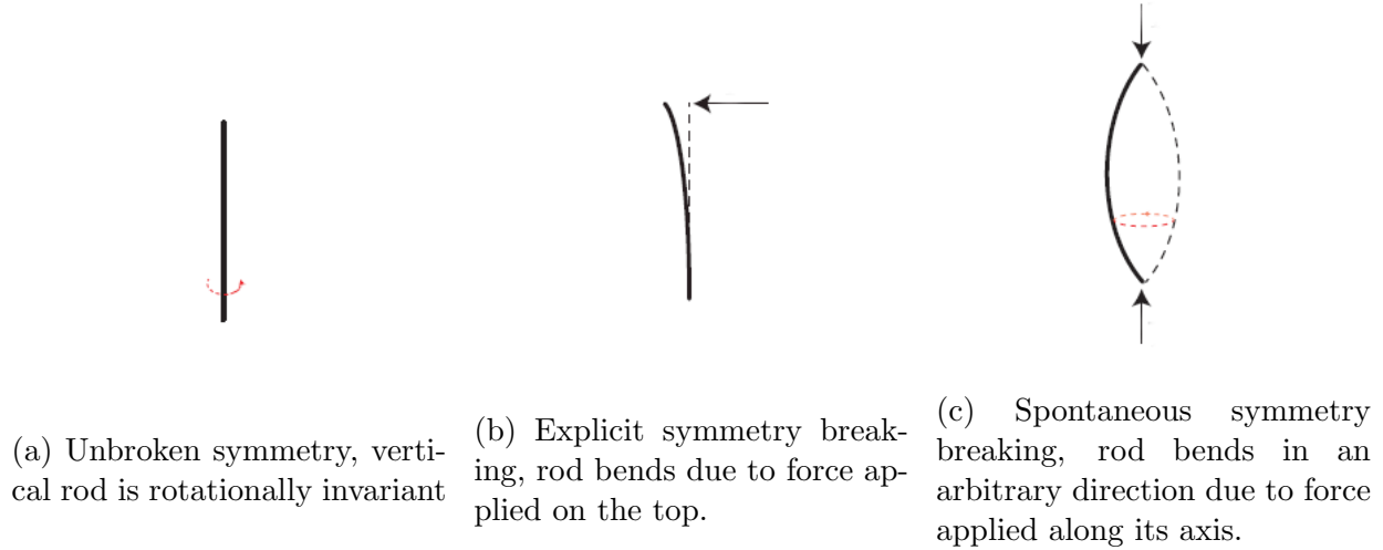
Figure 1.4: Spontaneous symmetry breaking demonstrated by a bending vertical rod.
