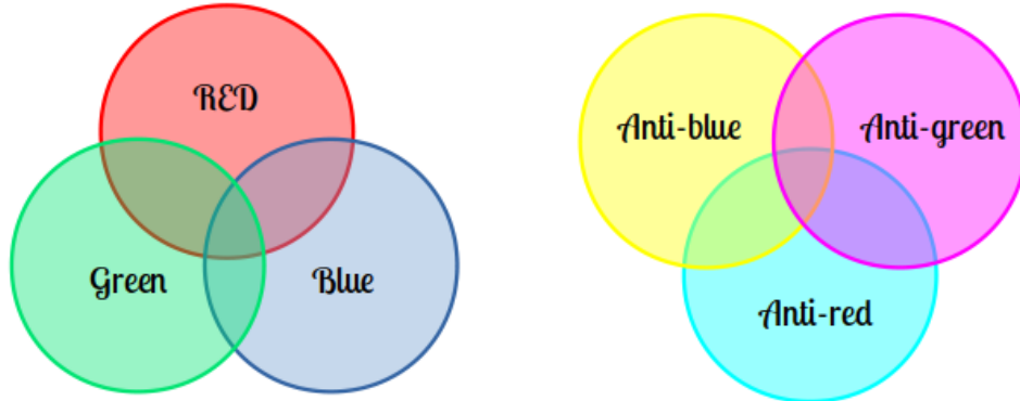
Figure 1.3: The quark colour charges, (red, green, blue) and anti-quark colour charges (anti-red, anti-green, anti-blue) which combine to be colourless.
