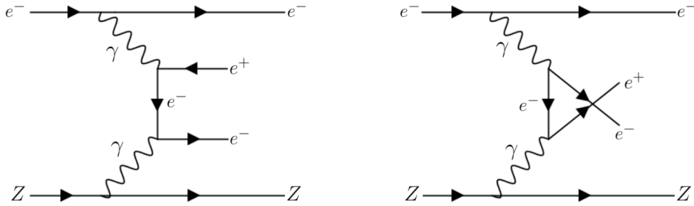
Figure 2.3: Feynman diagrams of the QED Bethe-Heitler (space-like) trident reactions. It may appear as though the lower photon is radiated forwards in time from the Z boson upwards, however this is not the case, for this process the lower photon is radiated by the electron. In the diagram on the right the two final state electrons are swapped.
