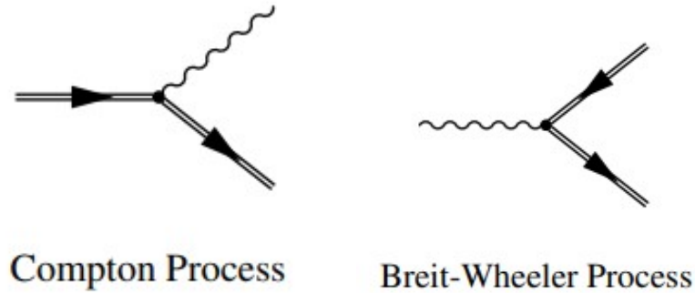
Figure 4.1: Feynman diagrams showing processes for the non-linear Compton scattering and Breit-Wheeler pair production in the non-perturbative regime from Ref [105].
