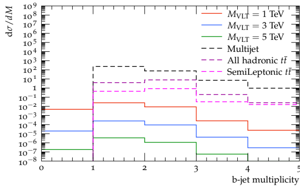
Figure 2.18: Number of b -jets for signal for the three masses considered, corresponding to VLT masses of 1, 3 and 5 TeV.
