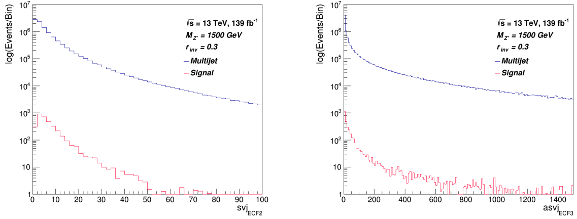
Figure 3.8: ECF2 distribution for svj (left) and ECF3 distribution for anti-svj (right) against multijet background.
