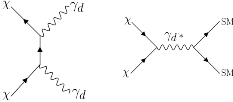
Figure 2.1: Feynman diagrams showing dark photon production via \chi\chi \rightarrow \gamma_d\gamma_d (left) and the resonant production of SM particles \chi\chi \rightarrow \gamma_d \rightarrow \text{SM SM} (right).
