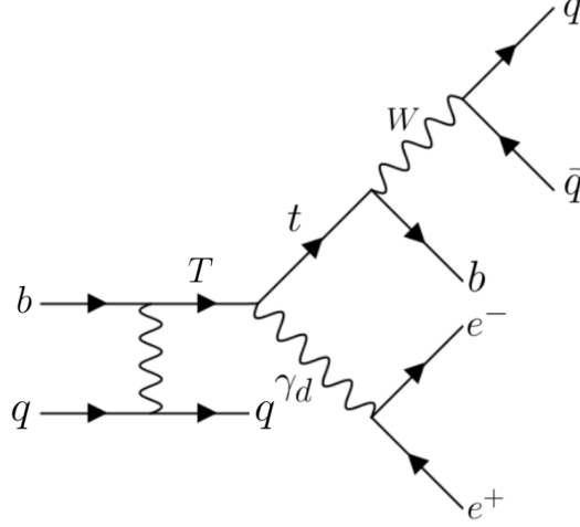
Figure 2.12: Feynman diagram showing the production and hadronic decay of VLT to a dark photon and top quark and the dark photon production from the VLT and its decay to a lepton jet.
