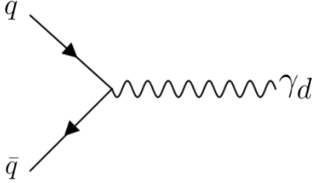
Figure 2.8: Feynman diagram showing Drell Yan production of a dark photon.
