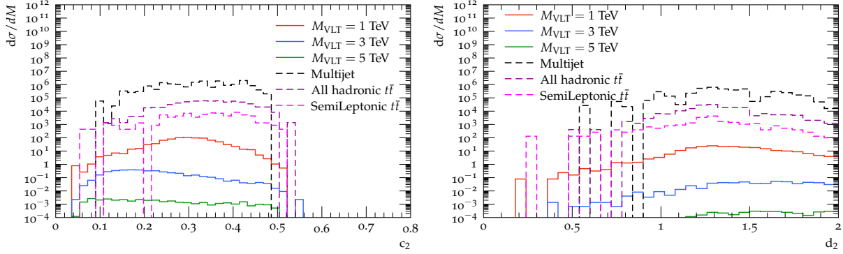
Figure 2.16: Plot showing C_2 (left) and D_2 (right) distributions for signal for the three masses considered, corresponding to VLT masses of 1, 3 and 5 TeV, with the dominant background processes shown.
