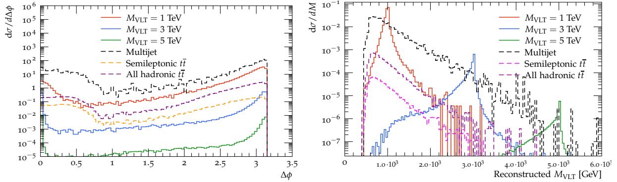
Figure 2.22: \Delta\phi between the lepton jet and top jet (left) and the invariant mass of the VLT top partner is reconstructed from the four-momenta of the top jet and lepton jet candidates (right) for the three masses considered, corresponding to VLT masses of 1, 3 and 5 TeV, with the dominant background processes shown.
