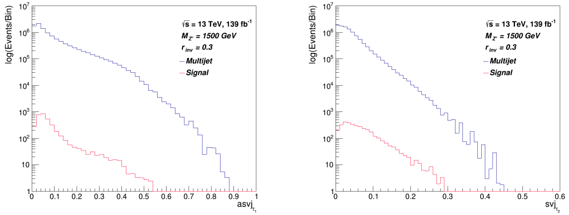
Figure 3.10: \tau_1 (left) distribution for anti-svj and, \tau_2 (right) distribution for svj against multijet background.
