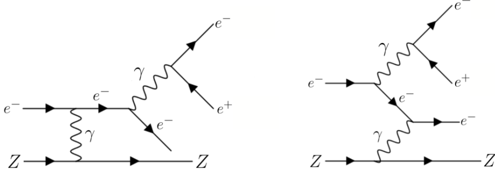
Figure 2.4: Feynman diagrams of the QED radiative (time-like) tridents reactions.
