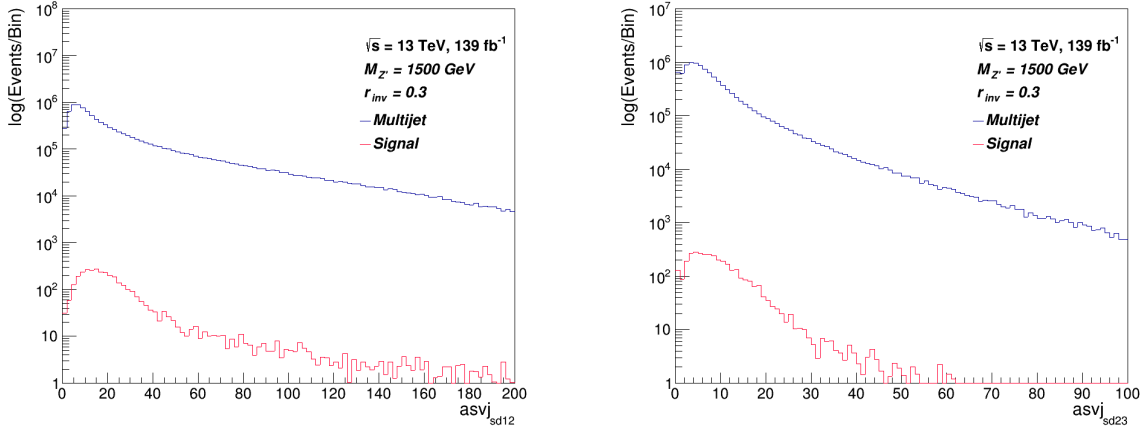
Figure 3.14: sd_{12} and sd_{23} distributions for anti-svj (left and right respectively) against multijet background.
