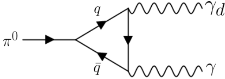
Figure 2.7: Feynman diagram showing neutral meson decay to dark photon and standard model photon.
