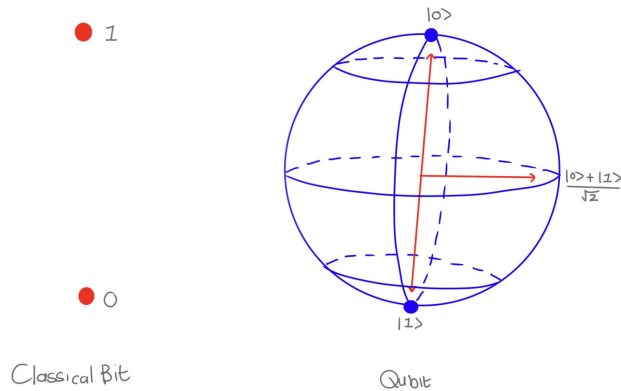
Figure 4.3: Classical bit representation (left) and Bloch sphere representation of the qubit (right).
