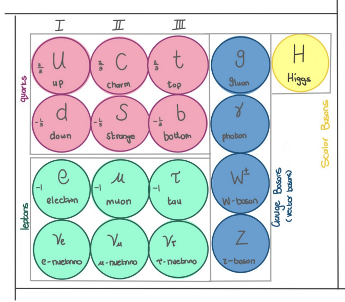
Figure 1.1: Summary of SM, the pink and turquoise circles show the fermions and represent the three generations of quarks and leptons. The blue circles represent the gauge boson where g is the gluon, \gamma is the photon and W and Z are the W and Z boson. The yellow circle is the scalar Higgs boson.
