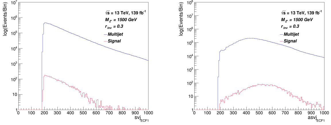
Figure 3.7: ECF1 for svj and anti-svj signal (left and right respectively) against multijet background.
