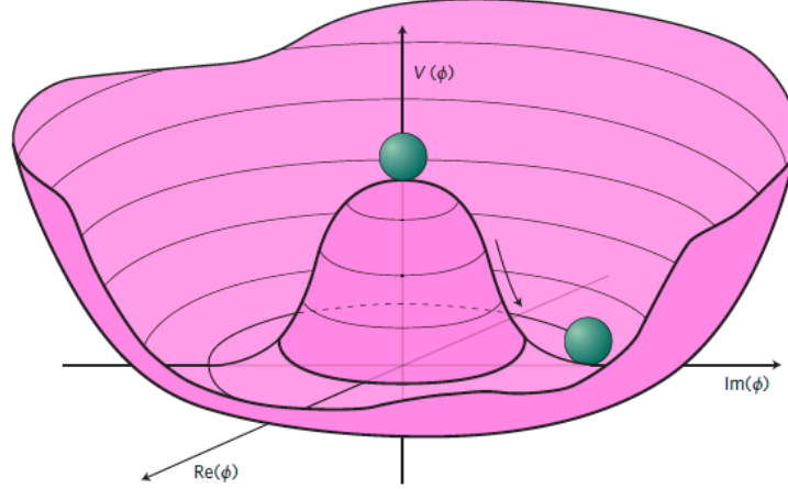
Figure 1.5: Shape of the potential of a complex scalar field, having an infinite number of degenerate minima rotated by the phase rotation, leading to SSB [16].
