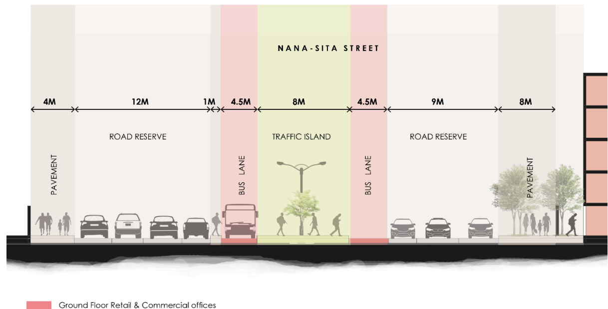
Figure 9: A sectional elevation A-A of Nana-Sita. (Drawn by Tswai, 2021).
