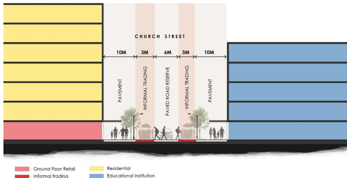
Figure 3: a sectional elevation A-A of Church street. (Drawn by Tswai, 2021).
