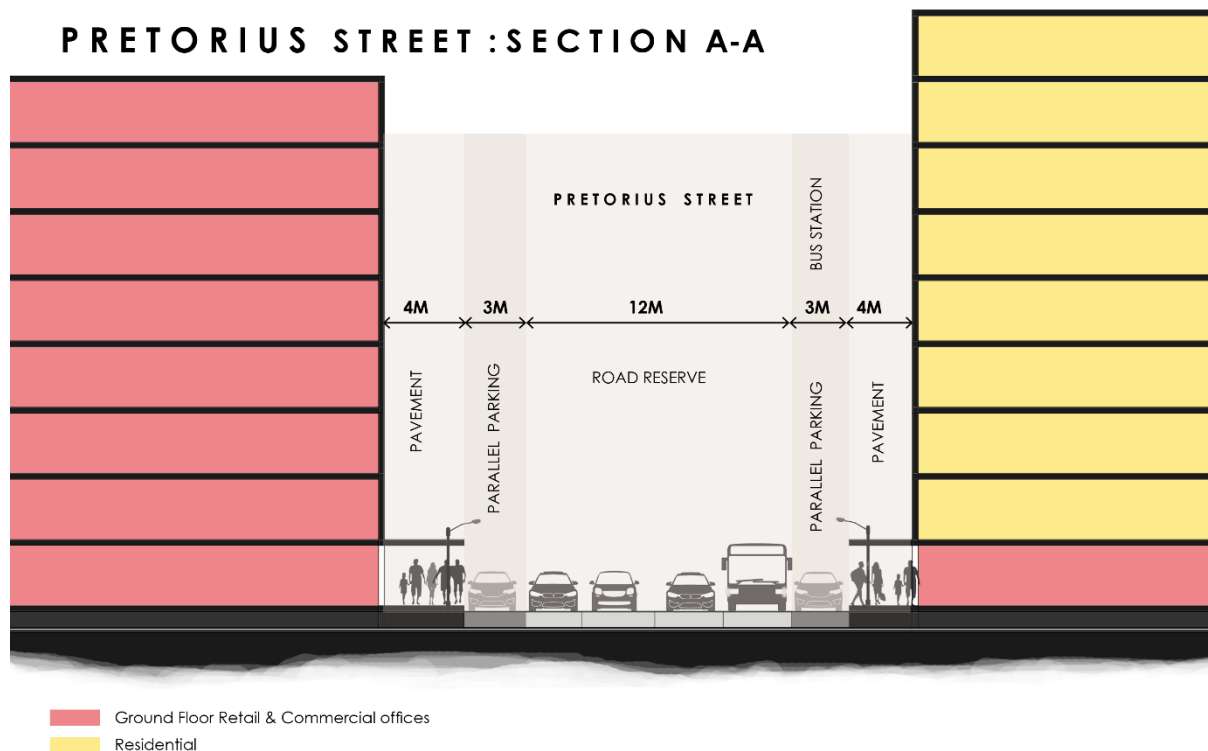
Figure 6: A sectional elevation A-A of Pretorius street. (Drawn by Tswai, 2021).
