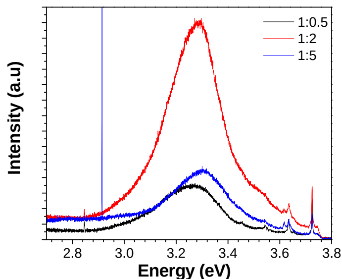
Fig. 6.7: Room temperature PL spectra of the GaN nanostructures with different ratios of \text{Ga}_2\text{O}_3/\text{C} using the 325 nm excitation.
