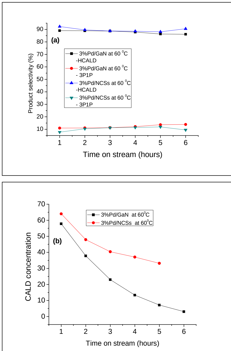
Fig. 7.6: Graphs showing (a) the product selectivity to HCALD and 3P1P (b) CALD remaining as a function of time on stream at 60°C for 3%Pd/GaN and 3% Pd/NCSs catalysts.
