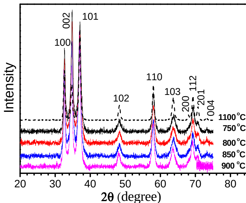
Fig. 4.3: PXRD pattern of GaN nanostructures synthesized using \text{Ga}_2\text{O}_3 and \text{NH}_3 at various growth conditions. Spectra are shifted vertically for clarity.
