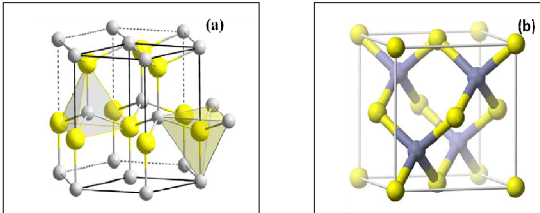
Fig. 2.1: Crystal structure of (a) Wurtzite GaN and (b) Zinc-blende GaN [17].
