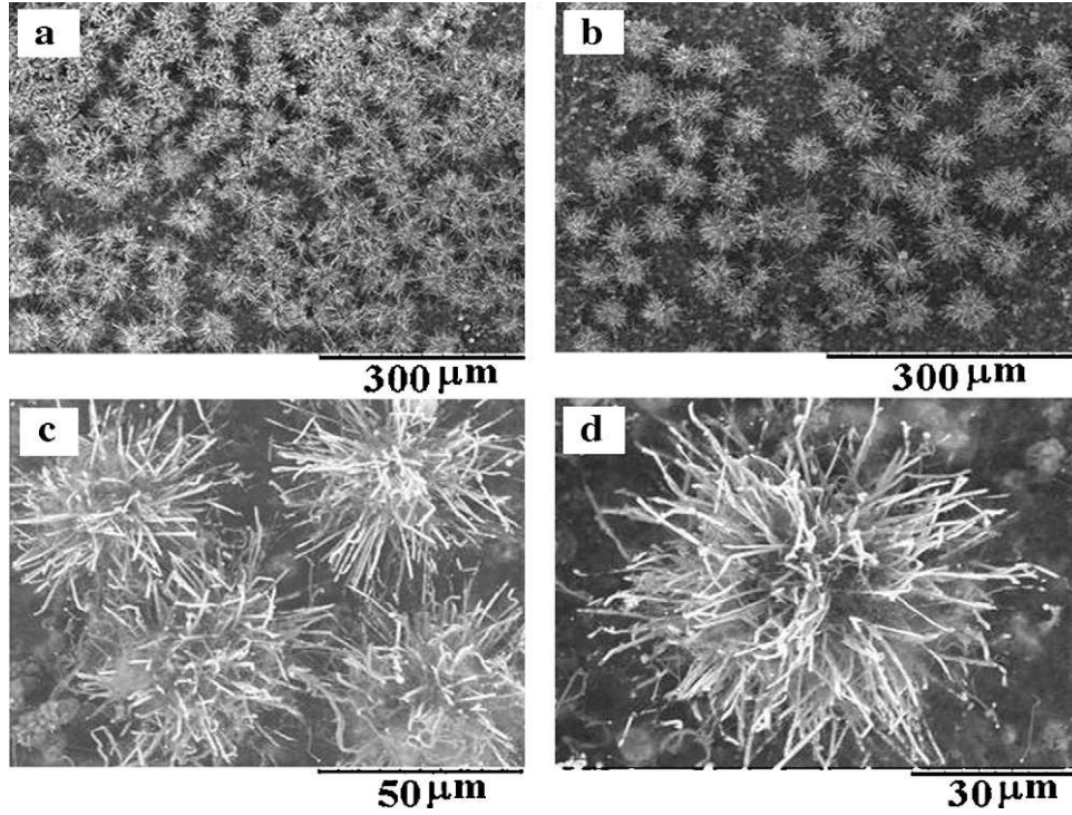
Fig. 2.14: (a and b) shows the low magnification images and (c and d) shows high magnification of SEM images of dandelion-like GaN microstructures [52].
