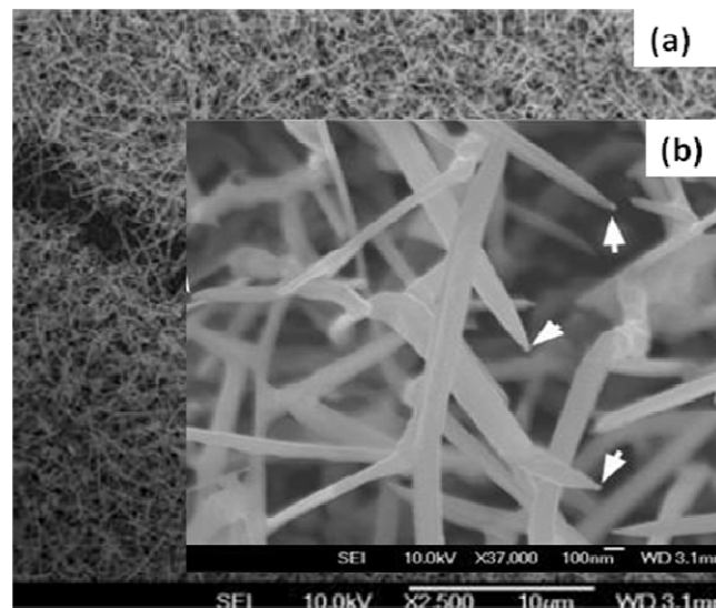
Fig. 2.18: (a) Low magnification and (b) high magnification SEM images for the needle-like GaN nanowires [55].
