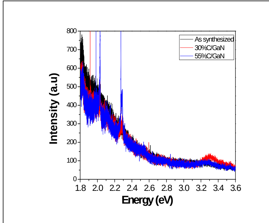
Fig. 5.8: Room temperature PL spectra for GaN/C and fGaN/C.
