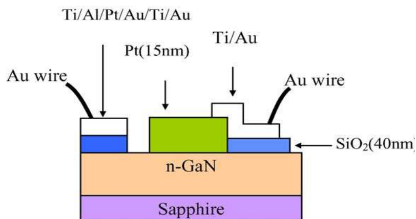
Fig. 2.25: Schematic of Pt/GaN Schottky diode for hydrogen gas sensing [86].
