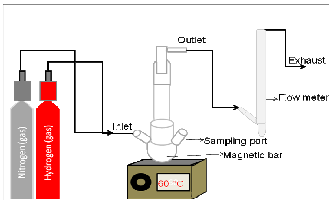
Fig. 3.3: Reaction setup used for hydrogenation reaction.
