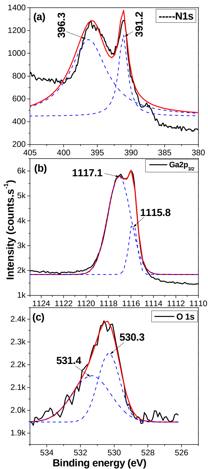
Fig. 4.7. Typical high resolution binding energy spectra of the N1s (a), Ga2p 3/2 (b) and O1s (c) observed in the GaN nanostructures synthesized at 900 °C in the two stage furnace.
