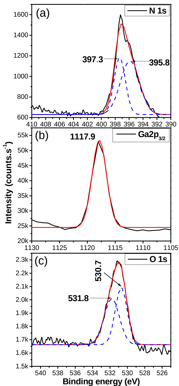
Fig. 4.5. Typical high resolution binding energy spectra of the N1s (a), Ga2p 3/2 (b) and O1s (c) observed in the GaN nanostructures synthesized at 800 °C in the two stage furnace.
