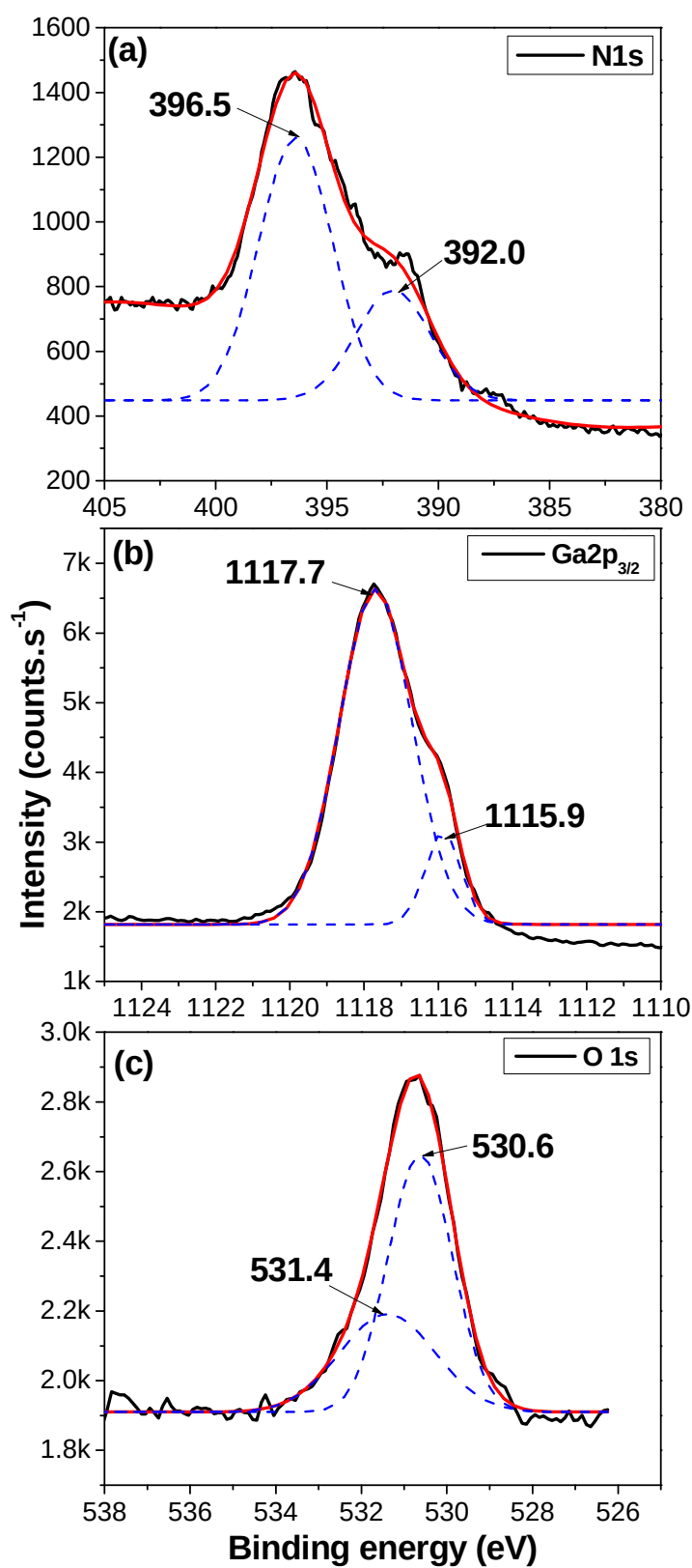
Fig. 4.8. Typical high resolution binding energy spectra of the N1s (a), Ga2p 3/2 (b) and O1s (c) observed in the GaN nanostructures synthesized at 1100 °C in the single stage furnace.
