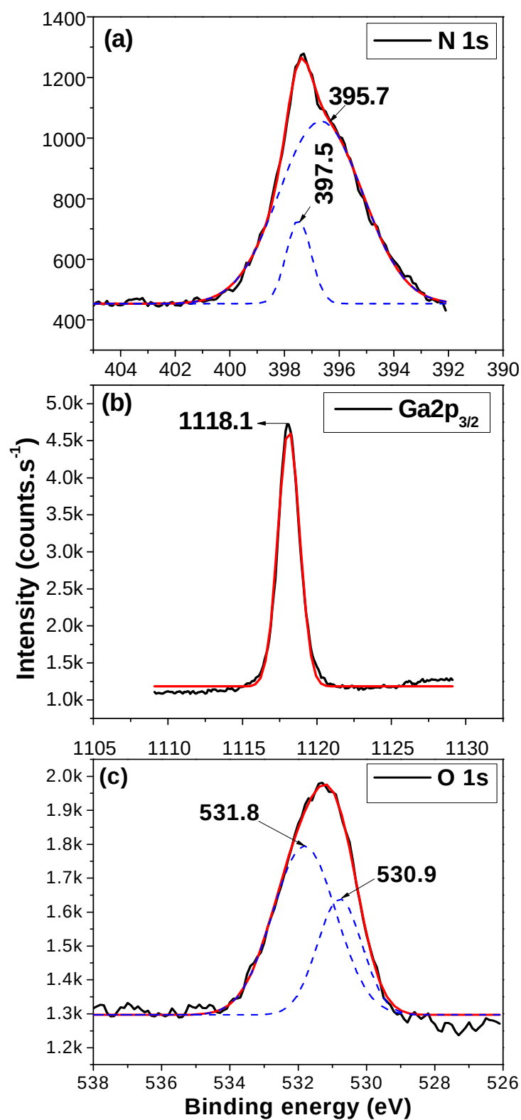
Fig. 4.6. Typical high resolution binding energy spectra of the N1s (a), Ga2p 3/2 (b) and O1s (c) observed in the GaN nanostructures synthesized at 850 °C in the two stage furnace.
