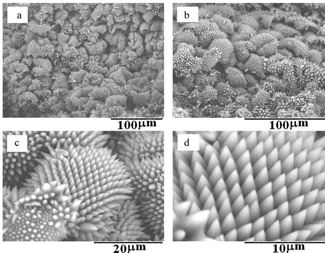
Fig. 2.13: (a and b) Low magnification SEM images of durian-like GaN. (c) Medium magnification of durian-like GaN. (d) High magnification images of durian-like GaN having sharp tips [51].
