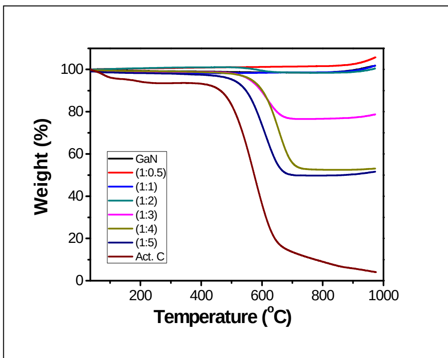
Fig. 6.4: TGA profiles of GaN NSs synthesized with and without activated carbon at 1100 °C.
