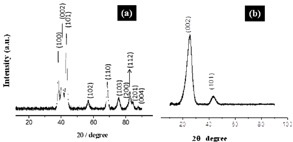
Fig.7.2: PXRD patterns of (a) as-synthesized GaN NSs (synthesis temp = 750 °C) and (b) as-synthesized NCSs.
