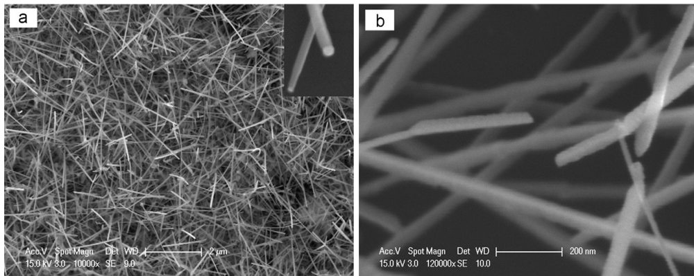
Fig. 2.16: FESEM images of GaN nanowires grown on Si (100) at (a) low magnification and (b) high magnification. The inset shows the existence of the Au catalysts at the end of the nanowires [53].
