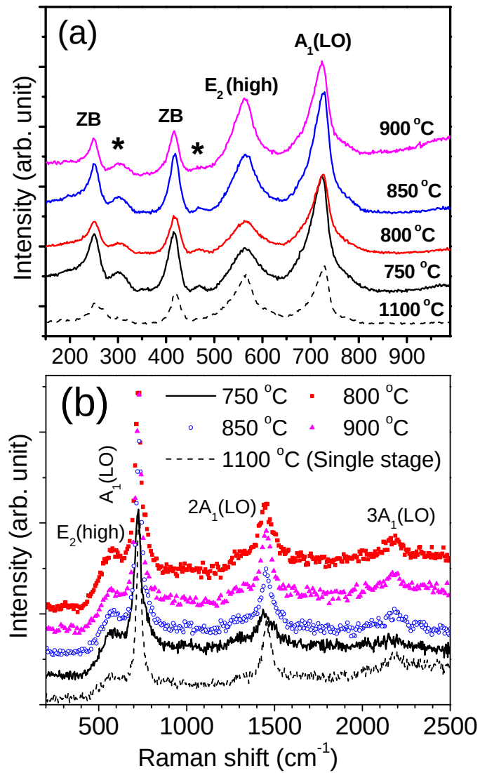
Fig. 4.9: a) Raman spectra of GaN nanostructures synthesized at different growth temperatures using 514.5 nm excitation. b) Resonance Raman spectra of GaN nanostructures synthesized at different growth temperatures using 325 nm excitation. Spectra are shifted vertically for clarity.
