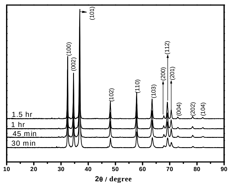
Fig. 6.1: PXRd patterns showing the effect of synthesis time on GaN synthesis using a \text{Ga}_2\text{O}_3/\text{C} ratio (1:3) in \text{NH}_3 at 1100 °C.
