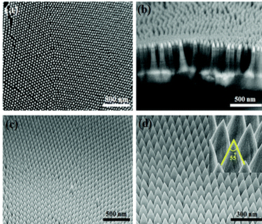
Fig. 2.17: FESEM images of GaN nanorods prepared at 1100^\circ\text{C} (a) top view, (b) side view, (c) low magnification tilted view and (d) high magnification tilted view (inset is the tip angle) [54].
