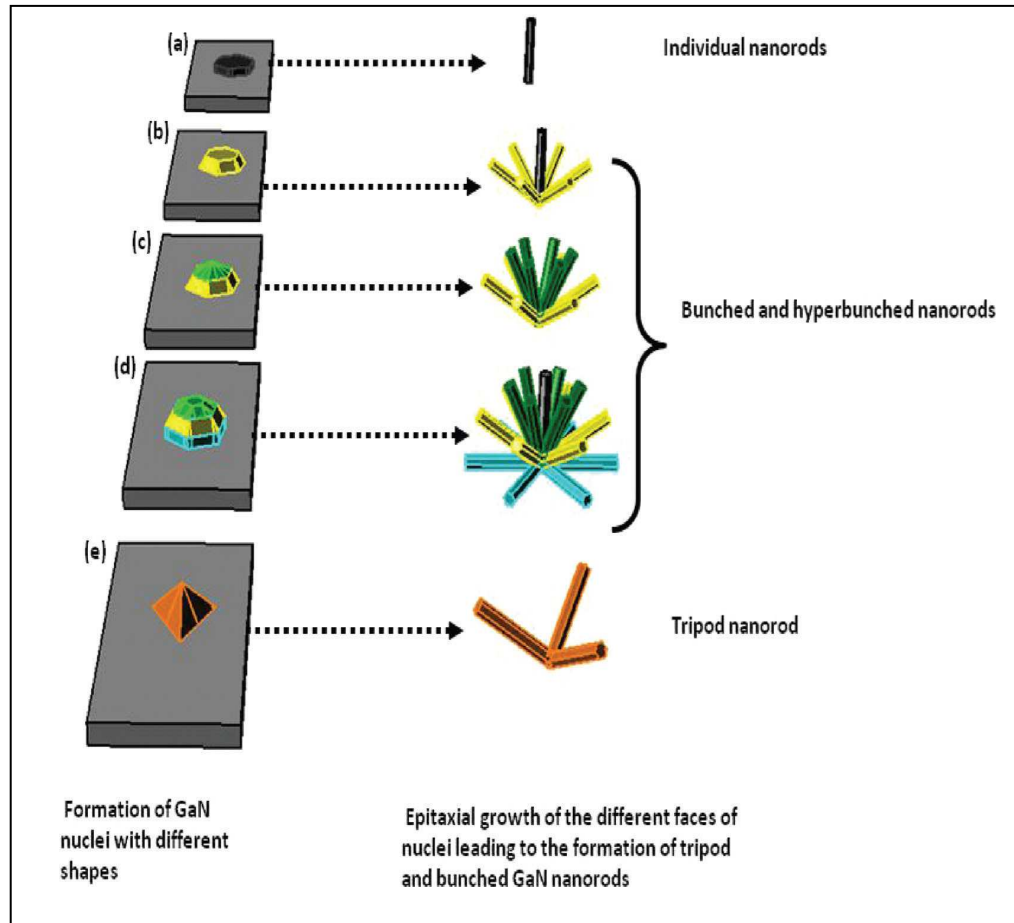
Fig. 2.4: Schematic illustration of the condensation growth mechanism for GaN nanorods. (Left) GaN nuclei responsible for the tripod, bunched and hyperbunched growth. (Right) Final GaN NR morphologies depending on the crystal symmetry of the nuclei [58].
