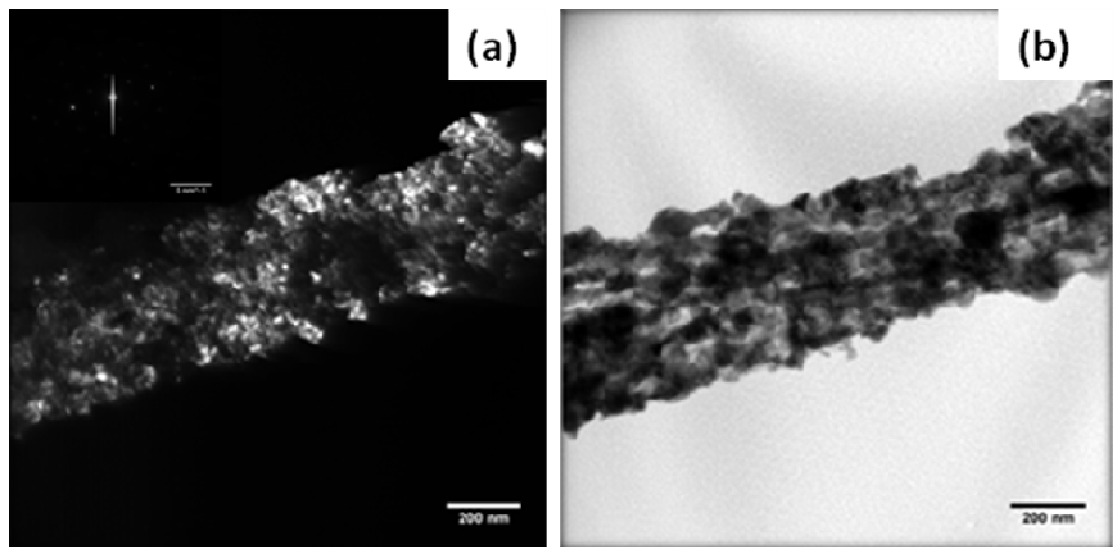
Fig. 5.1: TEM images. (a) Dark field image and SAED pattern (inset) (b) bright field image of GaN/C.
