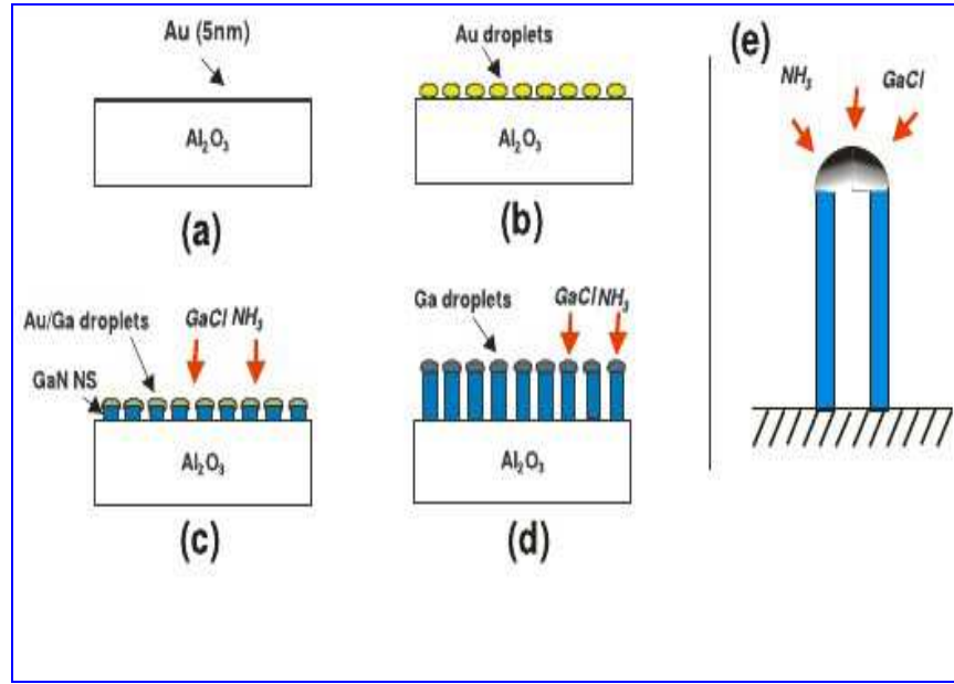
Fig. 2.9: A schematic illustration of the formation process of GaN nanotubes: (a) substrate before growth; (b) formation of Au droplets upon heating to growth temperature; (c) initial growth of GaN nanotubes using an Au/Ga alloy as catalyst; (d) continuous growth of nanotubes using Ga droplets as catalyst; (e) cross-sectional image of a nanotube illustrating the diffusion-limited growth process. The N concentration in the Ga droplet is schematically depicted by the gray scale (darker indicates higher N concentration) [42].
