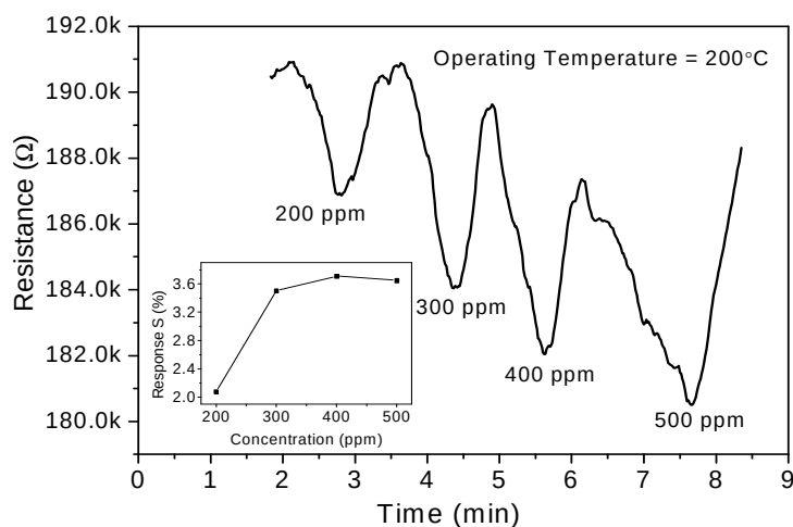
Fig. 6.10: Resistance and response curve (inset) of the GaN/C to different H 2 concentrations at 200°C.
