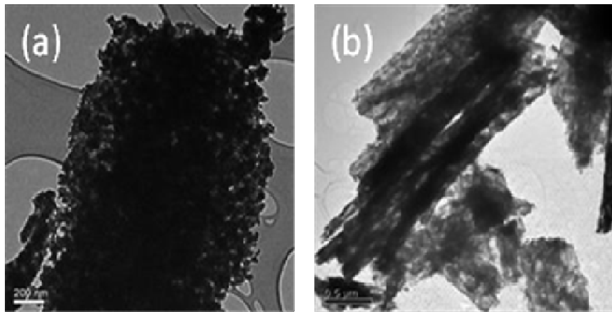
Fig. 4.2: TEM image shows the (a) agglomerated nanoparticles typically grown in the two stage furnace at 750 °C (b) morphology of the GaN materials at 1100 °C grown in single stage furnace.
