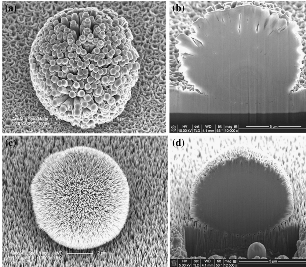
Fig. 2.22: FE-SEM images of (a) a GaN nanorod chestnut, (b) a cross-sectional image of a nanorod chestnut, (c) a nanoneedle chestnut, and (d) a cross-sectional image of a nanoneedle chestnut [57].
