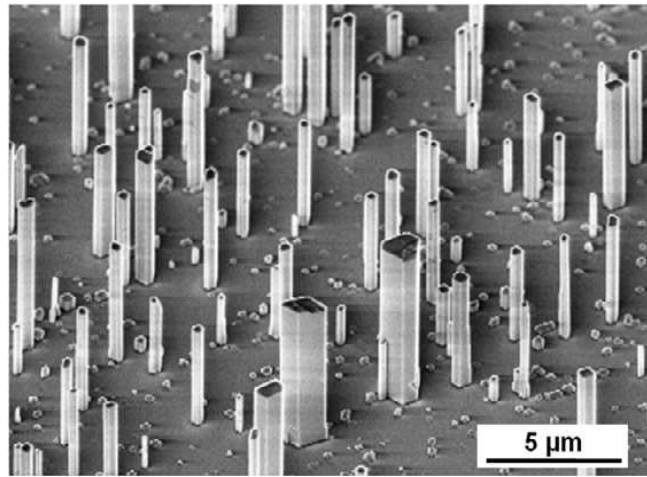
Fig. 2.6: 45°-Tilted scanning electron microscopy (SEM) view of a typical non-catalytic MOVPE growth of self-assembled GaN single-crystal wires on a c-plane sapphire substrate. The growth is homogeneous on the whole 2 inch wafer surface [41].
