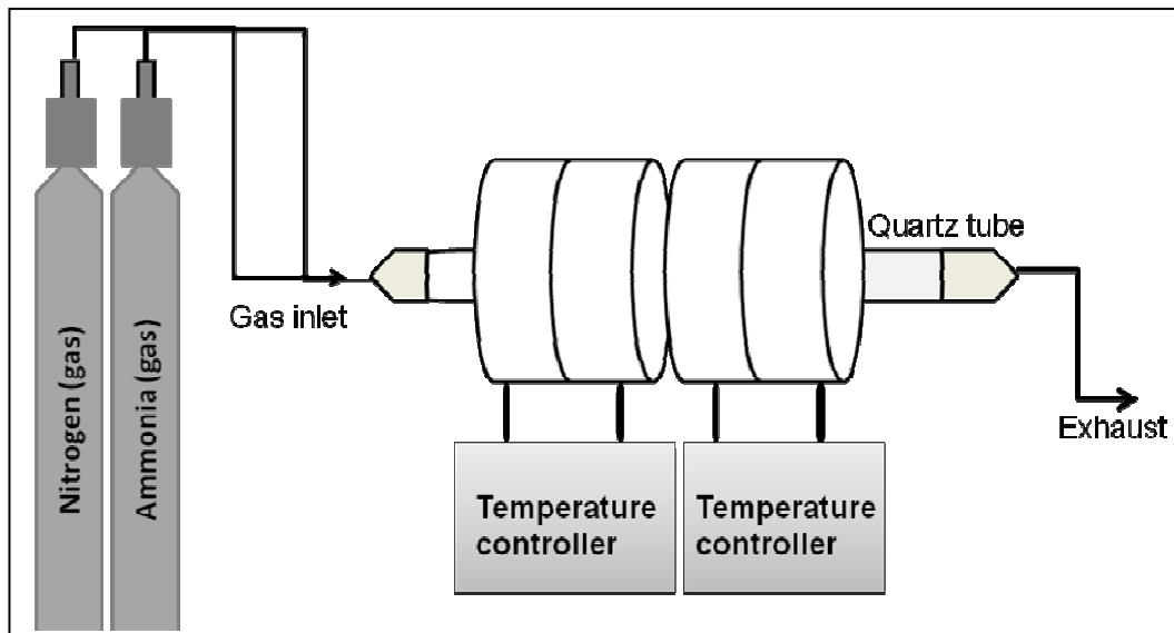
Fig. 3.2: Double stage furnace used in CVD synthesis of GaN materials.
