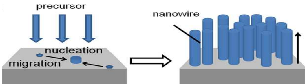
Fig. 2.7: Growth mechanism of GaN nanowires by catalyst free MOVPE [26].
