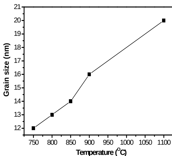
Fig. 4.4: Average grain sizes of the GaN nanostructures synthesized at different growth temperatures (750 – 900 °C) in a double stage furnace and 1100 °C in a single stage furnace. The line acts as a guide to the eye.
