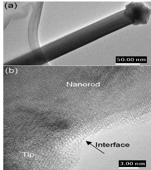
Fig. 2.2: (a) Low-magnification image of a GaN nanorod including its tip, (b) a high-magnification image of the interface of the tip and the nanorod [38].
