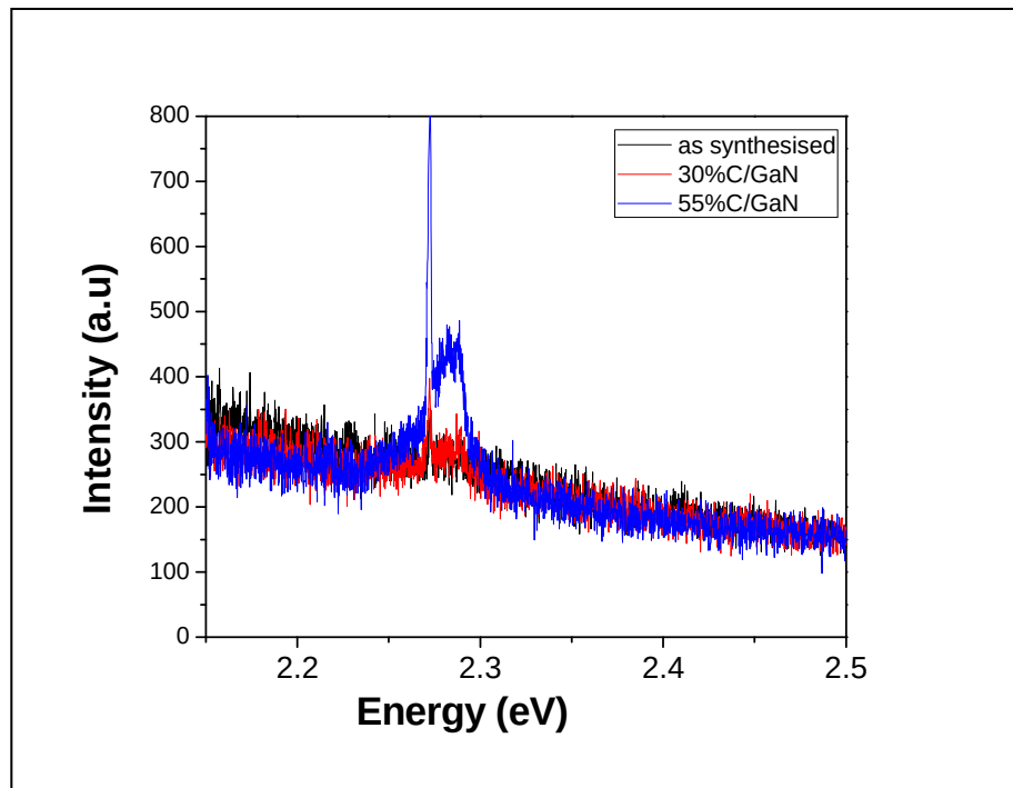
Fig. 5.9: Room temperature PL spectra (zoom) for GaN/C and functionalized GaN/C.
