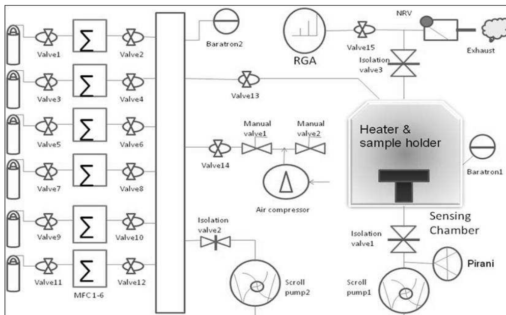
Fig. 3.6: Schematic diagram of gas measurement system.
