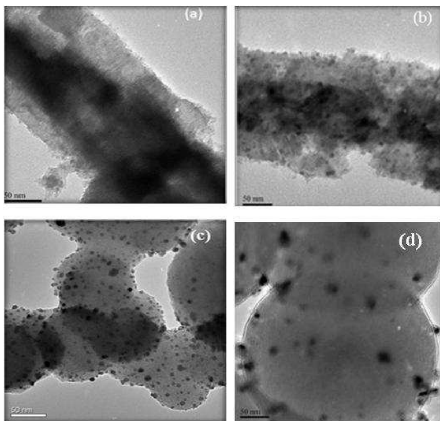
Fig.7.3: TEM images of (a) 1%Pd/GaN, (b) 3%Pd/GaN, (c) 1%Pd/NCSs and (d) 3%Pd/NCSs. The dark spots are Pd nanoparticles.
