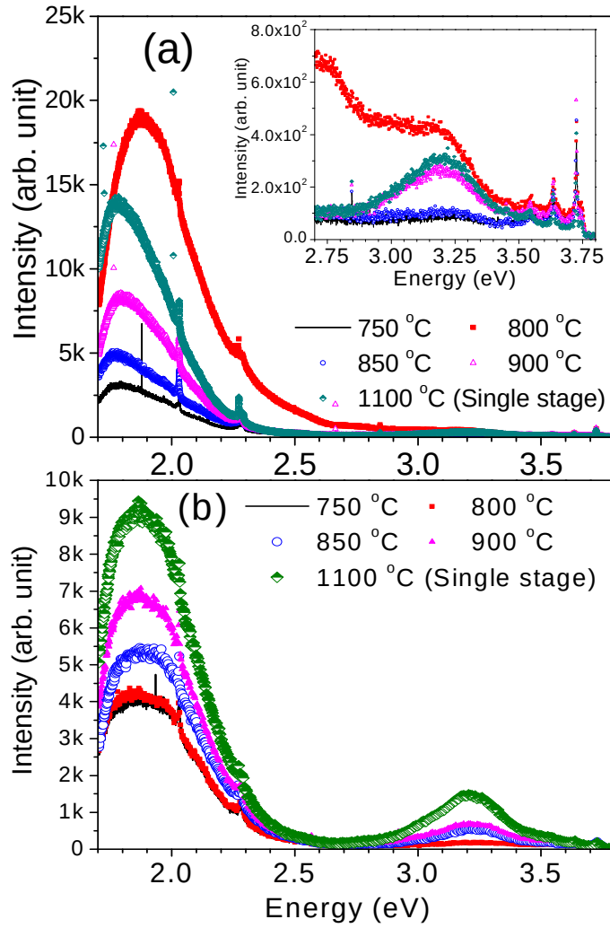
Fig. 4.10: Room temperature PL spectra a) for pristine GaN nanostructures synthesized at various growth temperatures showing broad and intense peak in the range of 1.7-2.1 eV. Inset shows the zoomed spectra for free-to-bound emission at around 3.25 eV, b) for post-annealed GaN nanostructures synthesized at various growth temperatures showing clear free-to-bound emission peak at around 3.25 eV.
