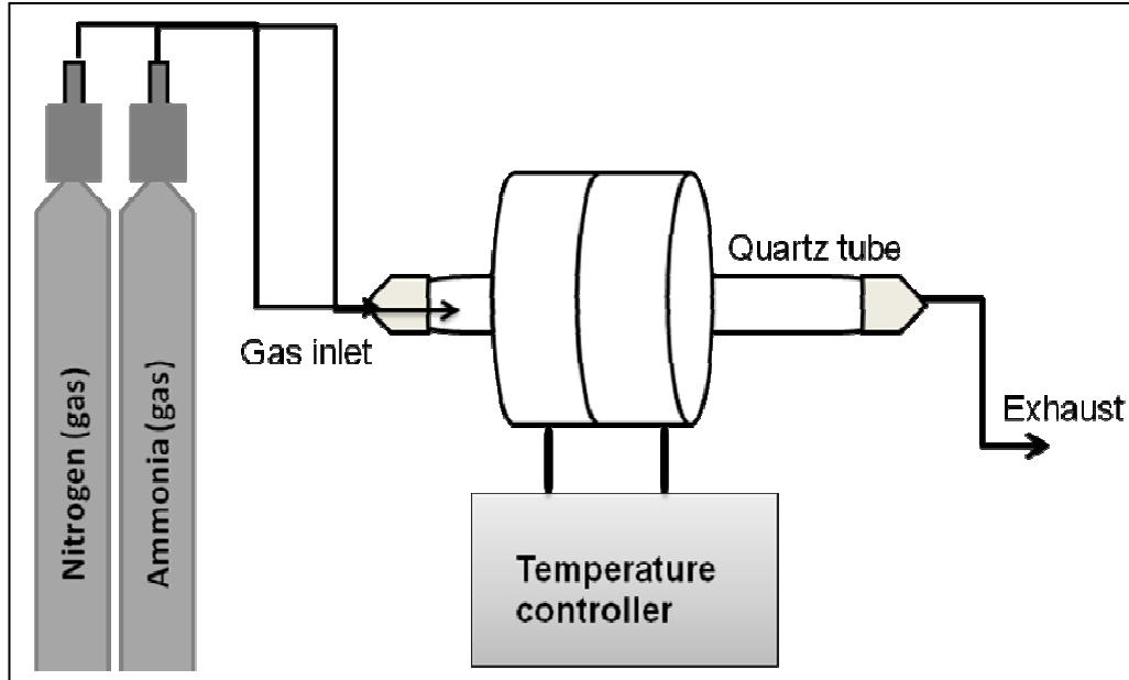
Fig. 3.1: Single stage furnace for CVD synthesis of GaN materials.
