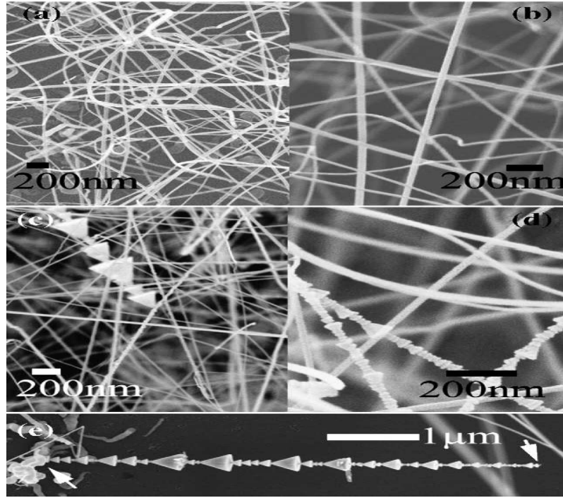
Fig. 2.5: GaN nanowire growth on different substrates. (a, c) Si(100), (b, d) Si(111). In the case of (a) and (b), the flow rates were 50 sccm for \text{NH}_3 and 100 for Ar, and in the case of (c) and (d), the flow rates are 125 sccm for \text{NH}_3 and 25 sccm for Ar; (e) higher magnification image of the cones [40].
