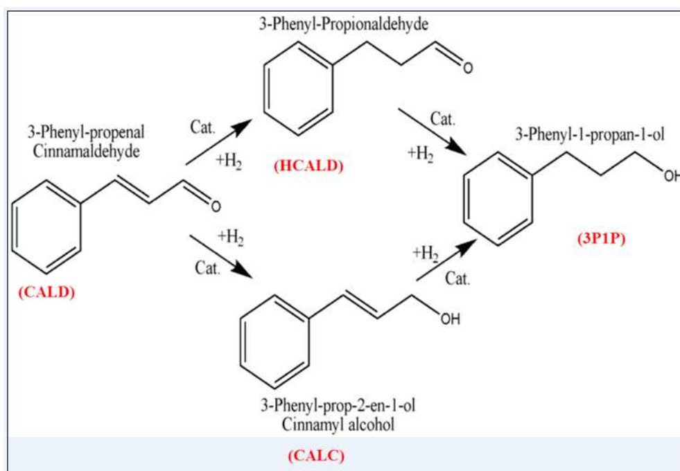
Fig. 7.1: Reaction scheme proposed for the selective hydrogenation of cinnamaldehyde [12].
