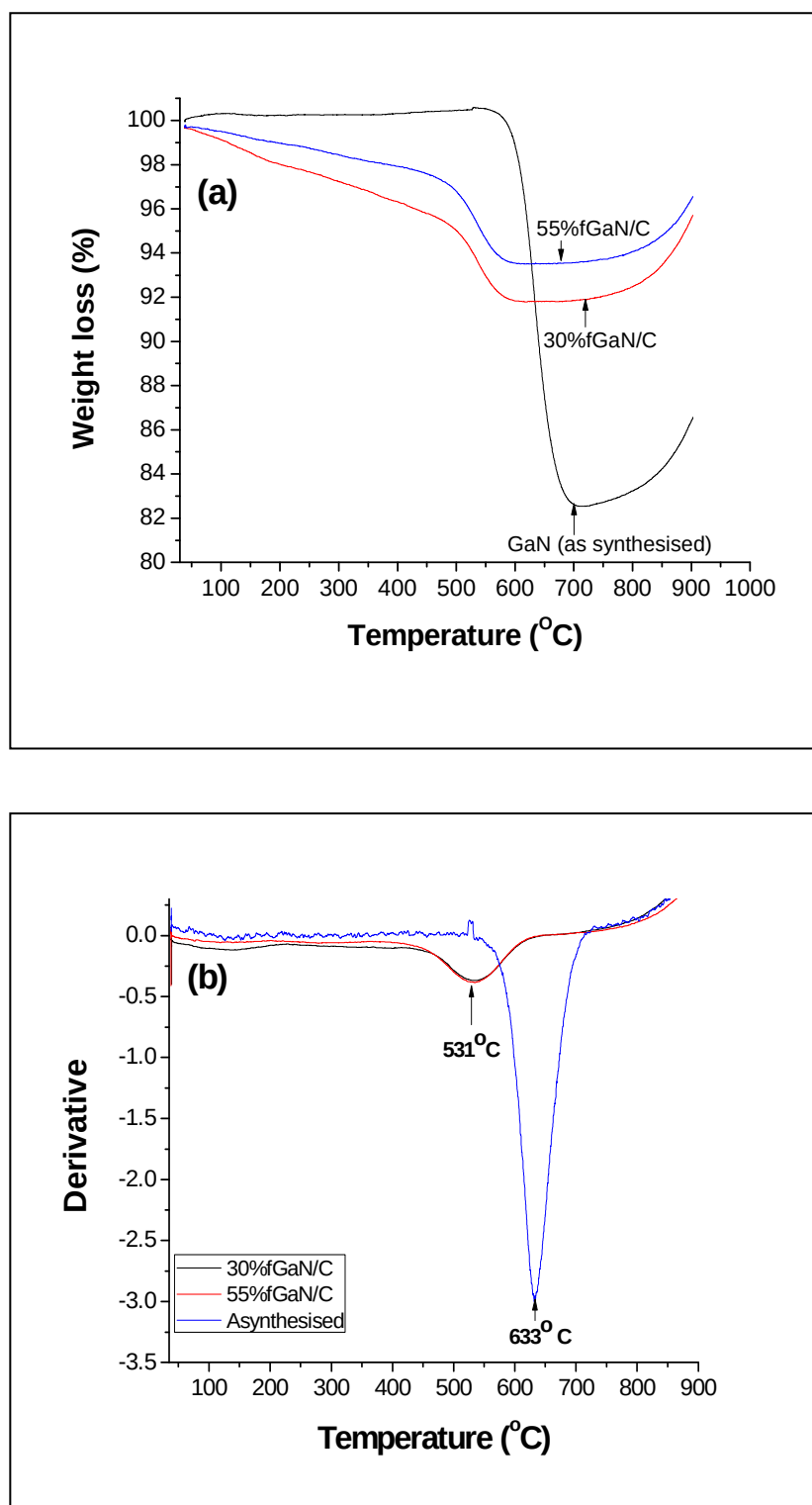
Fig. 5.6: TGA profile of (a) the functionalized samples and as synthesized GaN/C and (b) their derivative curves.
