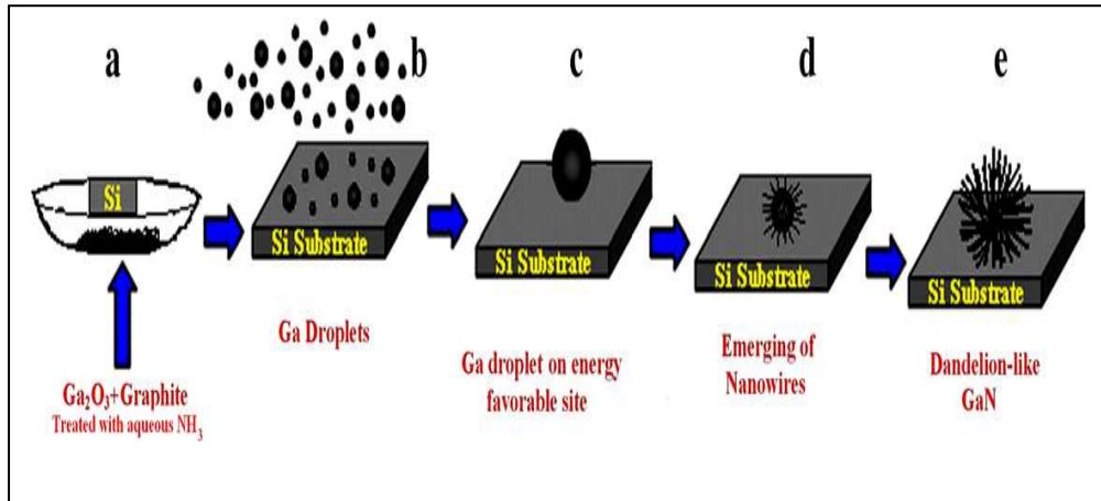
Fig. 2.15: The growth mechanism for the formation of dandelion-like GaN microstructures [52].
