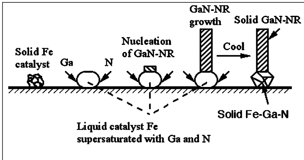
Fig. 2.3: Schematic illustration of VLS process for GaN nanorod (GaN-NR) growth by a pyrolysis route [38].
