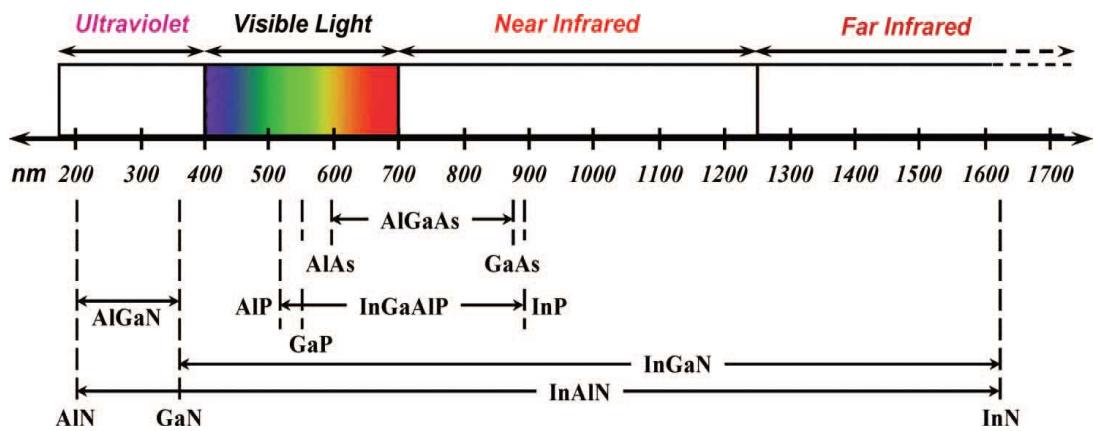
Fig. 2.24: Various ternary and quaternary materials used for LEDs with the wavelength ranges indicated [84].
