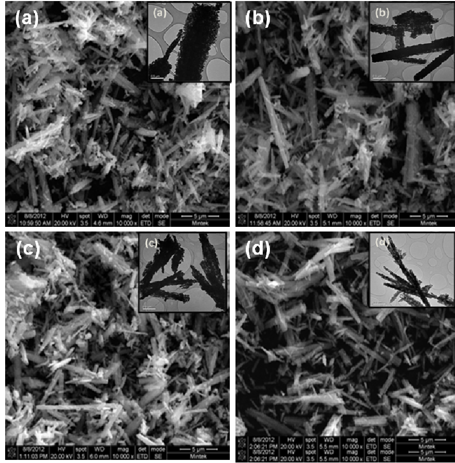
Fig. 4.1: SEM and TEM (inset) images of GaN nanostructures grown in the two stage furnace at (a) 750 °C, and (b) 800 °C, for 2 h; (c) 850 °C and (d) 900 °C for 1 h.
