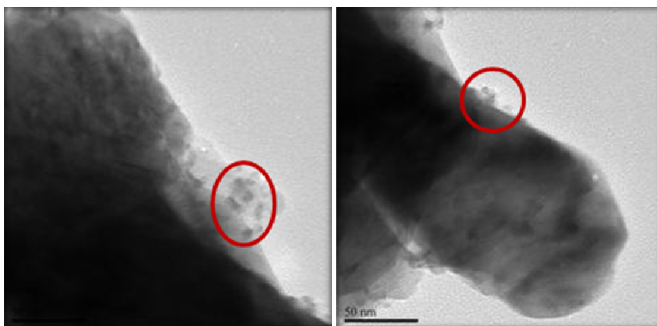
Fig. 6.8: TEM images of 3%Pd /GaN/C (1:2) synthesized at 1100 °C.
