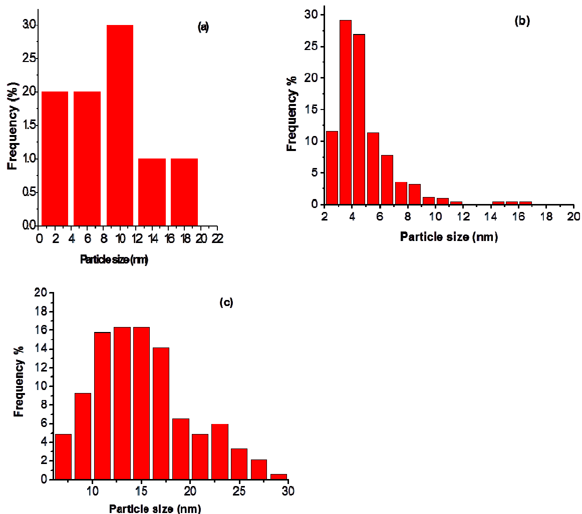
Fig. 7.4: Particle size distribution graphs of (a) 3 % Pd/GaN, (b) 1 % Pd/NCSs and (c) 3 % Pd/NCSs.
