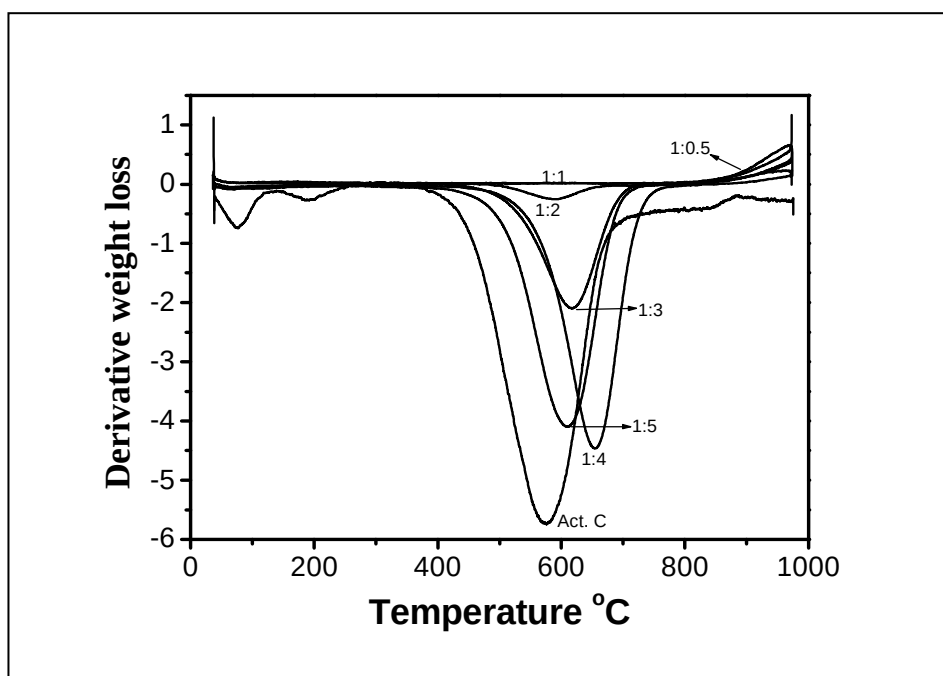
Fig. 6.5: Derivative plots of GaN-NSs synthesized with and without activated carbon at 1100 °C.
