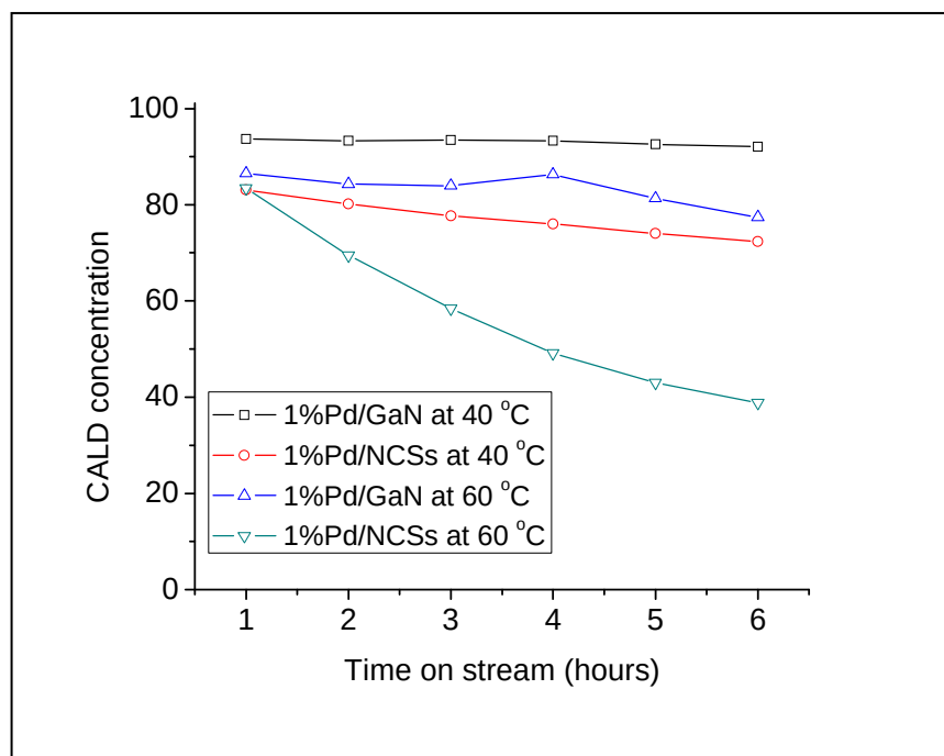
Fig. 7.5: Graphs showing CALD remaining as a function of time on stream at 40 and 60°C for 1% Pd/GaN and 1% Pd/NCSs catalysts.
