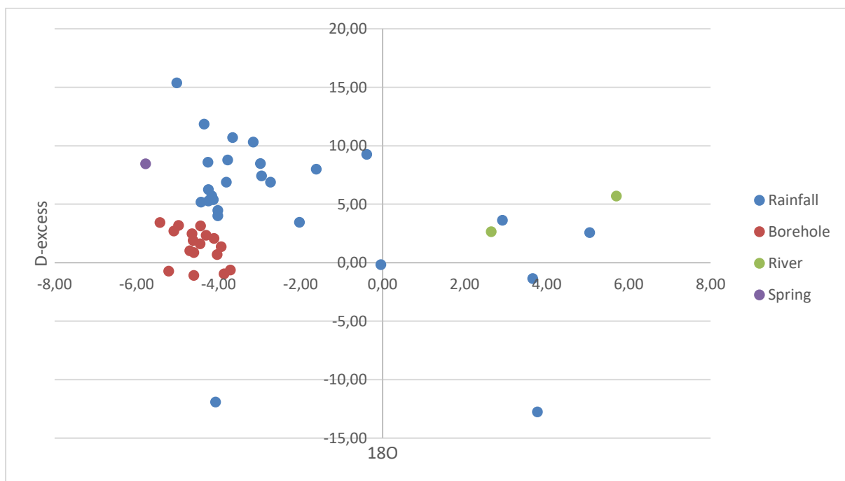
Figure 6.3: Hout River Catchment stable isotopes in rainfall, borehole, river and dam and springs. The LMWL is given by \delta D = 6.7\delta^{18}O + 7.2\text{‰} and GMWL by \delta D = 8\delta^{18}O + 10\text{‰} (Craig, 1961).
