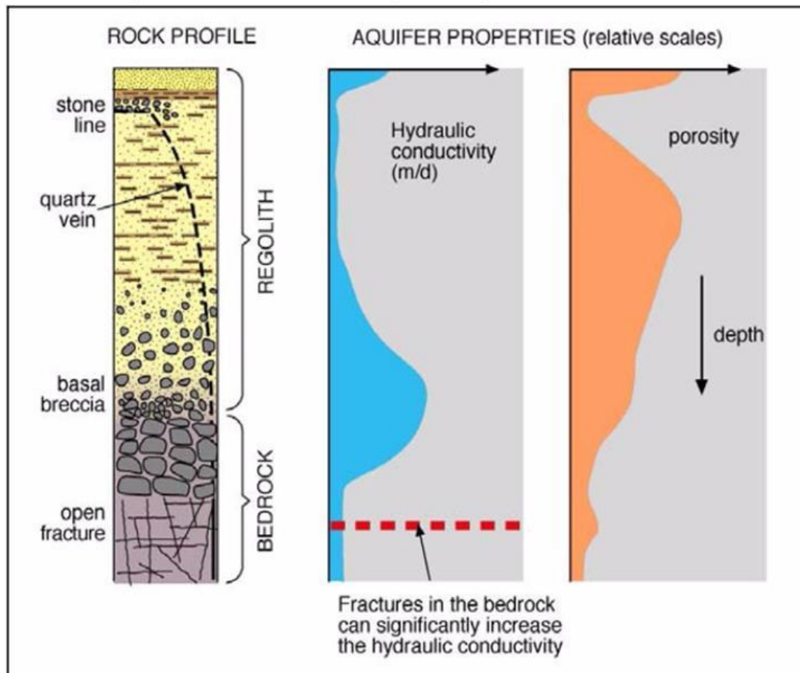
Figure 2.2: Bedrock aquifer layers and their hydraulic properties (Source: Chilton and Foster, 1995).
