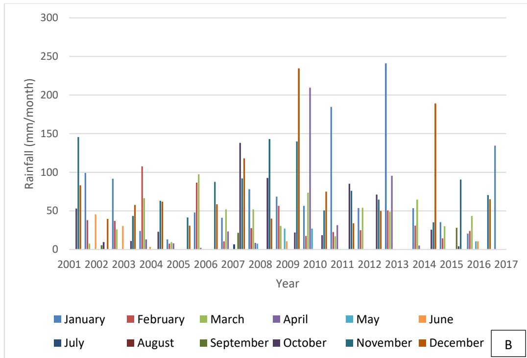
Figure 3.2: Long-term rainfall of the Mara (A) and Mogwadi (B) rainfall stations (Data Source: South African Weather Service (SAWS)).
