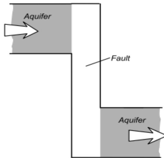
Figure 2.5: Vertical Fault (barrier fault) displacing an aquifer (Source: Bense et al., 2013).
