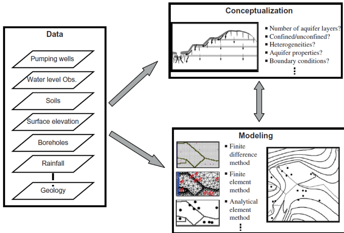
Figure 2.1: Three main components of groundwater studies (adapted from Maidment and Hopper, 2005 in Yang et al., 2010).
