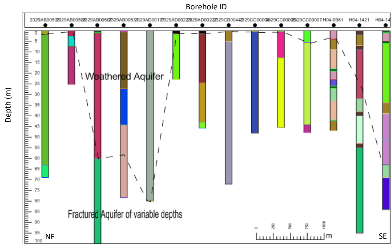
Figure 6.14: Hydrostratigraphic units of the HRC.
