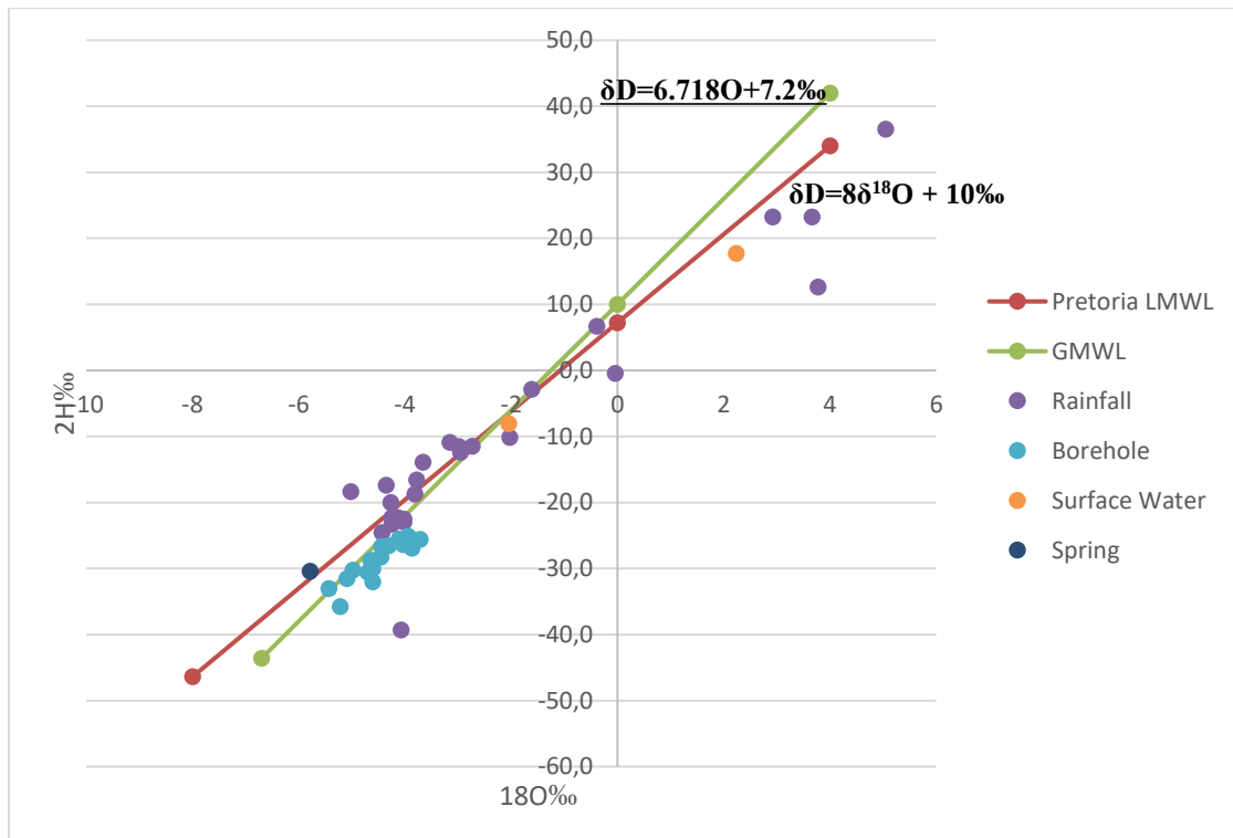
Figure 6.3: Hout River Catchment stable isotopes in rainfall, borehole, river and dam and springs. The LMWL is given by \delta D = 6.7\delta^{18}O + 7.2\text{‰} and GMWL by \delta D = 8\delta^{18}O + 10\text{‰} (Craig, 1961).
