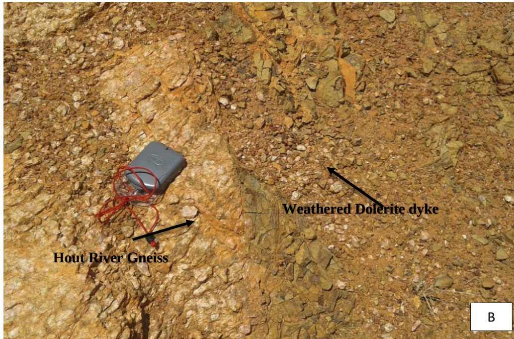
Figure 4.2: A) Folded basement Goudplaats Gneiss. B) Highly weathered Hout River Gneiss with an intrusive dolerite dyke.
