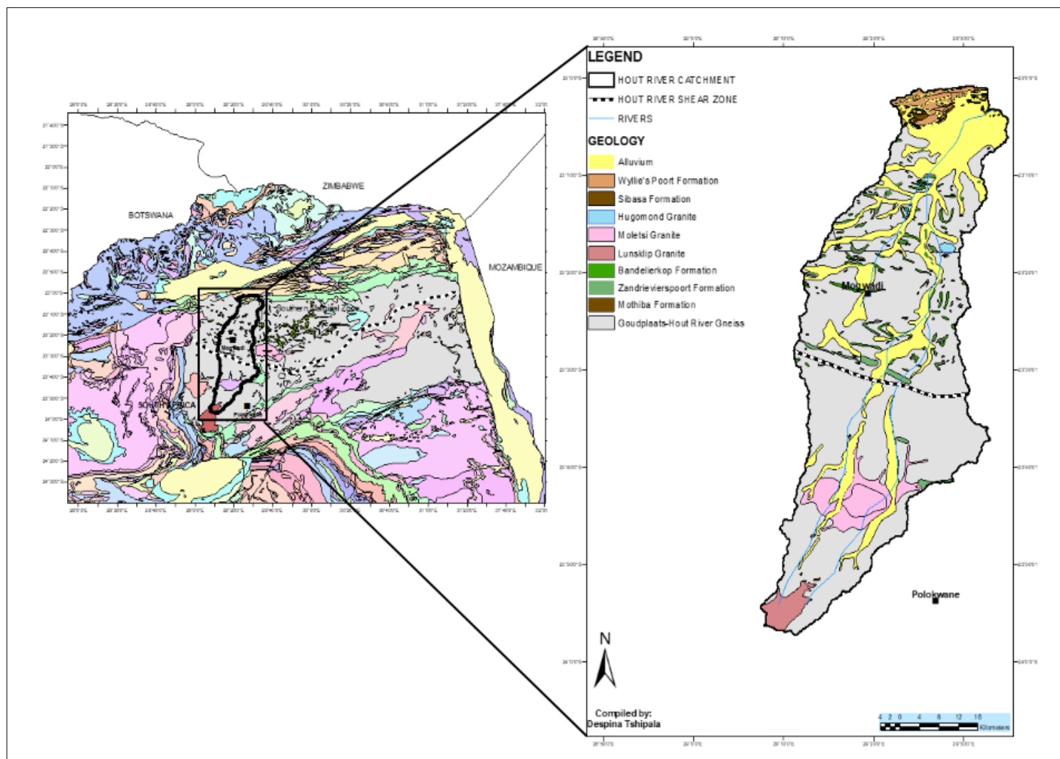
Figure 4.3: Geological map of the Hout River Catchment (Data Source: Council of Geosciences (SA)).
