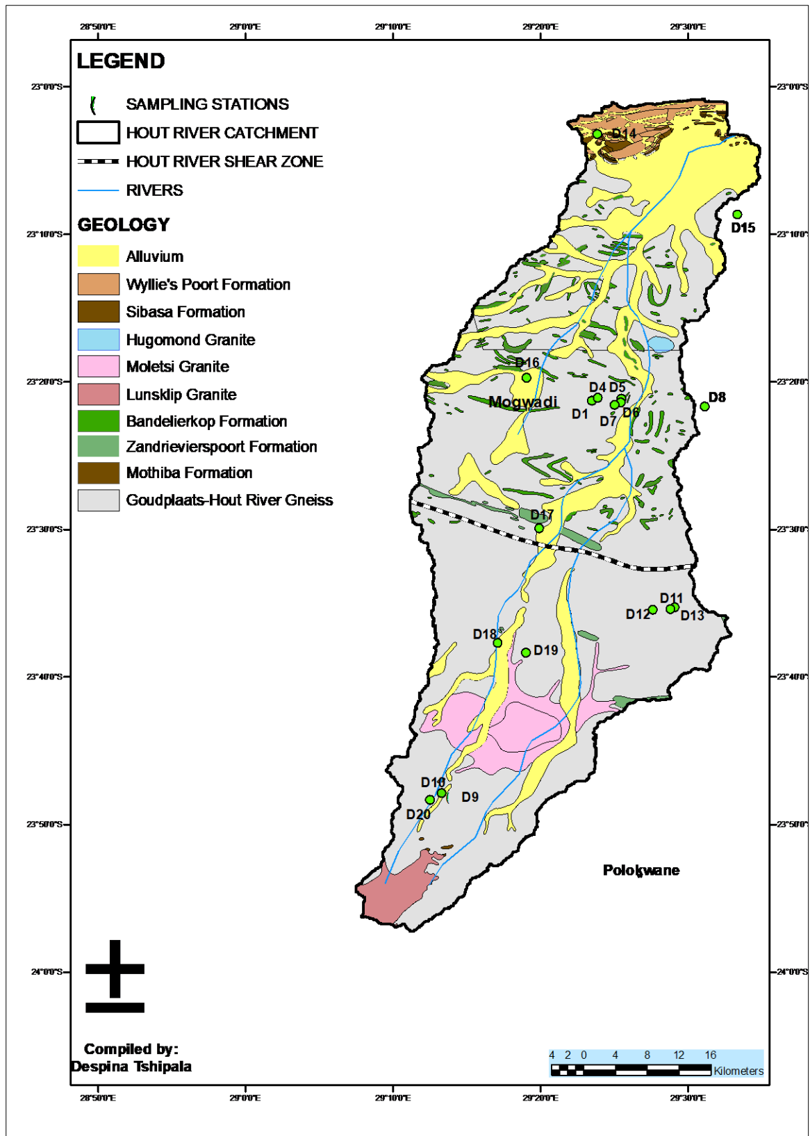
Figure 5.1: Sampling stations within the Hout River Catchment. (Source: CGS).
