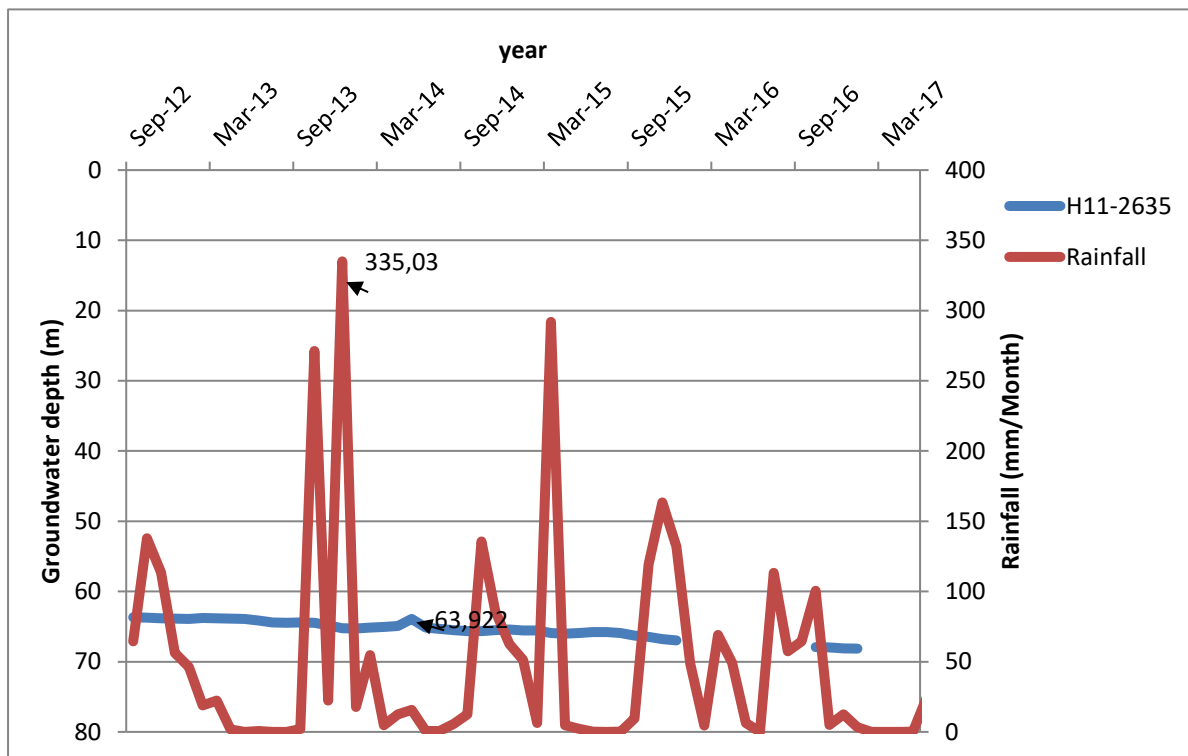
Figure 4.7: Groundwater level trends of the monitoring boreholes against long-term annual rainfalls within the Hout River Catchment.
