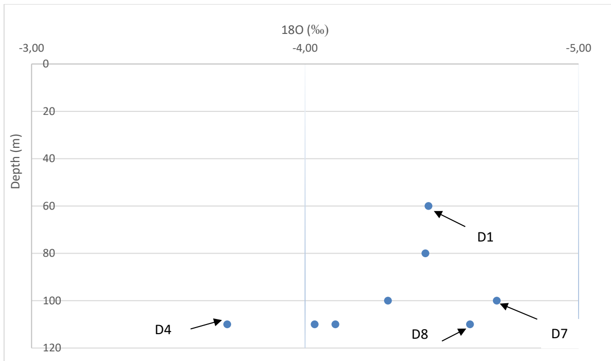
Figure 6.5: Depth against ^{18}\text{O} for Boreholes (D1 to D8) located within the Mogwadi and eastern-outside the catchment.
