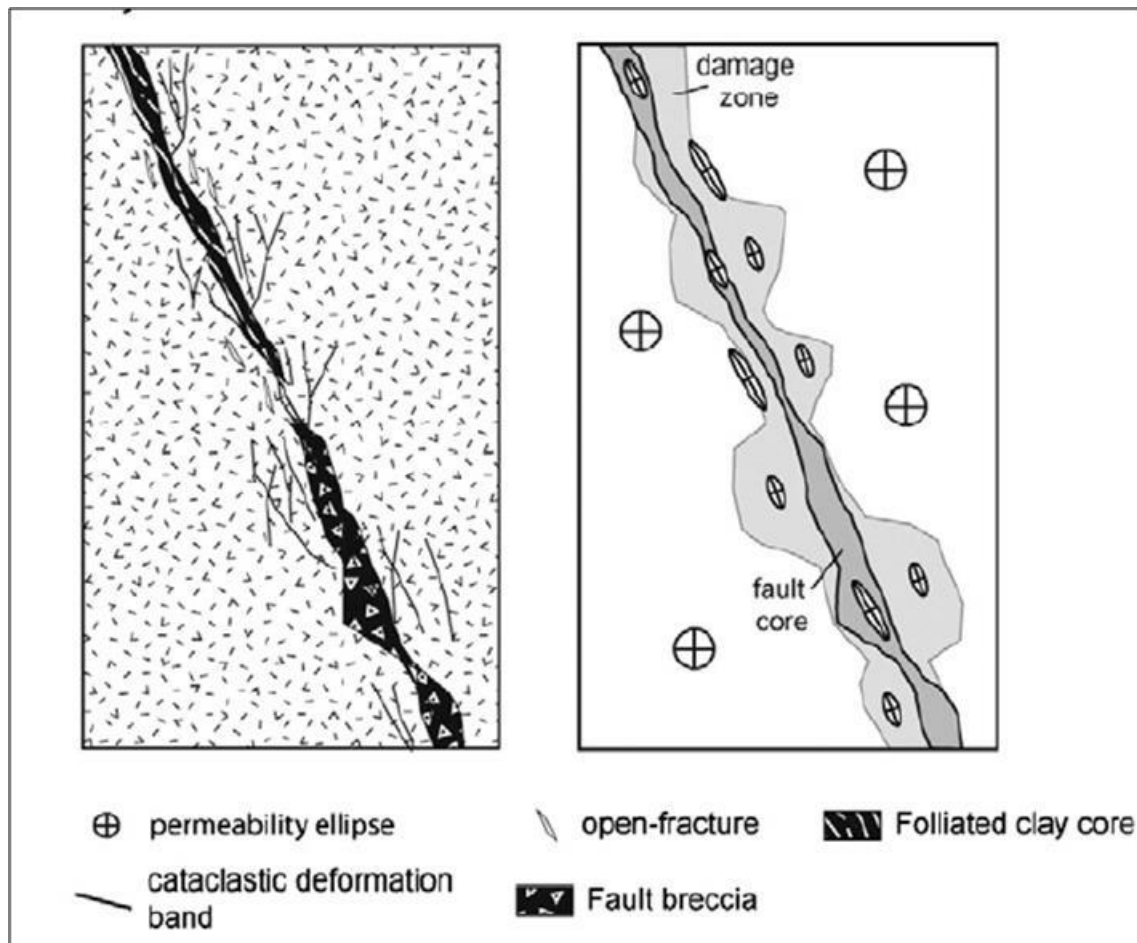
Figure 2.4: Fault anatomy (Source: Bense et al., 2013).
