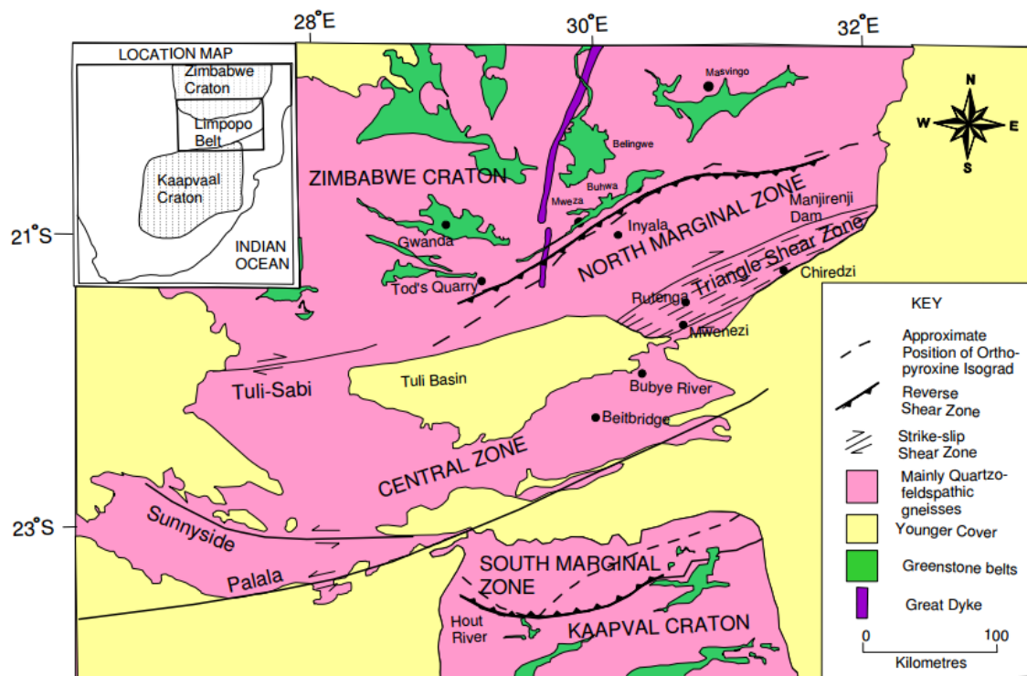
Figure 4.1: Regional geology of the study area (Source: Chinoda et al., 2009).
