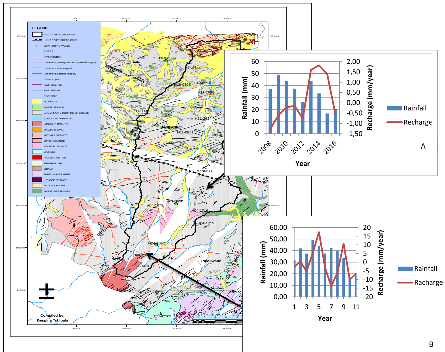
Figure 6.12: Groundwater recharge rates from boreholes (a) A7N0641 and (b) A7N0635 with rainfall within the Hout River Catchment.
