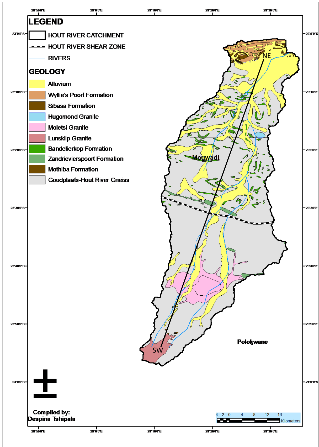
Figure 6.13: Surface delineation of the area within the catchment used for cross-section construction.
