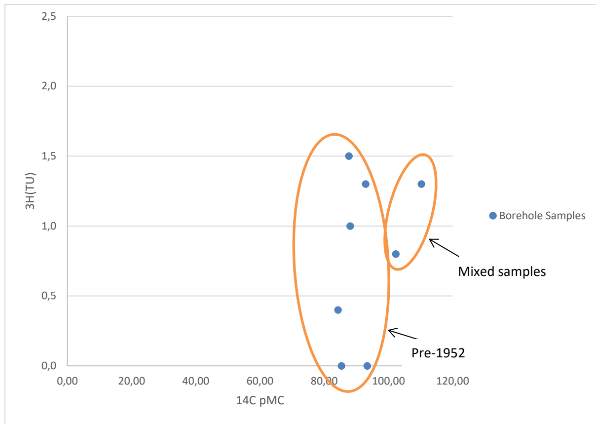
Figure 6.6: A plot of ^3\text{H} and ^{14}\text{C} for the groundwater samples for pre-1952 and post-1952 recharge.
