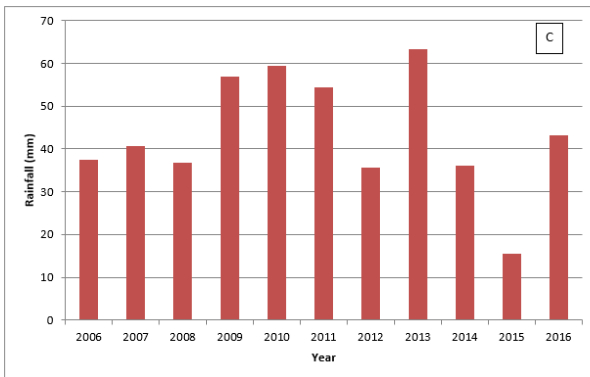
Figure 6.10: A) Rainfall pattern from 2005 to 2016 from the Mogwadi Rainfall Station. B) Rainfall pattern from 1940 to 2013 from the Lekgraal Rainfall Station. C) Rainfall pattern from the Mara PP Rainfall Station.
