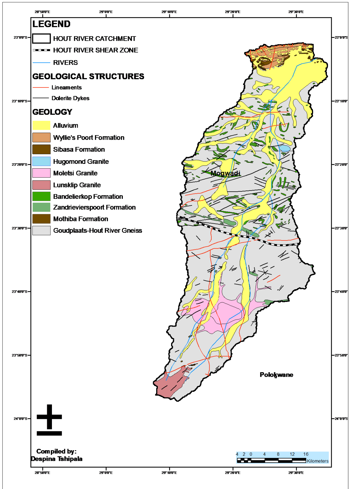
Figure 4.6: Structural map of the Hout River Catchment (Data source: Council of Geoscience (SA)).
