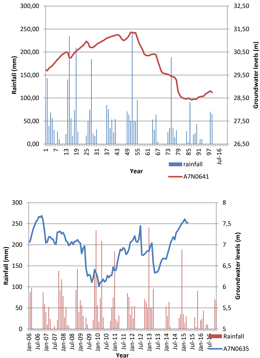
Figure 6.11: A) Hydrograph of averaged groundwater levels from the borehole (A7N0641) from 2008 to 2016 and rainfall record from the Mogwadi rainfall station. B) Hydrograph of
