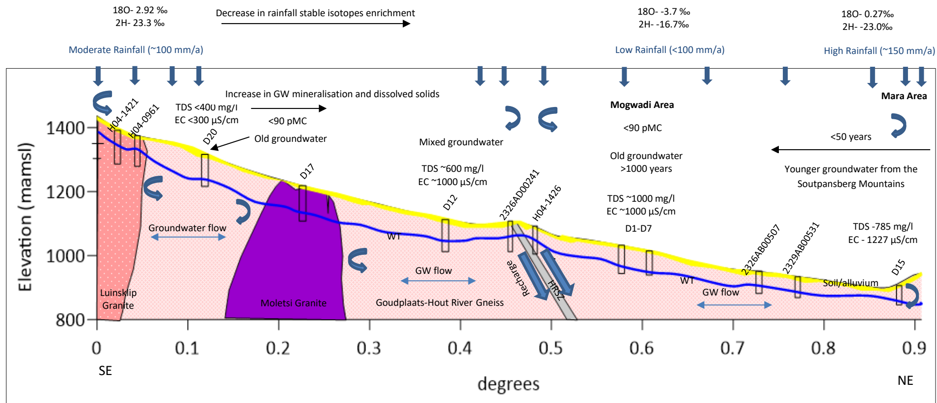
Figure 6.15: Conceptual model of the Hout River Catchment (groundwater age was determined from the tritium and C-14 results).
