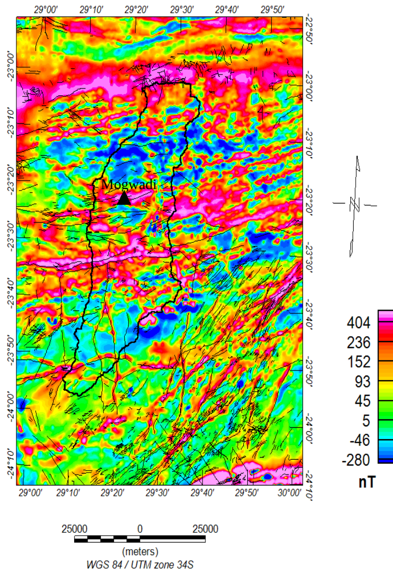
Figure 6.1: Aeromagnetic map with superimposed geological structures of the Hout River Catchment.
