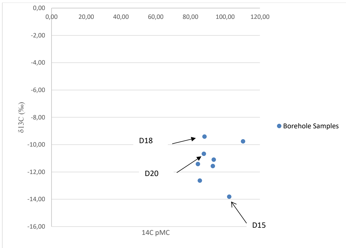
Figure 6.7: A plot of ^{13}\text{C} and ^{14}\text{C} from the groundwater samples within the HRC.
