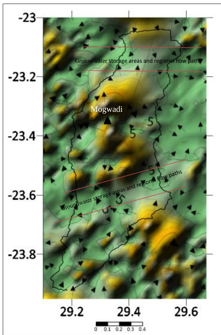
Figure 6.2: Groundwater flow patterns.
