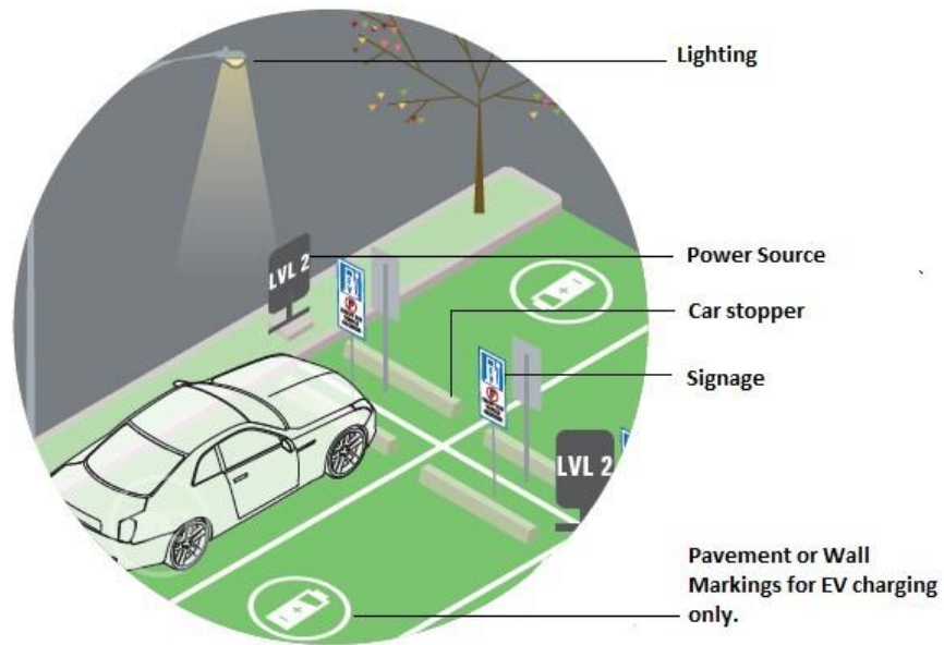
Figure 2. 2: Commercial Parking lot EV charging facility (image adapted from Transportation and Climate initiative, 2012)
