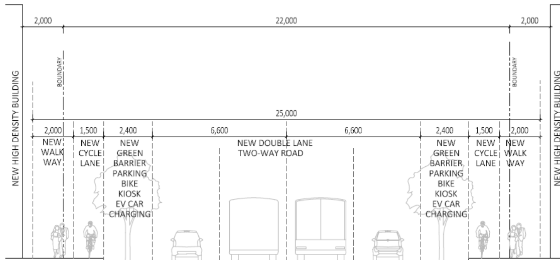
ZCW-ITN STREETSCAPE INTERVENTION TYPE 5 - CLASS 3 ROAD
