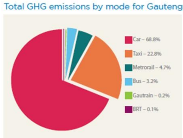
Figure 1. 2: GHG emissions in Gauteng (Source: EVIA, 2016)
