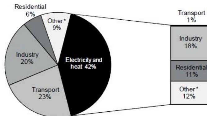
Figure 1. 1: World CO 2 emissions by sector in 2012 (Source: IEA, 2014)
