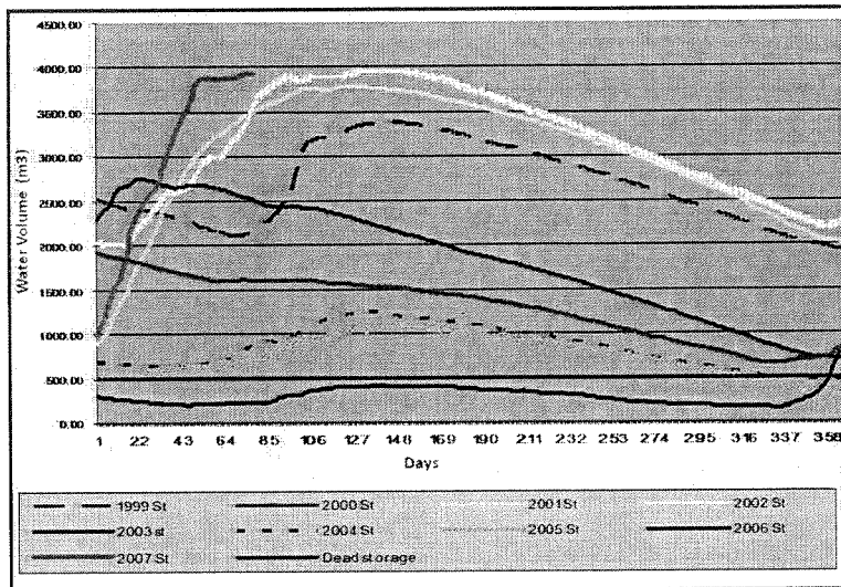
Figure 7.1: Water levels in Mtera Dam (Source; RBWO, 2006)
