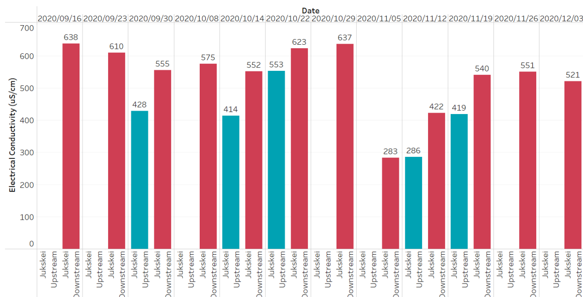
Figure 55: Results from electrical conductivity ( \mu\text{S}/\text{cm} ) tests conducted on samples from the Jukskei River upstream and downstream of Alexandra
