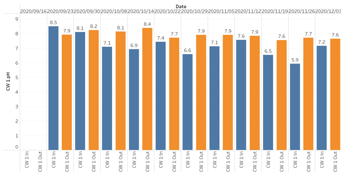
Figure 33: Results from pH tests conducted on influent and effluent streams of Constructed Wetland 1
