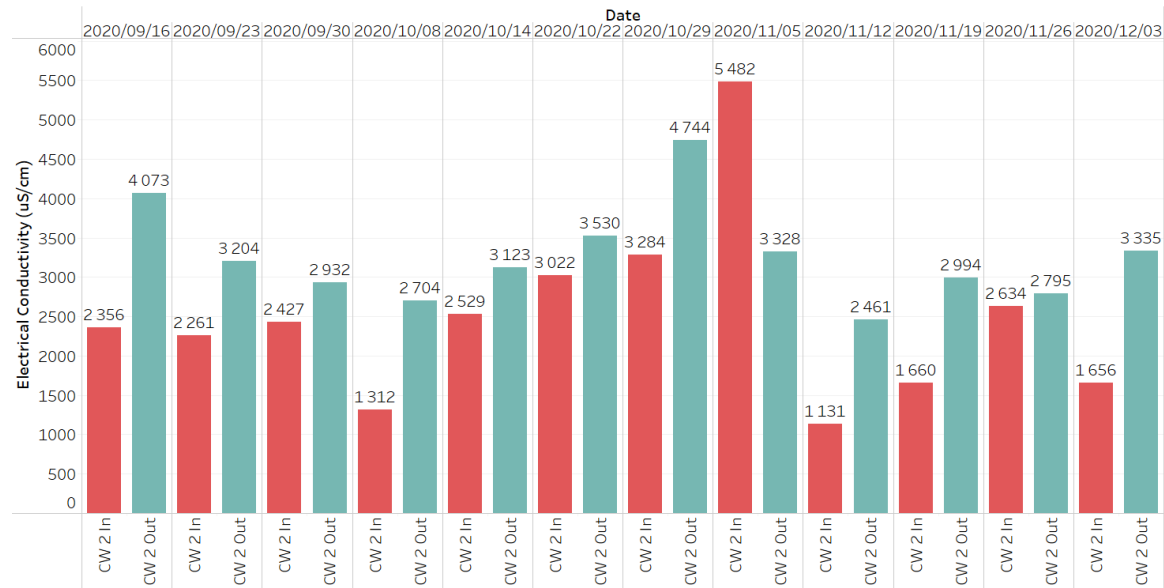
Figure 43: Results from electrical conductivity (µS/cm) tests conducted on influent and effluent streams of Constructed Wetland 2
