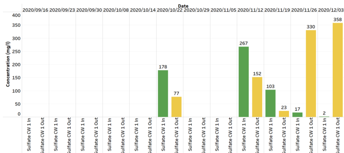
Figure 39: Results from sulfate concentration (mg/l) tests conducted on influent and effluent streams of Constructed Wetland 1
