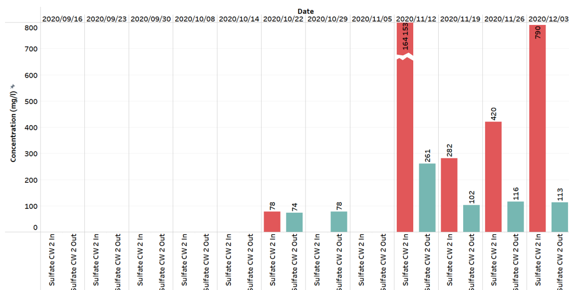
Figure 51: Results from sulfate concentration (mg/l) tests conducted on influent and effluent streams of Constructed Wetland 2
