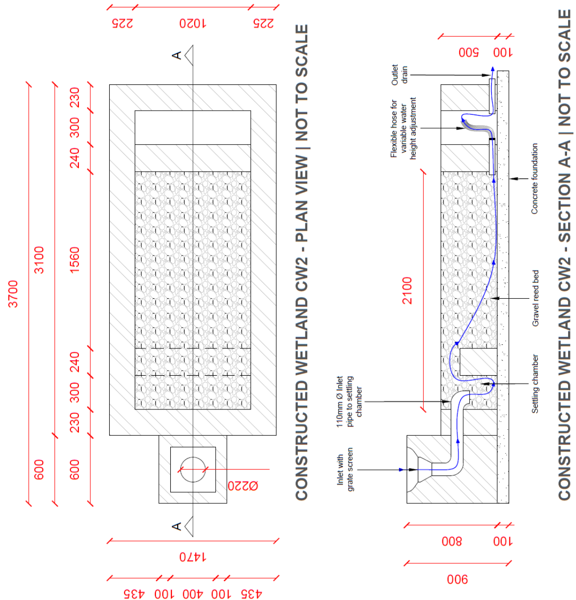
Figure 16: Technical Drawing for Constructed Wetland 2
