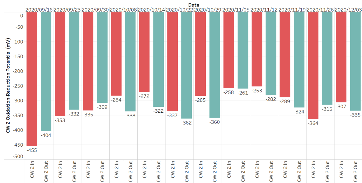
Figure 44: Results from oxidation-reduction potential (mV) tests conducted on influent and effluent streams of Constructed Wetland 2
