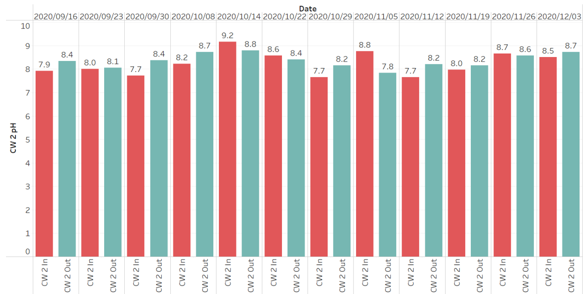
Figure 45: Results from pH tests conducted on influent and effluent streams of Constructed Wetland 2
