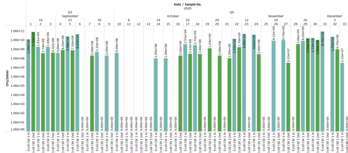
Figure 30: Results from Escherichia coli (CFU/100ml) tests conducted on influent and effluent streams of Constructed Wetland 1
