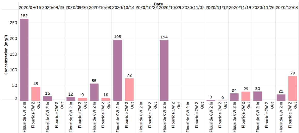
Figure 46: Results from fluoride concentration (mg/l) tests conducted on influent and effluent streams of Constructed Wetland 2
