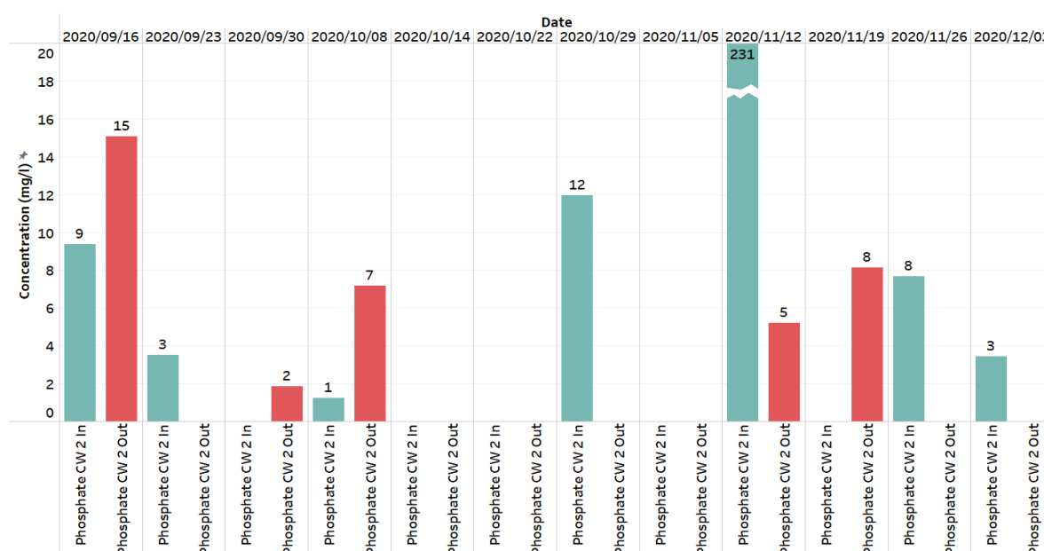
Figure 50: Results from phosphate concentration (mg/l) tests conducted on influent and effluent streams of Constructed Wetland 2
