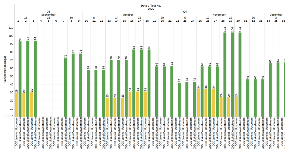
Figure 52: Results from chemical oxygen demand (COD) concentration (mg/l) tests conducted on samples from the Jukskei River upstream and downstream of Alexandra
