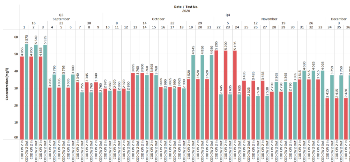
Figure 40: Results from chemical oxygen demand (COD) concentration (mg/l) tests conducted on influent and effluent streams of Constructed Wetland 2
