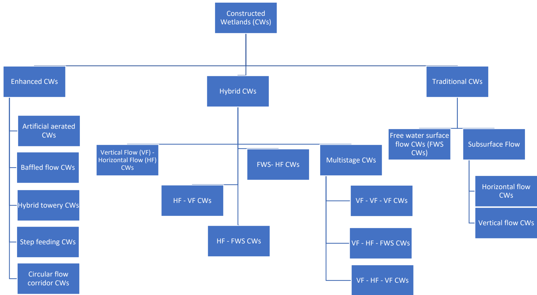
Figure 1: A classification of CWs used in wastewater treatment. Adapted from: Wu et al. (2015)
