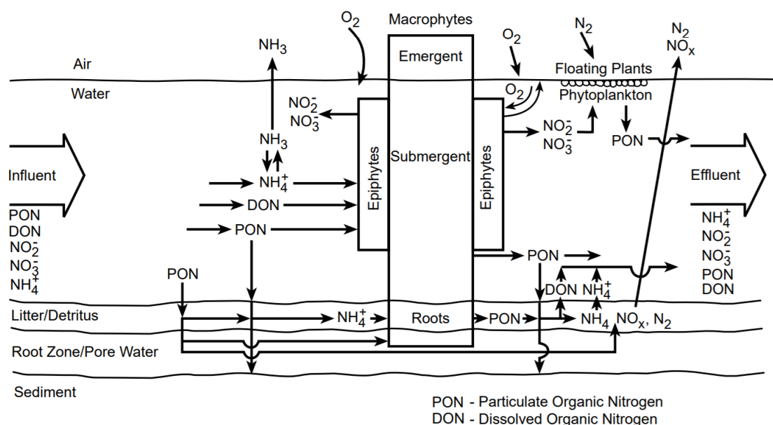
Figure 2 Nitrogen transformations in a free water surface constructed wetland (from: U.S. EPA, 2000)
