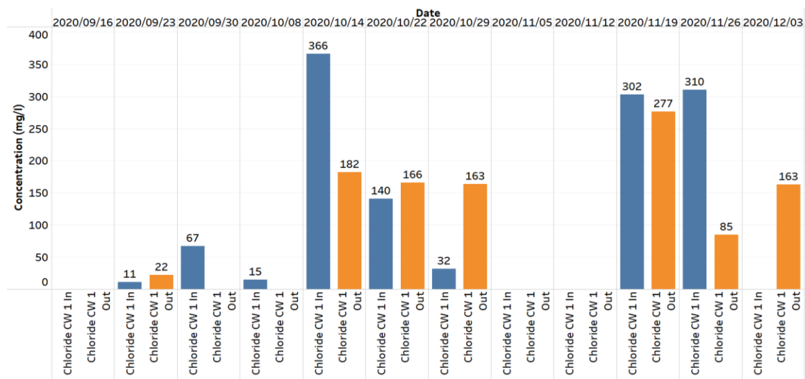
Figure 35: Results from chloride concentration (mg/l) tests conducted on influent and effluent streams of Constructed Wetland 1
