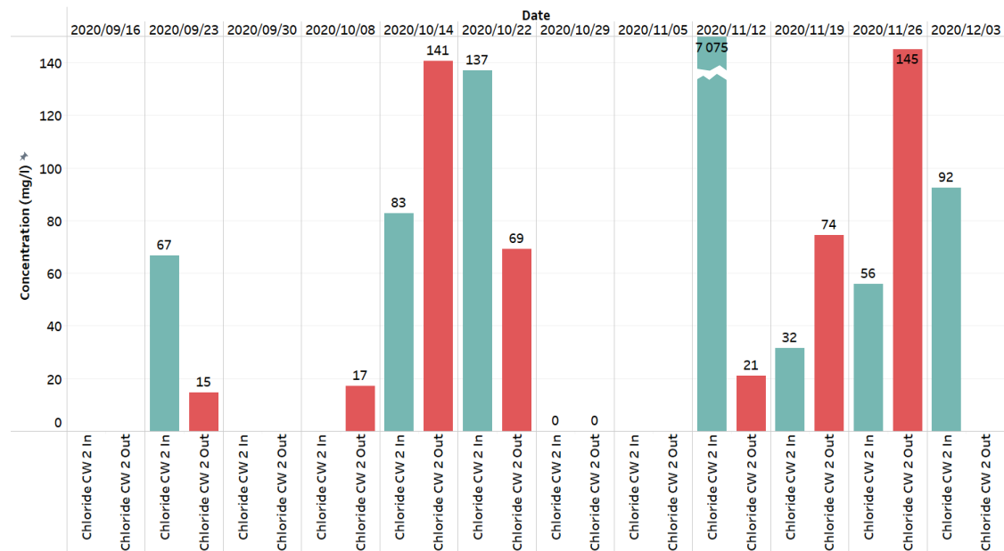
Figure 47: Results from chloride concentration (mg/l) tests conducted on influent and effluent streams of Constructed Wetland 2
