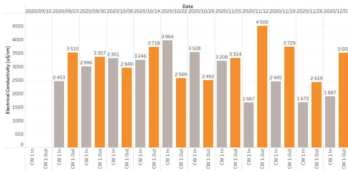
Figure 31: Results from electrical conductivity (µS/cm) tests conducted on influent and effluent streams of Constructed Wetland 1
