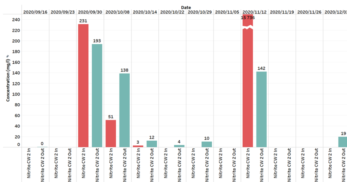
Figure 49: Results from nitrite concentration (mg/l) tests conducted on influent and effluent streams of Constructed Wetland 2
