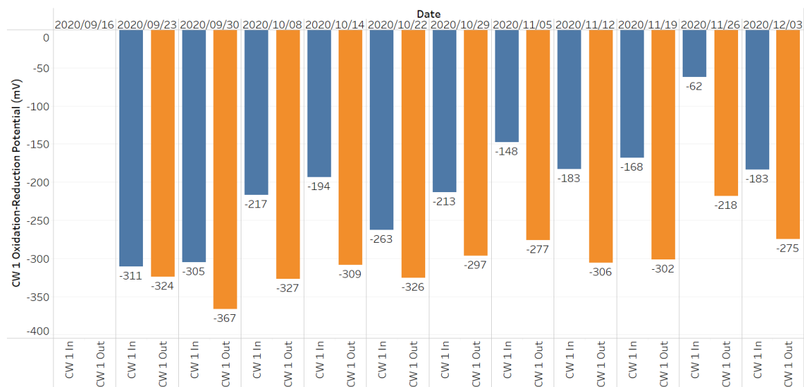
Figure 32: Results from oxidation-reduction potential (mV) tests conducted on influent and effluent streams of Constructed Wetland 1
