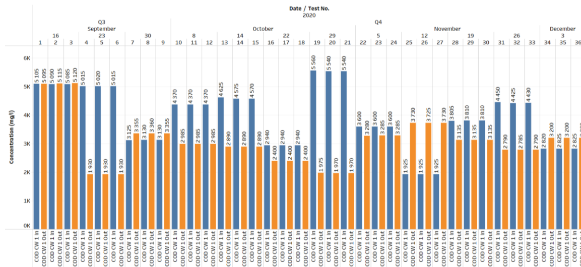
Figure 28: Results from chemical oxygen demand (COD) concentration (mg/l) tests conducted on influent and effluent streams of Constructed Wetland 1
