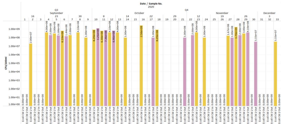
Figure 42: Results from Escherichia coli (CFU/100ml) tests conducted on influent and effluent streams of Constructed Wetland 2
