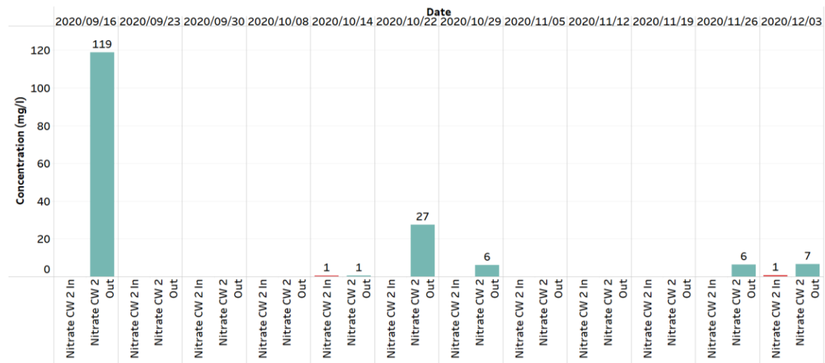
Figure 48: Results from nitrate concentration (mg/l) tests conducted on influent and effluent streams of Constructed Wetland 2
