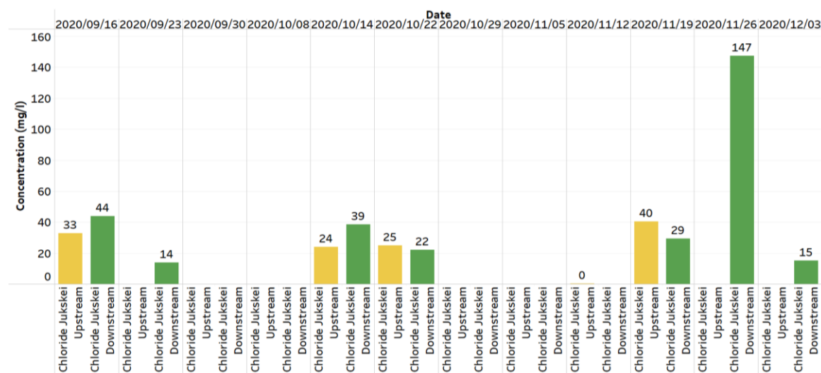
Figure 59: Results from chloride concentration (mg/l) tests conducted on samples from the Jukskei River upstream and downstream of Alexandra
