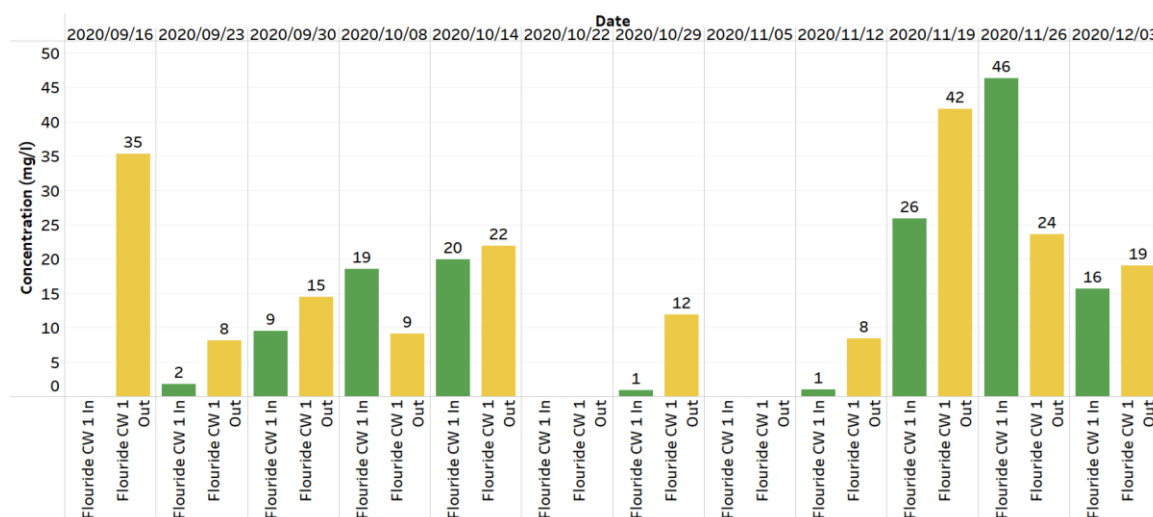
Figure 34: Results from fluoride concentration (mg/l) tests conducted on influent and effluent streams of Constructed Wetland 1
