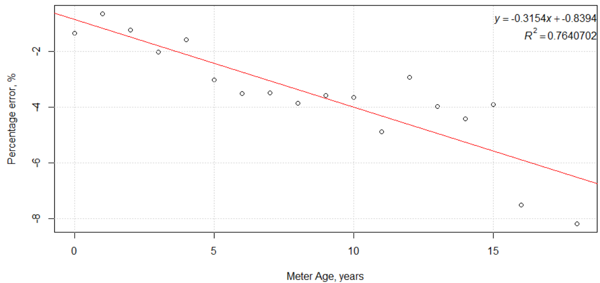
Figure 4-5: Accuracy degradation at q_{min} with meter age
