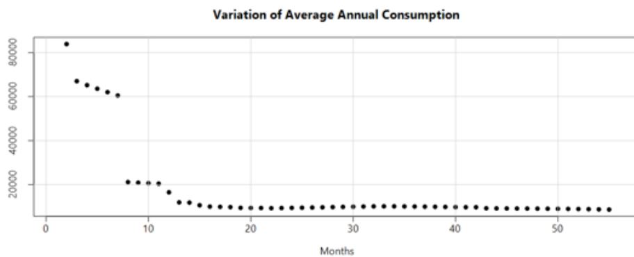
Figure 7-23: Data Preparation
