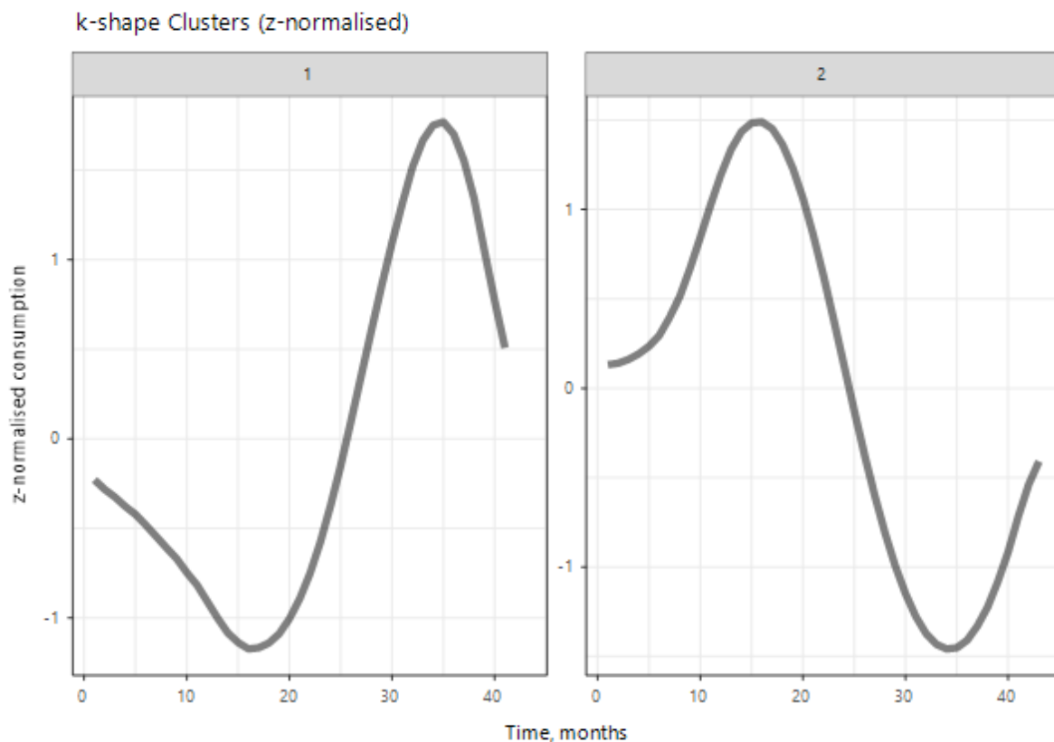
Figure 6-9: k-Shape Clusters
