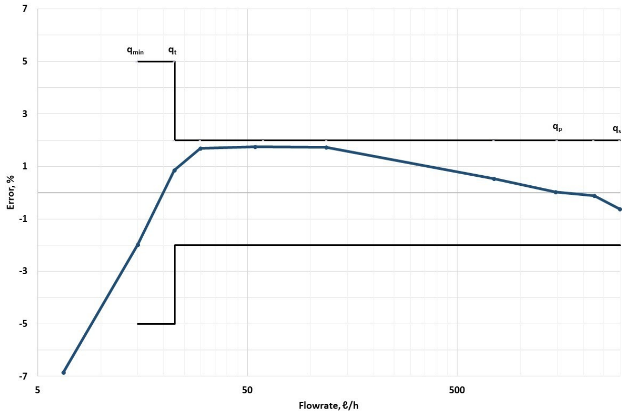
Figure 2-5: Meter Error Curve
