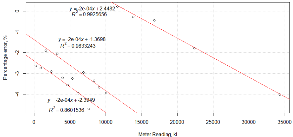
Figure 4-4: Accuracy degradation at q_{min} with meter reading
