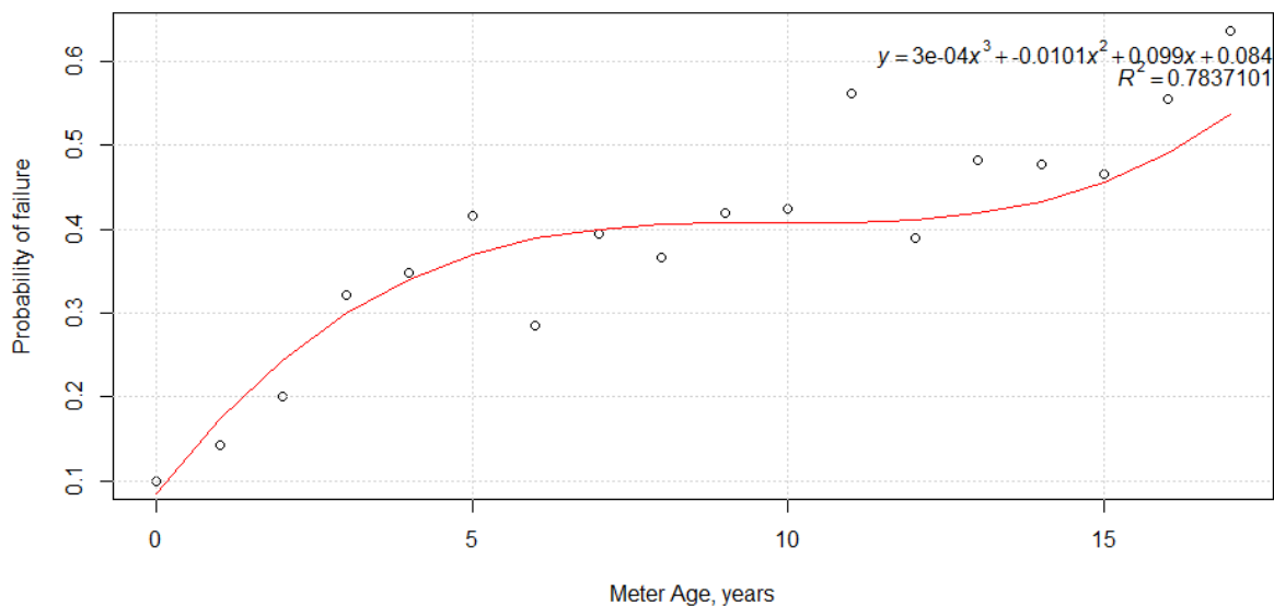
Figure 4-2: Probability of Failure with Age - Volumetric Meters
