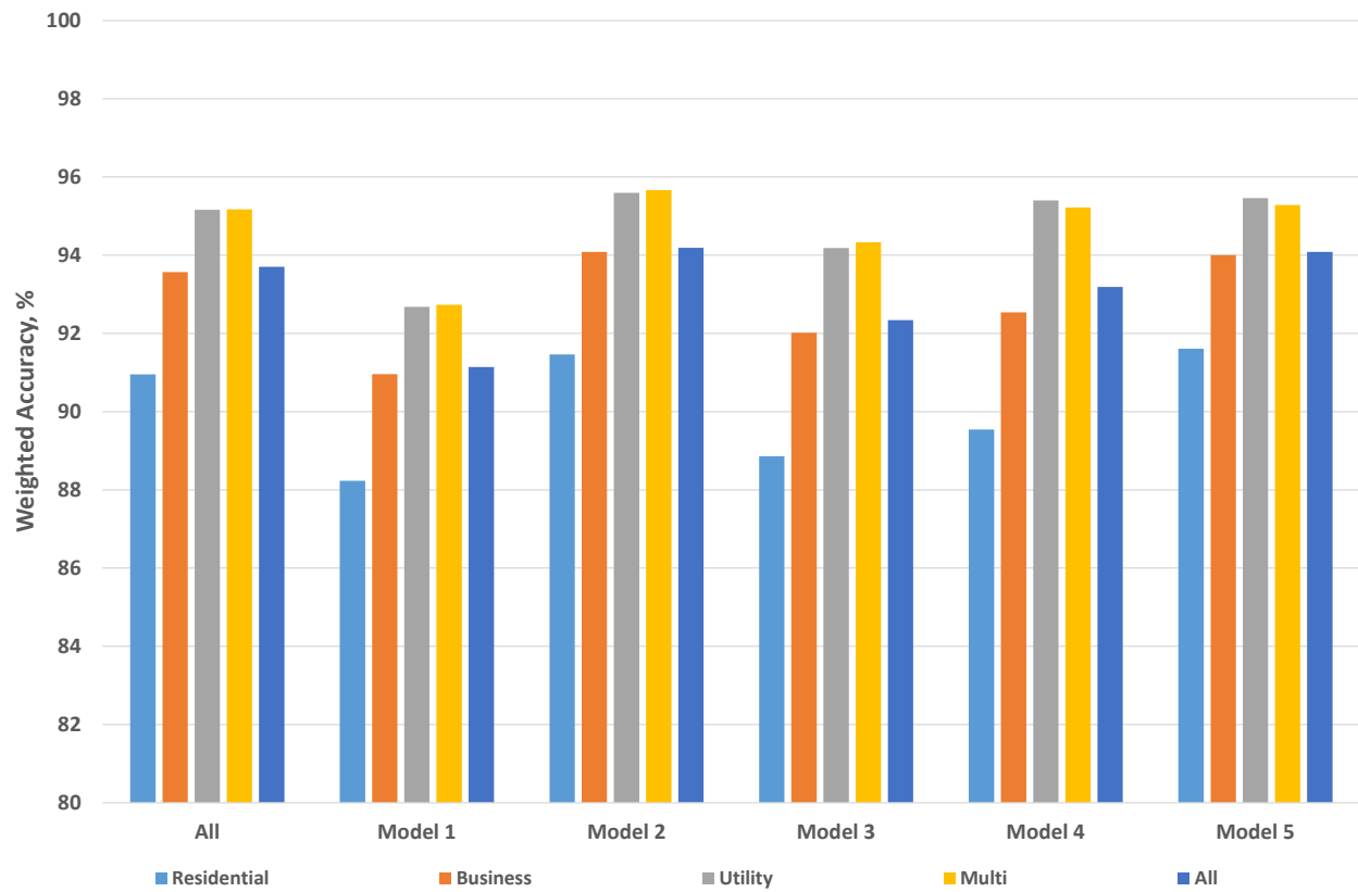
Figure 5-1: Weighted Meter Accuracy – 15mm Meters
