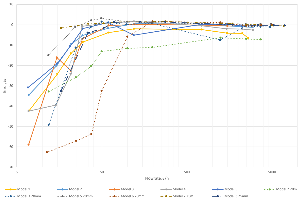
Figure 4-10: Average Error per Meter Model and Size
