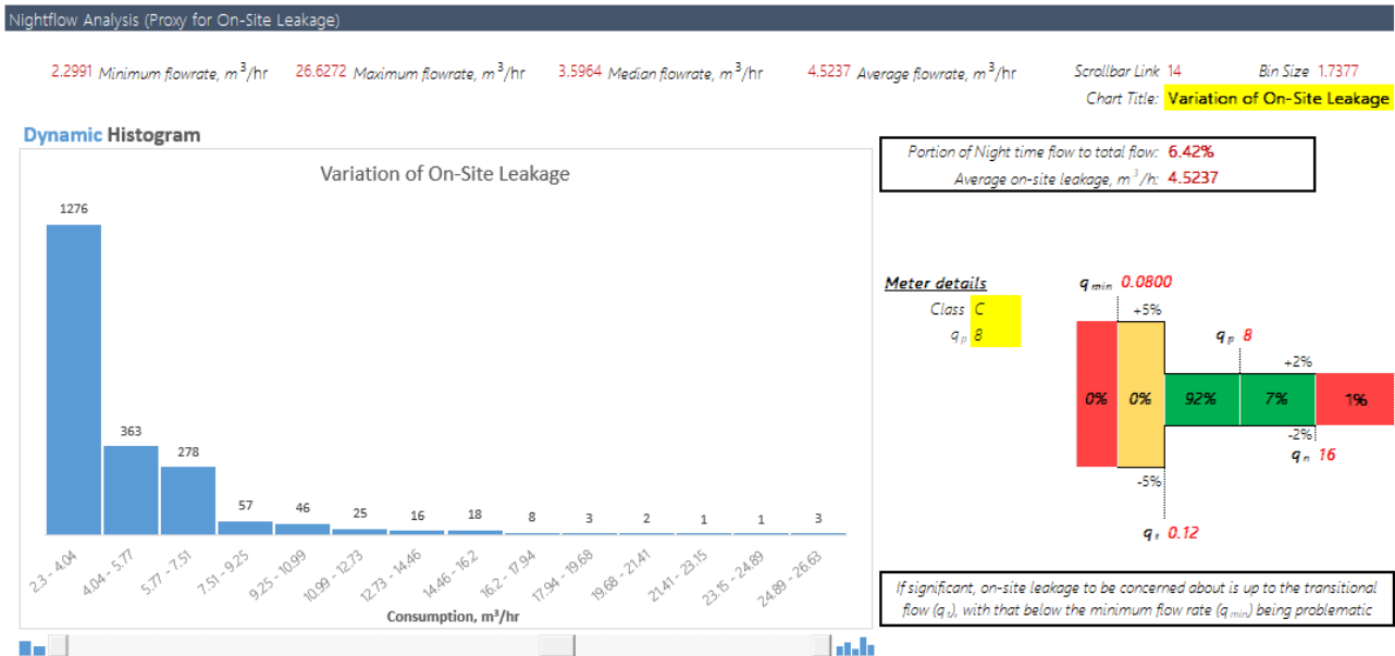
Figure 7-7: Night flow Analysis and Meter Sizing Implications
