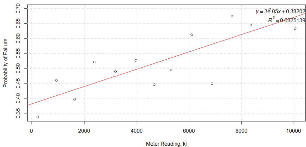
Figure 4-3: Probability of failure with Meter Reading - Volumetric Meters
