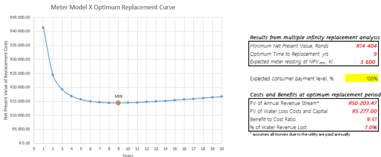
Figure 7-17: Optimum Replacement Period and CBA
