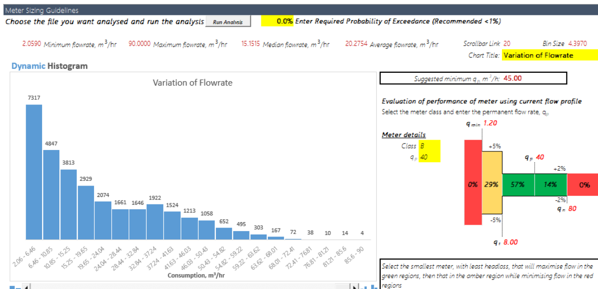
Figure 7-6: Consumption Profile and Meter Sizing Guideline
