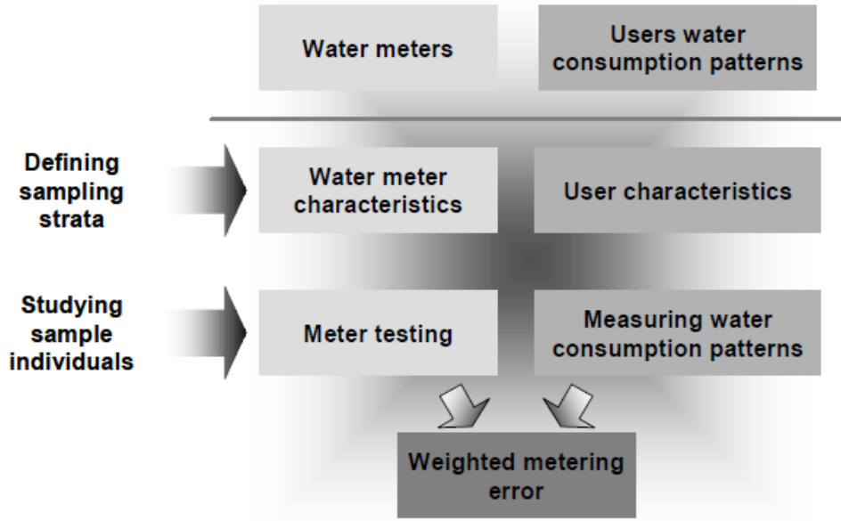
Figure 2-4: Methodology for determining weighted meter accuracy
