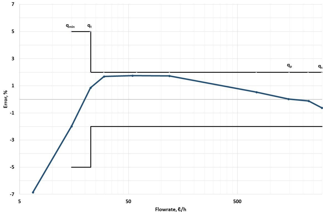
Figure 5-3: Error Curve for a random 15mm meter
