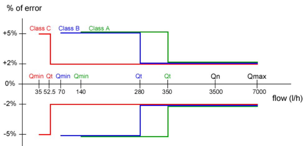
Figure 2-8: Illustration of Difference in Meter Classes ( Q_p = 3,500 \text{ l/h} )
