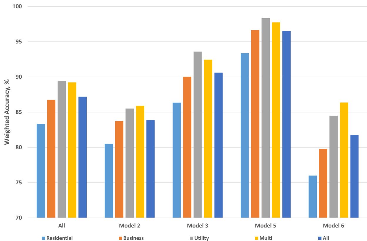
Figure 5-2: Weighted Meter Accuracy – 20mm Meters
