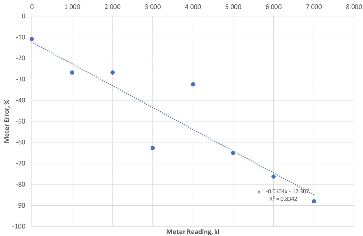
Figure 4-9: Q1 Error Degradation – Volumetric Meters
