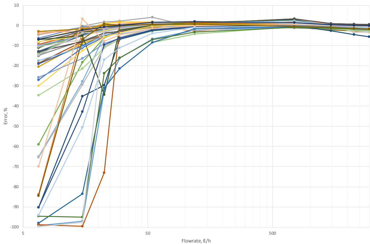
Figure 4-8: Model 2 – 15mm Test Results
