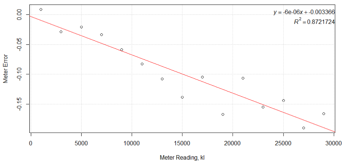
Figure 5-6: Error degradation with meter reading - Meter Change
