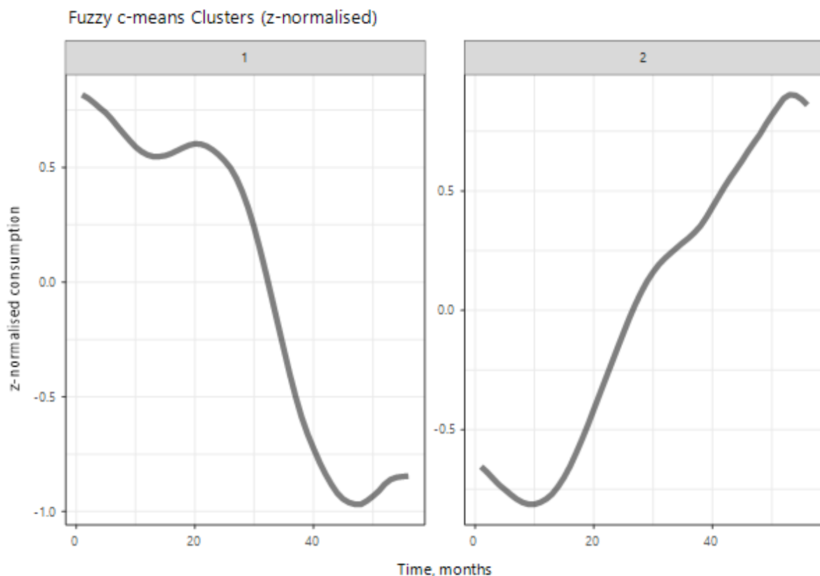
Figure 6-10: Fuzzy Clusters
