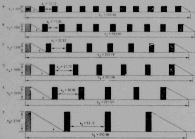
Fig. 25 b) If the illumination angle and the number of rooms remain the same, the site area diminishes as the number of storeys increases
