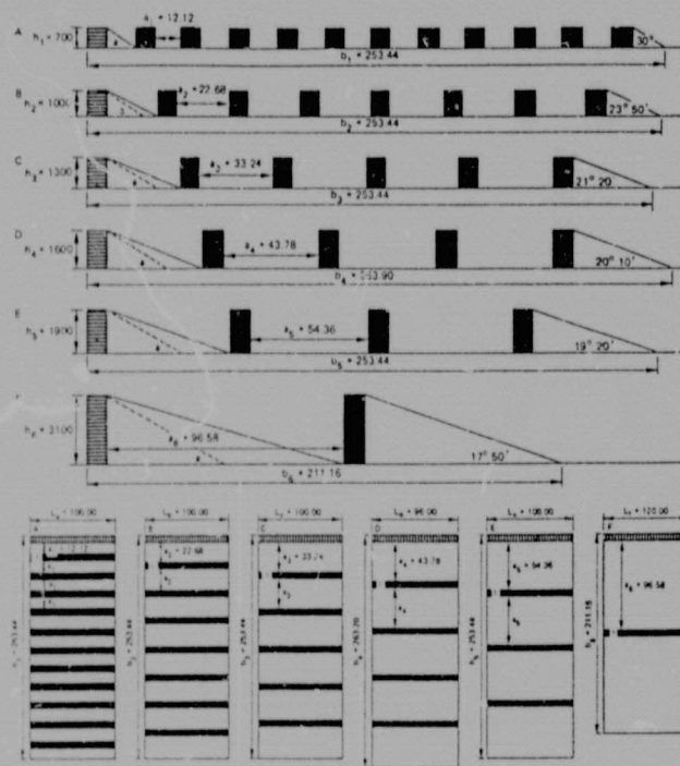
Fig. 25 c) If the site area and the number of rooms remains the same, the illumination angle diminishes and the sun exposure improves with the number of storeys
