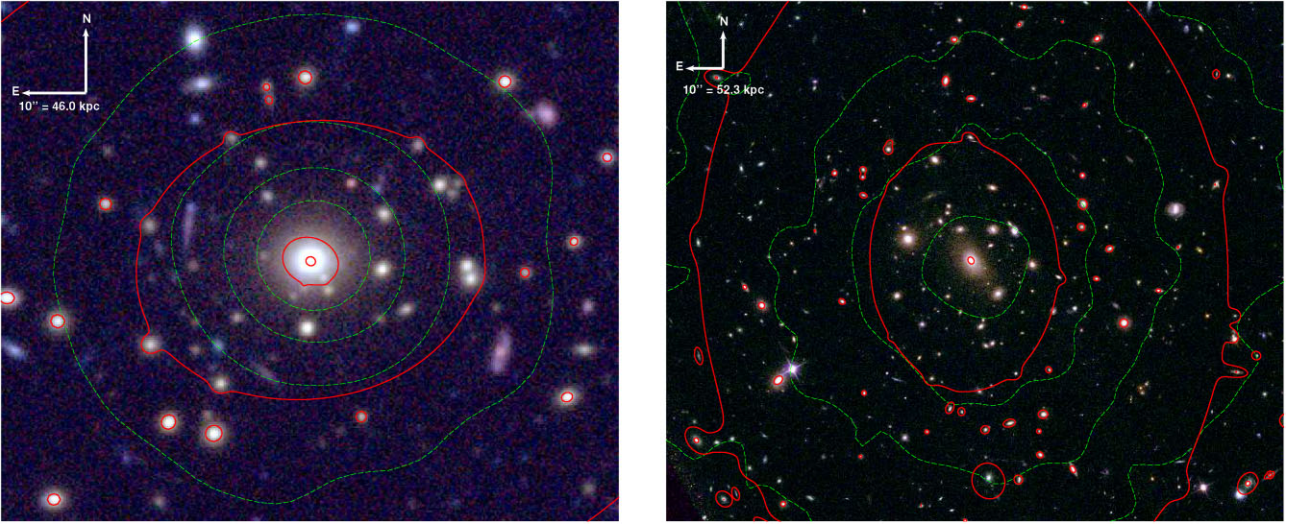
Figure 1. Composite RGB colour images of the two lensing clusters. Left: Composite DES colour image of MACSJ0242. Right: Composite colour HST image of MACSJ0949. Green: Hot gas distribution, obtained with XMM-Newton observations. Red: Contours of equal density, inferred from lensing models.
