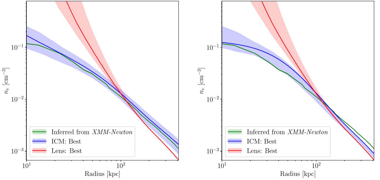
Figure 7. Electron density n_e for i dPIE model, for cluster MACS J0242. Green : X-ray surface brightness deprojected profile (assuming spherical symmetry). Blue : Best ICM-optimized profile, with an i dPIE model. Red : Best lens model inferred profile. Left : In the case of the optimization of parameters \rho_{0,1} , a_1 , s_1 , and \rho_{0,2} , as illustrated in Fig. 6. Right : In the case of the optimization of parameters \rho_{0,1} , a_1 and \rho_{0,2} , as illustrated in Fig. E2. This shows the lens-optimized ICM density model to be inconsistent with the X-ray data. As shown on Fig. 6, the X-ray optimized \rho_{0,2} parameter yields lower values than the SL ones. This may be caused by ICM turbulence in the centre, or simply due to central total densities much larger than modelled through the polytropic temperature model (equation 24). More significantly, the offset in the ICM-optimized model on the right-hand panel shows that if s_1 is not optimized, the larger scales ( \gtrsim 100 kpc) n_e densities can not be properly fitted.
