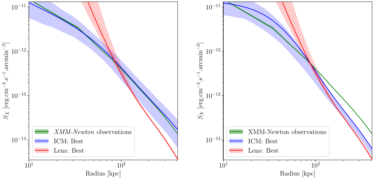
Figure 8. Expected X-ray surface brightness S_X for i dPIE model, for cluster MACS J0242. Green : X-ray surface brightness deprojected profile (assuming spherical symmetry). Blue : Best ICM-optimized profile, with an i dPIE model. Red : Best lens model inferred profile. Left : In the case of the optimization of parameters \rho_{0,1} , a_1 , s_1 , and \rho_{0,2} , as illustrated in Fig. 6. Right : In the case of the optimization of parameters \rho_{0,1} , a_1 , and \rho_{0,2} , as illustrated in Fig. E2.
