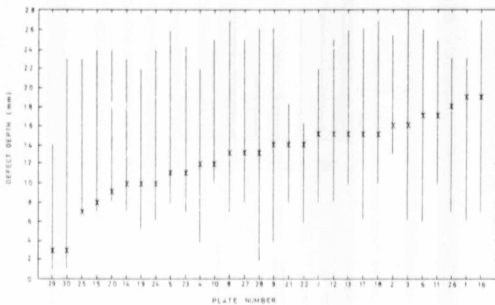
Figure 2.7 The range in UT predictions of defect depths. (Actual defect depth indicated by X).
