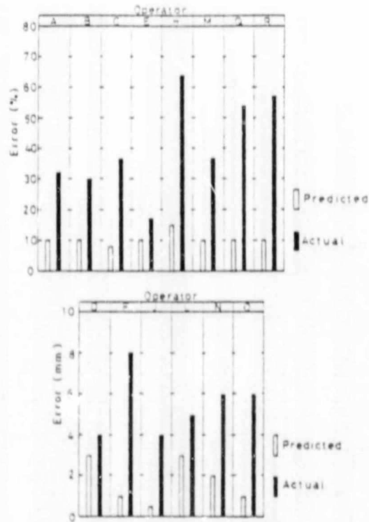
Figure 2.8 The calculated average error of each operator compared to his estimated error on defect heights.
