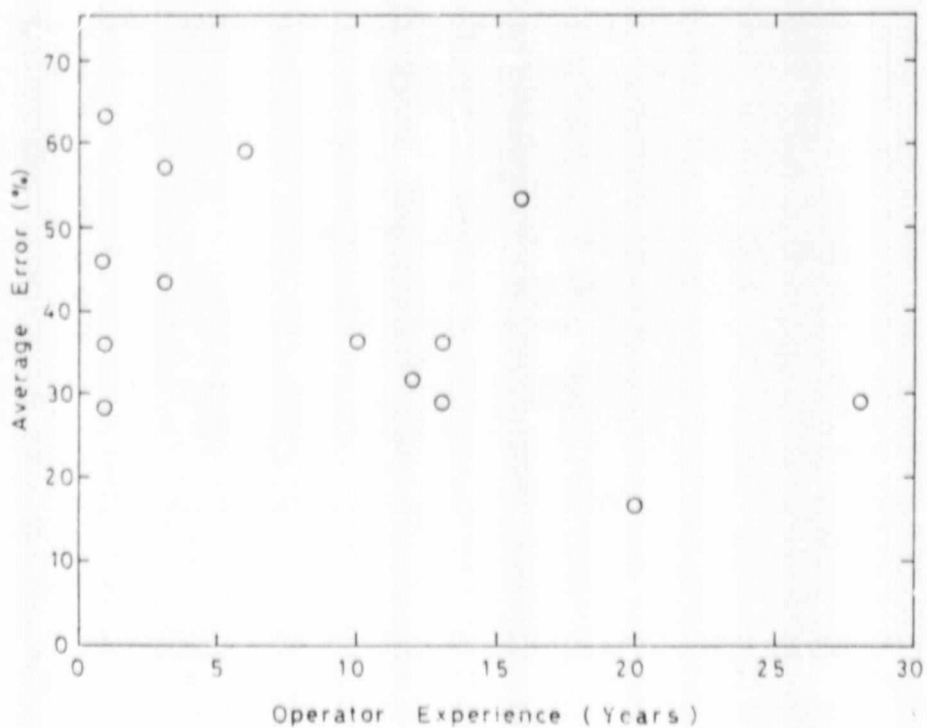
Figure 2.11 The average error in predicting defect heights plotted against the number of years experience of each operator.
