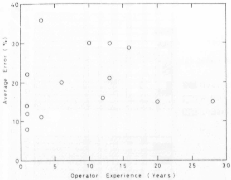
Figure 2.12 The average error in predicting defect lengths plotted against the number of years experience of each operator.
