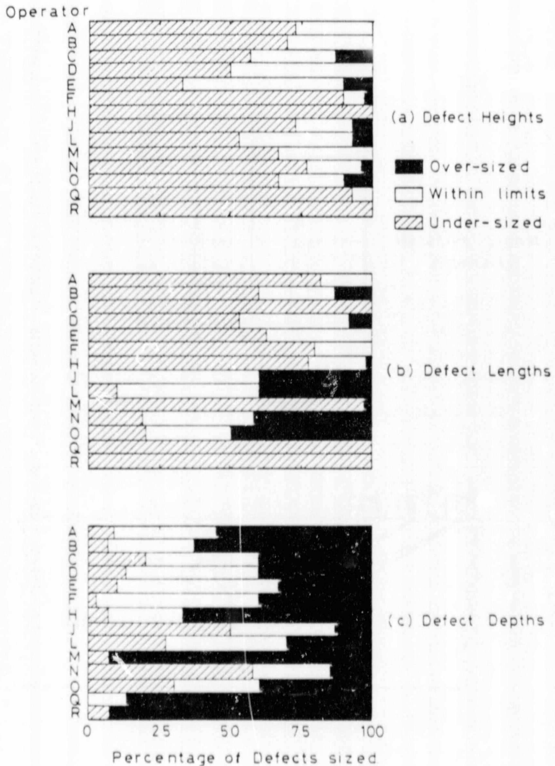
Figure 2.14 Schematic illustration of the ability of each operator to measure the defects to within his own error band. (eg. in the height measurements, operator E undersized 10 of the 30 defects (33%), oversized 3 of the defects (10%) and sized the remaining 17 defects (57%) within his estimated error of \pm 10\% ).
