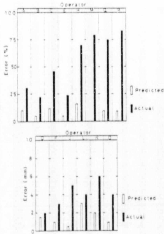
Figure 2.10 The calculated average error of each operator compared to his estimated error on defect depths.
