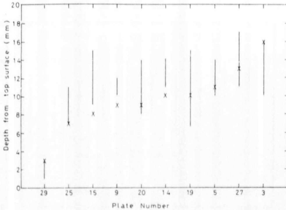
Figure 2.16 The range in ultrasonic predictions of defect depths from the top surface, as measured in the second test programme. The actual depth in each case is indicated by X.
