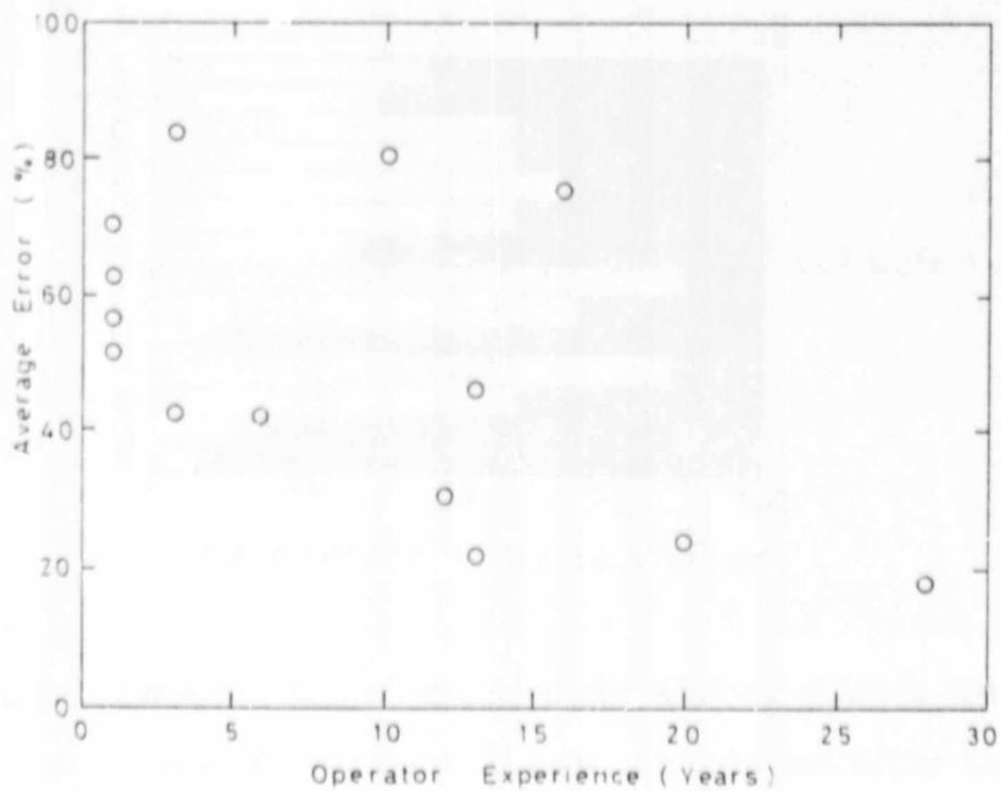
Figure 2.13 The average error in predicting defect depths plotted against the number of years experience of each operator.
