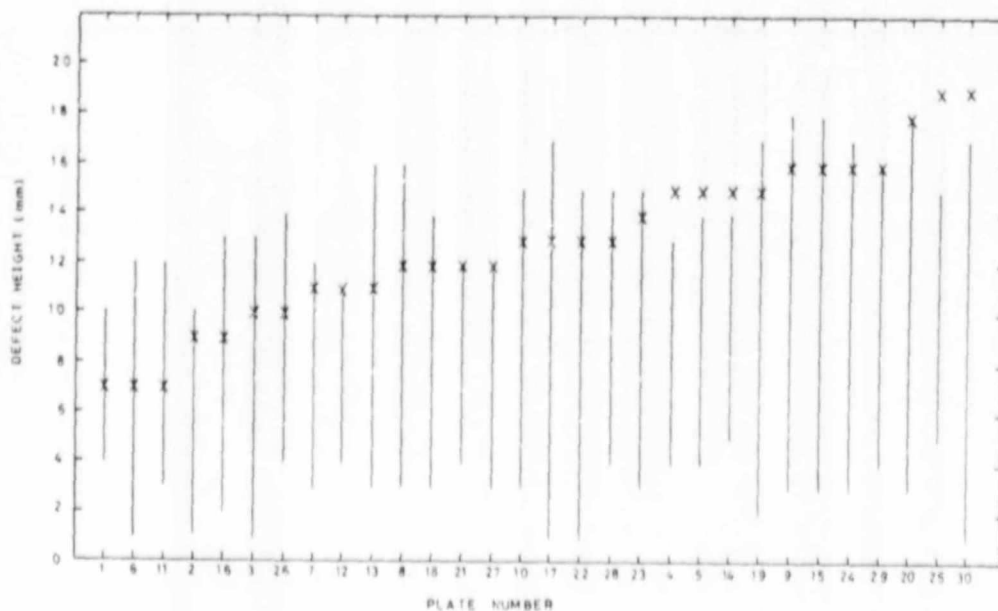
Figure 2.5 The range in UT predictions of defect heights. (Actual defect height indicated by X).
