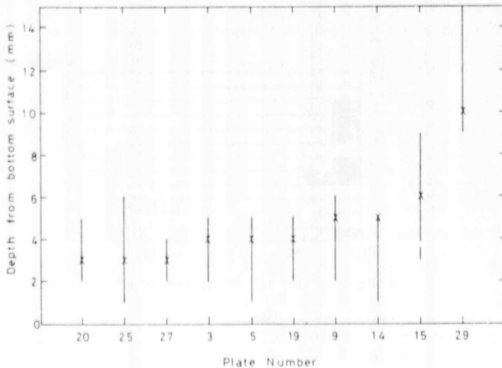
Figure 2.17 The range in ultrasonic predictions of defect depths from the bottom surface, as measured in the second test programme. The actual depth in each case is indicated by X.
