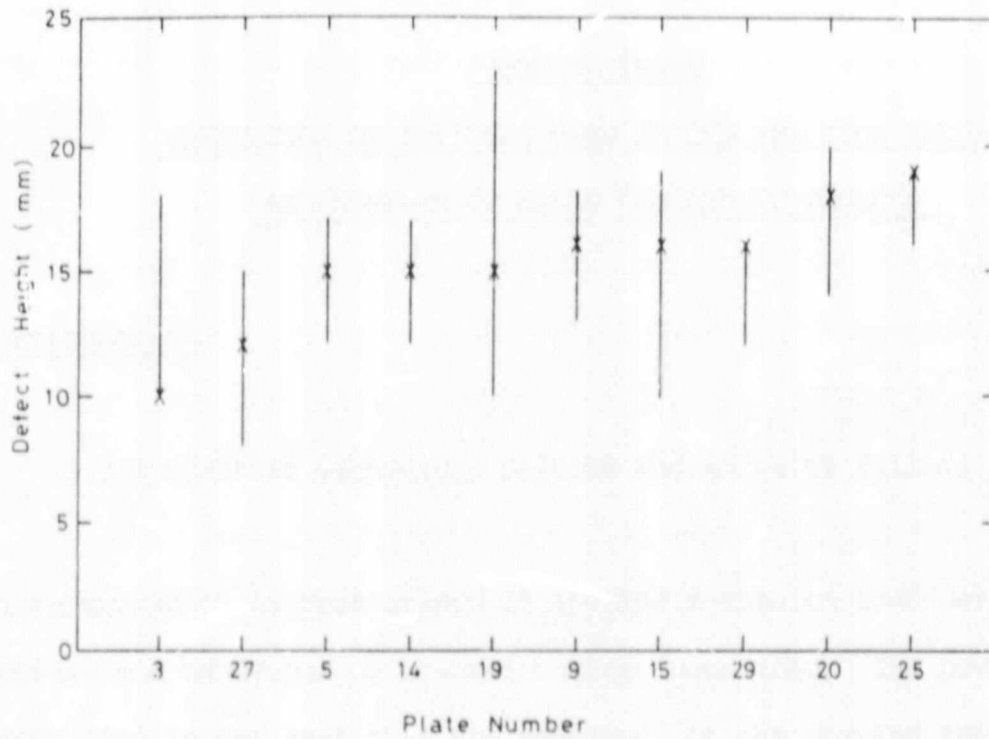
Figure 2.18 The range in ultrasonic predictions of defect heights, as measured in the second test programme. The actual height in each case is indicated by X.
