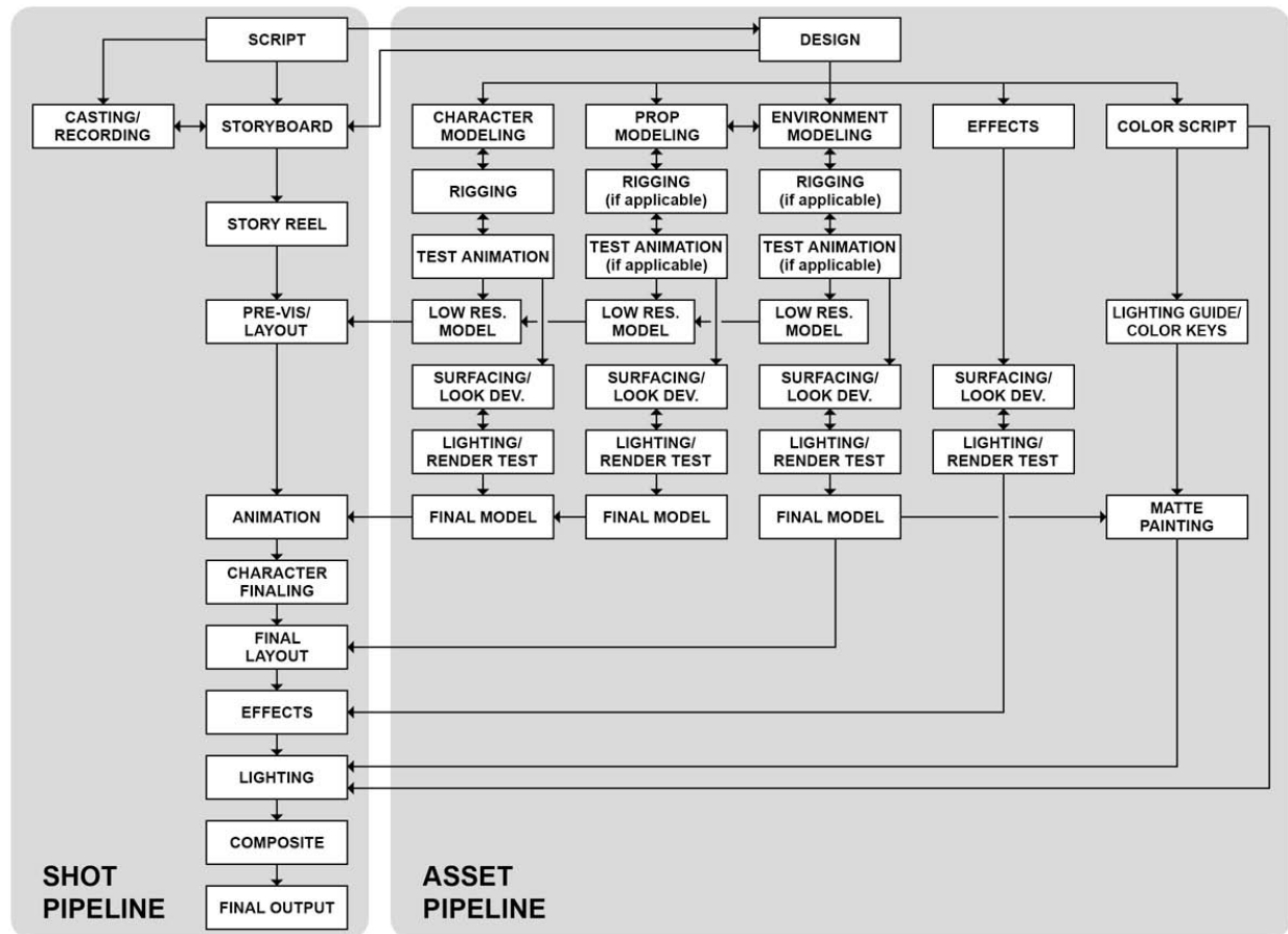
Figure 1: 3D CGI Production Pipeline (Winder and Dowlatbadi 250).
