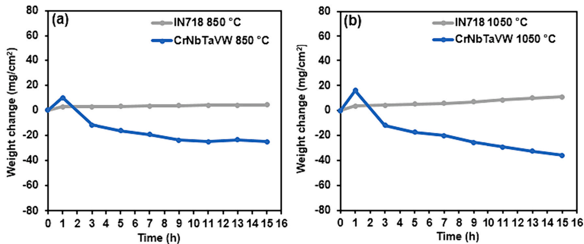
Fig. 6. Cyclic oxidation curve of CrNbTaVW RHEA and IN718 alloy at 850 °C (a); Cyclic oxidation oxidation curve of CrNbTaVW RHEA and IN718 alloy at 1050 °C (b).
