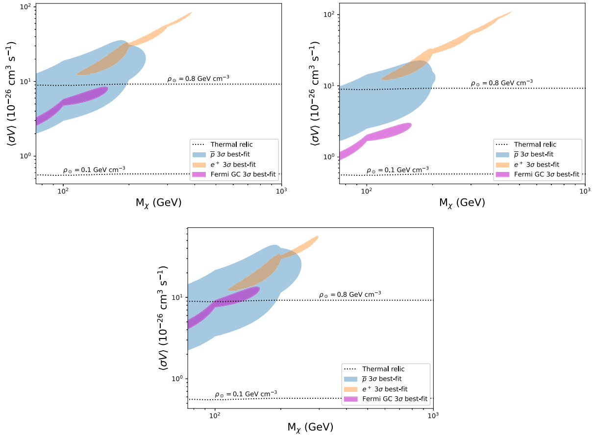
Fig. 3. The parameter space fitting the 2 \rightarrow 2 scattering to the Fermi-LAT galactic centre excess, AMS-02 anti-proton and positron spectra. The shaded regions represent the 3\sigma confidence interval. The region between the thermal relic lines represents the uncertainties in local DM density and galactic halo profile. This plot assumes the MED diffusion scenario. The 3 plots correspond to different Milky-Way DM halo profiles from [43]. Top left: Einasto profile. Top right: contracted Einasto. Bottom: NFW.
