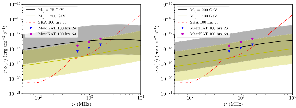
Fig. 4. Radio spectrum prediction for Reticulum II with the Einasto profile. The shaded regions encompass the cross-section uncertainties from 3, as well as those from the J-factor of the halo and magnetic field. Left: 2 \rightarrow 2 scattering. Right: 2 \rightarrow 3 scattering.
