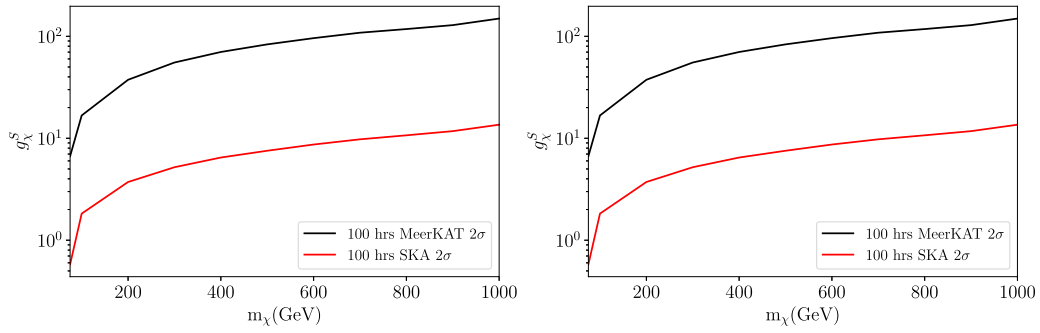
Fig. 7. Non-observation 2\sigma exclusion projections on the coupling between S and \chi ( 2 \rightarrow 2 case) for Reticulum II (Einasto profile) with MeerKAT and the SKA. Left: Milky-Way galactic centre with Einasto profile. Right: Milky-Way galactic centre with NFW profile.
