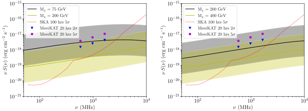
Fig. 5. Radio spectrum prediction for Reticulum II with the Einasto profile. The shaded regions encompass the cross-section uncertainties from 3, as well as those from the J-factor of the halo and magnetic field. Left: 2 \rightarrow 2 scattering. Right: 2 \rightarrow 3 scattering.
