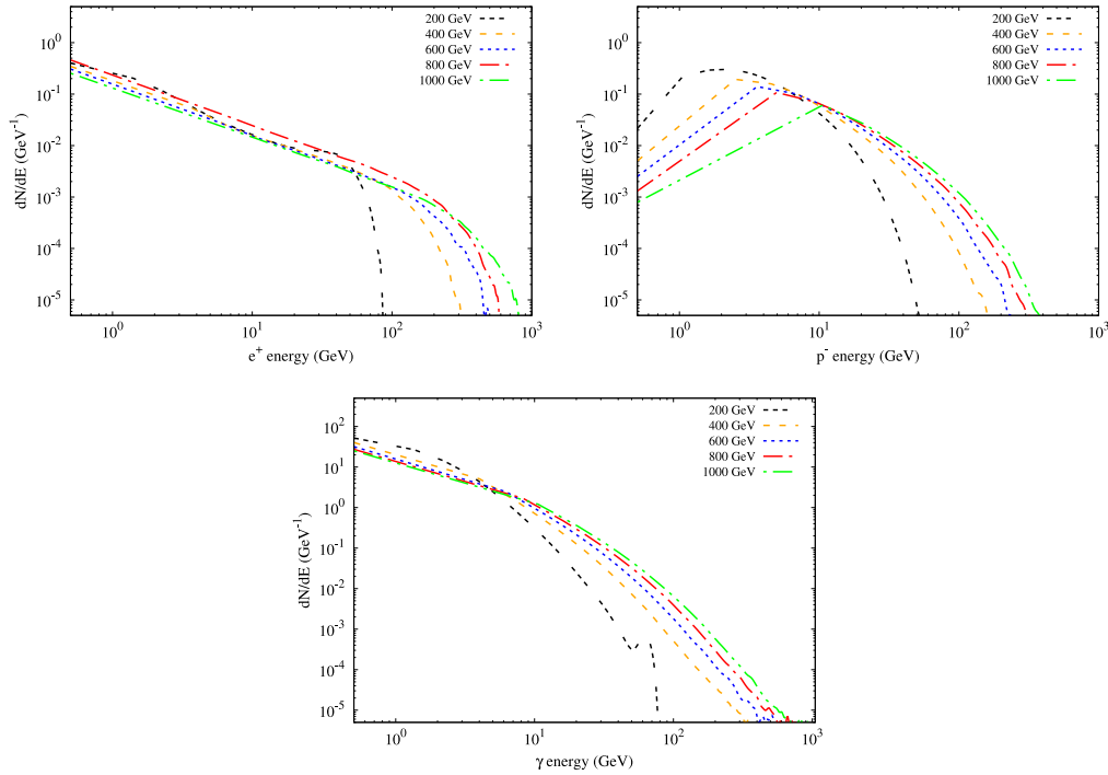
Fig. 2. Differential yields of positrons, anti-protons and photons for the 2 \rightarrow 3 annihilation process of Spin-0 DM for a variety of WIMP masses. Model parameters are fixed according to [9,10], based on LHC data.
