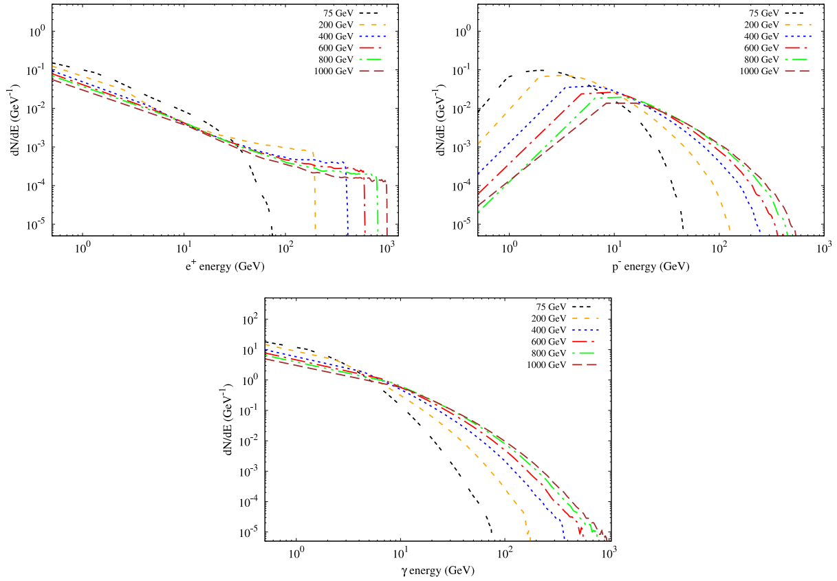
Fig. 1. Differential yields of positrons, anti-protons and photons for the 2 \rightarrow 2 annihilation process of Spin-0 DM for a variety of WIMP masses. Model parameters are fixed according to [9,10], based on LHC data.
