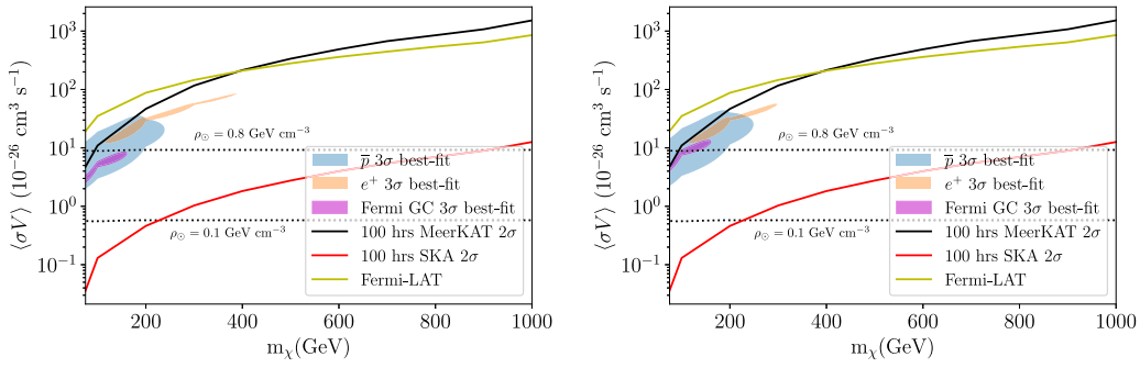
Fig. 6. Non-observation 2\sigma exclusion projections for Reticulum II (Einasto profile) with MeerKAT and the SKA. Left: Milkyway-Way galactic centre with Einasto profile. Right: Milkyway-Way galactic centre with NFW profile. The shaded regions are drawn from Fig. 3. The Fermi-LAT limits are drawn from data found in [72] and we use a 30' integration region in this case.
