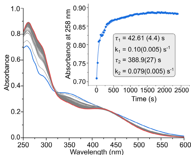
Figure 5. Electronic absorption spectra of 40 \mu\text{M} AuL in a water (10% V/V) and DMSO mixture containing GSH at a molar ratio of 1:1 [\text{AuL}]:[\text{GSH}] . The inset shows the change in absorbance at 258 nm as a function of time. The data are fitted to a standard double exponential kinetic function, = K_1 e^{-x/t_1} + K_2 e^{-x/t_2} + A_\infty , where k_1 and k_2 are adjustable pre-exponential factors, t_1 and t_2 are the time constants, and A_\infty the limiting absorbance.
