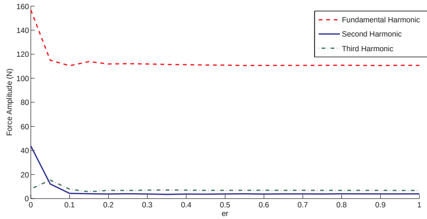
Figure 4.25: Second order harmonic while changing er . (Configuration 2)
