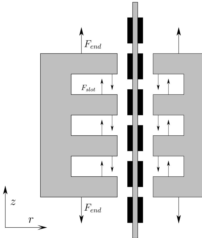
Figure 4.2: Cogging Forces.
