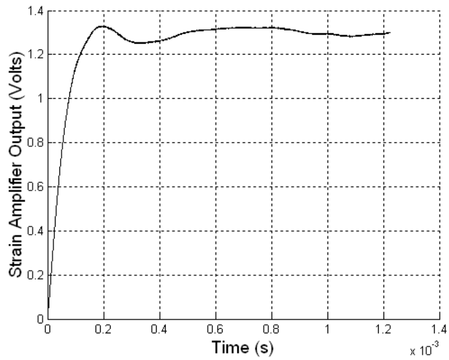
Figure 5.5 Step Response for Cone 3
