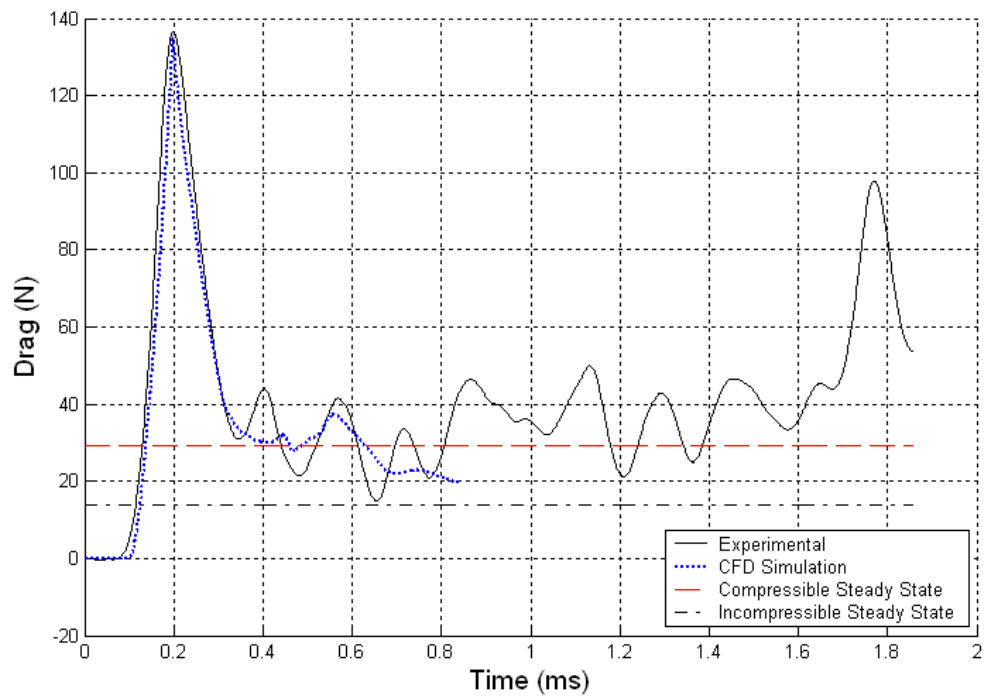
Figure 5.27 Combined Drag Results – Cone 1 Mach 1.27
