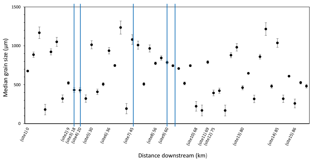
Figure 7. Scatterplot of median grain size ( \mu\text{m} ) of sediment samples from the Letaba River, arranged in a downstream direction from site 1. Error bars indicated one standard deviation. The vertical blue lines indicate the major tributaries as locations of sediment input (named in Table 1).
