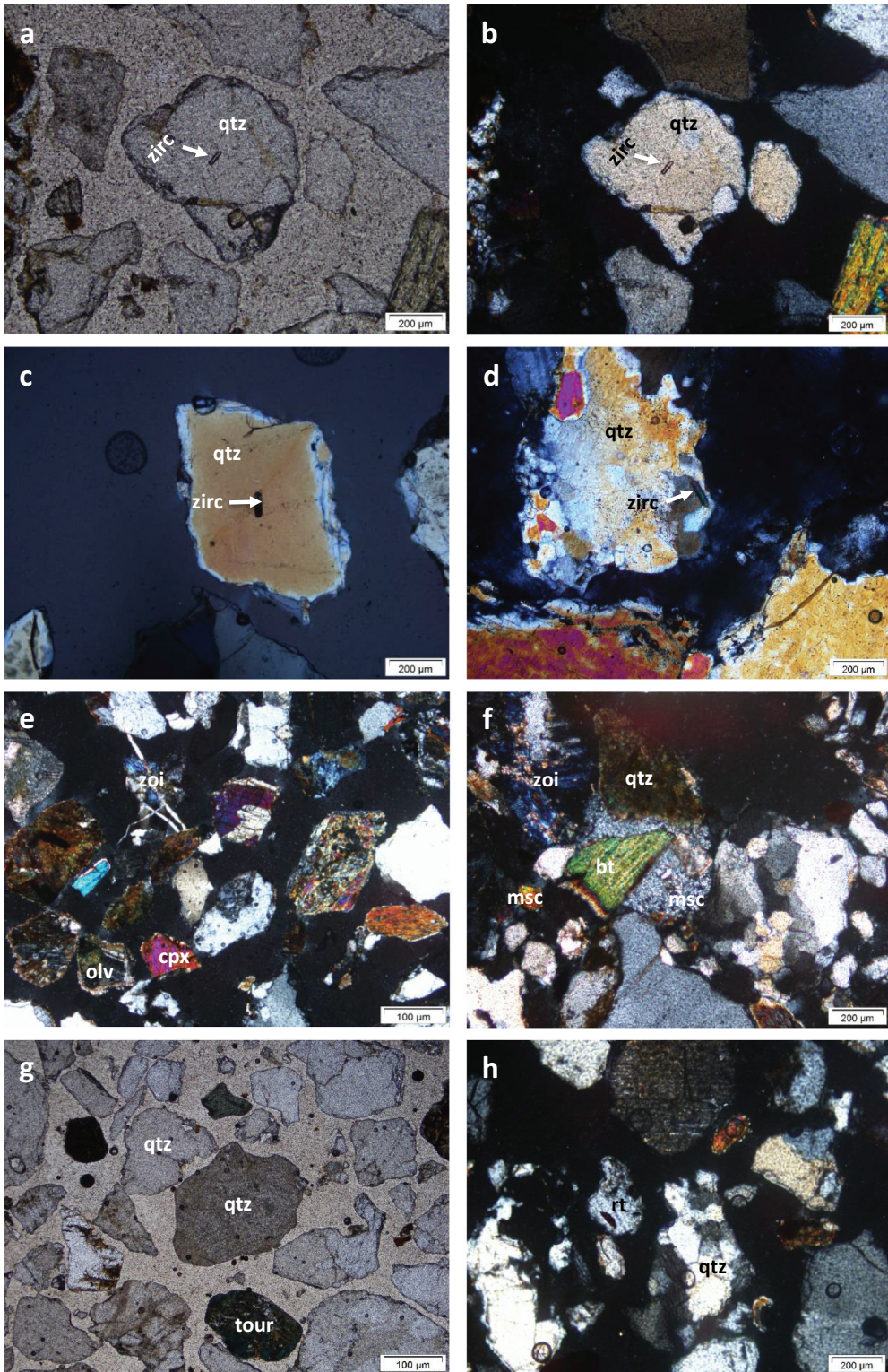
Figure 8. Images from polished slides indicating minerals present in the sediment. (a, b) Columnar zircon inclusion in a quartz grain from site 10, in plain light (a) and crossed polar (b), (c) zircon
