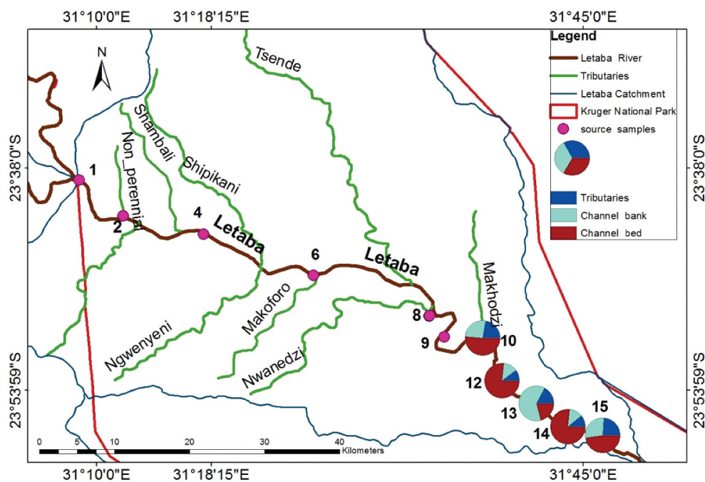
Figure 10. Map showing the contribution of tributary, channel bank and channel bed sources to downstream sites 10–15.
