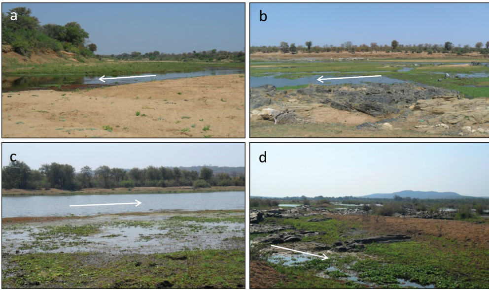
Figure 5. Field photos from the Letaba River. (a) The Groot Letaba River (site 1) with a vegetated sandbar alongside the active channel; (b) vegetated sandbars separating multiple channels (site 4); (c) a single, straight deep channel with a wide, flat, vegetated floodplain (site 10); (d) bedrock outcrops and isolated sediment patches (site 15). Arrows show water flow direction.
