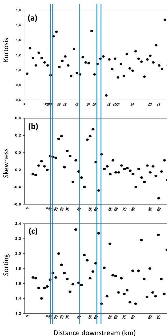
Figure 6. Scatterplots of (a) kurtosis, (b) skewness and (c) sorting of sediment samples from the Letaba River, arranged in a downstream direction from site 1. The vertical blue lines indicate the major tributaries as locations of sediment input (named in Table 1).
