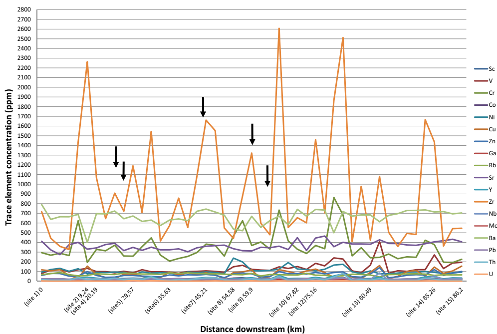
Figure 9. Graph indicating the trace elements and their abundance in different sediment samples in a downstream direction from site 1 from left to right. The arrows indicate the locations of major tributaries (Table 1). Precise values of trace elements are given in supplementary data file A.
