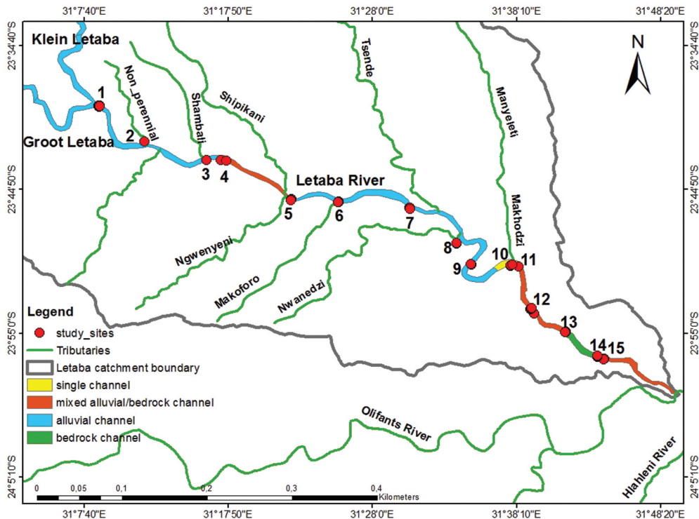
Figure 4. Map of the lower Letaba River within Kruger National Park, showing the geomorphic classification of river reaches (based on Moon & Heritage, 2001, and updated with mapping in this study), and the locations of sites 1–15 (see Table 1).
