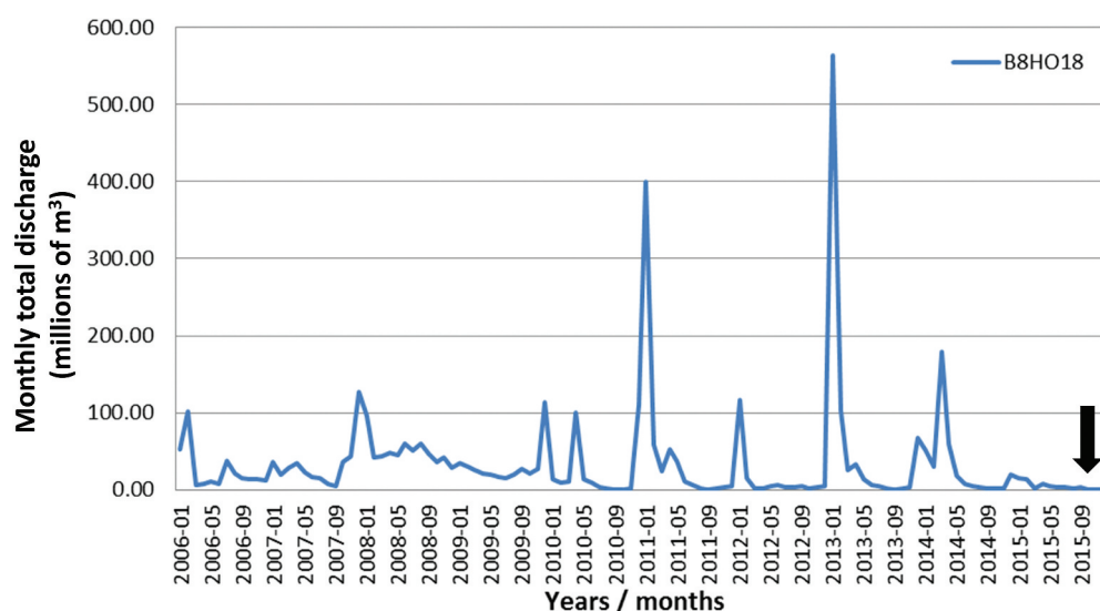
Figure 3. Graph of historical river discharge recorded at the Engelhardt Dam gauging station (B8H018) on the lower Letaba River (location is marked in Figure 2), for the period 2006–15, including the sediment sampling period in this study (indicated with the black arrow). Values represent total monthly water volumes in millions of \text{m}^3 .
