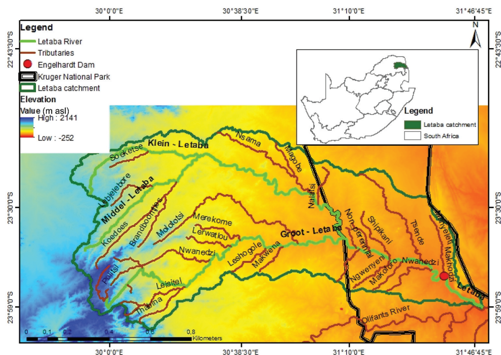
Figure 2. Topographic context of the Letaba River catchment and its major tributaries. The eastern half of the catchment flows through the Kruger National Park.
