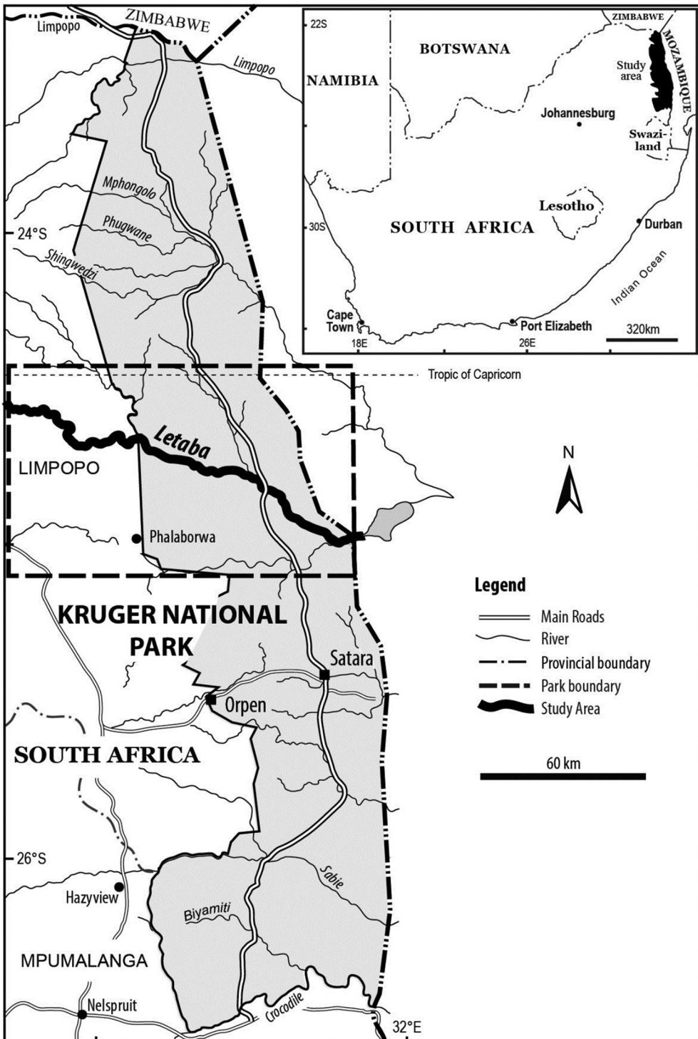
Figure 1. Location of the lower Letaba River (boxed) within the Kruger National Park and South Africa.
