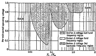
FIGURE 1-5-8 : Regions of possible neutral instability for the circuit of FIGURE 1-5-6
