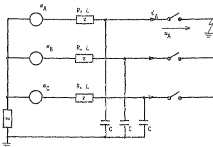
FIGURE 1-4-1 : Single phase to earth fault - equivalent diagram for transient analysis
