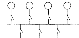
FIGURE A1 : Power station layout with generators paralleled at generator voltage.
