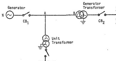
FIGURE 4-1 : Unit connected scheme utilising a generator circuit breaker.
