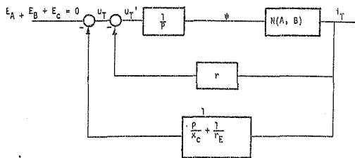
FIGURE C2 : Block diagram for "zero sequence" quantities.
