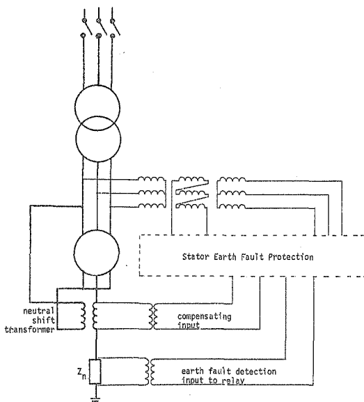
FIGURE 1-6-1 : Stator Earth fault protection scheme to ensure 100% coverage of stator winding.
