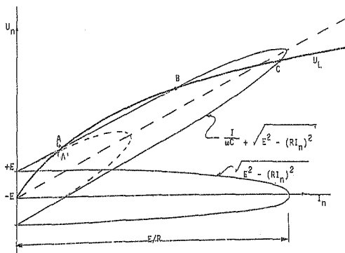
FIGURE 1-5-5 : Graphical analysis for R_n \neq 0
