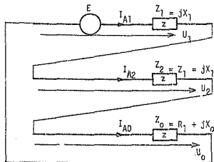
FIGURE B1 : Sequence networks for single phase to earth fault.
