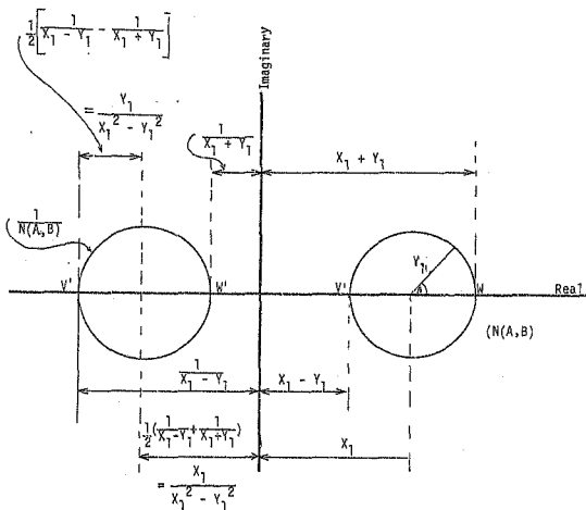
FIGURE DL : Locus of -\frac{1}{N(A,B)} derived from N(A,B) in the complex plane (A and B constant and \beta variable).
