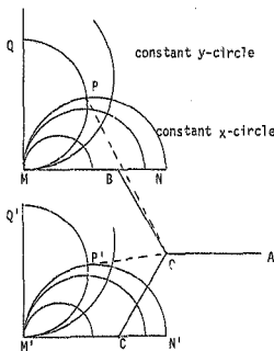
FIGURE B2 : Diagram for steady state overvoltages on sound phases during a single phase to earth faults.
