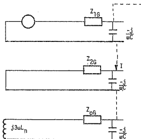
FIGURE 2-1-3 (b) : Interconnected sequence diagram for FIGURE 2-1-3 (a).
