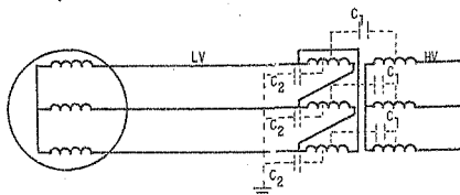
FIGURE 2-1-1 : Capacitive coupling between high and low voltage windings of generator transformer when HV neutral is not earthed.
