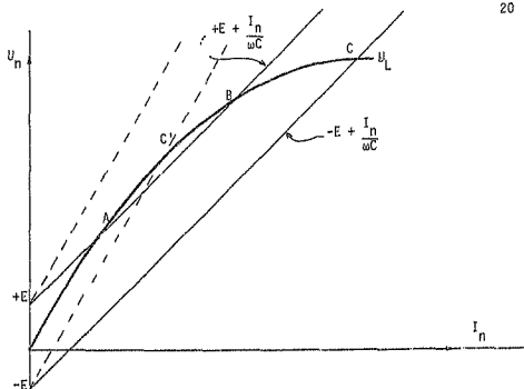
FIGURE 1-5-4 : Graphical Analysis of circuit with R_n = 0
