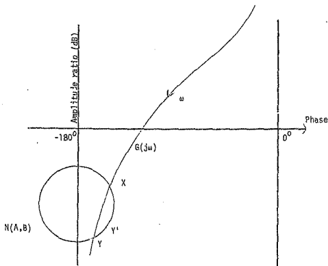
FIGURE 1-5-14 : Circular describing function characteristic and frequency transfer function in the amplitude ratio/phase plane
