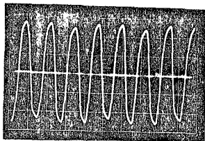
FIGURE 1-5-16 : Third harmonic neutral displacement voltage U_n .
