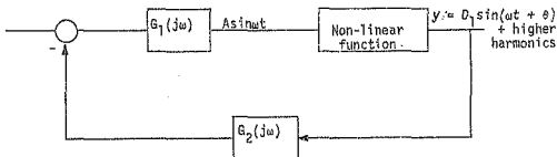
FIGURE 1-5-9 : Block diagram of system for DF analysis
