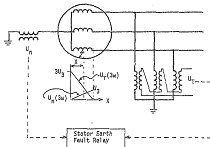
FIGURE 1-6-3 : Earth fault protection utilising both neutral and terminal third harmonic voltages for 100% stator earth fault protection.
