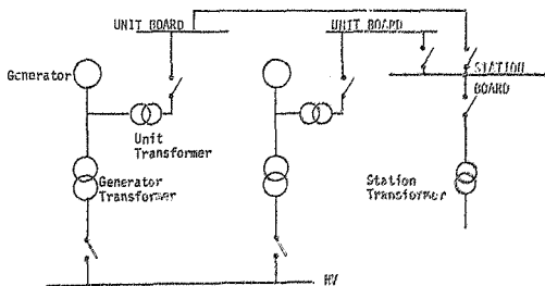
FIGURE A2 : Unit-connected power station layout.
