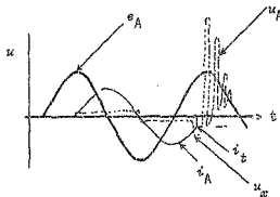
FIGURE 1-4-2 (a) : Recovery voltage across circuit breaker for reactor earthing
