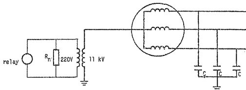
FIGURE 2-1-2 : High resistance earthing scheme for generator distribution transformer earthing.
