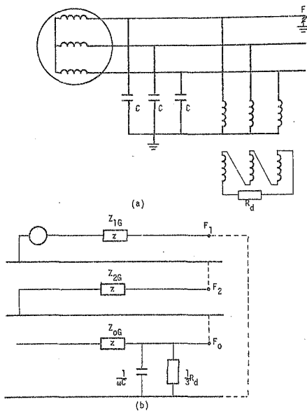
FIGURE 4-3 : Earthing scheme and sequence networks for a single phase to earth fault.
