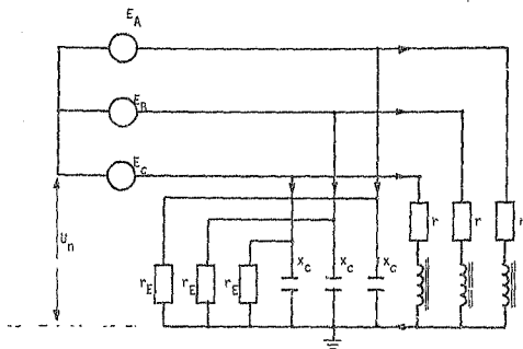
FIGURE 1-5-10 : Complete three phase diagram under analysis
