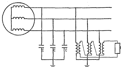
FIGURE 1-6-2 : Generator earth fault protection scheme utilising third harmonic voltage for 100% coverage.
