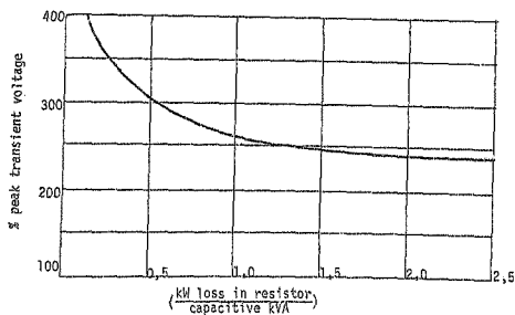
FIGURE 1-4-5 : Transient voltages for any number of restrikes in fault arc or cross circuit breaker contacts
