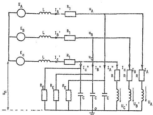
FIGURE C1 : Circuit diagram for three phase generator earthing scheme.
