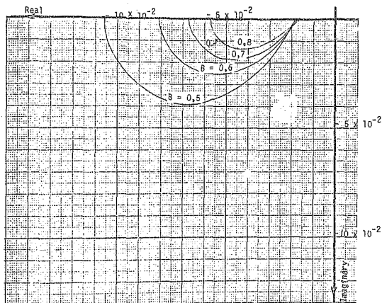
FIGURE 1-5-17 : Third harmonic DF for experimental set up. Complex value of G(x_c) indicated by point Q.
