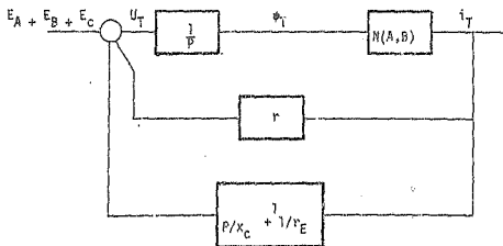
FIGURE 1-5-11 : Block diagram for zero sequence quantities
