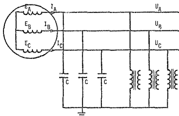
FIGURE 1-5-6 : Circuit for analysis of neutral instability
