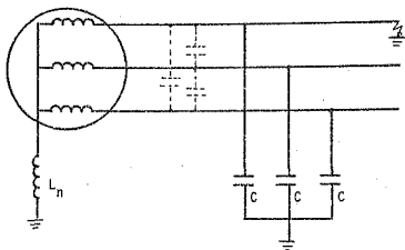
FIGURE 2-1-3 (a) : Resonant earthing of generator - Single phase to earth fault.
