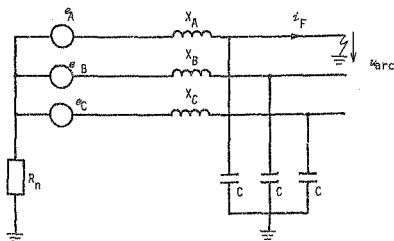
FIGURE 1-4-3 (a) : Single phase fault to earth on a resistively earthed generator
