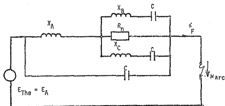
FIGURE 1-4-3 (b): Thévenin equivalent circuit for current in and voltage across arc
