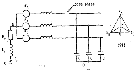
FIGURE 1-5-1 (a) : Broken phase conductor on generator: (i) Circuit diagram and (ii) phasor diagram for ON open circuited.
