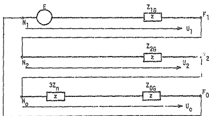
FIGURE 1-2-1 (b) : Sequence networks for FIGURE 1-2-1 (a)
