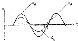
FIGURE 1-4-2 (b) : Recovery voltage across circuit breaker for resistive earthing
