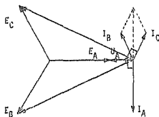
FIGURE 1-5-7 (b) : Phasor diagram for the circuit of FIGURE 1-5-6
