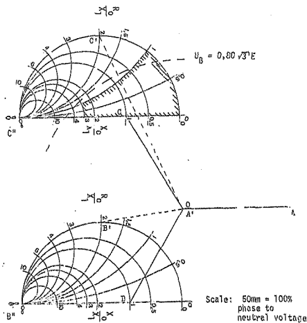
FIGURE 1-3-1 : Steady state overvoltage on phases B and C during a single phase to earth fault on phase A.
