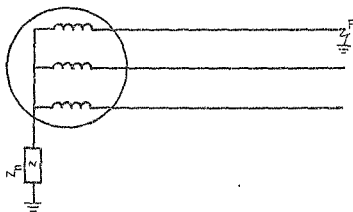
FIGURE 1-2-1 (a) : Single phase fault to earth at generator terminals
