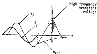
FIGURE 1-4-4 : Voltages and currents pertaining to FIGURE 1-4-3 (a)
