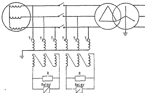
FIGURE 4-2 : Earthing scheme for generator with generator circuit breaker.
