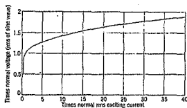
FIGURE 1-5-12: Magnetisation curve of transformer derived from equation
