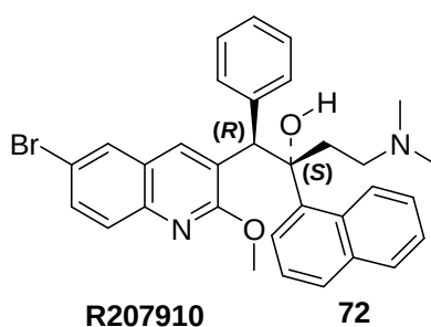
Figure 18: Diarylquinoline derivative.
