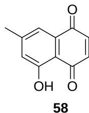
Figure 14: 7-Methyljuglone.
