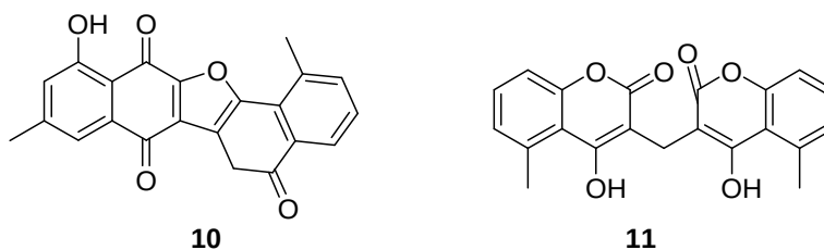
Figure 5: Crassiflorone derivatives
