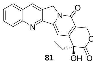
Figure 26: Camptothecin
