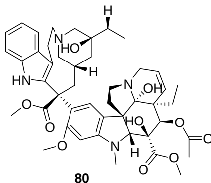
Figure 25: Vinblastine
