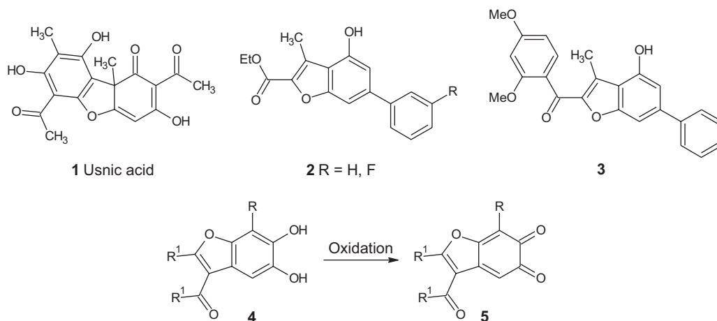
Figure 1. Benzofuran scaffolds.
