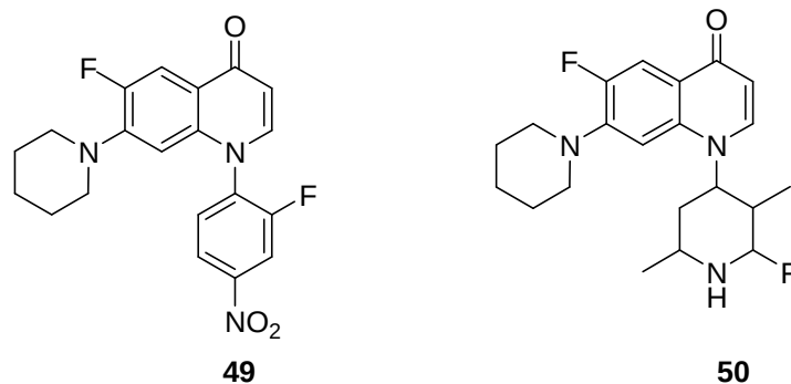
Figure 9: Fluoroquinolone derivatives
