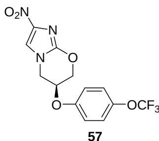
Figure 13: Nitroimidazopyran, PA824.
