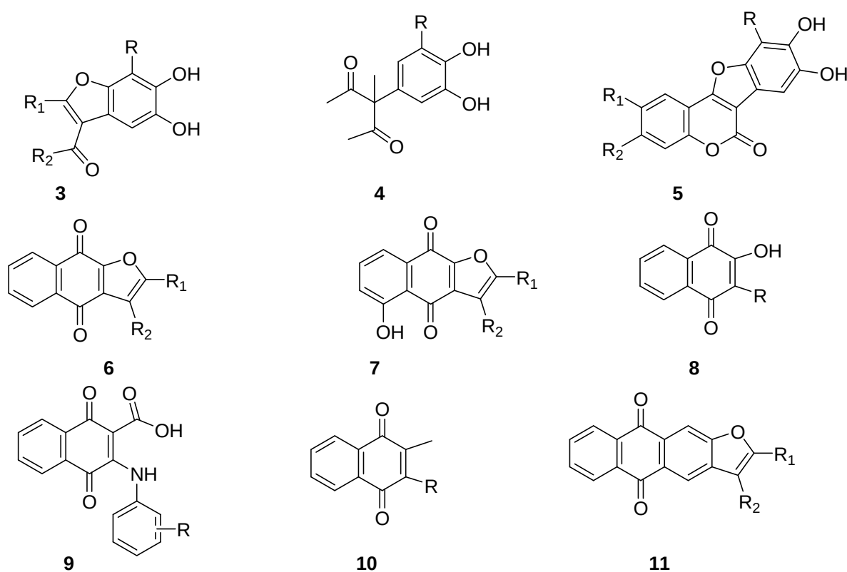
Figure 2: Targeted compounds.
