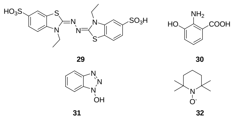
Figure 3: Laccase mediators
