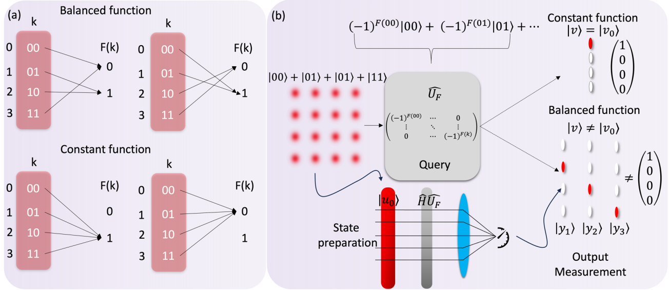
FIG. 2. (a) Conceptual illustration of the balanced and constant functions involved in the Deutsch–Jozsa algorithm for binary strings of length two, i.e., 00, 01, 10, and 11. The two top figures showcase a balanced function that maps half of its inputs to 0 and the other half to 1, and the two bottom figures showcase a constant function that maps all its inputs to either 0 or 1. (b) Illustration of our optical implementation of the Deutsch–Jozsa algorithm. A lattice of Gaussian beams representing the superposition of states is simultaneously prepared by Alice. The state is then queried by Bob in parallel with the action of the compound oracle and Hadamard operations, which impart function evaluations spatially on the state through phase transformations and map us back into the computational basis. A constant function returns the state mapping onto the binary string 00, indicated by the vector lighting up on the first elements. A balanced function returns a state orthogonal to 00, shown by light lobes at different positions.
