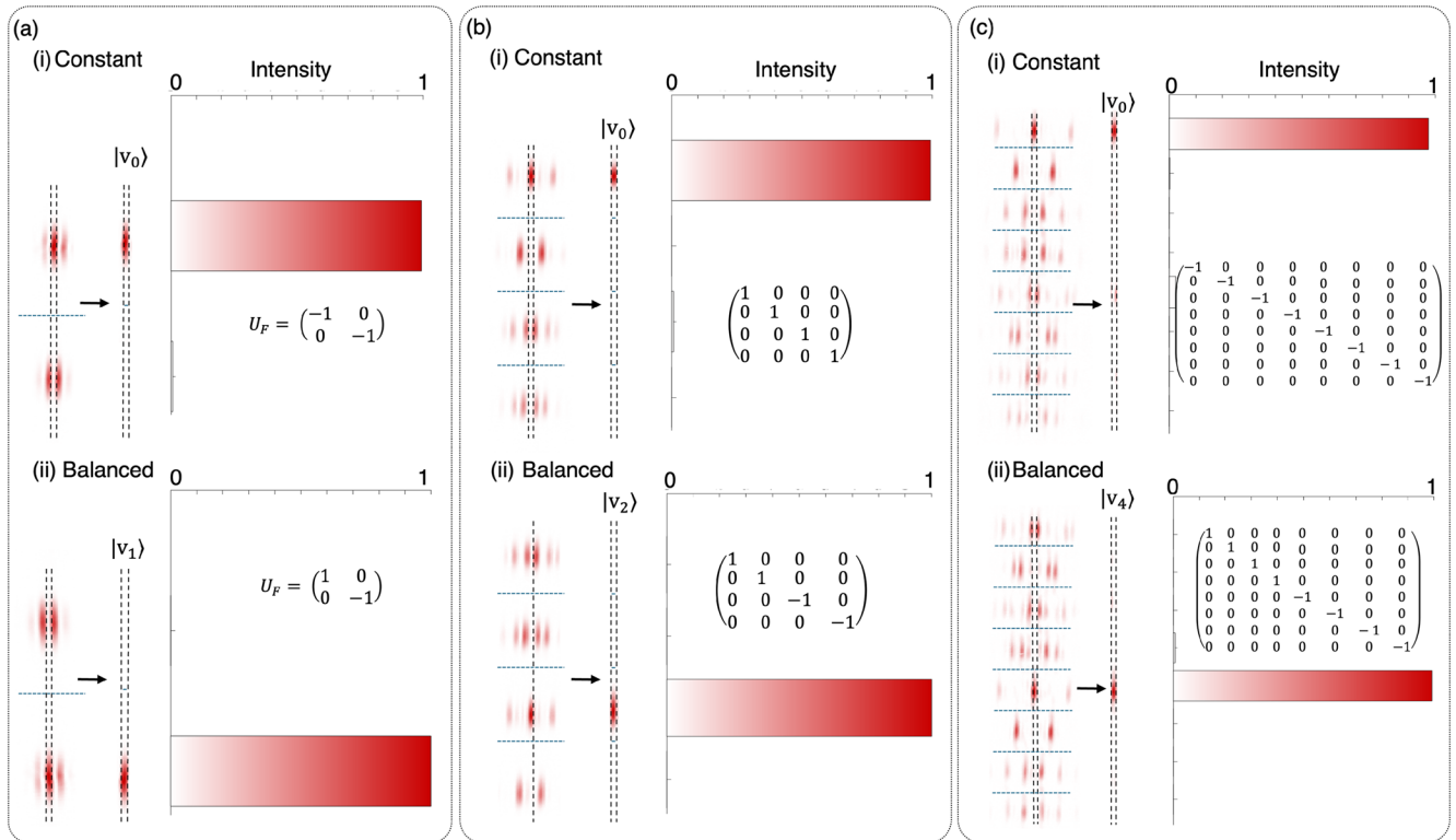
FIG. 5. Deutsch-Jozsa algorithm results: Algorithm results for the Deutsch-Jozsa algorithm implementation. Panels (a)–(c) show the intensity distributions for single-qubit, two-qubit, and three-qubit systems, respectively, with the form of the oracle diagonal matrix U_F . In each panel: (1) Unfiltered images representing the initial light distribution, and (2) filtered intensity images corresponding to the central fringe at k = 0 . Subpanels (i) correspond to the constant function, and subpanels (ii) correspond to the balanced function. The bar graphs depict the normalized intensity against the row position, allowing the determination of the function type. The presence or absence of light in the first vector element's spatial position indicates whether the function is balanced or constant.
