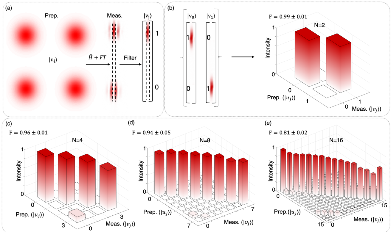
FIG. 4. Setup characterization: Intensity images collected by the CCD camera when encoding a Hadamard matrix on the second SLM and the vector built from one of the Hadamard matrix's columns on the first SLM. In (a), the extraction of the central lobe containing our solution vector from the multiplication of a 2 \times 2 Hadamard matrix with the first column is highlighted. (b) We then stack these to form a diagonal matrix consisting of the light fringes as our elements. This diagonal matrix is then used to form a crosstalk matrix, from which the fidelity of the computation is computed. (c)–(e) Extension of this process to higher dimensional matrices, up to 16 dimensions.
