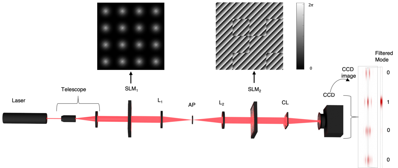
FIG. 3. A laser beam is expanded using a telescope to overfill the active area of the first Spatial Light Modulator (SLM 1). At this point, the beam is transformed to encode the input vector as repeated rows in a matrix of Gaussian beams. This output is then relayed to SLM 2 using the 4f system of lenses ( L_2 and L_1 ), where the lattice undergoes an additional phase encoding. An aperture (AP) at the focal plane of lens L_1 filters out the first-order diffraction pattern. Subsequently, the beam is propagated through a cylindrical lens (CL) and undergoes a one-dimensional Fourier transform in the x -coordinate. The final outcome is captured by a CCD camera, with the result of the multiplication found on the central fringe, which is filtered out (as shown in the inset). The filtered mode image on the CCD camera displays the result of the matrix-vector multiplication, where regions of no intensity correspond to zero elements and bright regions correspond to non-zero elements. The holograms encoded on each SLM are shown as grayscale images.
