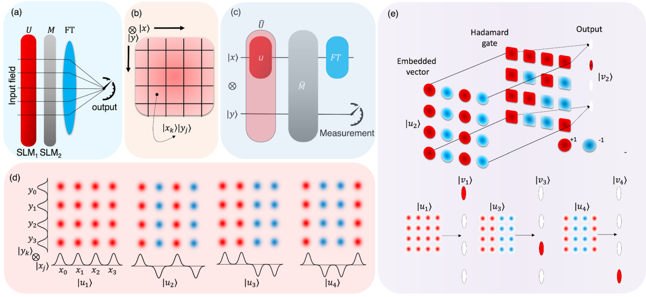
FIG. 1. (a) Analog of quantum computing using optical vector-matrix multiplication. SLM 1 encodes the lattice state via an operation, U , by copying the vector components encoded in the x -direction into the y -direction following Ref. 27. The second SLM encodes the matrix operation M . After this, a cylindrical lens focuses the field in the x -direction to produce the final matrix-vector product at the output farfield plane. (b) The encodings performed by the spatial light modulators (SLMs) operate on the tensor product states |x_k\rangle \otimes |y_j\rangle corresponding to the discrete position states that can be obtained by partitioning the Cartesian plane ( \mathbb{R}_2 ) into non-overlapping segments. (c) A quantum circuit for performing matrix multiplication using our basis states |x_k\rangle \otimes |y_j\rangle , corresponding to the coordinates of the partitions. The operations are represented as operators that act on the x -coordinate and y -coordinate degrees of freedom. (d) An example of the Hadamard basis states, |u_j\rangle , encoded onto the lattice states for N = 4 . Here, the lattice is formed from propagation invariant Gaussian modes, each encoded into the independent partitions. To demonstrate that they form a tensor product space, \mathcal{H}_N \otimes \mathcal{H}_N , we show the individual states for the x and y coordinates, where the final lattice is obtained from their tensor products. These states are orthogonal. (e) Example of one of the states being acted on by the Hadamard gate and then focused to perform the column-wise summation. The embedded state vector is modulated point-wise with an SLM encoding the Hadamard matrix/gate. This is then focused in the farfield with a cylindrical lens, where the zero order component of the pattern contains the result in the vertical direction. The outcomes are shown for other states in the Hadamard basis mapping from |u_j\rangle to the |v_j\rangle .
