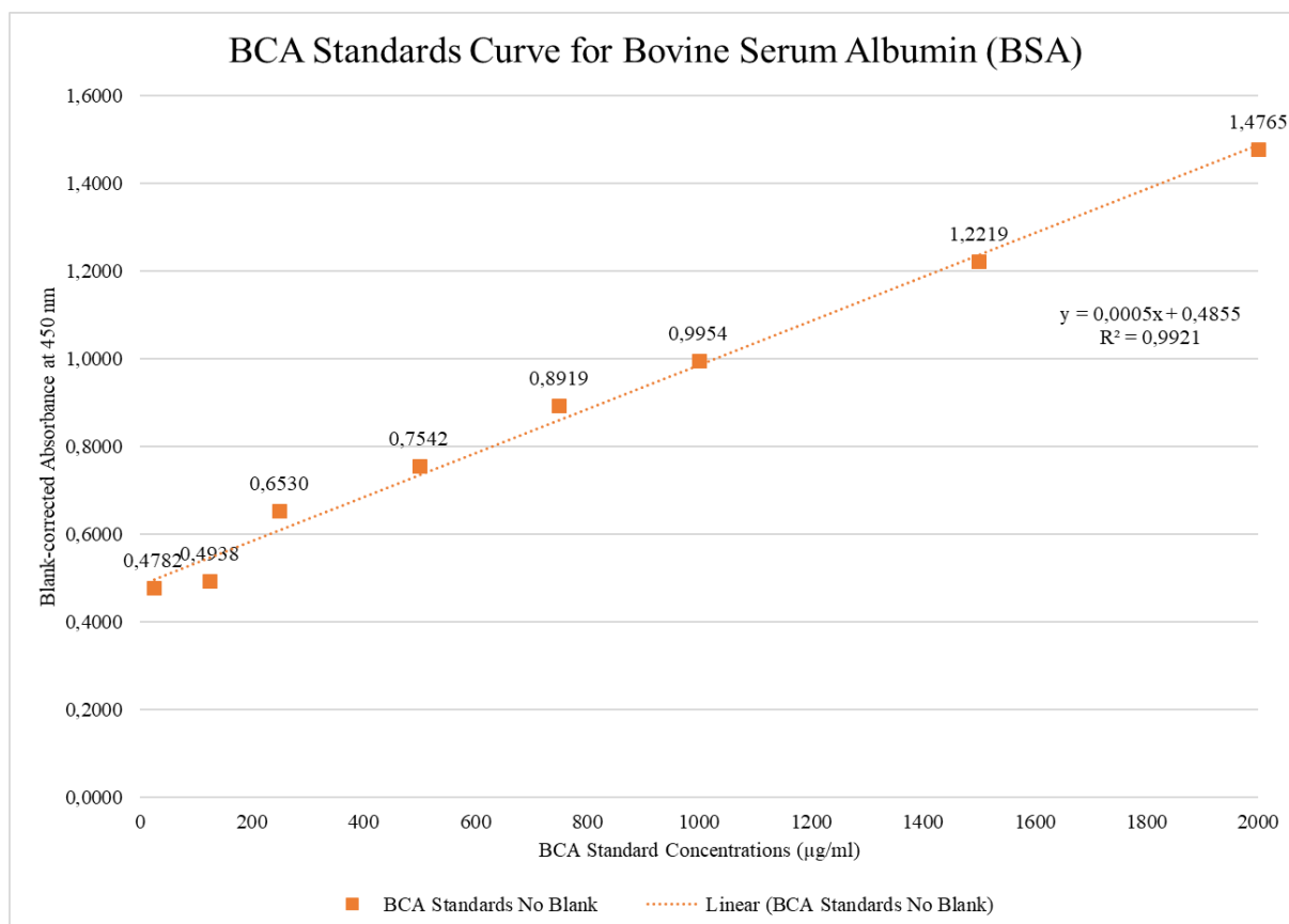
Fig 3.11: BSA standard curve for total protein concentrations ranging from 25–2000 \mu g/ml at an Absorbance of 450 nm. Orange line indicates the linear regression line ( y = 0.0005x + 0.4855 ) for BSA standards. R^2 = 0.9921
