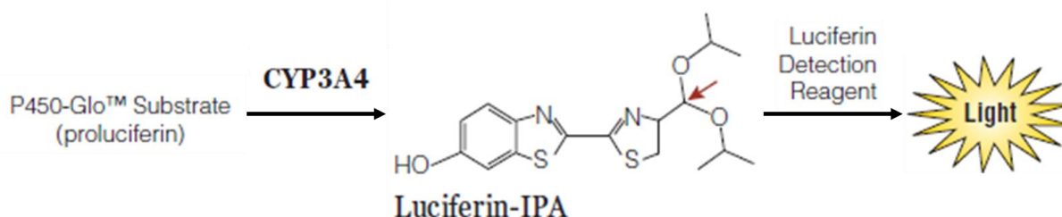
Fig 3.5: Conversion of P450-Glo™ substrate to luciferin by cytochrome P450 and detection mechanism. Image from Promega (2016).
