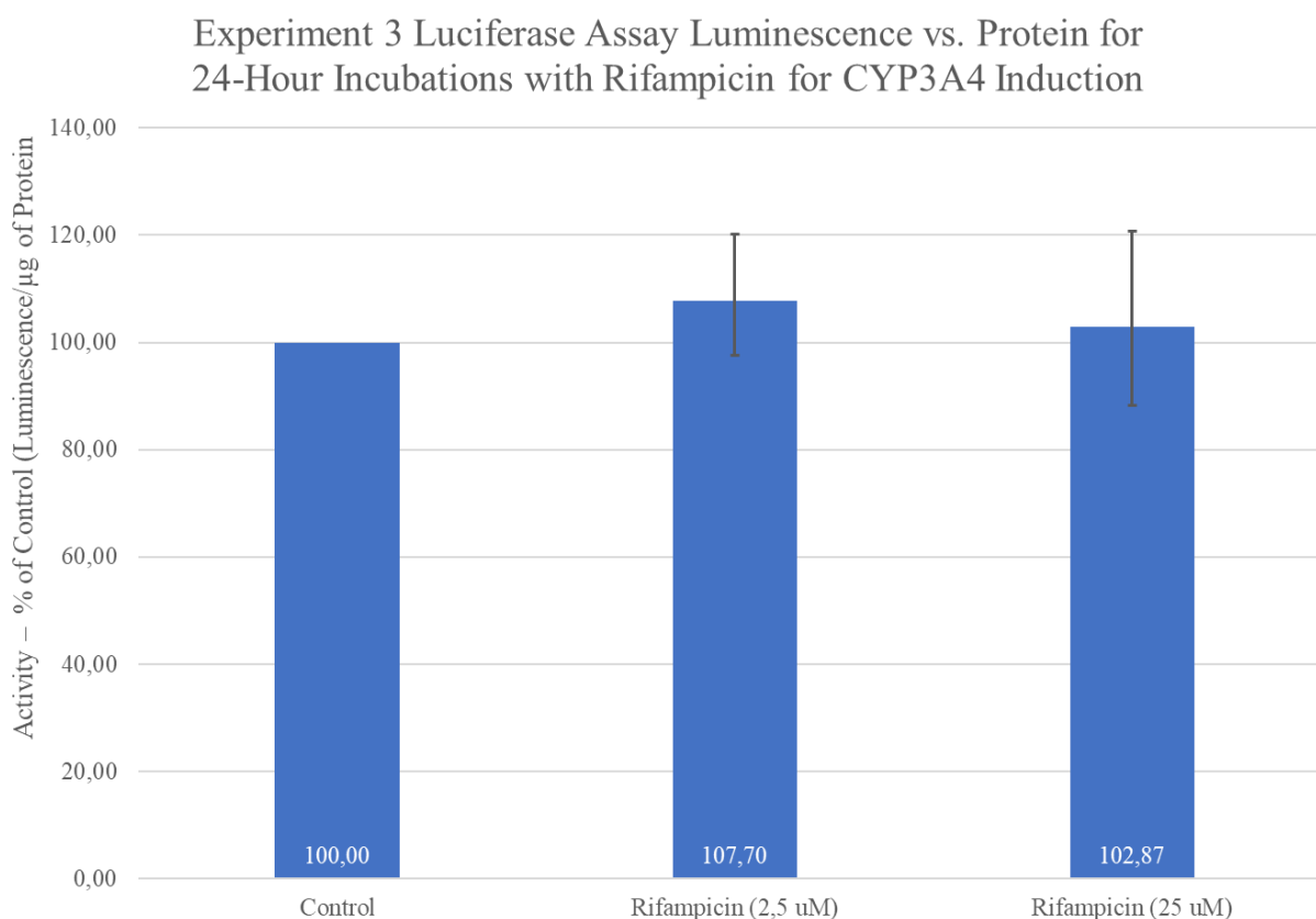
Fig 3.12: Experiment 3 luciferase assay CYP3A4 activity after 24-hour with rifampicin induction. Luminescence values were normalised to BCA total protein concentrations as a measurement of luminescence versus protein concentration. All reactions were run in duplicate. Standard error estimates are based on best fit of the average.
