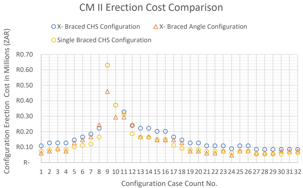
Figure 4-44 Hypothetical Configuration Erection Cost Comparison for CM II
