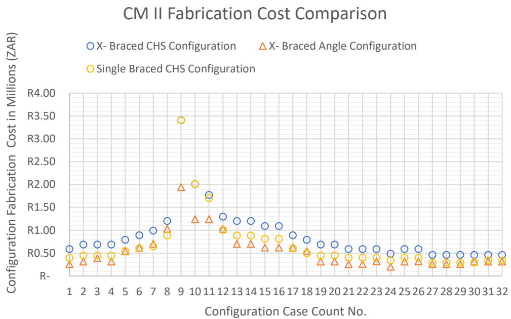
Figure 4-40 Hypothetical Configuration Fabrication Cost Comparison for CM II
