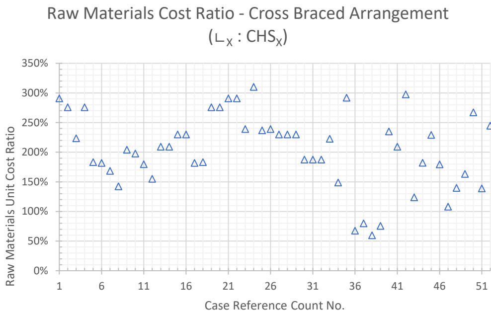
Figure 4-33 Raw Materials Cost Ratio Comparison for Cross-braced CHS and Angle Arrangements by Case Count Number
