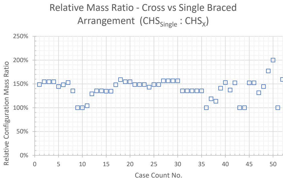
Figure 4-28 Relative Mass Ratio Comparison for Cross- and Single-braced CHS Arrangements
