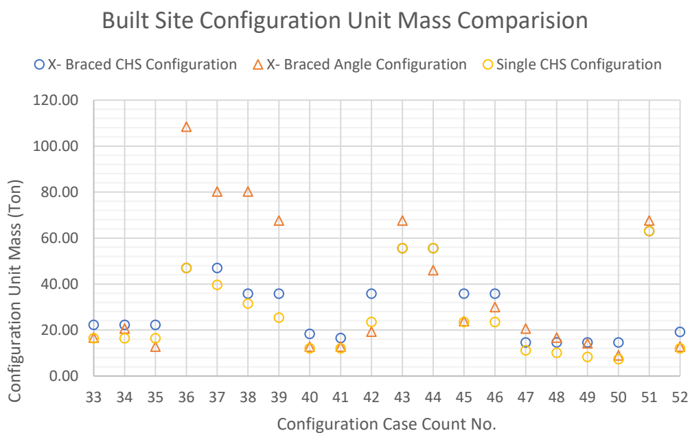
Figure 4-24 Reference and Comparative Built-site Configuration Unit Mass Analysis
