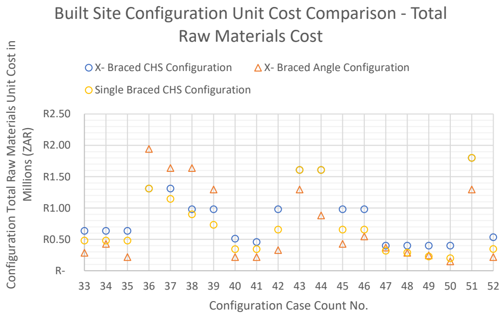
Figure 4-32 Built-site Configuration Unit Cost Comparison for Raw Materials Costs
