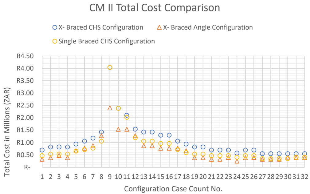
Figure 4-48 Hypothetical Configuration Total Cost Comparison for CM II
