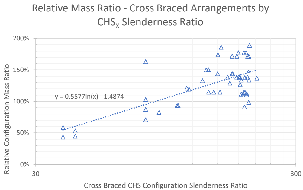
Figure 4-26 Relative Mass Ratio Comparison for Cross-braced CHS and Angle Arrangements by Cross-braced CHS Slenderness Ratio
