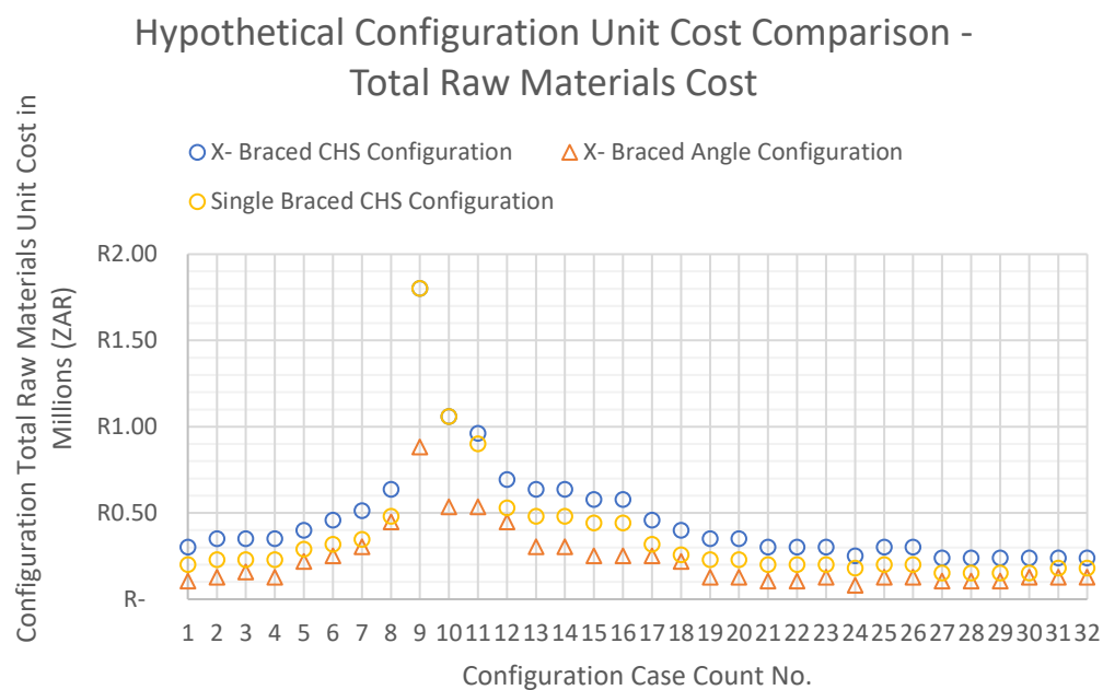
Figure 4-31 Hypothetical Configuration Unit Cost Comparison for Raw Materials Costs
