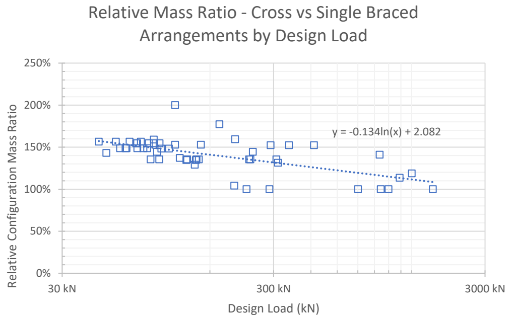
Figure 4-30 Relative Mass Ratio Comparison for Cross and Single-braced CHS Arrangements by Comparative Configuration Design Load
