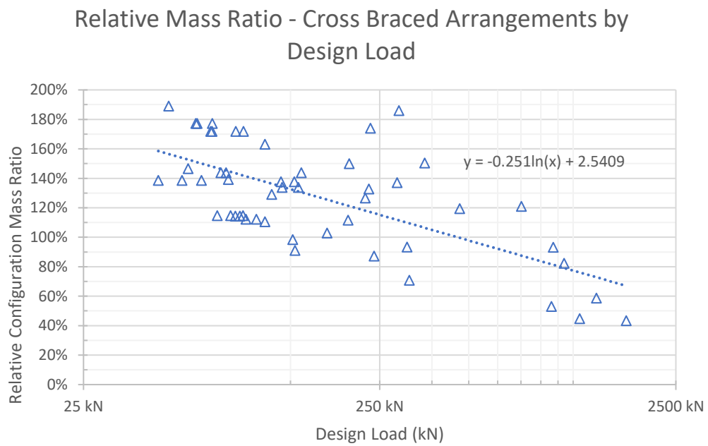
Figure 4-27 Relative Mass Ratio Comparison for Cross-braced CHS and Angle Arrangements by Comparative Configuration Design Load
