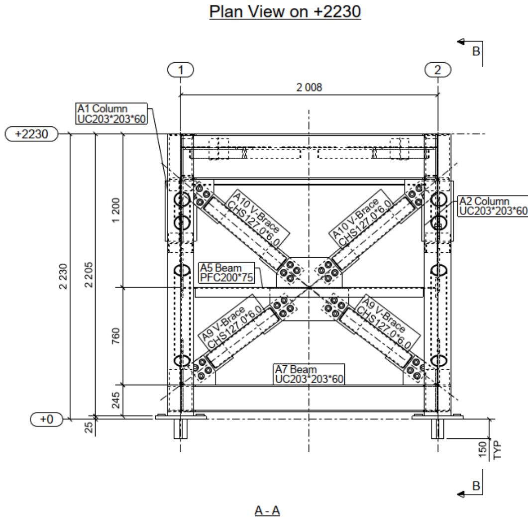
Figure 4-9 Site D Cross-braced CHS Member General Arrangement Elevation (Site D-C1)
