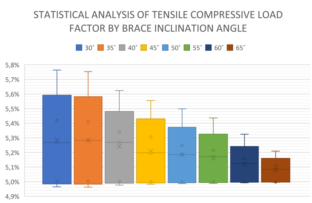
Figure 4-2 Box and Whisker Diagram for Compressive Load Share Factor Statistical Analysis
