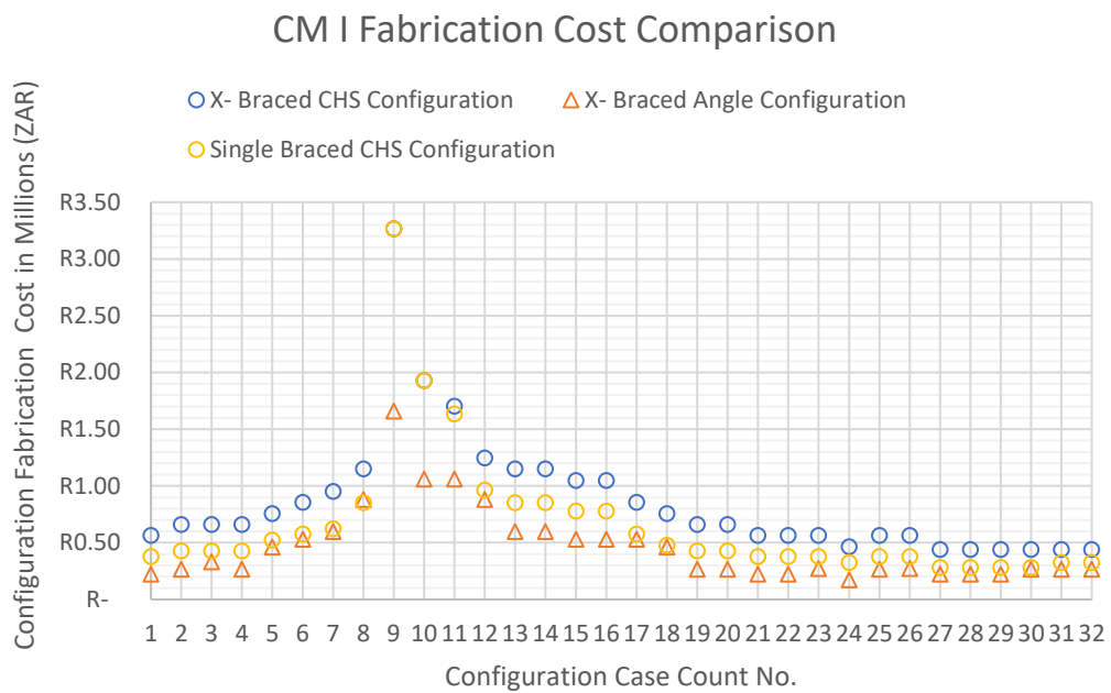
Figure 4-39 Hypothetical Configuration Fabrication Cost Comparison for CM I
