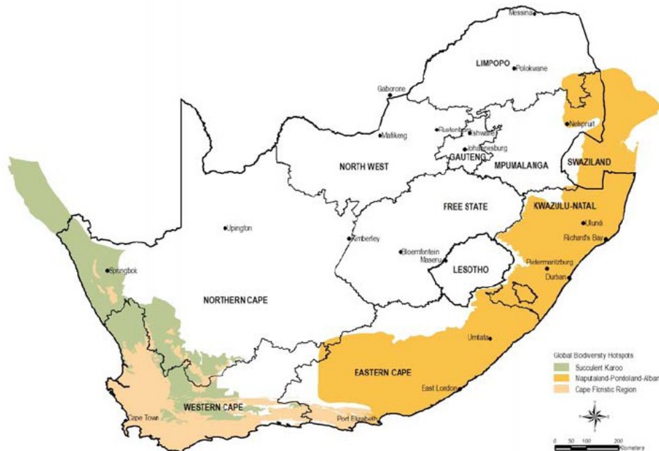
Map 2. Biomes and Biodiversity hotspots of South Africa (Source: Low and Rebelo, 1996; Mittermeier et al. , 2005; King et al. , 2005)
