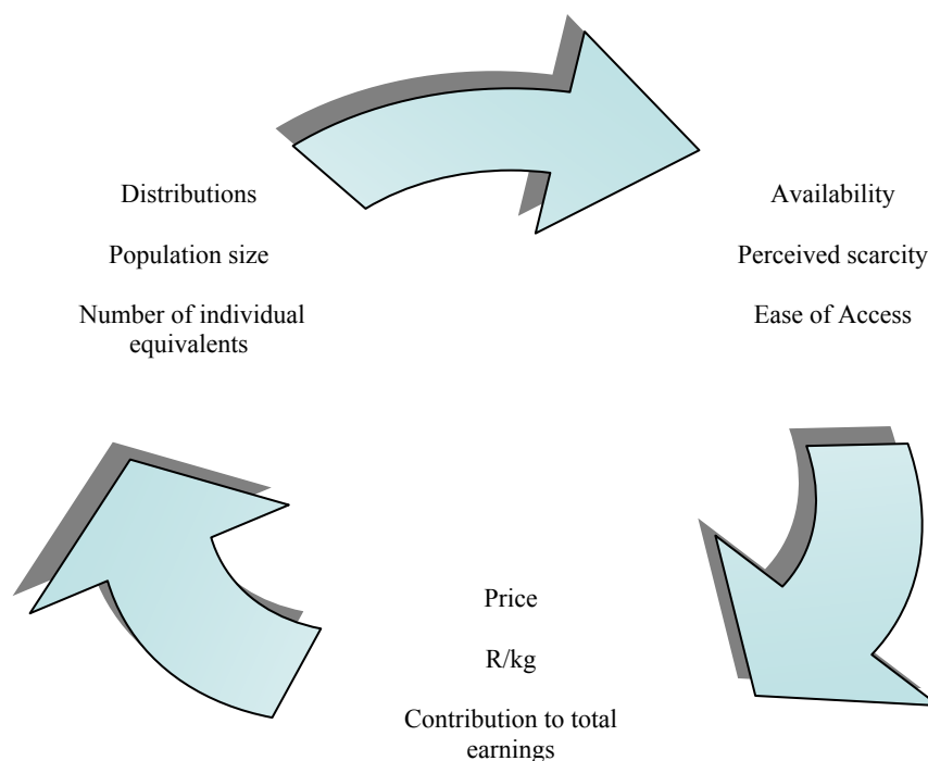
Figure 2: Conceptual diagram of the inter-relationships between population, trade and economic factors.
