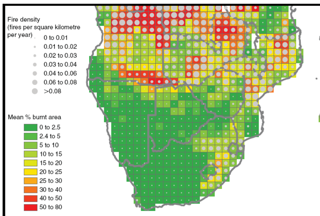
Figure 3: Maximum density of fires per square kilometre plotted over the mean % burnt area for southern Africa (from Archibald et al. , 2010)
