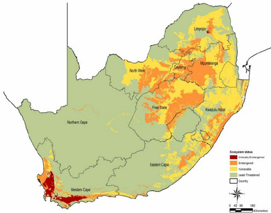
Map 1. Ecosystem status of terrestrial ecosystems (Source: Driver et al. , 2005; King et al. , 2005)
