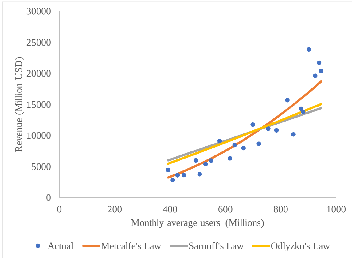
Figure 2. E-commerce: Actual vs Value curves
