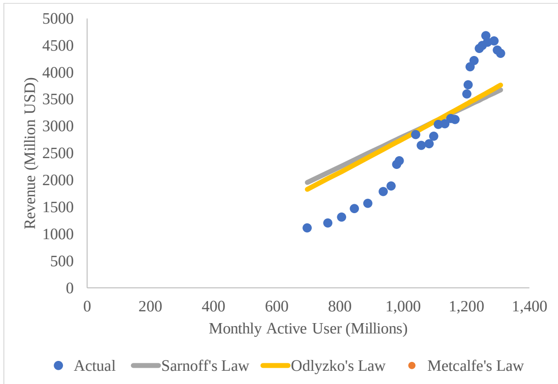
Figure 1. Social Networks: Actual vs Value curves
