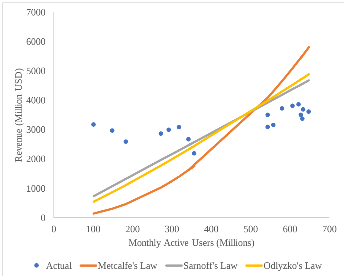
Figure 3. Search engine: Actual vs Value curves
