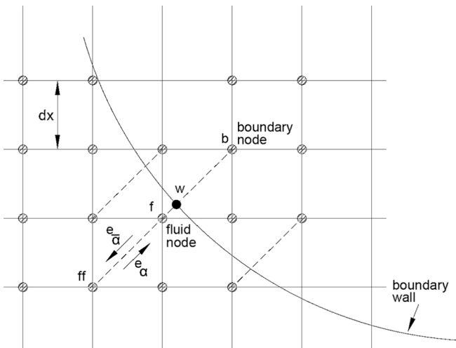
Fig. 3. Plan view of the boundary of the curved wall in two dimensions in LBM.
