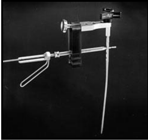
Figure 2: Ulna rod and locking guide system
