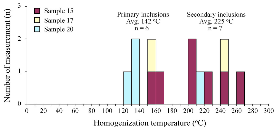
Fig. 8. Homogenization temperature ( T_h ) from primary (average 142 °C) and secondary (average 225 °C) fluid inclusions in calcite.
