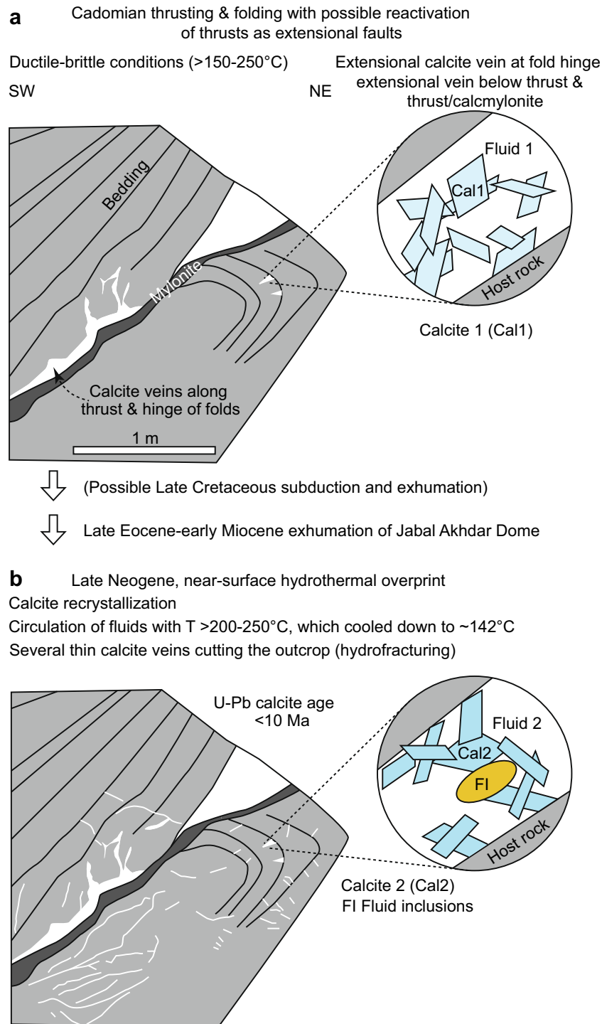
Fig. 9. Summary of calcite vein development in Wadi Bani Awf. a) Cadomian thrusting and associated folding produced calc-mylonites and extensional veins in the fold hinges. Precipitation of Calcite 1. Ductile deformation occurred at temperatures of >150\text{--}250^\circ\text{C} . b) After possible Late Cretaceous subduction and exhumation as well as late Eocene-early Miocene exhumation, the rocks were overprinted by a Late Cenozoic hydrothermal event. Initial metamorphic fluids were non-oxidizing and equilibrated at temperatures of >200\text{--}250^\circ\text{C} (based on Eu-anomalies). Fluids cooled down to \sim 142^\circ\text{C} (primary fluid inclusions in Calcite 2) and precipitated calcite at <10 \text{ Ma} . Local and minor late-stage overprint during the same event produced secondary fluid inclusion at \sim 225^\circ\text{C} . Calcite microstructures (twins, minor dynamic recrystallization) confirm that Calcite 2 was deformed at temperatures between <170 and 250^\circ\text{C} . Carbon and oxygen isotope signatures of Calcite 2 are adopted from the host rock and deep metamorphic fluids, respectively. Calcite 2 preserves the geochemical trace element fingerprint of Cadomian(?) Calcite 1.
