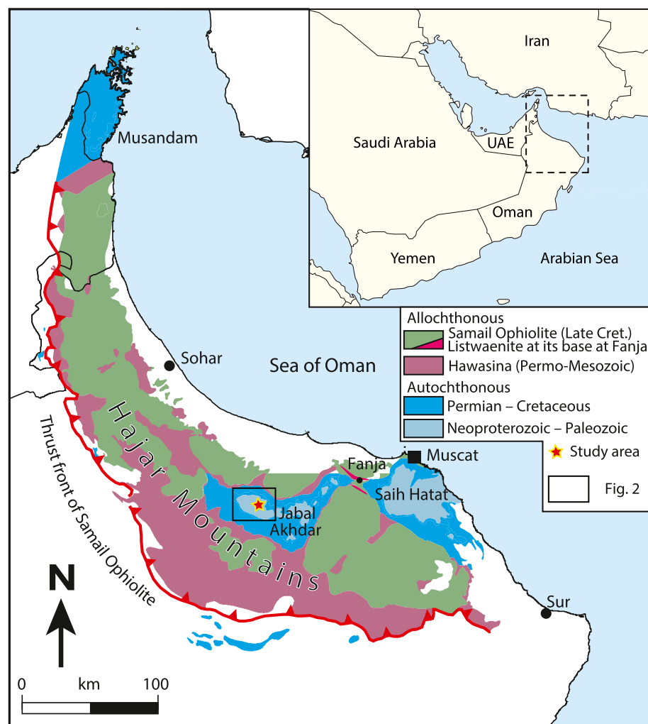
Fig. 1. Geological overview map of the Hajar Mountains and the study area located at the center of the JAD, modified after Forbes et al. (2010) and Callegari et al. (2022).
