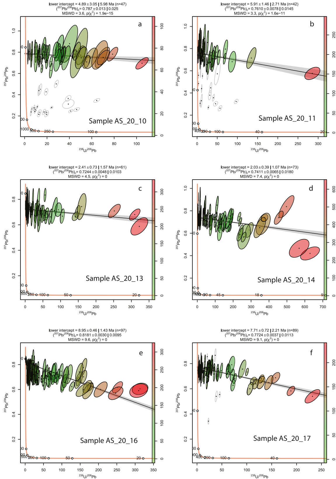
Fig. 6. Tera-Wasserburg diagrams showing U–Pb age data of six deformation-related carbonate samples; in all samples, calcite was dated; graphic representation and age calculation utilized IsoplotR (Vermeesch, 2018). Error ellipses represent two standard errors of mean; gray areas around discordia represent 2σ uncertainty of linear regression. Analytical precision (age, initial ^{207}\text{Pb}/^{206}\text{Pb} ) is indicated as analytical uncertainty (first value), “studentized 100(1–α)% confidence interval for t using the appropriate number of degrees of freedom” (second value) and “approximate 100(1–α)% confidence interval for t with over-dispersion, calculated as z=y/\text{MSWD} ” (value 3). MSWD = mean squared weighted deviations; n = numbers of spot analyses. The U–Pb data ellipses are color-coded according to their ^{238}\text{U}/^{206}\text{Pb} value, displayed in the individual color scales at the right margin of the diagrams.
