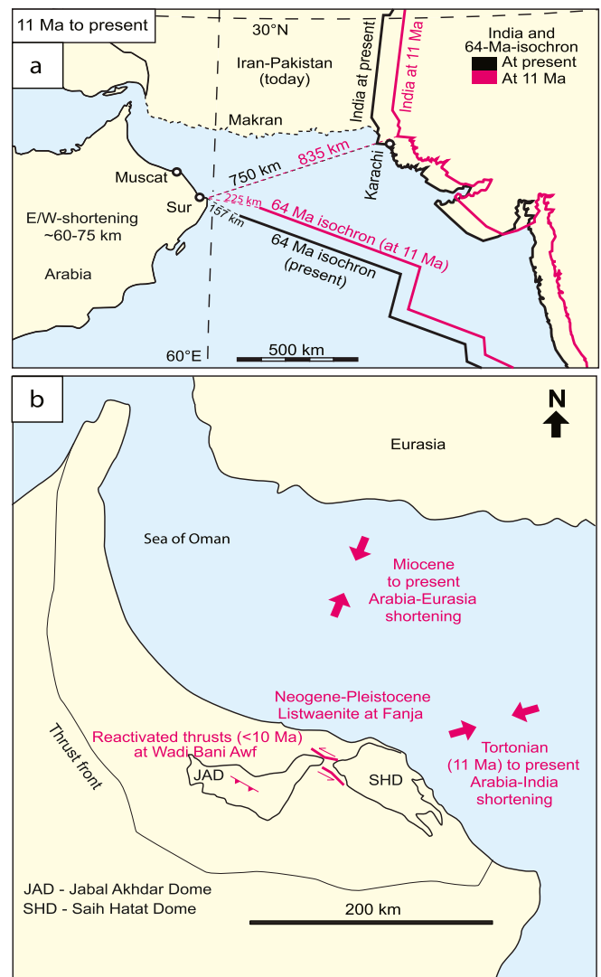
Fig. 10. Paleogeographic reconstruction of the greater study area from 11 Ma until present, modified from Scharf et al. (2022b). a) Arabia/India-shortening amounts to ~60–75 km from 11 Ma until present. b) ENE/WSW Arabia/India and/or NE/SW Arabia/Eurasia-shortening may account for reactivation of NW-striking thrusts in Wadi Bani Awf and NW-striking listwaenite bodies, associated with sinistral faults near Fanja, located between the JAD and SHD.
