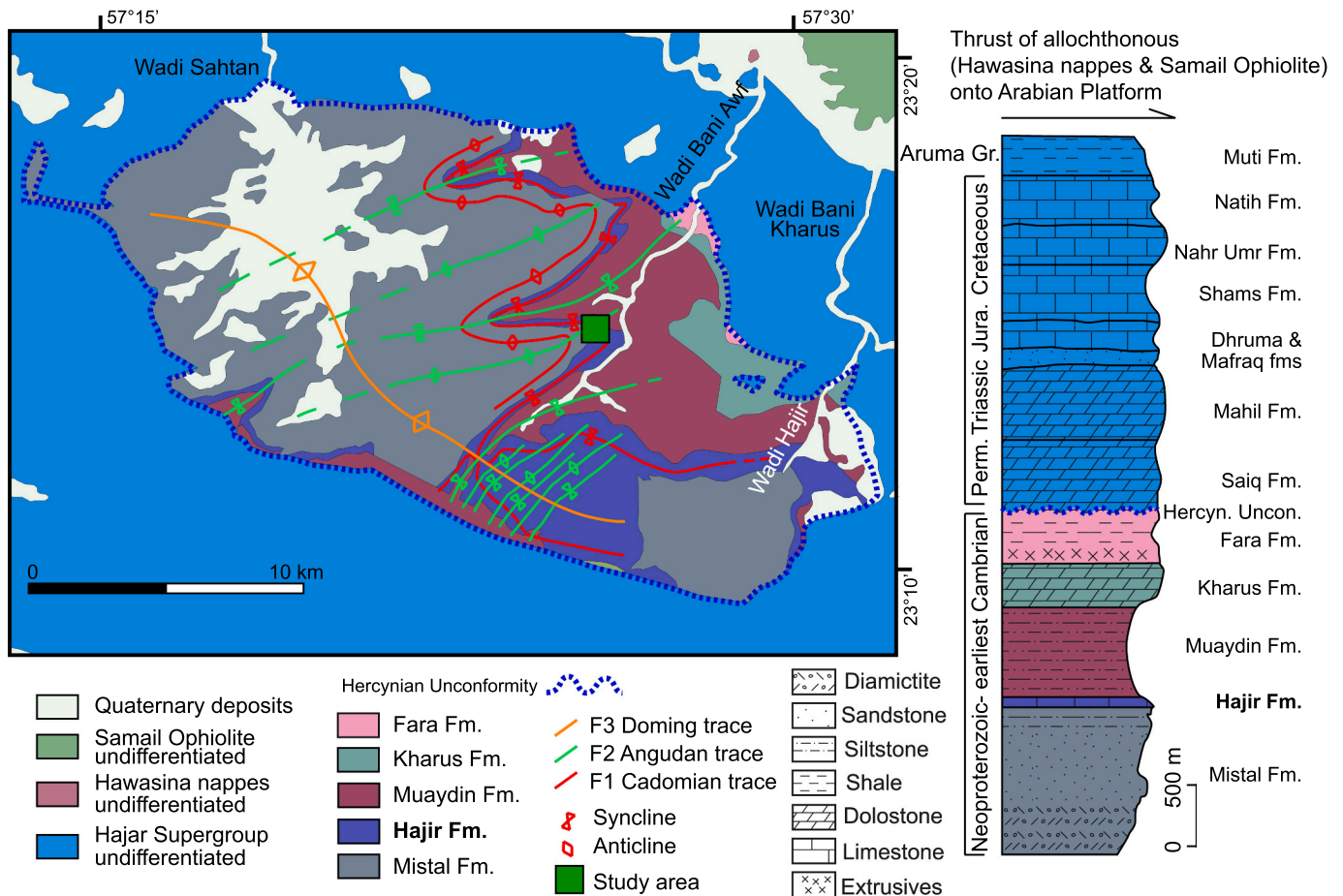
Fig. 2. Geological map and lithostratigraphic column of the western-central JAD, modified after Scharf et al. (2021a) . The studied outcrop lies within the hinge zone of a large Angudan anticline of Wadi Bani Awf, in the core area of the JAD, and consists of limestone of the Hajir Formation.
