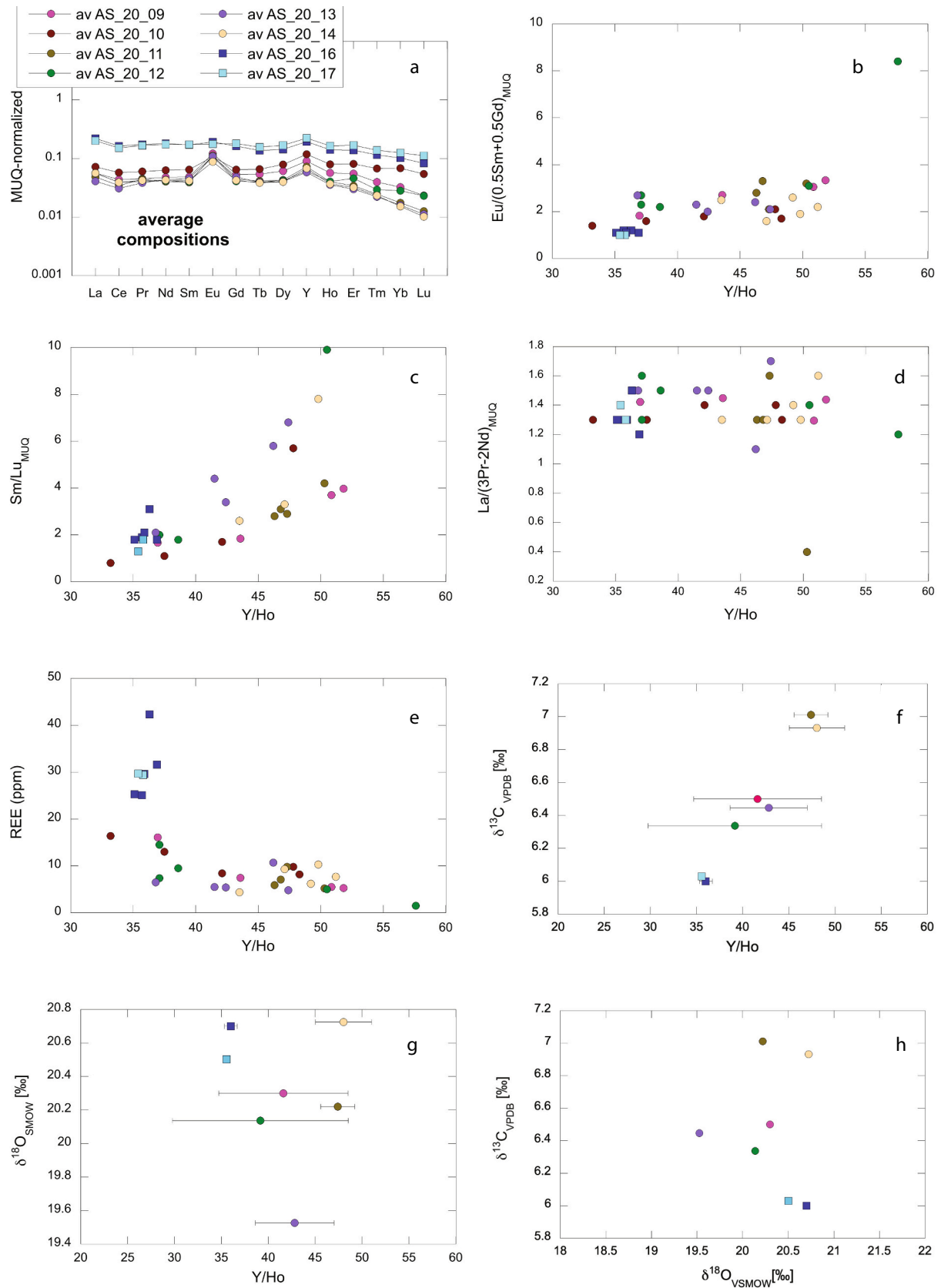
Fig. 7. a) Summary on REE patterns (overall average for each sample). Individual REE patterns are provided in Fig. S1. b-h) Diagrams showing trace element and isotopic compositions of carbonates; error bars in f and g are 1 SD of the mean. Averages were calculated using all analyses for each sample.
