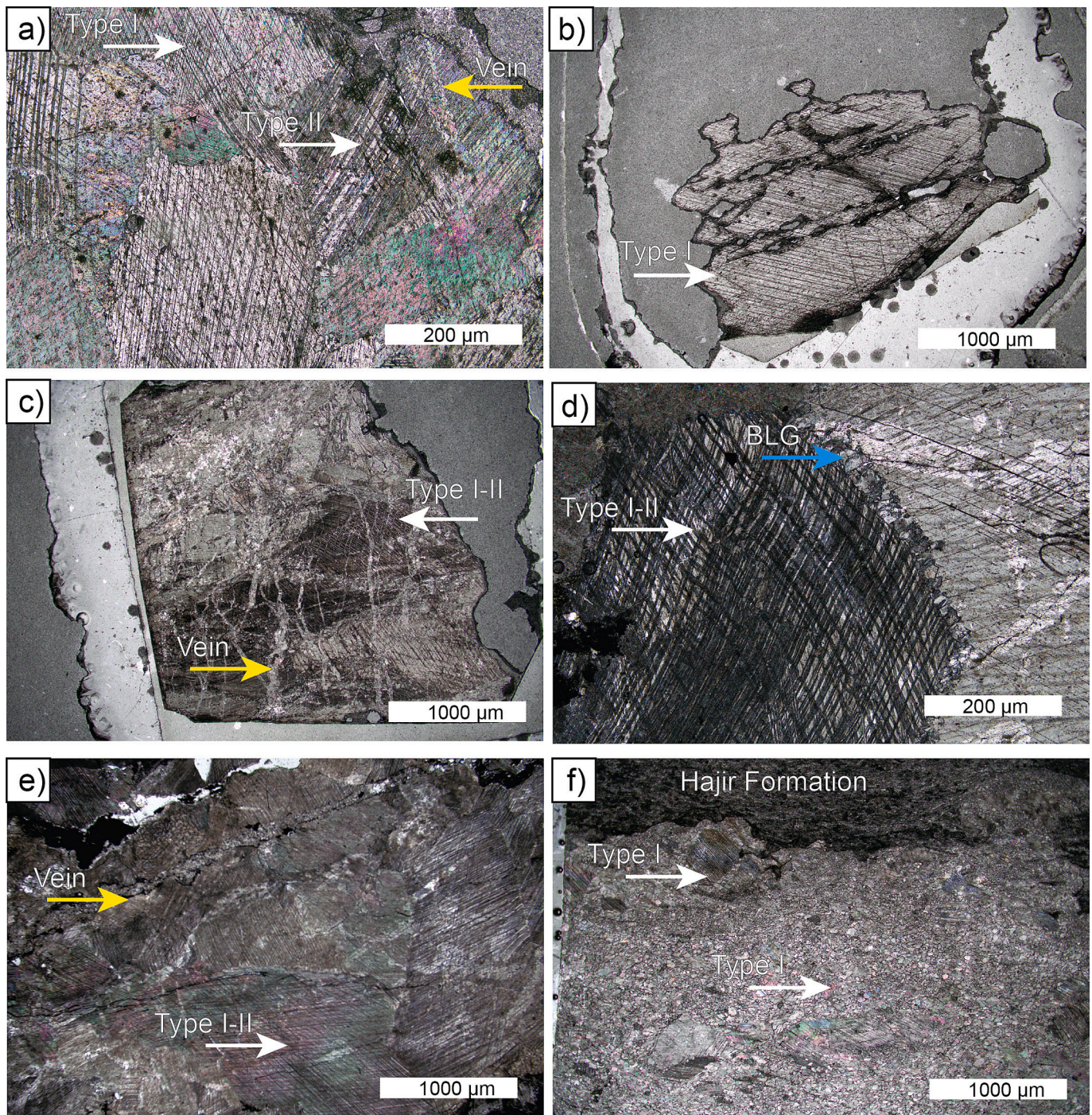
Fig. 5. Photomicrographs of vein gouge material as seen under cross-polarized light (XPL). (a) Sample AS-20-14 taken from a vein in extended part of a fold hinge displays large, blocky calcite crystals with Type I to Type II calcite twinning (arrows). Occasionally, small calcite-filled veins cut the large crystals (yellow arrow). (b) Sample AS-20-16, taken from extensional vein above a thrust, displays large calcite crystals with Type-I calcite twinning (arrow). (c) Sample AS-20-20 taken from a thrust. Large blocky calcite crystals with Type I to Type II calcite twinning (arrow) are cut by a network of thin calcite-filled veins (yellow arrow). (d) Sample JA-24-3 taken from a thrust. Detailed photograph of folded Type I to Type II calcite twins (arrow). Crystal boundary displays bulging recrystallization (BLG; blue arrow). (e) Sample JA-24-3 consists of large, blocky calcite crystals with Type I to Type II calcite twinning (arrow). Thin veinlet (yellow arrow) consists of an opaque iron oxide matrix. Locally, crystals are fractured with the fragmented calcite crystals being cemented by the opaque material. (f) Sample JA-24-4 is taken from a thrust. Top, dark part of the image displays the host rock (Hajir Formation). Within the vein, large calcite crystals with Type I twins (upper arrow) are surrounded by a matrix of small calcite crystals (lower arrow), which also display Type I calcite twins. (For interpretation of the references to color in this figure legend, the reader is referred to the web version of this article.)
