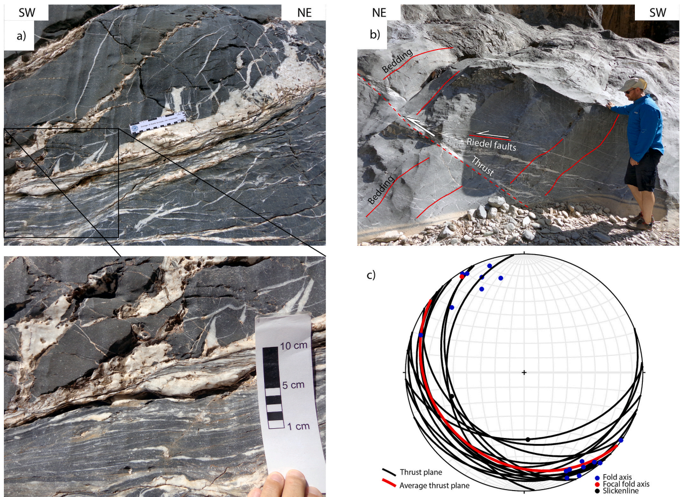
Fig. 4. a) Calc-mylonite of the thrust from Fig. 3 displaying ductile deformation of limestone. b) Thrust with Riedel faults indicating shear sense. c) Stereonet (lower hemisphere) compiling the structural measurements of the study area (utilizing Steronet v. 11 by Rick Allmendinger).
