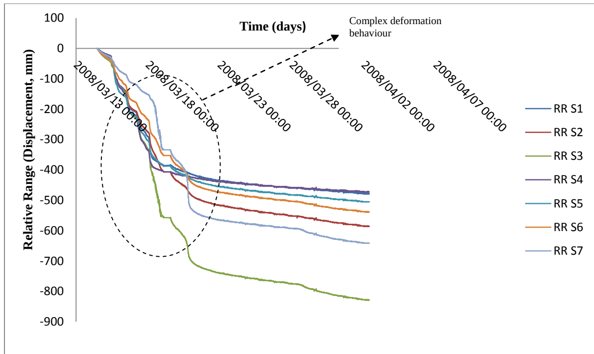
Figure 5.10: Relative range (Displacement, mm) of sections 1-7 of ramp 0 slope.
