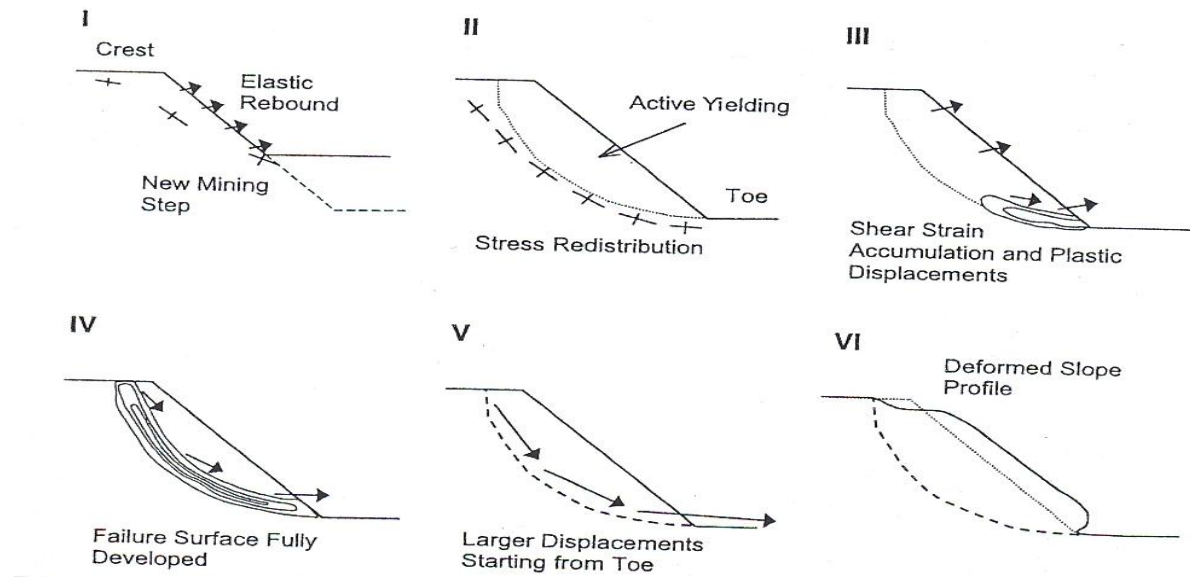
Figure 2.8: Failure stages for circular (rock mass) shear failure slope (After Sjöberg, 2000).
