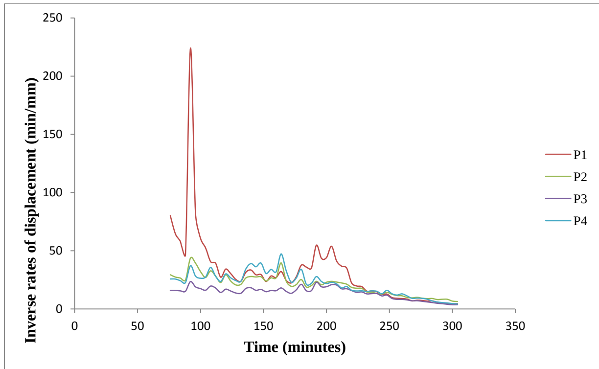
Figure 6.10: Inverse rates of displacement at 20 data interval (80 minutes).
