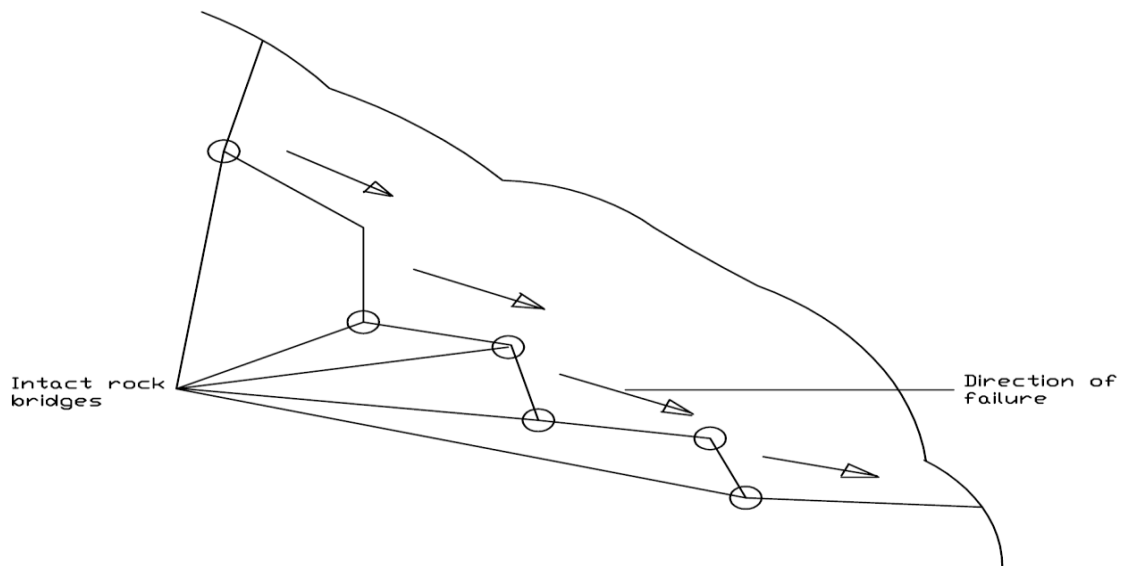
Figure 2.17: Complex failure mechanisms with multiple step-path failure (After Eberhardt, et al. 2004a and Stead, et al. 2006)
