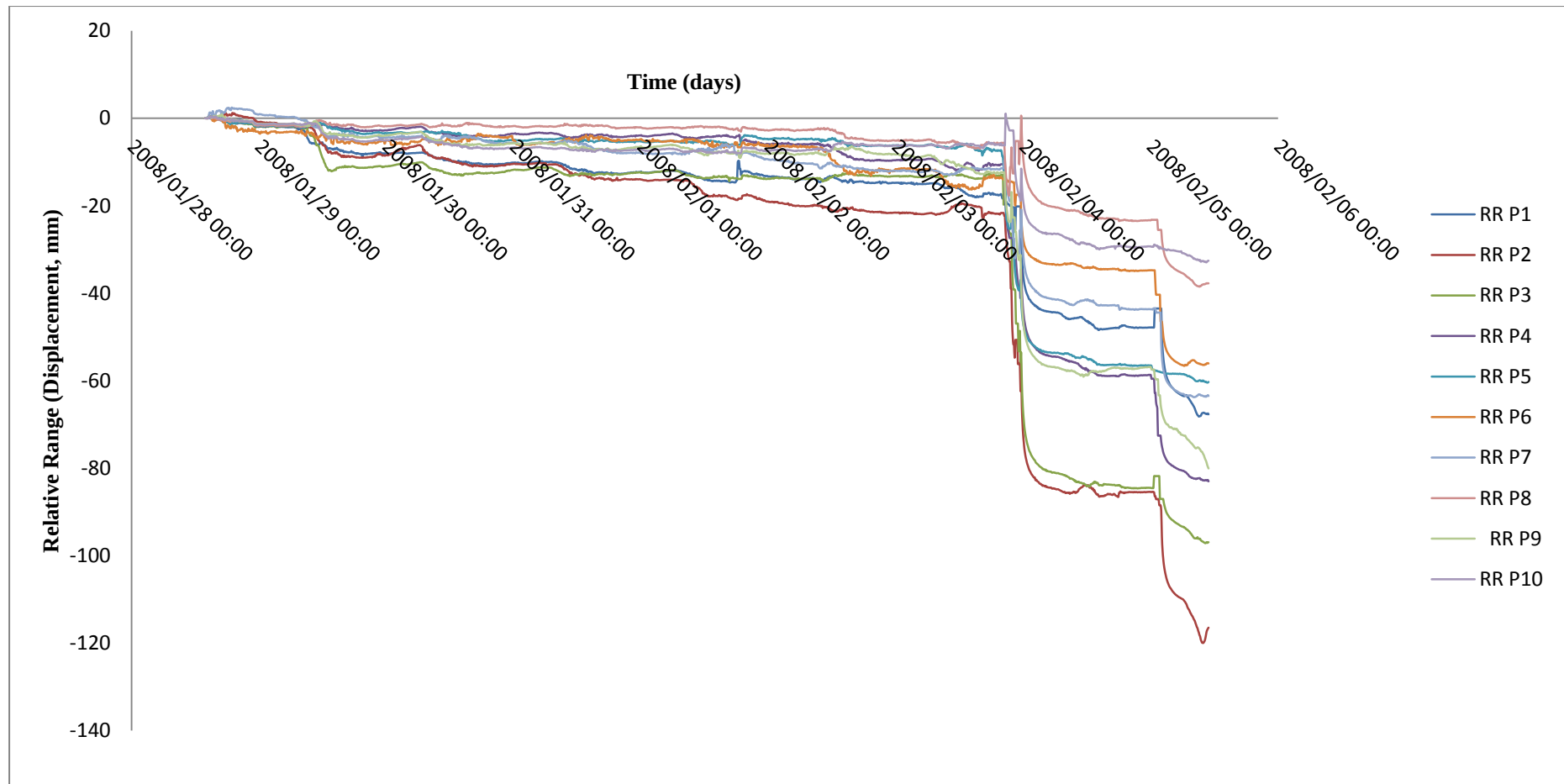
Figure 5.22: Relative range (Displacement, mm) of 10 points in ramp 11 failure sections.
