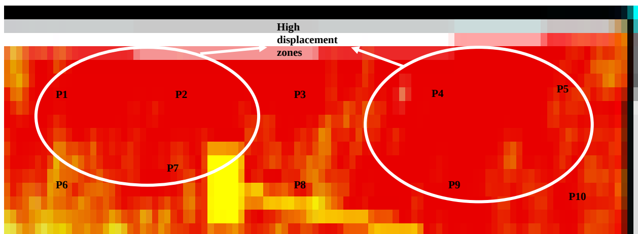
Figure 5.21: Failure section of ramp 11 slope failure showing the locations of ten selected points.
