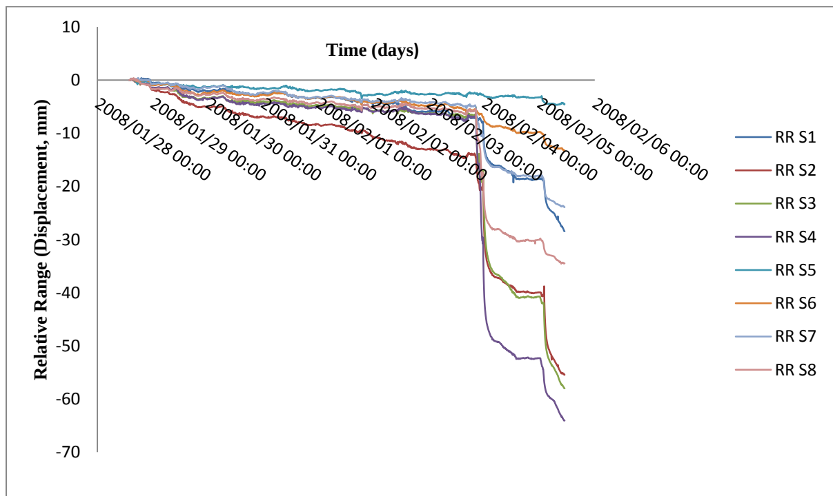
Figure 5.19: Relative range (Displacement, mm) of sections 1-8 of ramp 11 slope.
