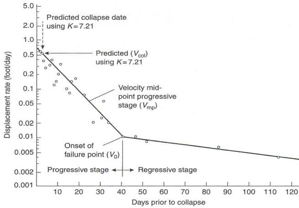
Figure 6.1: Displacement rate curve and failure collapse prediction (After Zavodni and Broadbent, 1980).
