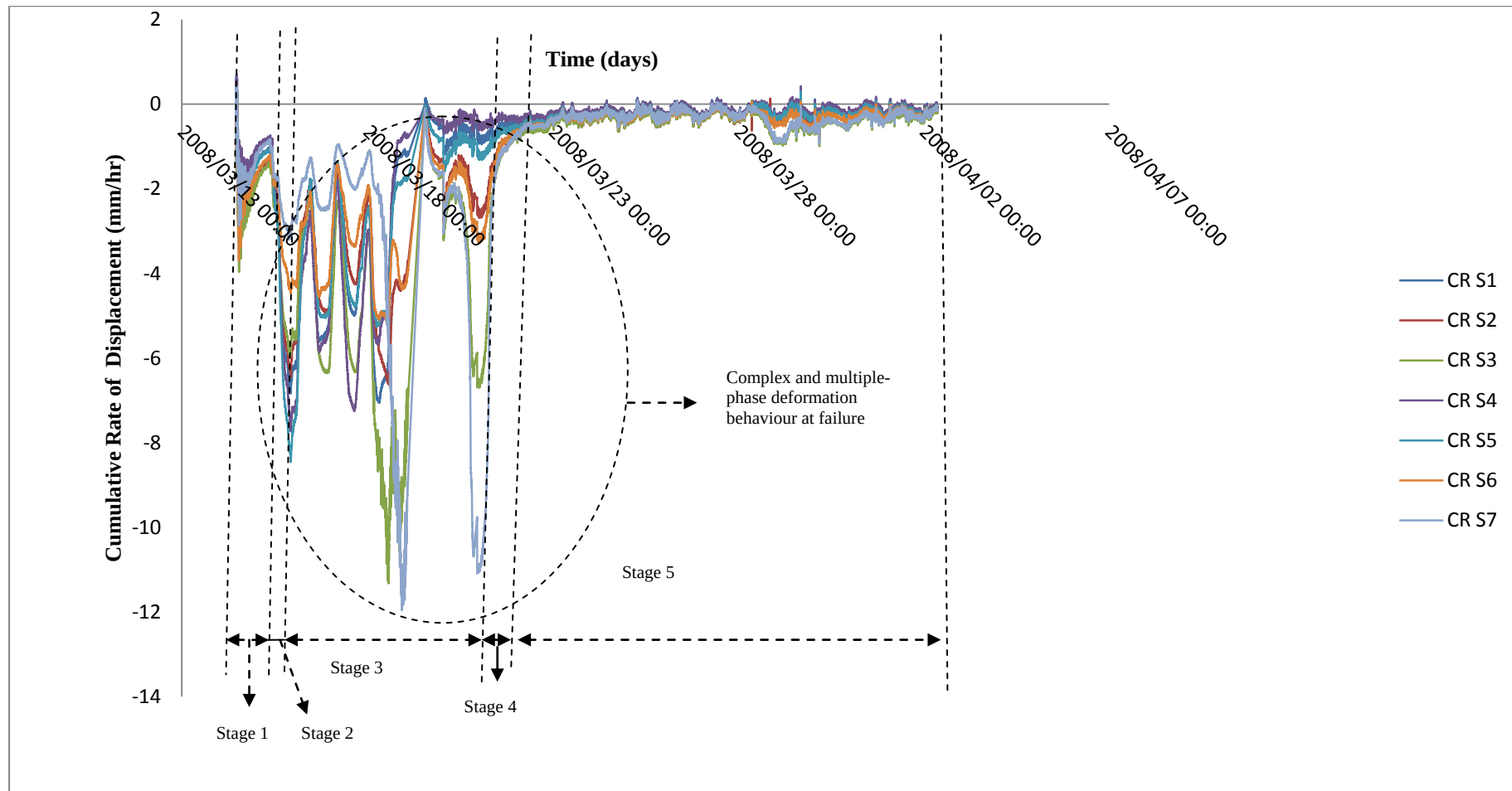
Figure 5.11: Cumulative rate of displacement (mm/hr) of sections 1-7 of ramp 0 slope.
