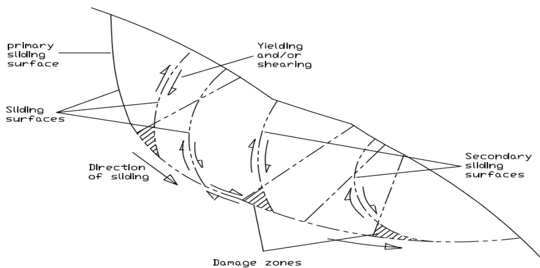
Figure 2.18: Complex failure mechanisms with deep-seated multi-block failure. Modified from Eberhardt, et al (2004a) and Stead, et al (2006)
