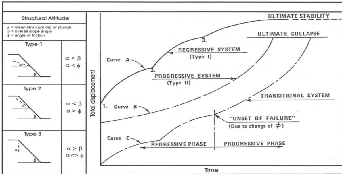
Figure 2.20: Typical regressive/progressive stage displacement curves (Broadbent and Zavodni, 1982).
