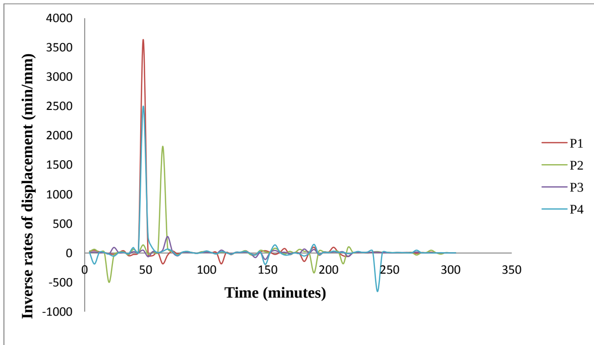
Figure 6.5: Inverse rates of displacement at 1 data interval (4 minutes).
