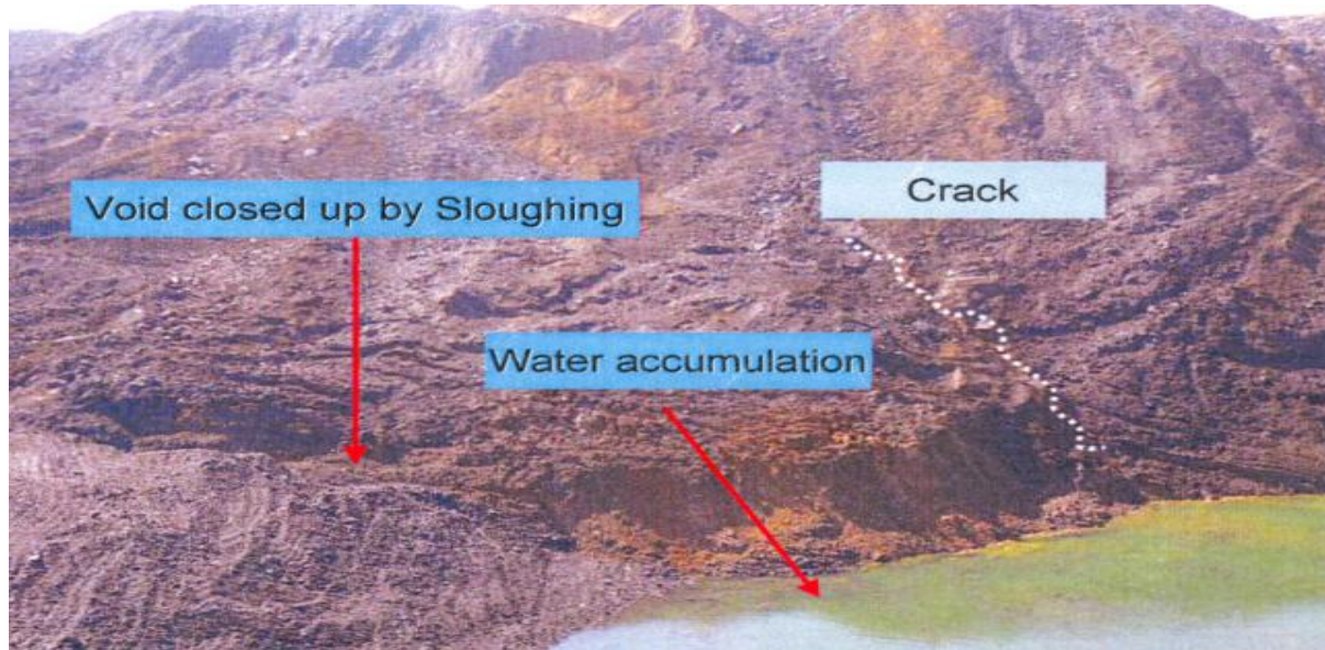
Figure 4.13: Unstable low-wall before failure (New Vaal Colliery, 2009b).
