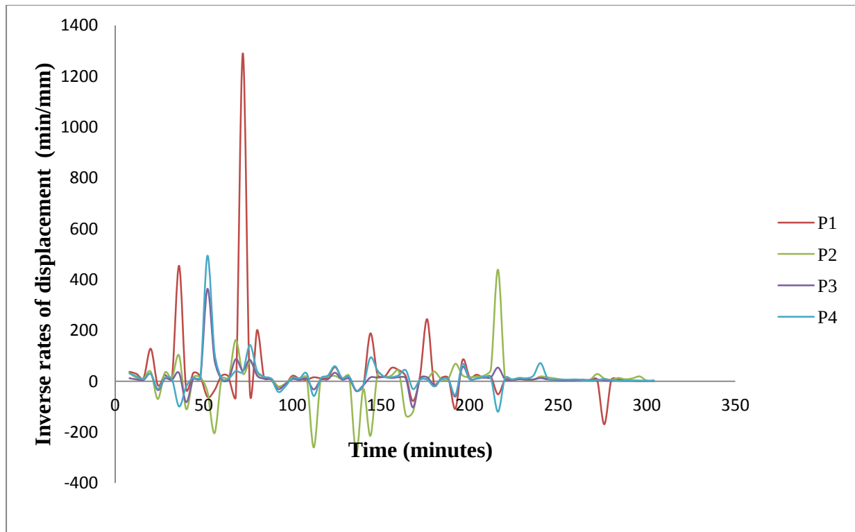
Figure 6.6: Inverse rates of displacement at 2 data interval (8 minutes).
