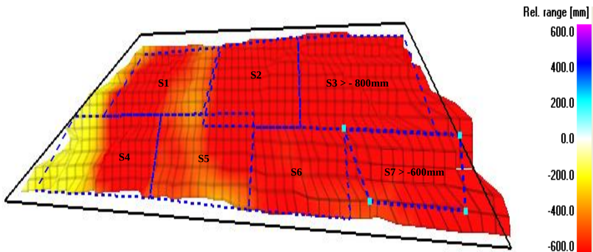
Figure 5.9: The scanned region of ramp 0 slope.
