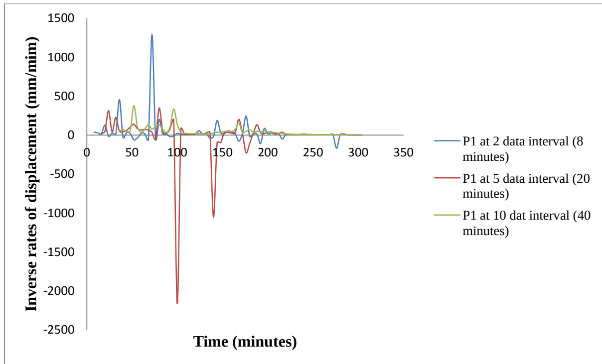
Figure 6. 12: Inverse rates of displacement at 2, 5 and 10 data interval (8, 20 and 40 minutes).
