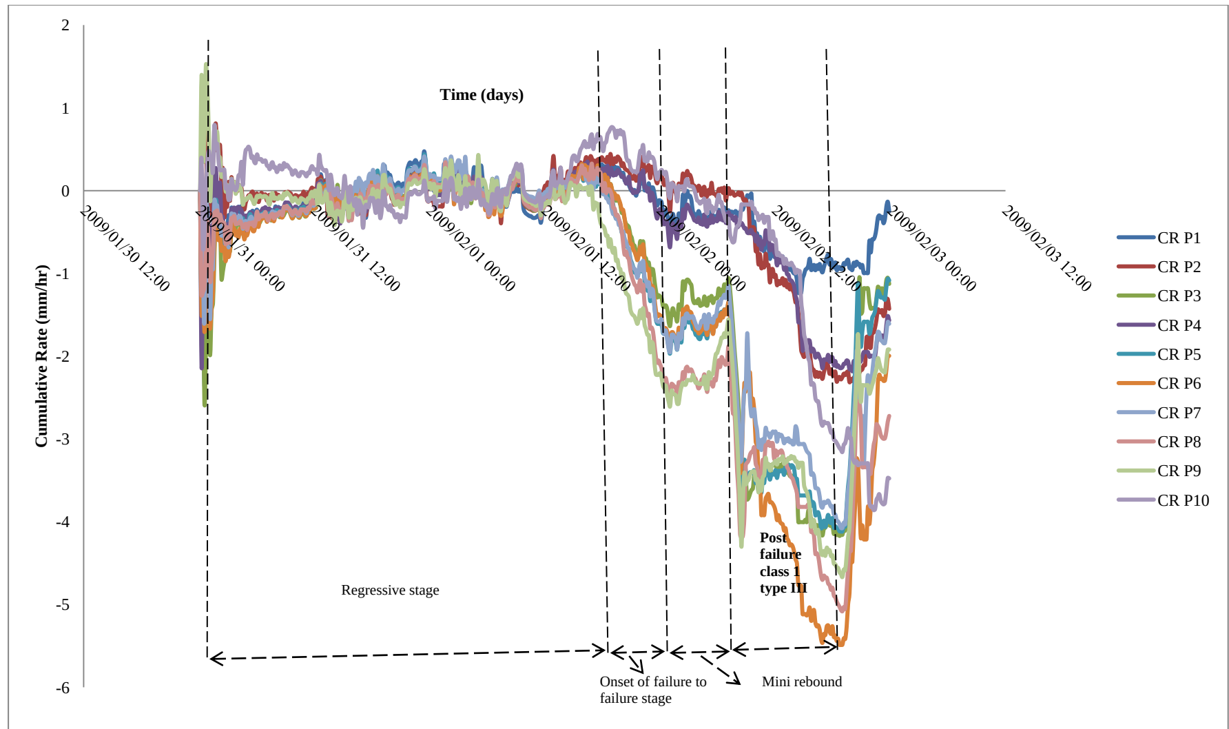
Figure 5.35: Post-failure class 1 type III displacement behaviour.
