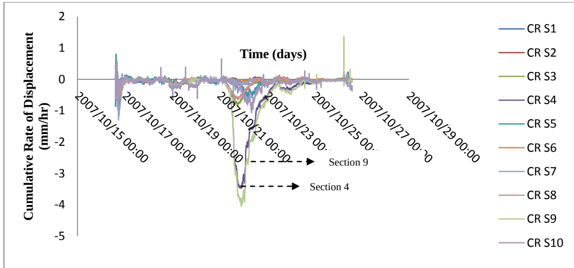
Figure 5.14: Cumulative rate of displacement (mm/hr) of sections 1-10 of ramp 5 slope.
