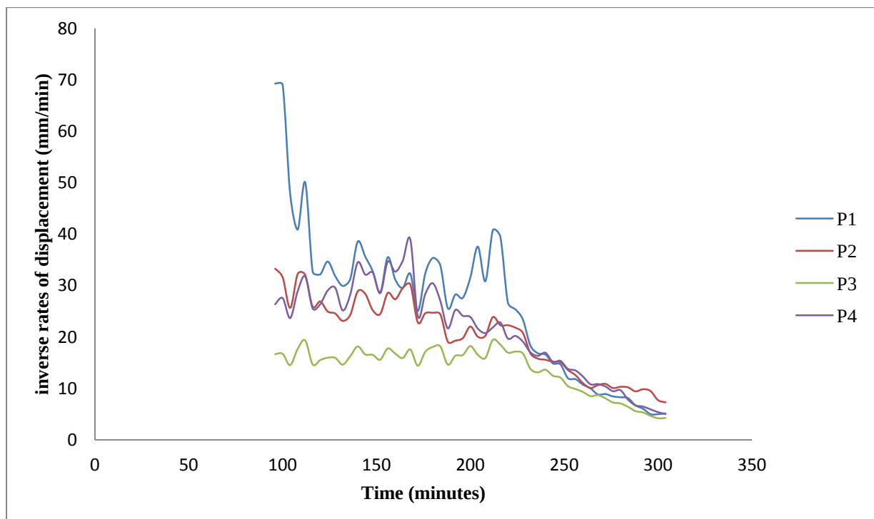
Figure 6.11: Inverse rates of displacement at 25 data interval (100 minutes).
