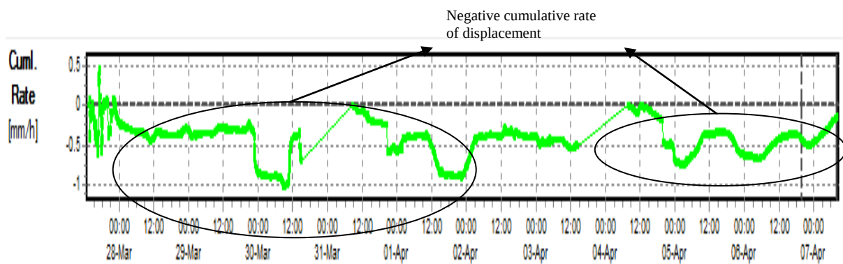
Figure 5. 2: Negative regressive behaviour of stable slope at Landau open-cast mine (Type I).
