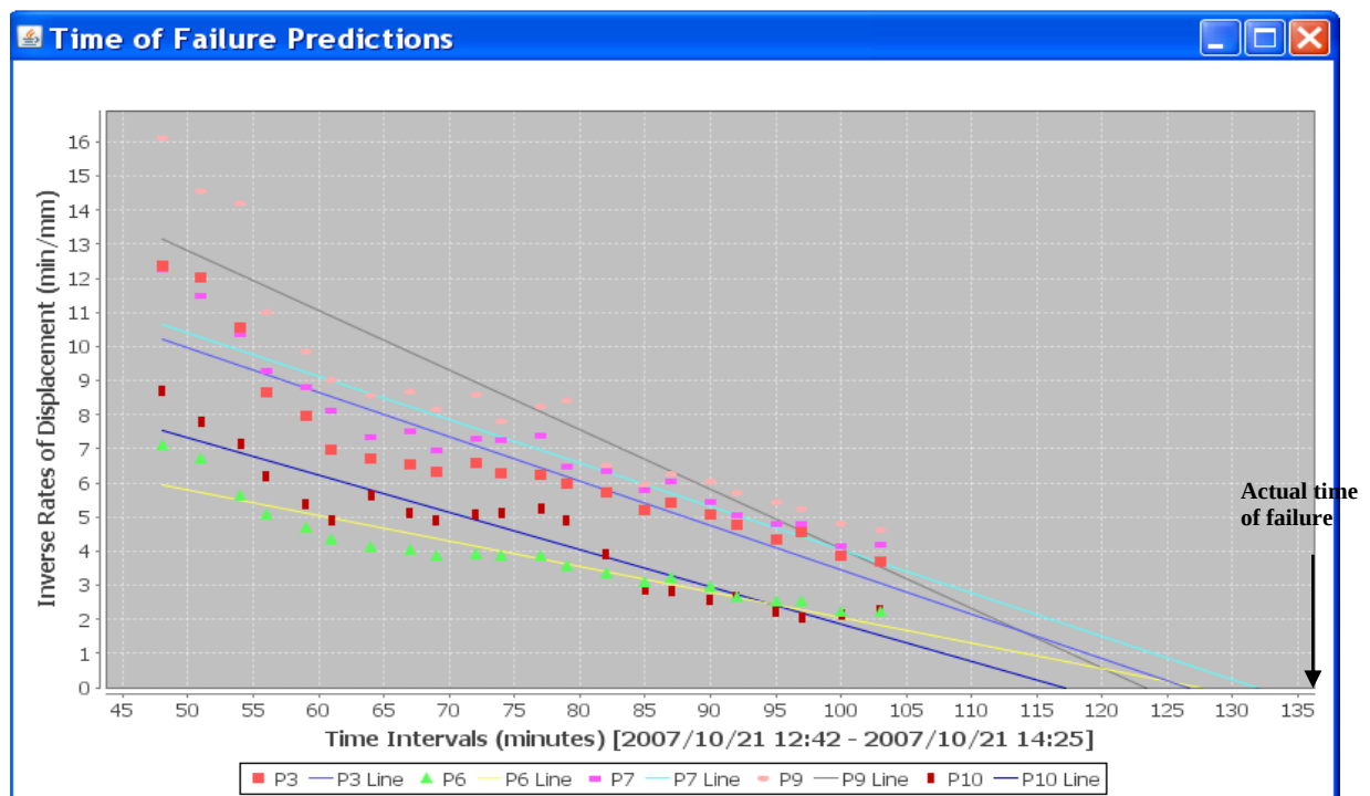
Figure 6.27: Graphical illustration of the five most active points of validation test 3.
