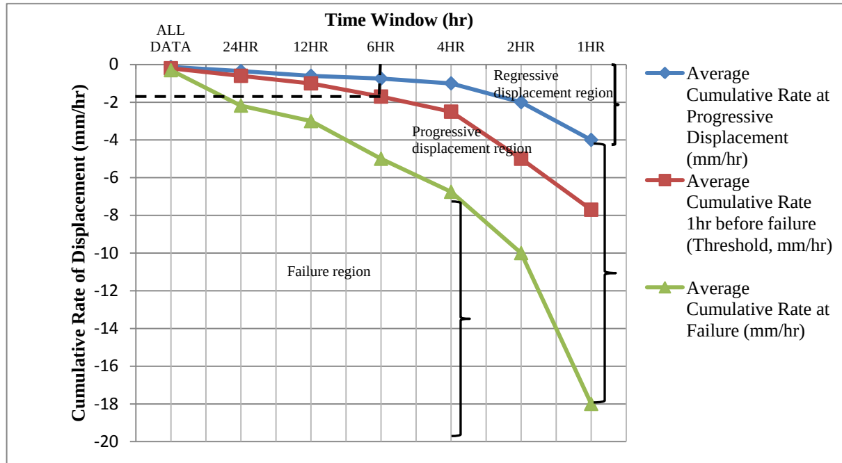
Figure 6.4: Cumulative rate of displacement (mm/hr) threshold determination based on point monitoring for the New Vaal coal mine.
