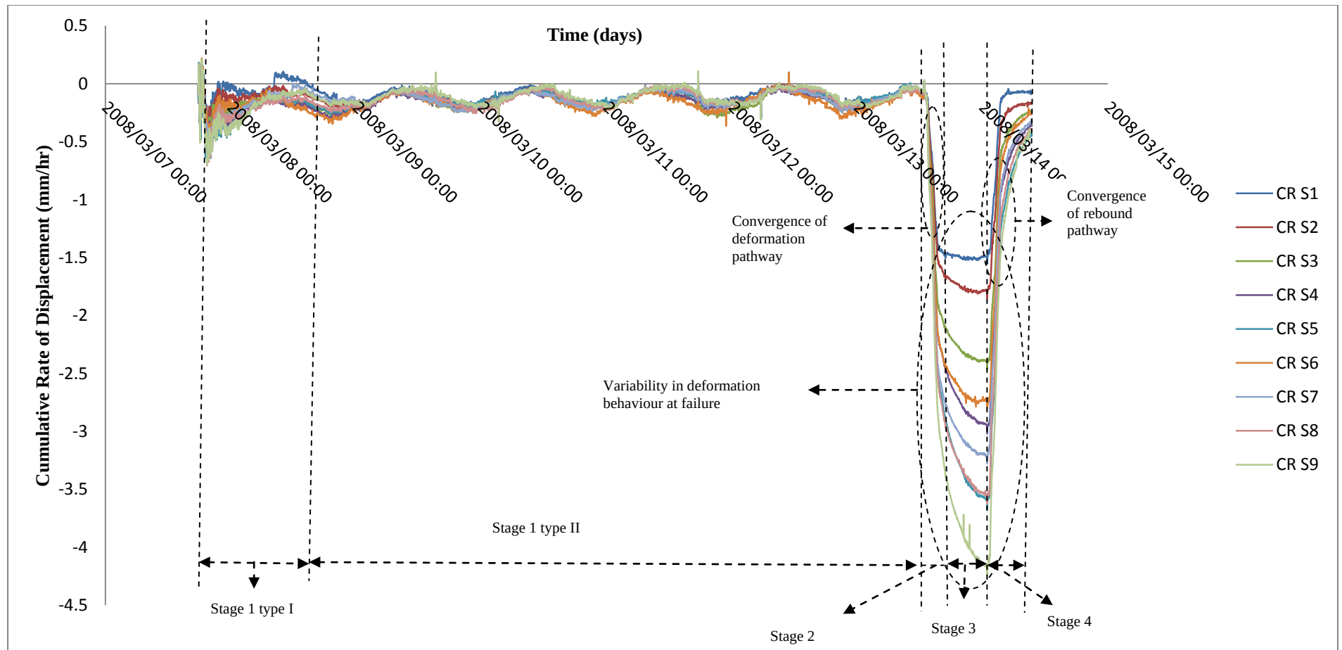
Figure 5.26: Cumulative rate of displacement (mm/hr) of sections 1-9 of ramp 12 slope.
