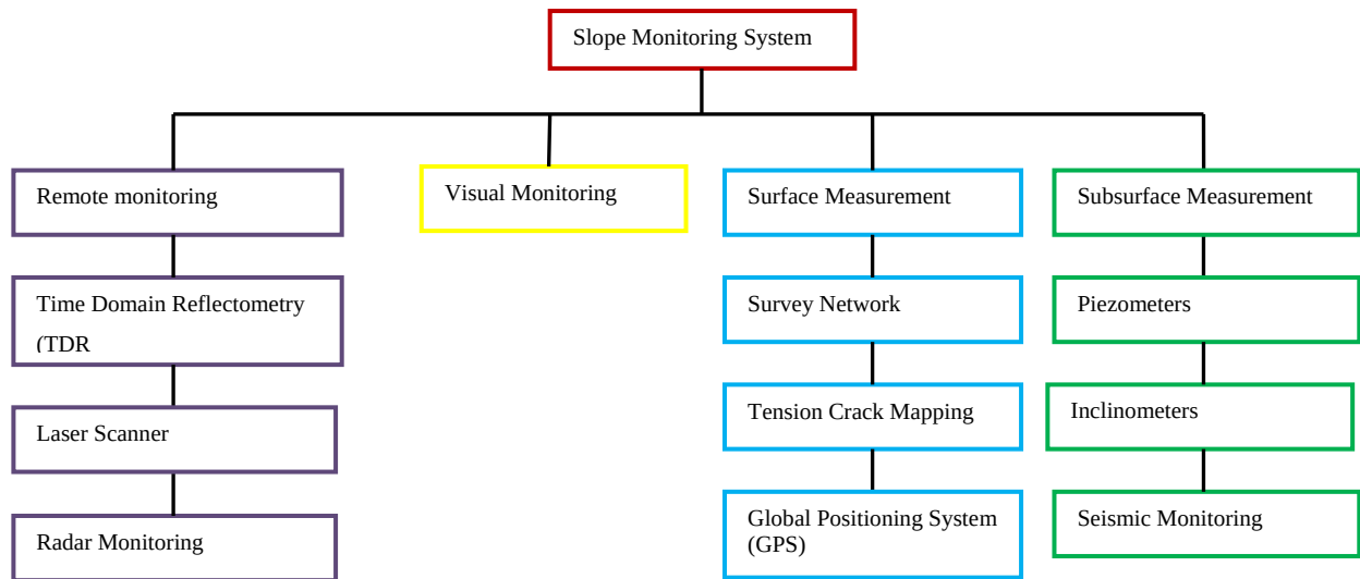
Figure 3.2: Slope monitoring system
