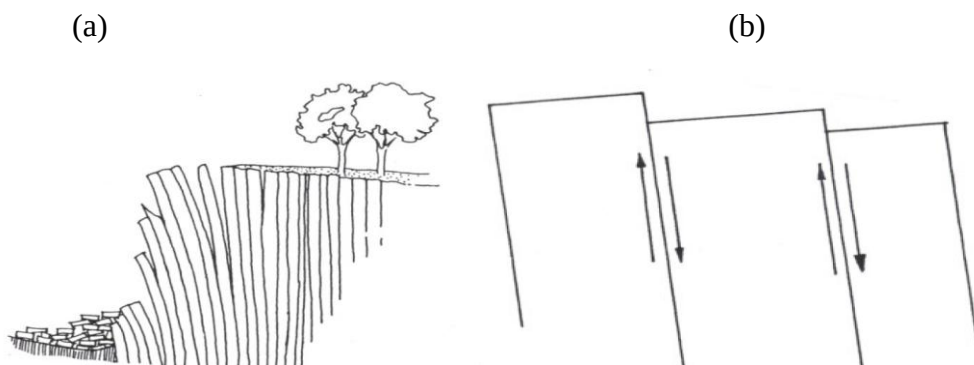
Figure 2.14: (a) Flexural toppling example (After Goodman and Bray, 1976) (b) Flexural toppling with a sliding movement between the faces of the toppling columns (After Hoek and Bray, 1981).
