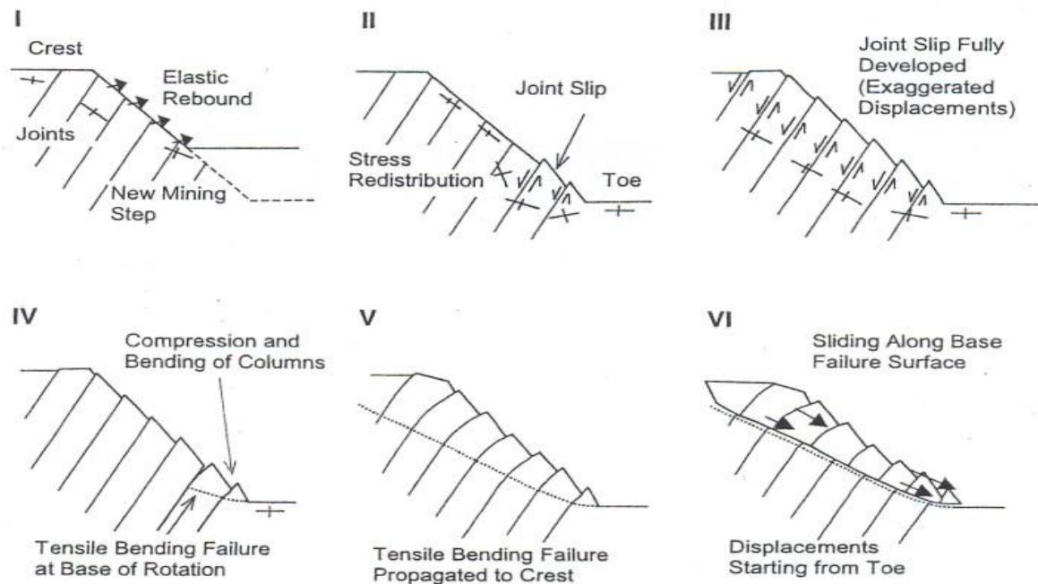
Figure 2.16: Failure stages for large-scale toppling failure in a slope (After Sjöberg, 2000).
