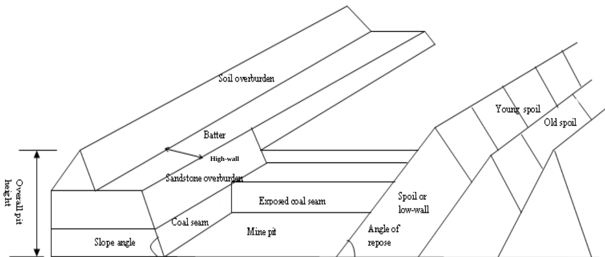
Figure 2.2: Open cast coal mine slope geometry.
