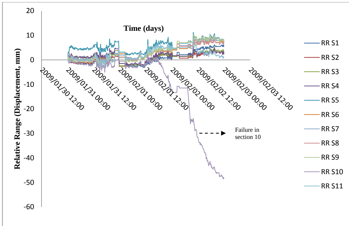
Figure 5.28: Relative range (Displacement, mm) of sections 1-11 of case example 6.
