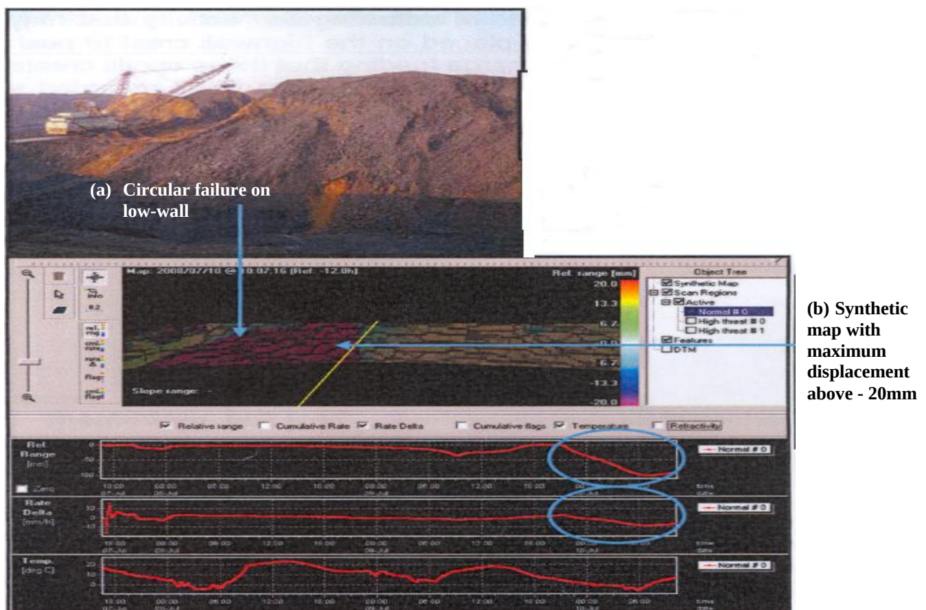
Figure 4.16: MSR synthetic map and trend plots of low-wall displacement (Zindela, 2008).
