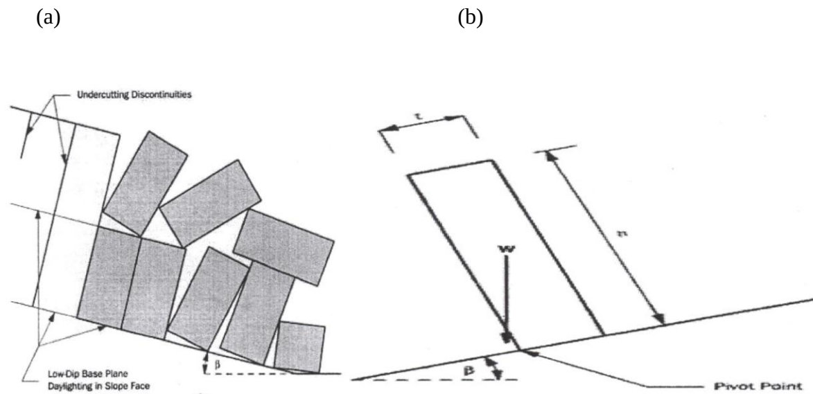
Figure 2.11: (a) Toppling failure mode. (b) Potential toppling failure when the vertical weight component, W , is outside the pivot point (After Kliche, 1999).
