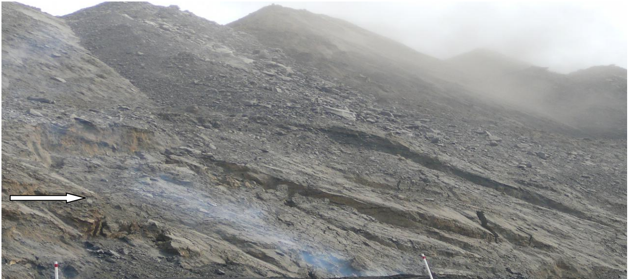
Figure 2.2: Rotational failure on low-wall (spoil) at New Vaal Open-cast coal mine.
