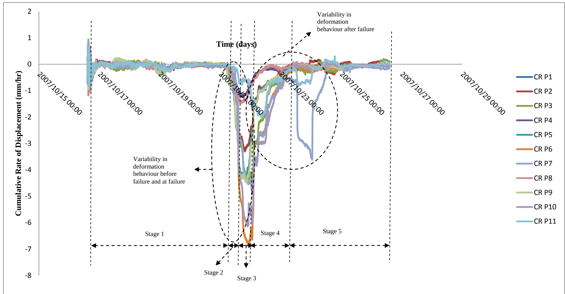
Figure 5.17: Cumulative rate of displacement (mm/hr) of eleven points in ramp 5 failure region.
