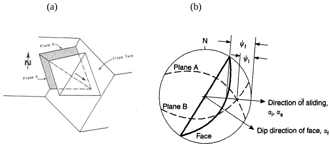
Figure 2.9: (a) Wedge failure mode (Piteau and Martin, 1982) (b) Kinematic analysis of wedge failure.
