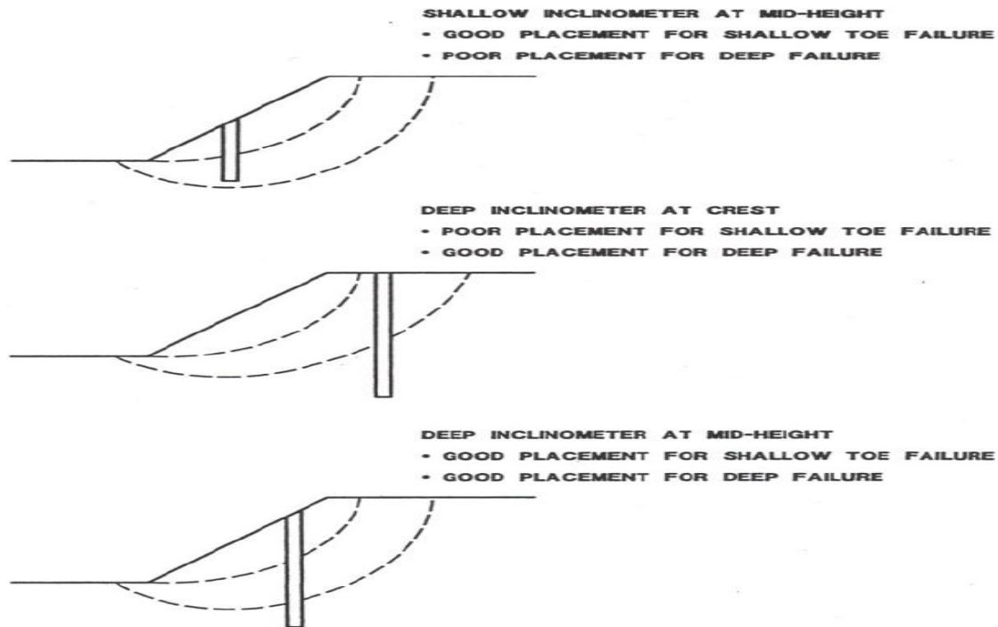
Figure 3.4: Proper inclinometer placement in a slope (Abramson, et al. 2002).
