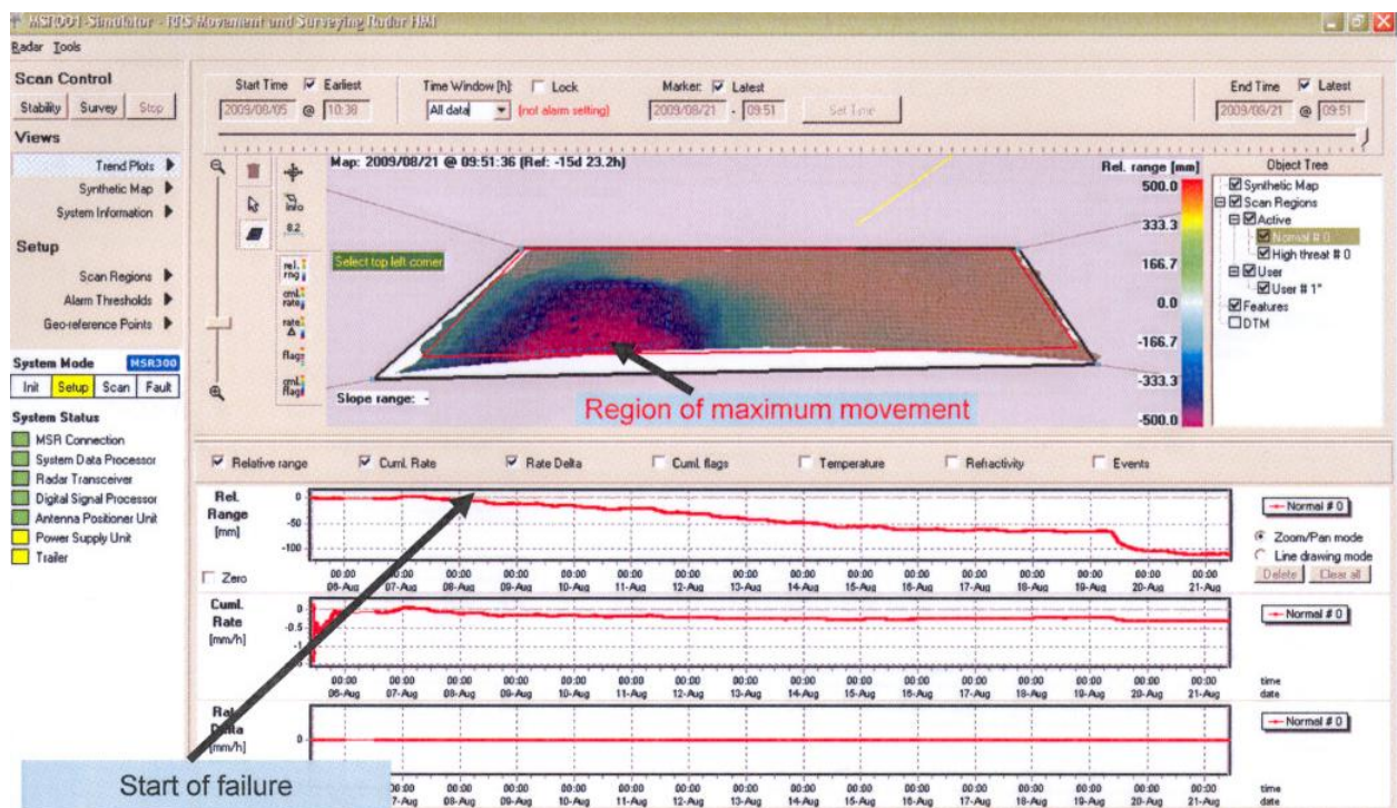
Figure 4.12: MSR trend plots and synthetic map of the scanned low-wall (New Vaal Colliery, 2009b).
