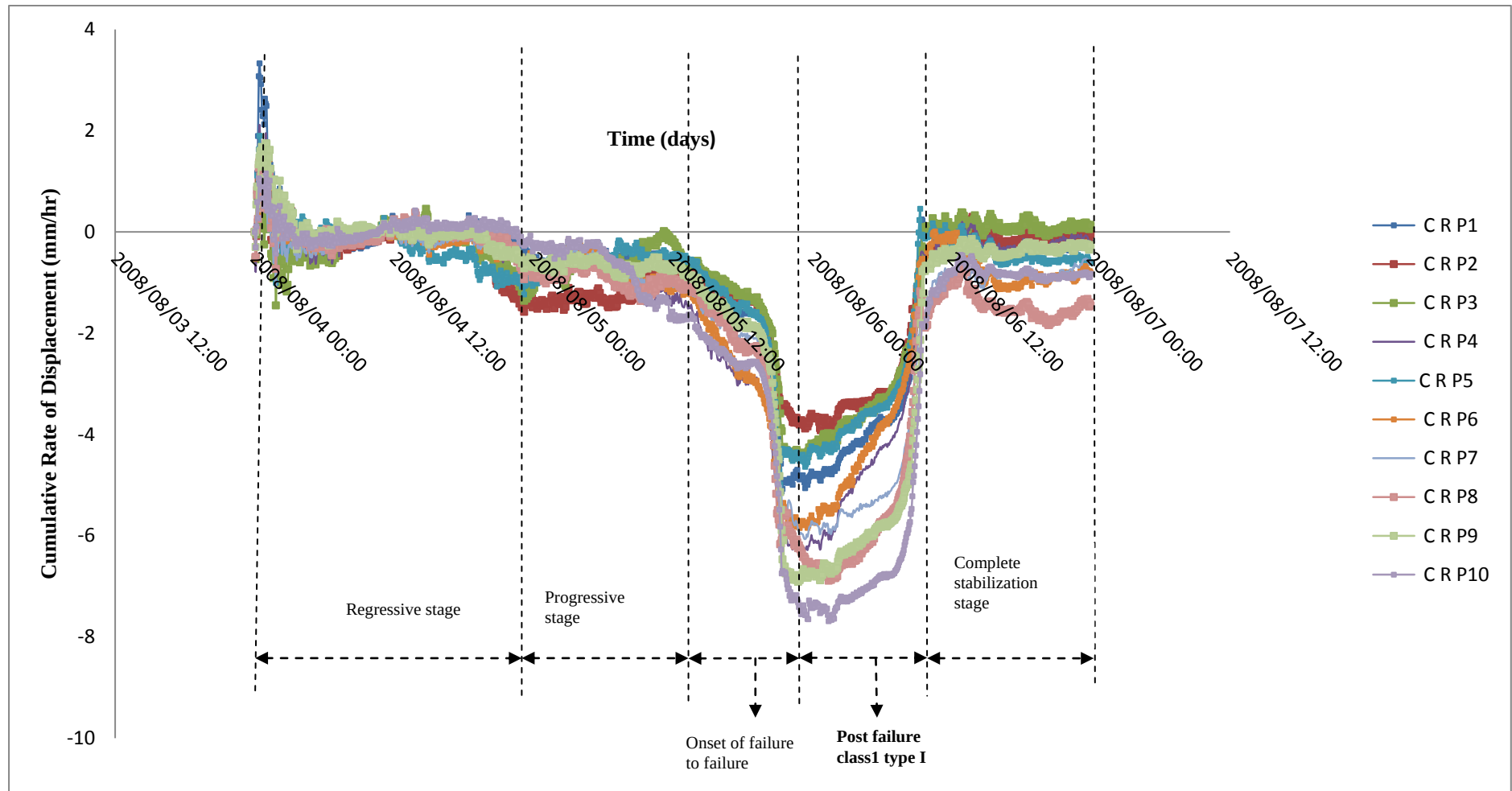
Figure 5.33: Post-failure class 1 type I displacement behaviour.
