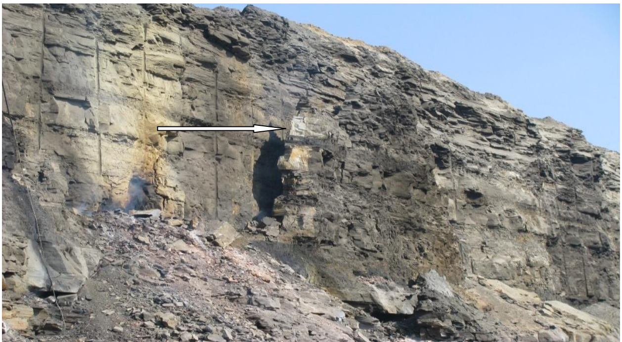
Figure 1.8: Dangerous overhang on high-wall at Kleinkopje open-cast coal mine.
