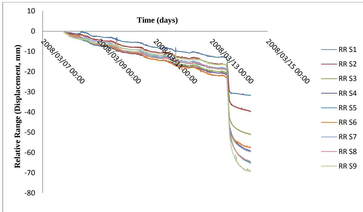
Figure 5.25: Relative range (Displacement, mm) of sections 1-9 of ramp 12 slope.
