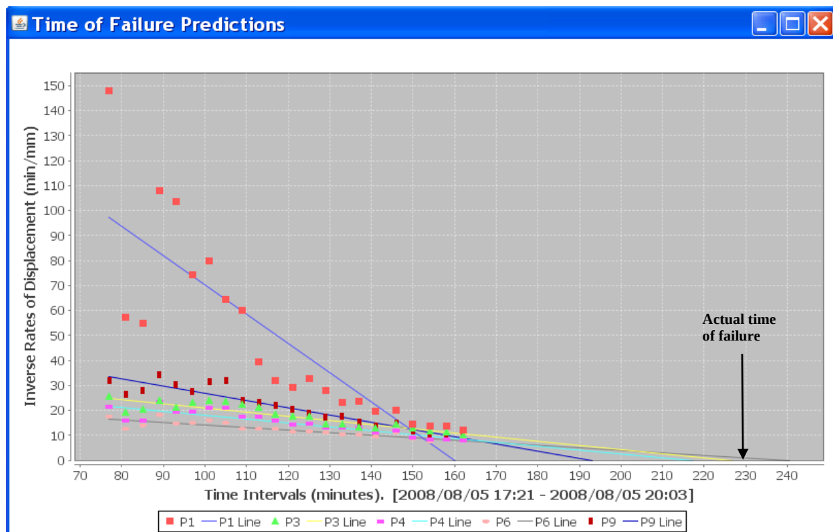
Figure 6.20: Graphical illustration of the five most active points of validation test 1.
