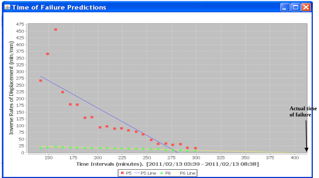
Figure 6.31: Graphical illustration of the two most active points of validation test 4.
