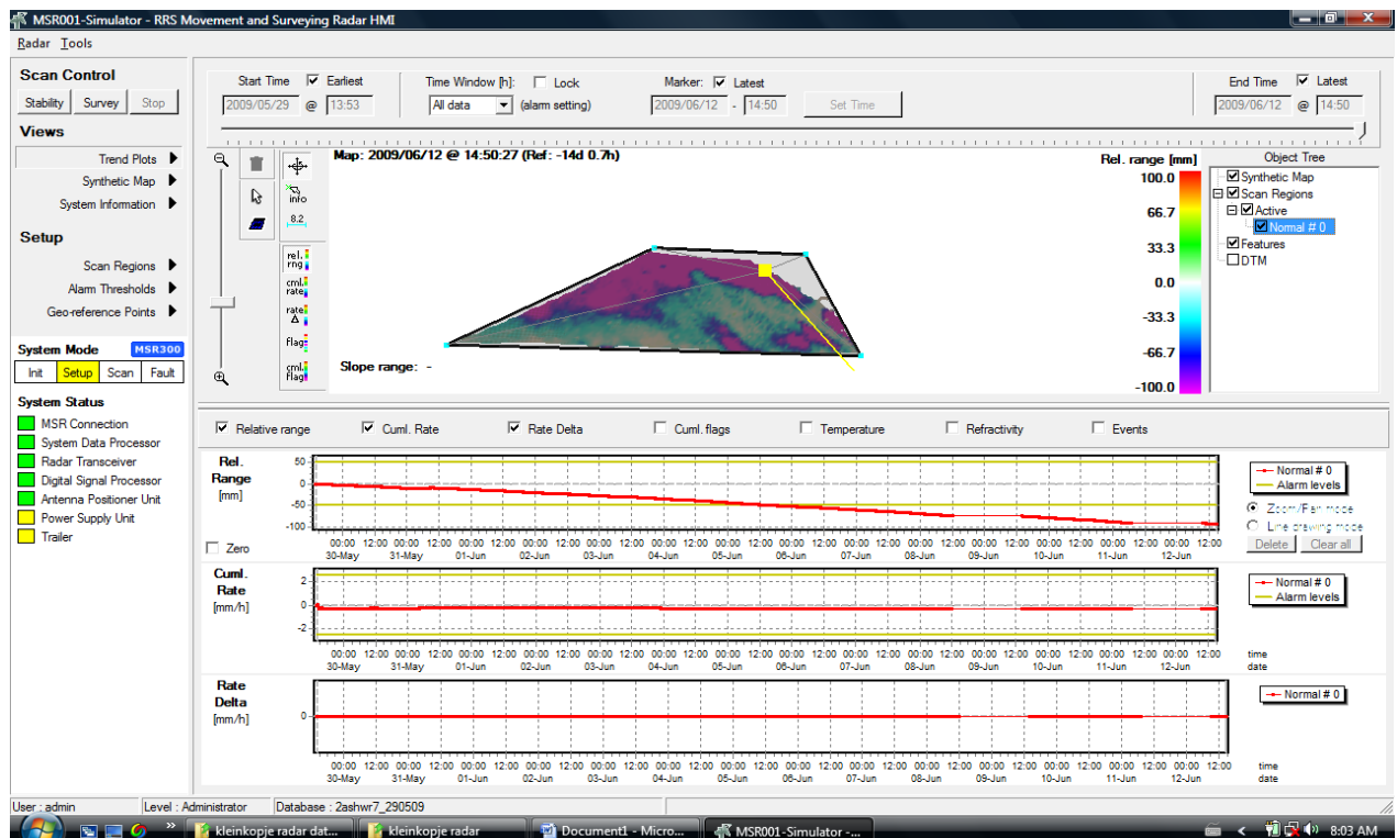
Figure 4.4: Trend plot of Kleinkopje open cast mine low-wall failure (Mottie, 2008).
