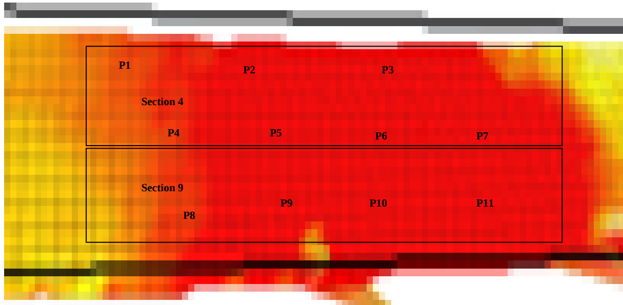
Figure 5.15: Failure section of ramp 5 showing the locations of eleven selected points.
