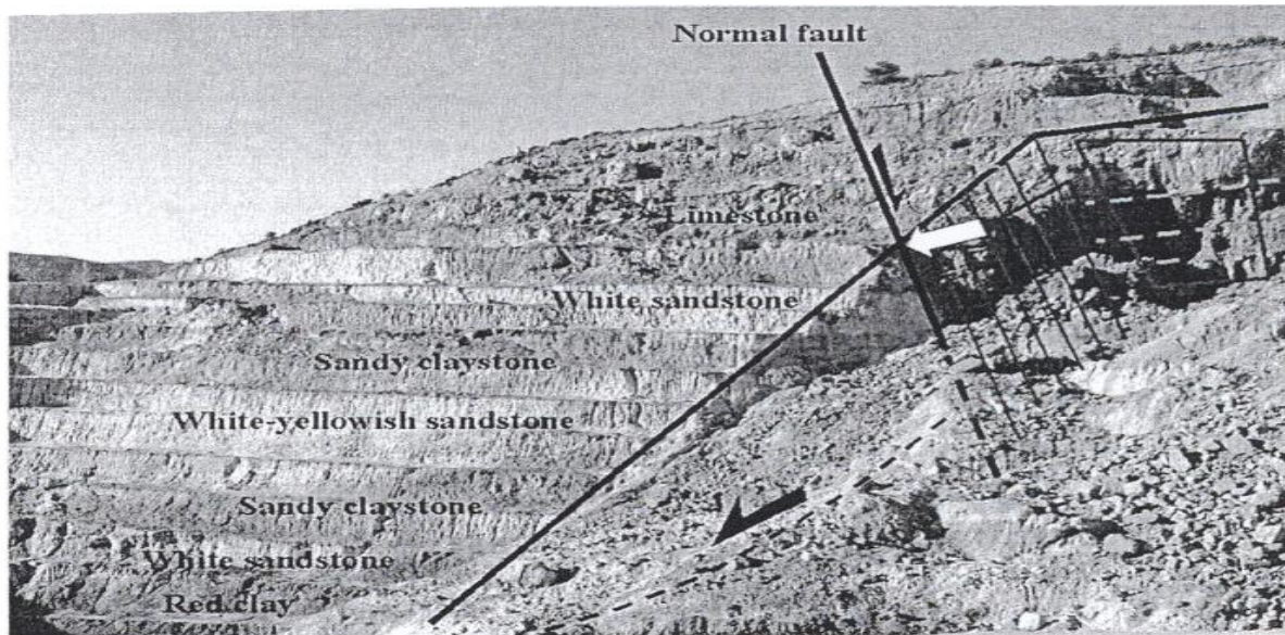
Figure 2.19: Toppling with circular failure (After Alejano, et al. 2010).
