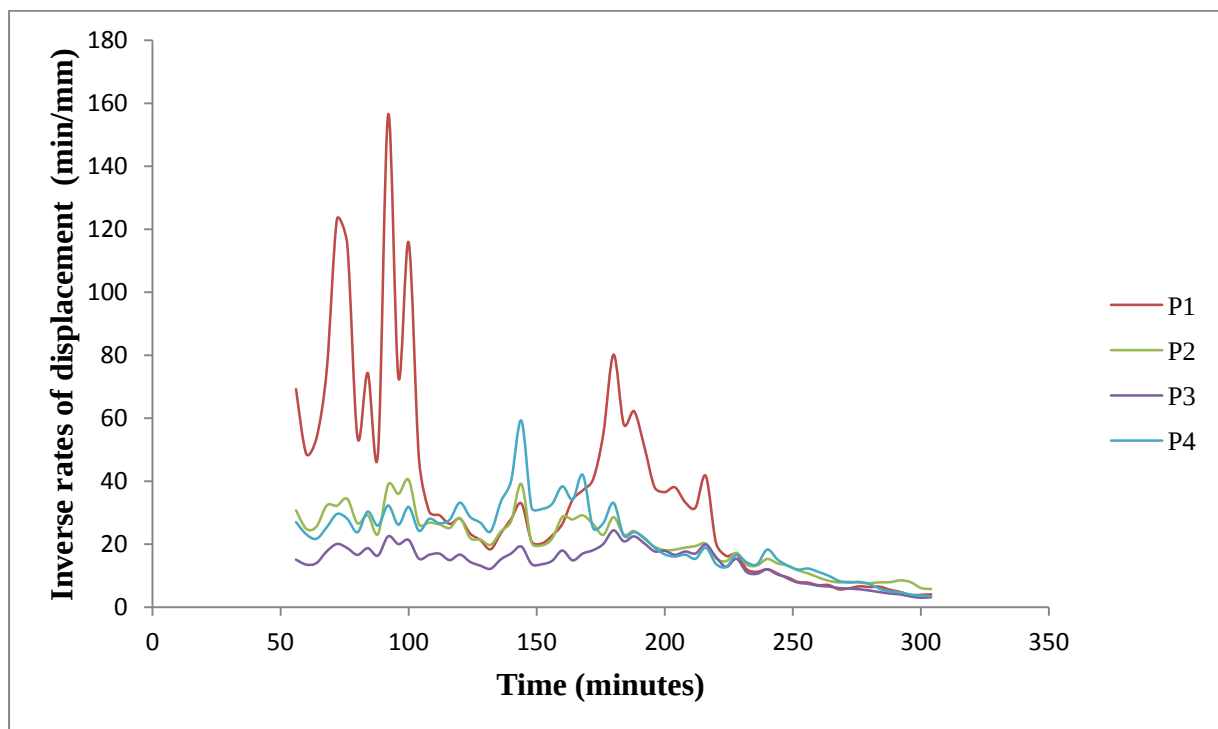
Figure 6.9: Inverse rates of displacement at 15 data interval (60 minutes).
