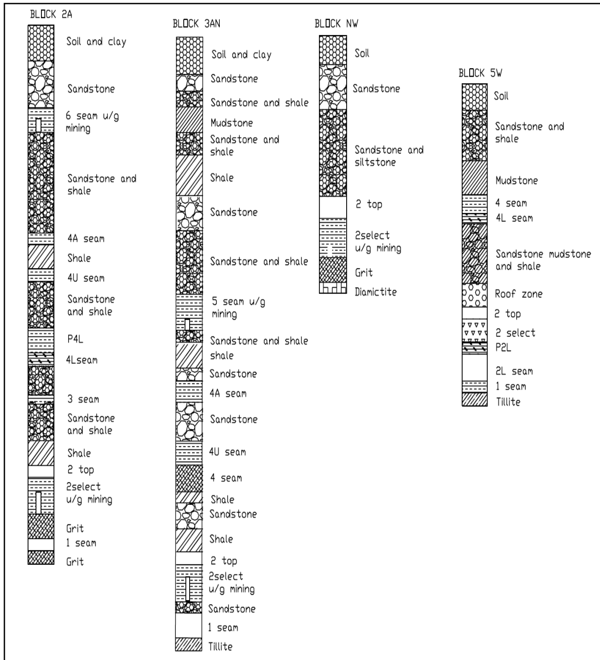
Figure 4.2: Typical borehole stratigraphy of Kleinkopje open-cast mine (Kleinkopje Colliery, 2009).
