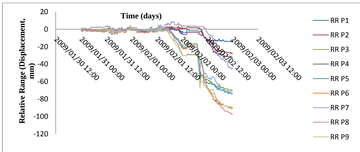
Figure 5.31: Relative range (Displacement, mm) of 10 points in the failure section of case example 6.
