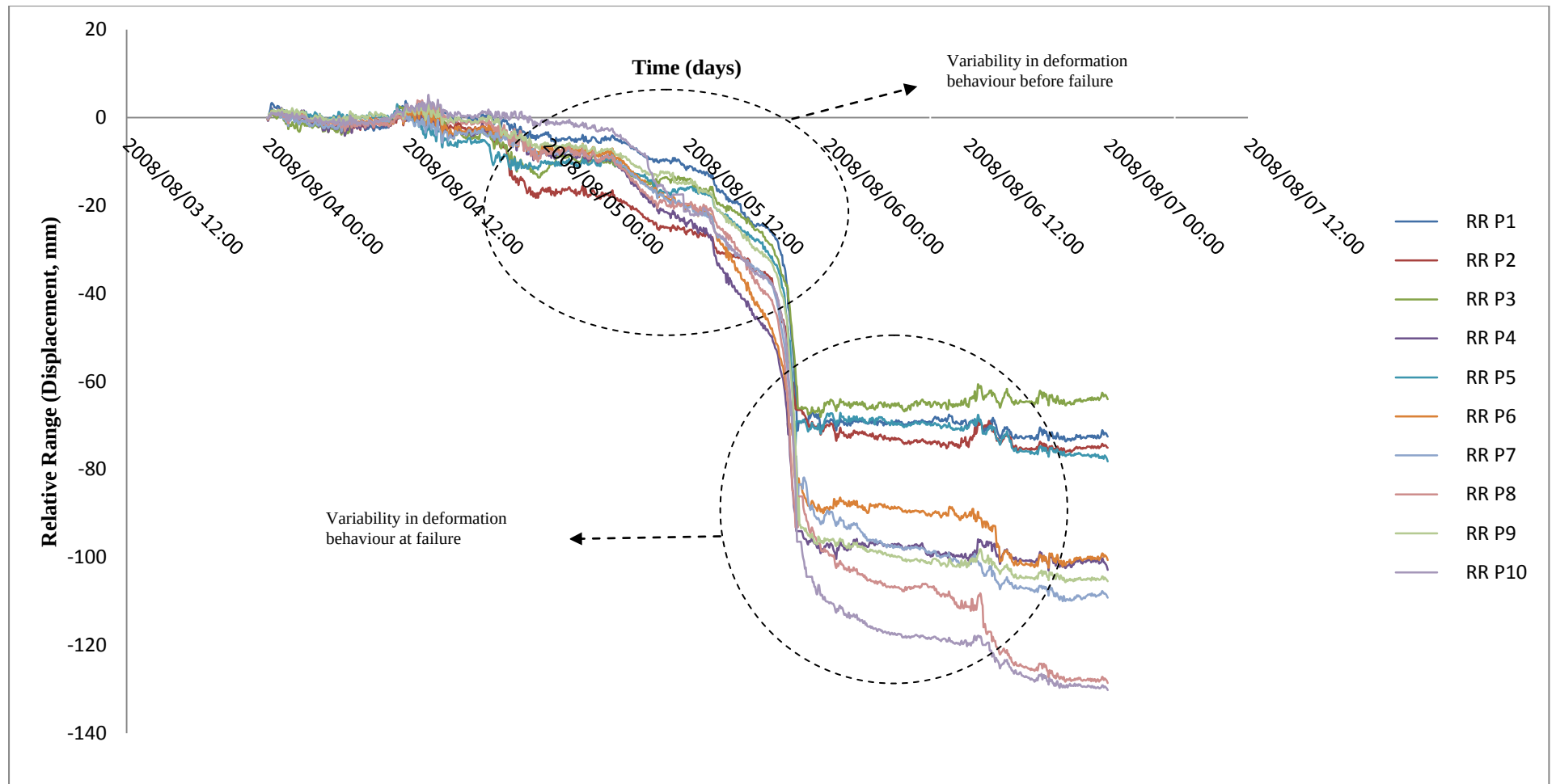
Figure 5.7: Relative range (Displacement, mm) of 10 points in the failure section of case example 1 slope.
