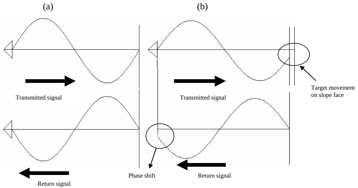
Figure 3.10: (a) First phase measurement of the MSR (b) Second phase measurement of the MSR (Reutech, 2006b).
