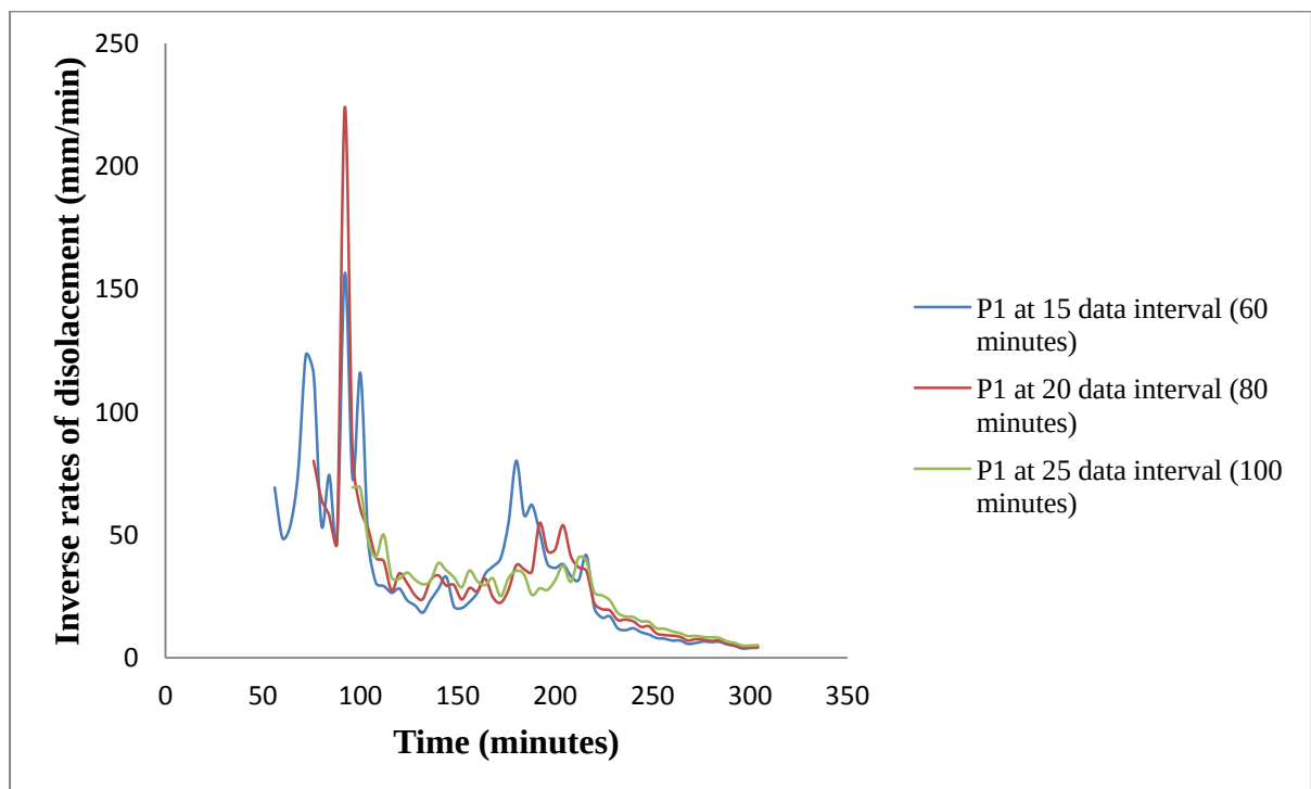
Figure 6.13: Inverse rates of displacement at 15, 20 and 25 data interval (60, 80 and 100 minutes).
