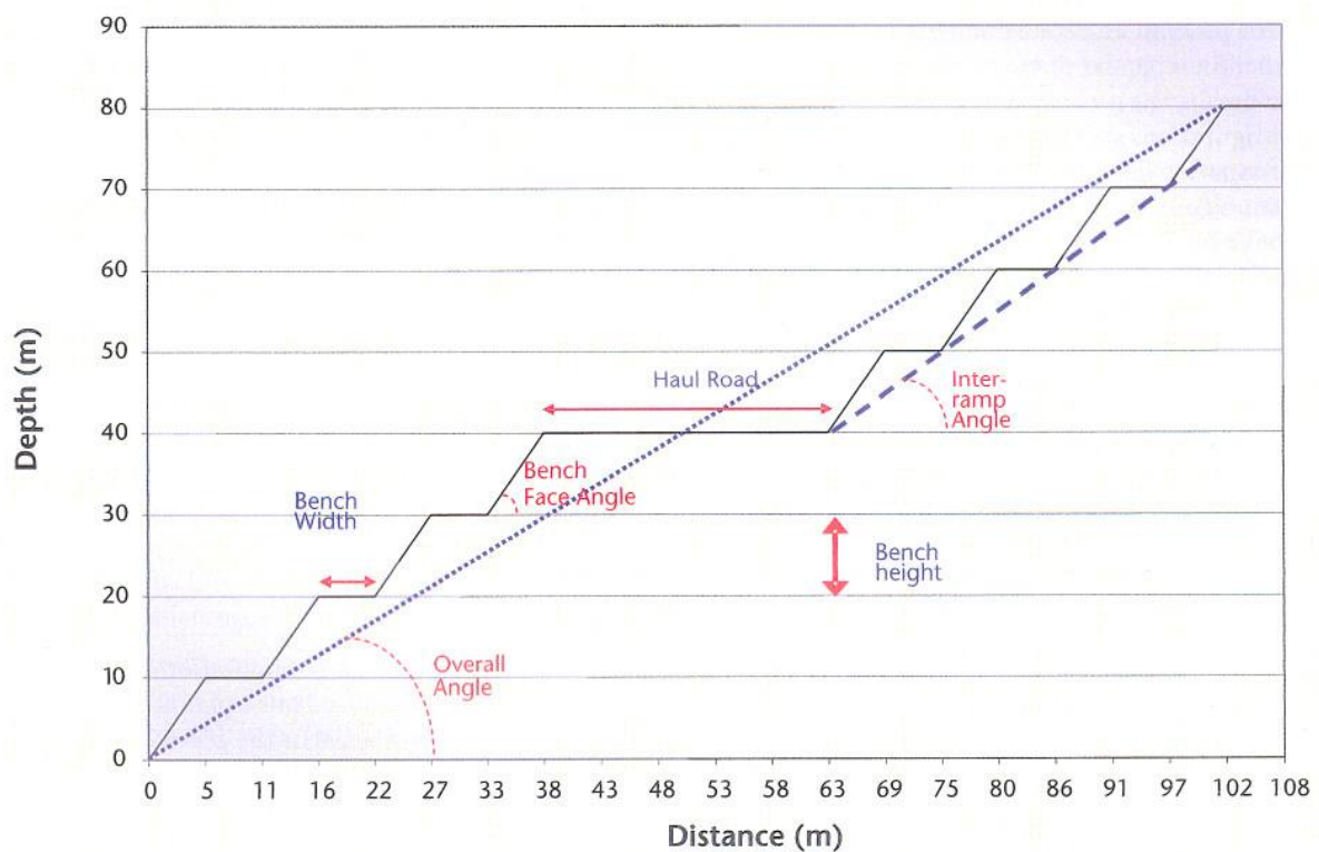
Figure 2.1: Open pit slope geometry showing relationship between overall slope angle, inter-ramp angle and bench (After Williams, et al. 2009).
