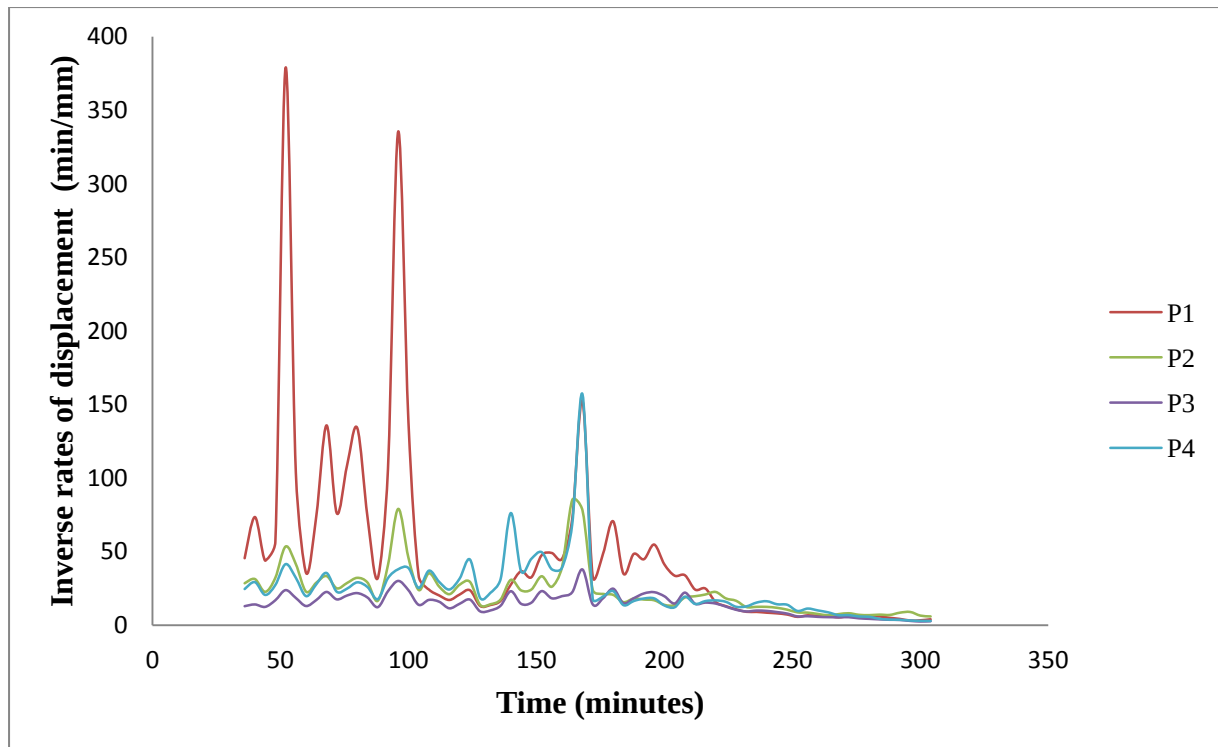
Figure 6.8: Inverse rates of displacement at 10 data interval (40 minutes).
