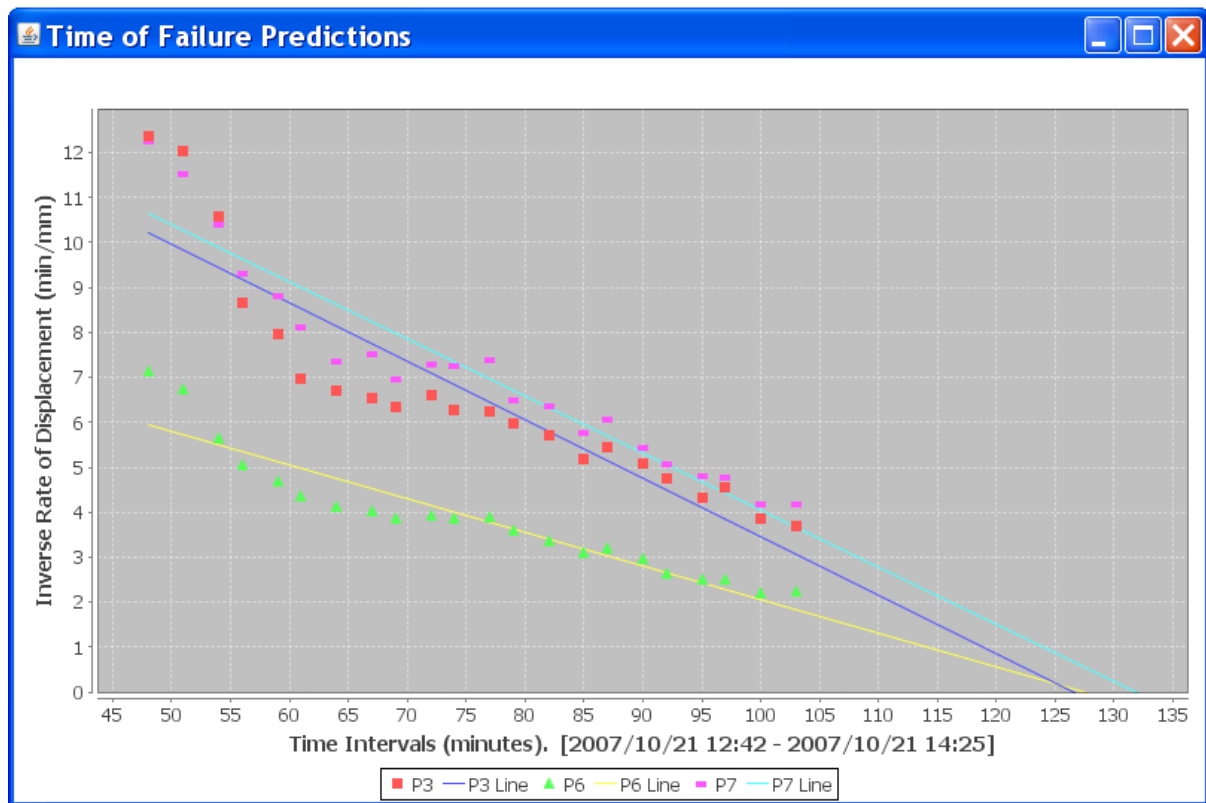
Figure 6.17: Graphical illustration of predictions from the active points.
