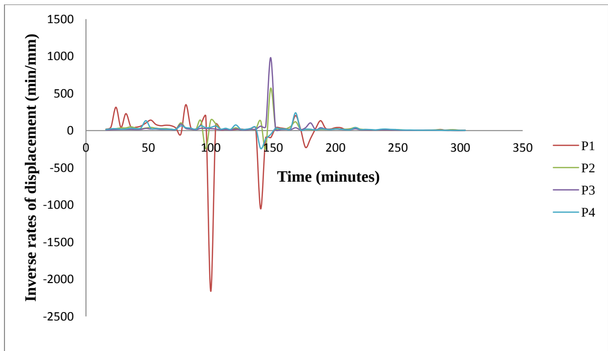
Figure 6.7: Inverse rates of displacement at 5 data interval (20 minutes).
