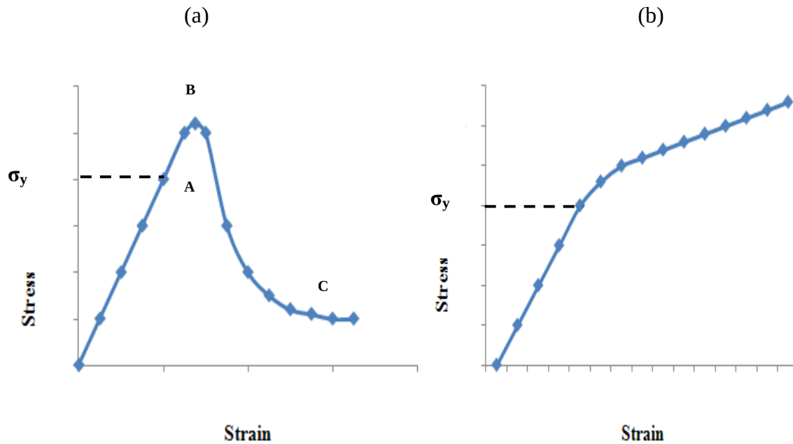
Figure 2.3: (a) Strain-softening stress-strain curve. (b) Strain-hardening stress-strain curve (After Brady and Brown, 2006).
