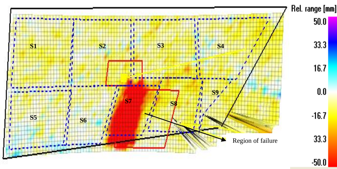
Figure 5.3: The scanned region of case example 1 slope
