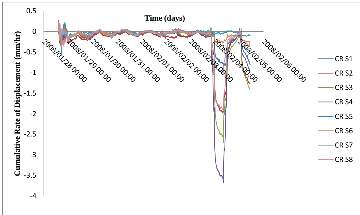
Figure 5.20: Cumulative rate of displacement (mm/hr) of sections 1-8 of ramp 11 slope.
