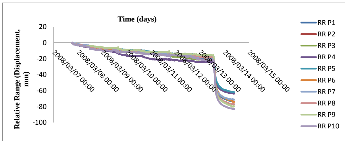
Figure 6.22: Relative range (Displacement, mm) of 10 points used for validation test 2.
