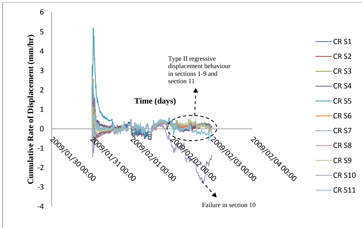
Figure 5.29: Cumulative rate of displacement (mm/hr) of sections 1-11 of case example 6.
