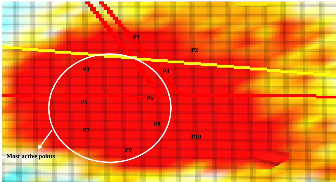
Figure 5.30: Failure section of case example 6 showing the locations of ten selected points.
