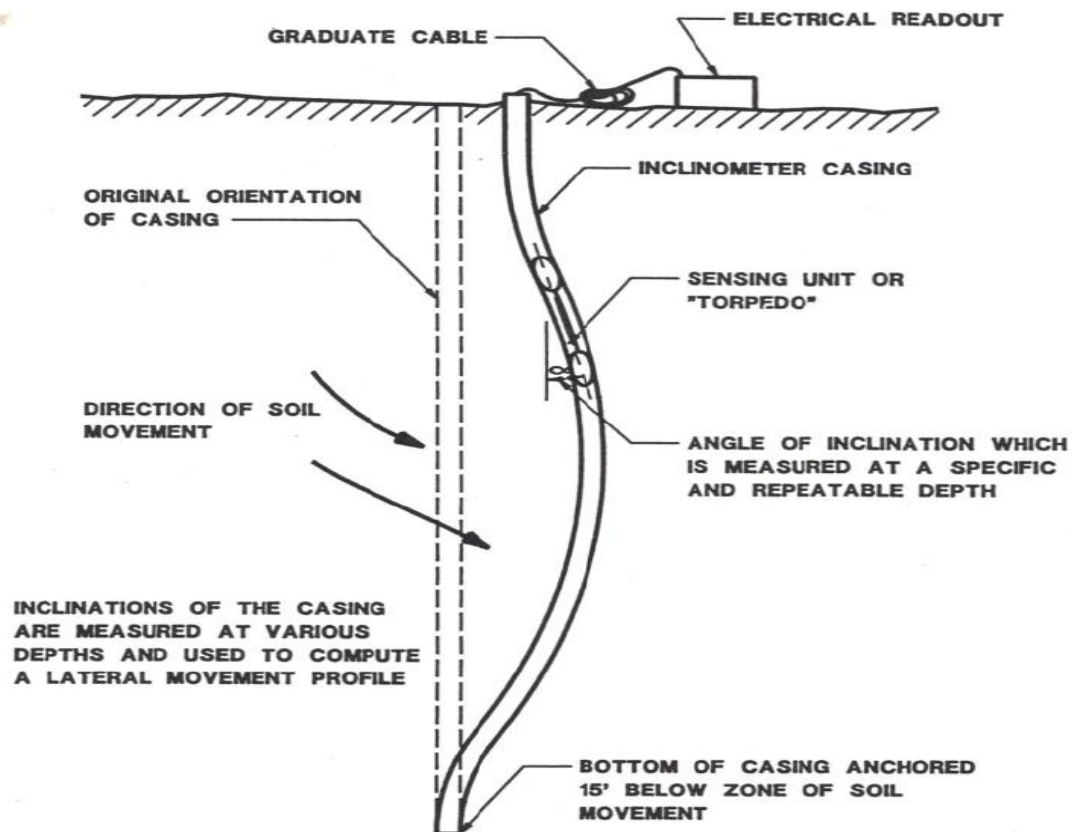
Figure 3.3: Portable borehole inclinometer system (Abramson, et al. 2002).
