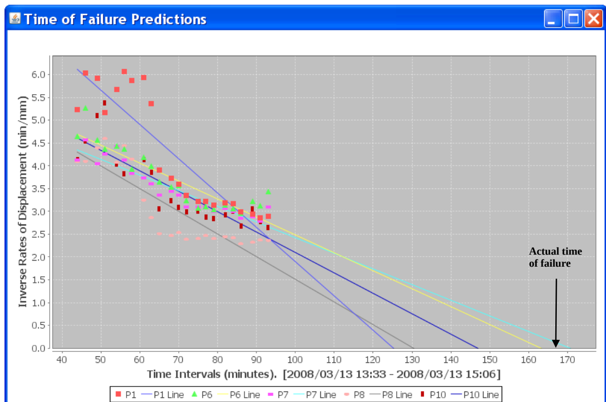
Figure 6.24: Graphical illustration of the five most active points of validation test 2.
