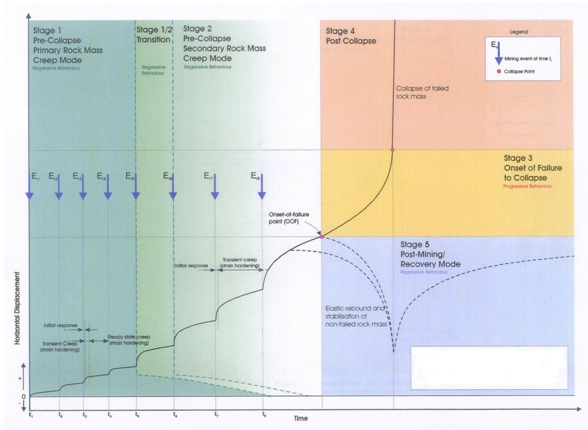
Figure 2.21: Generalised time and event dependent rock mass deformation model (After Mercer, 2006).
