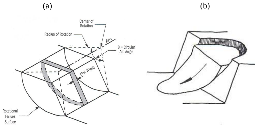
Figure 2.6: (a) Rotational failure mode (b) Circular failure mode, according to Hoek and Bray (1981).
