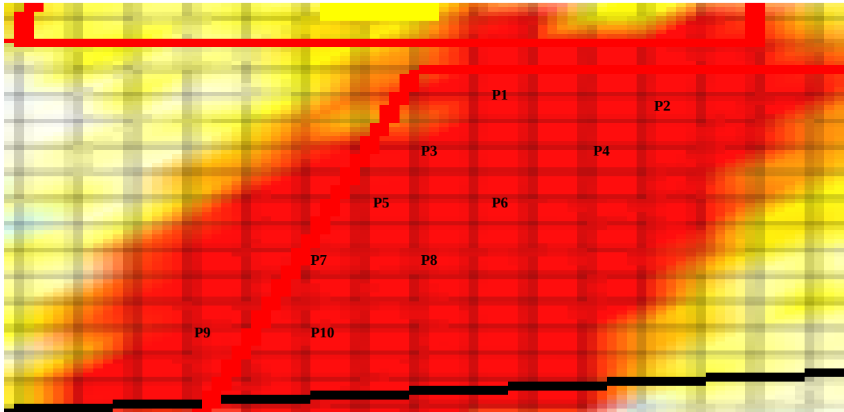
Figure 5.6: Failure section showing the locations of ten selected points in case example 1 slope.
