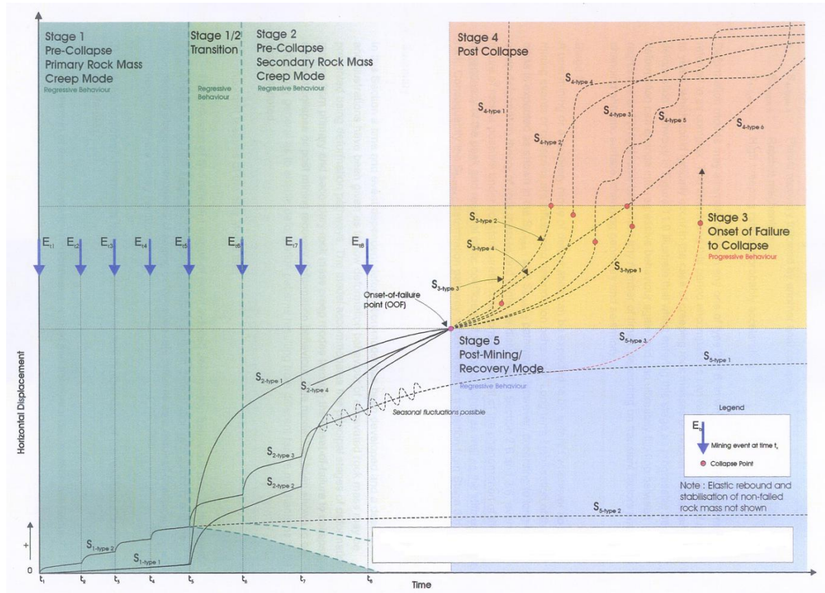
Figure 2.22. Generalised time and event dependent rock mass deformation model showing post collapse and post mining behaviour modes (Mercer, 2006).
