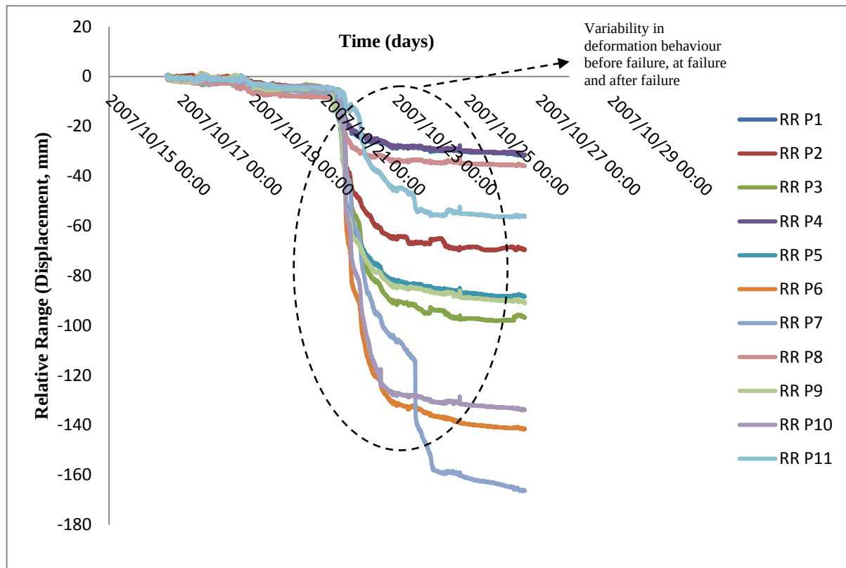
Figure 5.16: Relative range (Displacement, mm) of eleven points in ramp 5 failure region.
