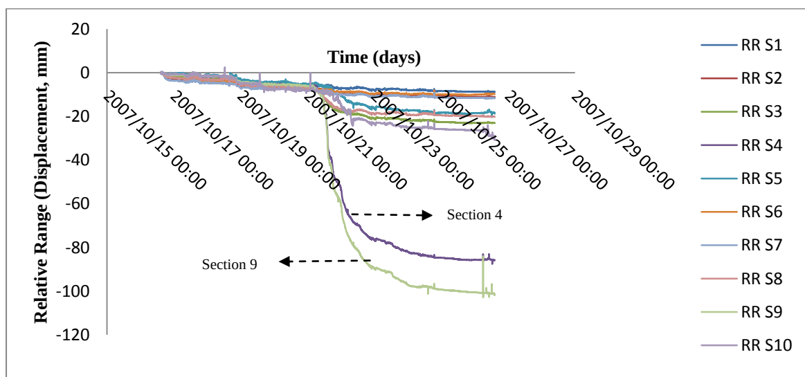
Figure 5.13: Relative range (Displacement, mm) of sections 1-10 of ramp 5 slope.
