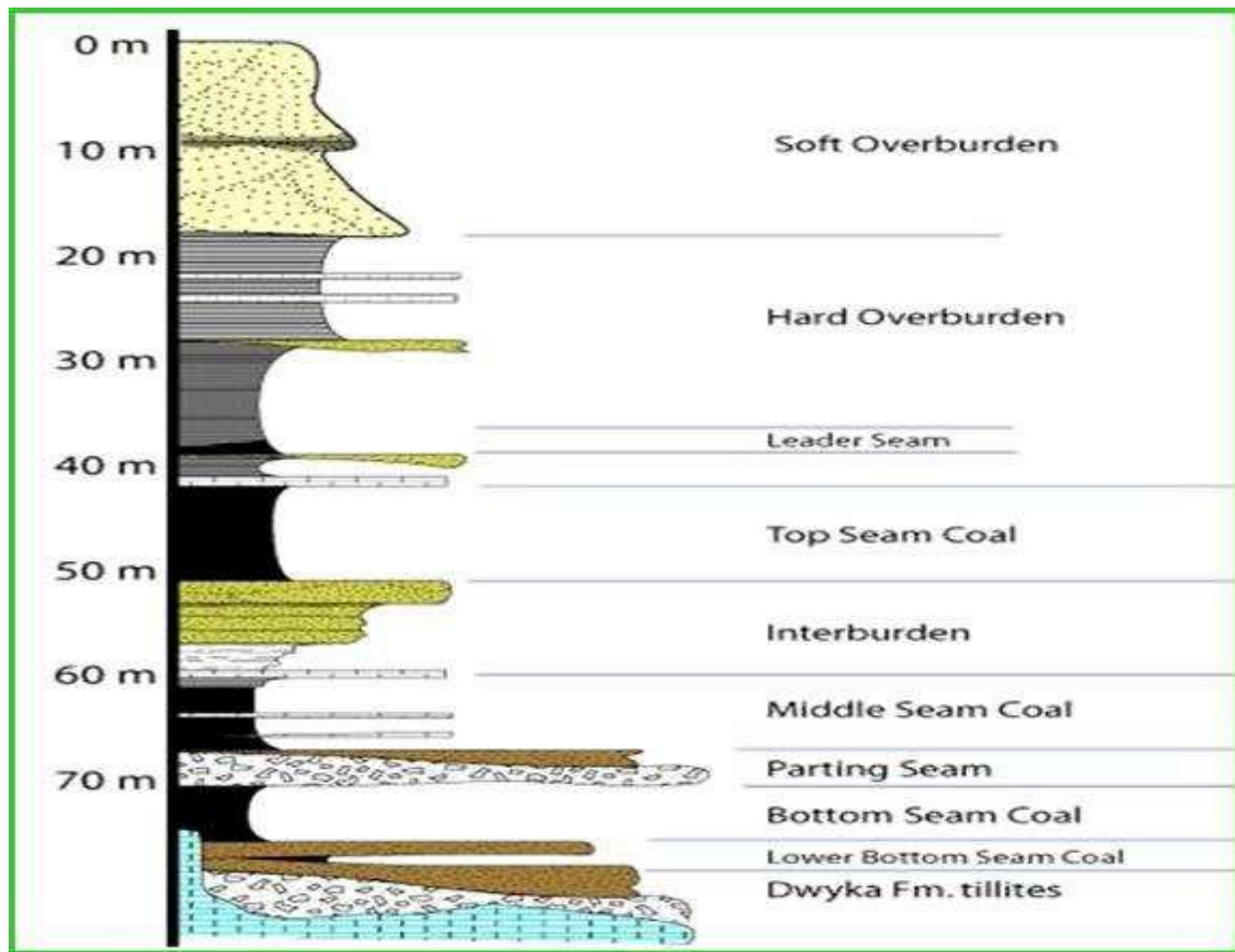
Figure 4.11: Typical stratigraphy column for New Vaal open cast mine (New Vaal Colliery, 2009a).
