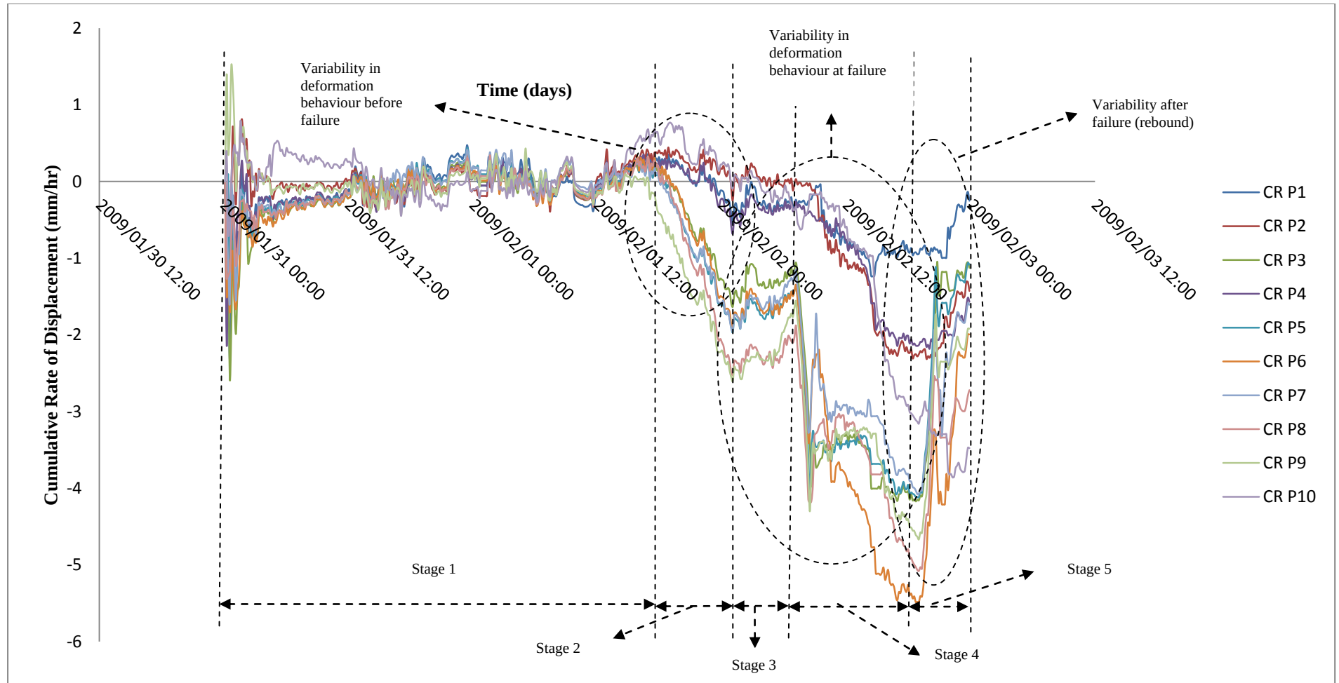
Figure 5.32: Cumulative rate of displacement (mm/hr) of 10 points in the failure section of case example 6.
