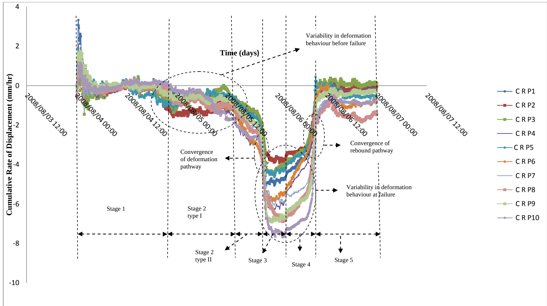
Figure 5.8: Cumulative rates of displacement, (mm/hr) of 10 points in section 7 of case example 1 slope.
