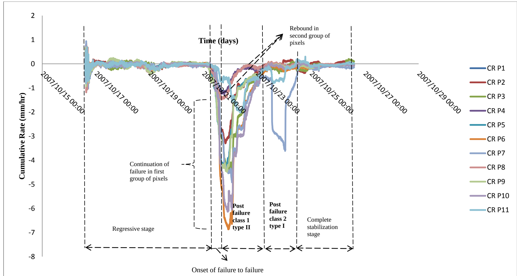
Figure 5.34: Post-failure class 1 type II and class 2 type I displacement behaviour.
