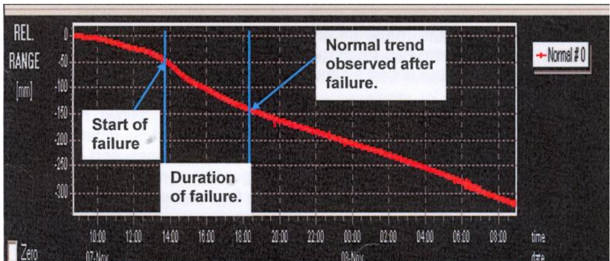
Figure 4.15: MSR trend plot of the high-wall displacement (Zindela, 2008).
