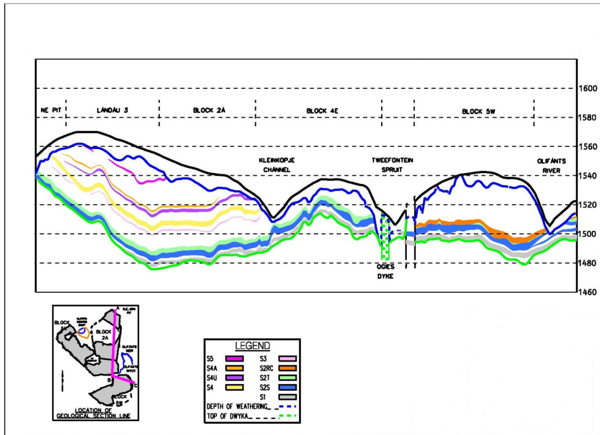
Figure 4.3: Typical geological cross section of Kleinkopje open-cast mine (Kleinkopje Colliery, 2009).
