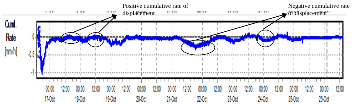
Figure 5. 1: Negative-positive regressive behaviour of stable slope at Landau open cast mine (Type I).
