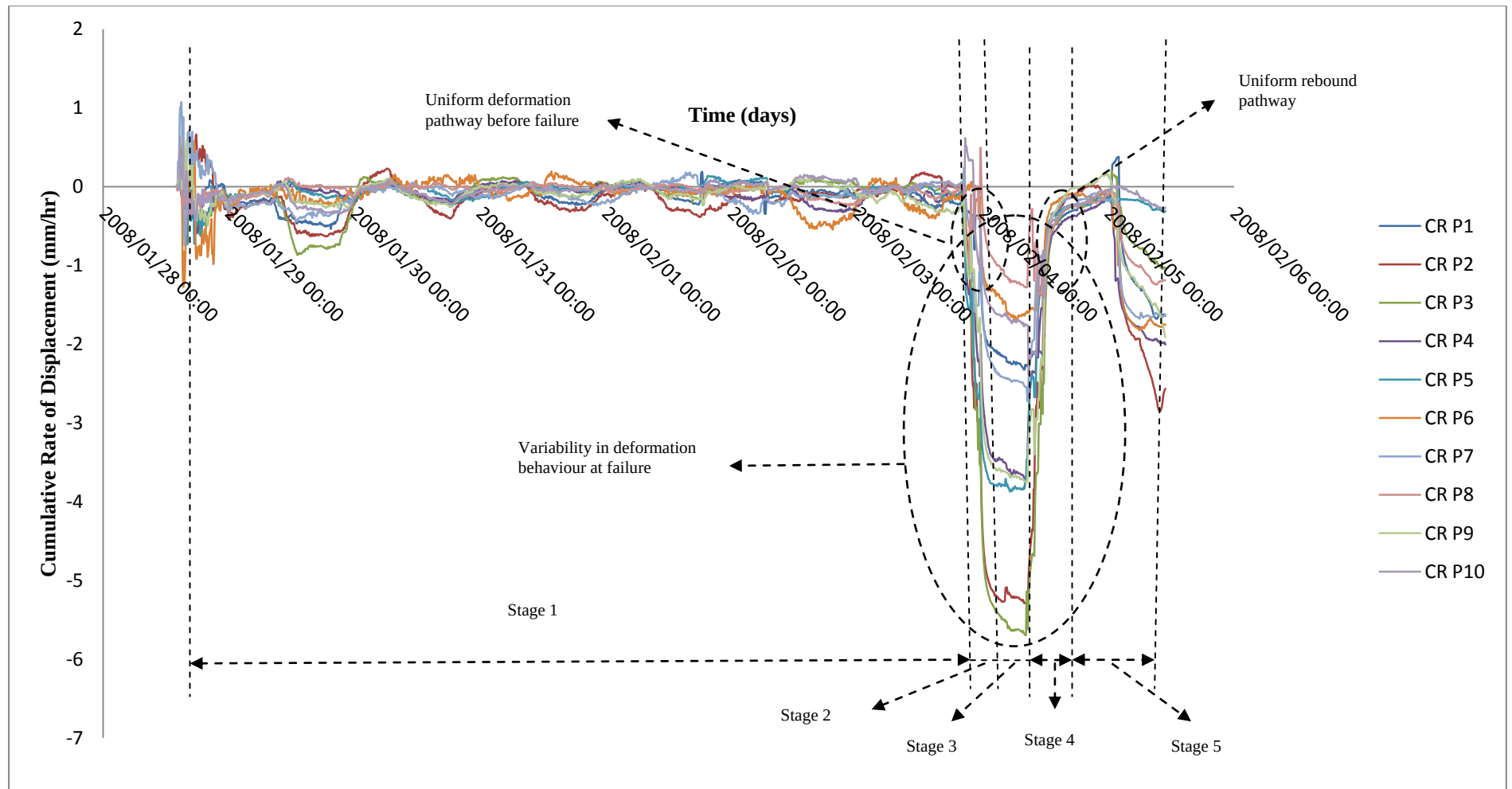
Figure 5.23: Cumulative rate of displacement (mm/hr) of 10 points in ramp 11 failure sections.
