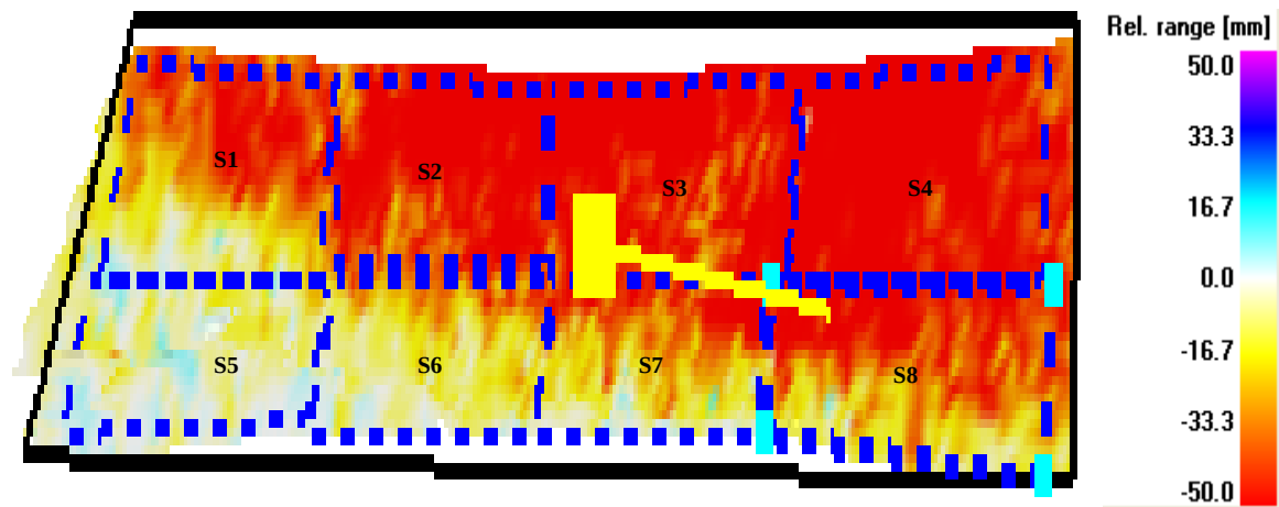
Figure 5.18: The scanned region of ramp 11 slope.
