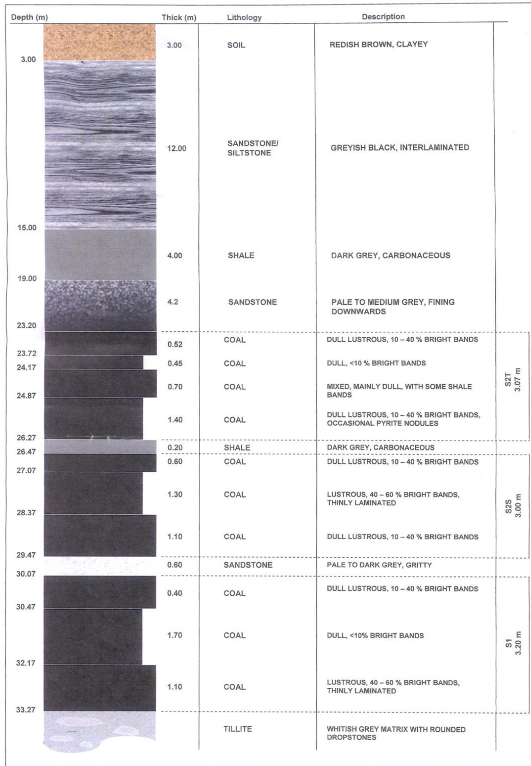
Figure 4.7: Typical borehole stratigraphy of Landau open cast mine (Landau Colliery, 2009).
