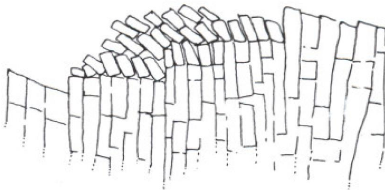
Figure 2.12: Block toppling example (After Goodman and Bray, 1976).
