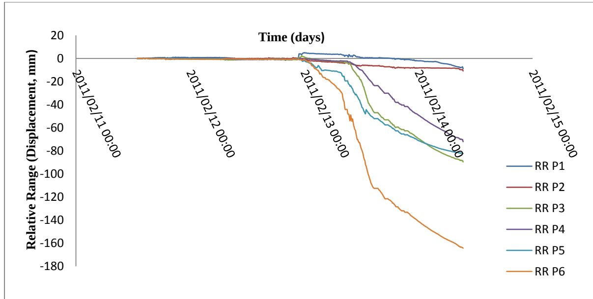
Figure 6.29: Relative range (Displacement, mm) of 6 points used for validation test 4.
