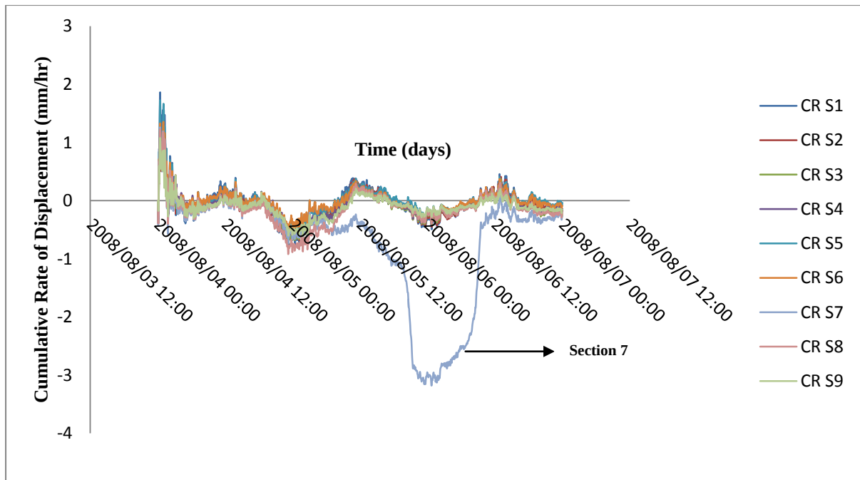
Figure 5.5: Cumulative rate of displacement (mm/hr) of sections 1- 9 of case example 1 slope.
