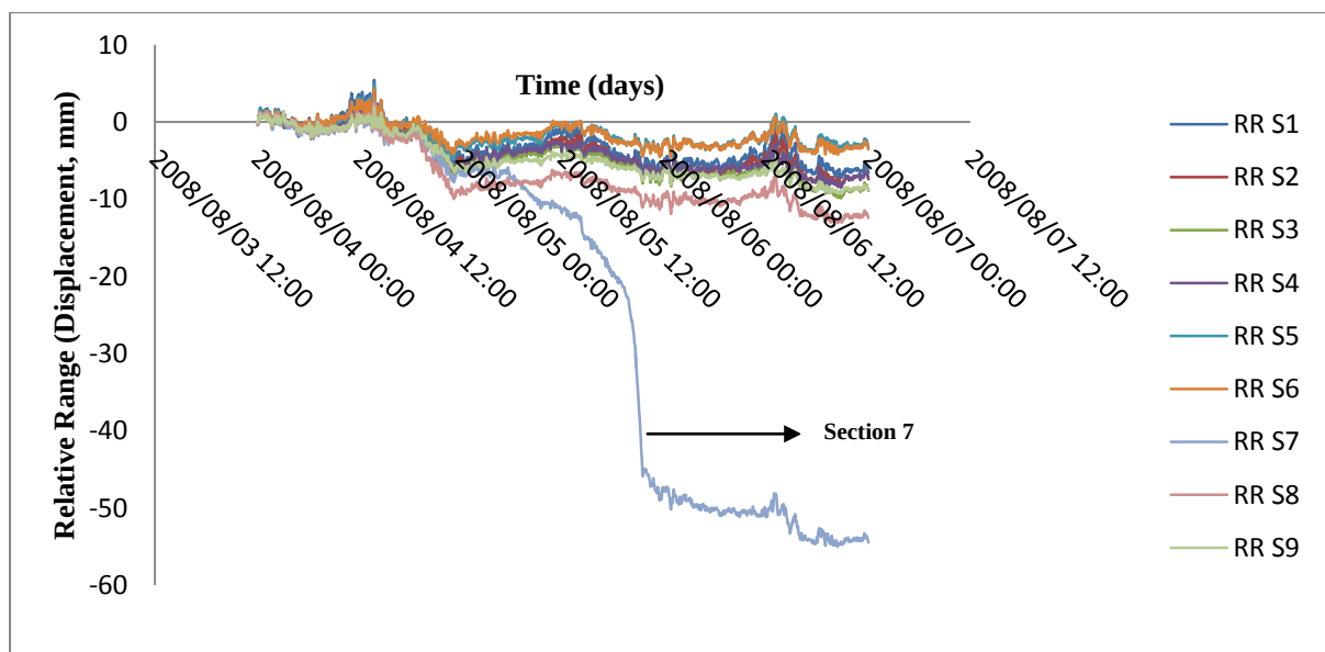
Figure 5.4: Relative range (Displacement, mm) of sections 1-9 of case example 1 slope.
