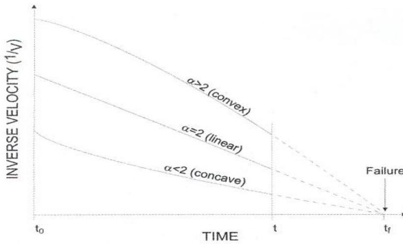
Figure 6.2: Inverse velocity versus time relationships preceding slope failure (After Fukuzono, 1985).
