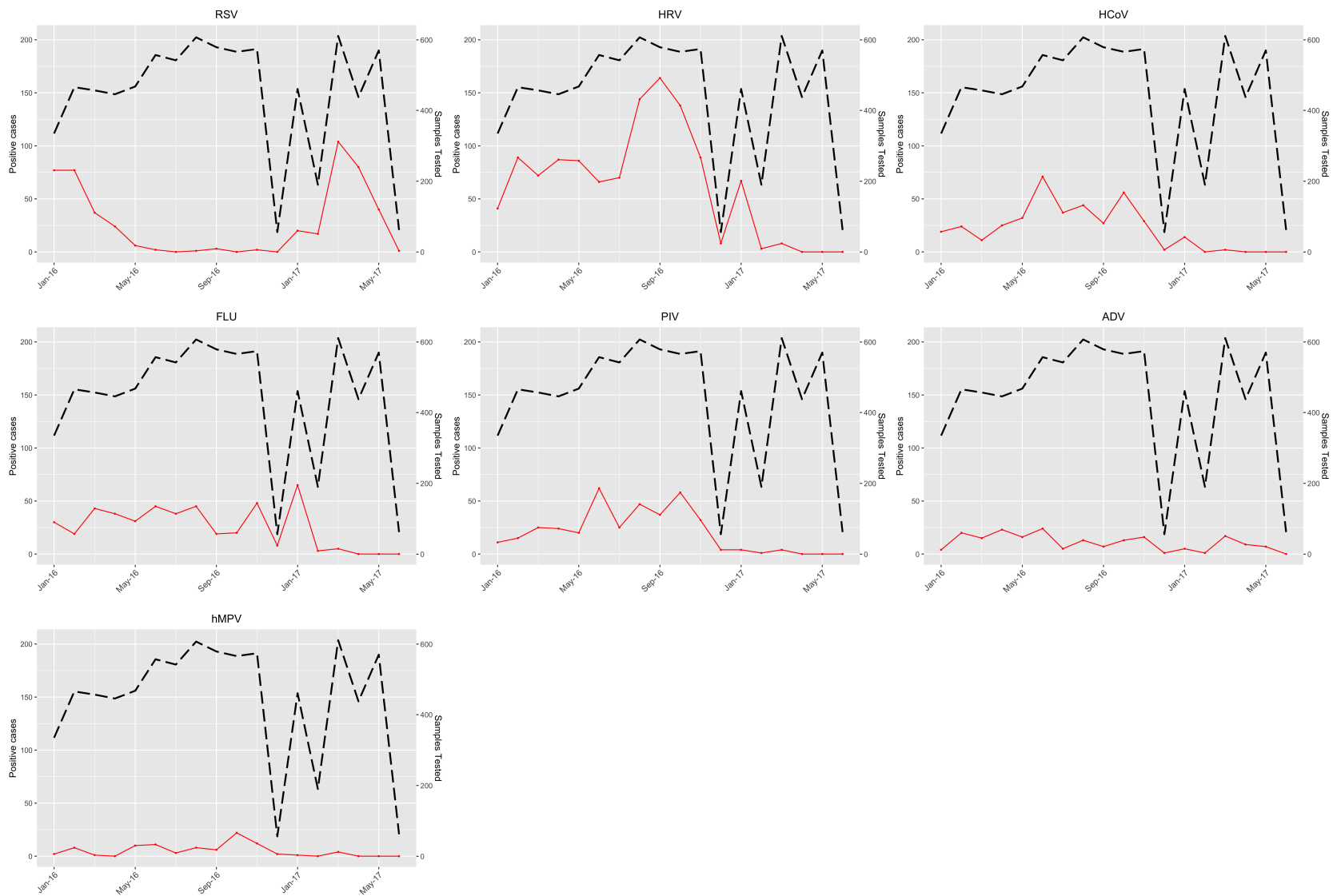
Figure 2.2: Panel of graphs showing the trends of each virus pathogen. The primary y-axis denotes the monthly numbers positive cases for each virus pathogen shown by the red solid line. The secondary y-axis denotes the number of samples tested shown by the black dashed line.
