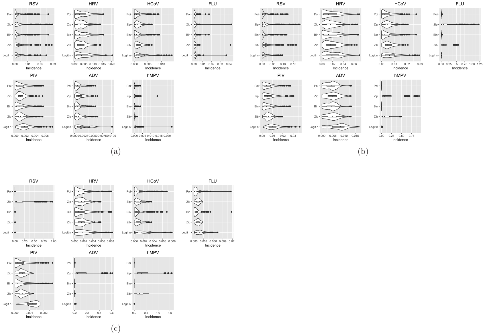
Figure 4.6: Panel of violin plots showing the estimated incidence rates by virus pathogen tested from each model fitted on the data. The panel plots are presented for all ages (a), under 5 year olds (b) and over 5 year olds (c).
