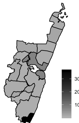
Figure 2.4: Panel of maps showing the estimated prevalence by virus pathogen children aged 0-59 months within the KHDSS.
