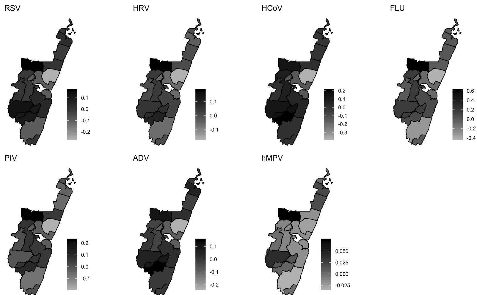
Figure 4.4a: Maps showing the residual spatial locations effects on the incidence rates of viral ARI in Kilifi for all ages
