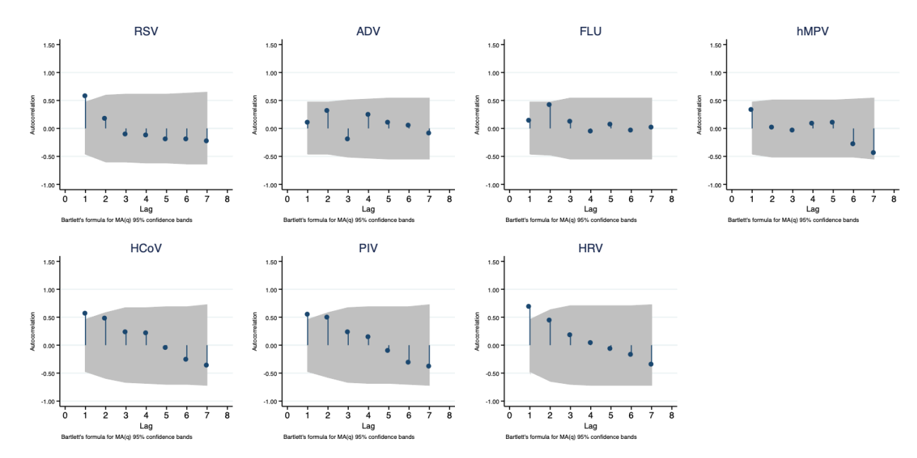
Figure 4.9: Autocorrelation plots for each virus pathogen tested in Kilifi.
