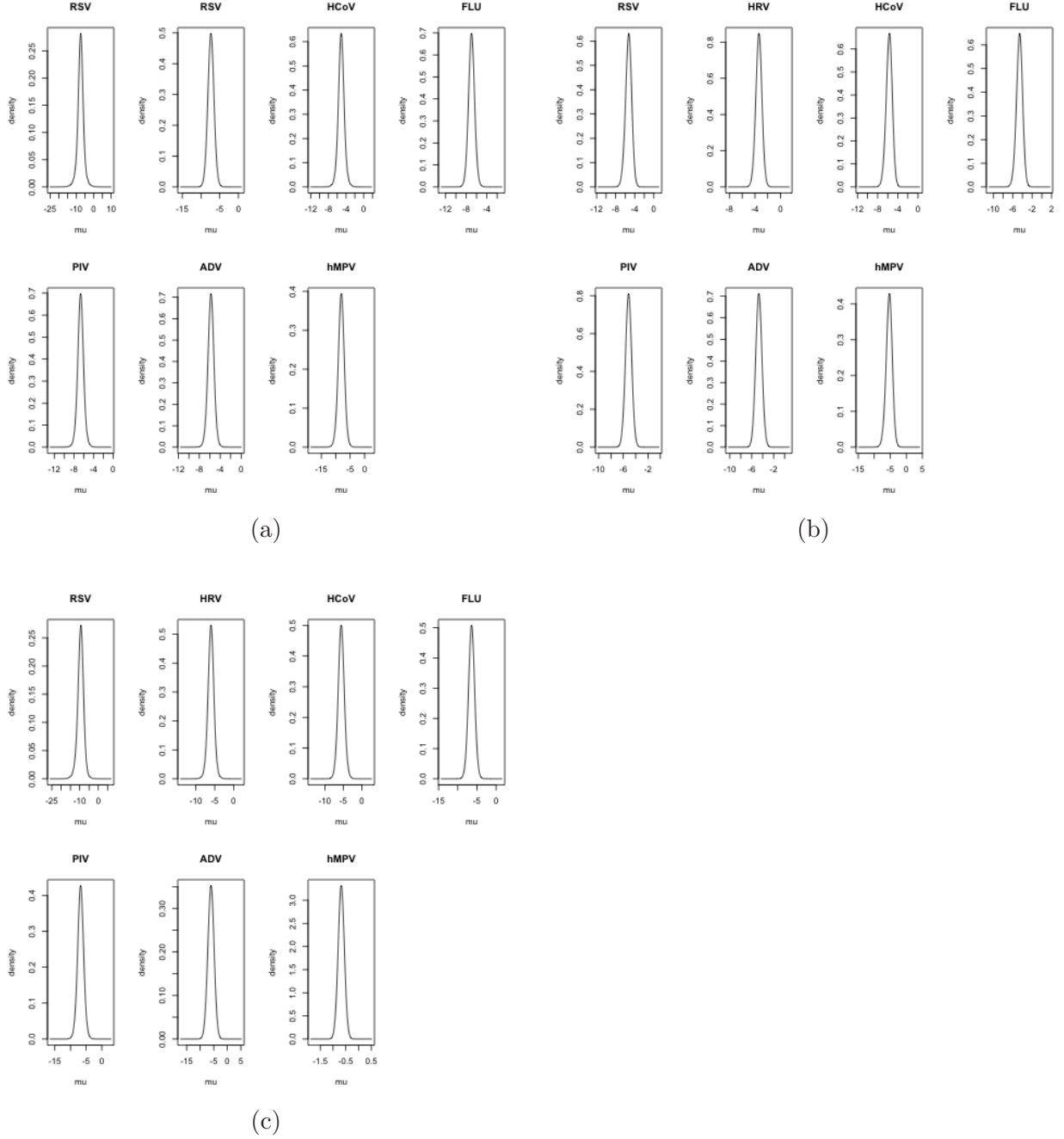
Figure 4.8: Panel of posterior density plots from models used to estimate incidence rates by virus pathogen tested. The panel plots are presented for all ages (a), under 5 year olds (b) and over 5 year olds (c).
