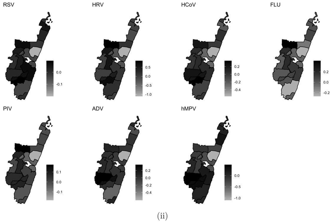
Figure 4.4b: Panel of maps showing the residual spatial locations effects on the incidence rates of viral ARI in Kilifi for under 5 year olds (i) and over 5 year olds (ii).
