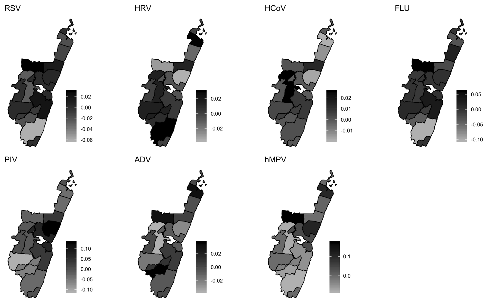
Figure 4.3a: Maps showing the residual spatial locations effects on the prevalence of viral ARI in Kilifi for all ages
