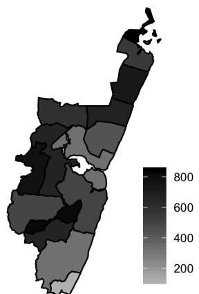
Figure 2.6: Panel of maps showing the estimated incidence rates per 100000 population by virus pathogen for children aged 0-59 months within the KHDSS.
