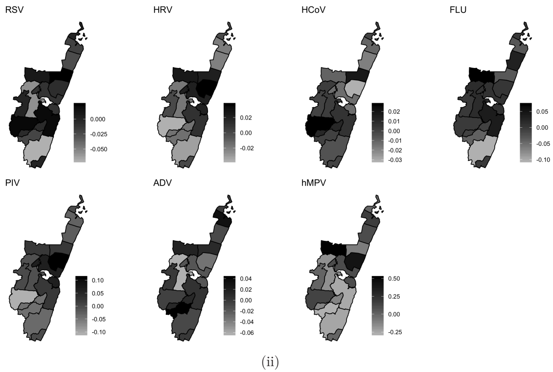
Figure 4.3b: Panel of maps showing the residual spatial locations effects on the prevalence of viral ARI in Kilifi for under 5 year olds (i) and over 5 year olds (ii).
