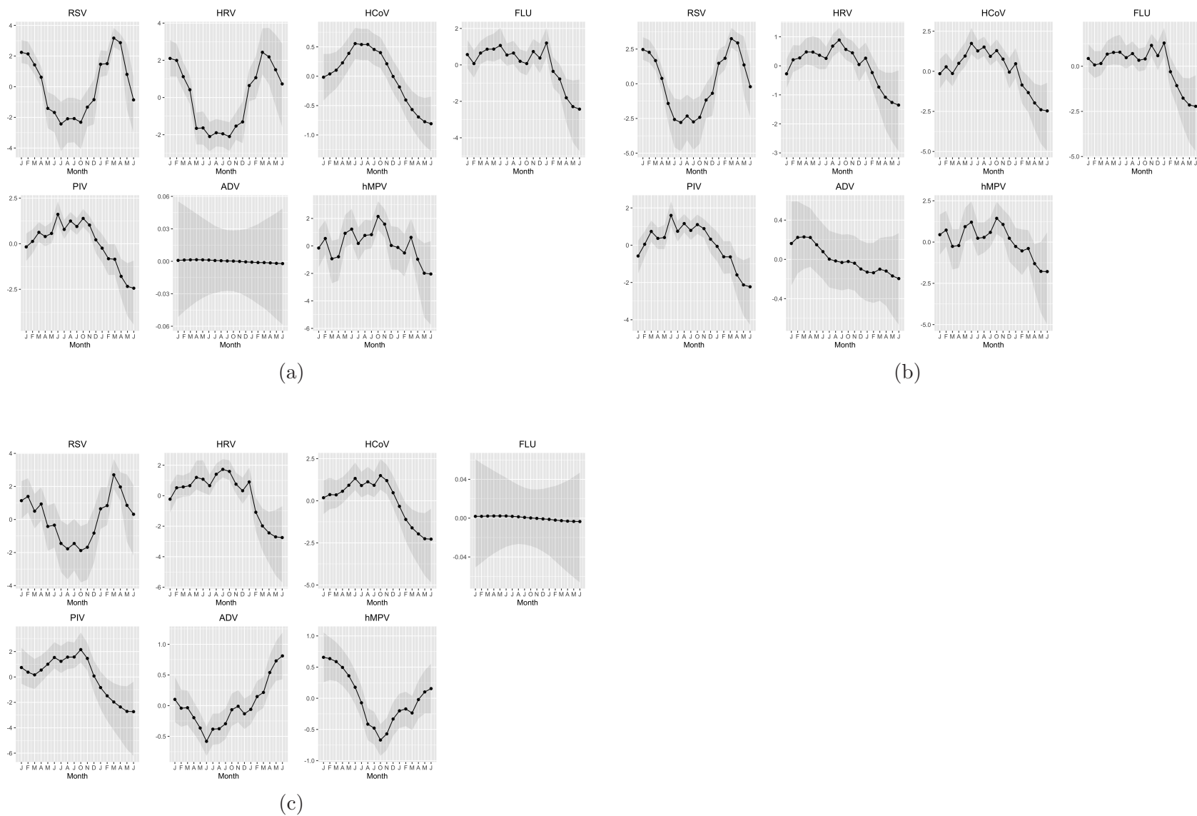
Figure 4.2: Panel of graphs showing non-linear effects of time in months on the incidence of viral ARI for all ages (a), under 5 year olds (b) and over 5 year olds (c). Shown are the posterior means together with 95intervals.
