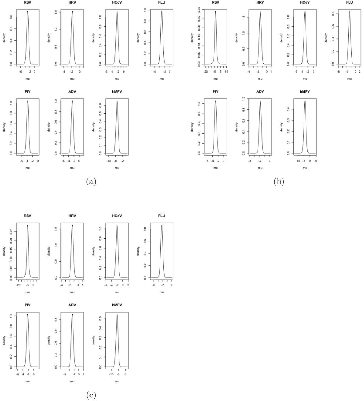
Figure 4.7: Panel of posterior density plots from models used to estimate ARI prevalence by virus pathogen tested. The panel plots are presented for all ages (a), under 5 year olds (b) and over 5 year olds (c).
