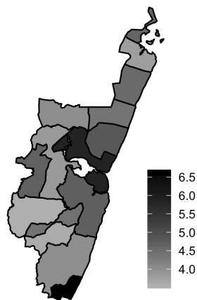
Figure 2.4: Panel of maps showing the estimated prevalence by virus pathogen children aged 0-59 months within the KHDSS.
