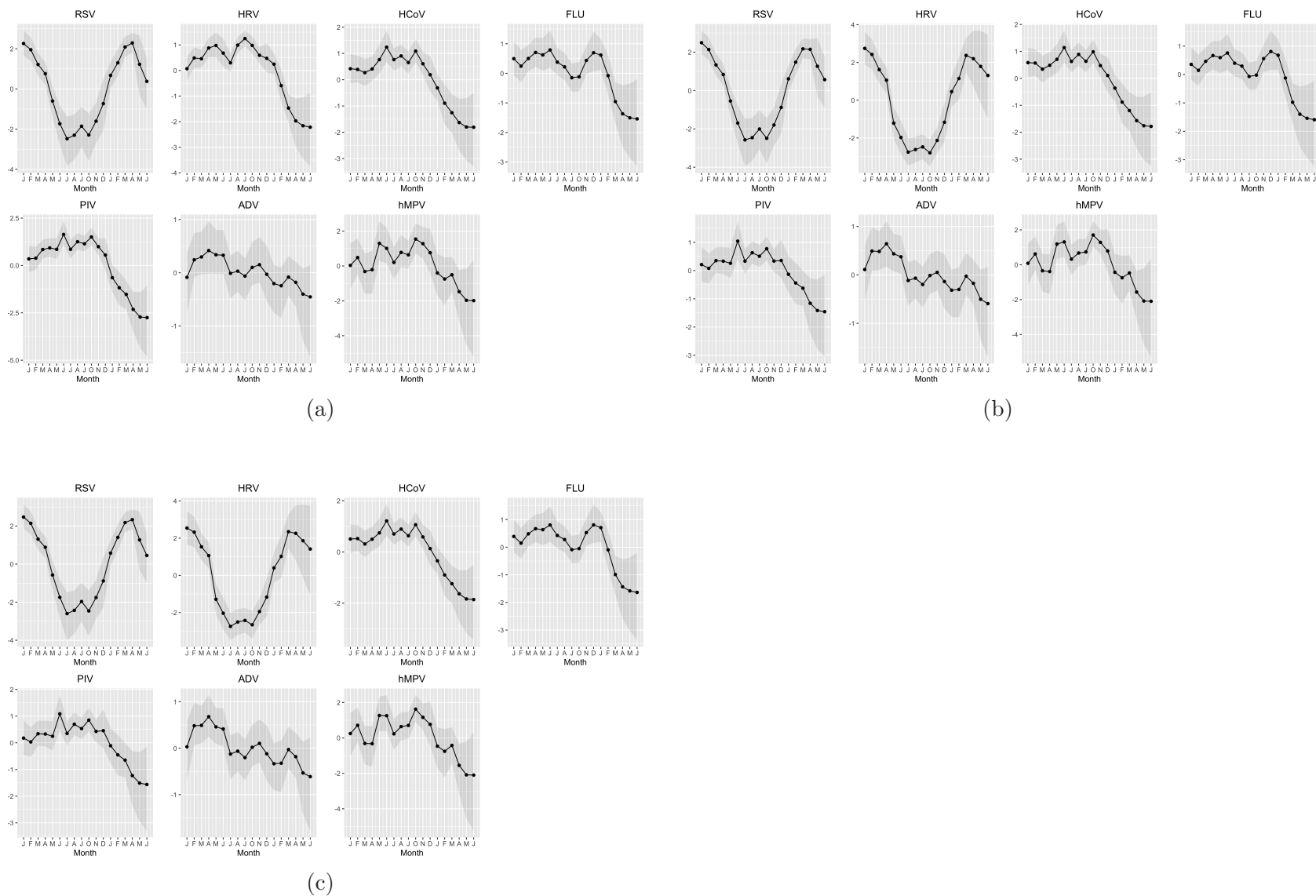
Figure 4.1: Panel of graphs showing non-linear effects of time in months on the prevalence of viral ARI for all ages (a), under 5 year olds (b) and over 5 year olds (c). Shown are the posterior means together with 95intervals.
