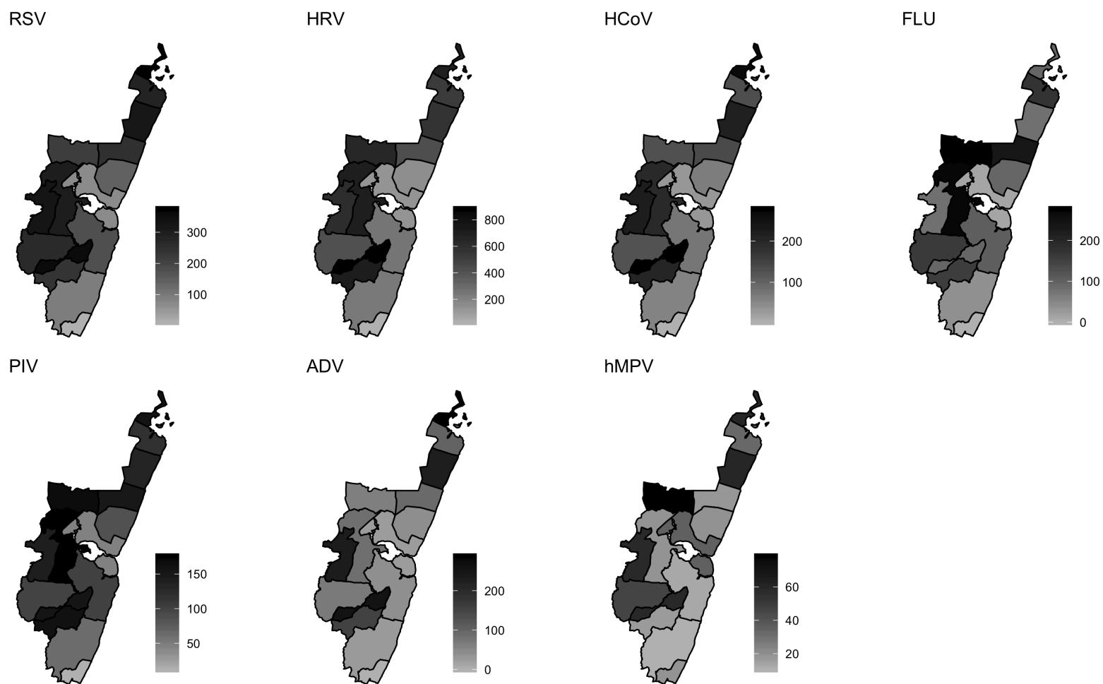
Figure 2.5: Panel of maps showing the estimated incidence rates by virus pathogen for all ages within the KHDSS.
