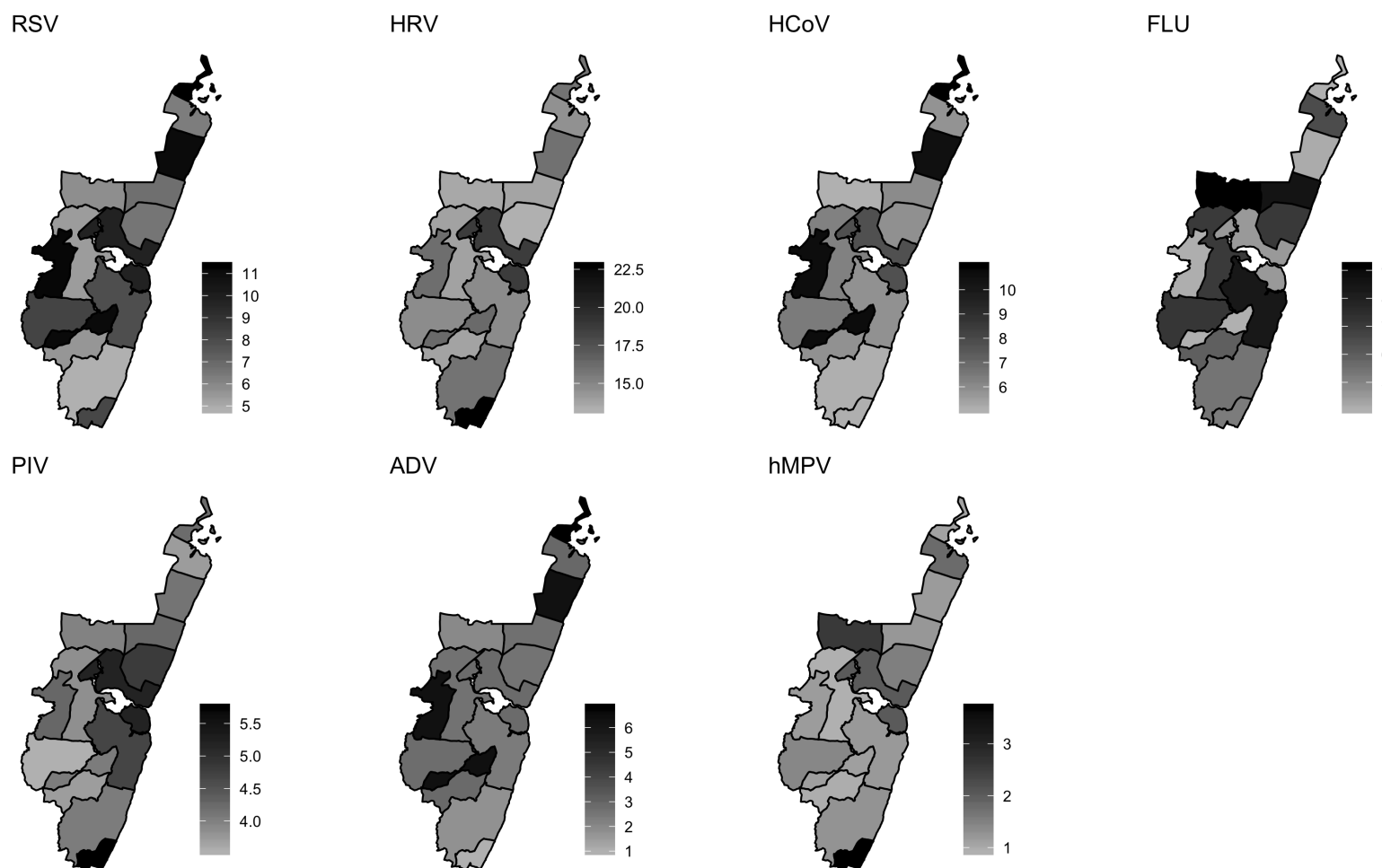
Figure 2.3: Panel of maps showing the estimated prevalence by virus pathogen for all ages within the KHDSS.
