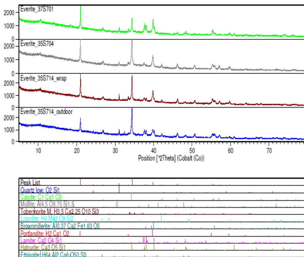
Figure B1: Quantitative XRD spectra ,for batches 37S701, 35S704 and 35S714, of fibrecement sheets incorporated with 3% kaolin, cured under different conditions – indoors unwrapped (green, black), indoors wrapped (brown) and outdoors (blue).
