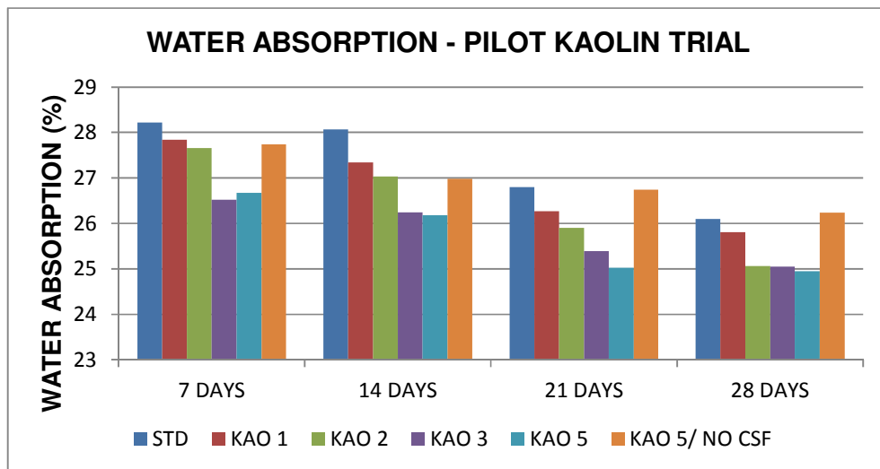
Figure 6.5: Comparison of water absorption for fibrecement composites with different kaolin replacement levels.
