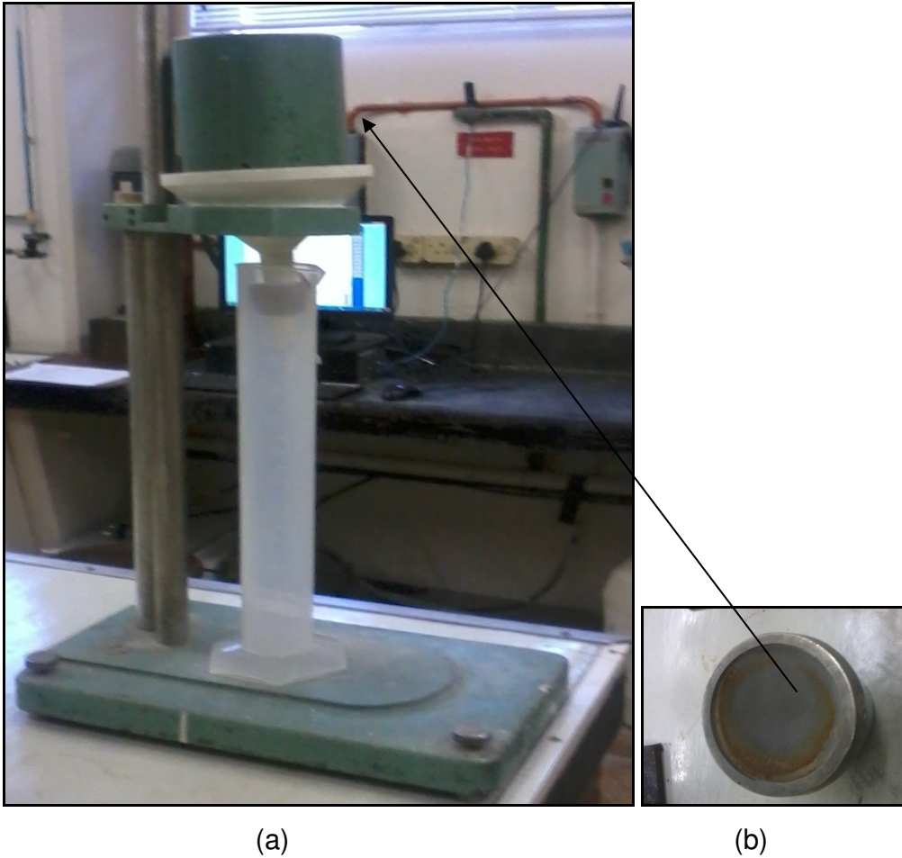
Figure 2.10: (a) Equipment used for flocculant selection, simulating the loss of solids at the sieves, (b) bottom of the container with a 45 mesh sieve
