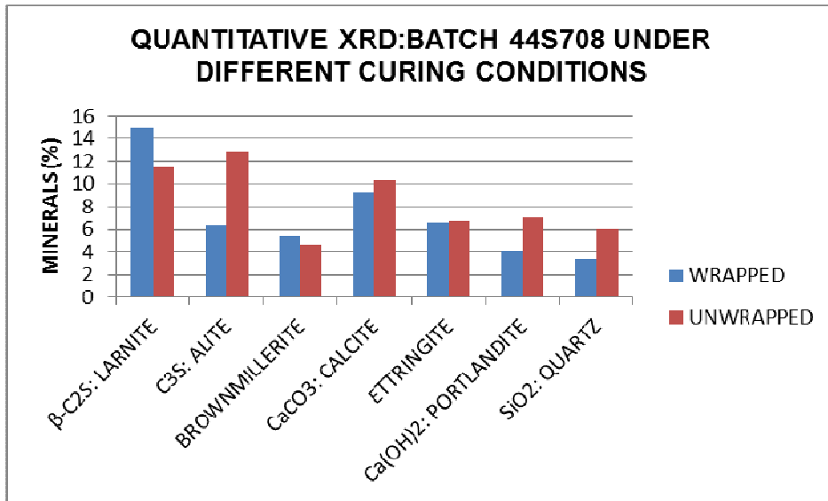
Figure 6.49: Quantitative XRD analysis for corrugated sheets incorporated with kaolin at 21 days curing under different conditions.
