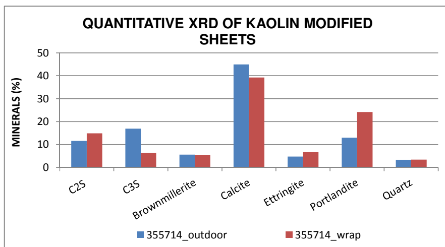
Figure A5: Minerals formed during the hydration process of kaolin modified sheets under different curing conditions.
