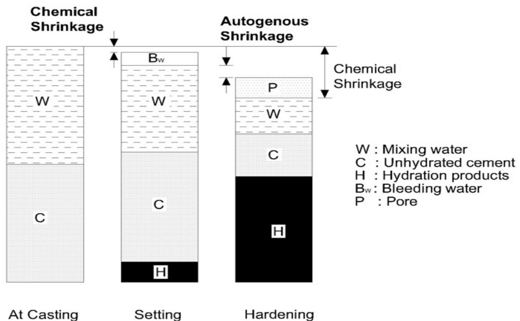
Figure 1.1: Chemical shrinkage and autogenous shrinkage of concrete [adapted after Mihashi and Leite (2004)]
