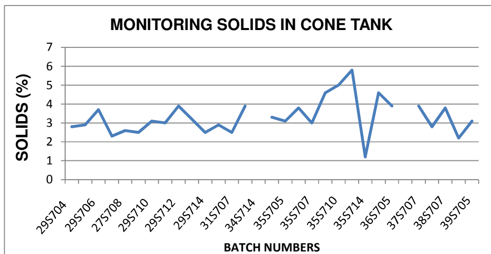
Figure 6.25: Monitoring solids during production of 3% kaolin modified corrugated fibreceement sheets.
