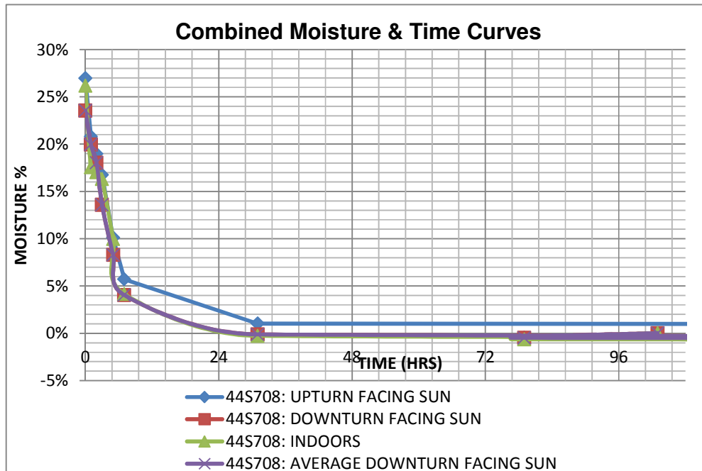
Figure 6.50: Evaluation of the rate of moisture loss in corrugated sheets under different curing conditions.
