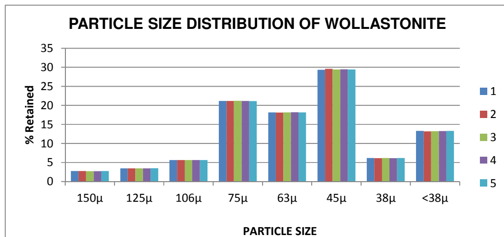
Figure 2.15: Particle size distribution of five samples of wollastonite
