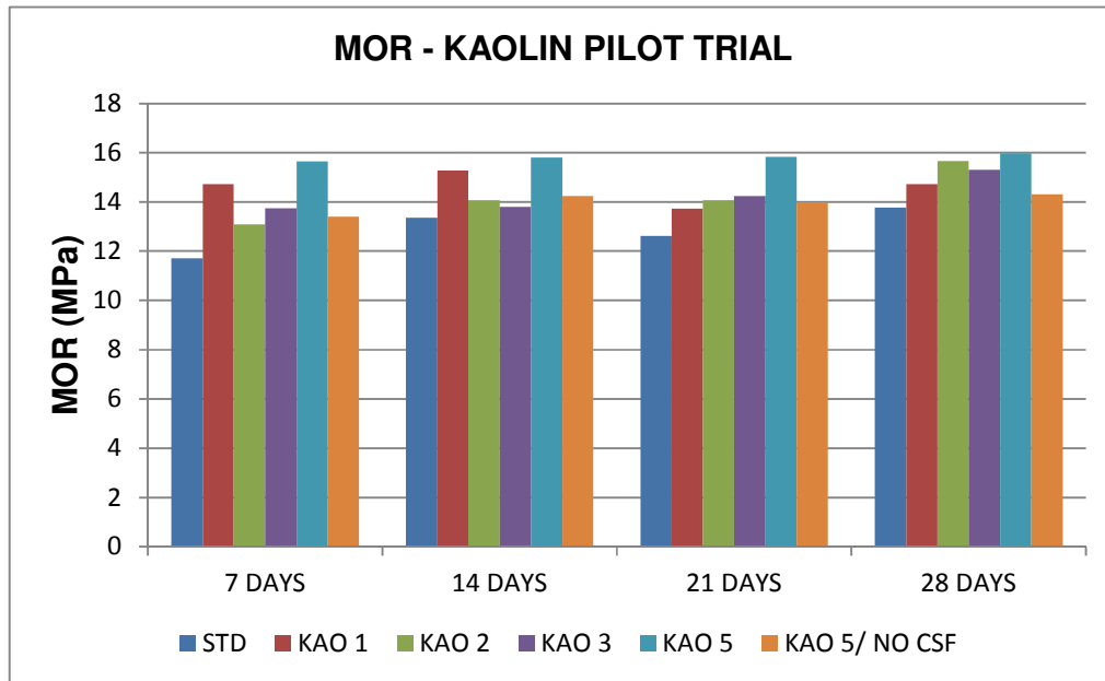
Figure 6.7: Strength development in kaolin-incorporated fibre-cement composites with age
