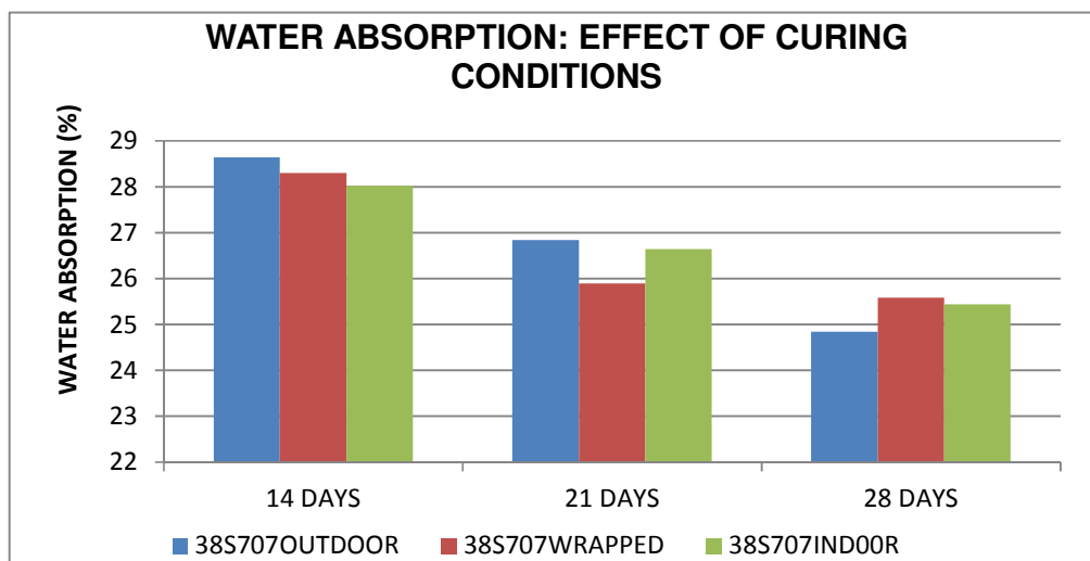
Figure 6.37: Effect of various curing conditions on water absorption of corrugated sheets with 3% kaolin inclusion as cement substitute.
