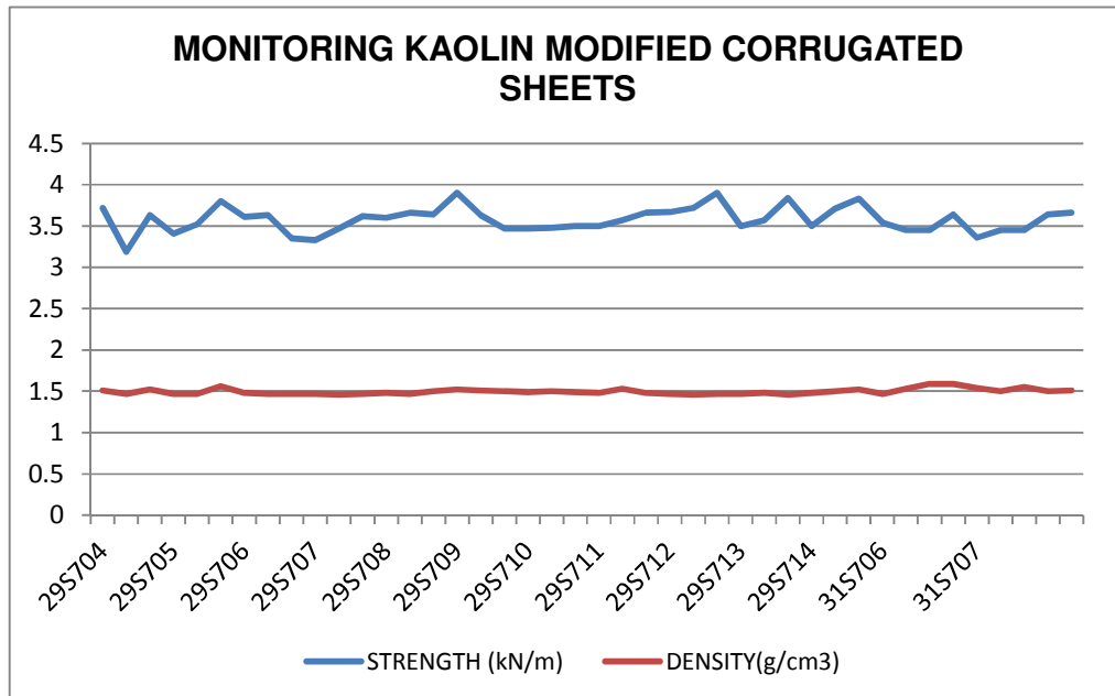
Figure 6.26: Monitoring mechanical properties of 3% kaolin modified corrugated fibreceement sheets, tested at 14 days curing.
