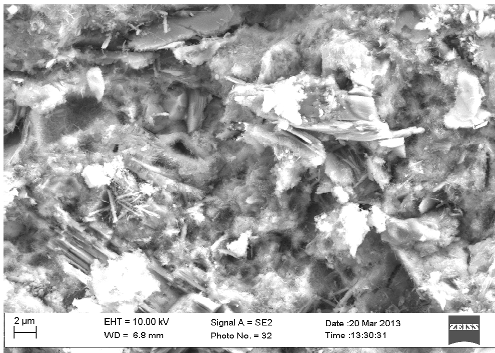
Figure C2: SEM micrographs for kaolin modified fibrecement sheets, production batch 35S704 stored indoors for 14 d before external exposure.
