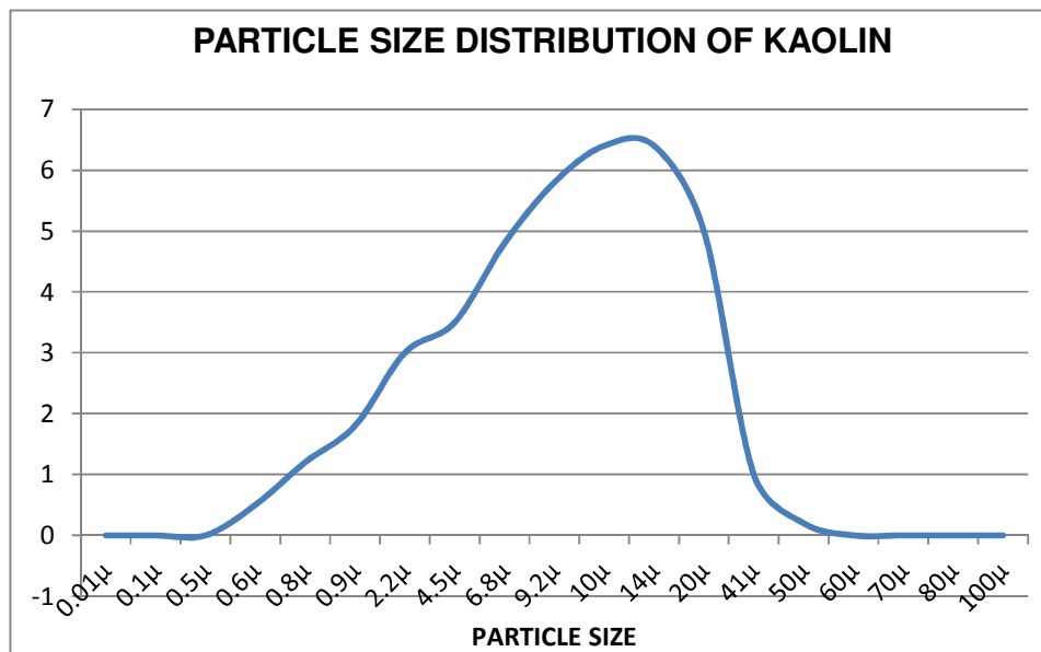
Figure 2.17: Particle size distribution of kaolin
