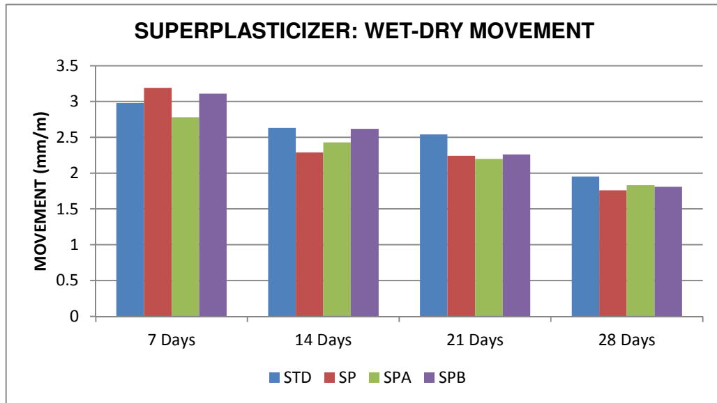
Figure 5.5 Movement of composite with superplasticizer after exposure to wet immersion for 24 h followed by 24 h drying during a testing interval
