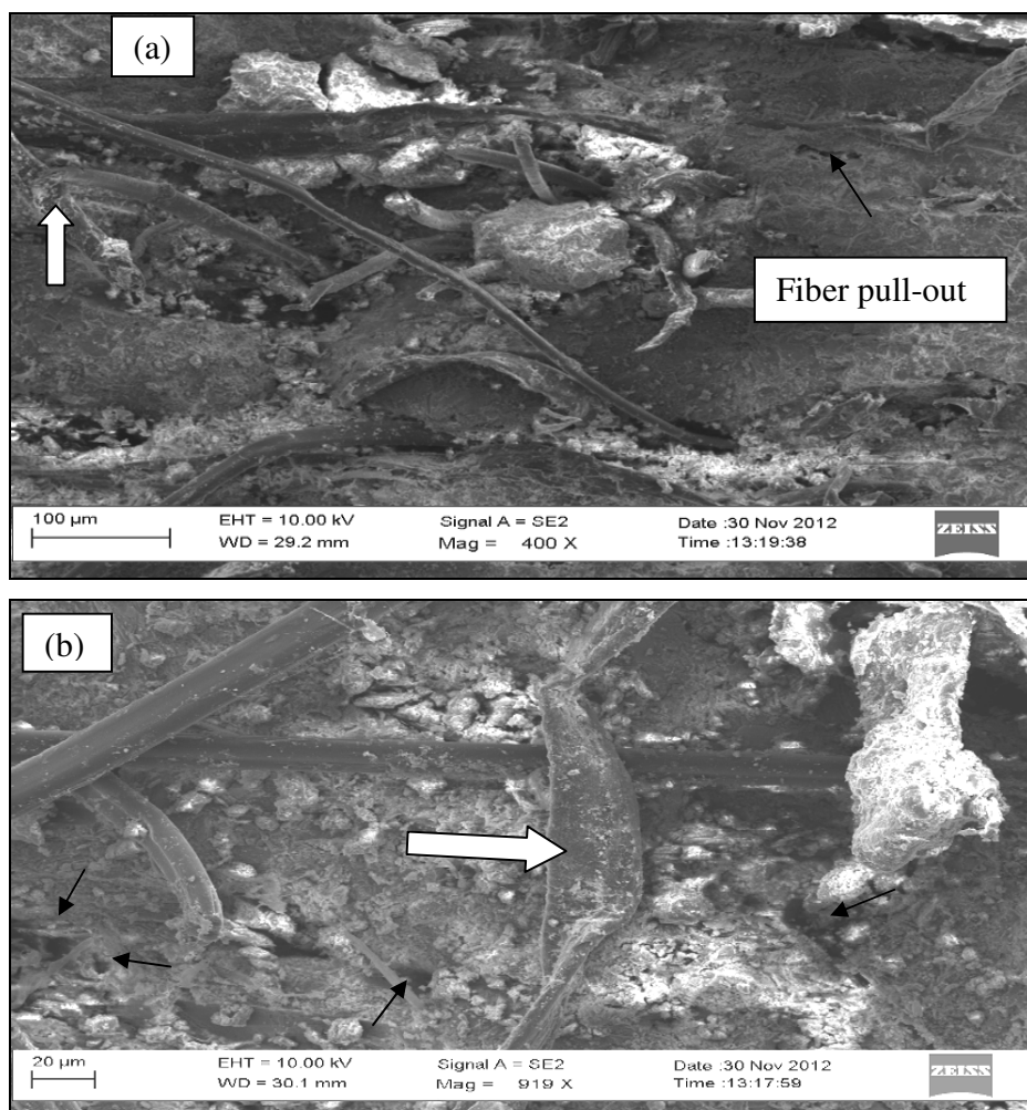
Figure 6.19: (a) and (b) SEM micrographs of corrugated sheets with standard formulation 4 months curing under natural weathering exposure
