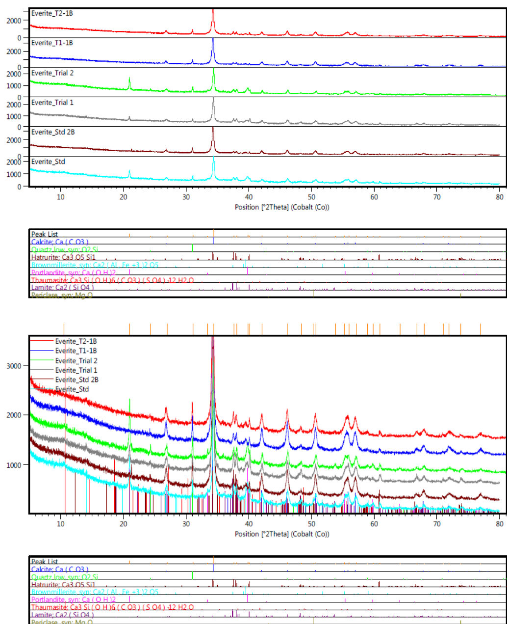
Figure B3: Quantitative XRD spectra of the first production trial of kaolin modified sheets, standard, trial 1 (3% kaolin), trial 2 (5% kaolin), all cured indoors for 14d thereafter outdoor exposure. The spectra with a B label, at the end, were the sheets subjected to accelerated carbonation.
