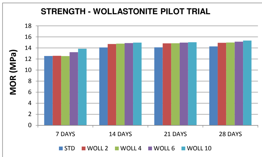
Figure 4.4 Development of strength for wollastonite composites over 28 days
