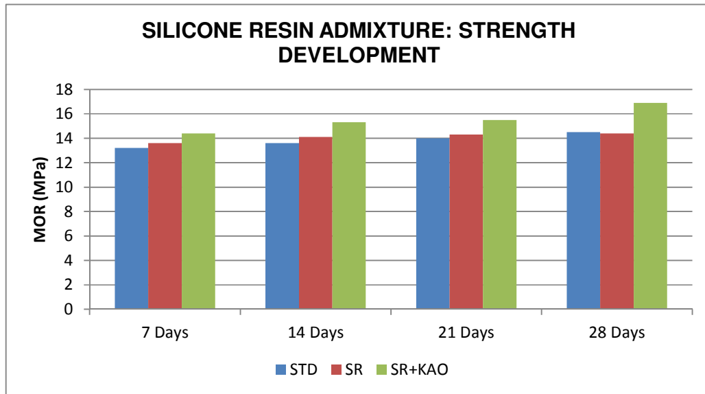
Figure 5.8 Strength development for composites with admixtures with age
