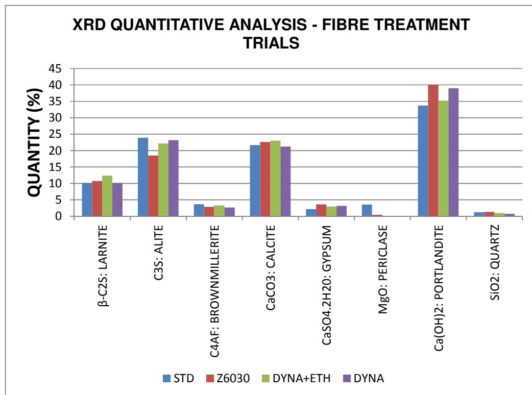
Figure 3.6 Mineralogical composition of cellulose pretreated sheets, 28 days
