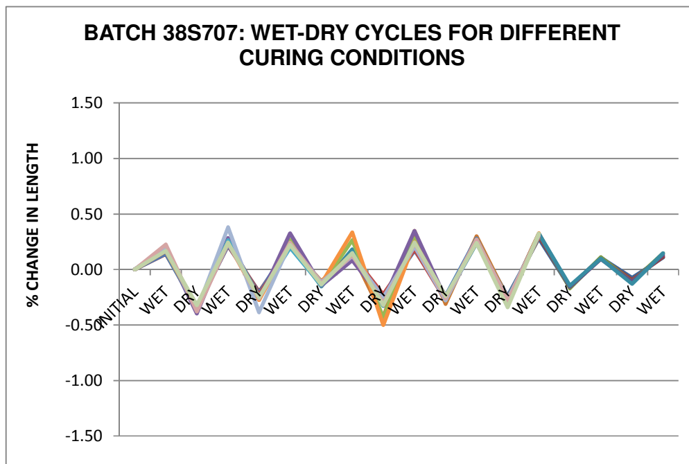
Figure 6.44: Change in length, as a result of wet-dry cycling, of kaolin modified sheets under different curing conditions.
