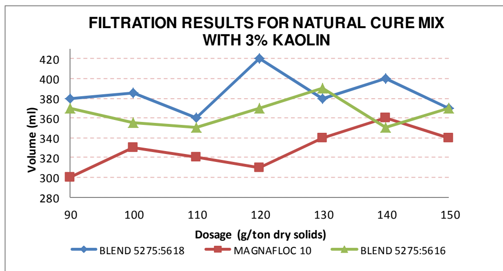
Figure 6.3 Selection of flocculant type and dosage for optimal filtration in the vats. Better filtration achieved with volume greater than 350 ml.
