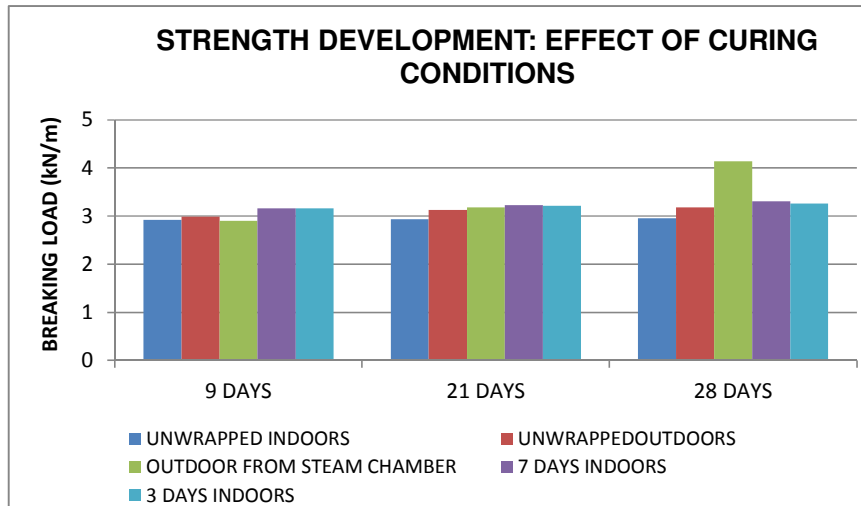
Figure 6.30: Strength development, over time, of kaolin modified sheets cured under different conditions.
