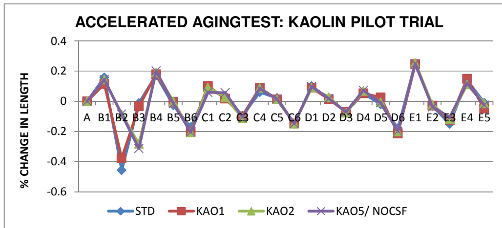
Figure 6.9: Accelerated aging test for kaolin-incorporated fibrecement composites. A- initial measurement, B, C, D, E represent 1 st , 2 nd , 3 rd and 4 th cycles respectively while the numbers 1, 2, 3, 4, 5 and 6 are wet, carbonation, dry, wet, carbonation, dry exposure respectively.
