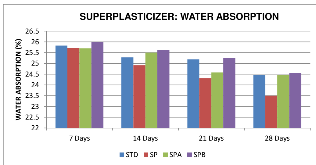
Figure 5.2: Effect of superplasticizer on water absorption of the fibrecement composites over a 28 days curing period
