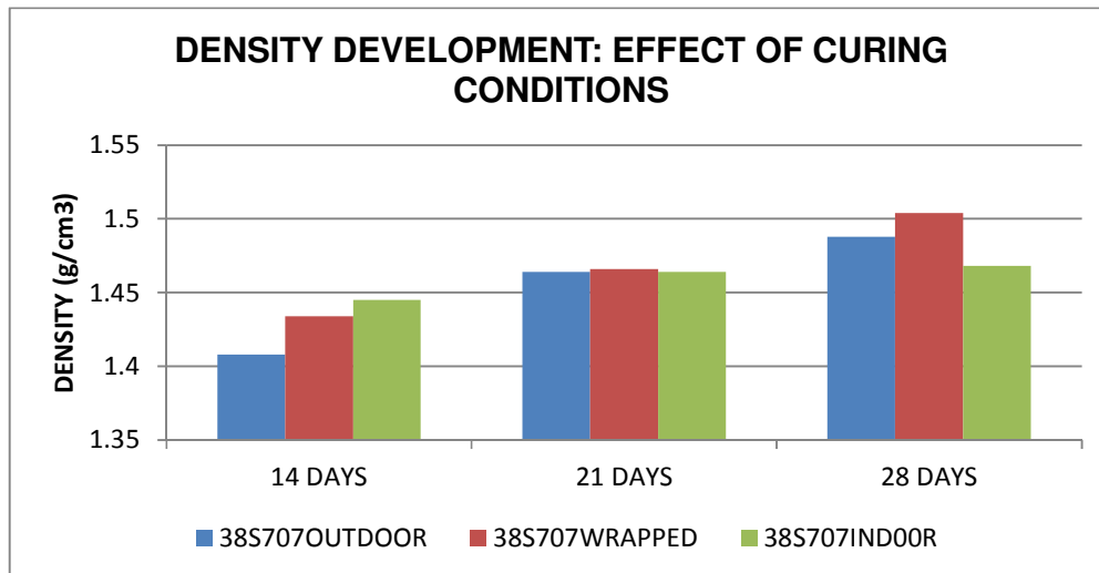
Figure 6.36: Density development of corrugated sheets incorporated with 3% kaolin as cement substitute under different curing conditions.
