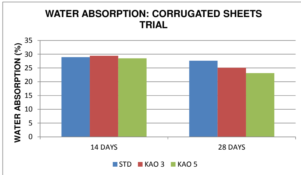
Figure 6.13: Water absorption of corrugated sheets as curing progressed and the impact of kaolin inclusion as replacement of cement.
