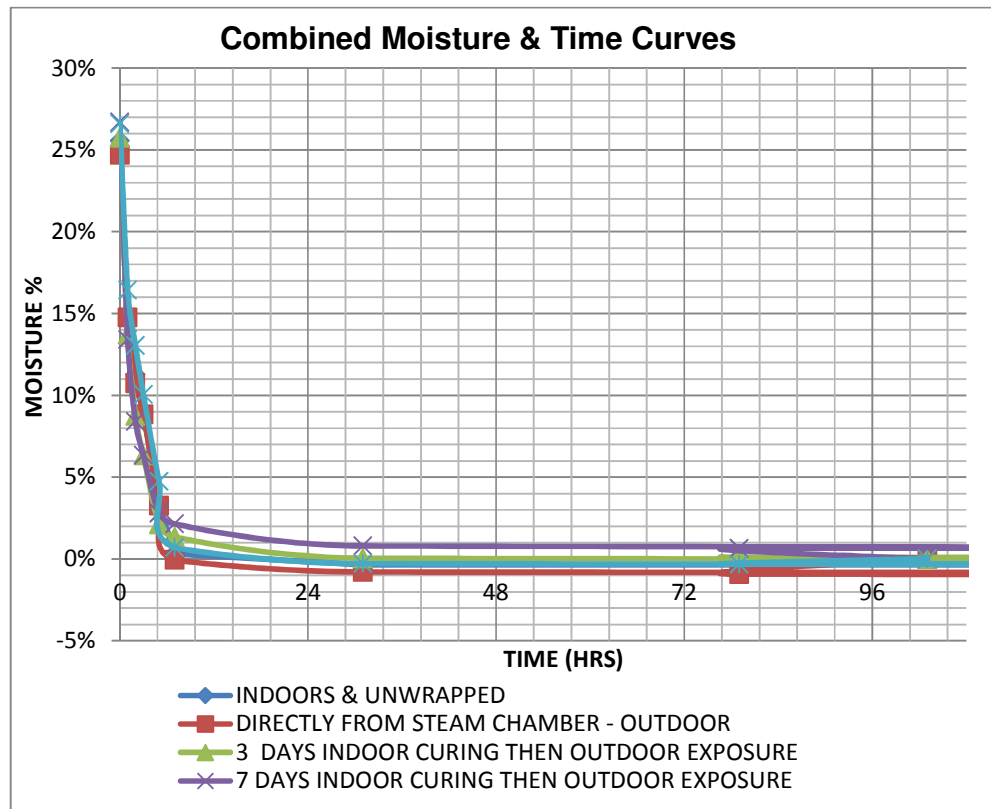
Figure 6.32: Monitoring moisture loss from the sheets, cured under different conditions, with time.
