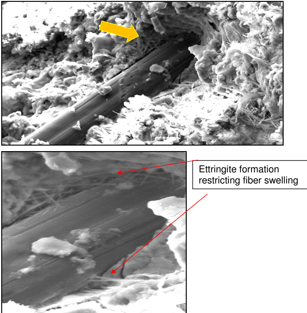
Figure 6.45: SEM micrograph showing needle-like ettringite formation which restricts fibre swelling, below insert of the area shown by the arrow.
