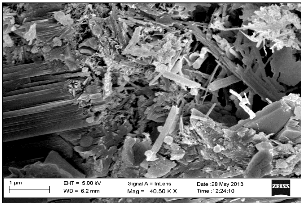
Figure 6.58: SEM micrograph showing ettringite crystal
