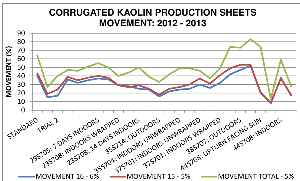
Figure A3: Movement measured in all the 3% kaolin incorporated fibrecement corrugated sheets produced between 2012 and 2013. The results demonstrated that this curve can be used for prediction of cracking
