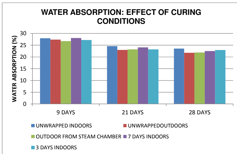
Figure 6.29: Water absorption of sheets with 3% kaolin, as replacement of cement, under different curing conditions for 28 days.
