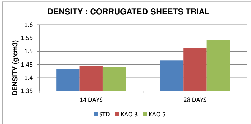
Figure 6.12: Density development of kaolin-incorporated corrugated fibrecement sheets, over 28 days curing
