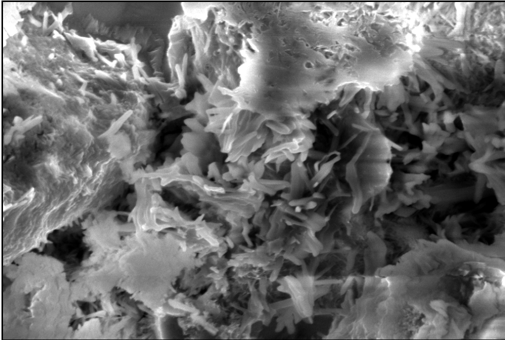
Figure 6.59: SEM micrograph of kaolin modified corrugated sheets illustrating presence of CSH and CaCO 3 .
