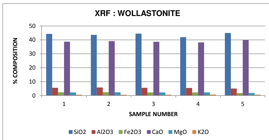
Figure 2.14: Chemical composition of five wollastonite samples received during testing
