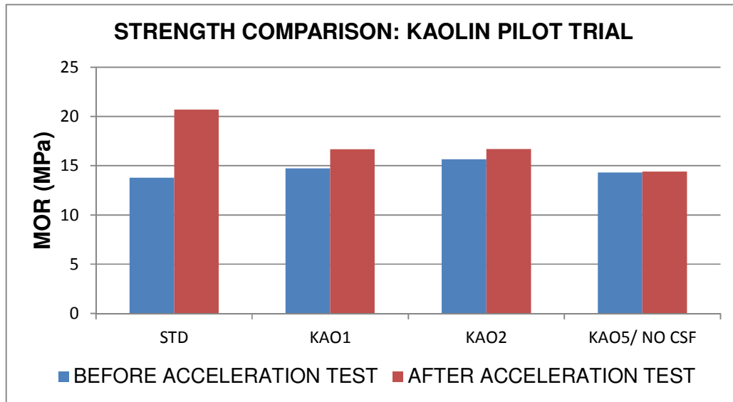
Figure 6.11: Comparison of strength with for kaolin-inclusion fibre cement composites, before and after accelerated aging
