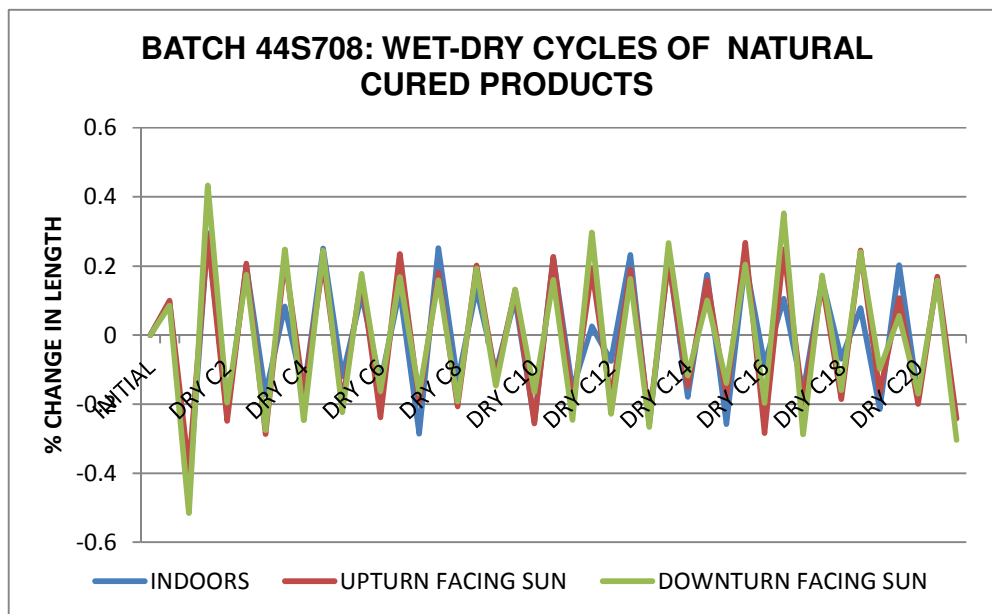
Figure 6.55: Durability test for kaolin modified corrugated sheets, cured under different conditions, subjected to 21 wet-dry cycles.
