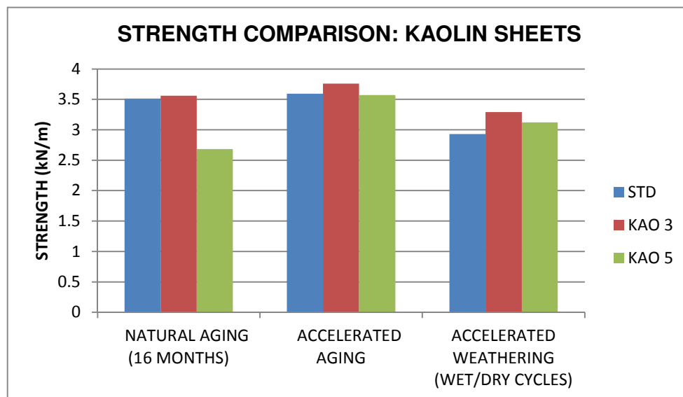
Figure 6.23: Strength comparison between natural exposure and accelerated test results
