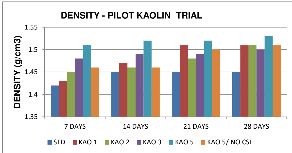
Figure 6.4: The development of density in fibrecement composite mixes with different kaolin replacement levels.
