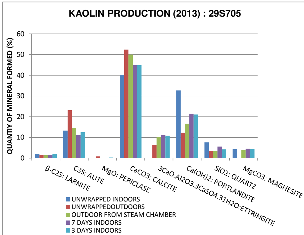
Figure 6.31: Quantitative XRD of fibrecement sheets, 3% kaolin, cured at various conditions.
