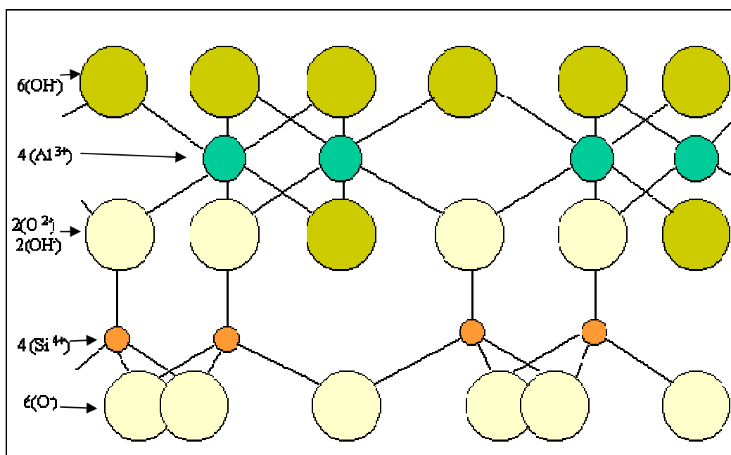
Figure 6.1 Schematic diagram of kaolinite structure
