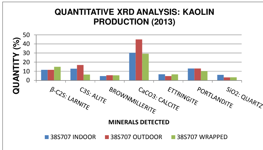
Figure 6.39: Quantitative XRD analysis of corrugated sheets with 3% kaolin as cement substitute identified at 28 days curing.
