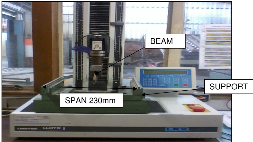
Figure 2.5: Lloyd machine for testing bending strength of flat fibre-cement composites
