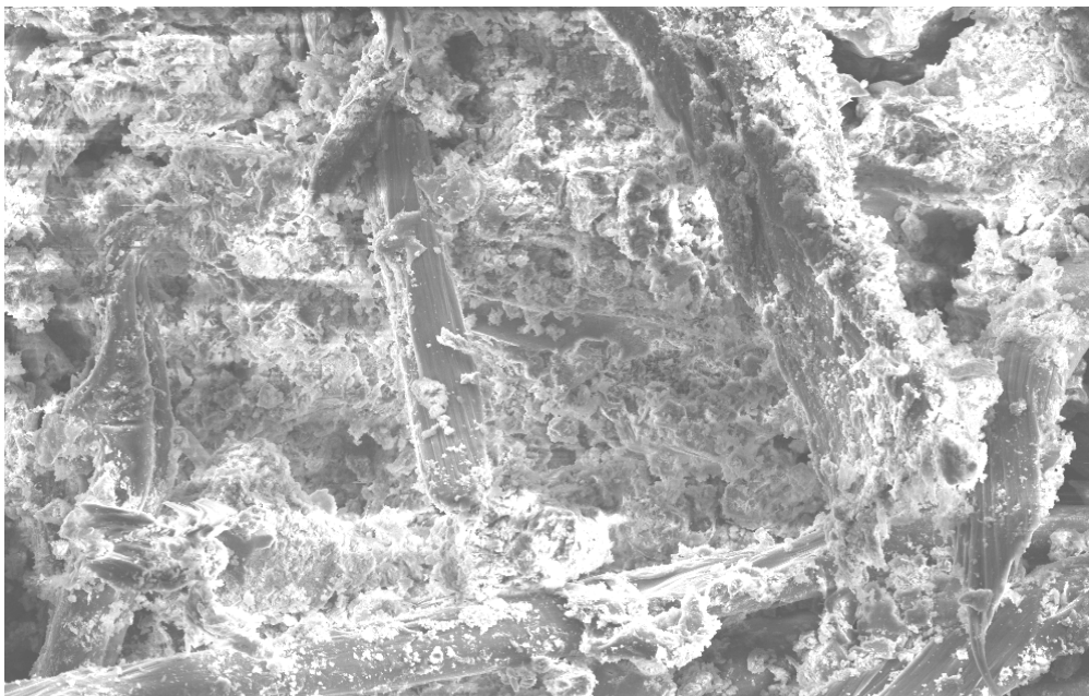
Figure C3: SEM micrographs of kaolin modified fibrecement sheets, batch 35S714 stored indoors unwrapped for 14 d prior to exposure outside.
