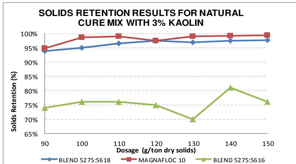
Figure 6.2 Flocculant retention results for fibrecement composite incorporated with 3% kaolin. For optimal performance, solids retention must be higher than 95%.
