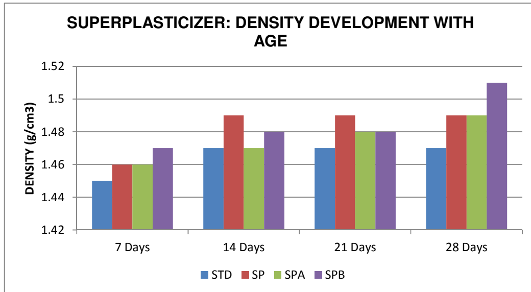
Figure 5.3 Effect of superplasticizer on the density as the fibrecement composites age
