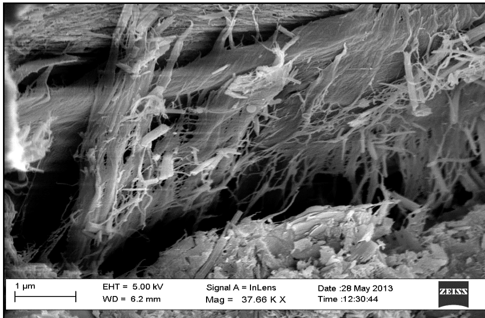
Figure 6.57: SEM micrograph of corrugated sheets indoors
