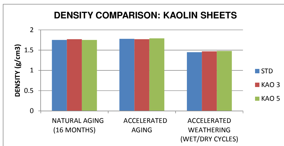
Figure 6.22: Density comparison between natural exposure and accelerated test results
