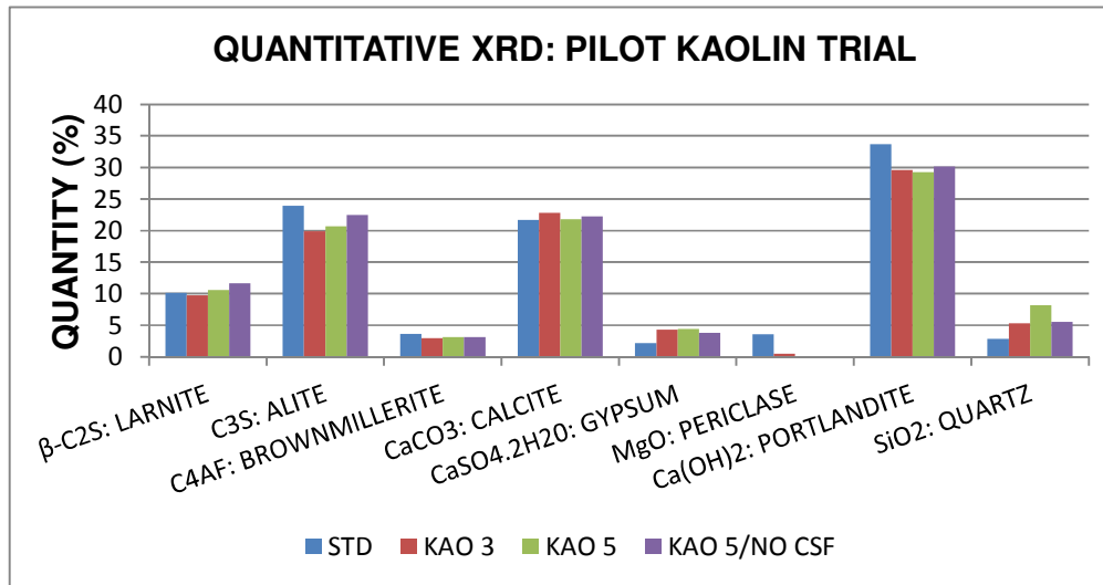
Figure 6.8: Identification of crystal structures in kaolin-incorporated fibrecement composites
