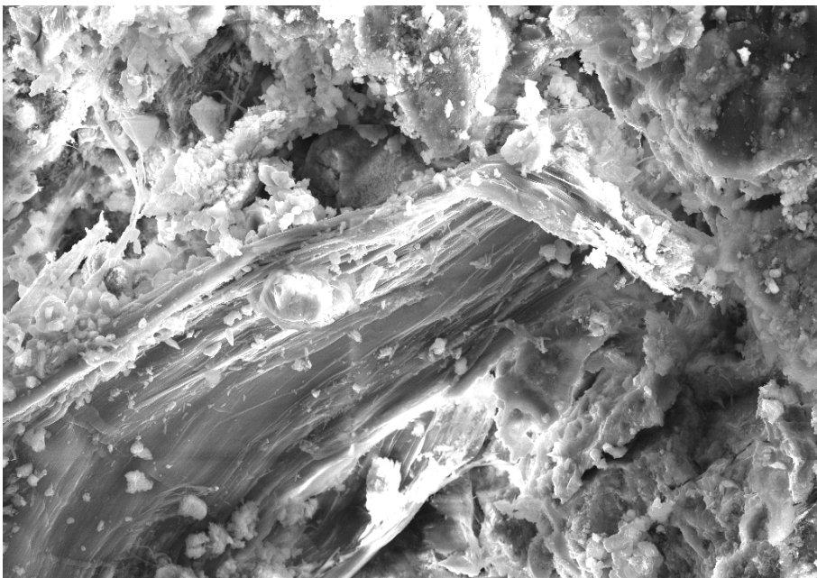
Figure C1: SEM micrographs for the kaolin modified corrugated fibre-cement sheets, batch 37S701, stored indoors for 14 d prior to external exposure.
