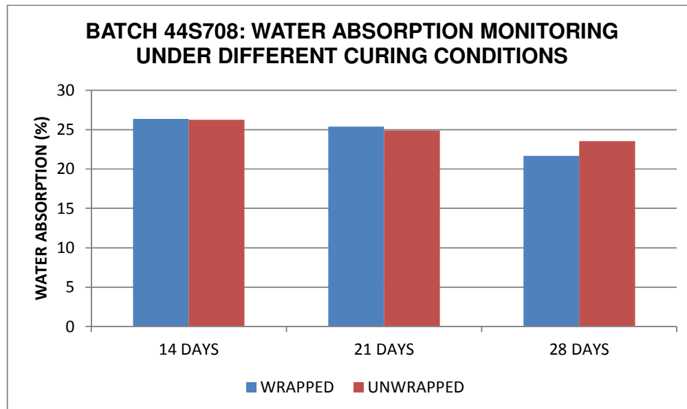
Figure 6.47: Reduction rate of water absorption for kaolin modified corrugated fibrecement sheets, incorporated with 3% kaolin as cement replacement, under different curing conditions.
