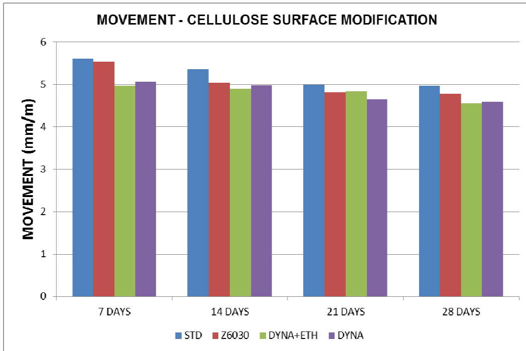
Figure 3.4: Wet-dry movement of cellulose pretreated sheets during curing
