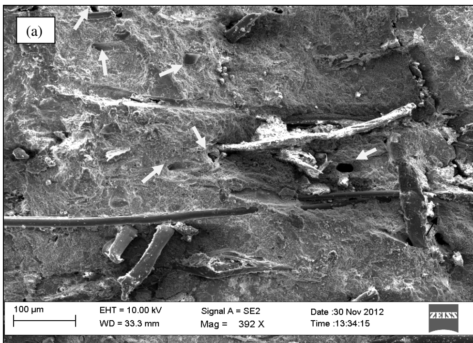
Figure 6.20 (a): SEM micrograph of fibrecement corrugated sheets with 3% kaolin as replacement of cement after 4 months.
