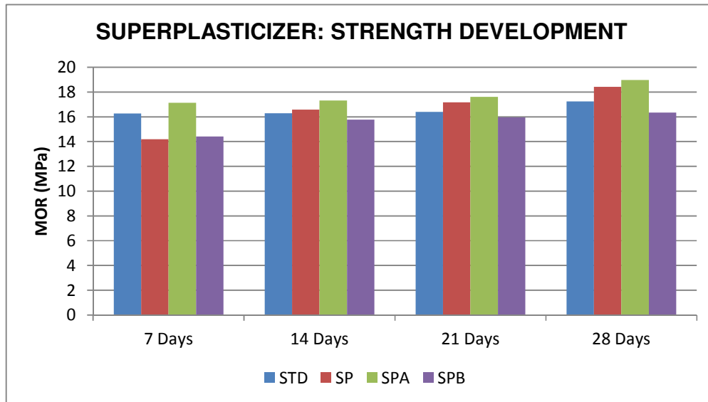
Figure 5.7 Comparison of strength development for standard mix formulation with superplasticizer incorporated mixes during the ageing process
