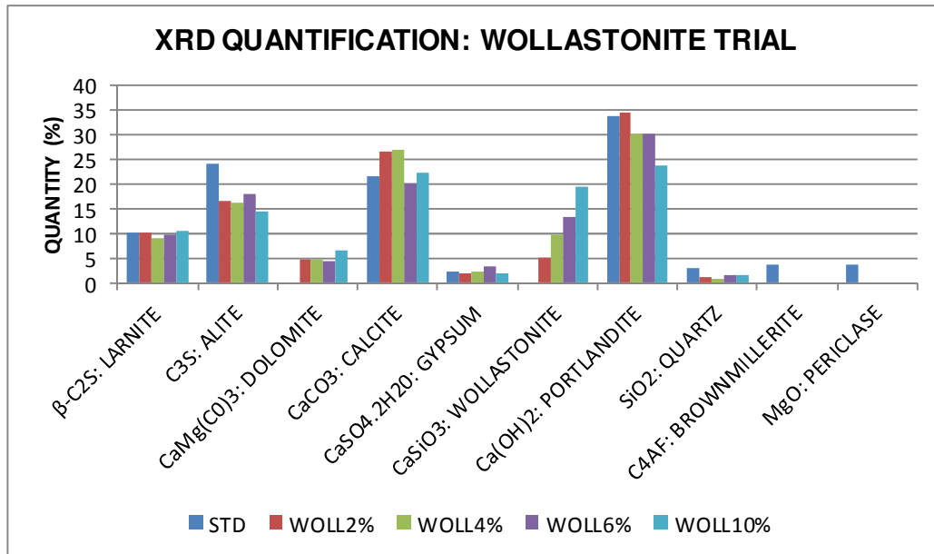
Figure 4.5 Mineralogical composition of wollastonite fibre cement composites at 14 days curing
