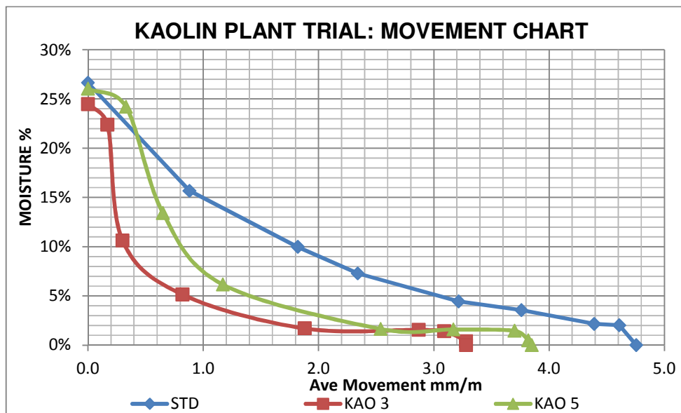
Figure 6.15 (b): Moisture movement in corrugated sheets incorporated with various levels of kaolin as partial replacement of cement
