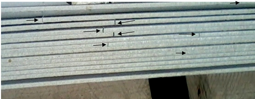
Figure 6.52: Corrugated fibrecement sheets, 3% kaolin replacing cement, with upturn orientated in the direction of highest incidence of solar radiation.
