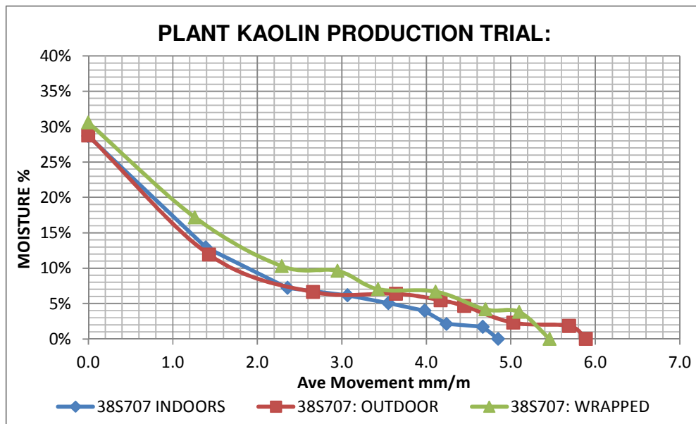
Figure 6.41: Movement determination in kaolin modified sheets with different curing conditions, tested at 22 days.
