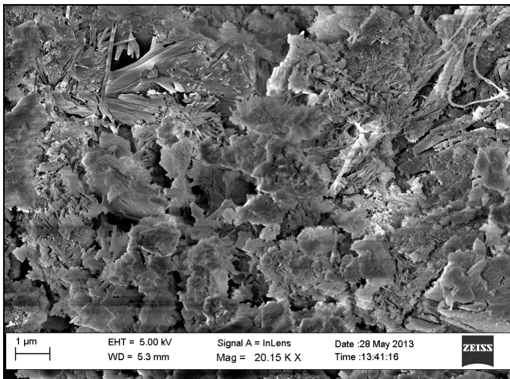
Figure 6.56: SEM micrograph of kaolin modified sheets stored indoors, showing hydration products
