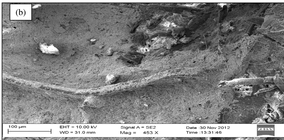
Figure 6.21: Micrographs of corrugated sheets with 5% kaolin inclusion as cement substitute after 4 months natural weathering exposure.
