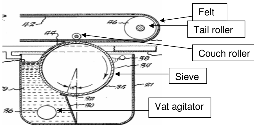
Figure 2.1: Schematic diagram of a vat component
