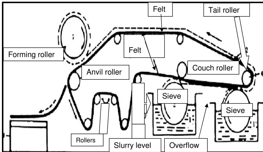
Figure 2.2: Schematic diagram of Hatschek Machine showing principal components
