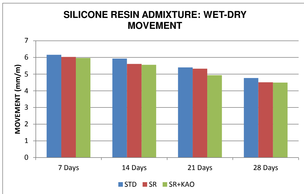
Figure 5.6 Effect of admixture on wet-dry movement of composites over a 28 day curing process
