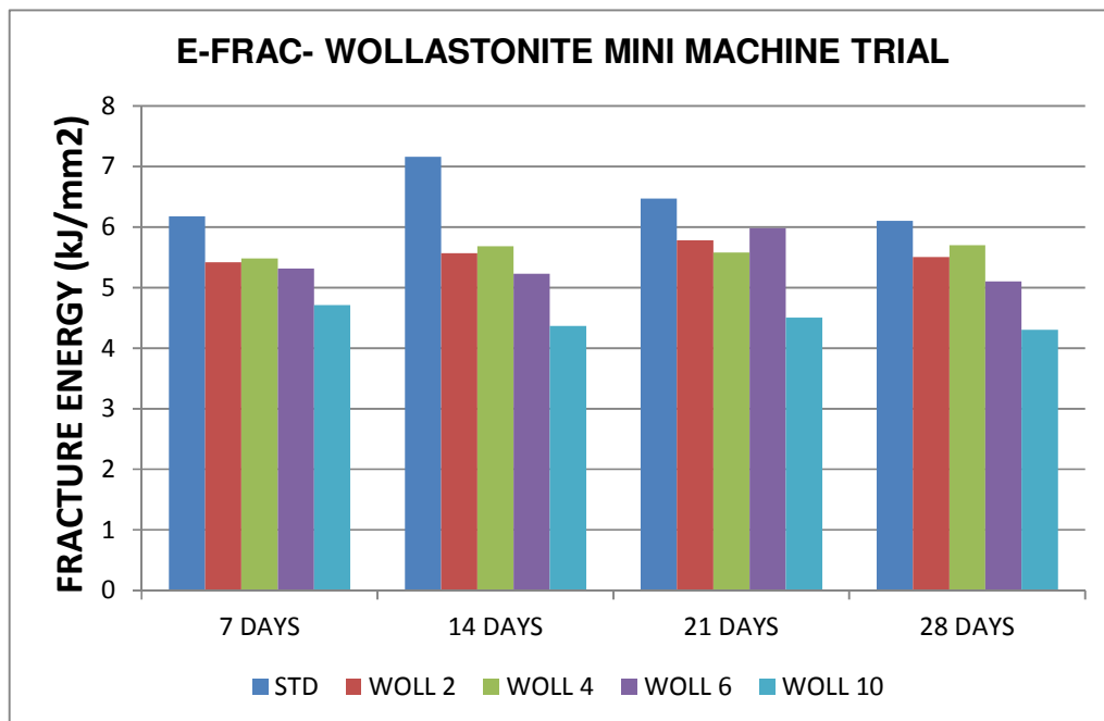
Figure 4.6 Fracture energy of fibre cement composites with different content of wollastonite
