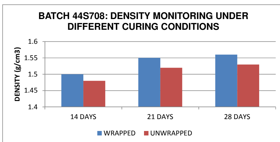
Figure 6.46: Development of density of kaolin modified sheets cured under different conditions, over 28 days.
