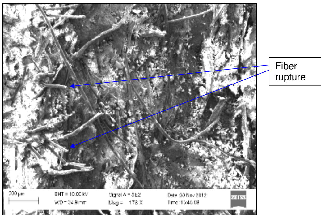
Figure 4.7 SEM micrograph of fibrecement composite incorporated with 6% wollastonite
