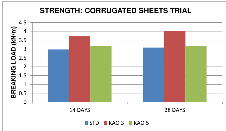
Figure 6.18: Development of strength in corrugated sheets with different kaolin replacement levels over time.
