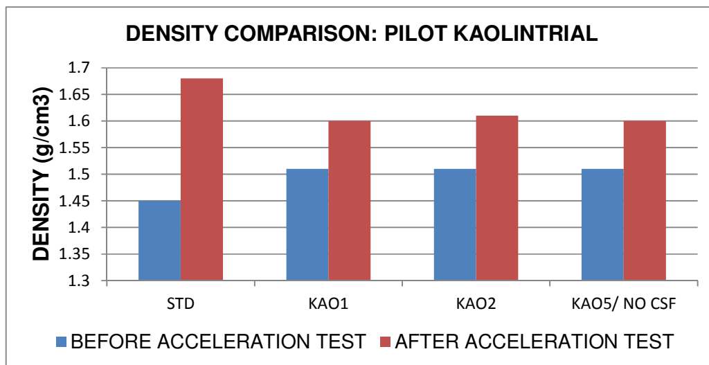
Figure 6.10: Density comparison for fibrecement composites, with various levels of kaolin inclusion, before and after exposure to accelerated aging cycles
