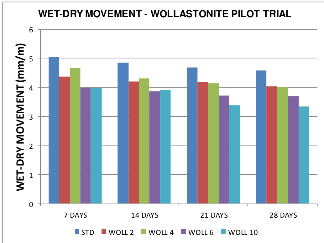
Figure 4.3 Movement curves of wollastonite composites over 28 days curing
