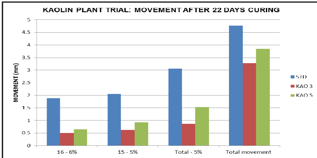
Figure 6.16: Movement of corrugated sheets at different ranges of moisture and the effect of various levels of kaolin to movement
