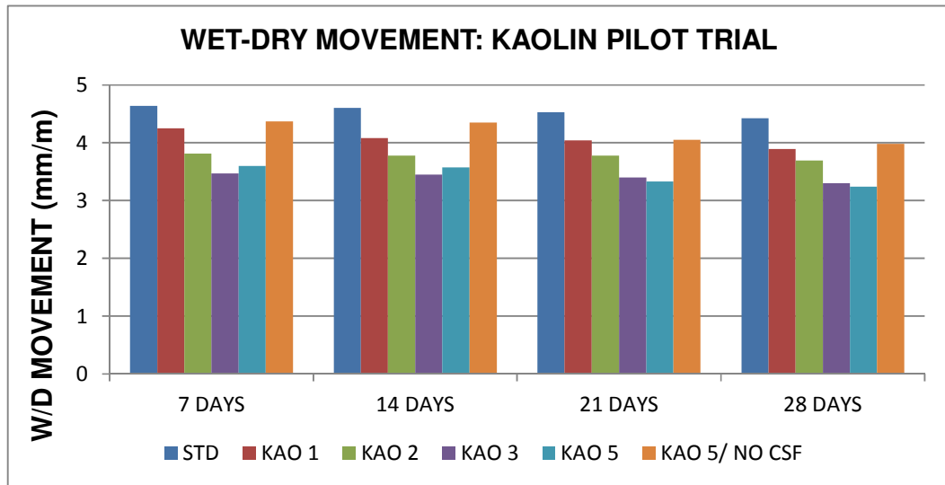
Figure 6.6: Effect of various kaolin levels on the wet-dry movement of fibrecement reinforced composites
