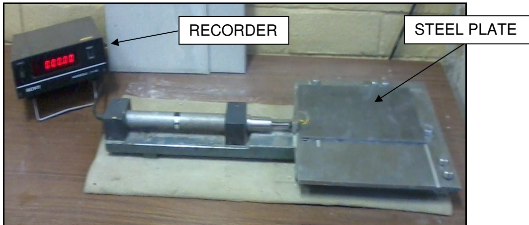
Figure 2.6: Instrument for measuring lengths of fibre cement sheets
