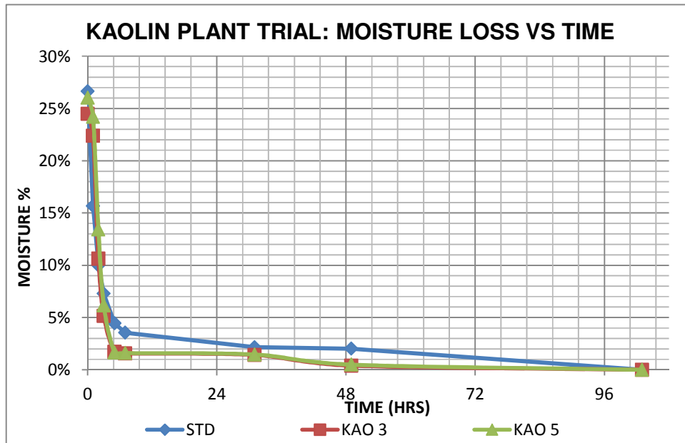
Figure 6.15 (a): Rate of moisture loss for corrugated sheets incorporated with kaolin at various contents.
