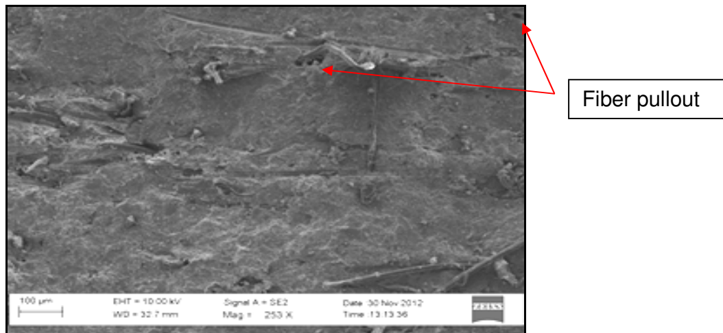
Figure 4.8 SEM micrograph of the control sample without wollastonite
