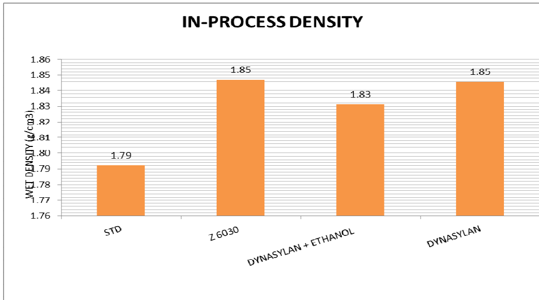
Figure 3.2: Density measurement of green cellulose pretreated sheets during the manufacturing process
