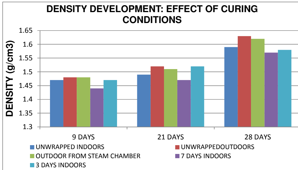
Figure 6.28: Development of density of 3% kaolin modified sheets over time, under various curing conditions
