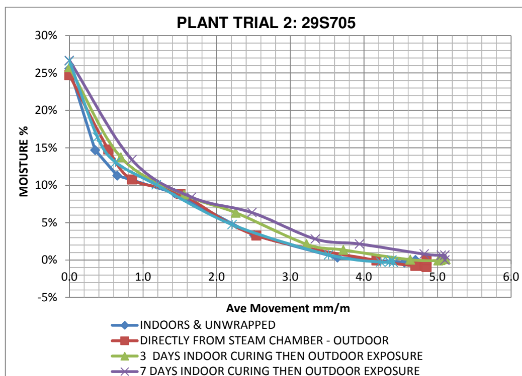
Figure 6.33: Monitoring movement of kaolin modified sheets, under different curing conditions, against moisture loss.
