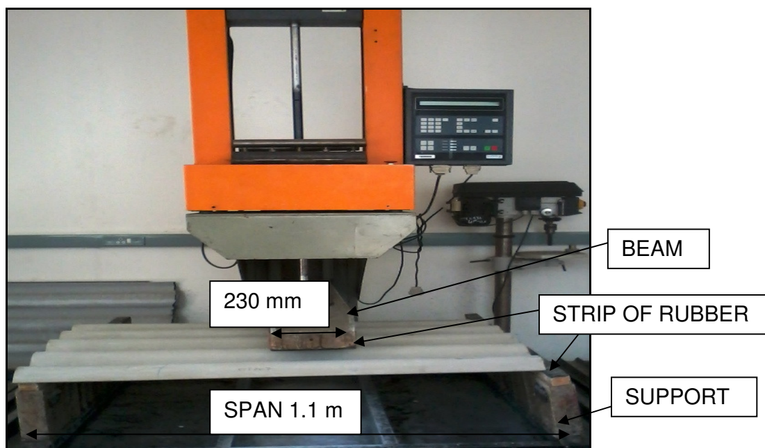
Figure 2.4: Lloyd machine for measuring breaking load of corrugated sheets
