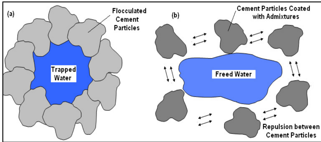
Figure 5.1 (a) Flocculation of cement particles resulting in trapped water. (b) Deflocculation of cement particles upon adsorption of water reducing admixtures (Law, 2004)
