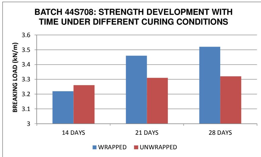
Figure 6.48: Development of strength in fibrecement corrugated sheets, with 3% inclusion as cement substitute, over 28 days curing under different conditions.
