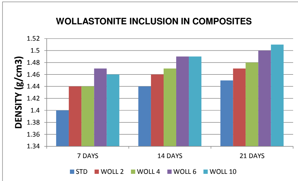
Figure 4.2 Development of density for wollastonite fibrecement sheets
