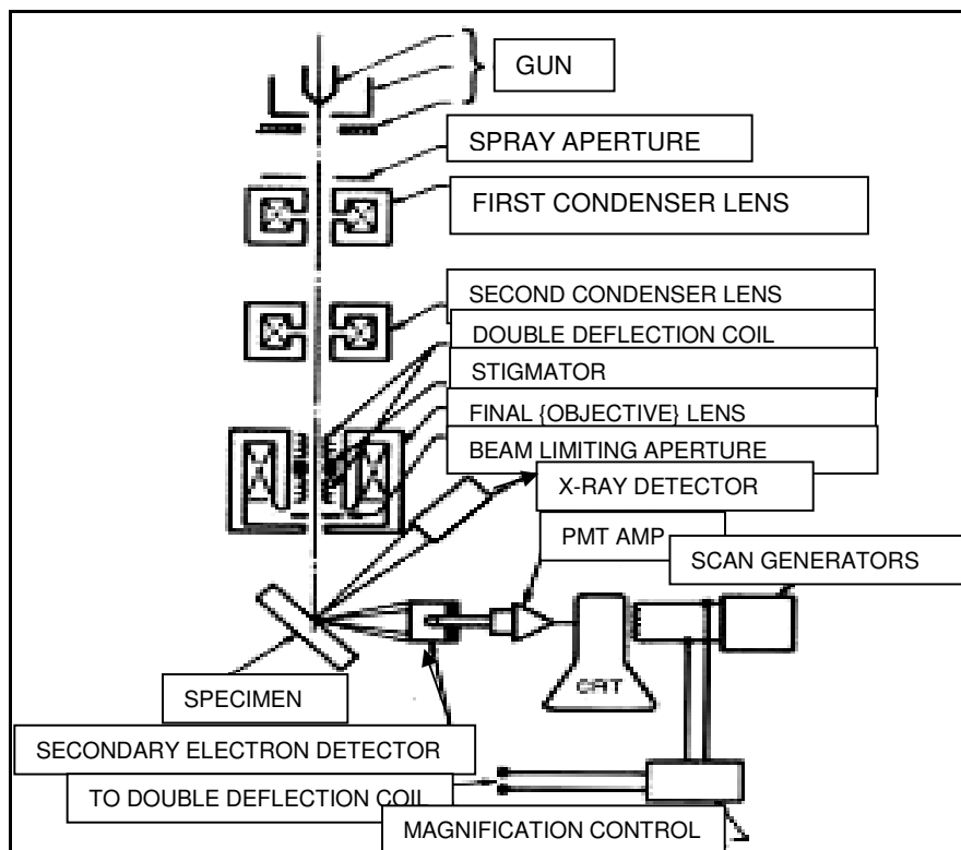
Figure 2.13: Schematic drawing of the SEM components [adapted after Swapp (2013)]
