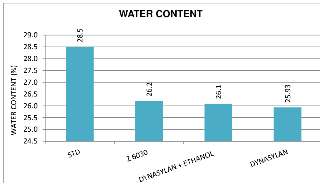
Figure 3.1: Process water content monitoring
