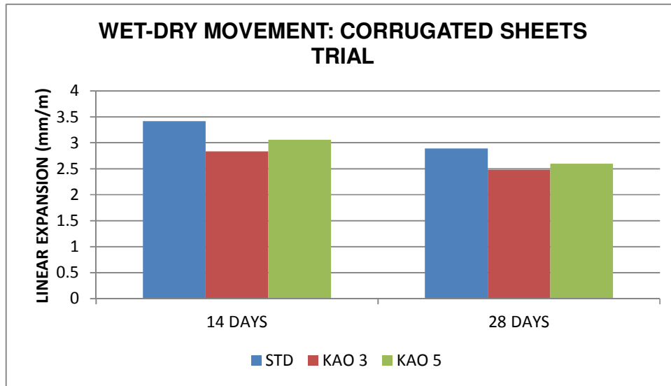
Figure 6.14: Wet-dry movement of corrugated sheets and the effect of incorporating kaolin as cement replacement over time.
