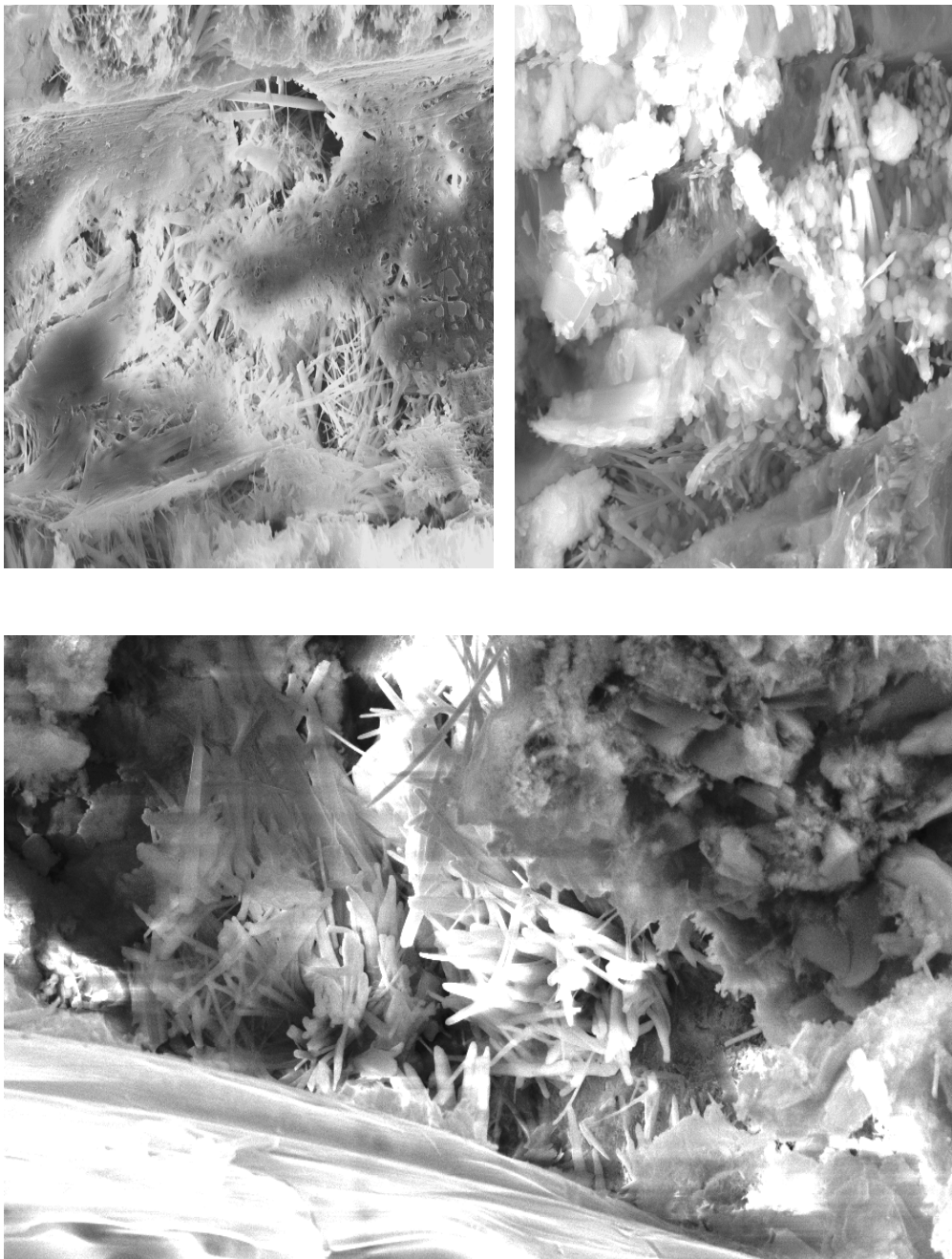
Figure C4: SEM micrographs of kaolin modified corrugated sheets, kept indoors wrapped, batch 35S714 for 14 d prior to exposure to natural environment.
