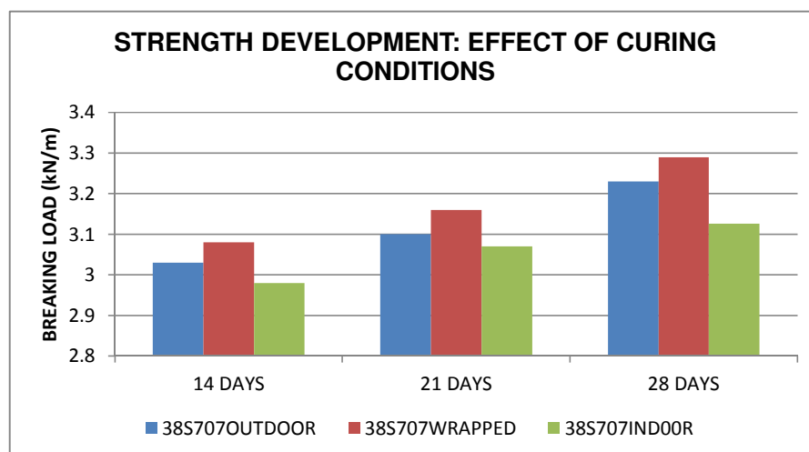
Figure 6.38 Development of strength of kaolin modified sheets over time under different curing conditions.
