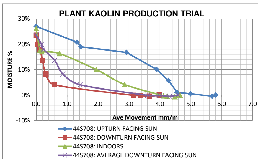
Figure 6.51: Moisture-movement curves of kaolin modified corrugated sheets, 3% replacing cement, cured under different conditions.
