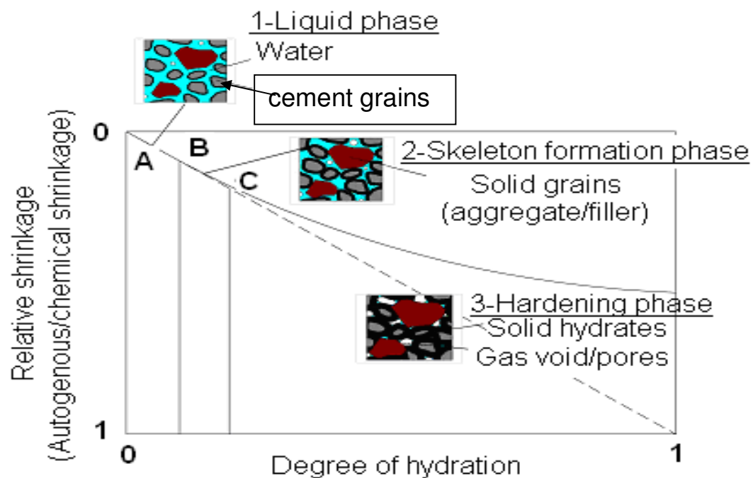
Figure 1.2: Autogenous and chemical shrinkage during different stages, as a function of degree of hydration [adapted after Holt (2001) and Esping (2007)]
