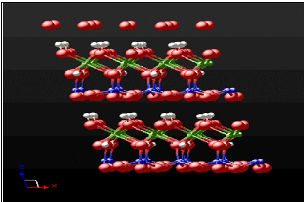
Figure 2.16: Kaolin structure showing the octahedral and tetrahedral sheets. (The white colour represents hydrogen atoms, red colour for oxygen atoms, green colour for aluminium atoms and blue for silicon atoms).
