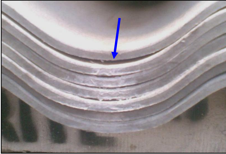
Figure 6.24: Thaumasite formation on corrugated fibre cement sheets with 5% kaolin inclusion as replacement of cement.
