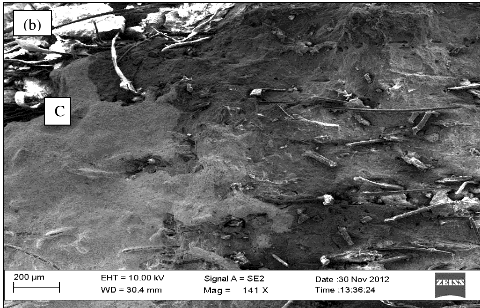
Figure 6.20 (b): SEM micrographs of corrugated sheets with 3% kaolin as replacement of cement taken after 4 months of natural weathering exposure.
