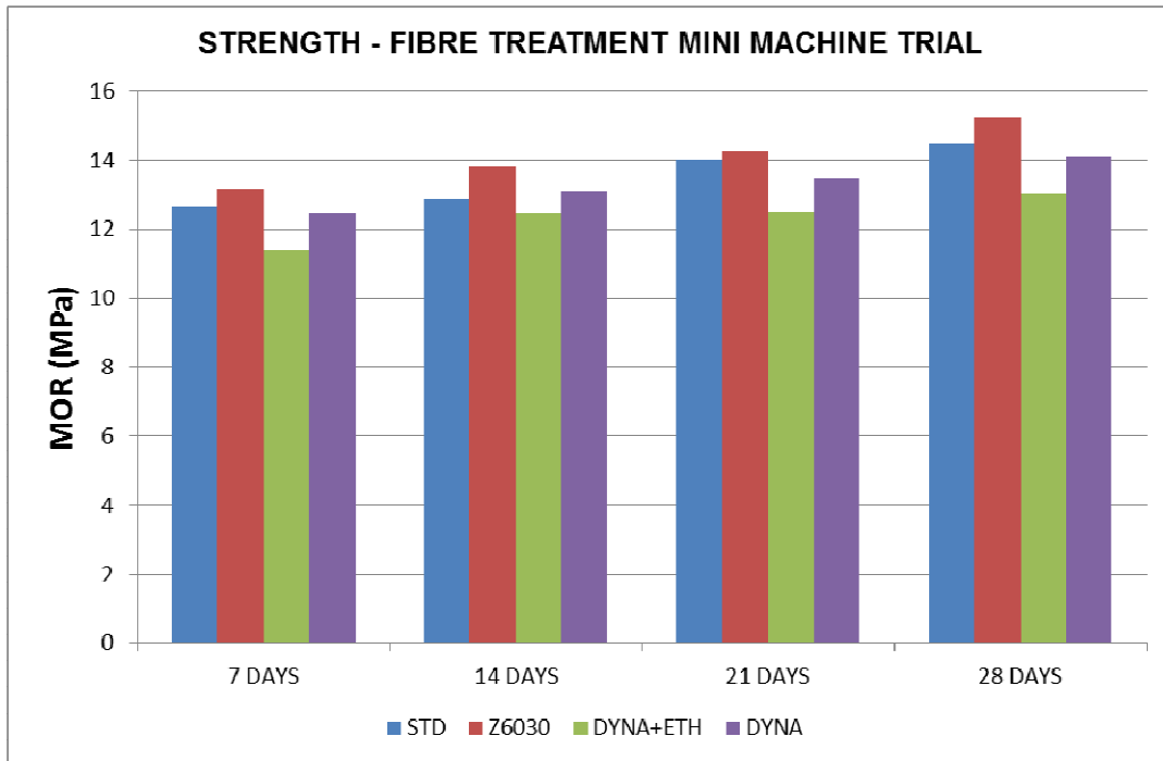
Figure 3.5: Strength development of cellulose pretreated sheets over 28 days
