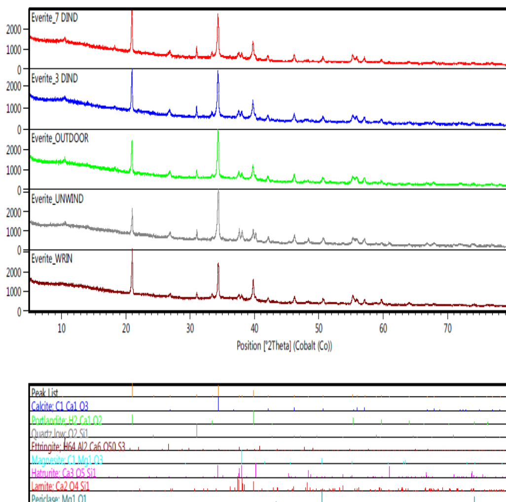
Figure B2: Quantitative XRD spectra for batch 29S705 of fibrecement corrugated sheets cured under various exposure conditions – 7d indoors (red), 3d indoors (blue), unwrapped indoors (black), wrapped indoors (brown) prior to outdoor exposure and outdoor exposure (green).
