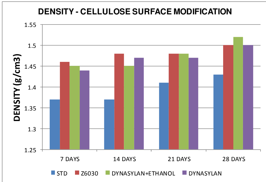
Figure 3.3: Density development of cellulose pretreated sheets over time
