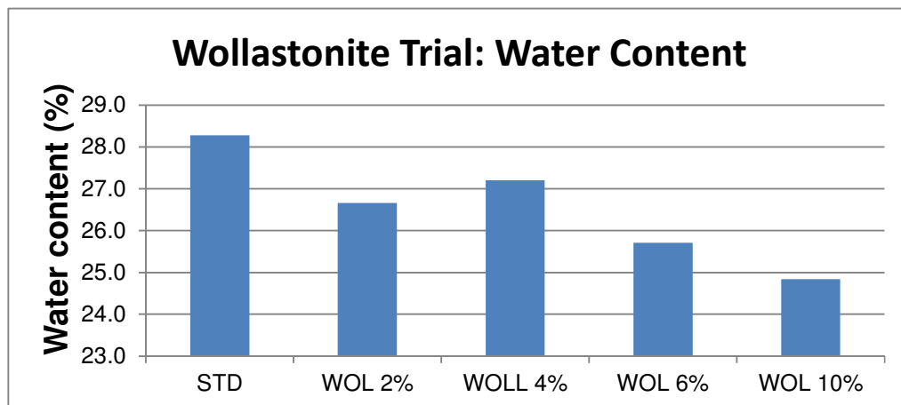
Figure 4.1: Water content of wollastonite fibrecement composites measured during the manufacturing process
