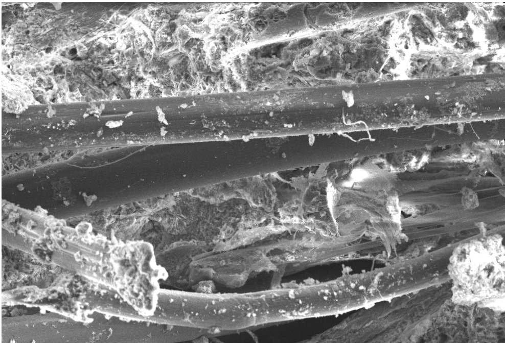
Figure C5: SEM micrographs of kaolin modified corrugated fibre cement sheets, batch 35S714 cured outdoors without wrapping.
