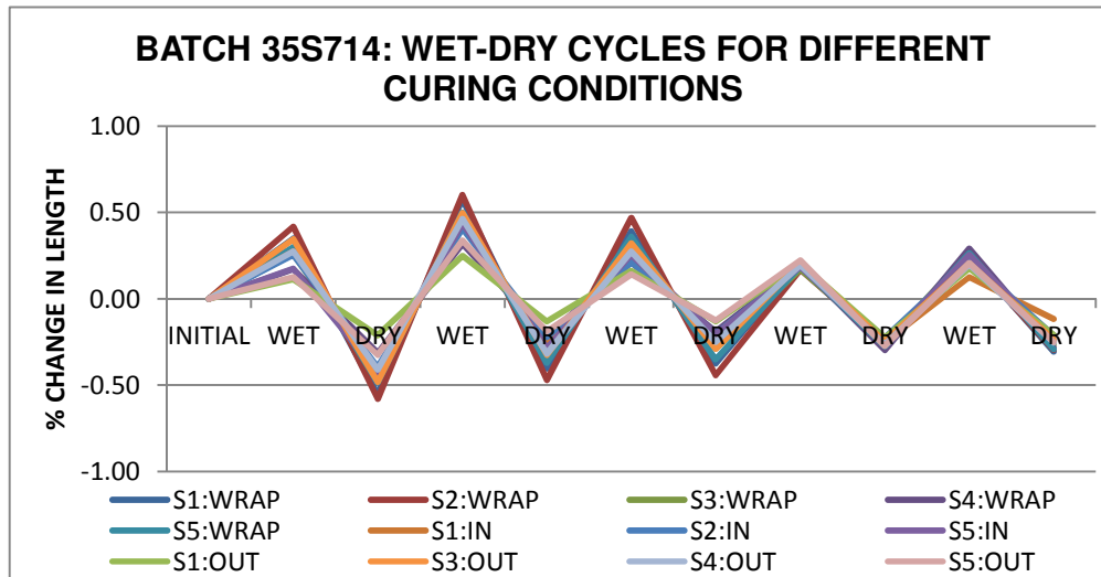
Figure A2: Wet-dry cycling curve for batch 35S714 for evaluation of durability of kaolin modified fibrecement sheets. Movement reduction noted after three cycles.
