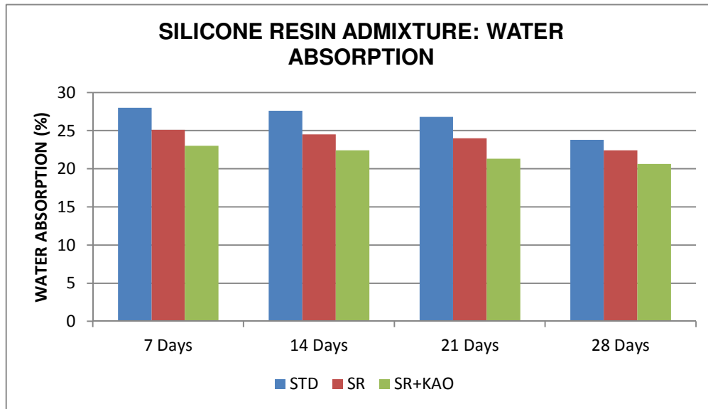
Figure 5.4 Development of water absorption for composites with admixture
