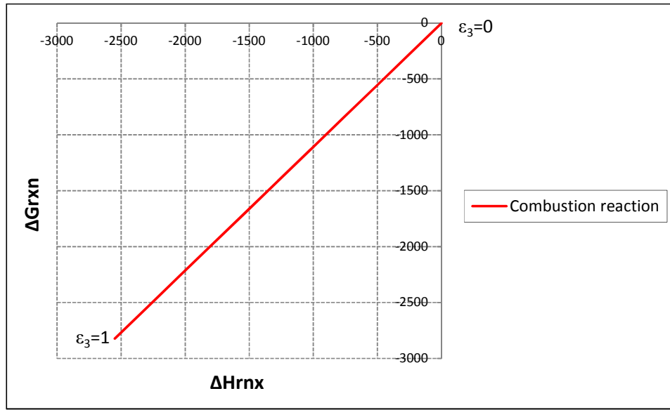
Figure 4.5 Reaction line for the combustion reaction by plotting the overall \Delta H_{rxn} and \Delta G_{rxn} over a range of extents.
