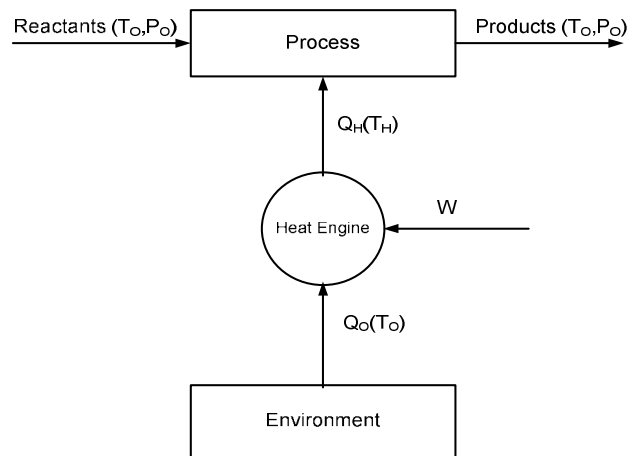
Figure 2.10 Heat Engine for processes that require Heat and Work input.
