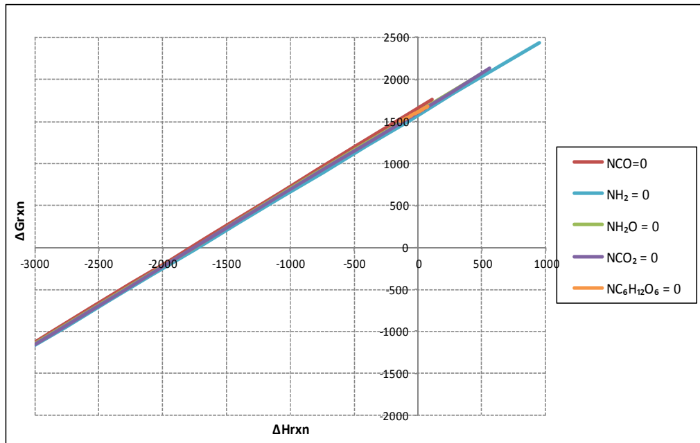
Figure 4.10 The effect of temperature on the gasification region at 800°C.
