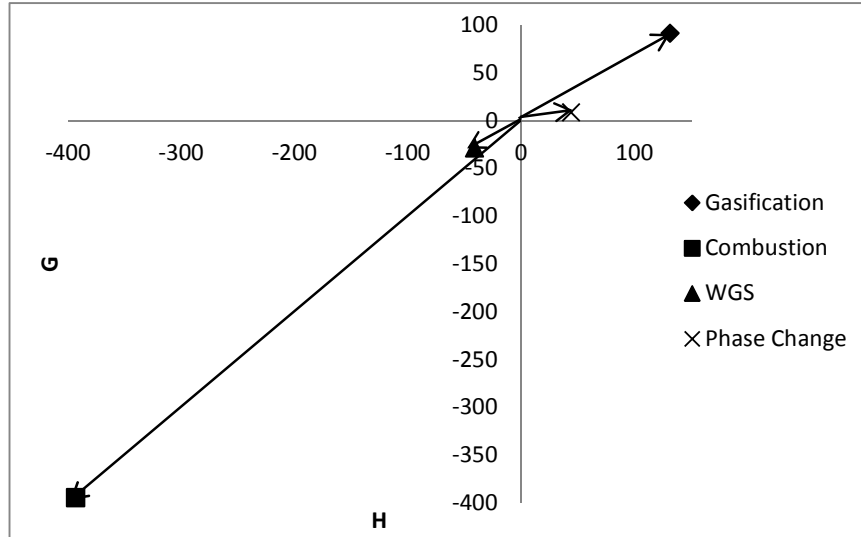
Figure 2. 9 The four gasification reactions as vectors on the g-h space.
