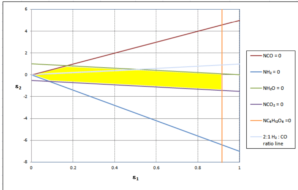
Figure 3.4 The gasification region
