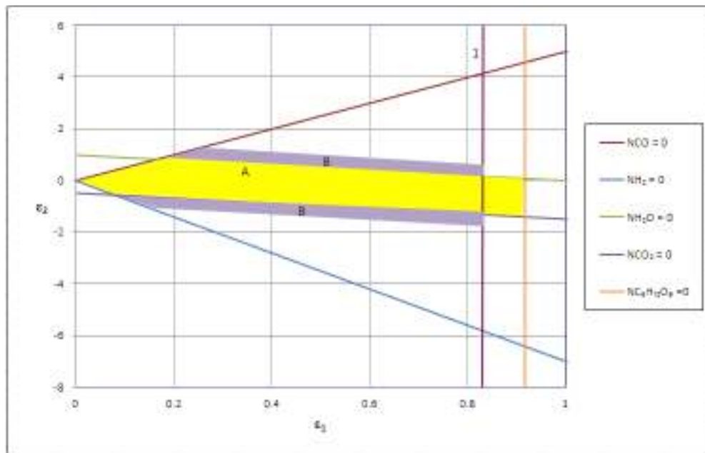
Figure 3.6 The effect of increasing oxygen in the feed stream.
