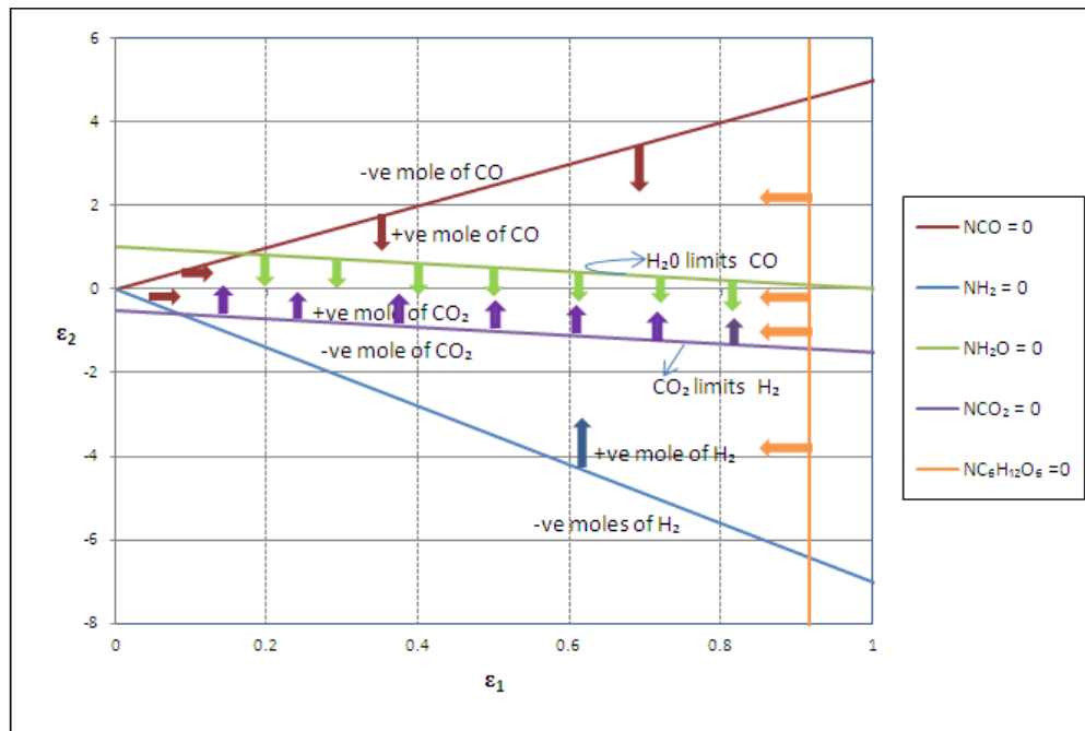
Figure 3.3 The mass balance region.
