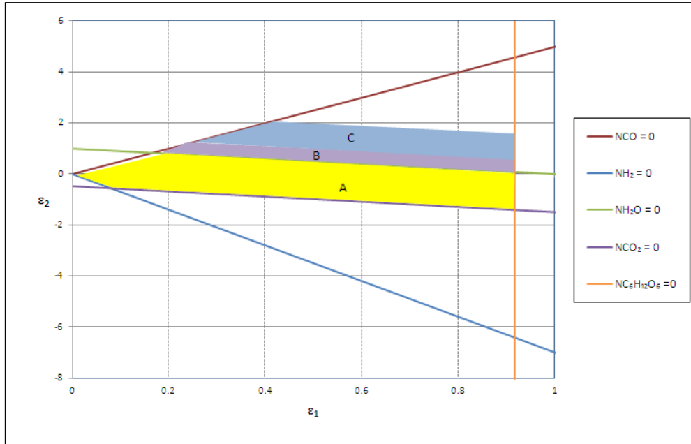
Figure 3.5 The effect of increasing water in the feed stream.
