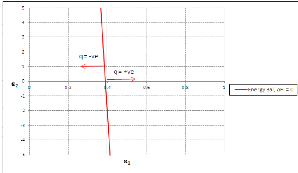
Figure 3.8 Plot of energy balance when \Delta H = 0 .
