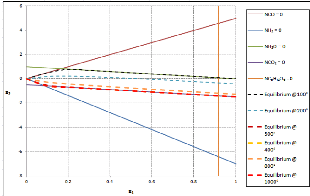
Figure 3.15 Effect of Temperature on the equilibrium.
