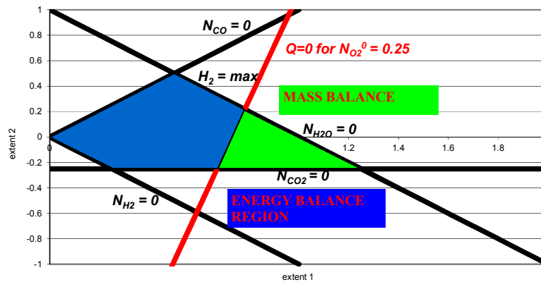
Figure 2.7 Combination of the mass and energy balance for a feed of N_{O_2}^0 = 0.25 and N_{H_2O}^0 = 1 . (Ngubevana et al., 2011)
