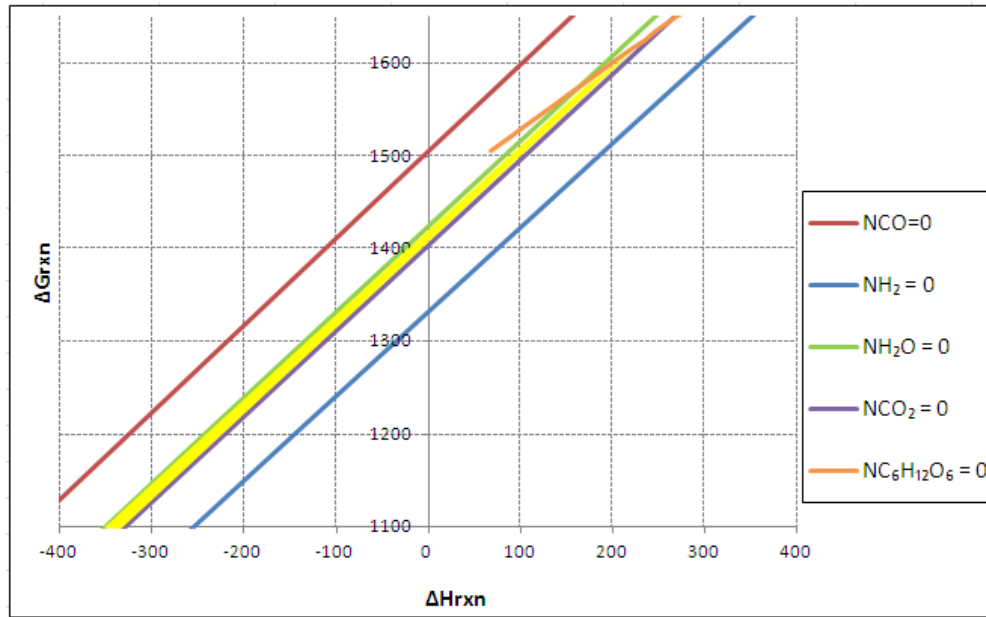
Figure 4.9 The expanded upper region of the effect of temperature on the gasification region at 400°C.
