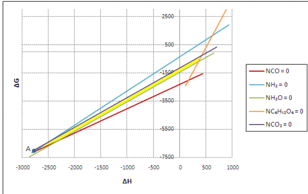
Figure 4.7 The mass balance region on the g-h space.
