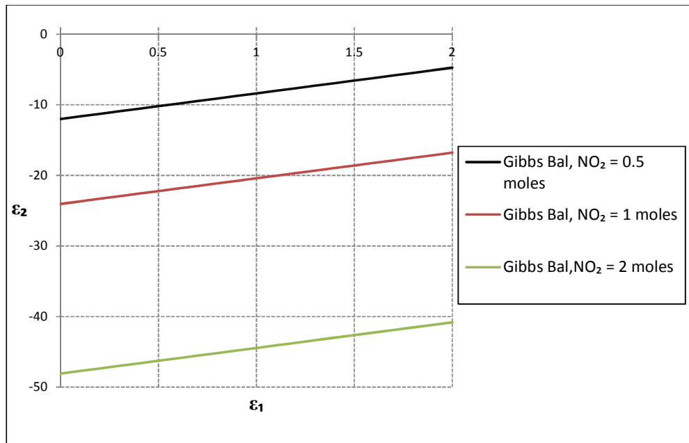
Figure 3.11 Gibbs free energy balance at different \text{NO}_2 feed.
