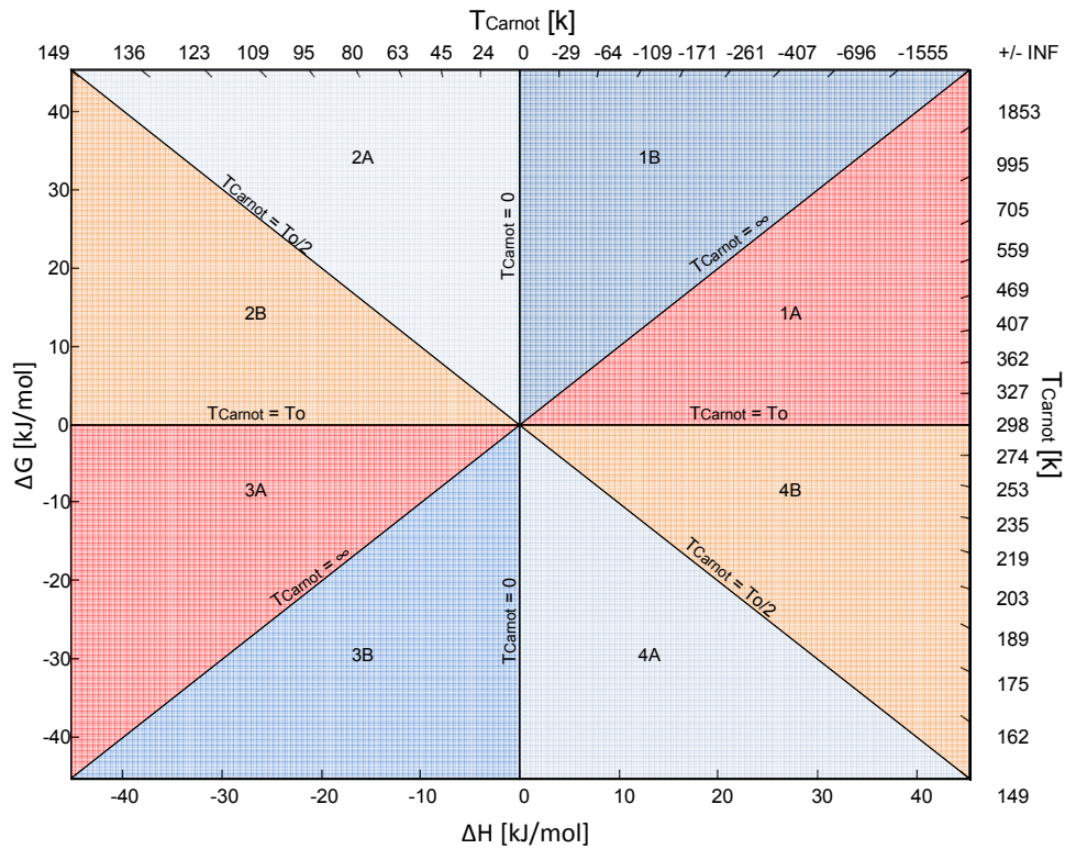
Figure 4.2 Thermodynamic regions on the g-h diagram. (Sempuga et al. 2010)
