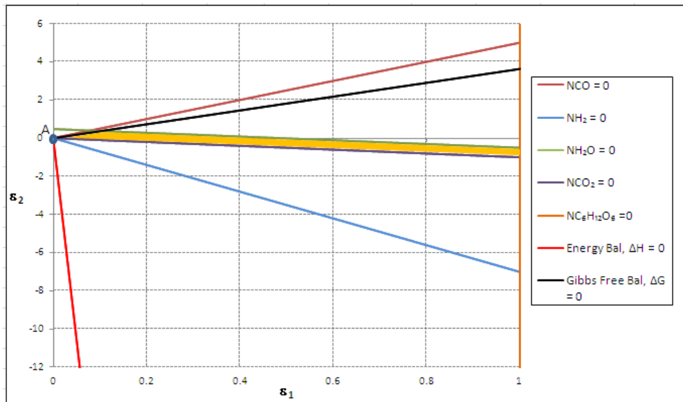
Figure 3.13 Combining Mass, Energy and Gibbs free Energy balance at the feed of N_{O_2}^0 = 0 mole, N_{H_2O}^0 = 0.5 mole and N_{C_6H_{12}O_6}^0 = 1 mole.
