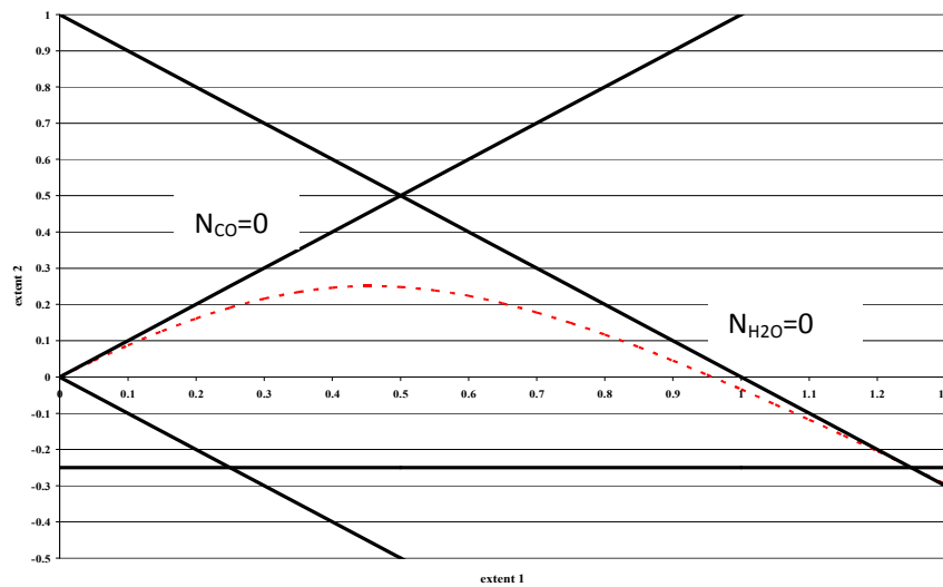
Figure 2.8 Equilibrium plot for WGS reaction at 1200 K for a feed of N_{H_2O}^0 = 1 , N_{O_2}^0 = 0.25 .(Ngubevana et al., 2011)
