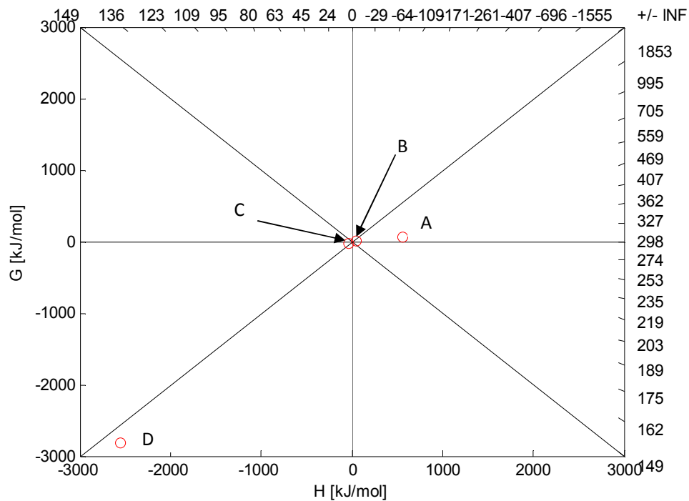
Figure 4.3 Gasification reactions in the thermodynamic regions.
