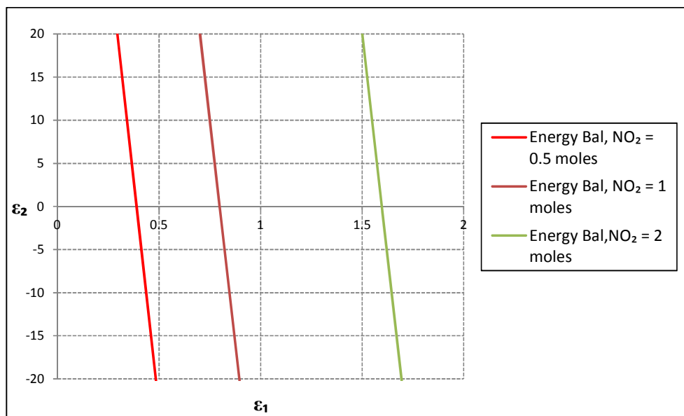
Figure 3.9 The feed effect on the Energy Balance.
