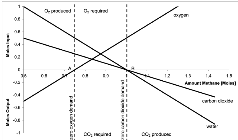
Figure 2.4 Molar amounts of each component required/produced as a function of the amount of methane fed to the process that produces one mole of methanol is varied (Patel et al. 2007).
