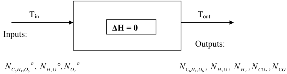
Figure 3.7 Adiabatic process.
