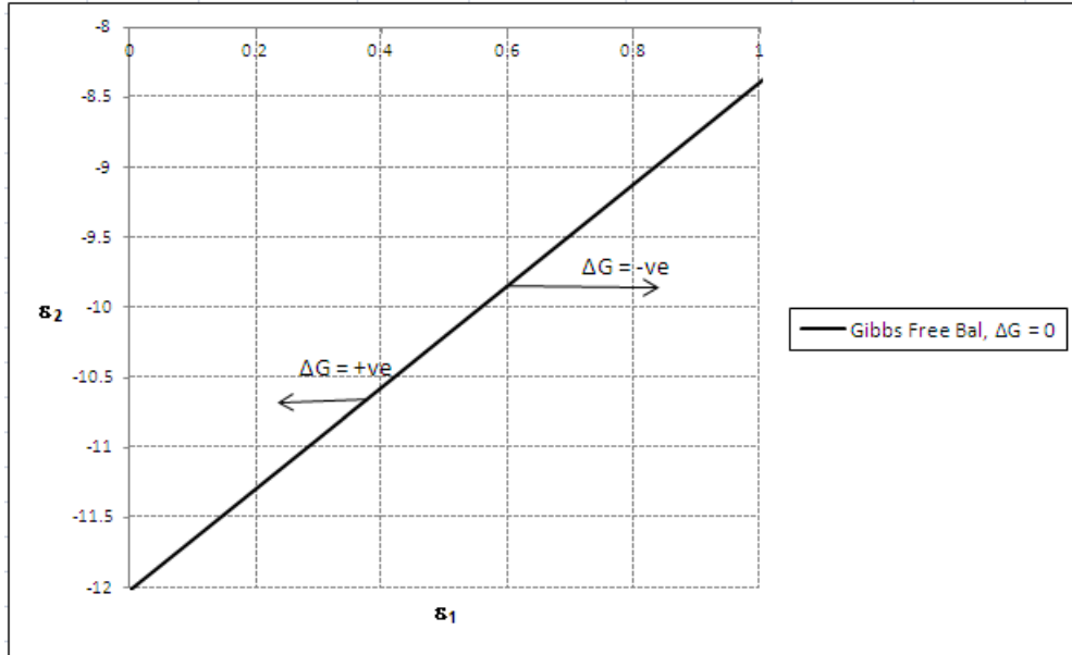
Figure 3.10 Plot of Gibbs free energy Balance, \Delta G = 0 .
