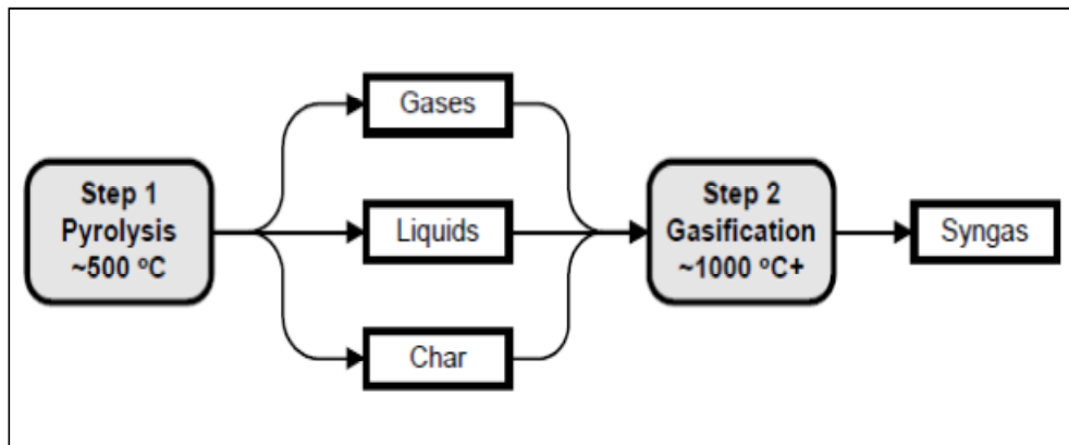
Figure 2. 3 Gasification steps.
