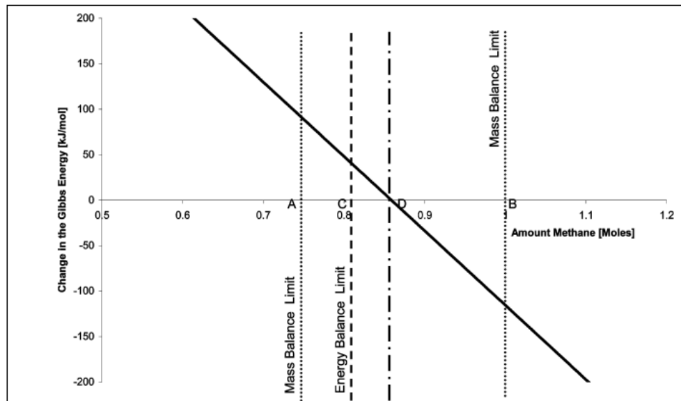
Figure 2.6 Gibbs energy change for the methanol synthesis process, as a function of the methane fed to the process. (A negative change in the Gibbs free energy would correspond to a work-consuming process, whereas a positive change in the Gibbs energy would mean a process would produce work).(Patel et al. 2007)
