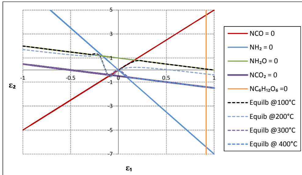
Figure 3.16 Temperature lines crossing through components zero lines.
