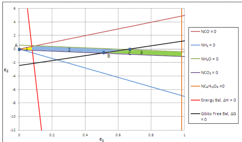
Figure 3.14 Combining Mass, Energy and Gibbs free Energy balance at the feed of N_{O_2}^0 = 0.1 mole, N_{H_2O}^0 = 0.5 mole and N_{C_6H_{12}O_6}^0 = 1 mole.
