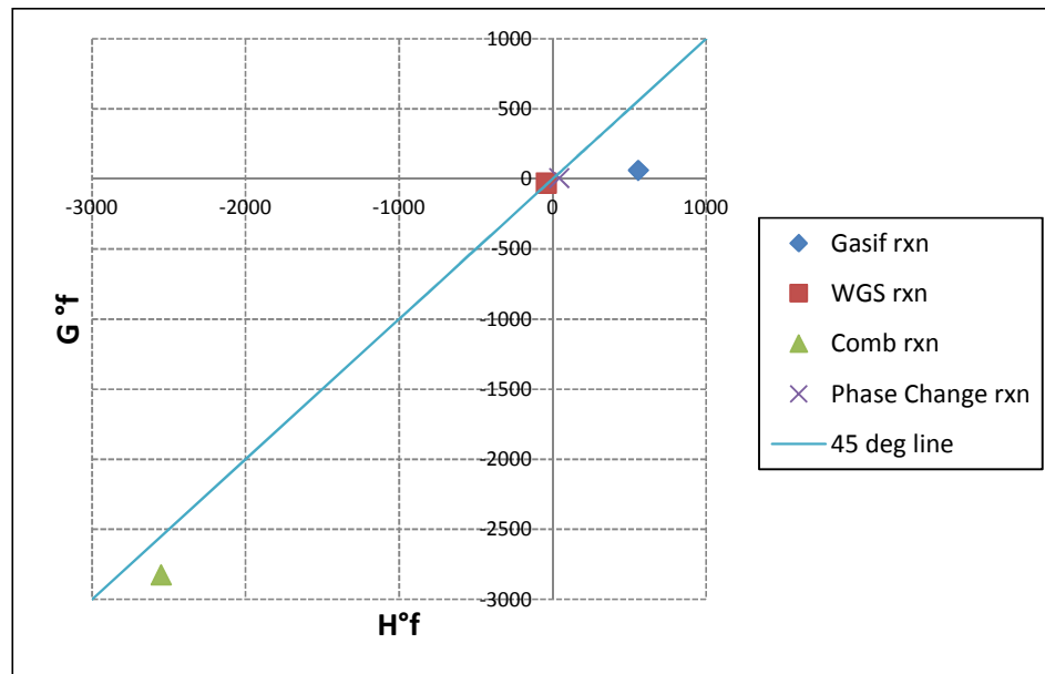
Figure 4.4 Reactions involved in the gasifier.
