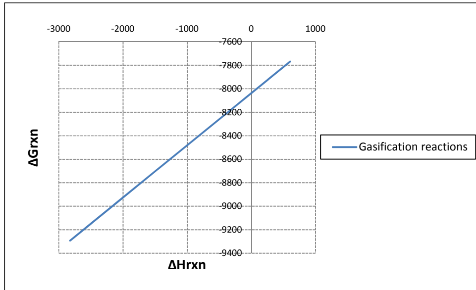
Figure 4.6 Reaction line for all the independent gasification reaction by plotting the overall \Delta H_{rxn} and \Delta G_{rxn} over a range of extents.
