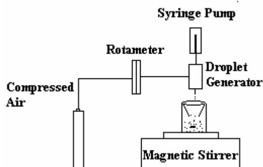
Figure 3.2.1: Apparatus set-up for microencapsulation
