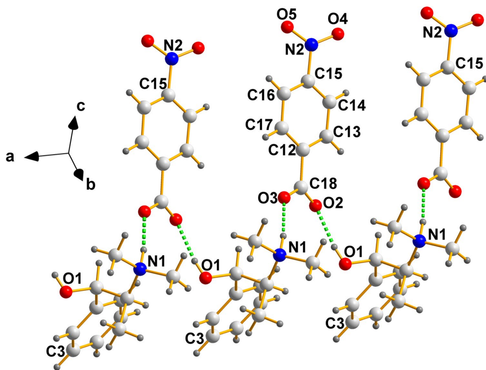
Fig. 2 Along the a -axis, the strings of ephedrinium cations are stitched together by hydrogen bonds with the carboxylate fragments of the nitro benzoate anions
