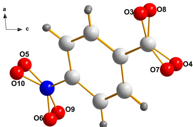
Fig. 6 The only significant deviation from near-perfect overlay is in the external oxygens associated with the nitro and carboxylic fragments, which are quite free to rotate about the single bonds to the phenyl rings
