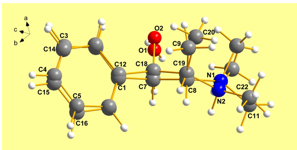
Fig. 5 The overlay of the two independent molecules in ( II ) was carried out with the cation coordinates directly from the final CIF. Note the chirality at C7-C18 (R and R) and C8-C19 (S and S) pairs are preserved
