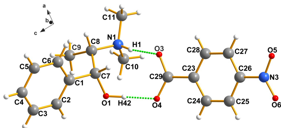
Fig. 4 C7(R) and C8(S) are the chiral carbons on the ephedrine cation. Note the hydrogen-bonded cation–anion pair in (II) is essentially identical with that in (I) (see Fig. 1)
