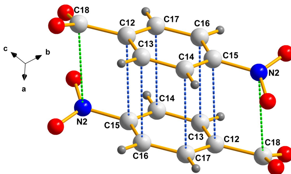
Fig. 3 Regarding \pi - \pi bonding, note the interesting head-to-tail arrangement of pairs of the carboxylate anions in (I)
