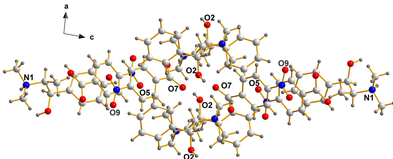
Fig. 7 The Center of Mass is located at 0.5049, 0.4360, 0.5110
