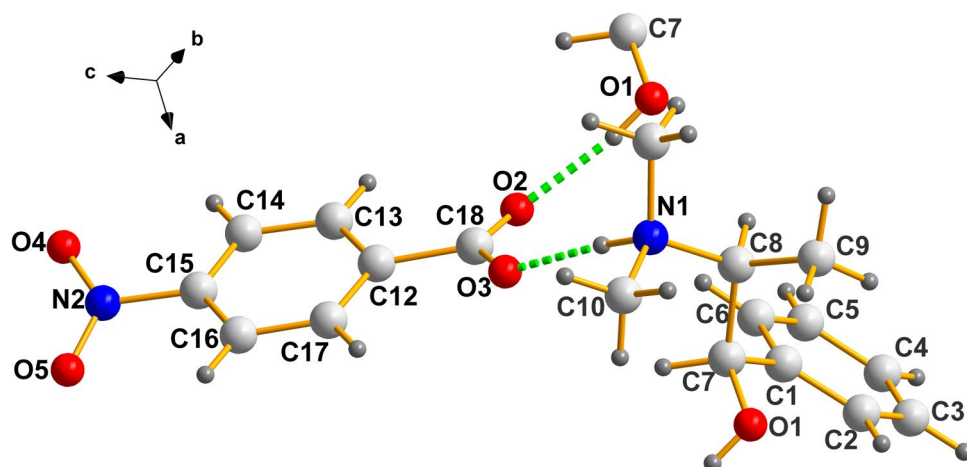
Fig. 1 describes the stereochemistry and atomic labeling of the racemate ( I ).
