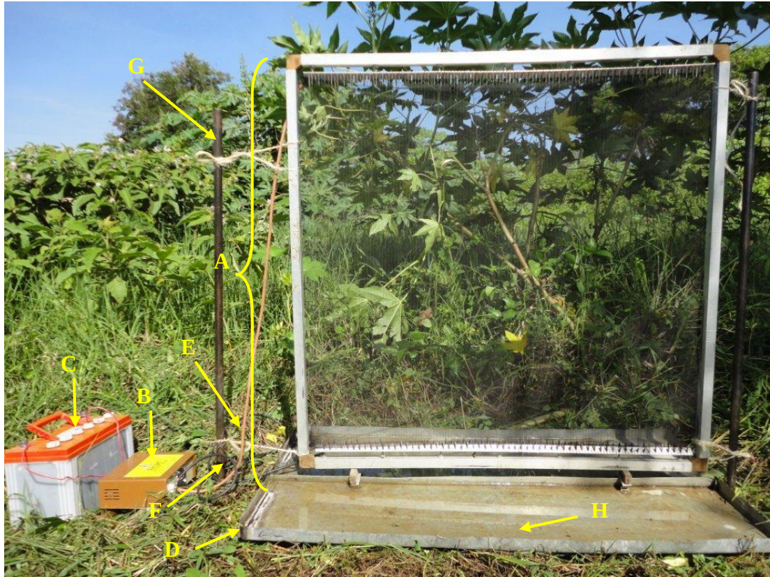
Figure 2.5 Electric grid (1x1 meter). (A) Electric net, (B) Spark box, (C) 12V battery, (D) Tray, (E) Positive wire, (F) Negative wire, (G) Supporting pole, (H) Soapy water 3-5cm deep in metal tray.
