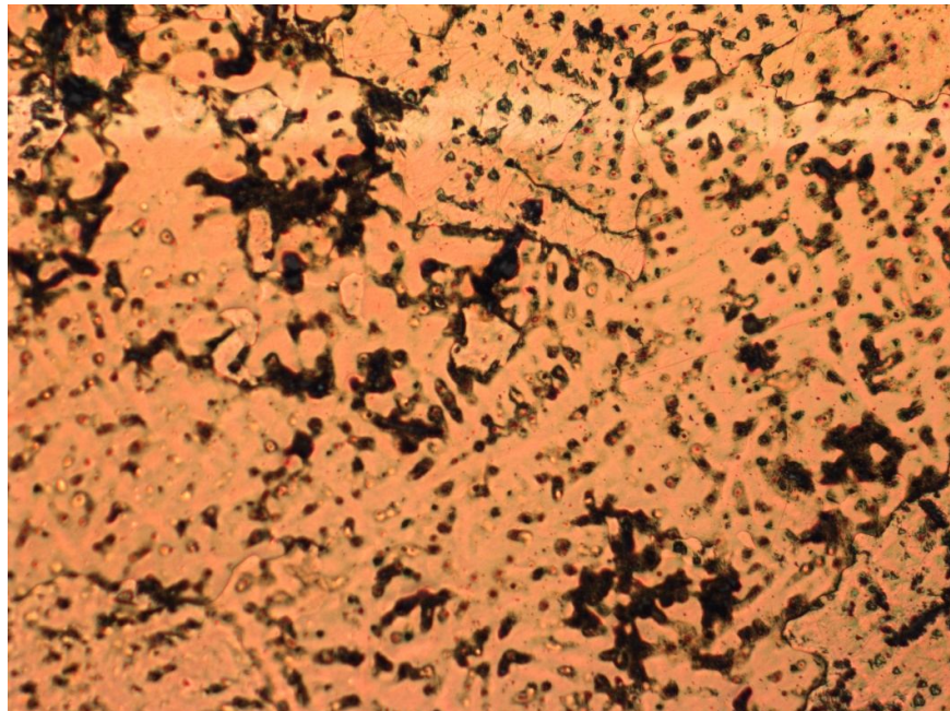
Figure 4.1.5p: Cast sample (Univ. of Joburg WBO, 200X)
