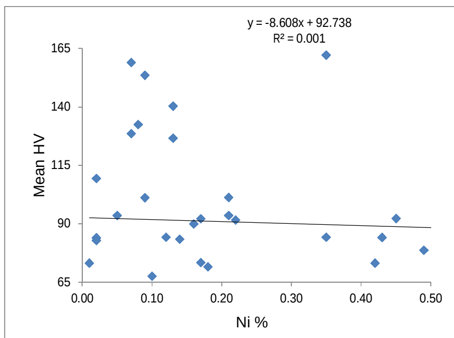
Figure4.1.4m: Impact of nickel content on hardness for standard samples
