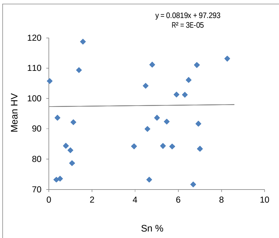
Figure4.1.4e: Impact of tin content on hardness for standard samples
