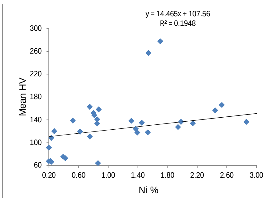
Figure4.1.4n: Impact of nickel content on hardness for cast samples
