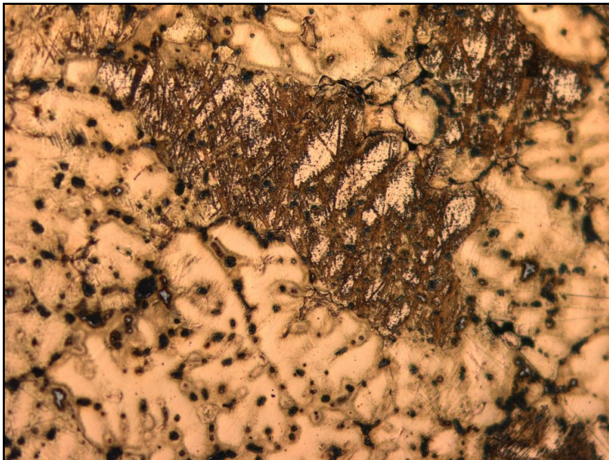
Figure 4.1.5f: Used bearing (Fox Foundry scrap FFD, 100X)
