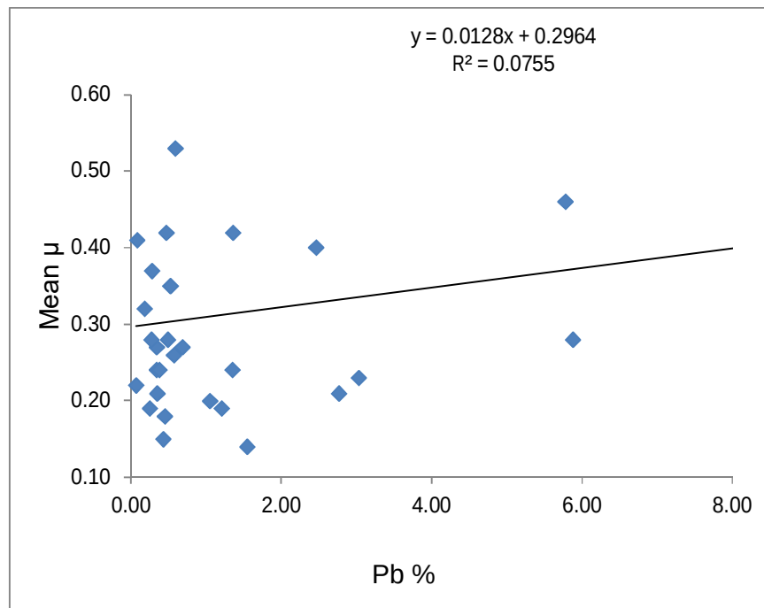
Figure4.1.4k: Impact of lead content on friction for standard samples
