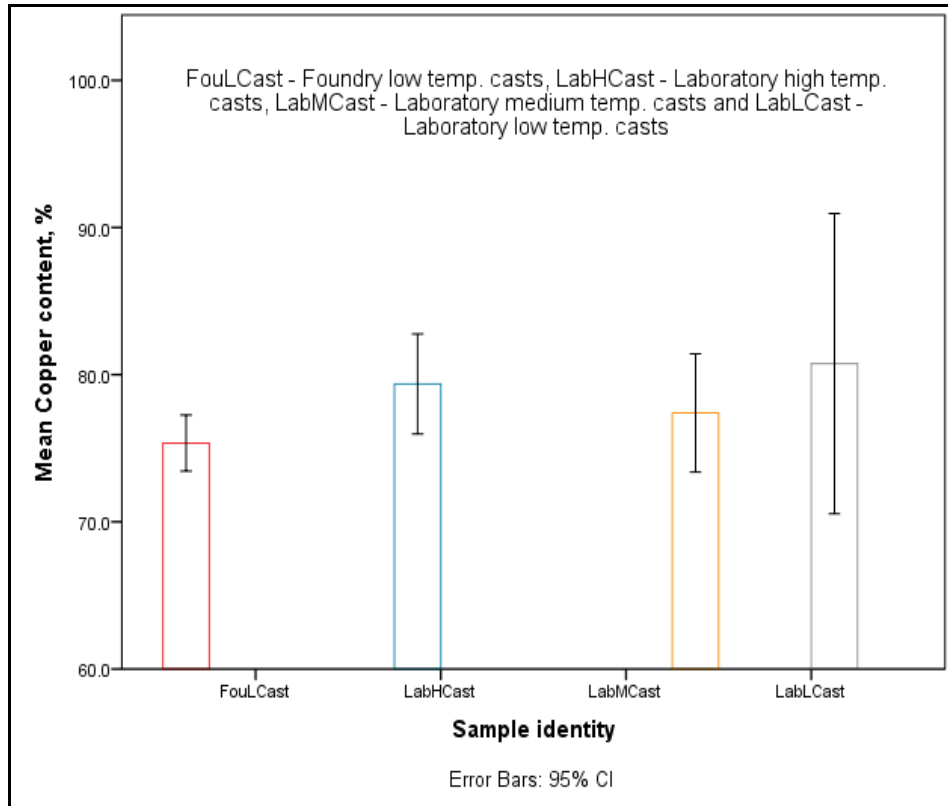
Figure4.1.2f: Comparison of copper content in various test castings
