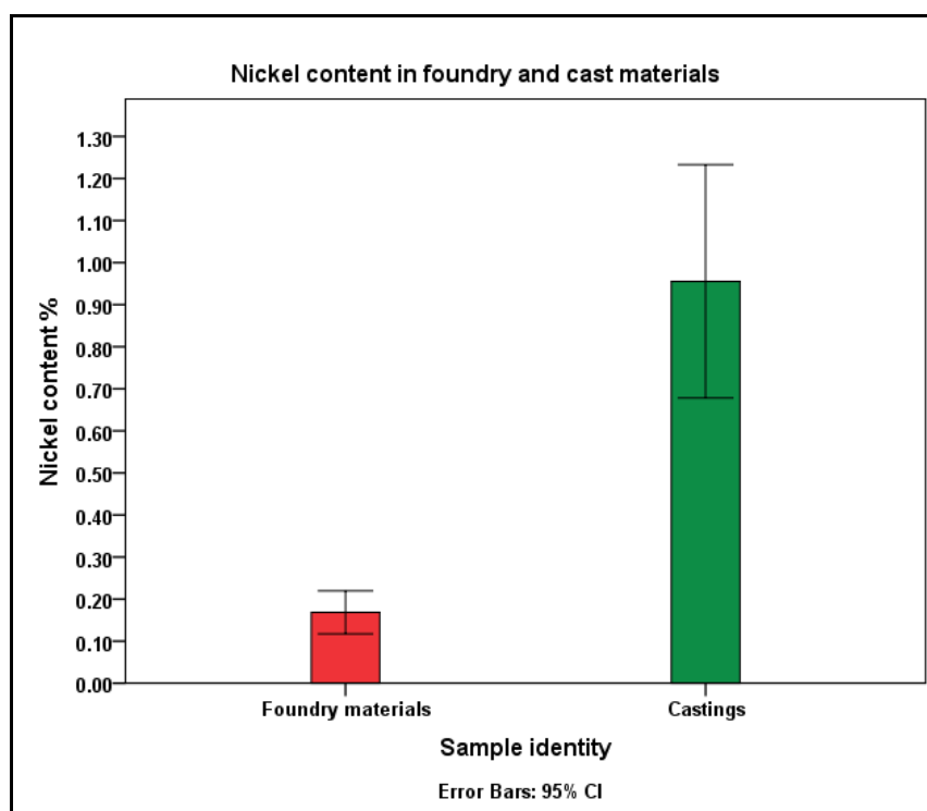
Figure4.1.2d: Nickel in foundry materials and castings
