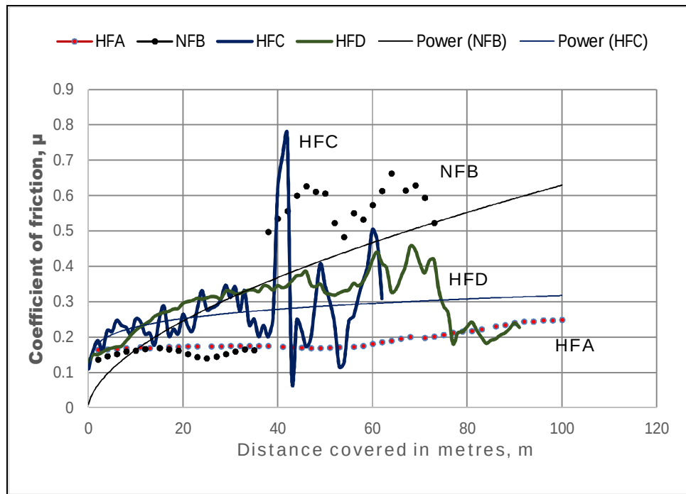
Figure 4.1.6b: Friction comparisons of foundry billets (NFB and HFA) and experimental casts
