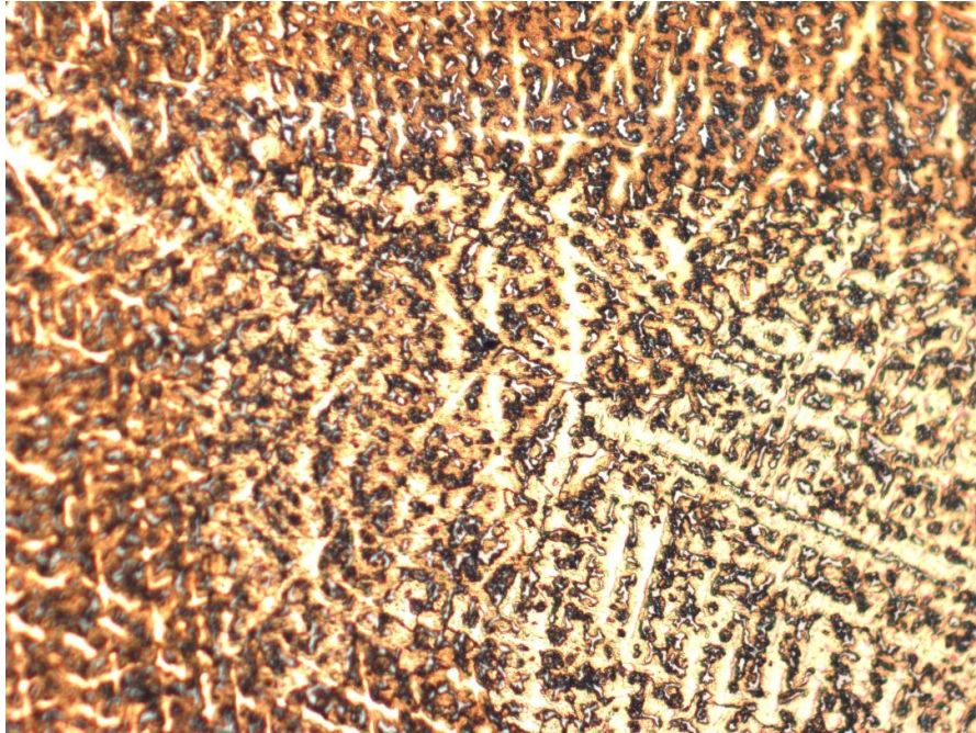
Figure 4.1.5m: Cast sample, WBH (Univ. of Joburg WBH, 200X)
