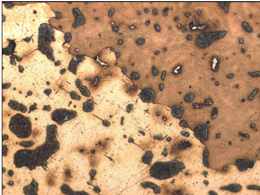
Figure 4.1.5b: Secondary crusher liner (Konkola Copper Mines KCA, 100X)
