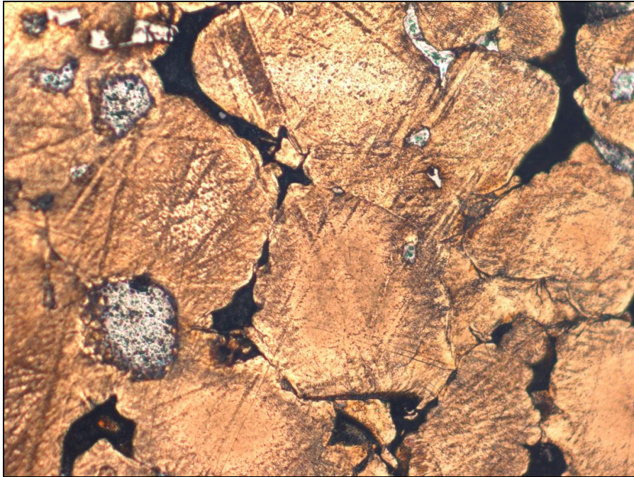
Figure 4.1.5e: Crusher shaft barrel bearing (Mopani Copper MCG, 200X)
