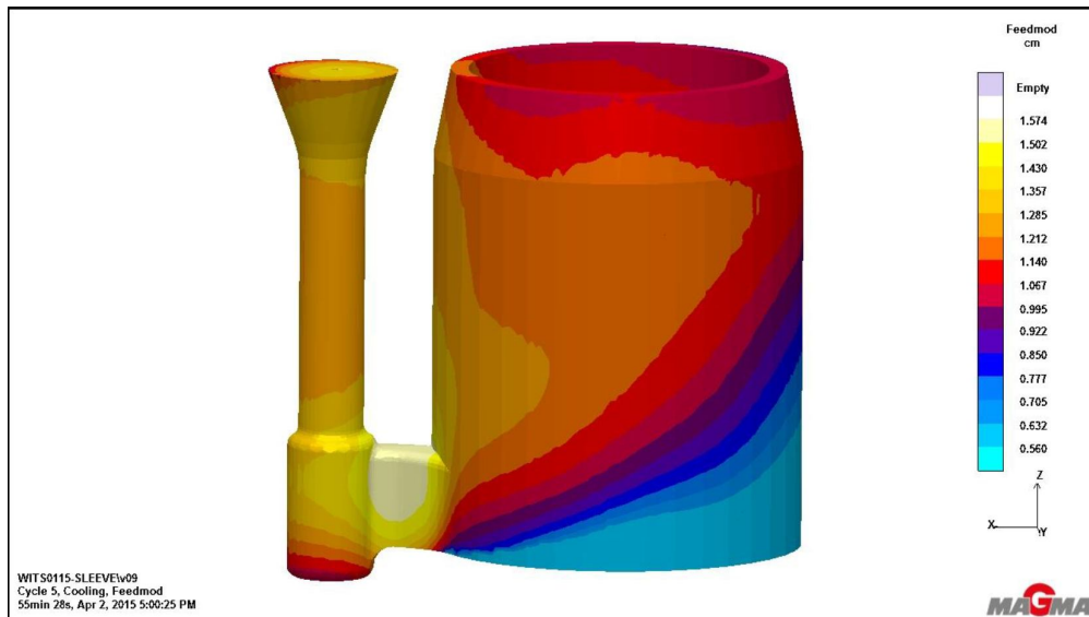
Figure 4.3b: Feed modulus distribution during pouring of metal from the initial 1100°C (Simulation by Ametex, April 2015)
