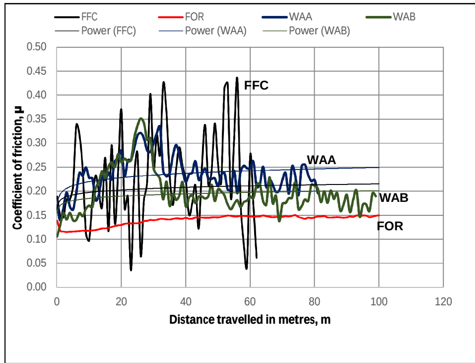
Figure4.1.6c: Friction comparisons of foundry billets (FFC and FOR) and experimental casts
