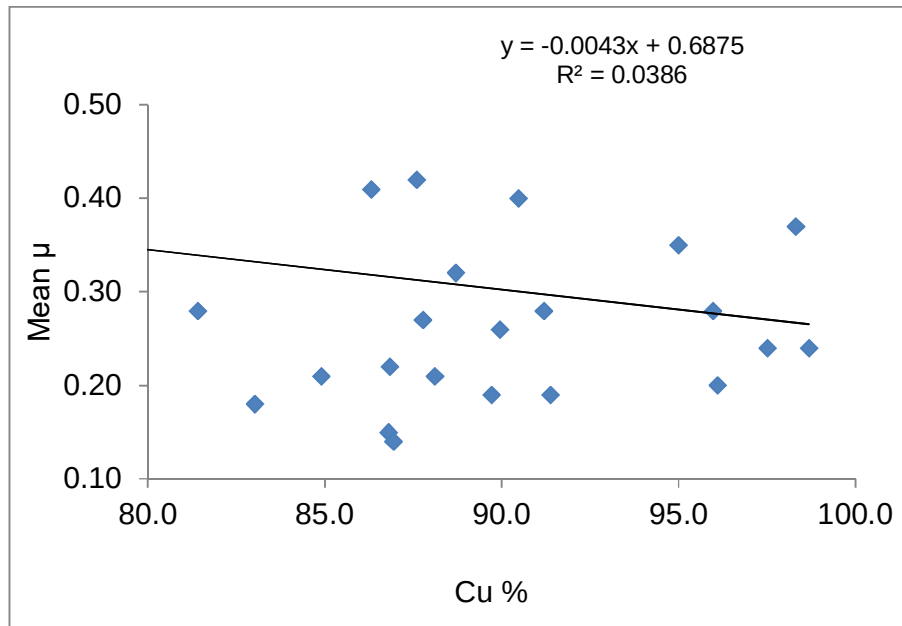
Figure4.1.4c: Impact of copper content on friction for standard samples
