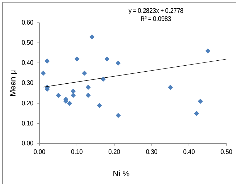
Figure4.1.4o: Impact of nickel content on friction for standard samples
