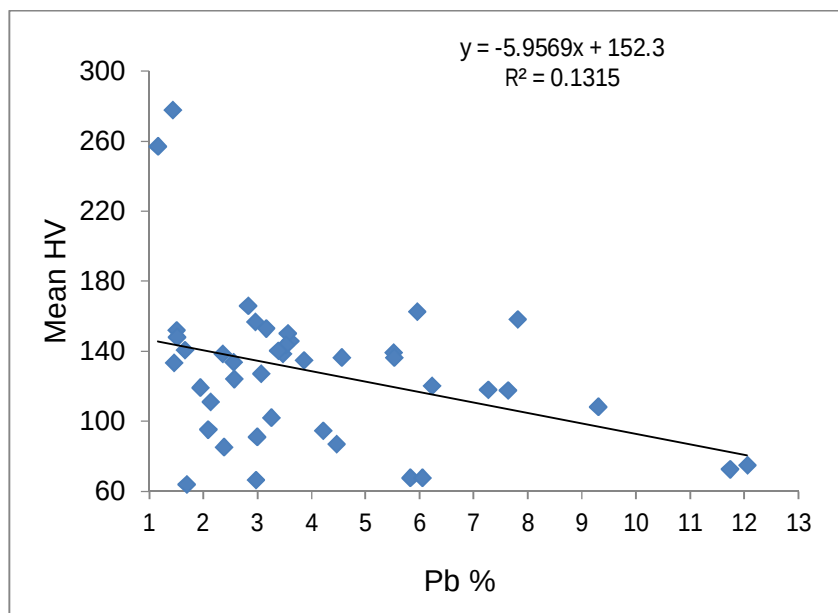
Figure4.1.4j: Impact of lead content on hardness for cast samples
