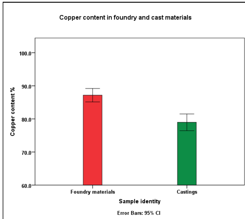
Figure4.1.2a: Copper in foundry materials and castings
