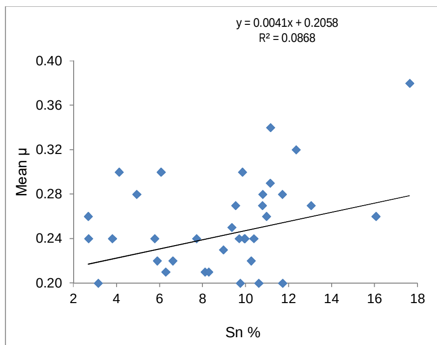
Figure4.1.4h: Impact of tin content on friction for cast samples
