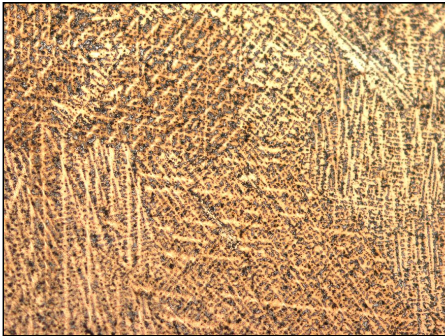
Figure 4.1.5j: Cast sample, WAY (Univ. of Joburg WAY, 100X)
