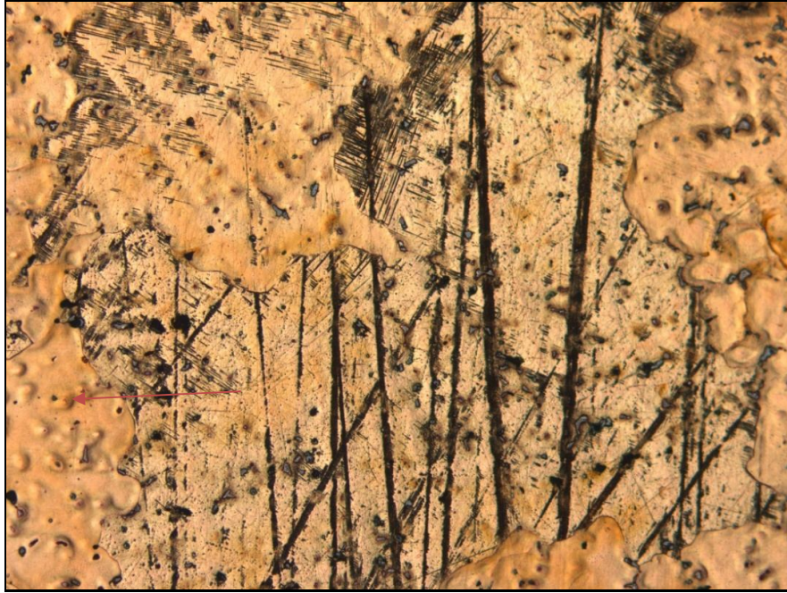
Figure 4.1.5a: Thrust ring with large \alpha grains (Fox Foundry scrap FFE, 50X)
