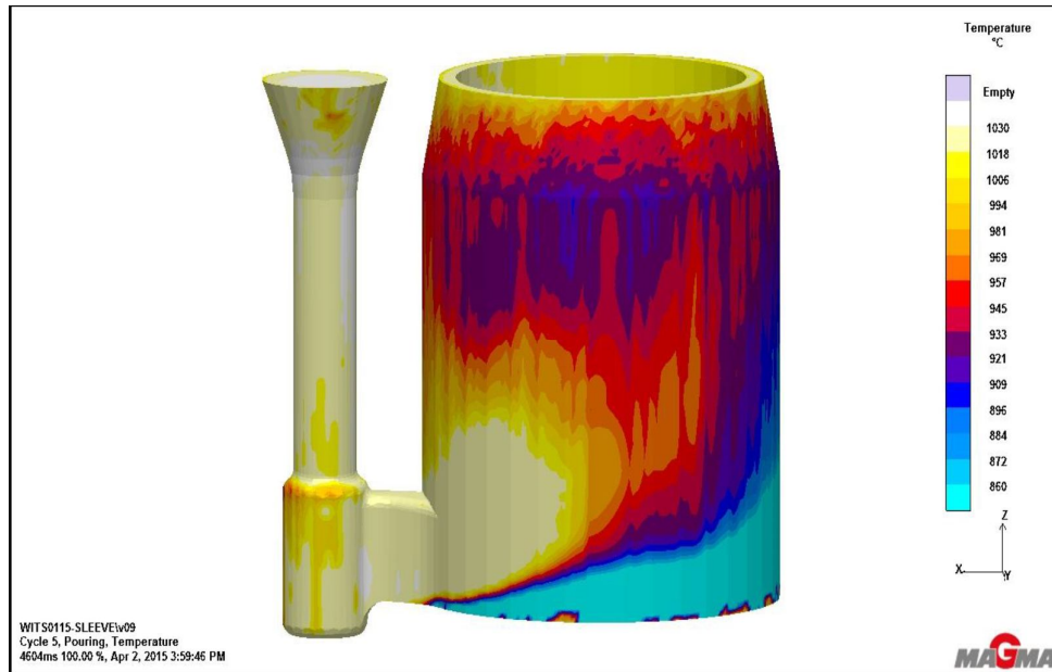
Figure 4.3a: Temperature distribution during pouring of metal from the initial 1100°C (Simulation by Ametex, April 2015)
