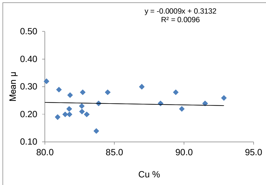
Figure4.1.4d: Impact of copper content on friction for cast samples
