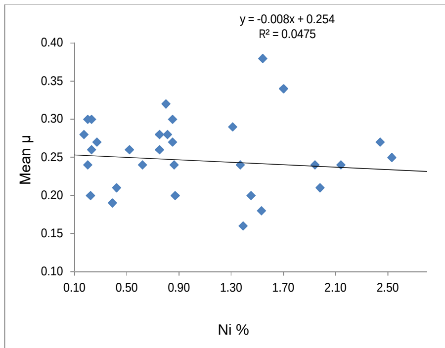
Figure4.1.4p: Impact of nickel content on friction for cast samples
