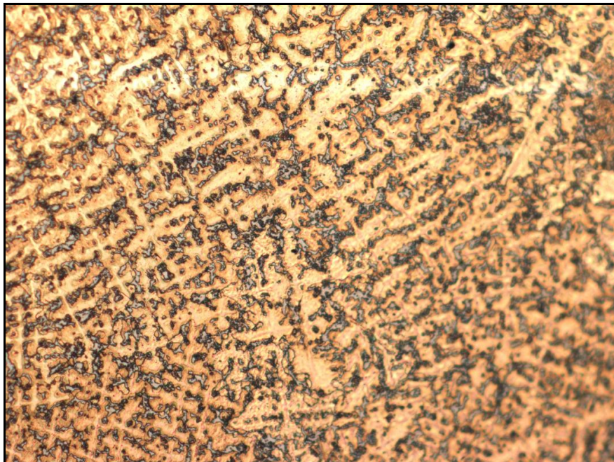
Figure 4.1.5l: Cast sample (Univ. of Joburg WBE, 200X)
