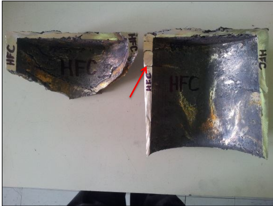
Figure4.3e: Sections of casting HFC
