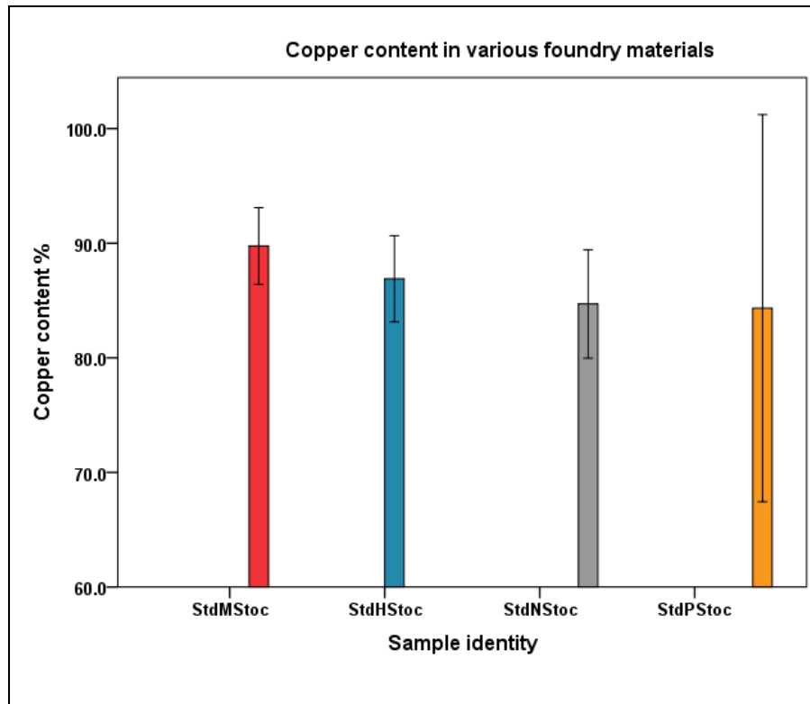
Figure4.1.2e: Comparison of copper content in various foundry materials
