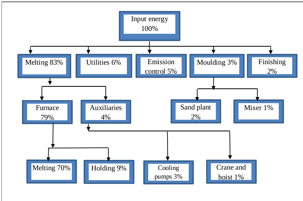
Figure 2.2.9f: Foundry process study with respect to energy use (Customised Energy Solutions)
