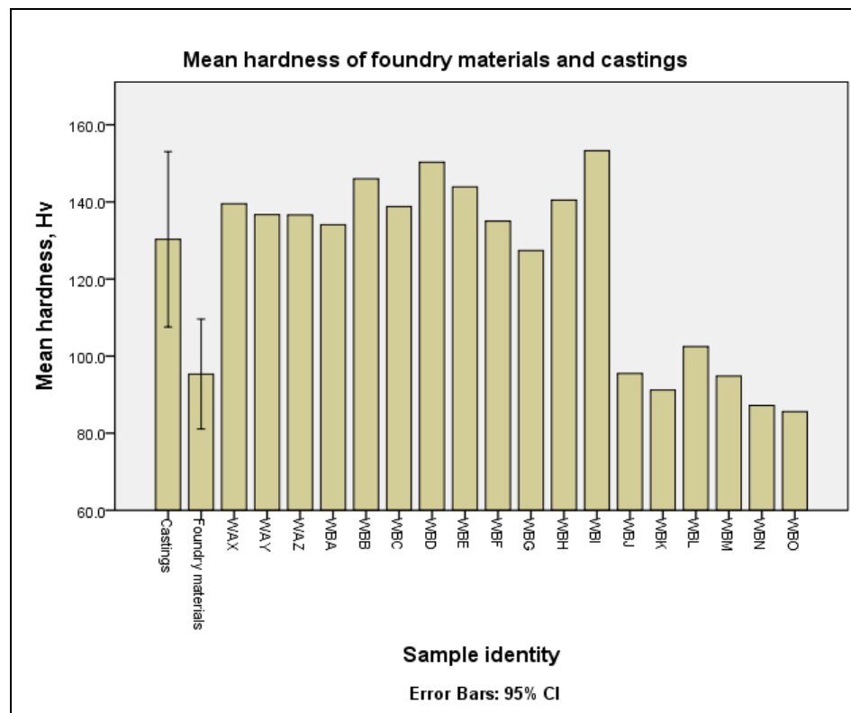
Figure4.1.3c: Hardness comparisons in groups and individual castings
