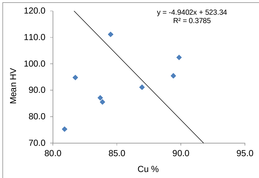
Figure4.1.4b: Impact of copper content on hardness for cast samples
