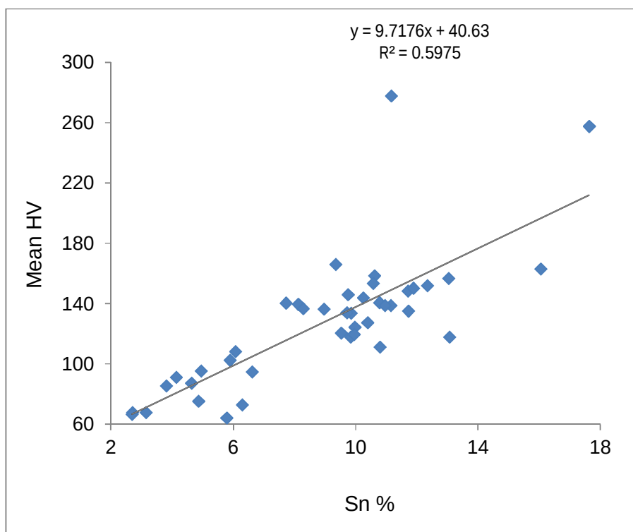
Figure4.1.4f: Impact of tin content on hardness for cast samples
