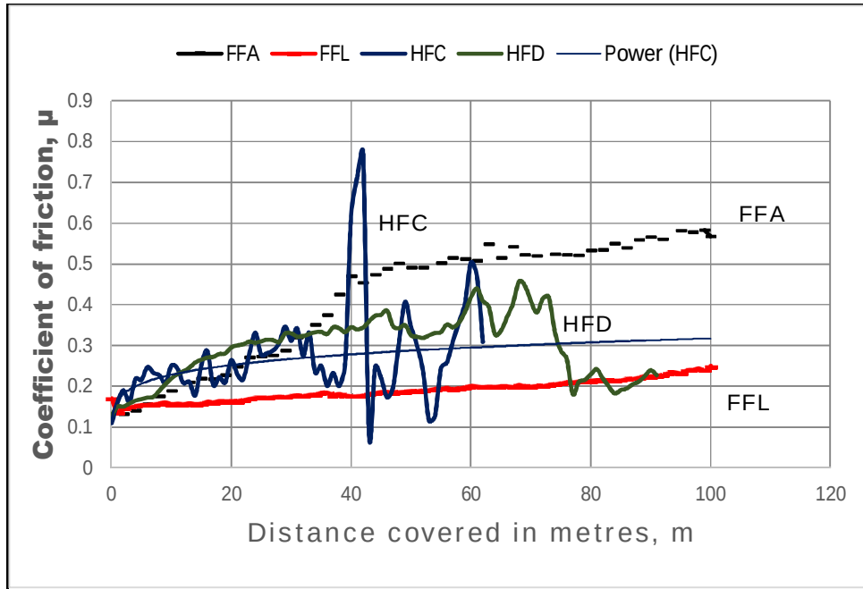
Figure 4.1.6a: Friction comparisons of foundry billets (FFA and FFL) and experimental casts
