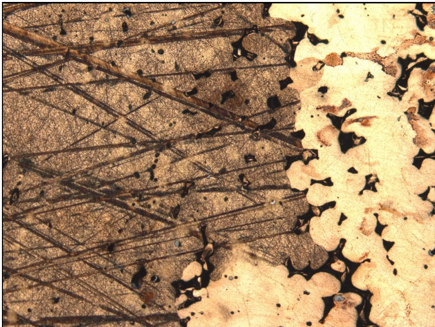
Figure 4.1.5d: Cast billet for sale (Fox Foundry FFA, 50X)
