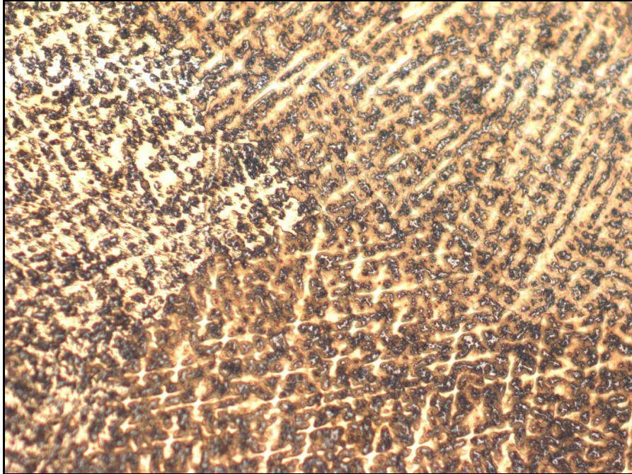
Figure 4.1.5k: Cast sample (Univ. of Joburg WBA, 200X)
