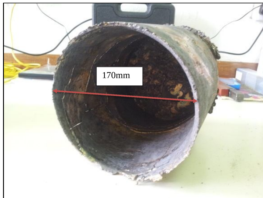
Figure4.3d: Casting HFC (Heroes, Jan. 2015)
