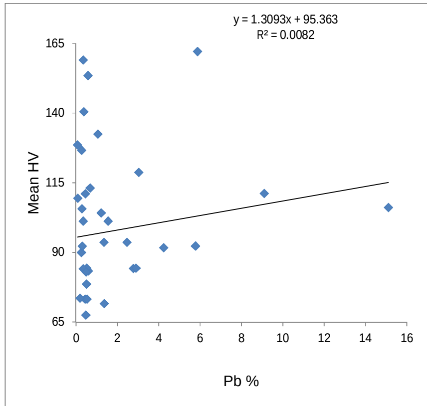
Figure4.1.4i: Impact of lead content on hardness for standard samples
