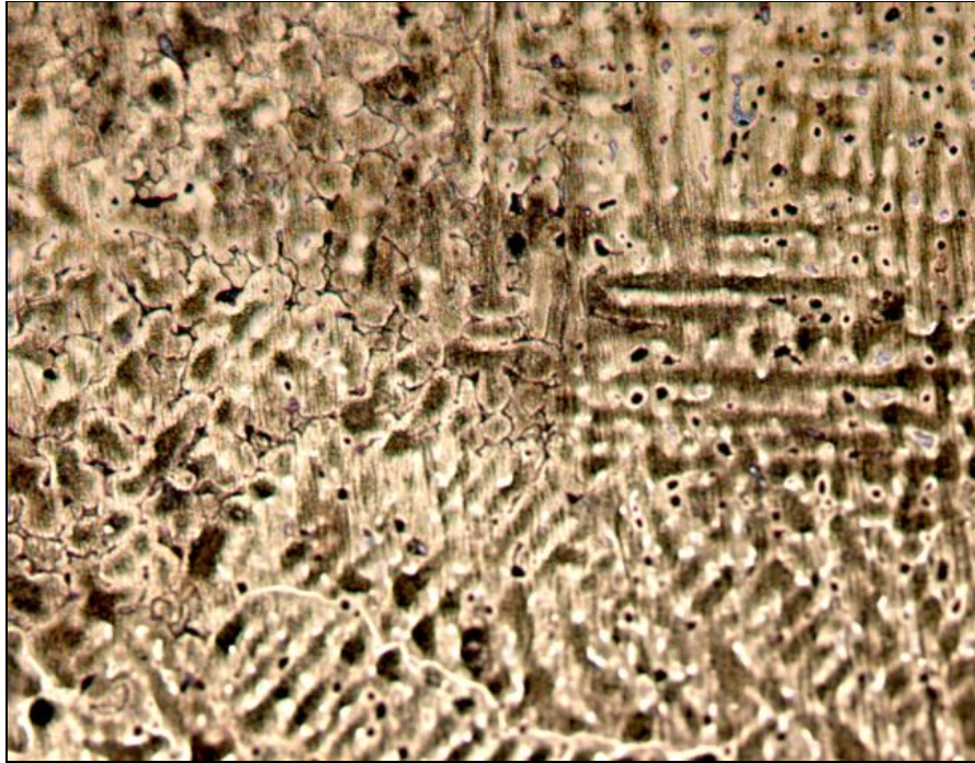
Figure 4.1.5c: Used bearing (Fox Foundry scrap FFG, 100X)
