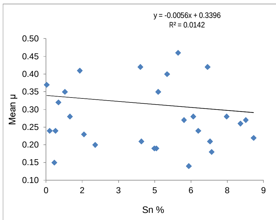
Figure4.1.4g: Impact of tin content on friction for standard ingot (machine bar) samples
