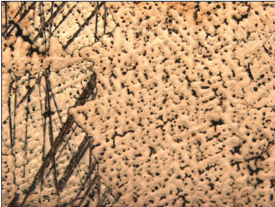
Figure 4.1.5h: Used bearing (Fox Foundry scrap FFJ, 50X)
