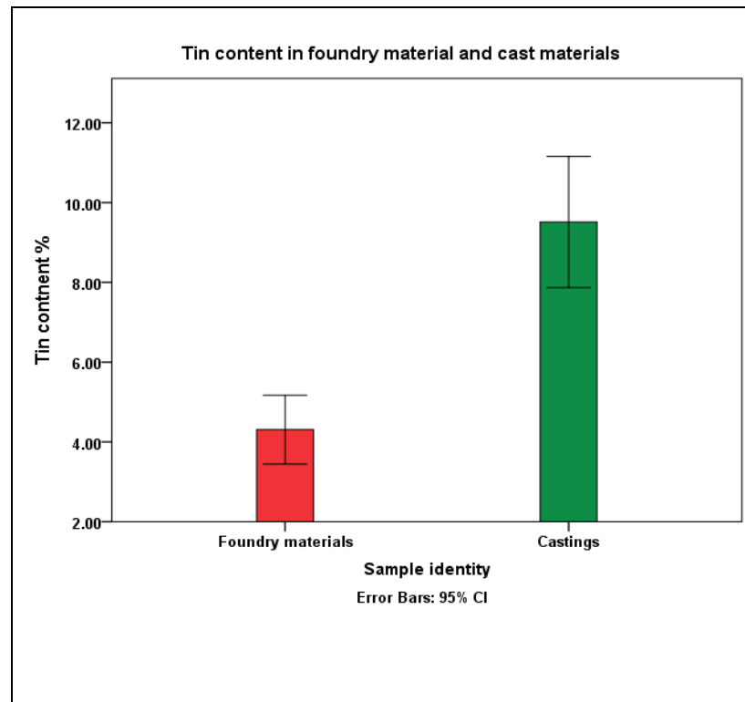
Figure4.1.2b: Tin in foundry materials and castings
