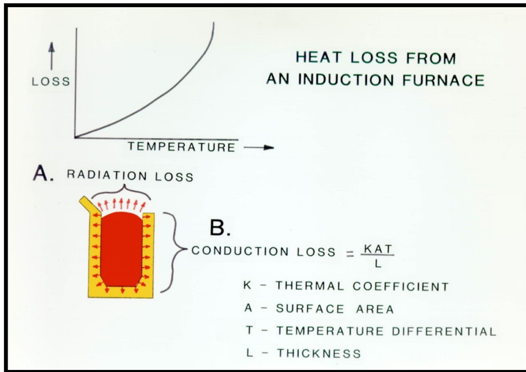
Figure 2.2.9e: Heat loss mechanism in an induction furnace (Inductotherm Corporation)
