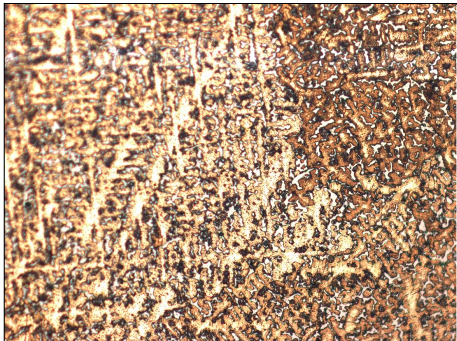
Figure 4.1.5n: Cast sample (Univ. of Joburg WBI, 200X)
