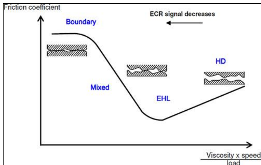
Figure 2.1.7a: Stribeck curve for lubricated sliding surfaces (CDA, 1997)
