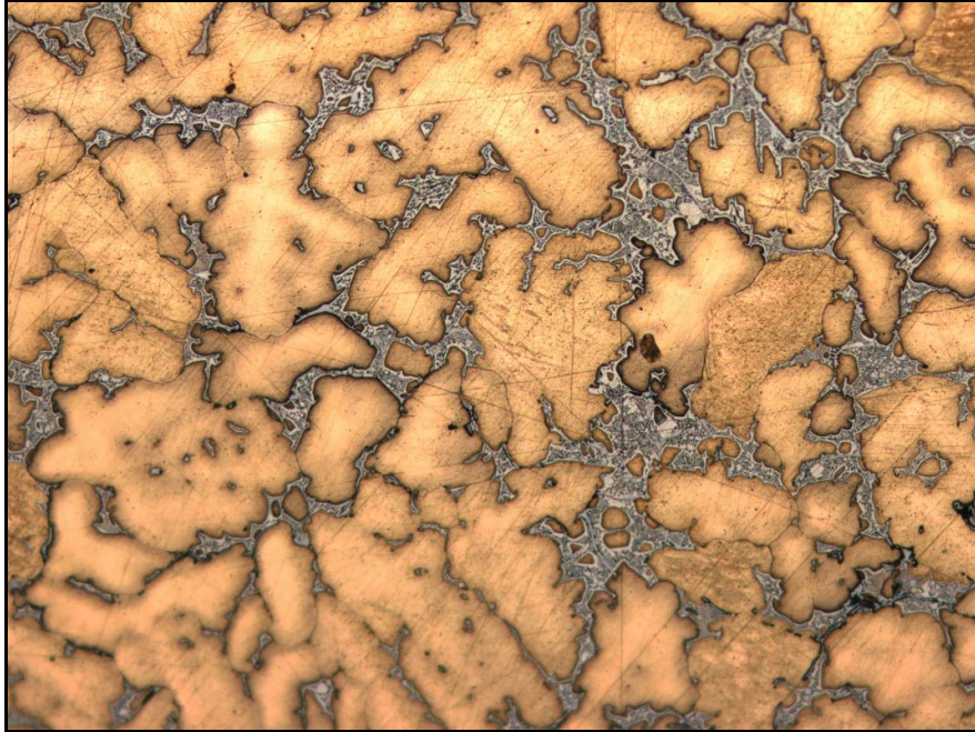
Figure 4.1.5g: Used bearing, FFC (Fox Foundry scrap FFC, 100X)
