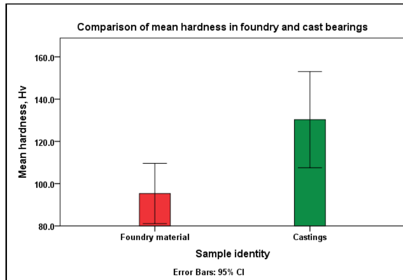
Figure4.1.3a: Hardness in foundry materials and castings
