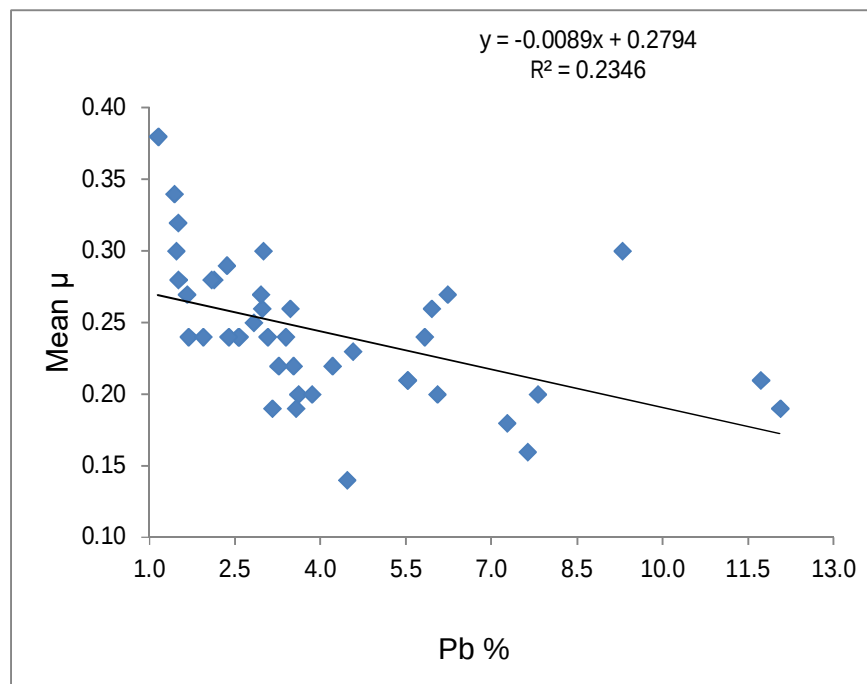
Figure4.1.4l: Impact of lead content on friction for cast samples
