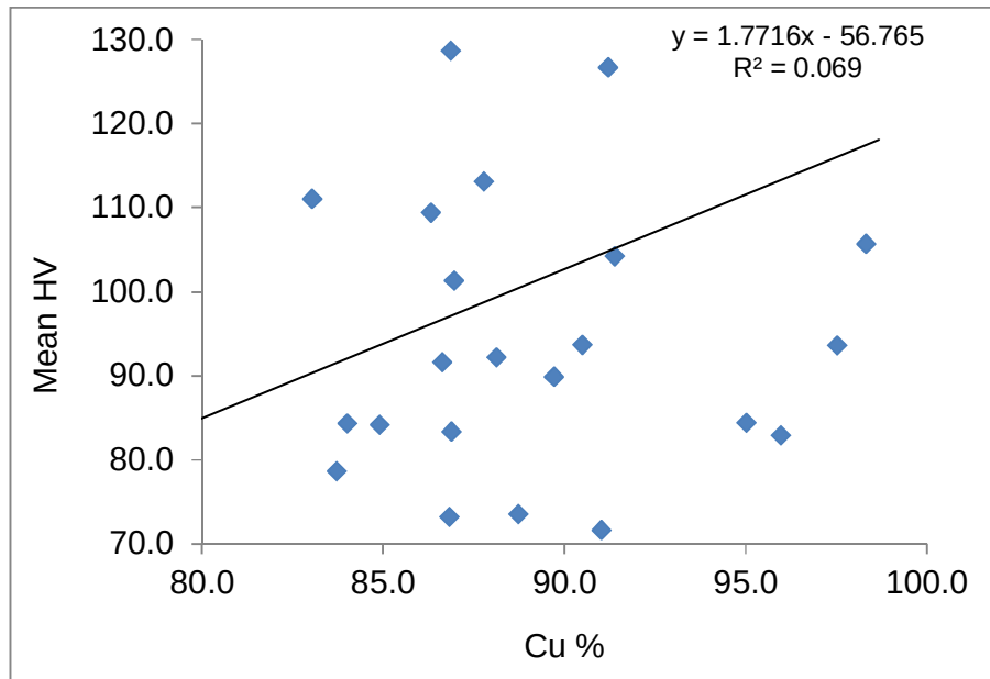
Figure4.1.4a: Impact of copper content on hardness for standard samples
